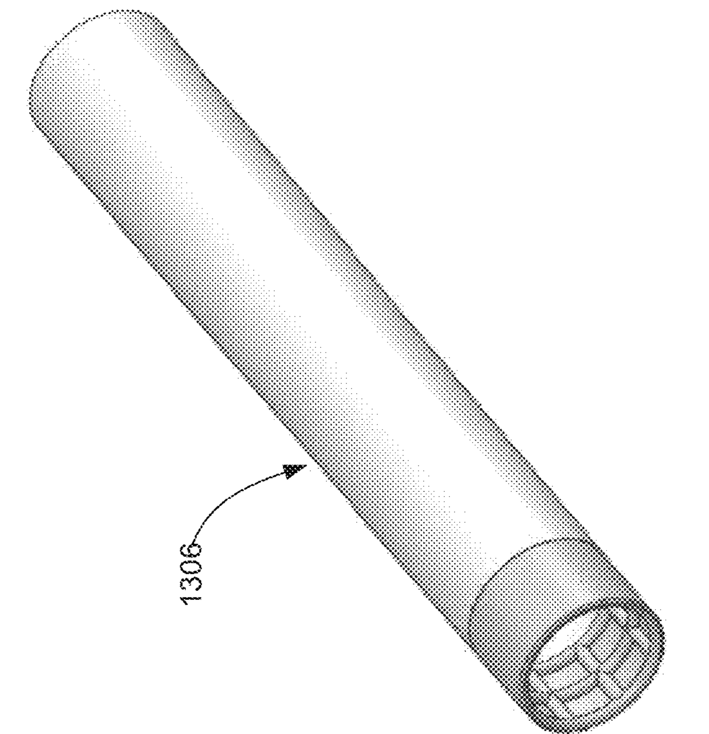
POST DIP WITH MANDREL FEATURE TRANSFERRED
