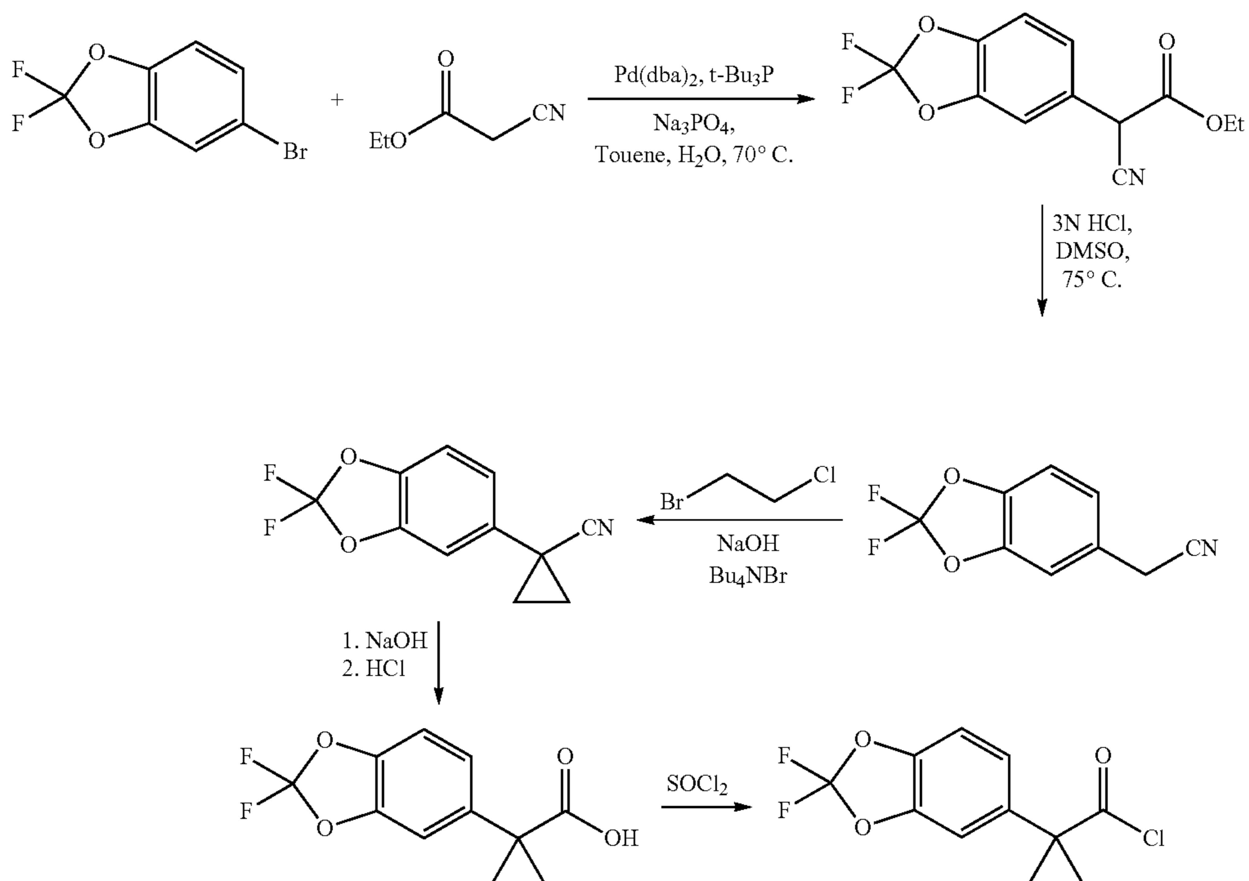
Scheme IV-B. Alternative synthesis of the acid chloride moiety.
