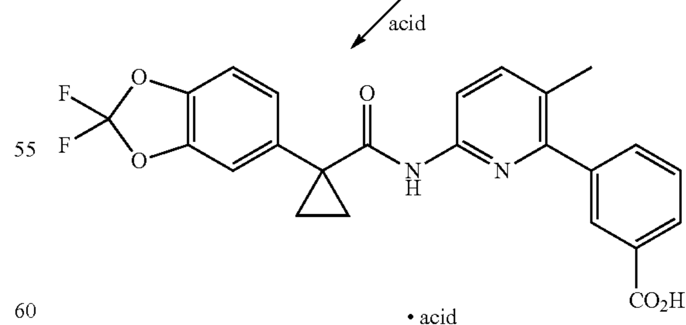
Scheme IV-D. Formation of an acid salt of 3-(6-(1-(2,2-difluorobenzo[d][1,3]dioxol-5-yl)cyclopropanecarboxamido)-3-methylpyridin-2-yl)benzoic acid.
