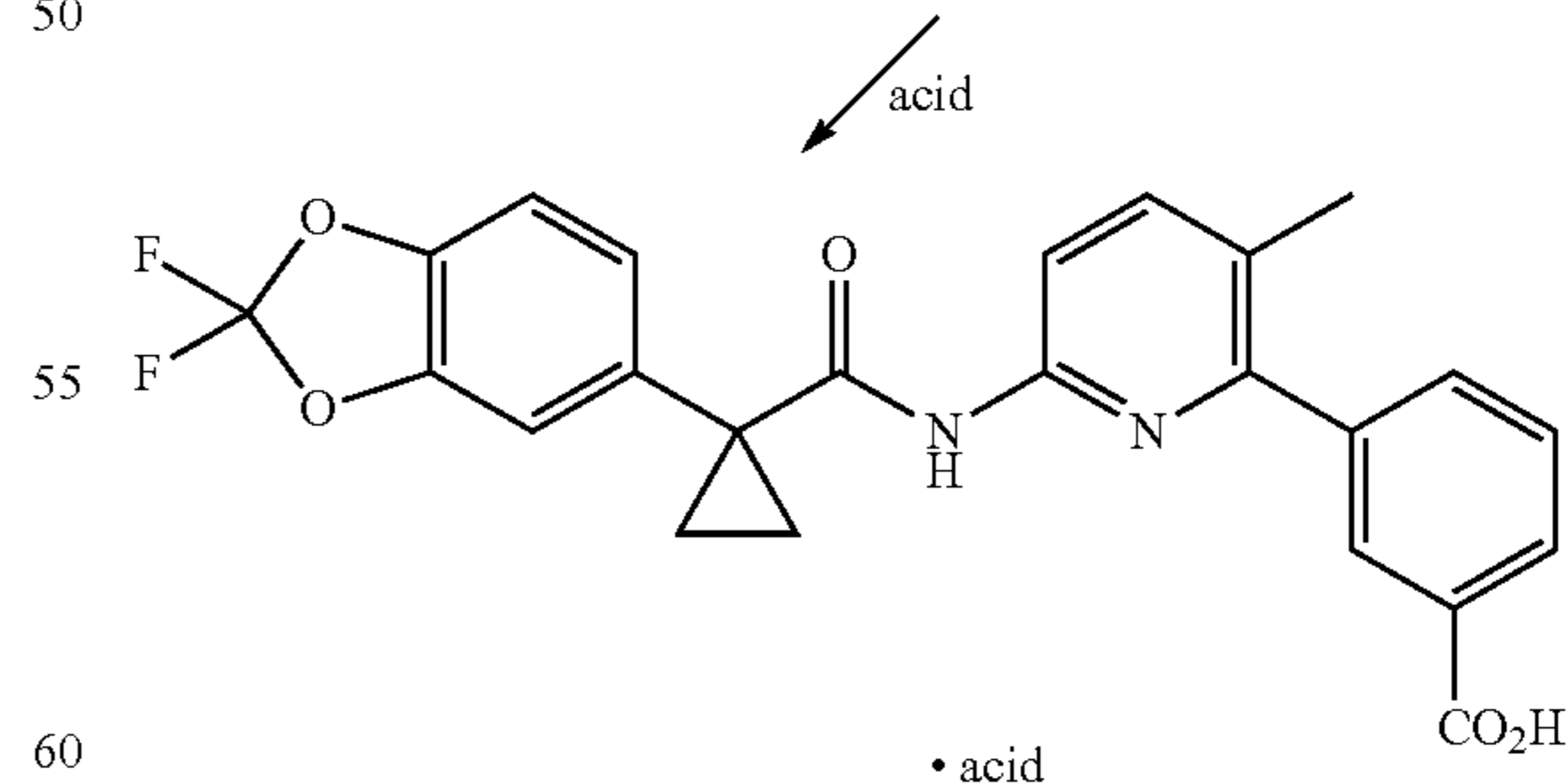
Scheme IV-D. Formation of an acid salt of 3-(6-(1-(2,2-difluorobenzo[d][1,3]dioxol-5-yl)cyclopropanecarboxamido)-3-methylpyridin-2-yl)benzoic acid.
