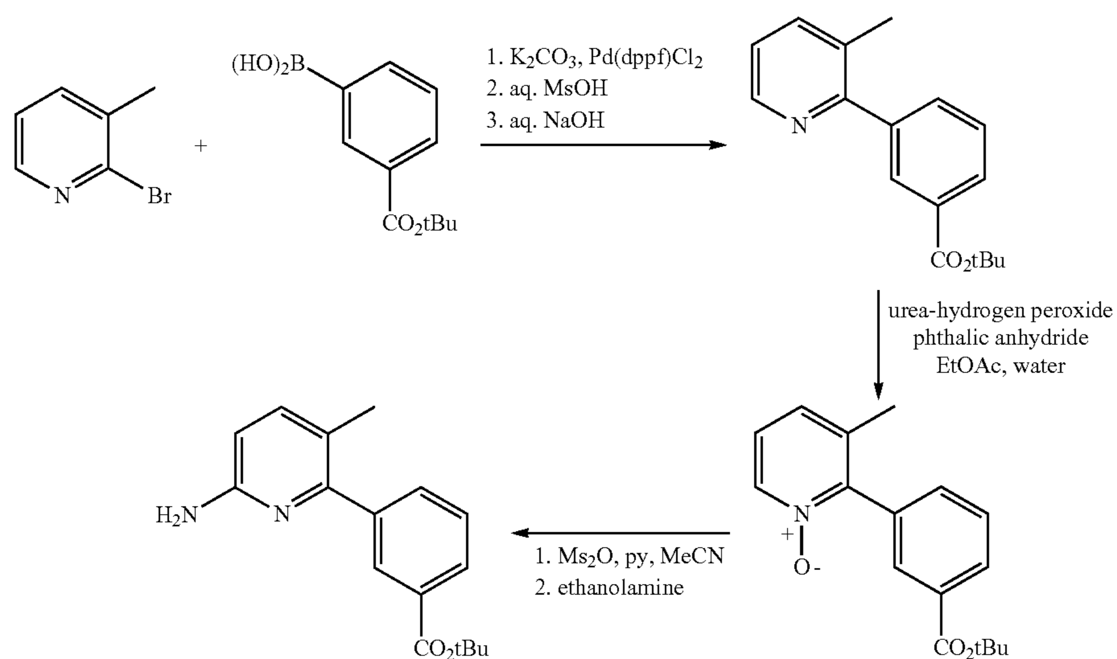
Scheme IV-C. Synthesis of the amine moiety.
