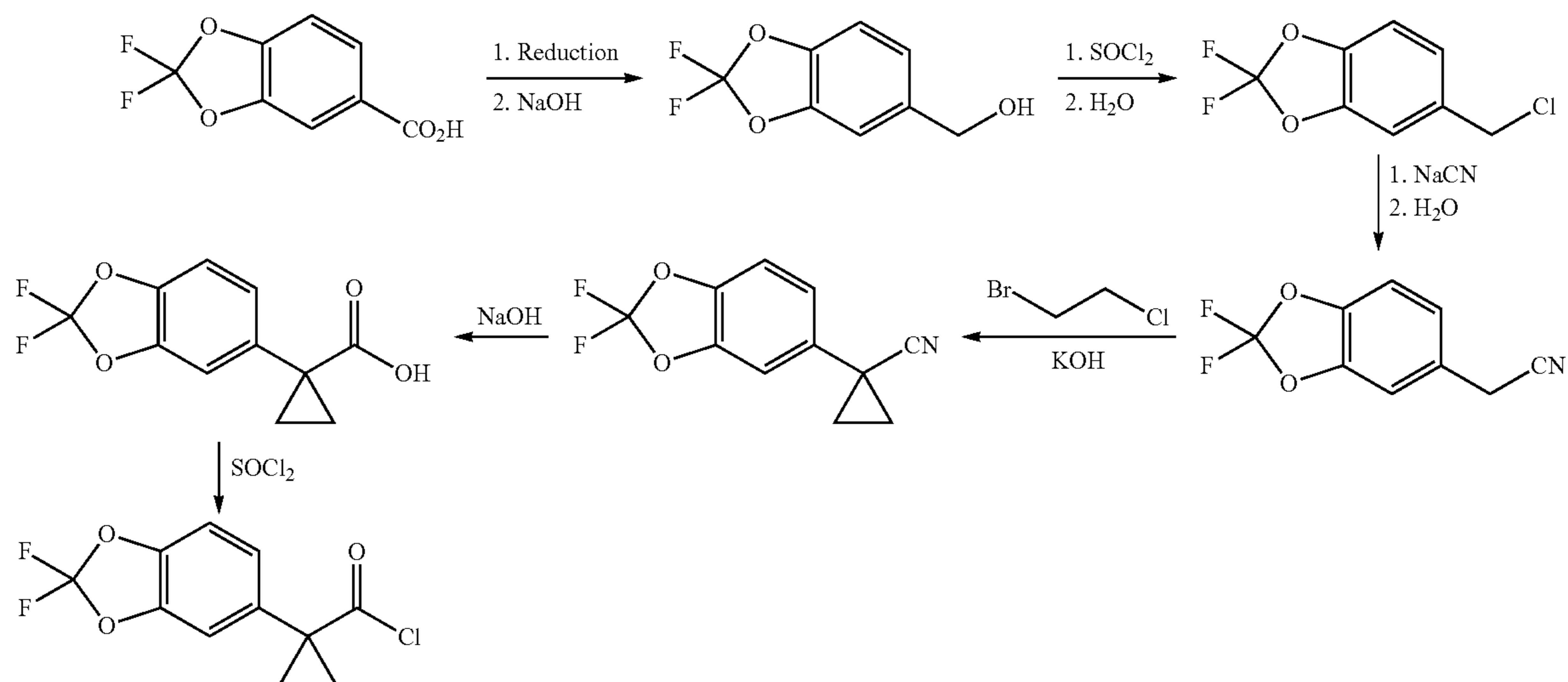
Scheme IV-A. Synthesis of the acid chloride moiety.
