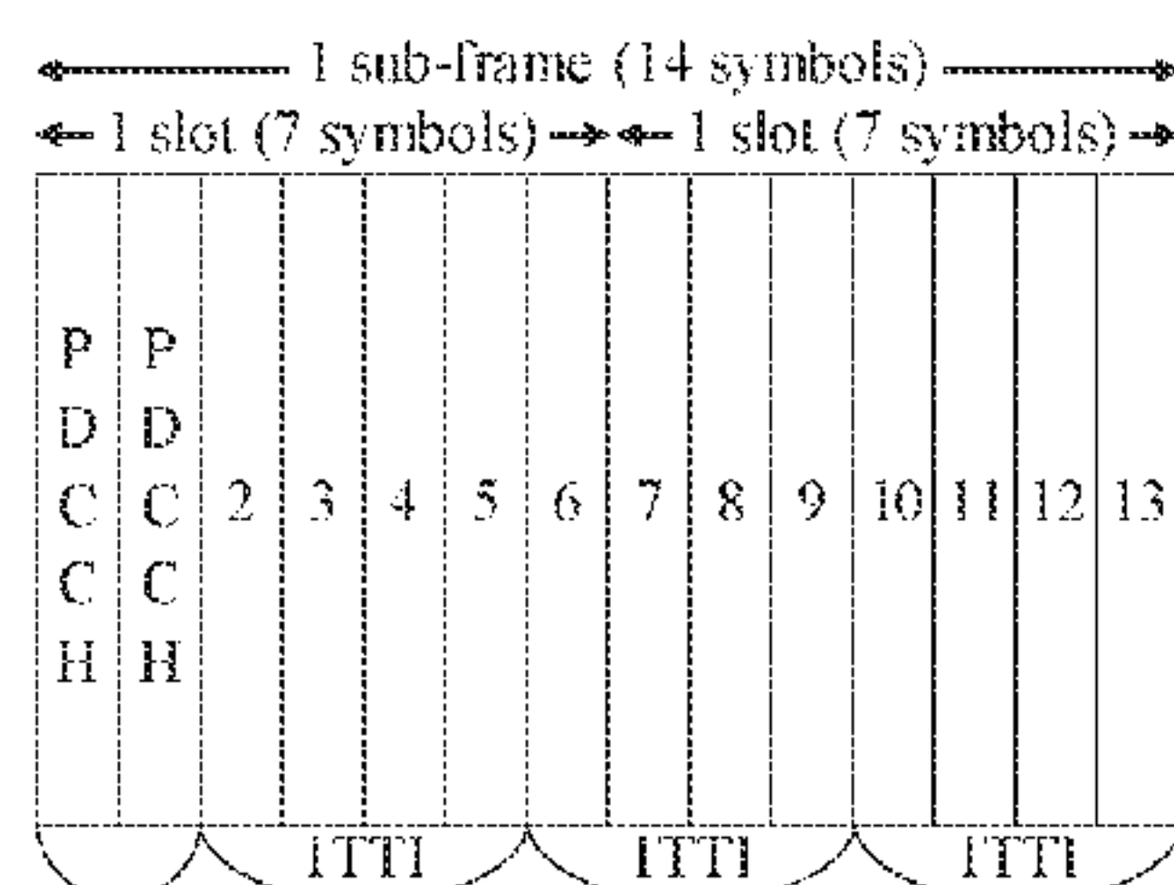
(c) 4 symbol TTI DL structure
