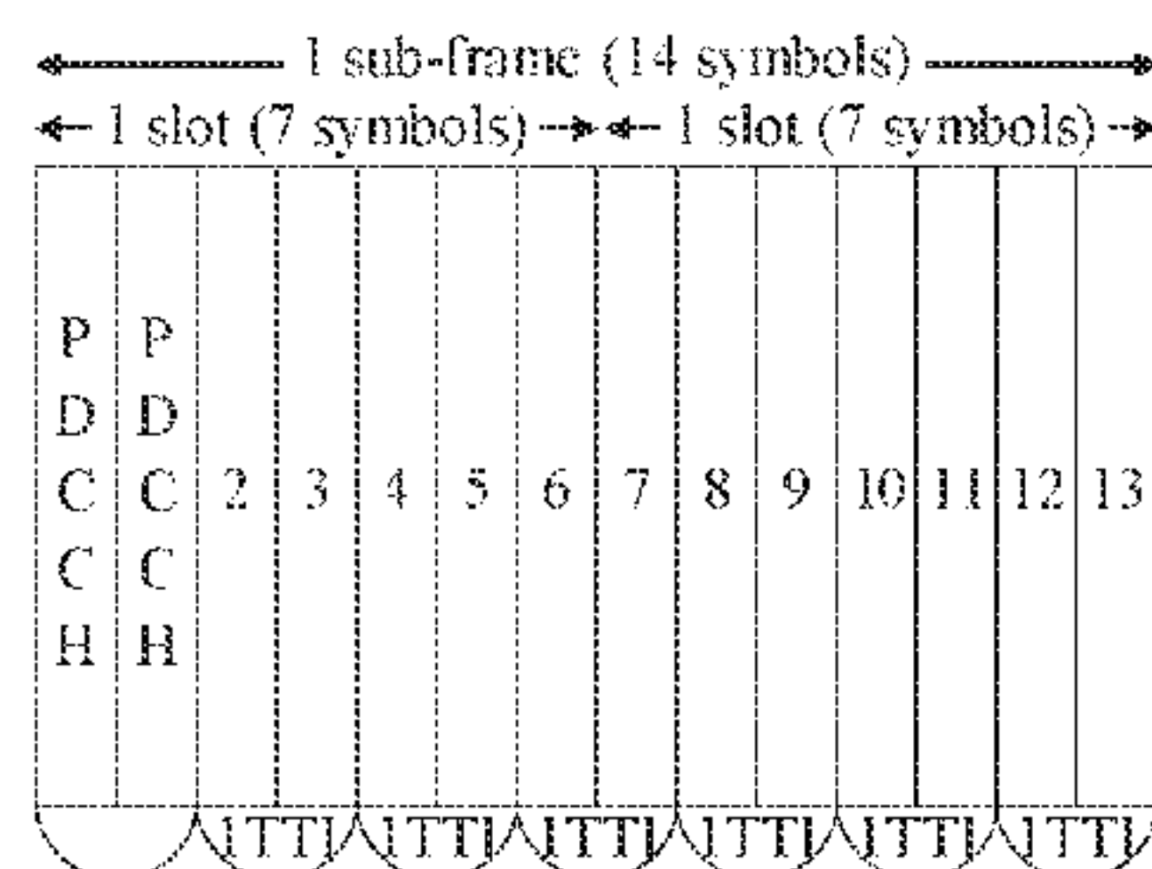
(a) 2 symbol TTI DL structure
