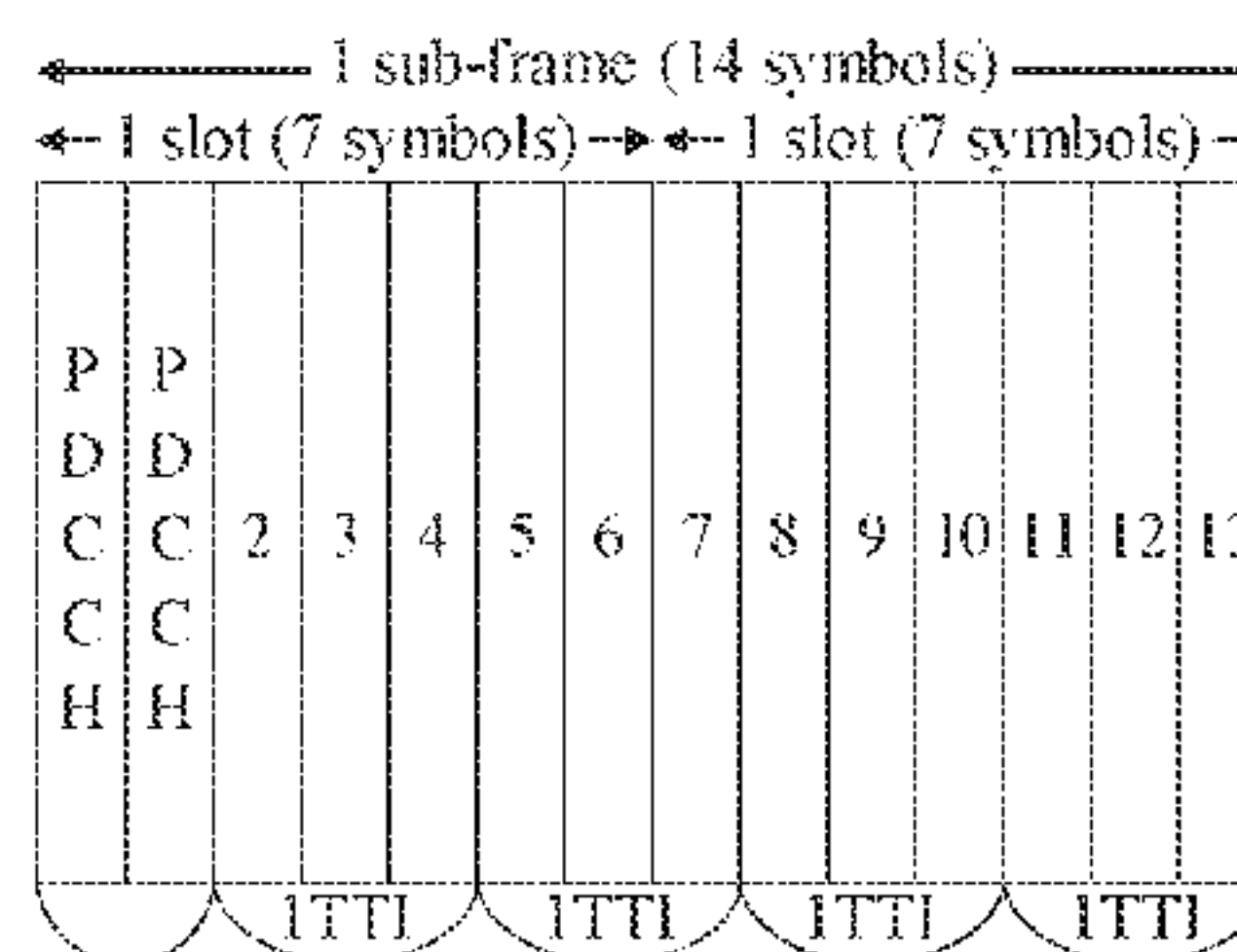
(b) 3 symbol TTI DL structure
