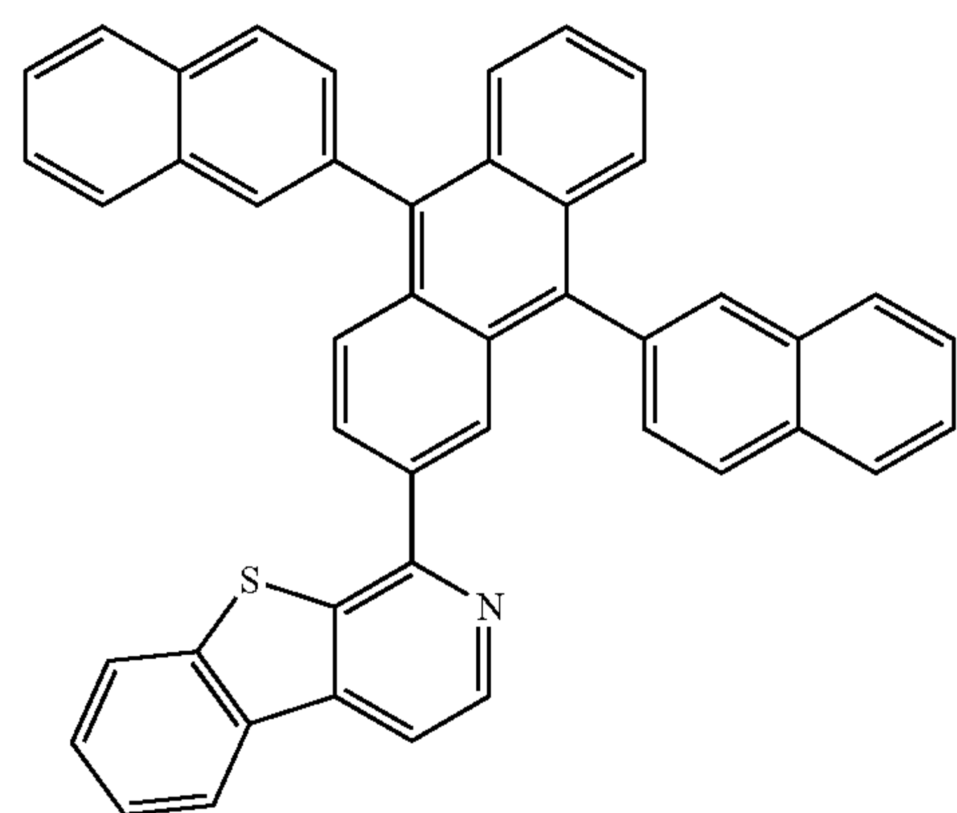
aDBT-ADN
