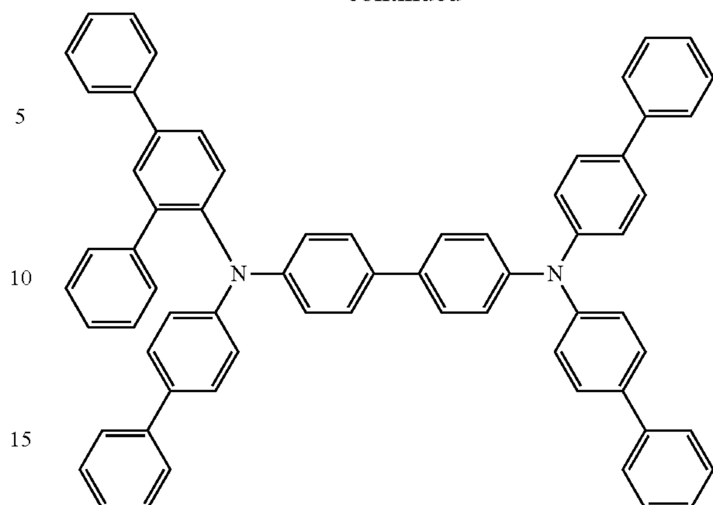
PPh-TPD
