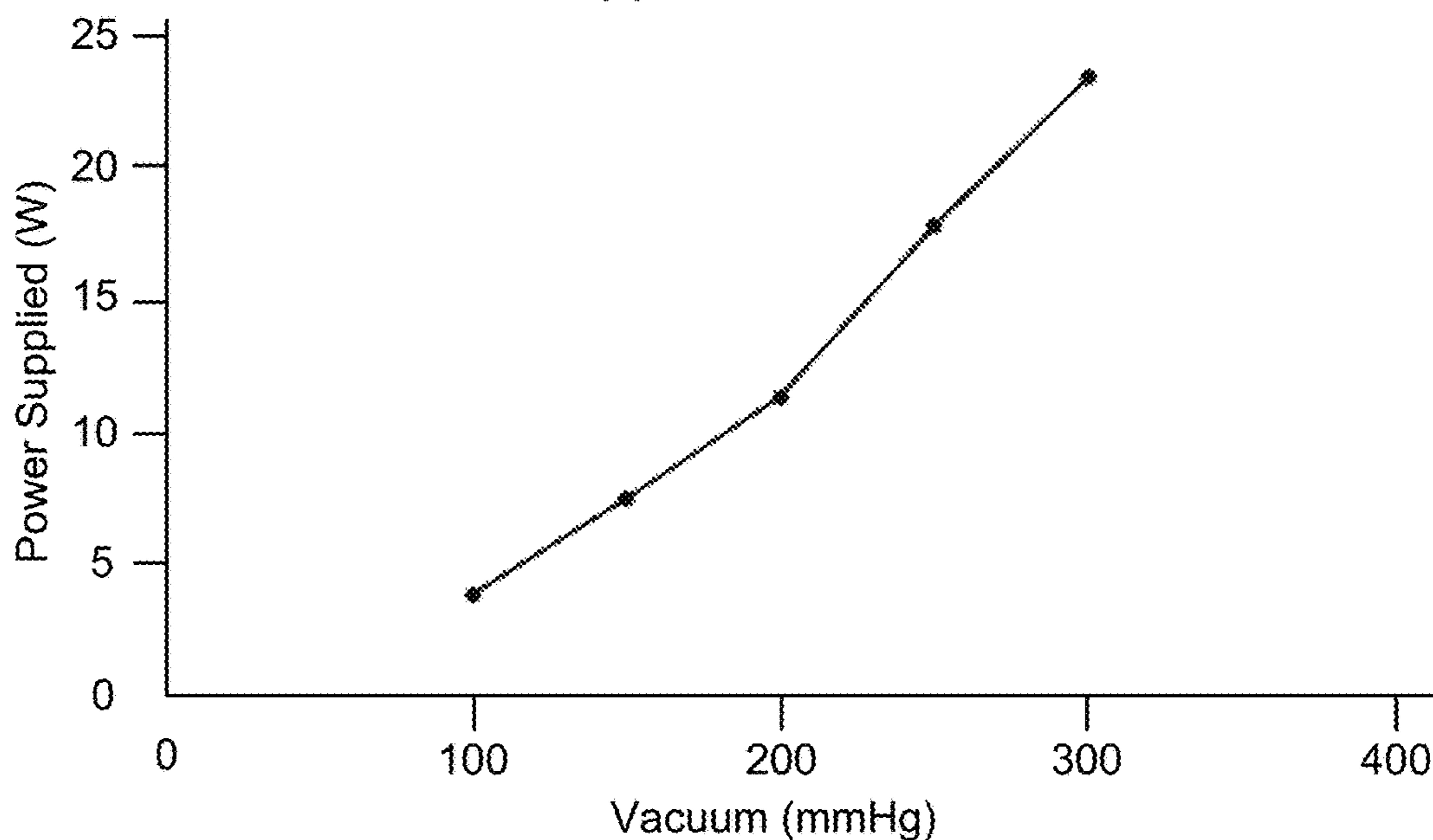
Power Supplied vs. Vacuum
