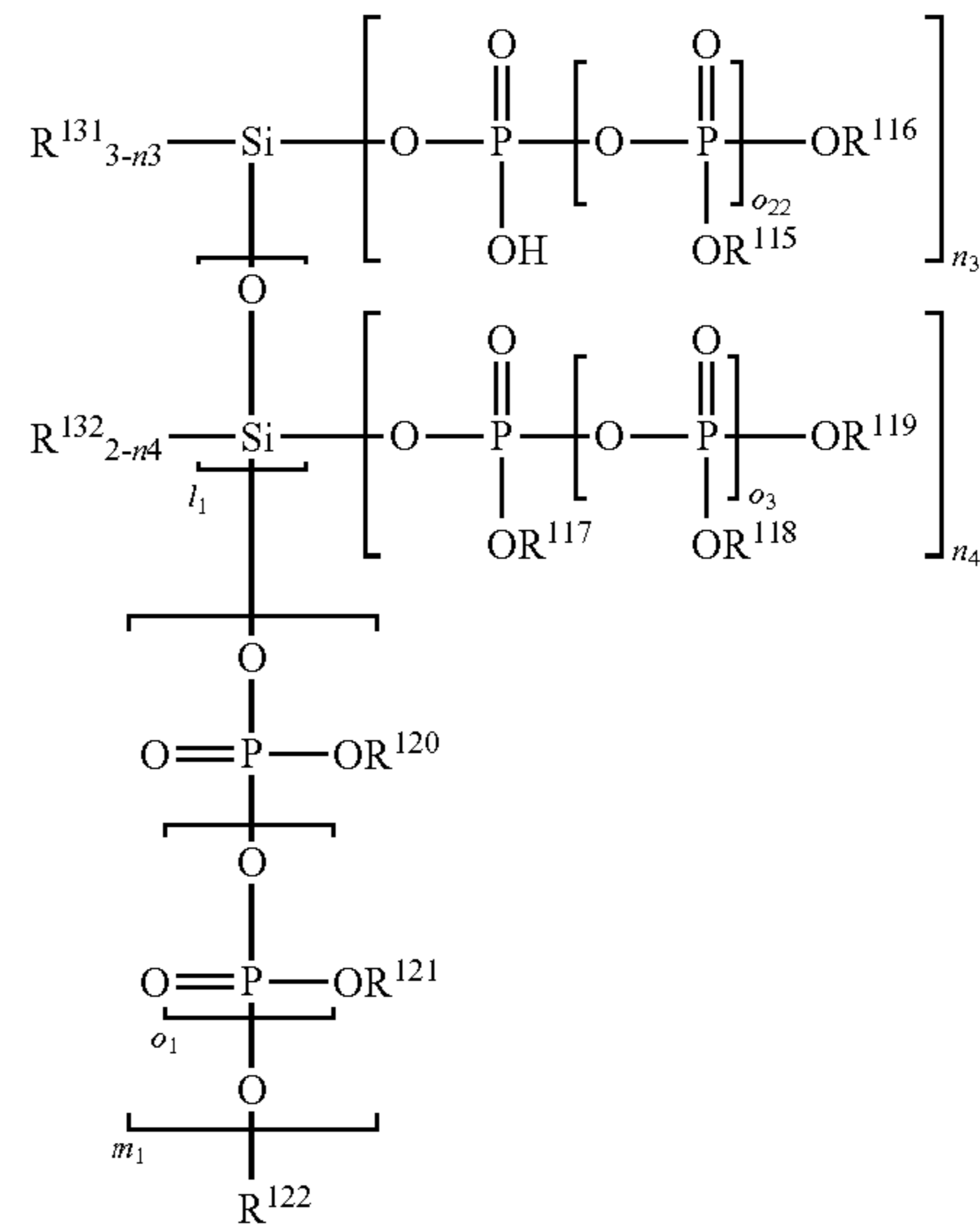
[Chemical Formula C220-1]
