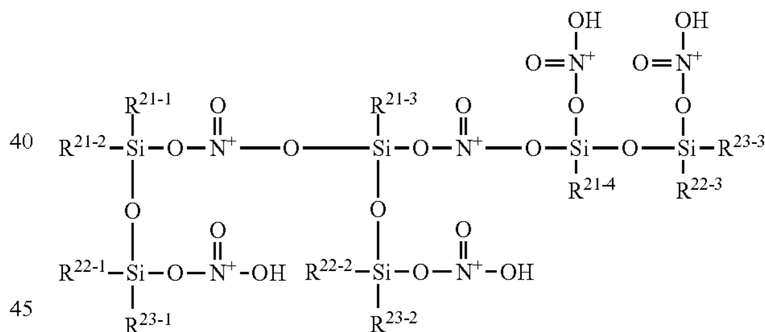
[Chemical Formula 269]
