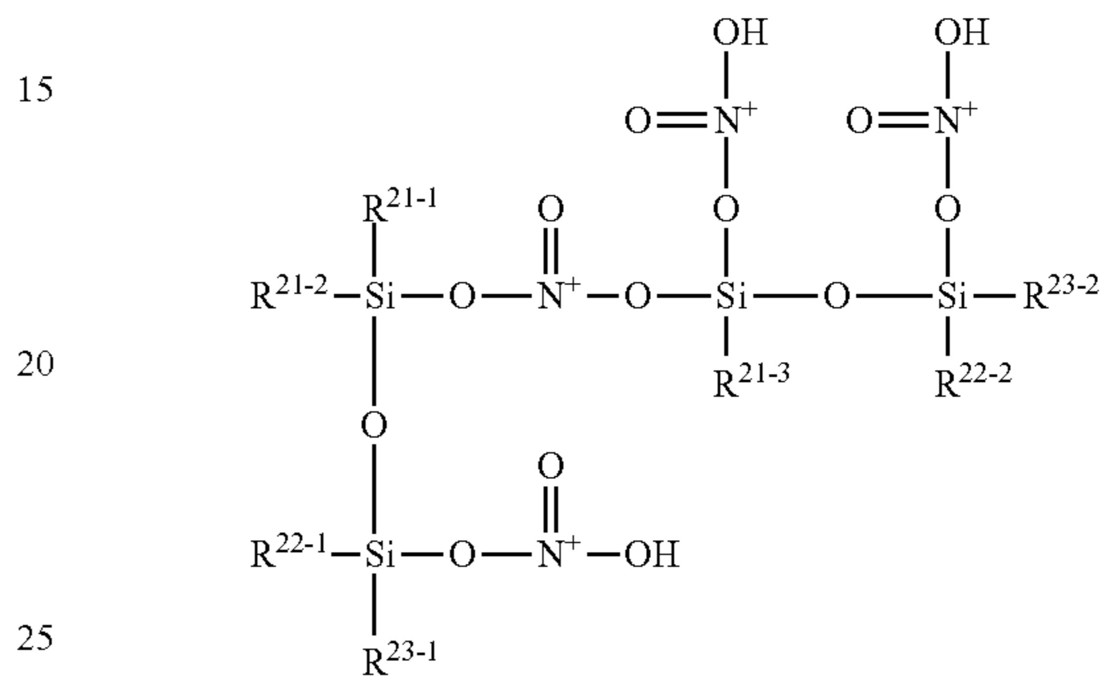
[Chemical Formula 268]
