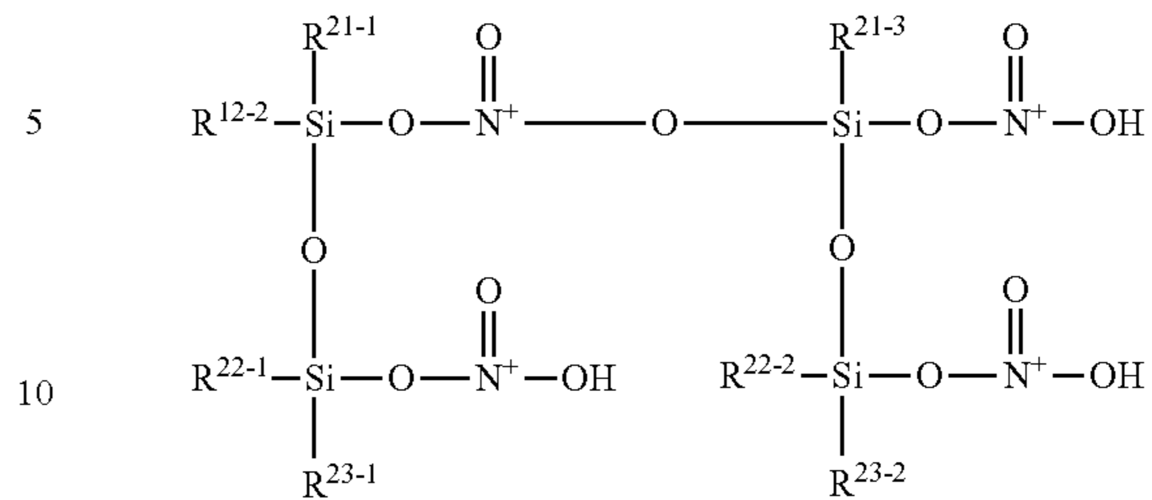
[Chemical Formula 267]
