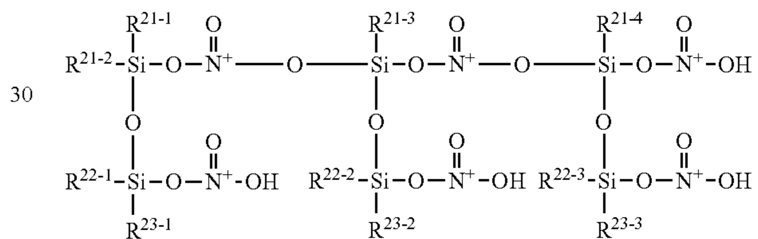
[Chemical Formula 269]
