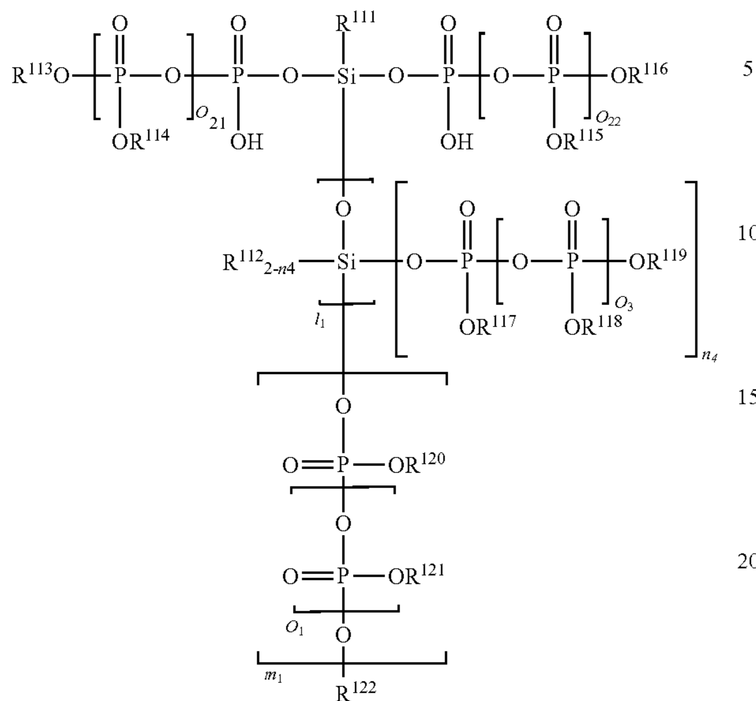
[Chemical Formula C200-1]
