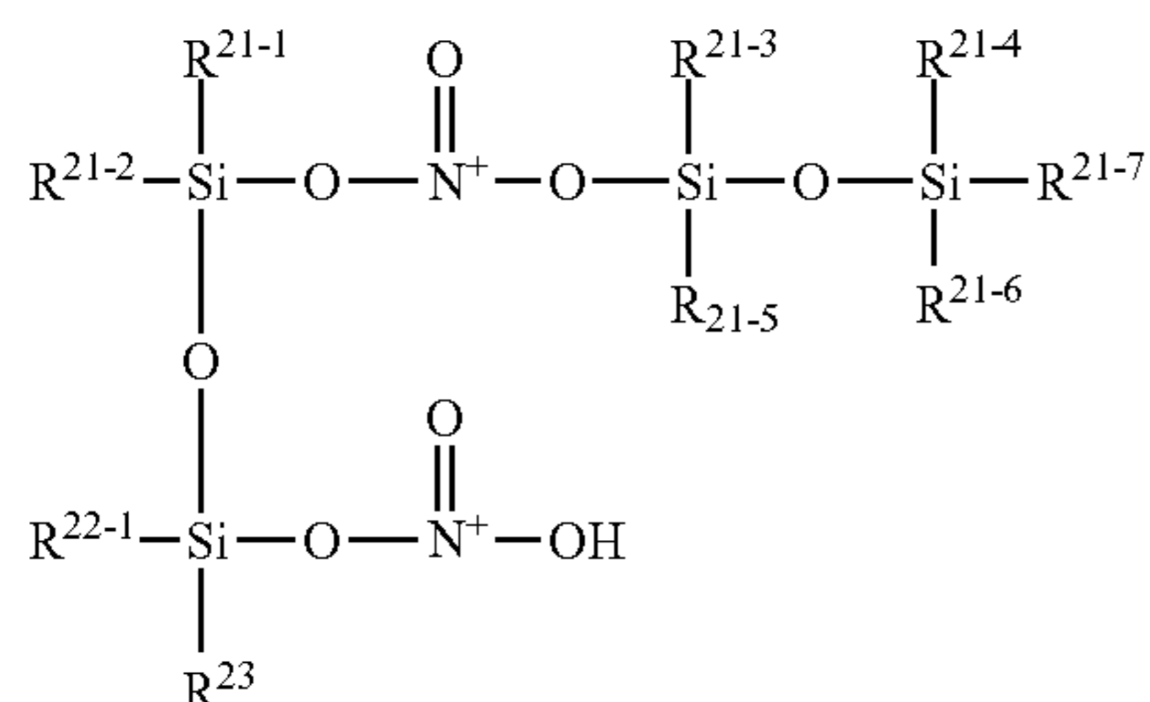
[Chemical Formula 265]
