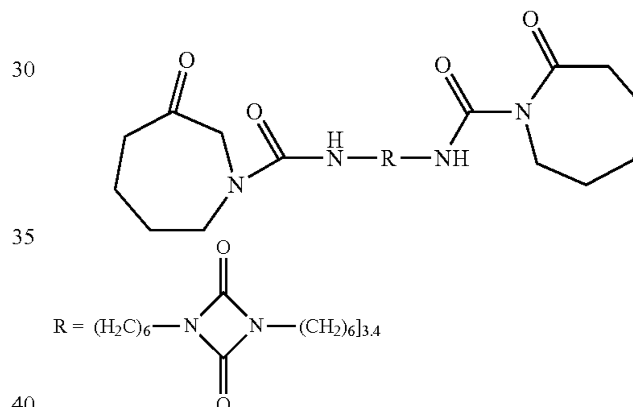
The Chemical Structure of Desmodur BL 3272, a Polyisocyanate that has \epsilon -Caprolactam Protecting Groups
