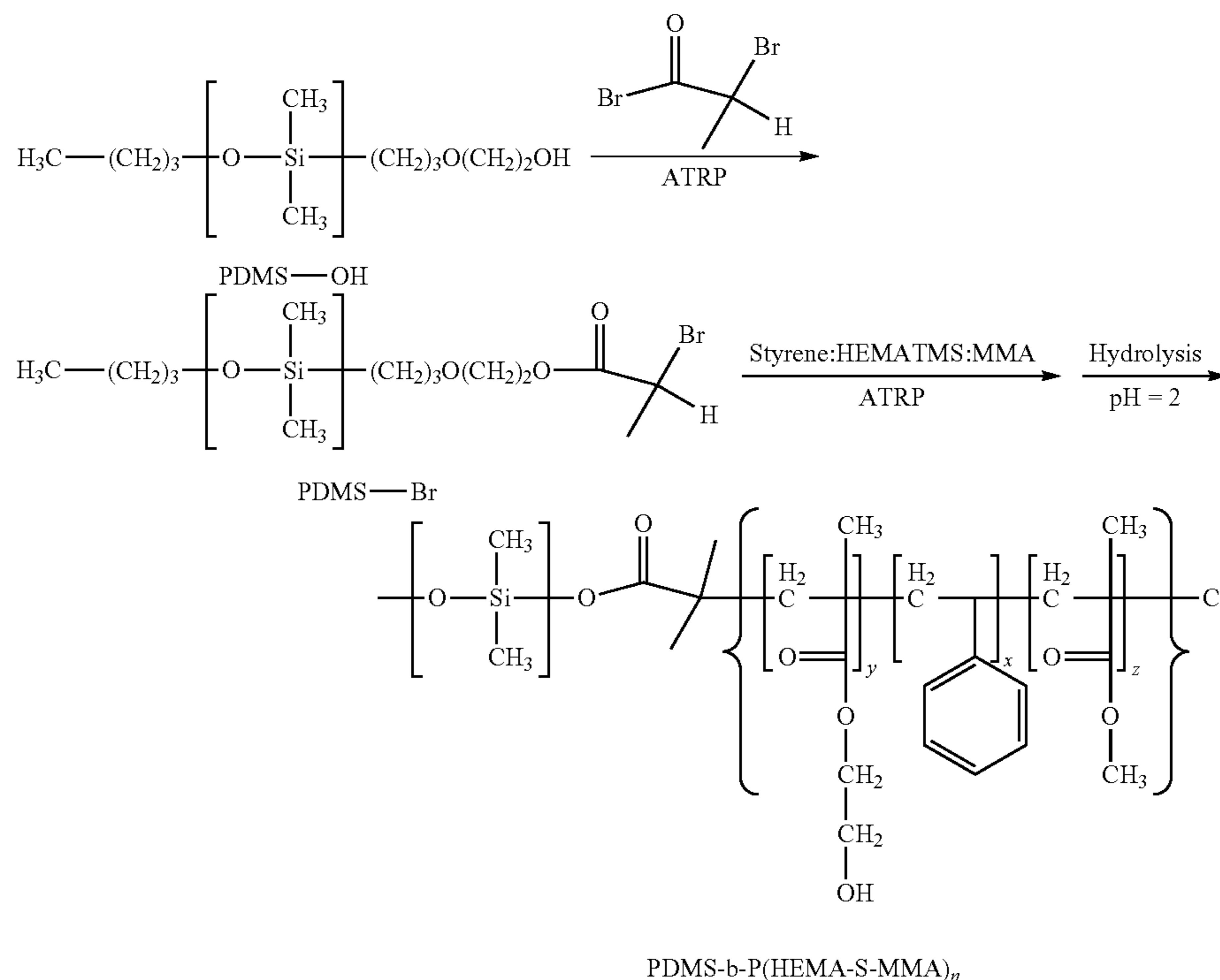
Scheme 6. Synthetic pathway toward PDMS-b-(HEMA-S-MMA) n .
