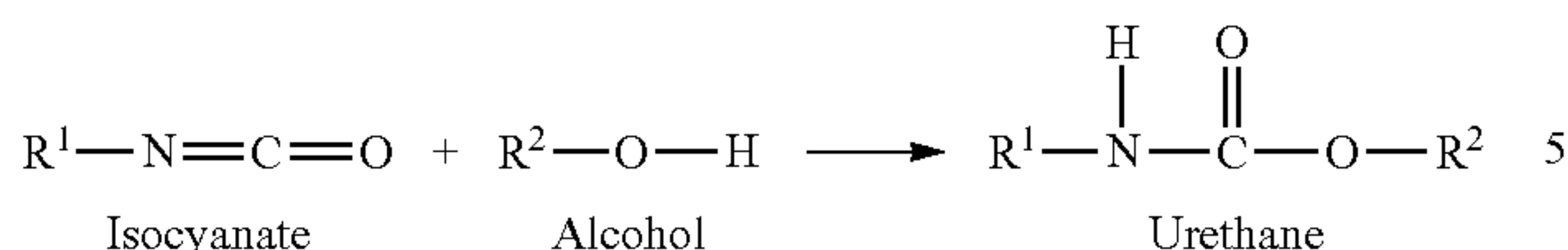
Scheme 7. Chemical reaction involved in the synthesis of polyurethane.
