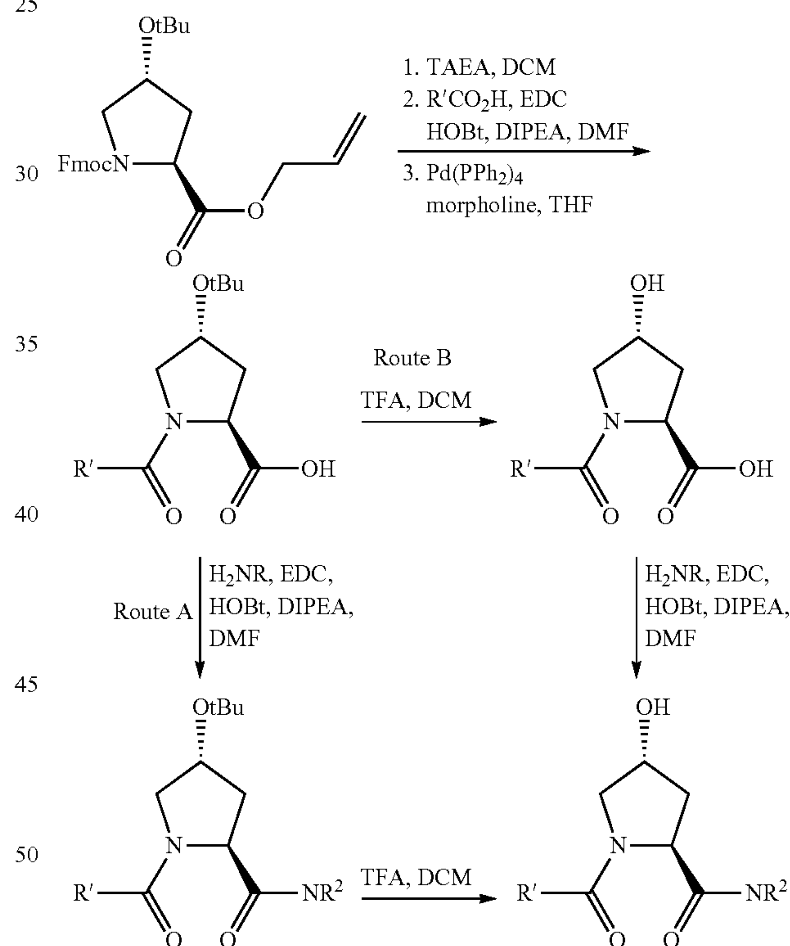
Scheme 1 Solution Phase Synthesis of ULM Derivatives According to the Present Invention
