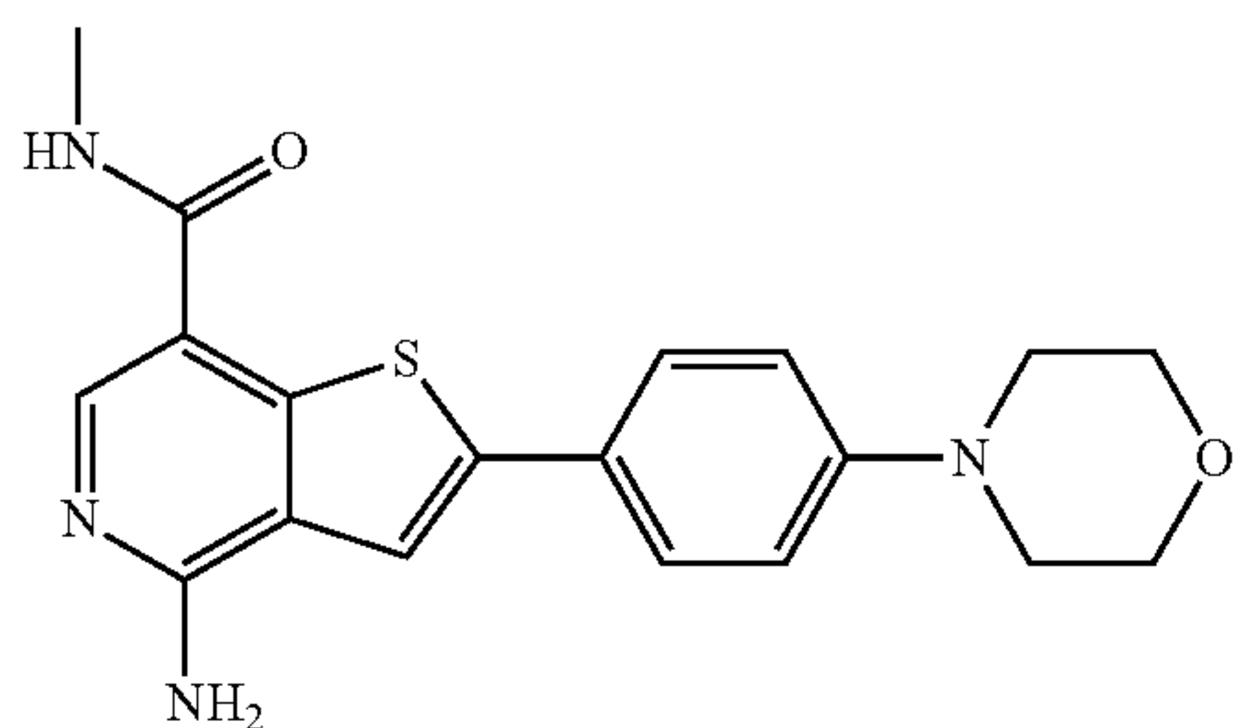
07P 4-amino-N-methyl-2-[4-(morpholin-4-yl)phenyl]thieno[3,2-c]pyridine-7-carboxamide Thienopyridine 8
