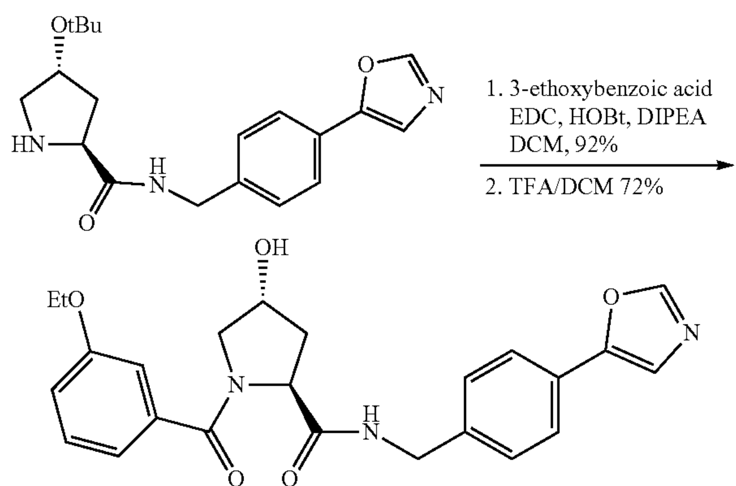
Synthesis of VL217
