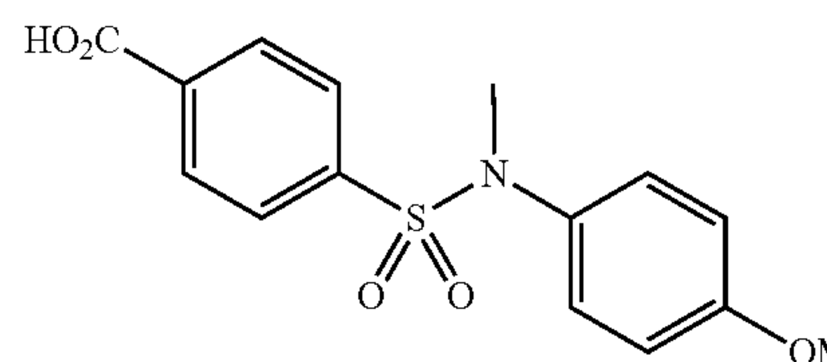
4-(N-(4-methoxyphenyl)-N-methylsulfonyl)benzoic acid
