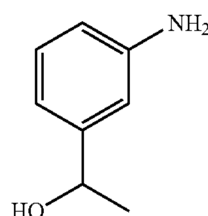
1-(3-aminophenyl)ethanol
