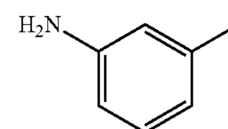
m-toluidine
