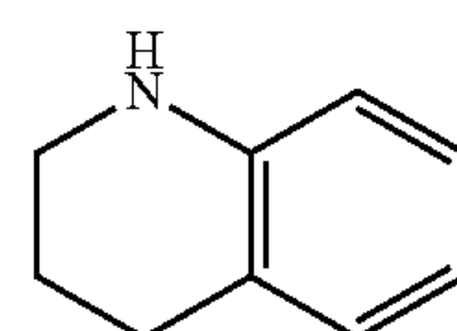
1,2,3,4-tetrahydroquinoline
