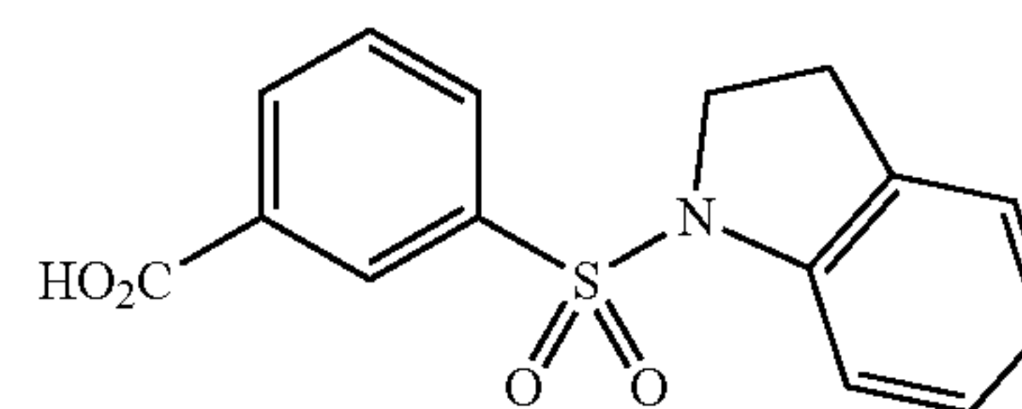
3-(indolin-1-ylsulfonyl)benzoic acid
