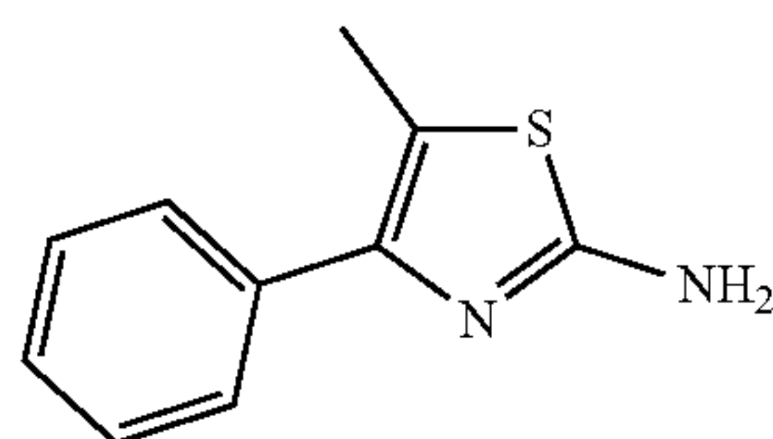
5-methyl-4-phenylthiazol-2-amine
