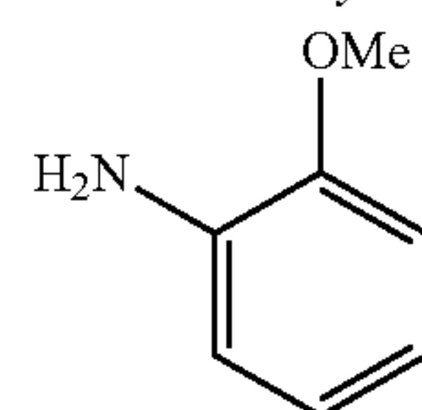
2-methoxyaniline
