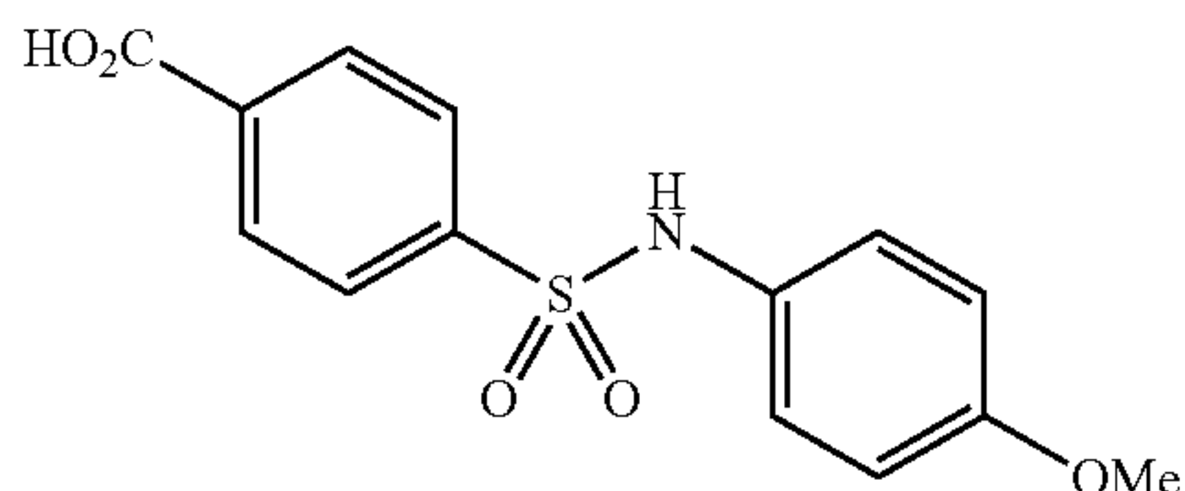
4-(N-(4-methoxyphenyl)sulfamoyl)benzoic acid
