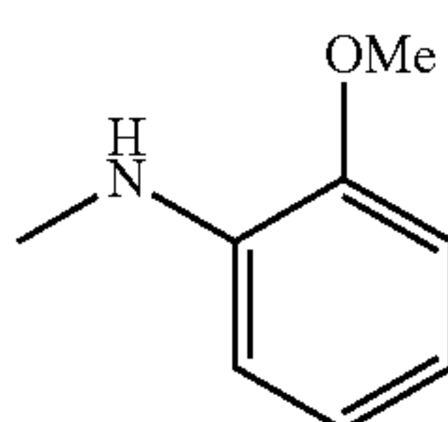
2-methoxy-N-methylaniline
