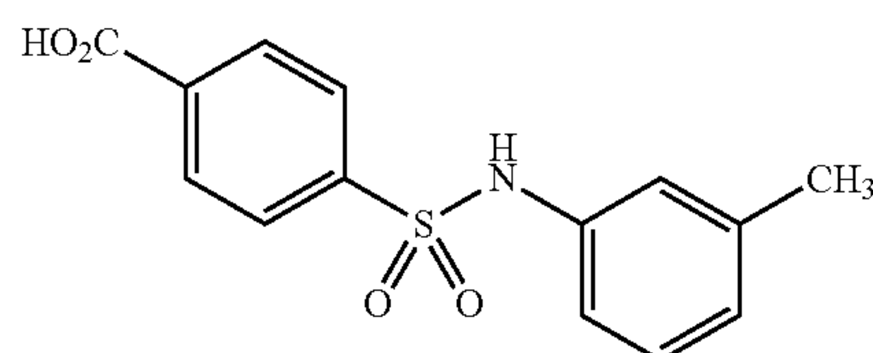
4-(N-m-tolylsulfamoyl)benzoic acid
