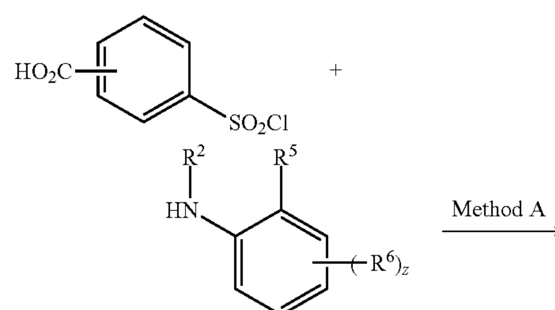
Scheme 1
