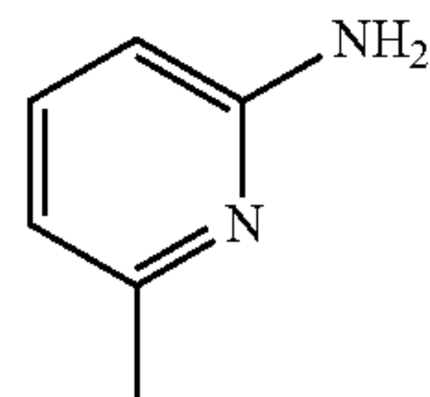
6-methylpyridin-2-amine
