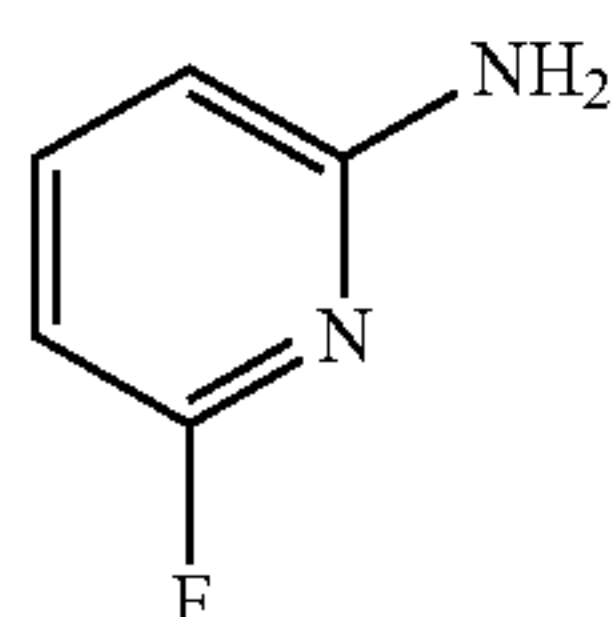
6-fluoropyridin-2-amine
