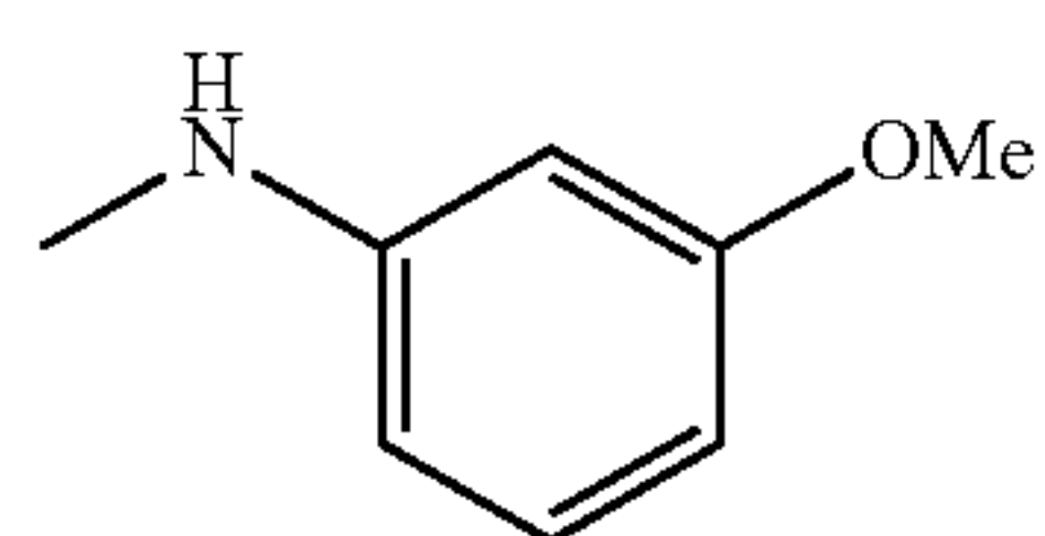
3-methoxy-N-methylaniline
