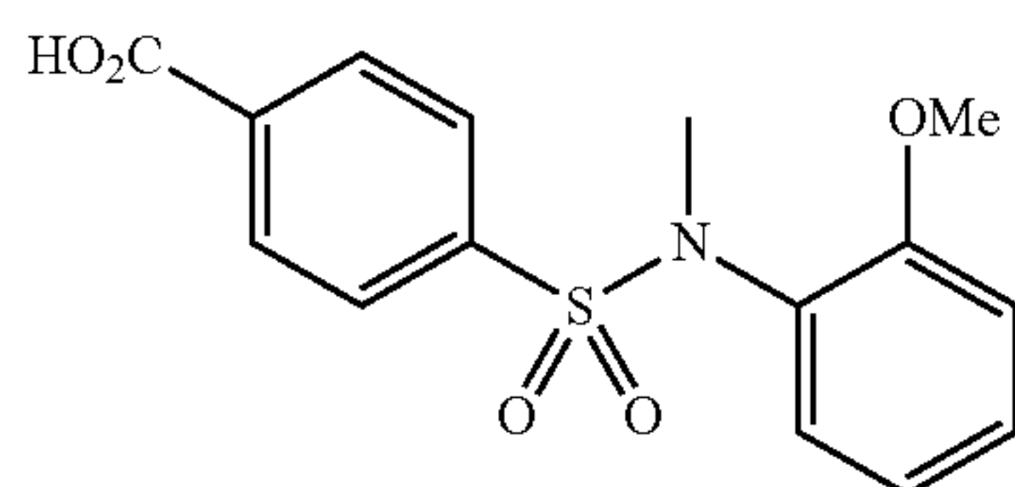
4-(N-(2-methoxyphenyl)-N-methylsulfamoyl)benzoic acid
