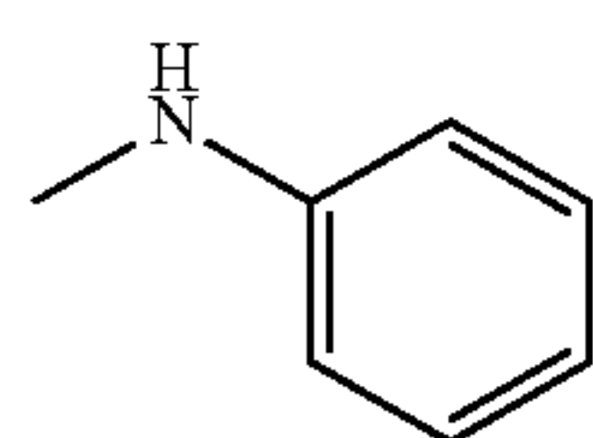
N-methylaniline
