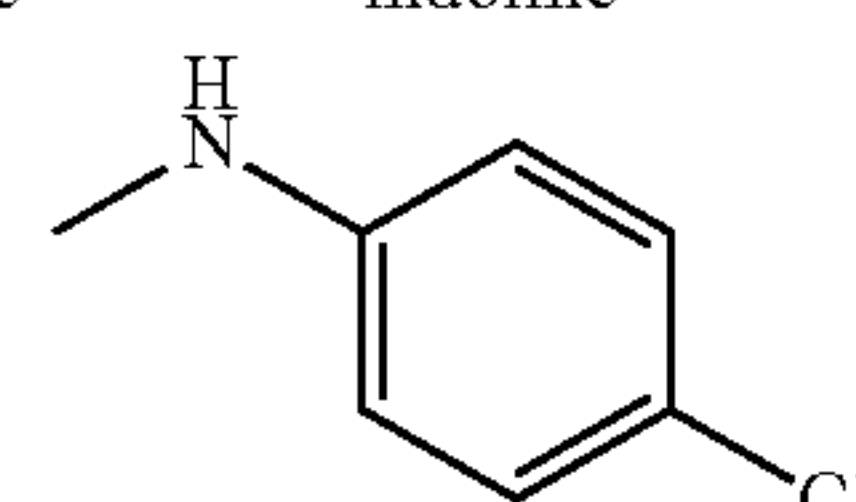
4-chloro-N-methylaniline
