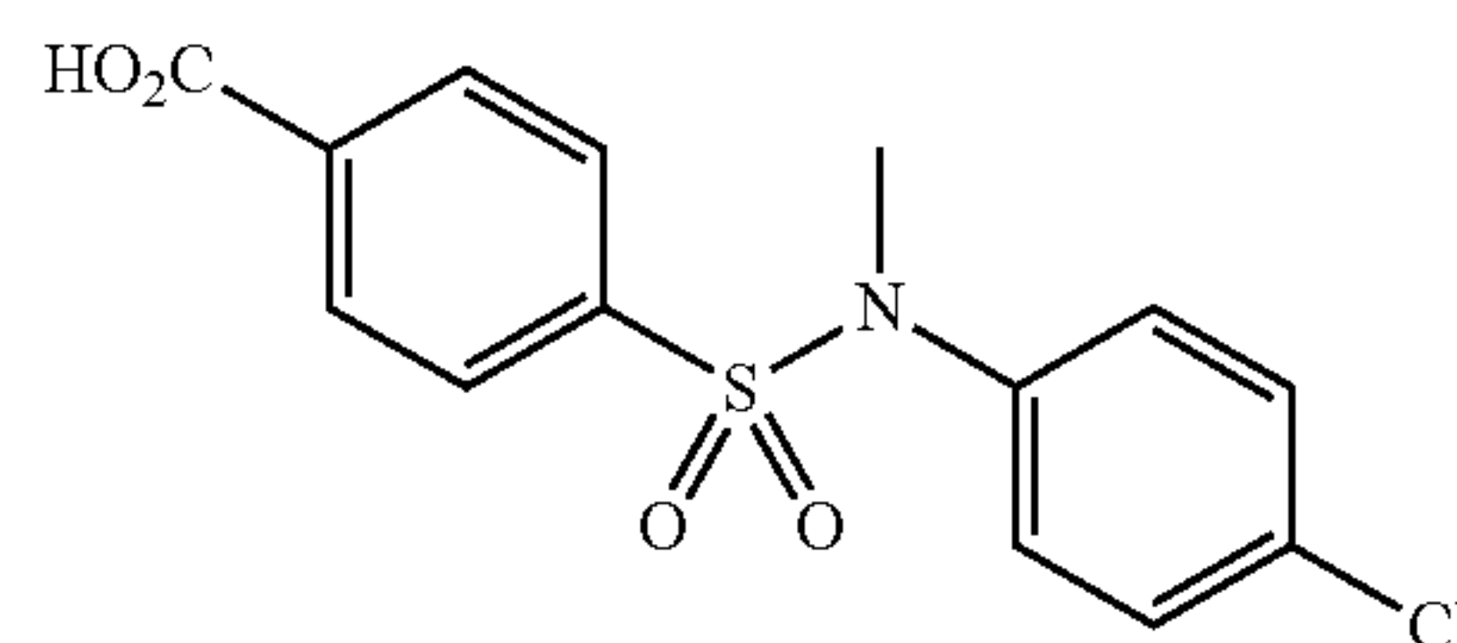
4-(N-methyl-N-(4-(trifluoromethyl)phenyl)sulfonyl)benzoic acid
