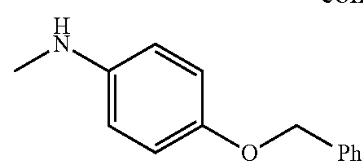
4-(benzyloxy)-N-methylaniline
