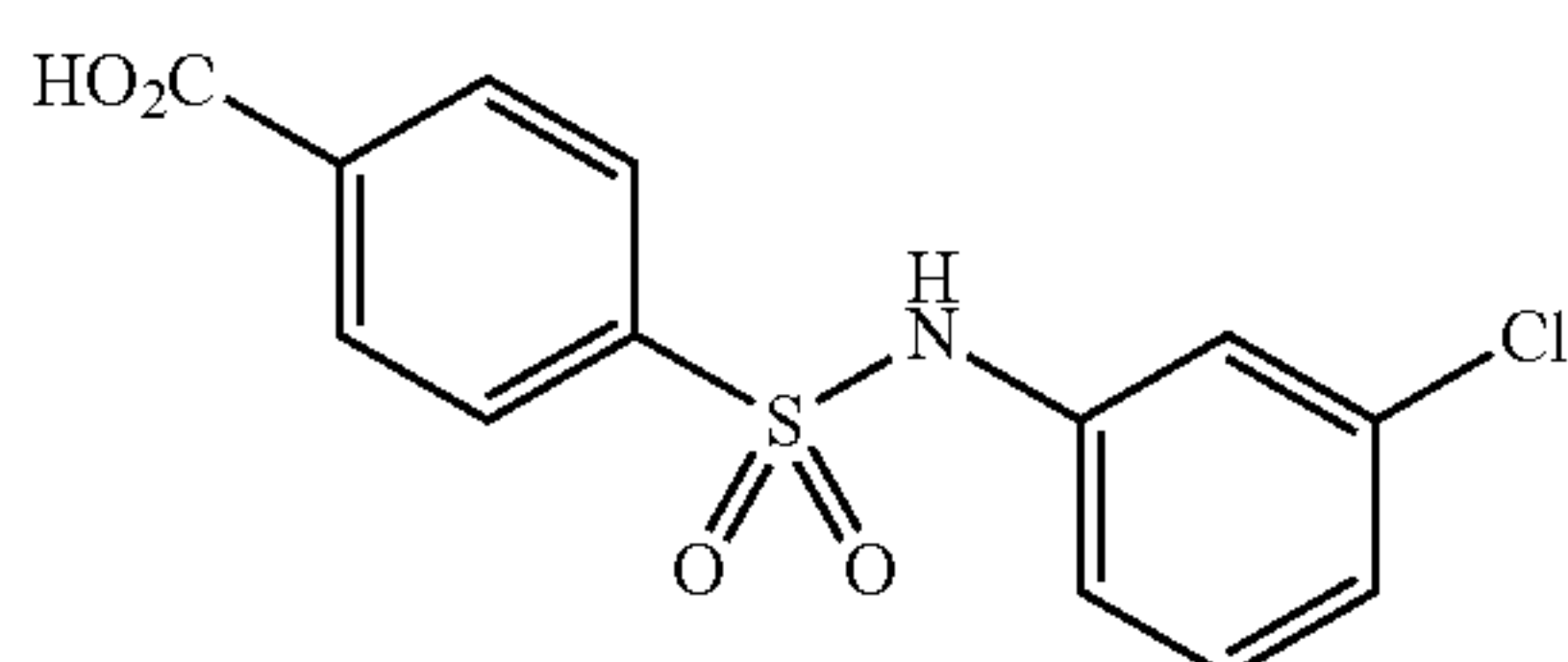
4-(N-(3-chlorophenyl)sulfamoyl)benzoic acid
