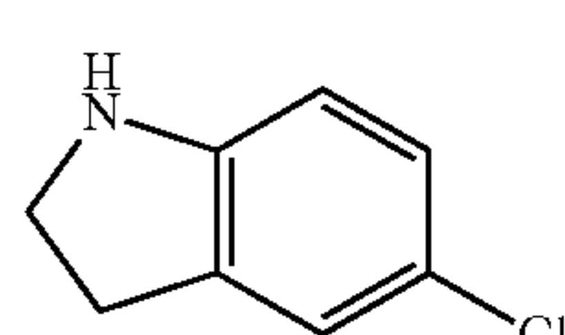
5-chloroindoline
