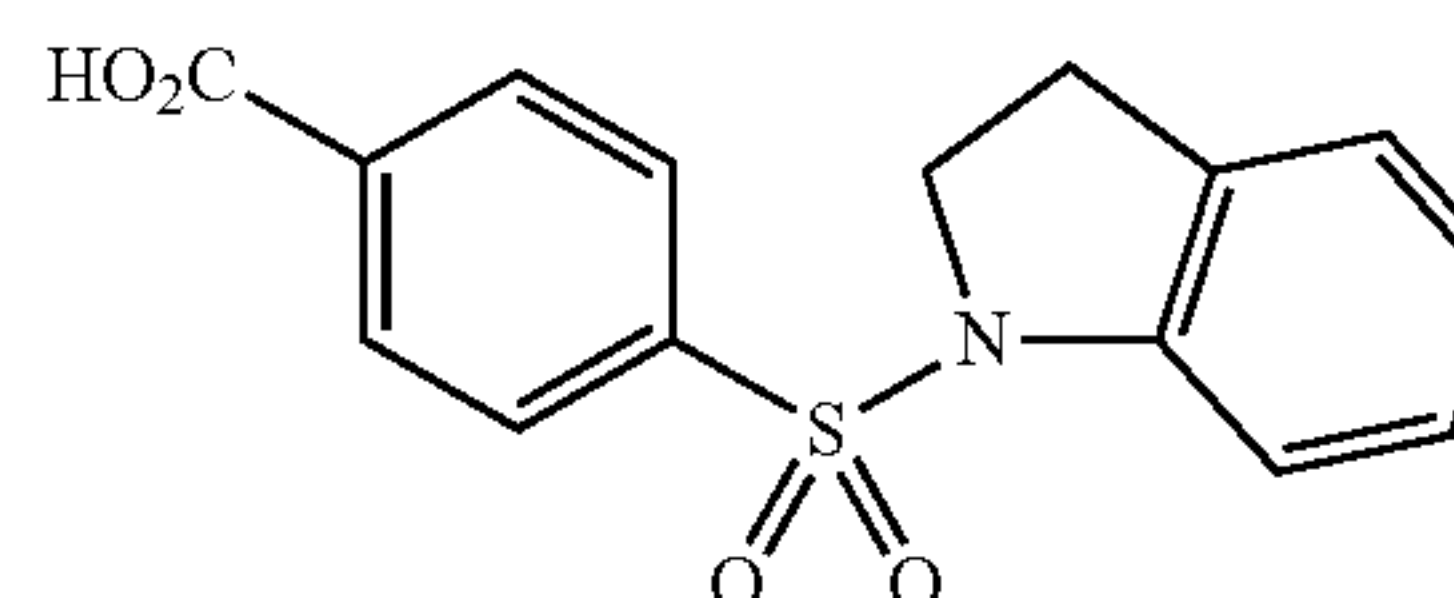
4-(indolin-1-ylsulfonyl)benzoic acid
