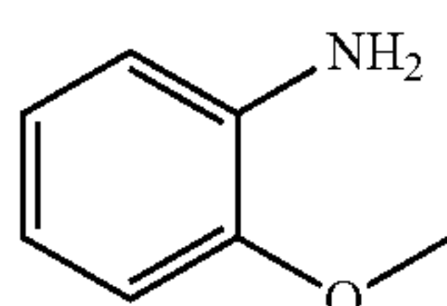
2-methoxyaniline
