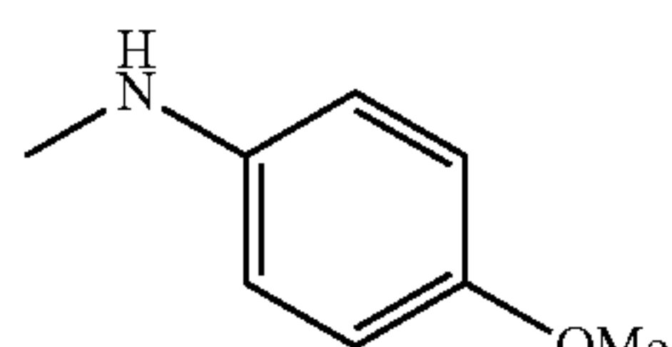
4-methoxy-N-methylaniline
