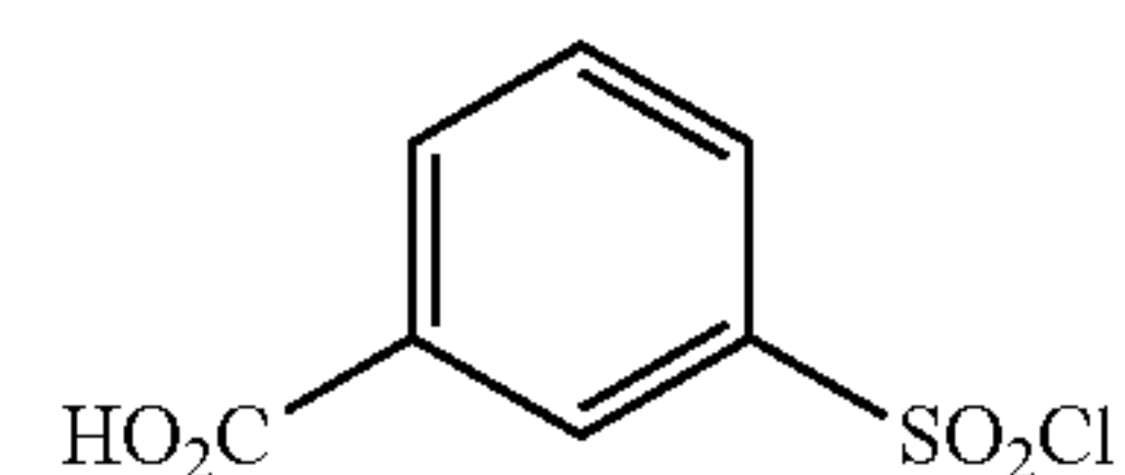
3-(chlorosulfonyl)benzoic acid
