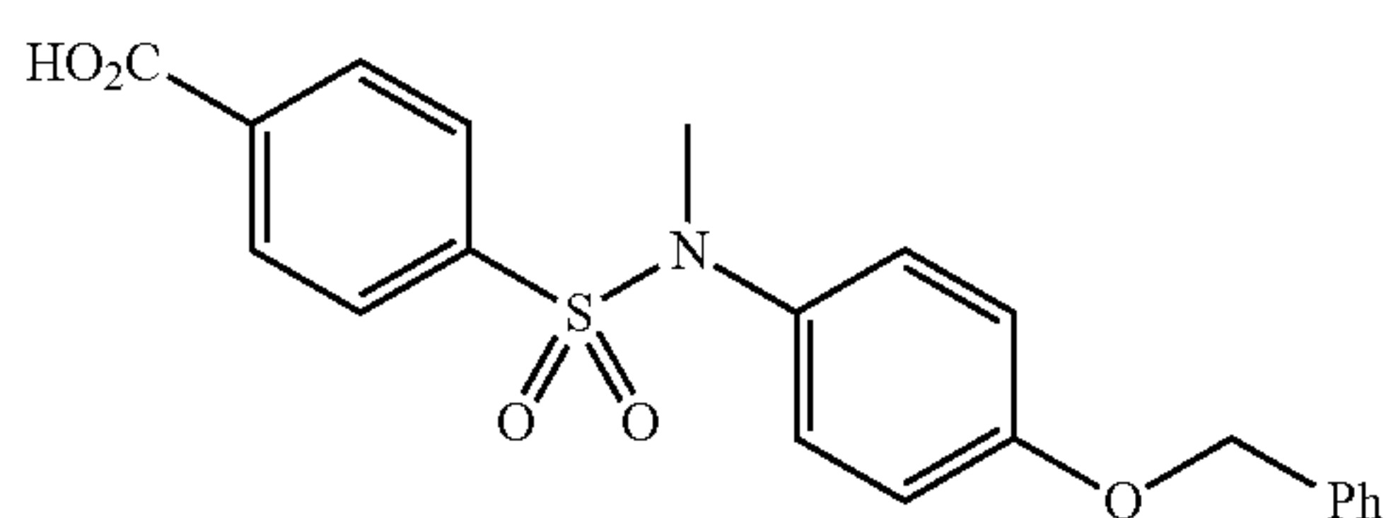
4-(N-(4-(benzyloxy)phenyl)-N-methylsulfamoyl)benzoic acid
