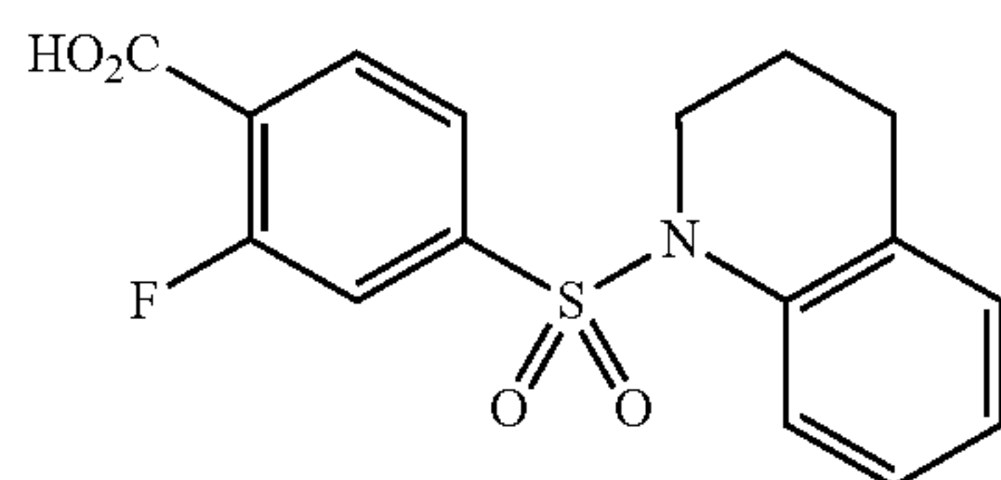
4-(3,4-dihydroquinolin-1(2H)-ylsulfonyl)-2-fluorobenzoic acid
