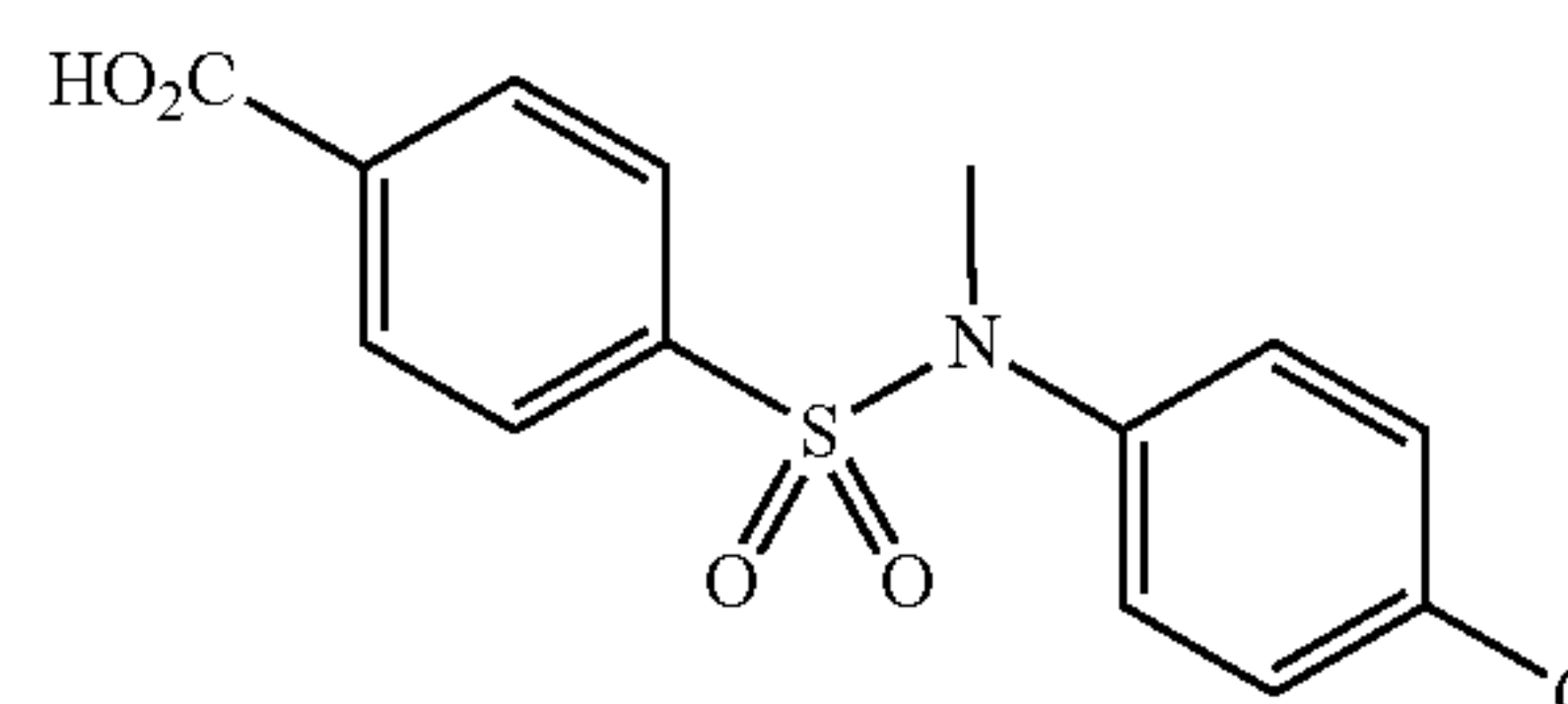
4-(N-(4-chlorophenyl)-N-methylsulfonyl)benzoic acid
