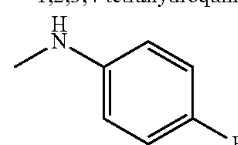
4-fluoro-N-methylaniline
