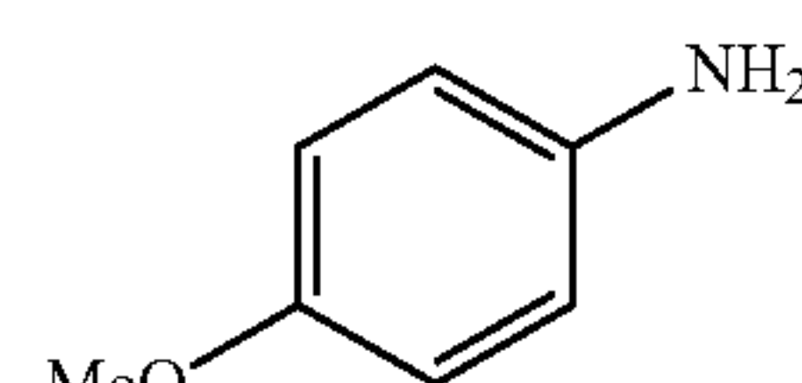
4-methoxyaniline
