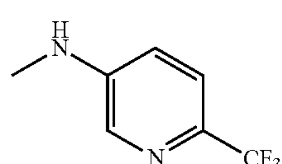
N-methyl-4-(trifluoromethyl)aniline
