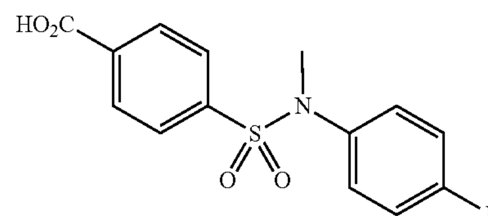
4-(N-(4-fluorophenyl)-N-methylsulfonyl)benzoic acid
