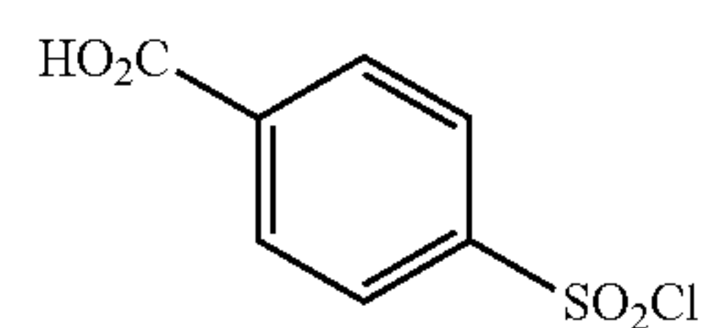
4-(chlorosulfonyl)benzoic acid
