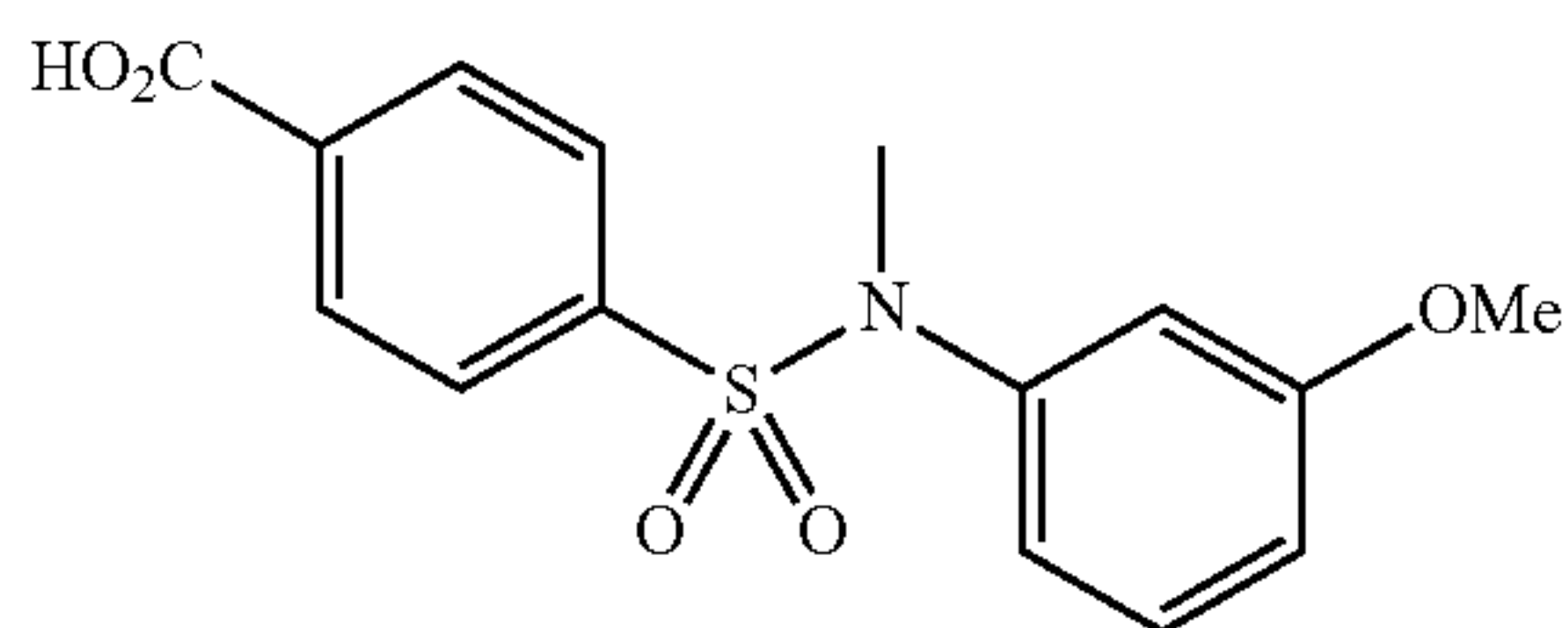
4-(N-(3-methoxyphenyl)-N-methylsulfamoyl)benzoic acid
