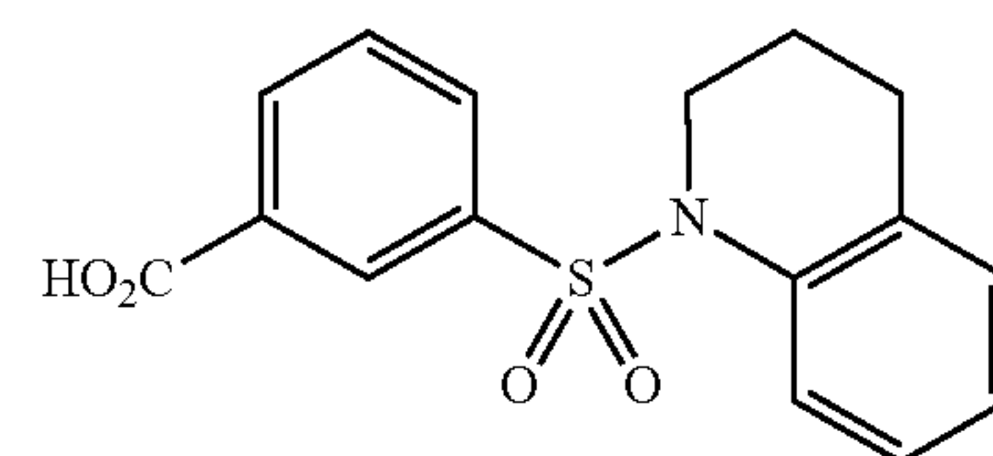
3-(3,4-dihydroquinolin-1(2H)-ylsulfonyl)benzoic acid
