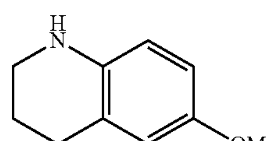
6-methoxy-1,2,3,4-tetrahydroquinoline
