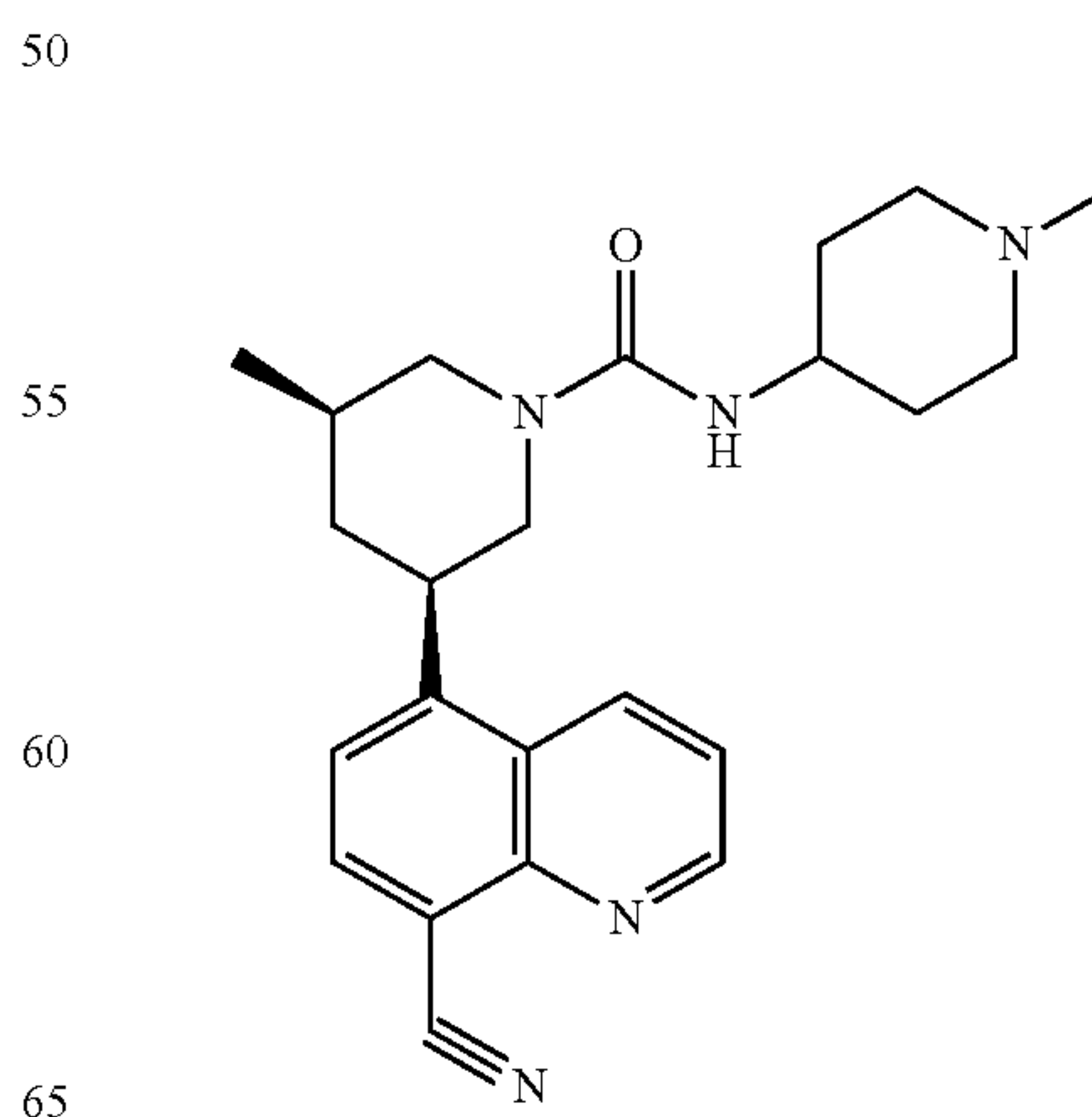
Compound 107
