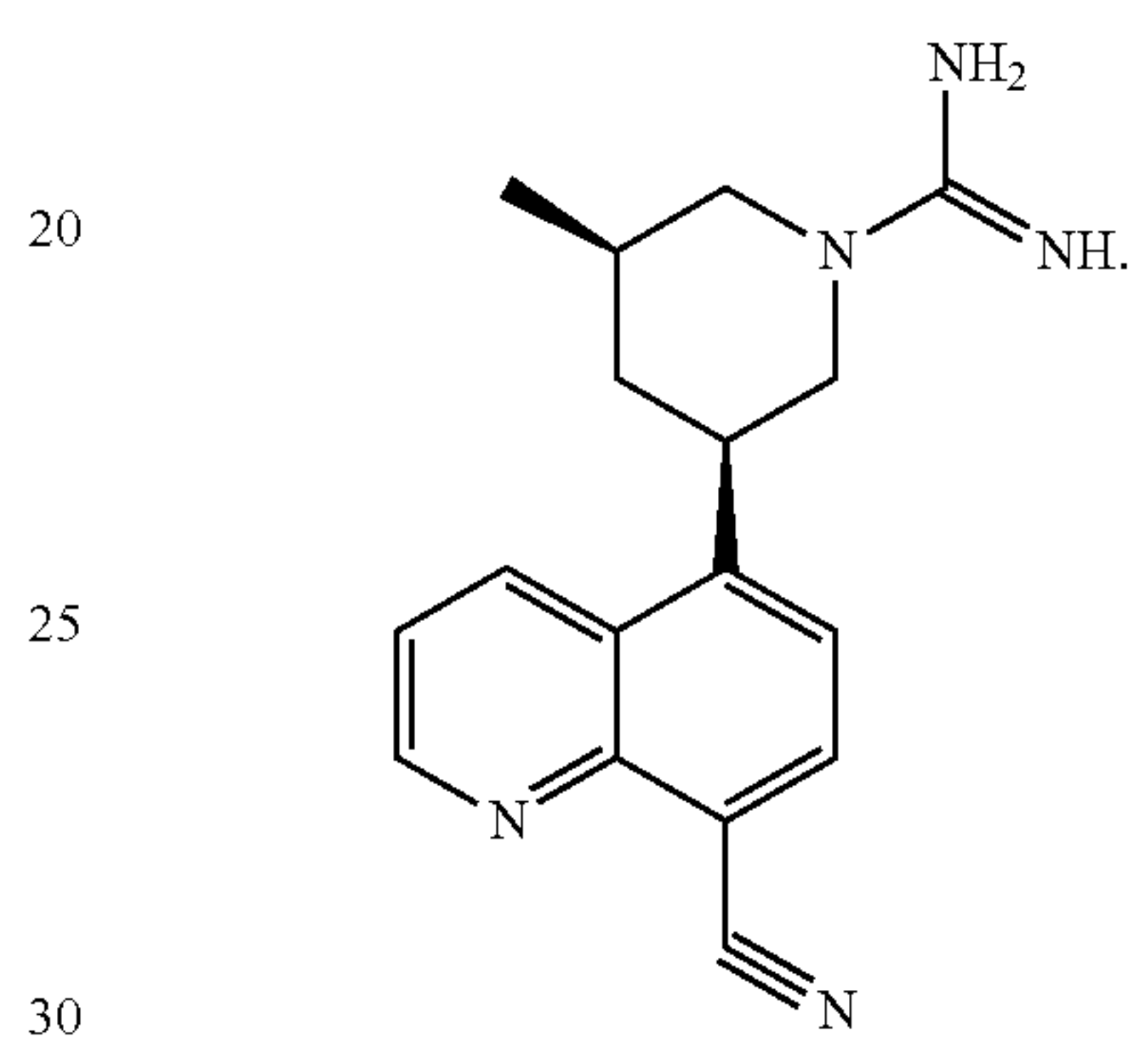
Compound 117
