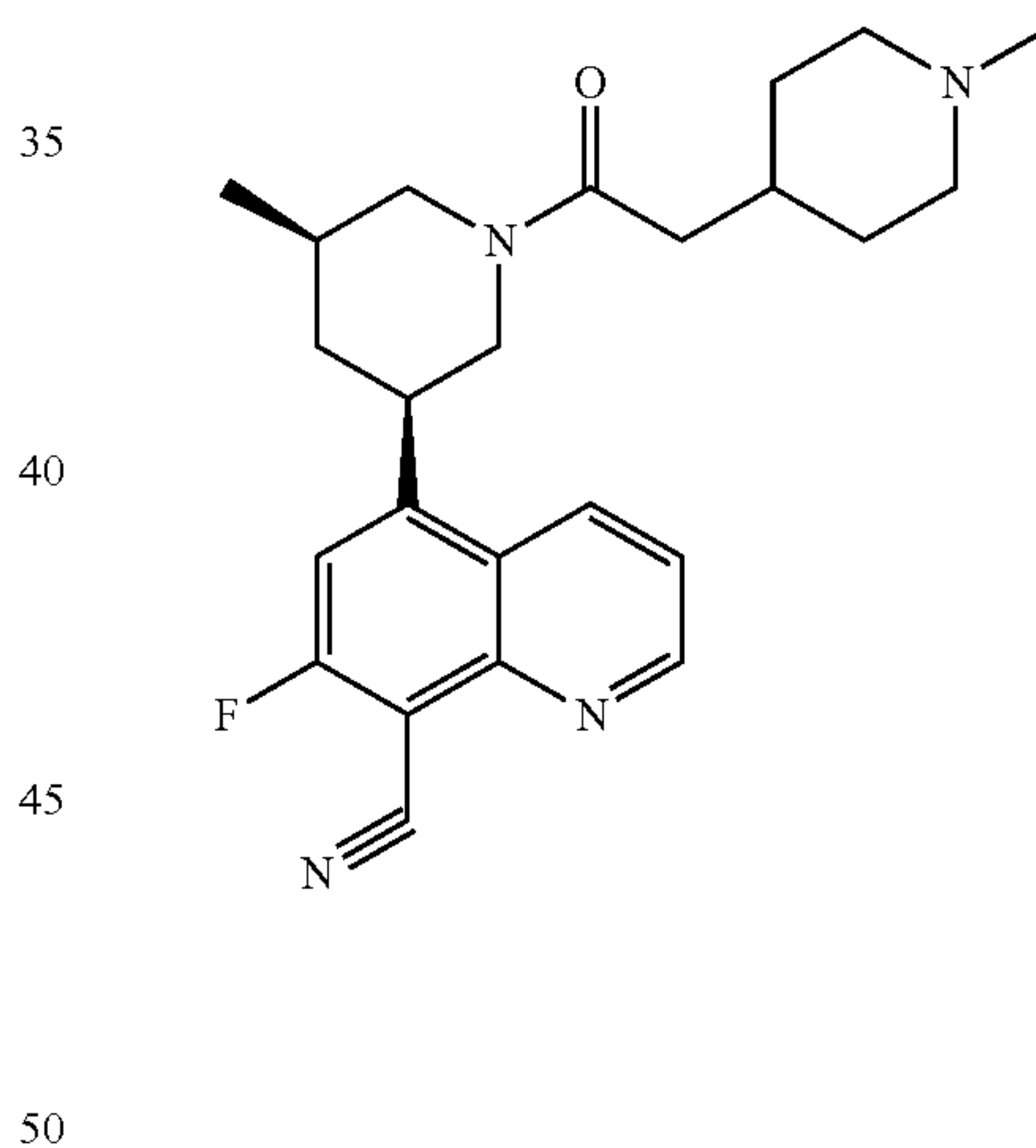
Compound 81
