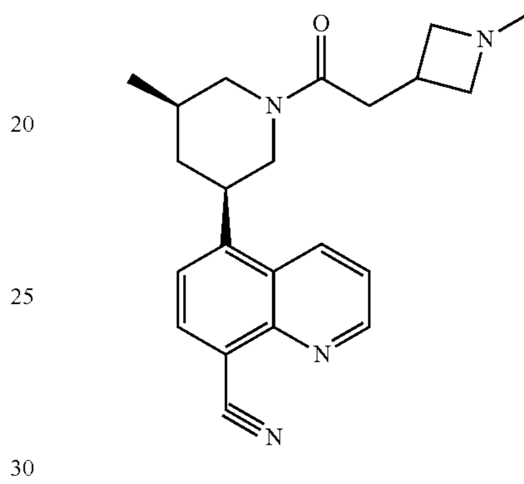
Compound 30
