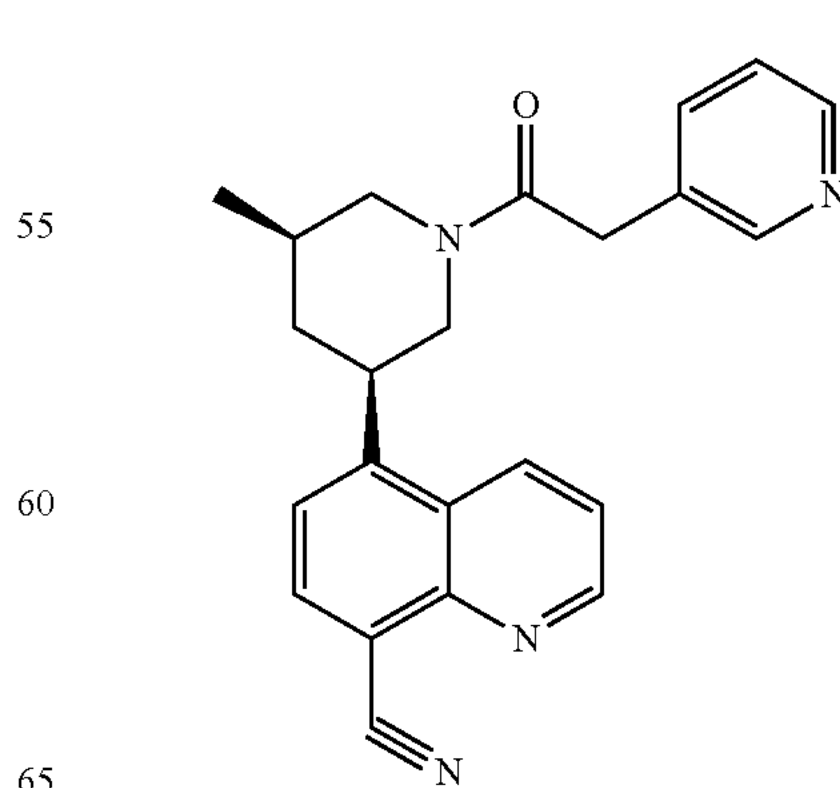
Compound 16
