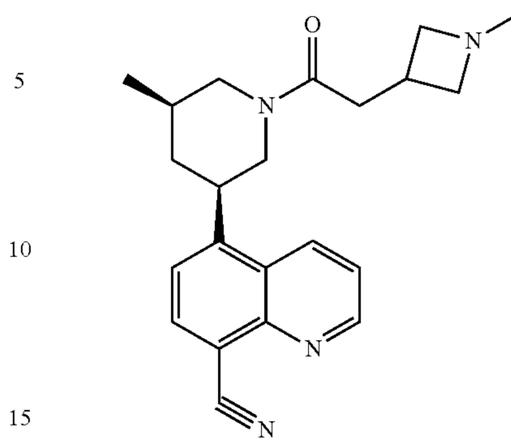
Compound 30
