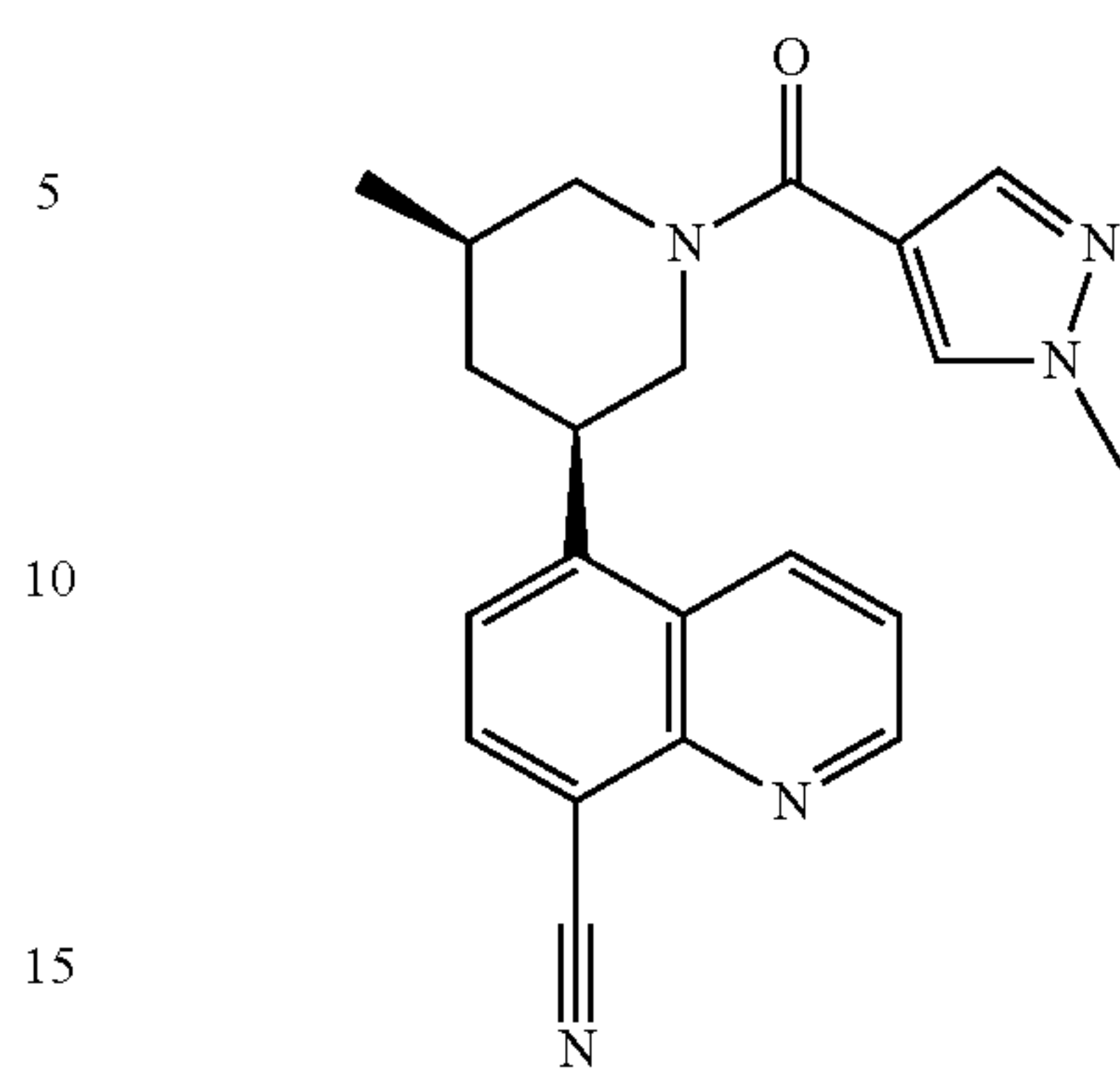
Compound 99
