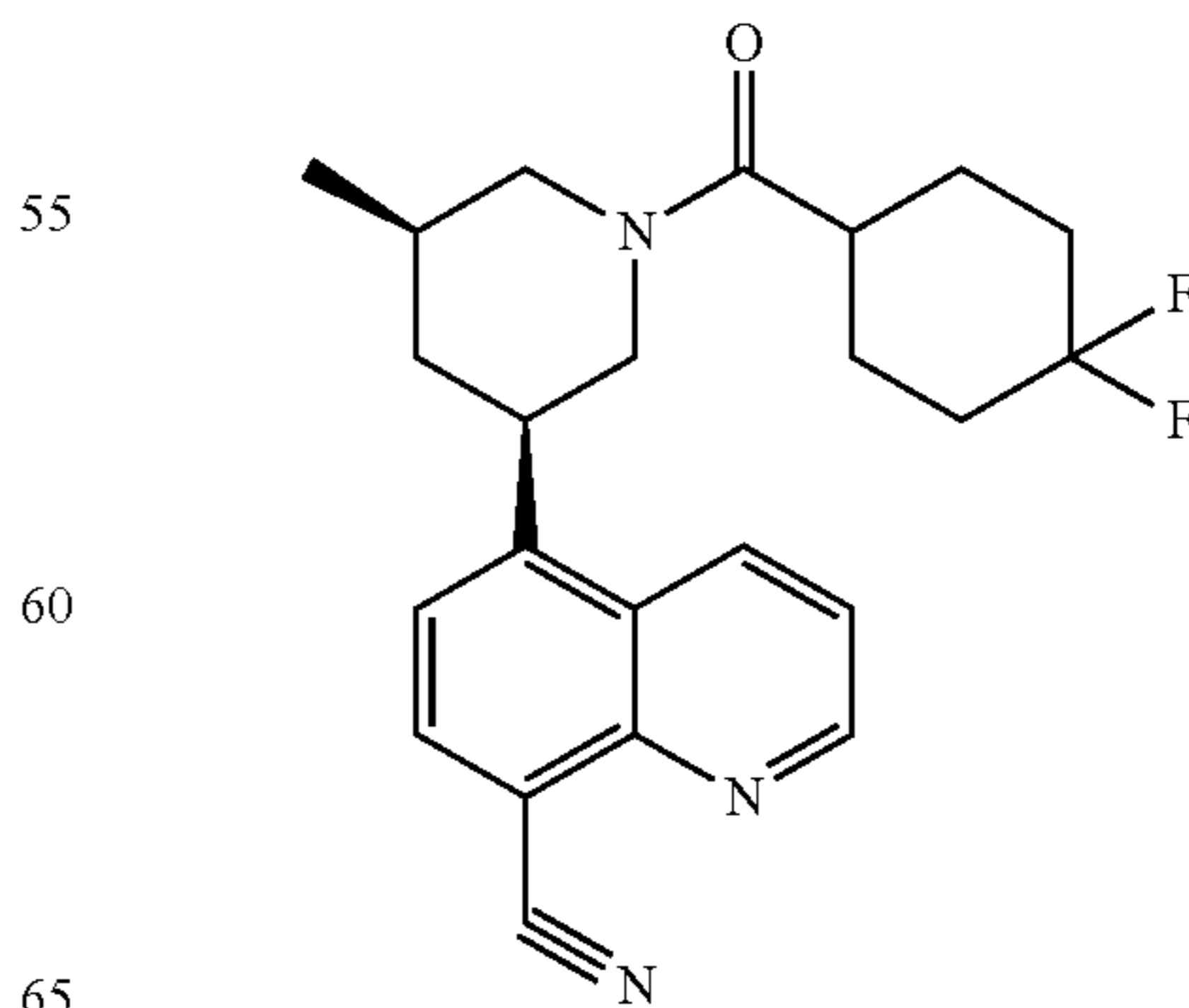
Compound 33
