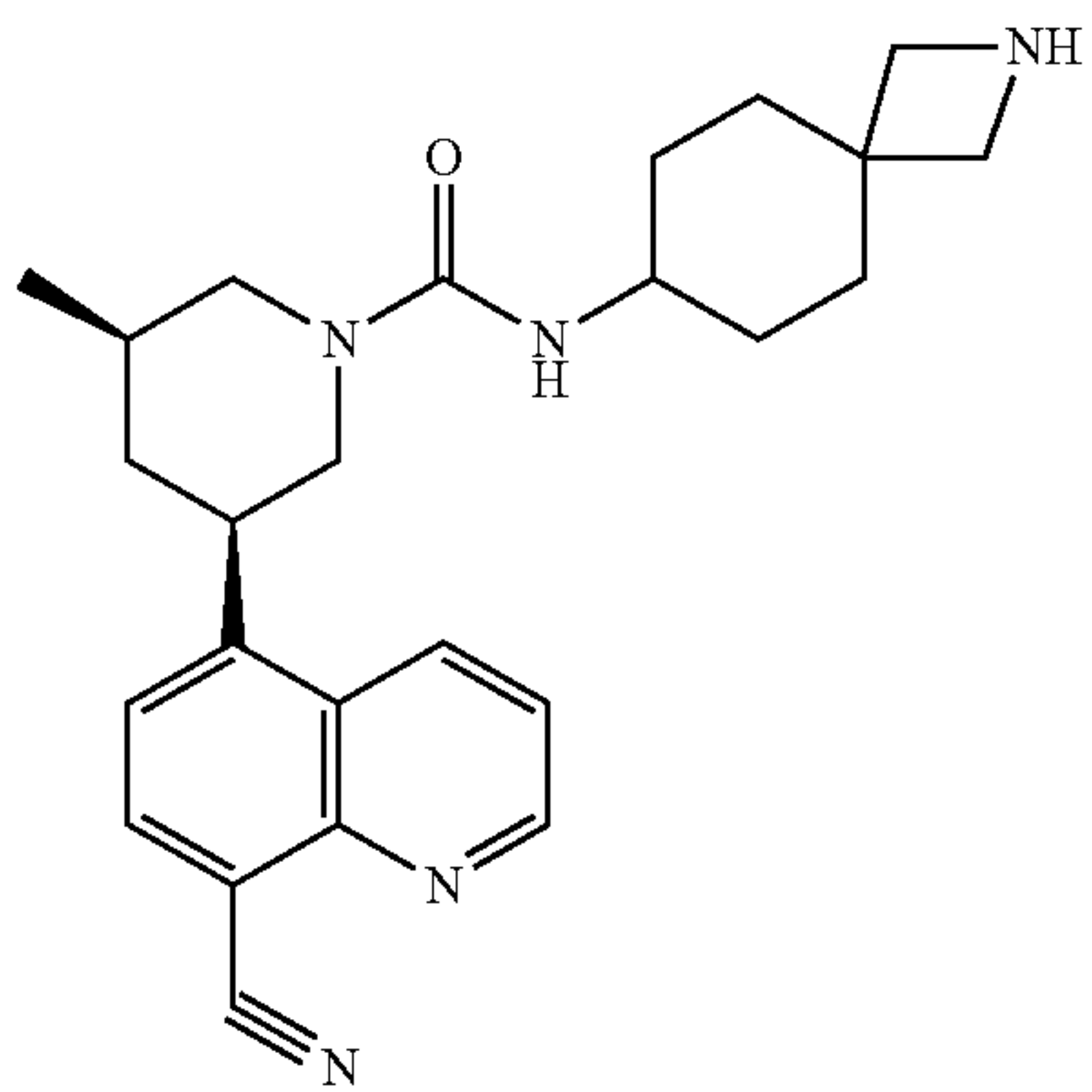
Compound 117
