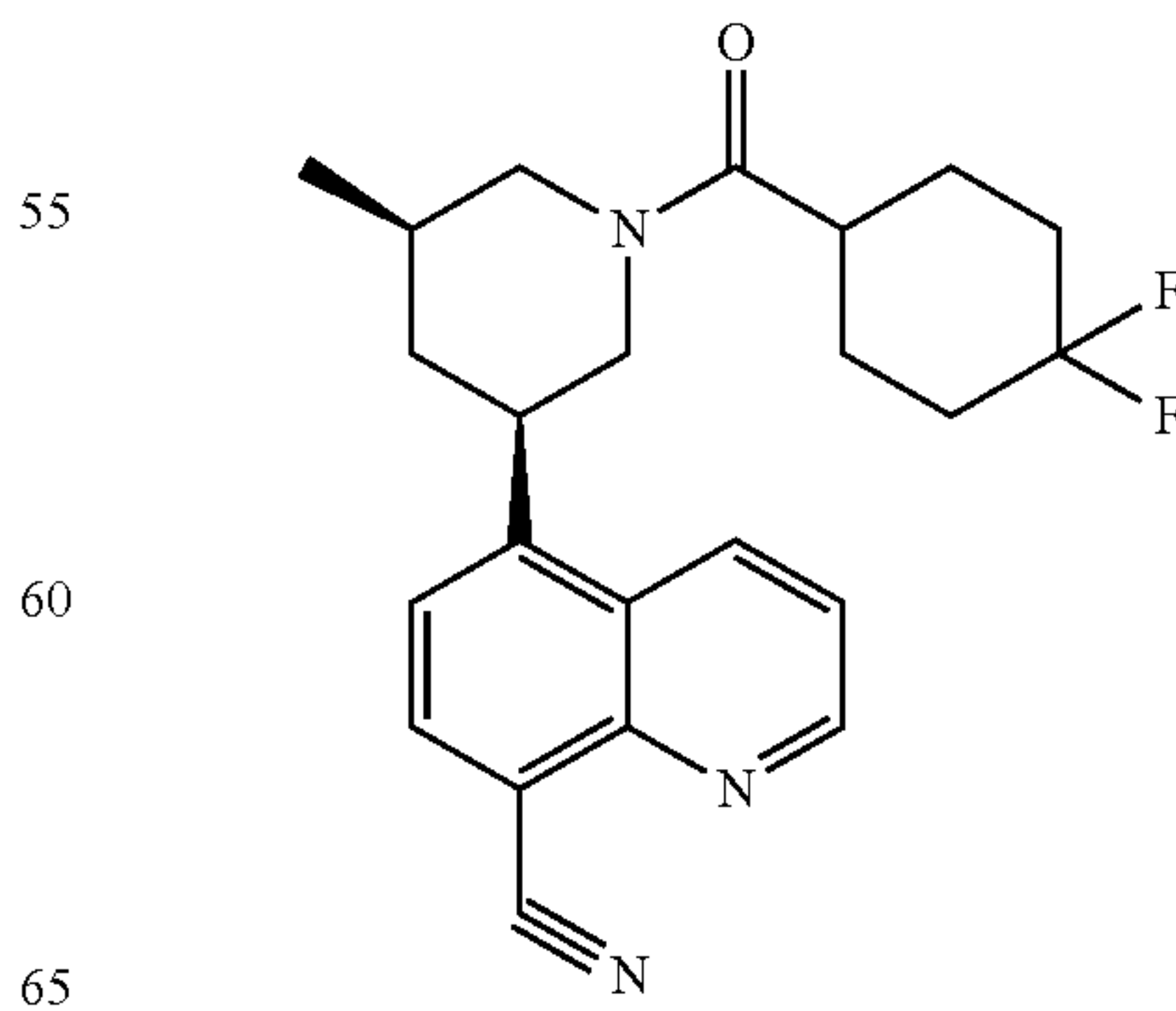
Compound 33
