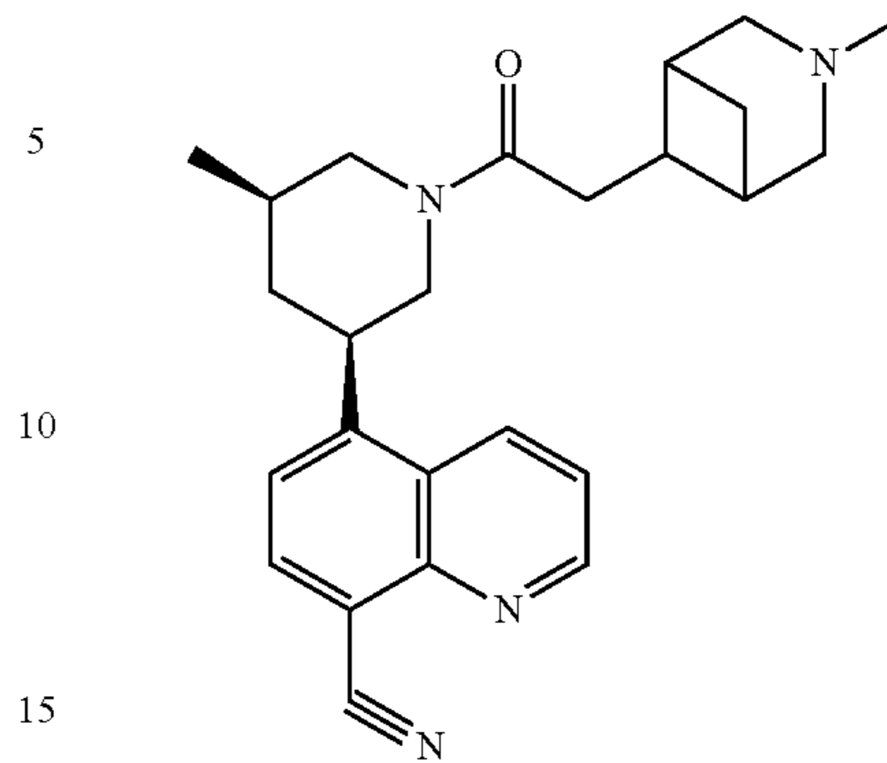
Compound 79
