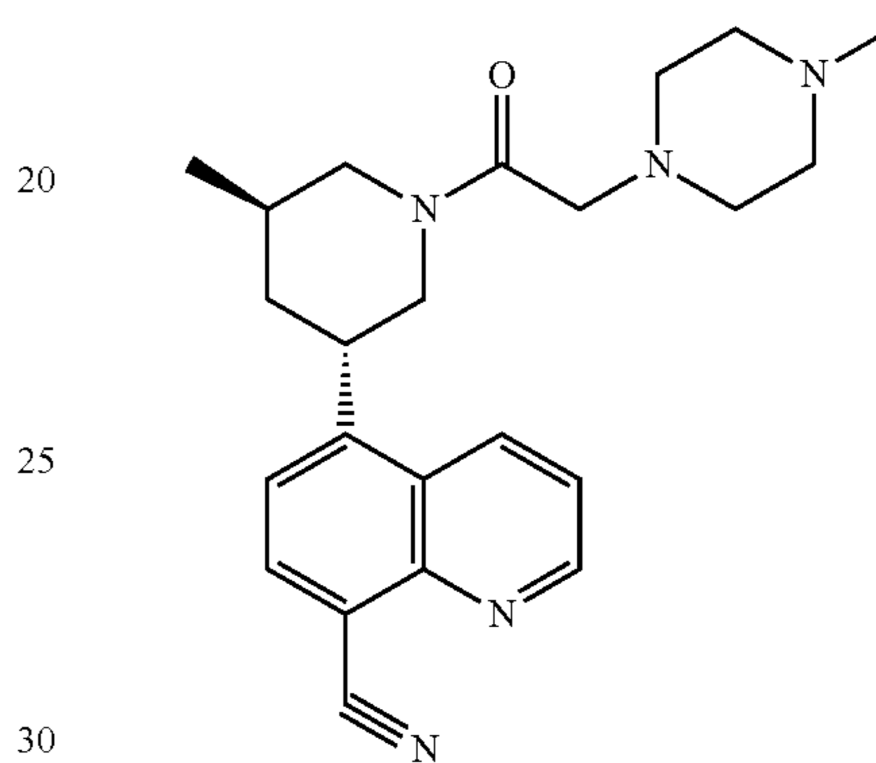
Compound 85
