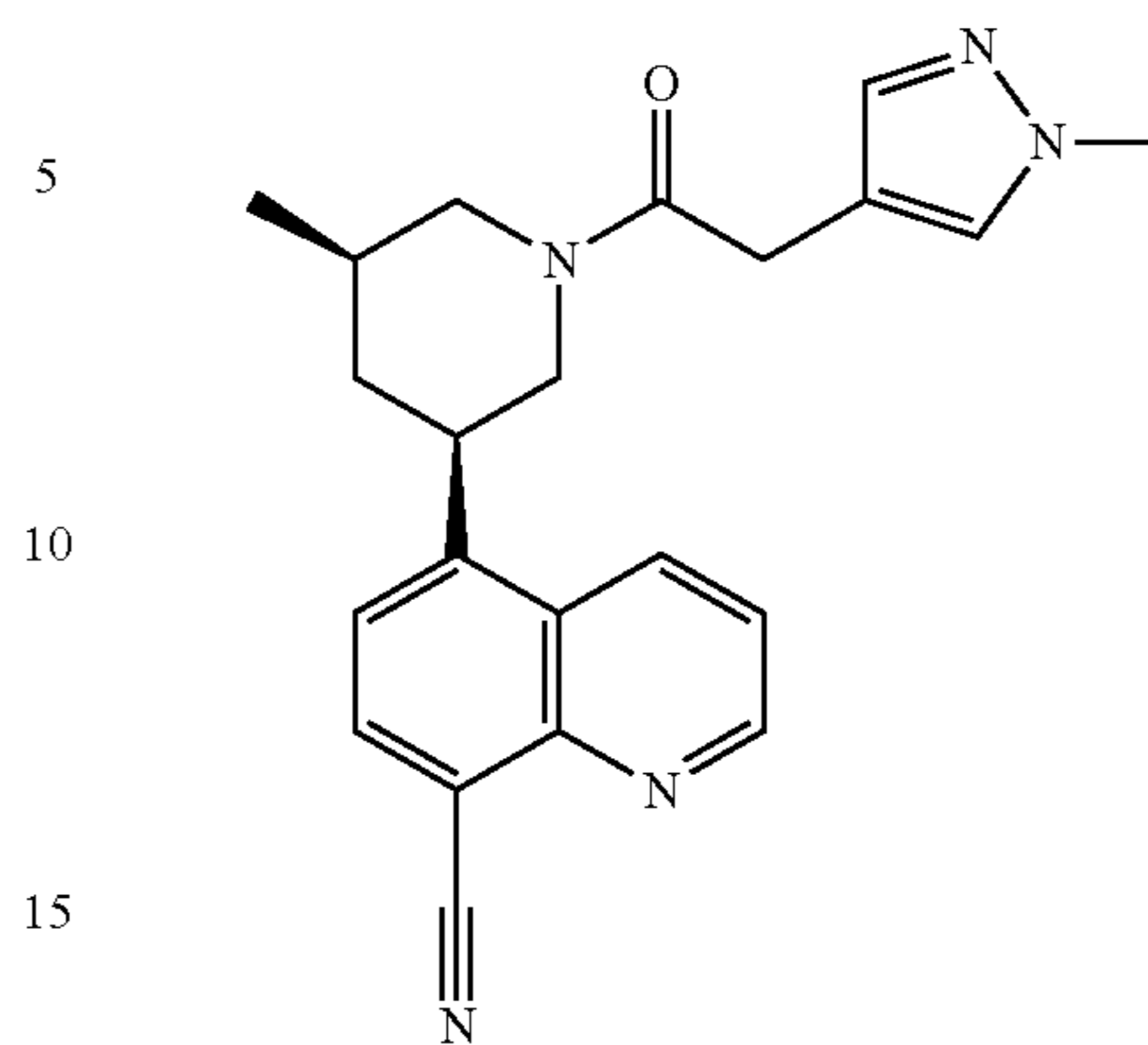
Compound 103
