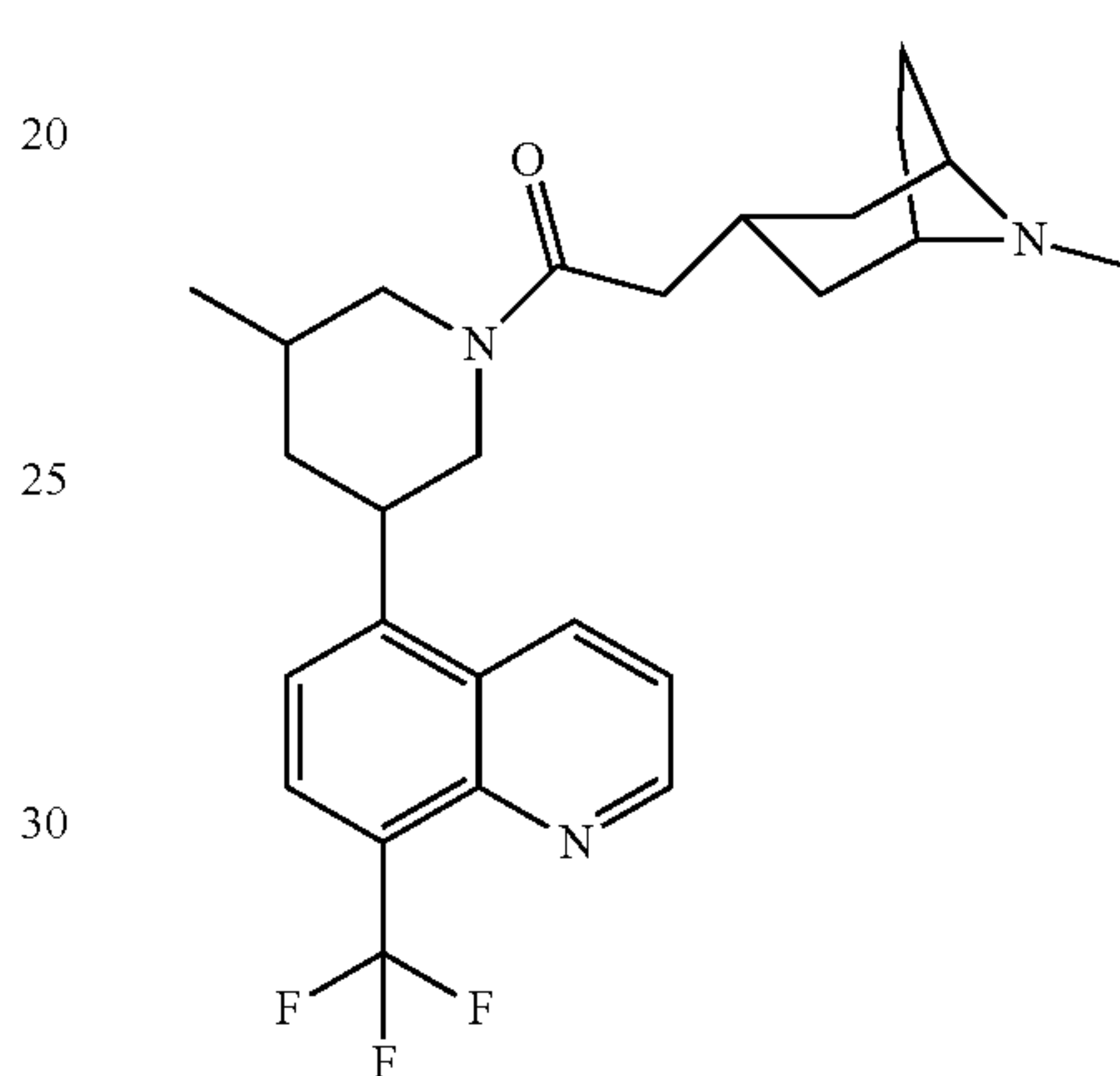
Compound 15
