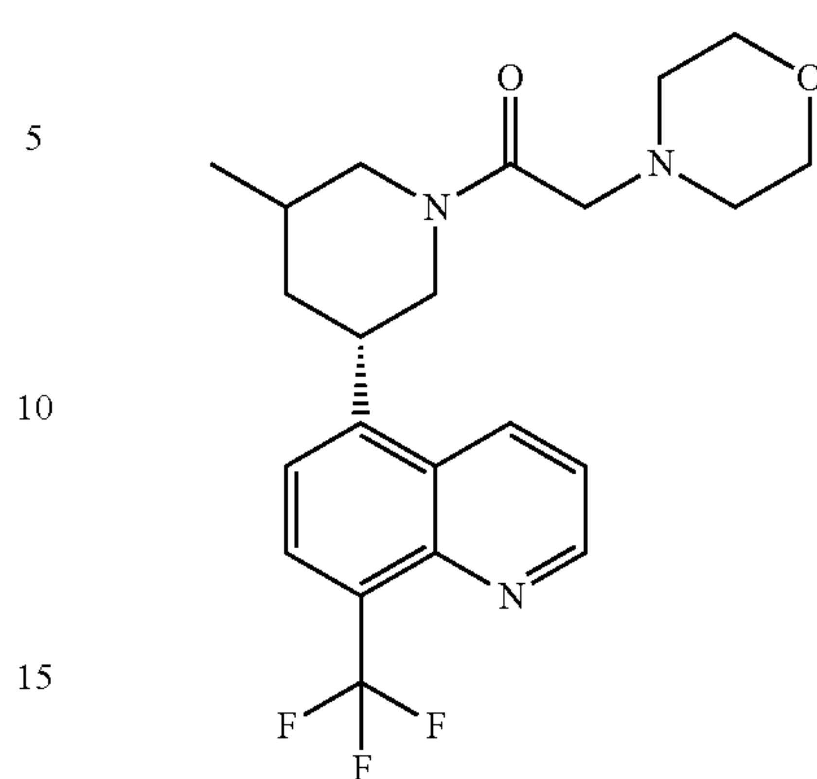
Compound 13
