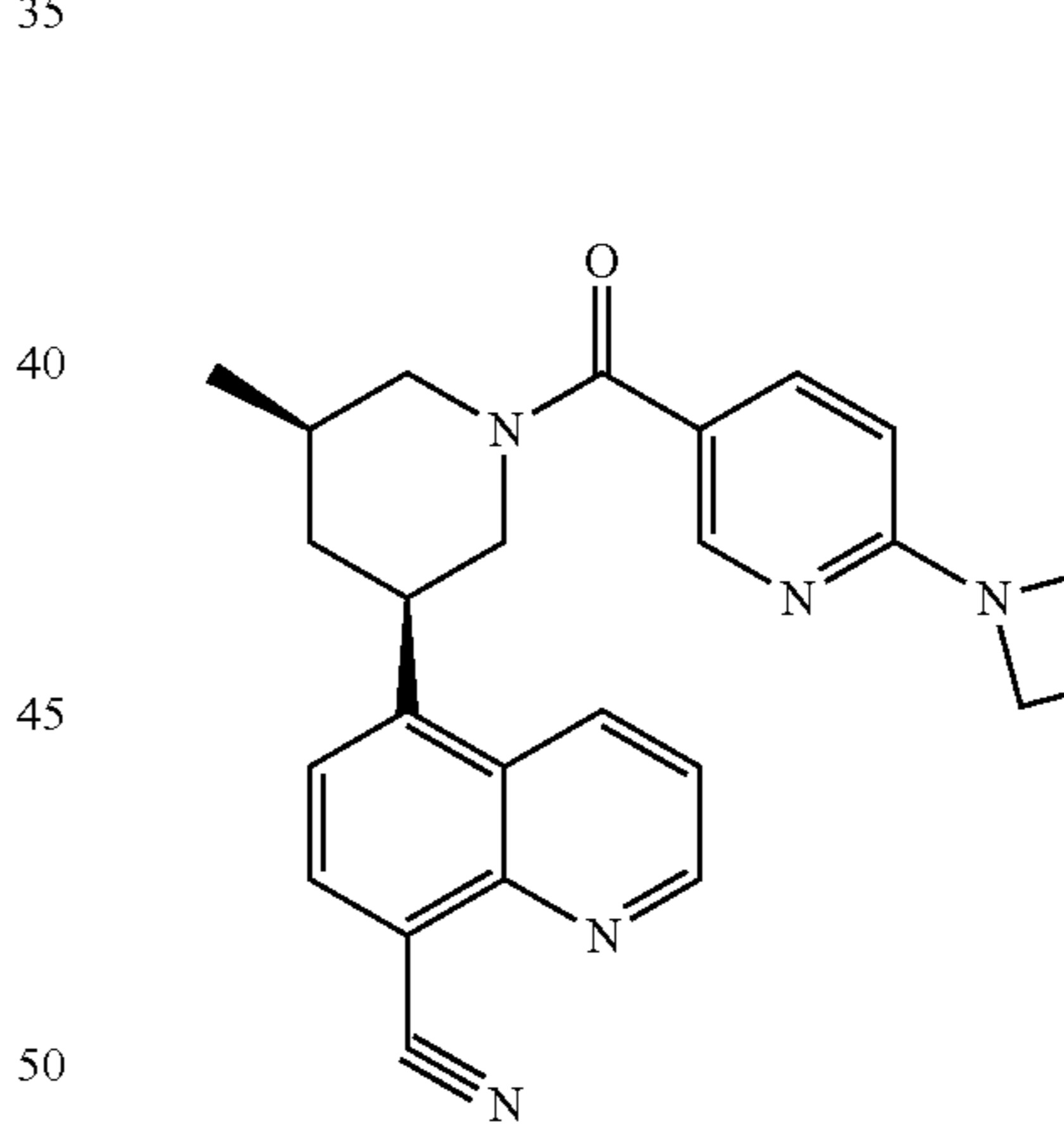
Compound 32
