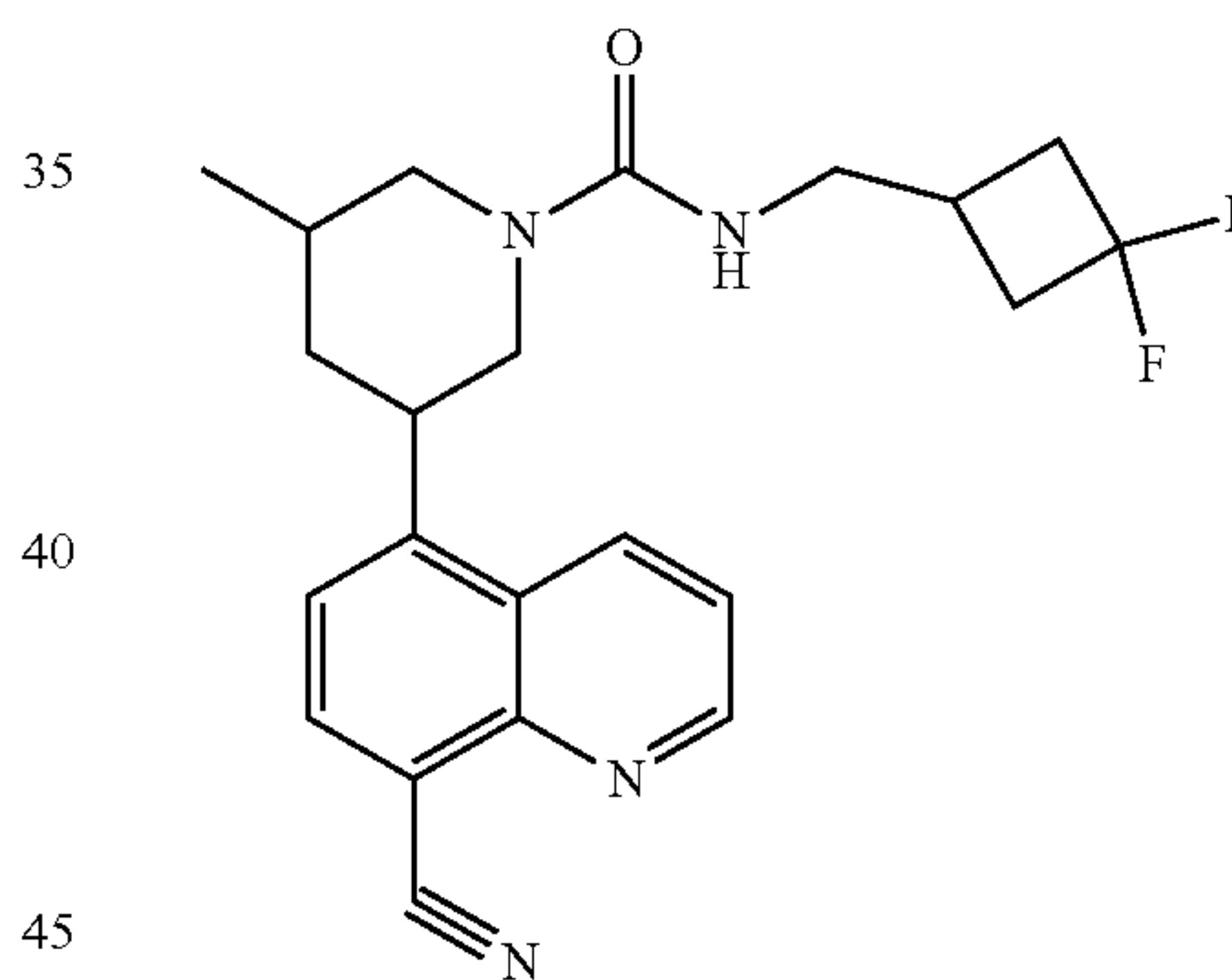
Compound 106
