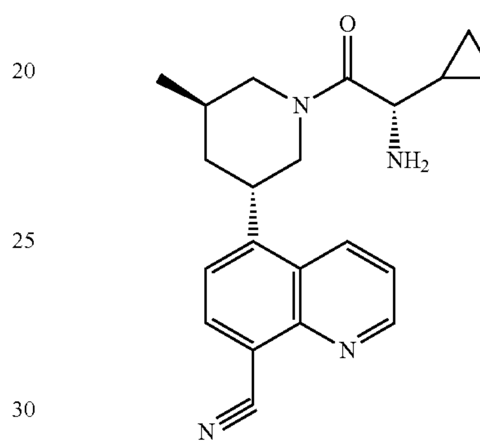
Compound 56
