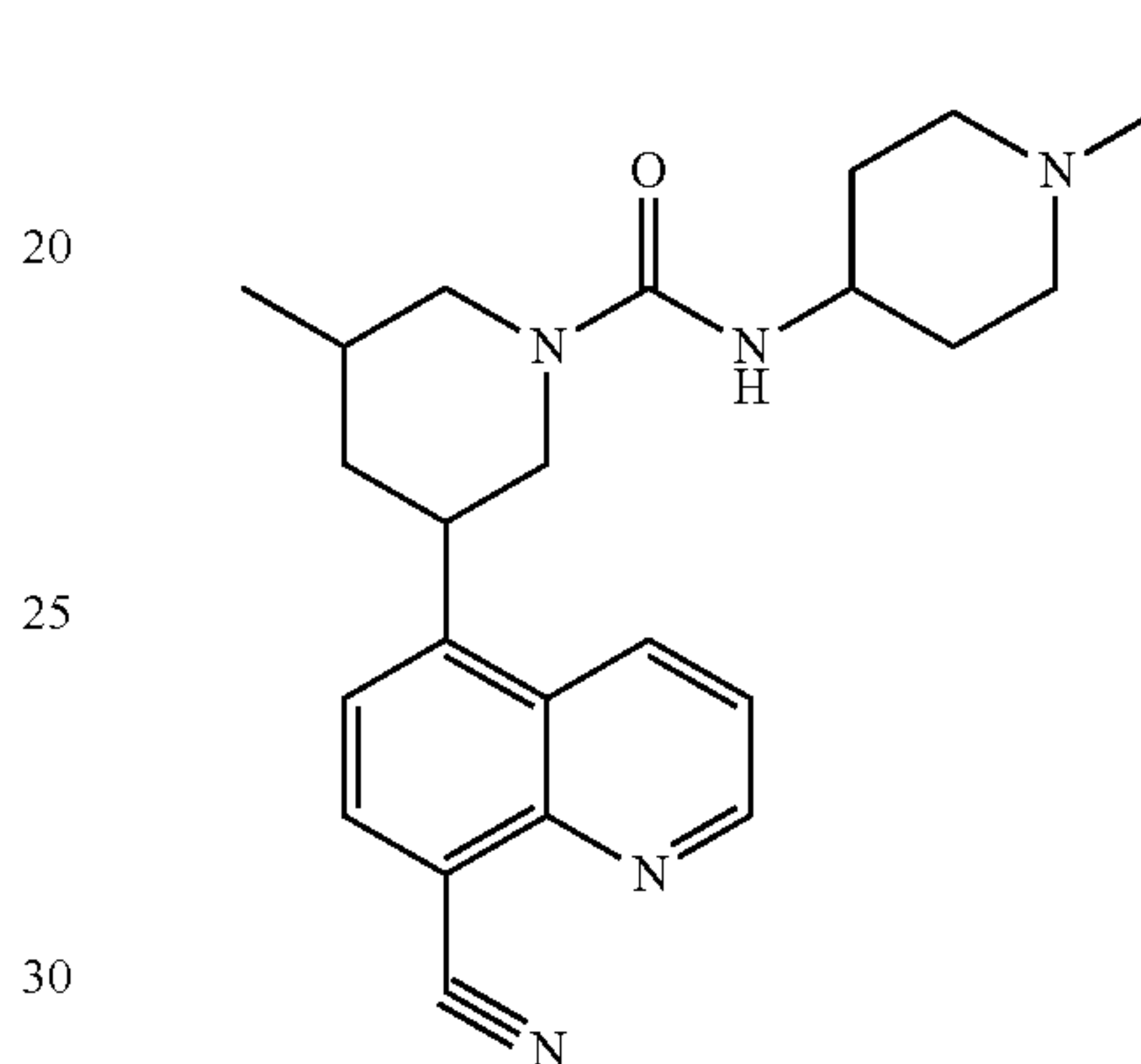
Compound 100
