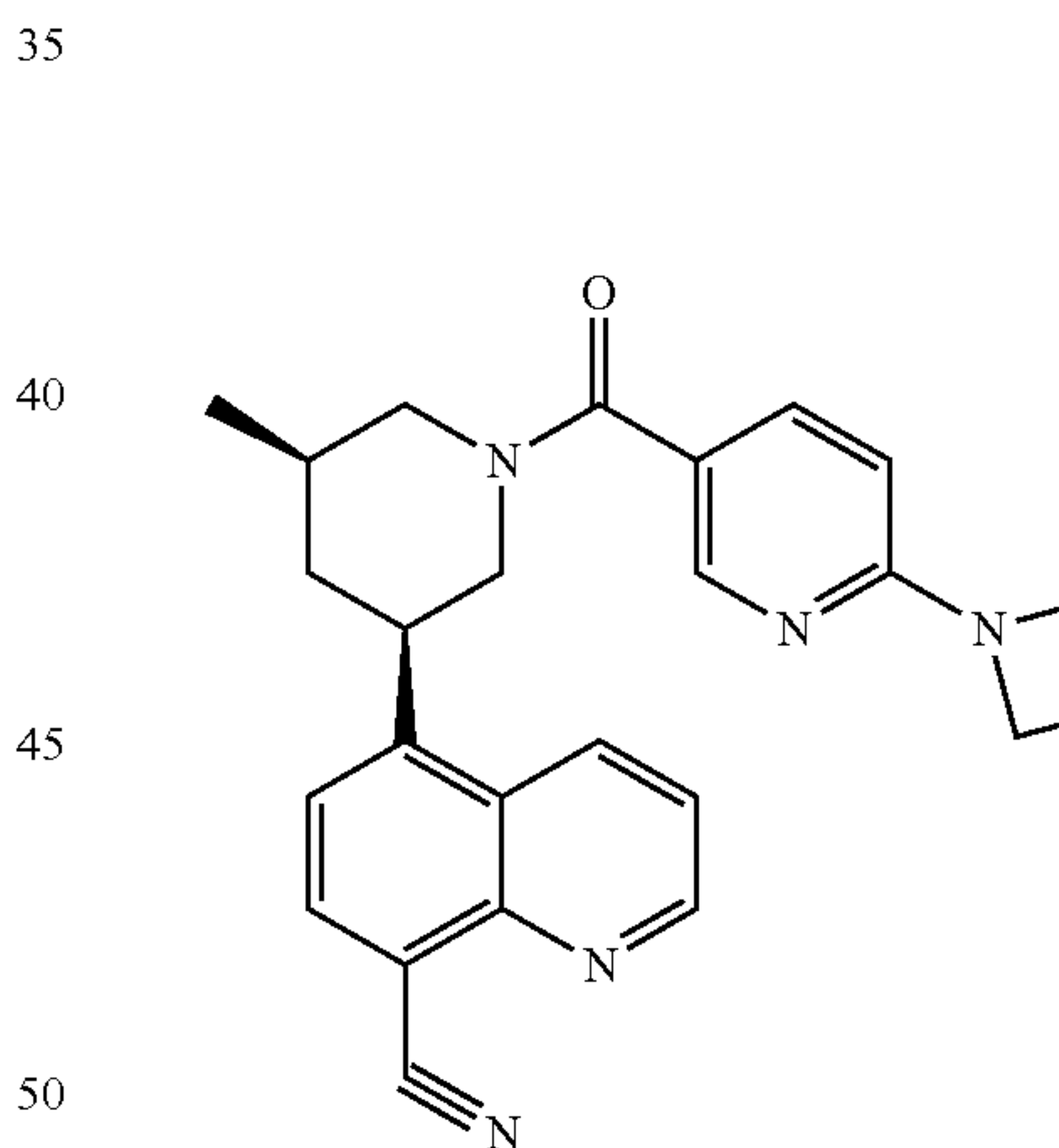
Compound 32
