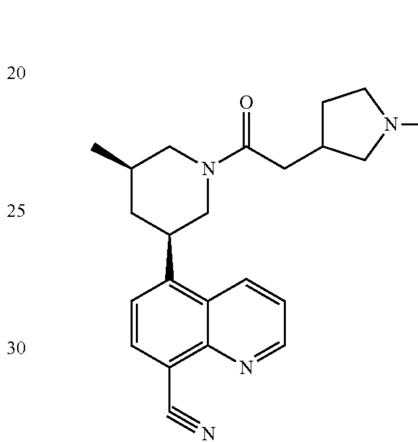
Compound 31
