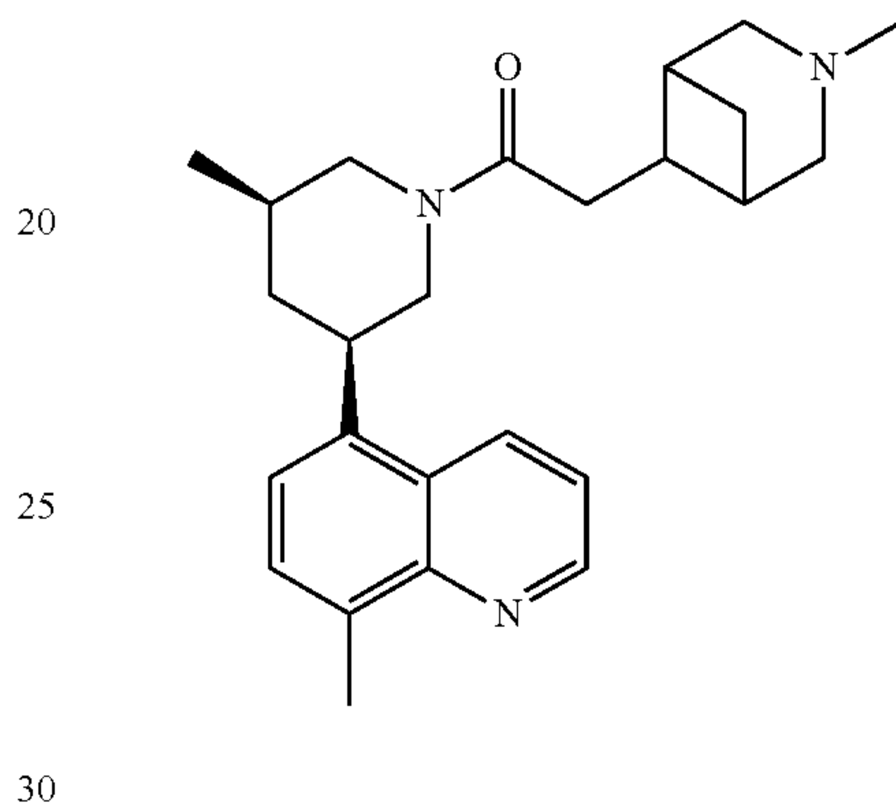
Compound 80
