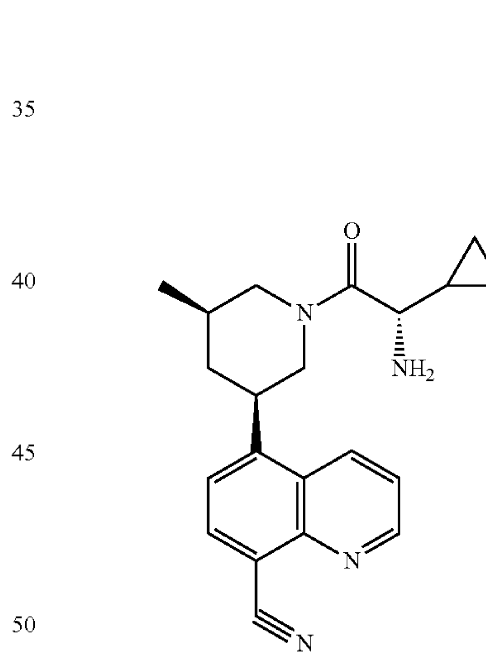
Compound 57
