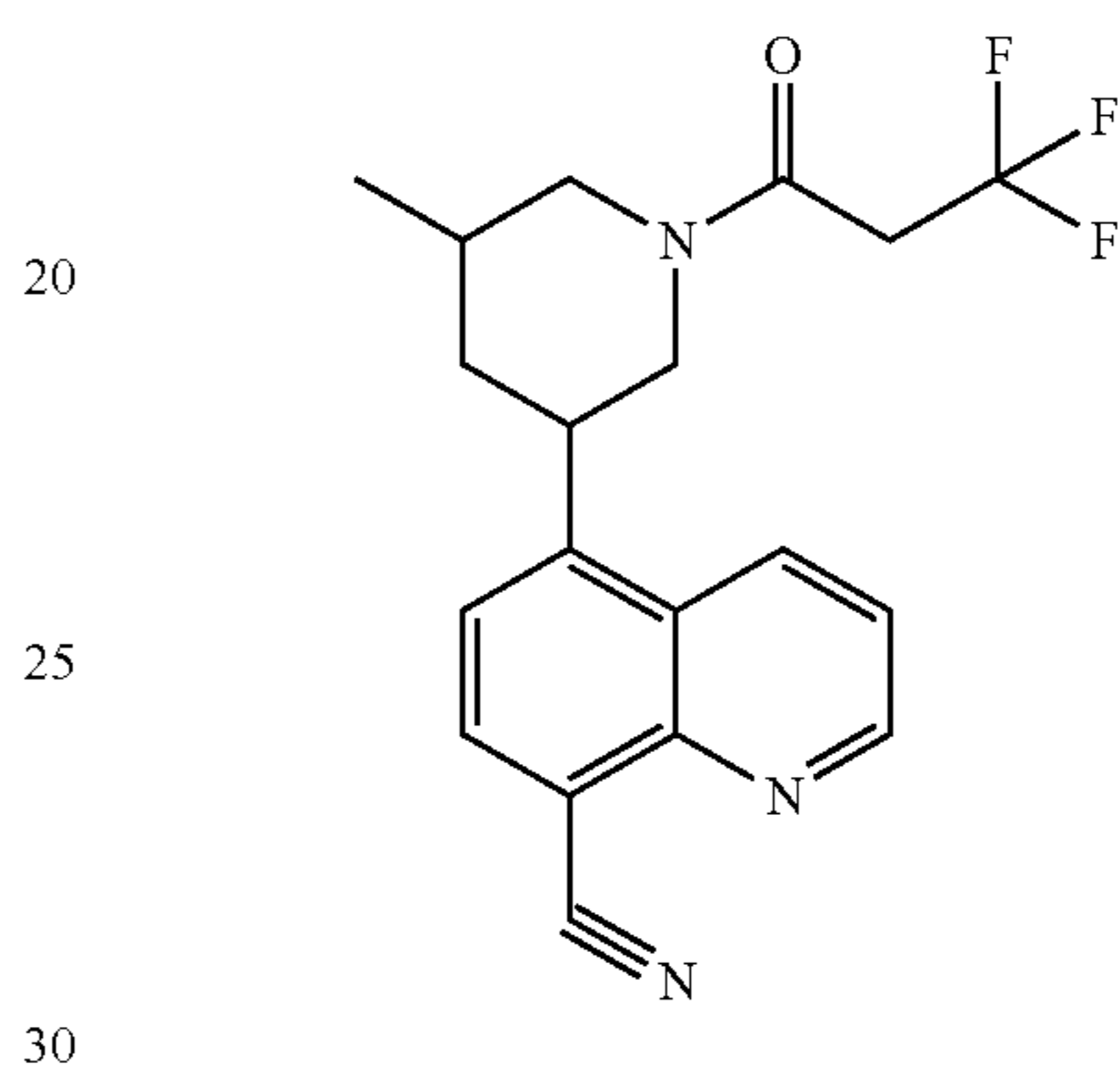
Compound 22
