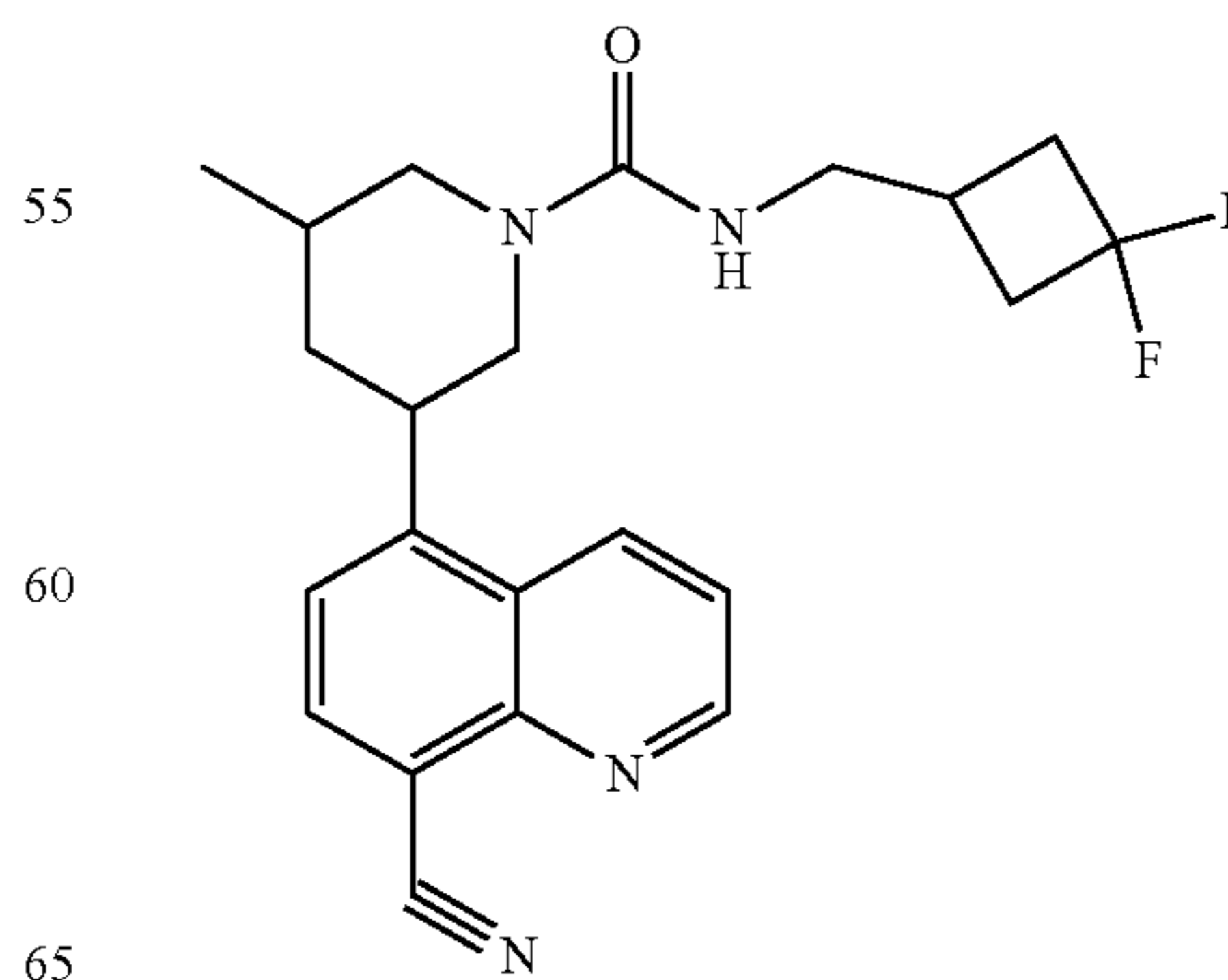
Compound 106
