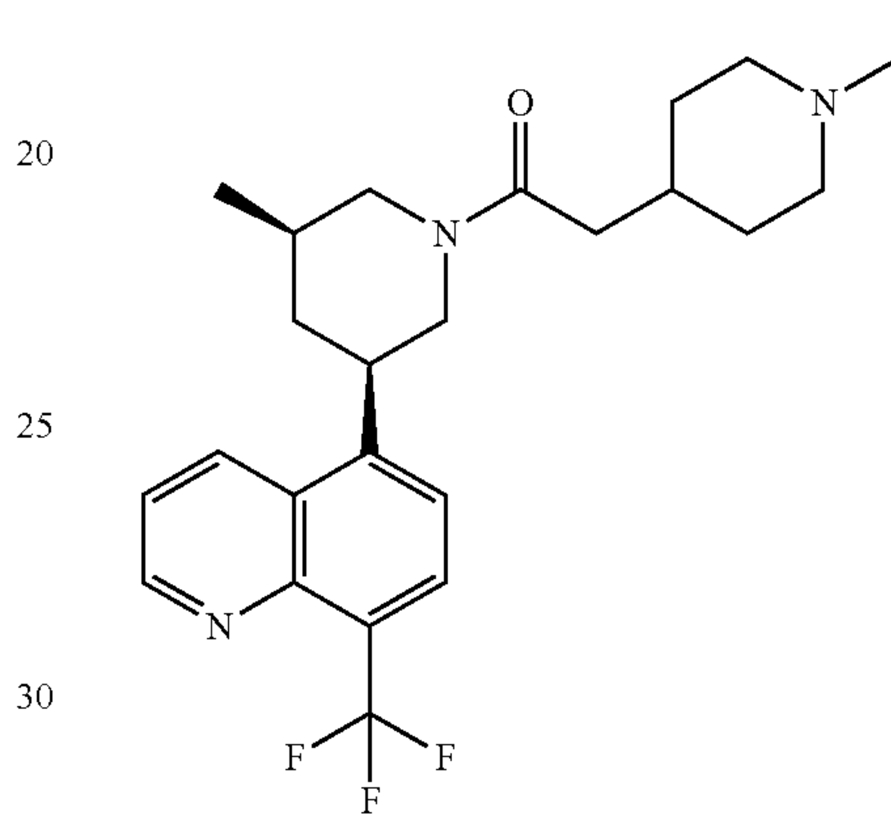
Compound 38
