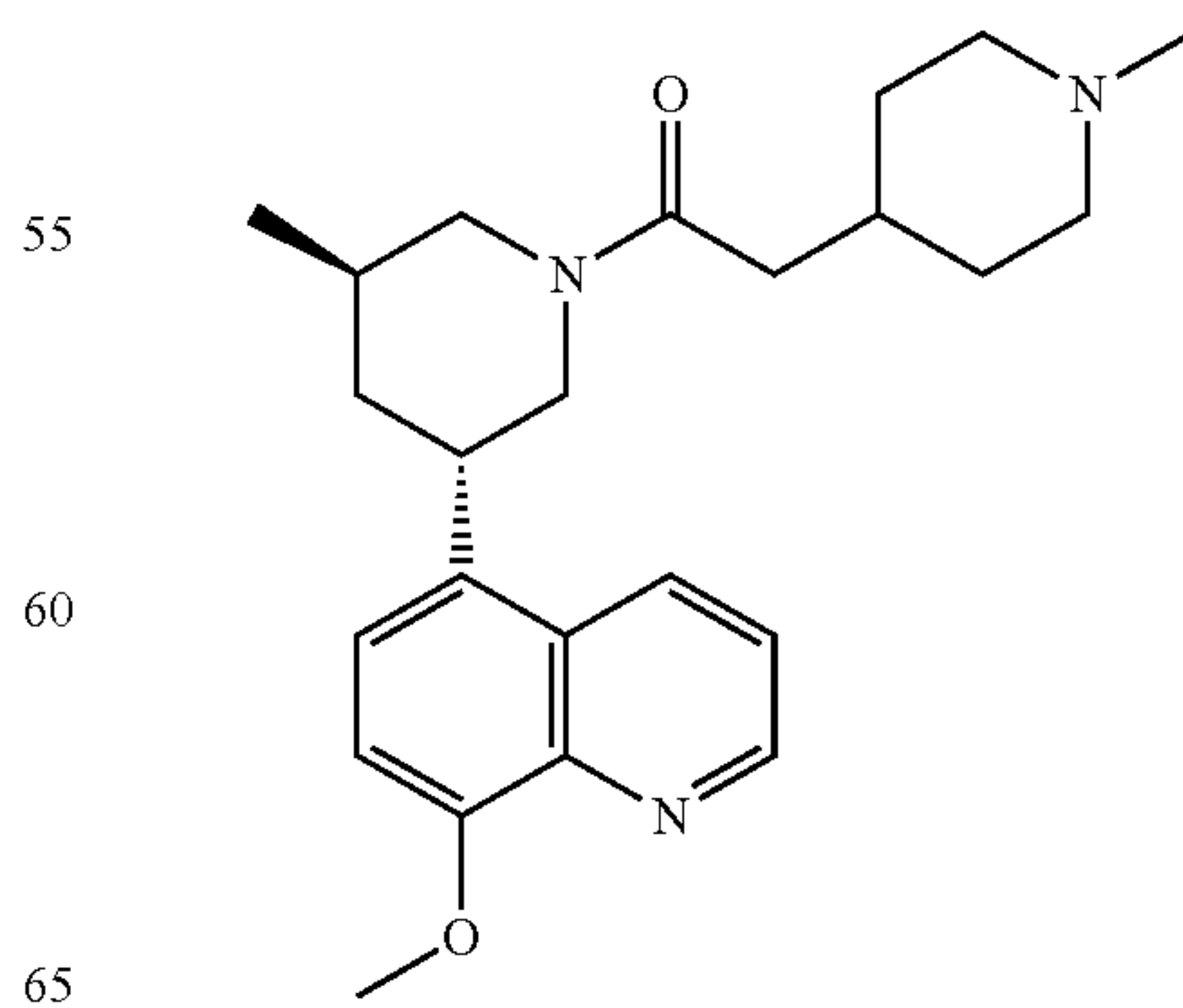
Compound 82
