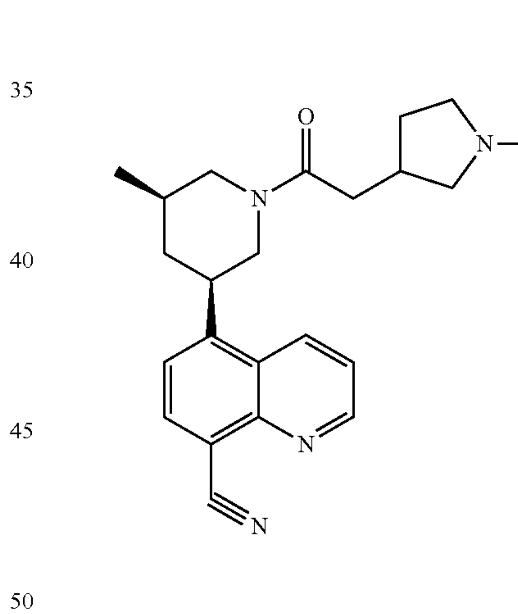
Compound 31
