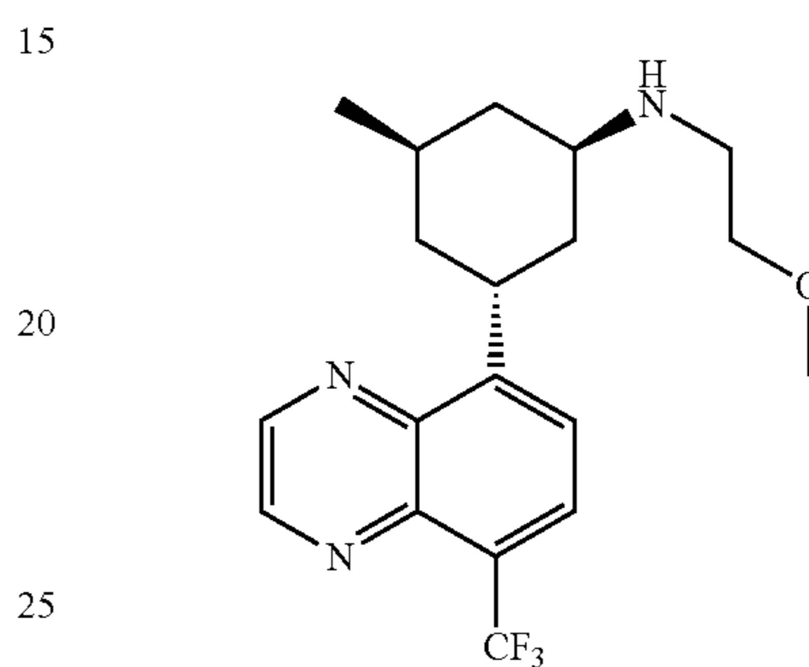
Compound 145
