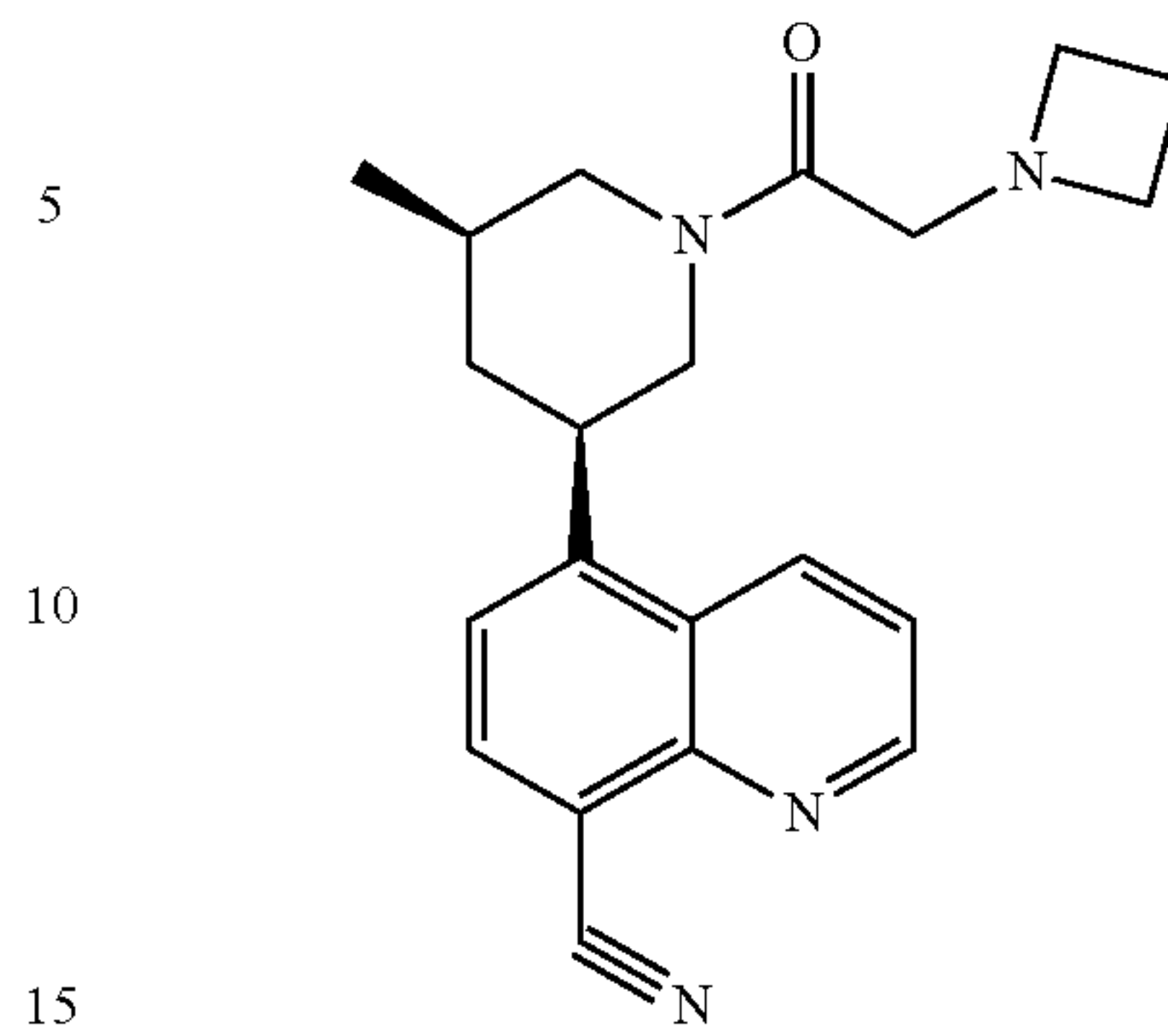
Compound 29
