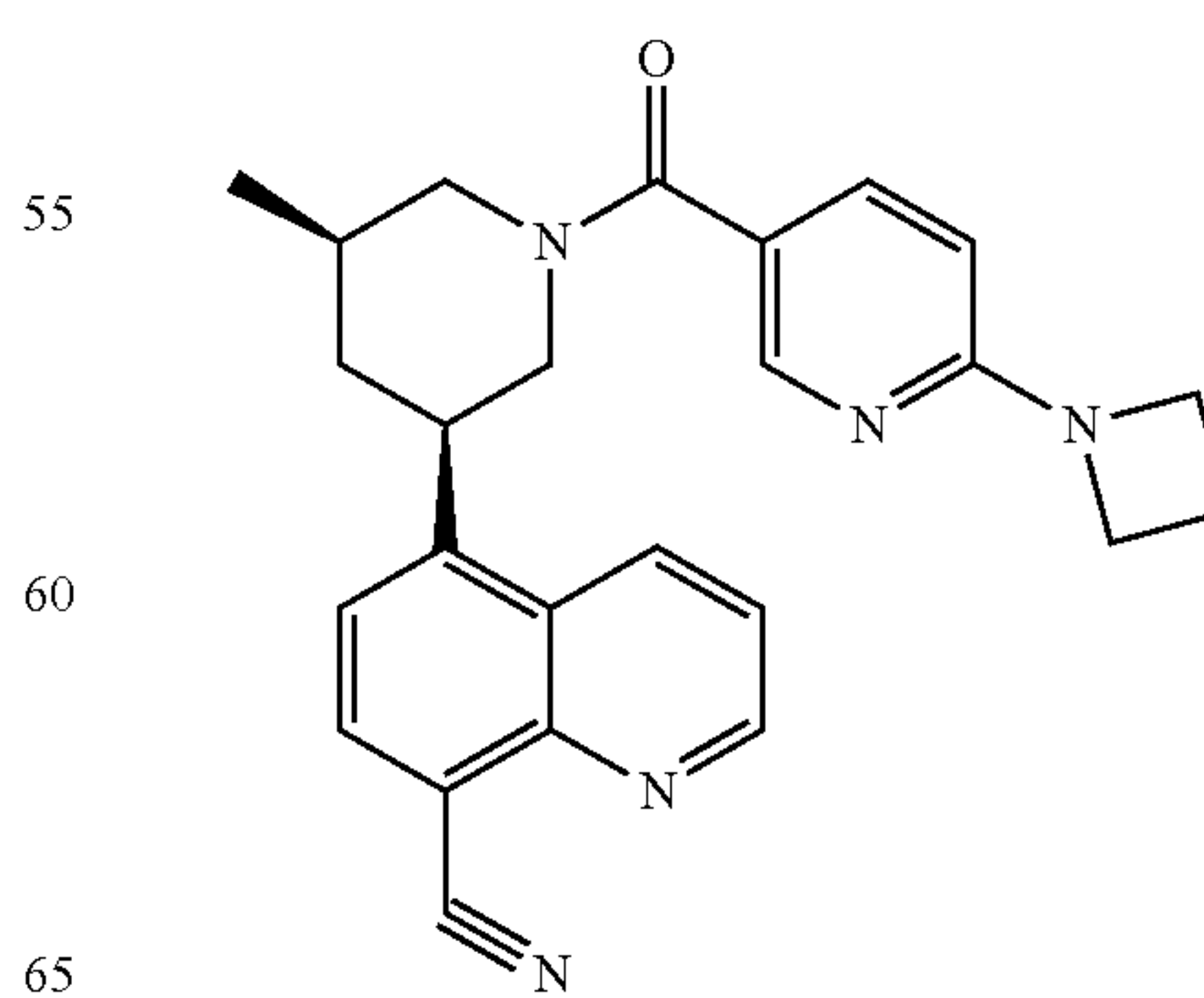
Compound 32
