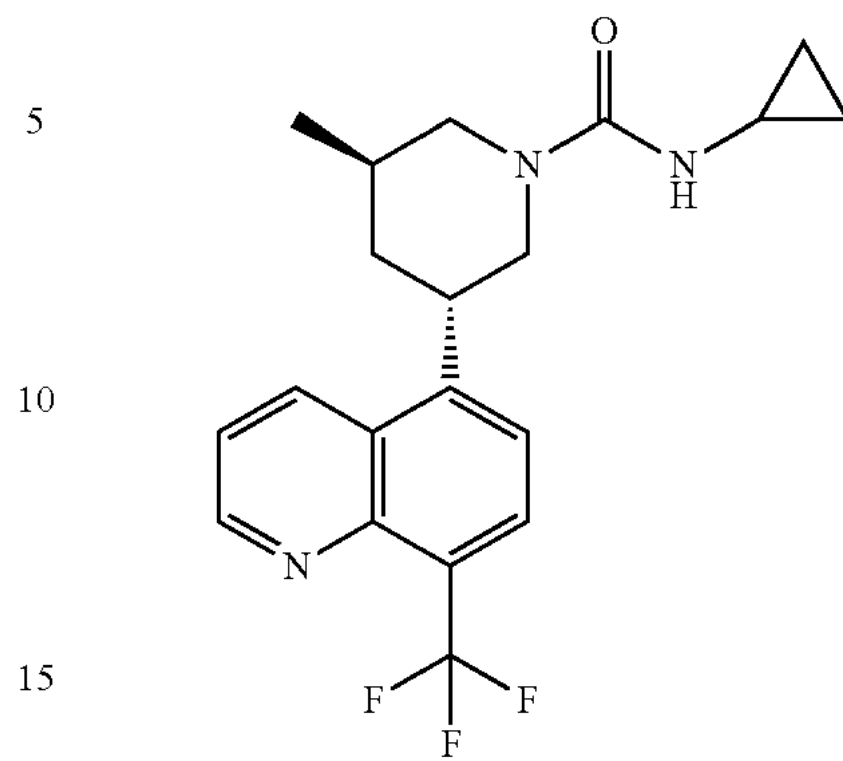
Compound 37
