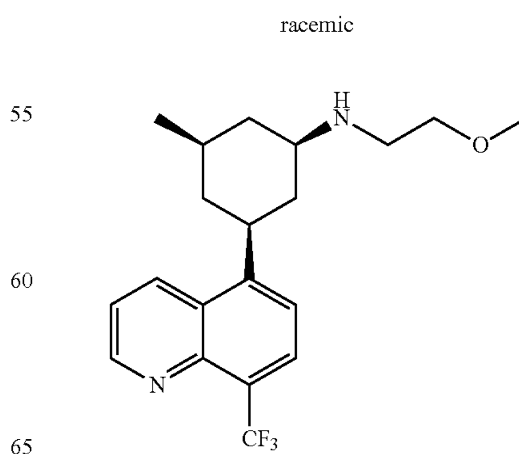
Compound 147
