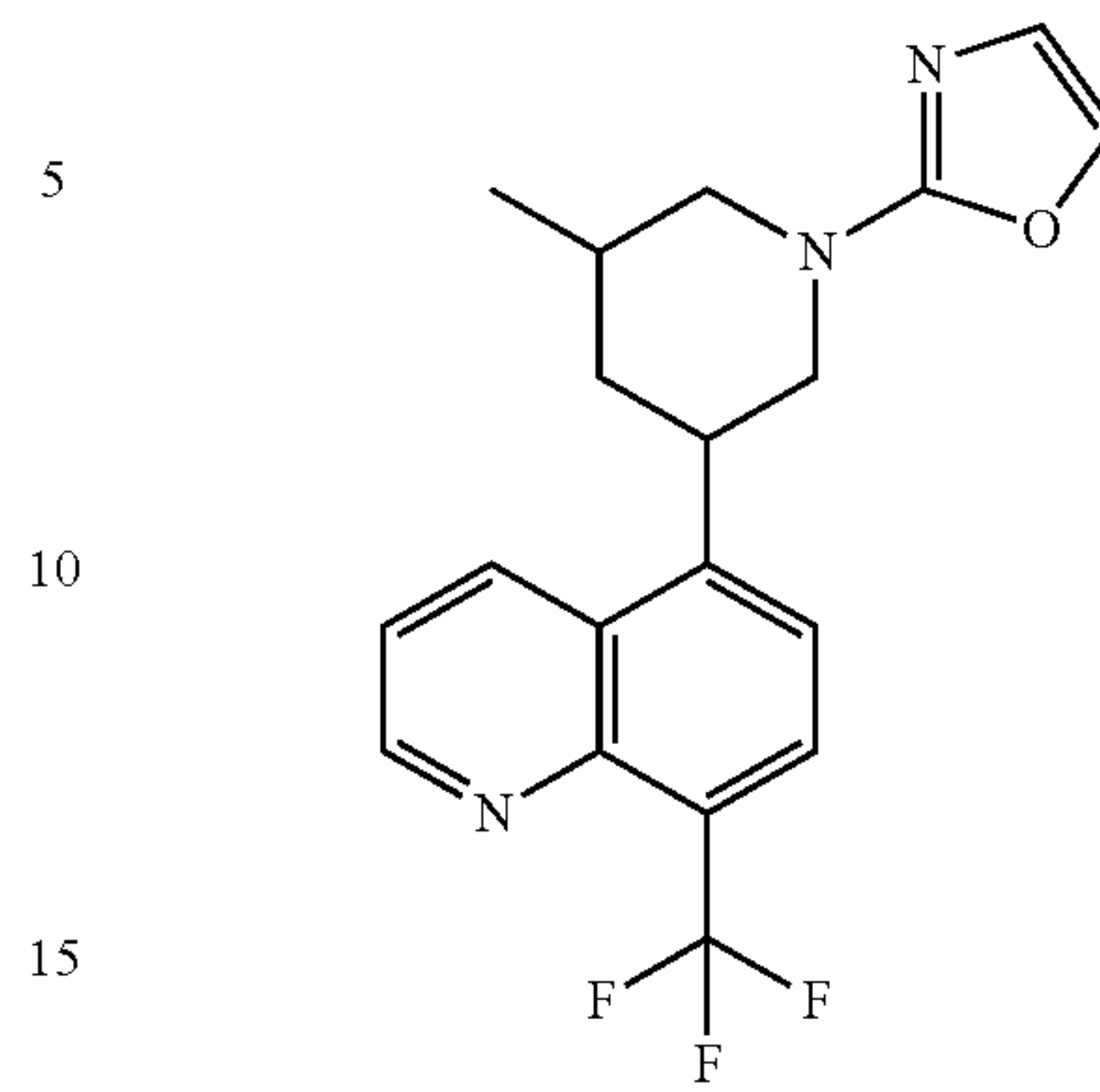
Compound 55
