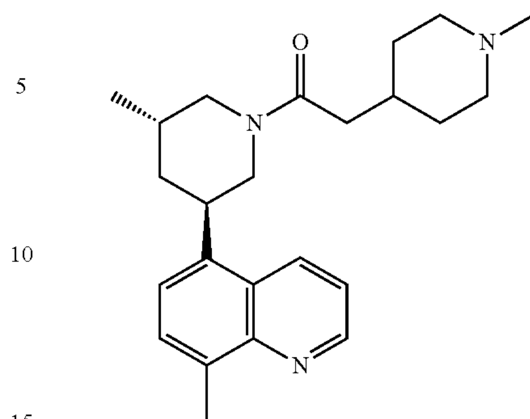
Compound 79
