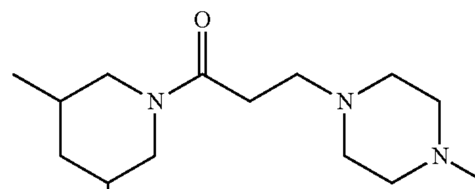
Compound 11
