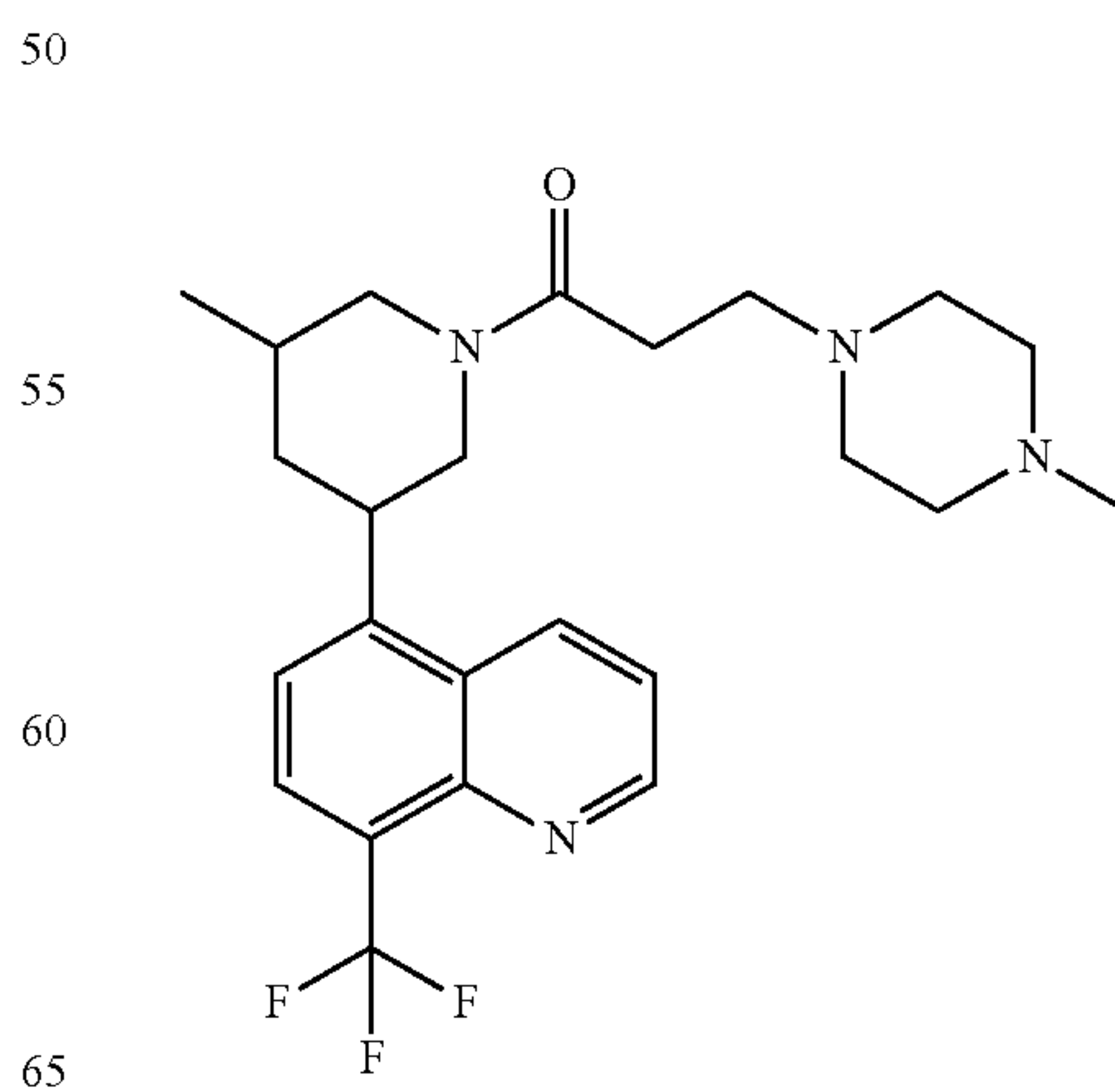
Compound 40
