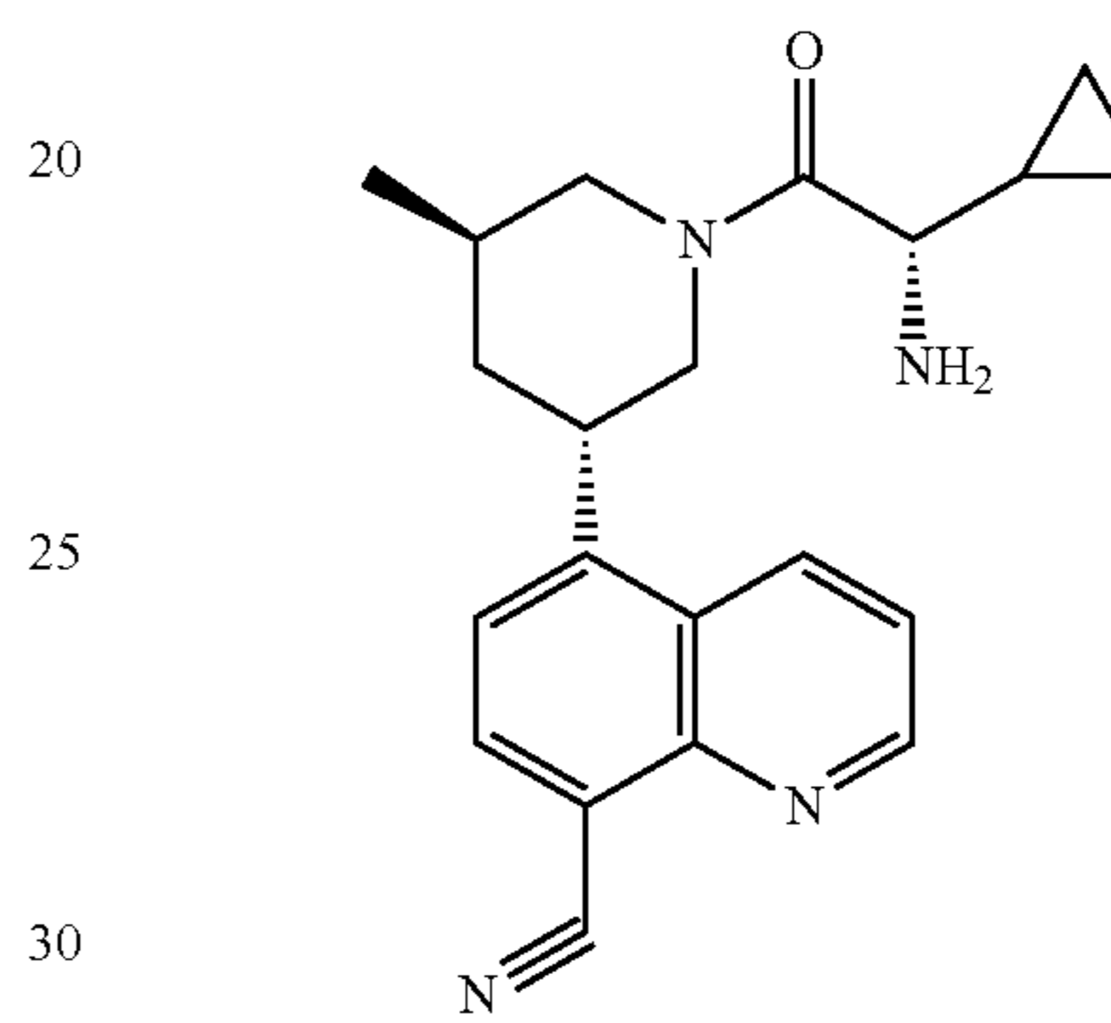
Compound 56
