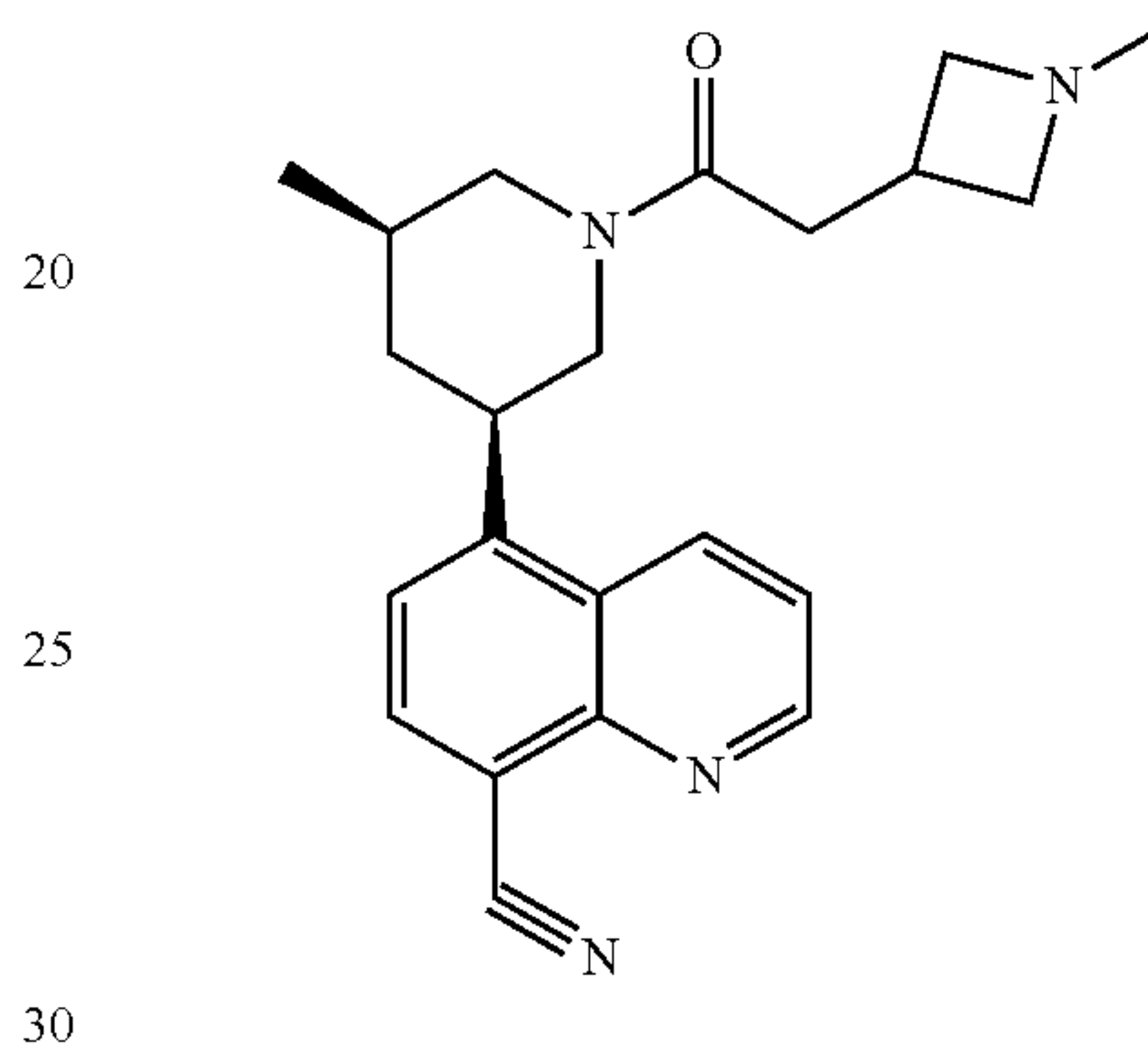
Compound 30
