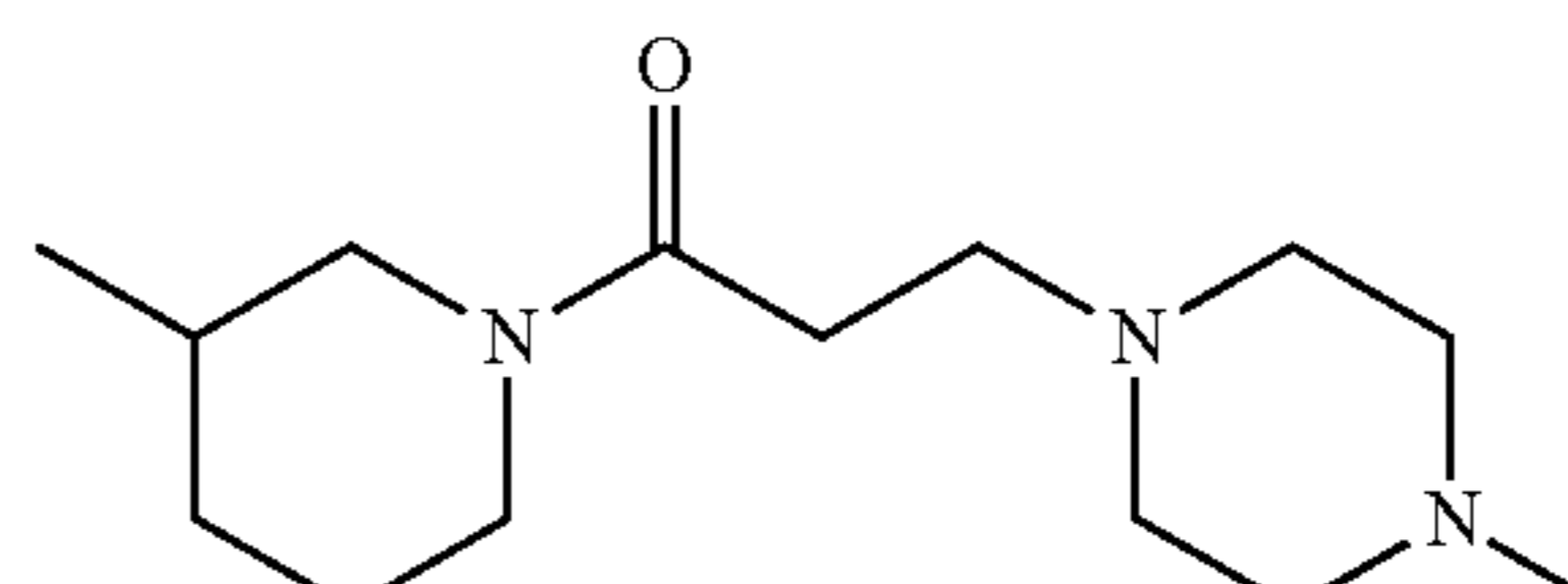
Compound 11
