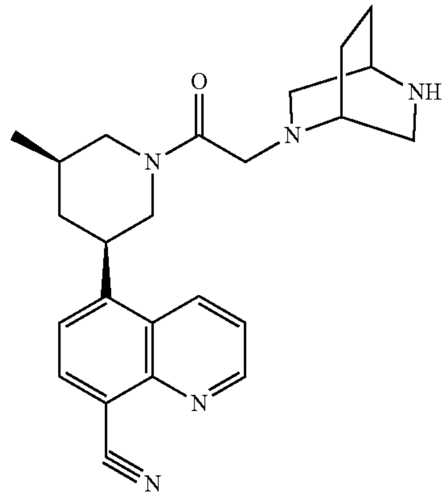
Compound 116
