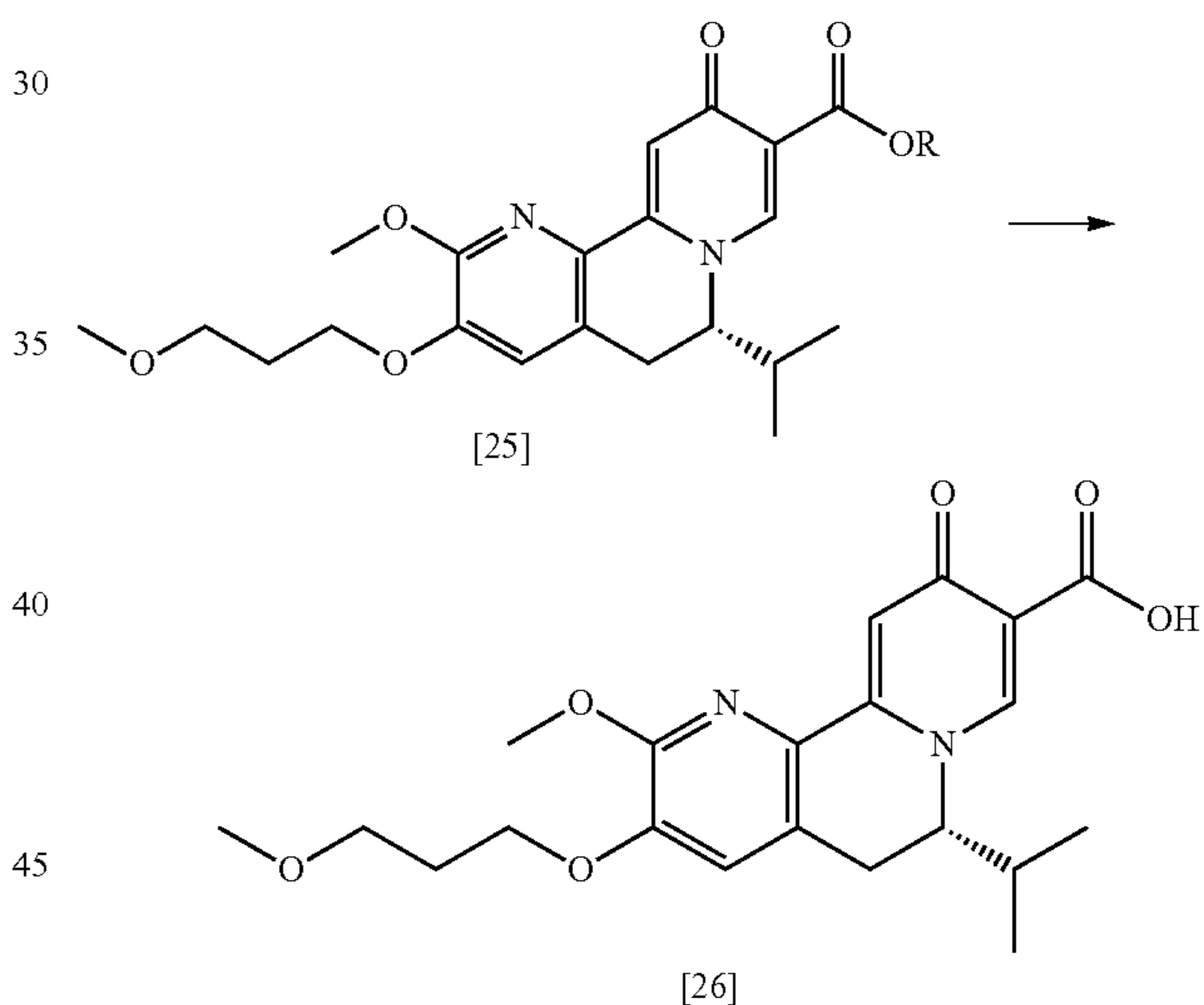
Scheme 1.
