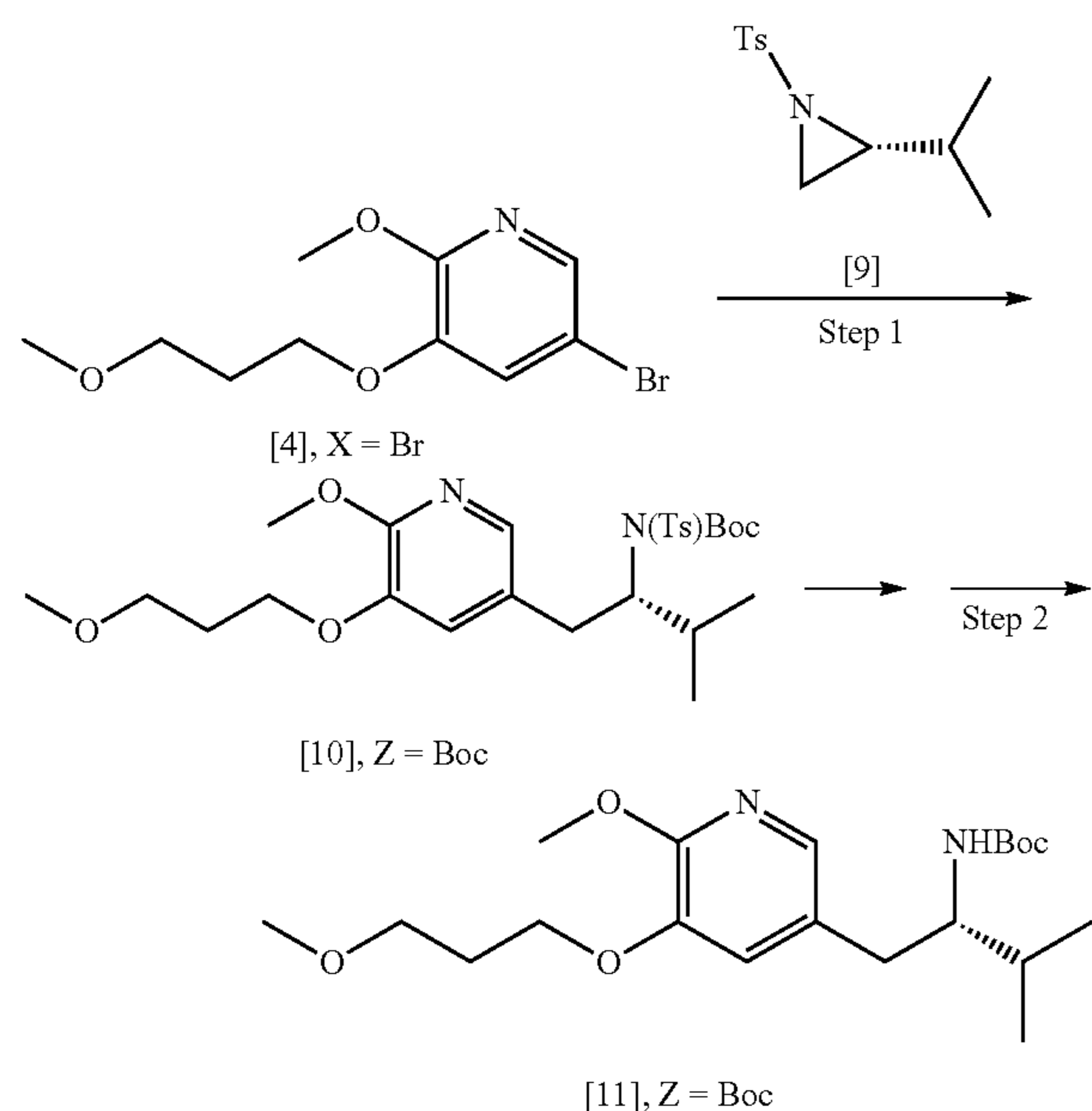
Scheme 15 (see also Scheme 5).
