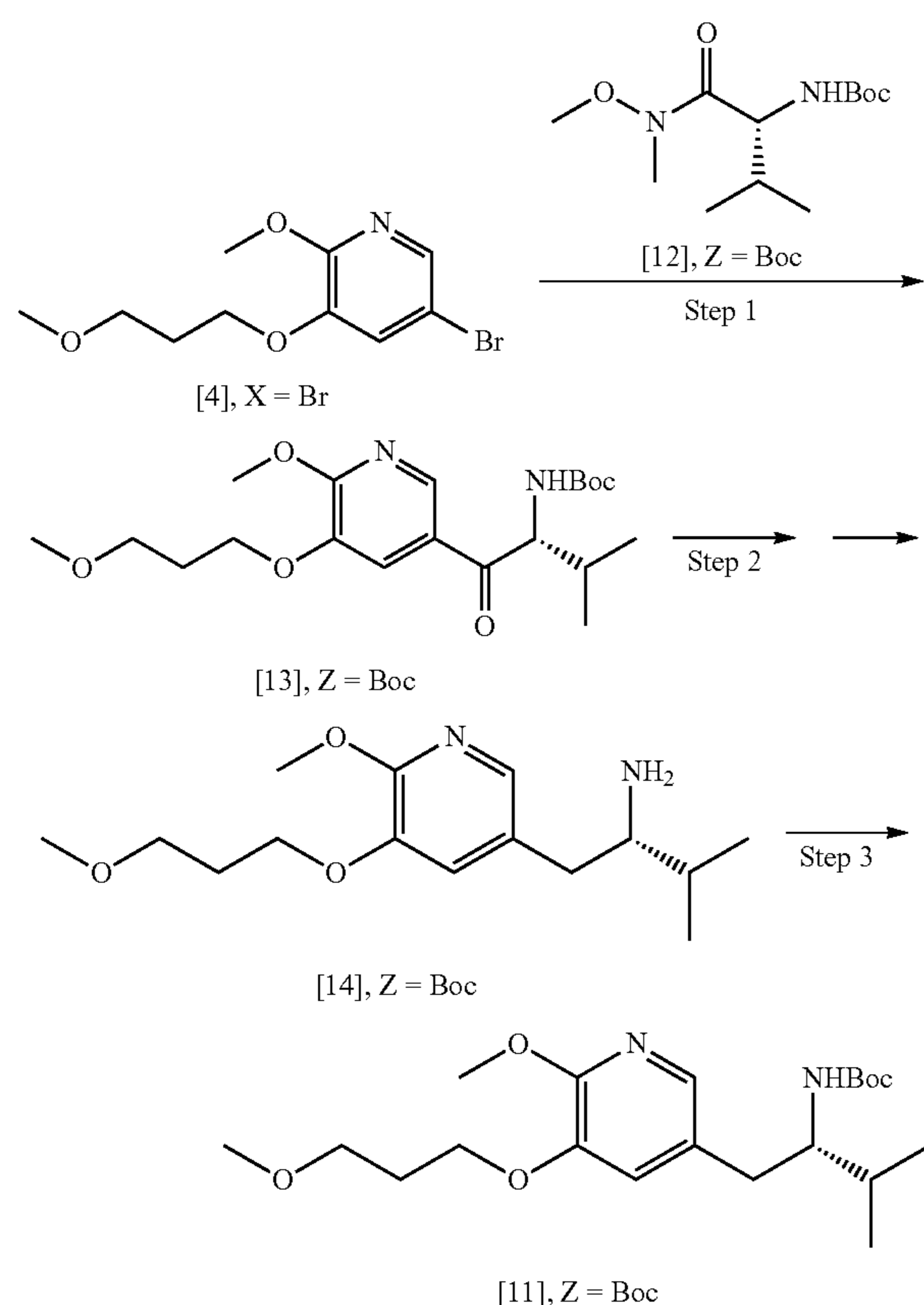
Scheme 16 (see also Scheme 6).
