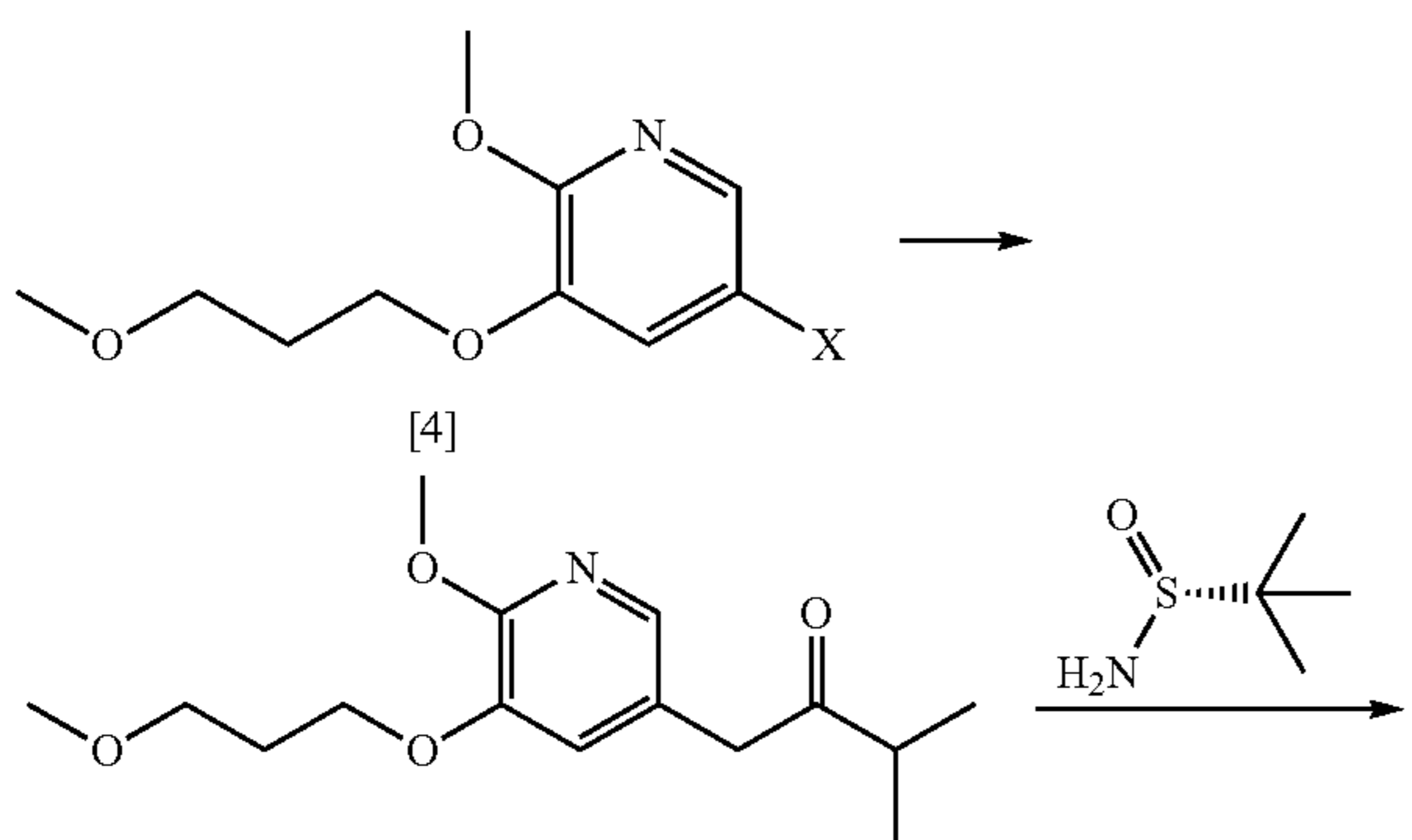
Scheme 8.
