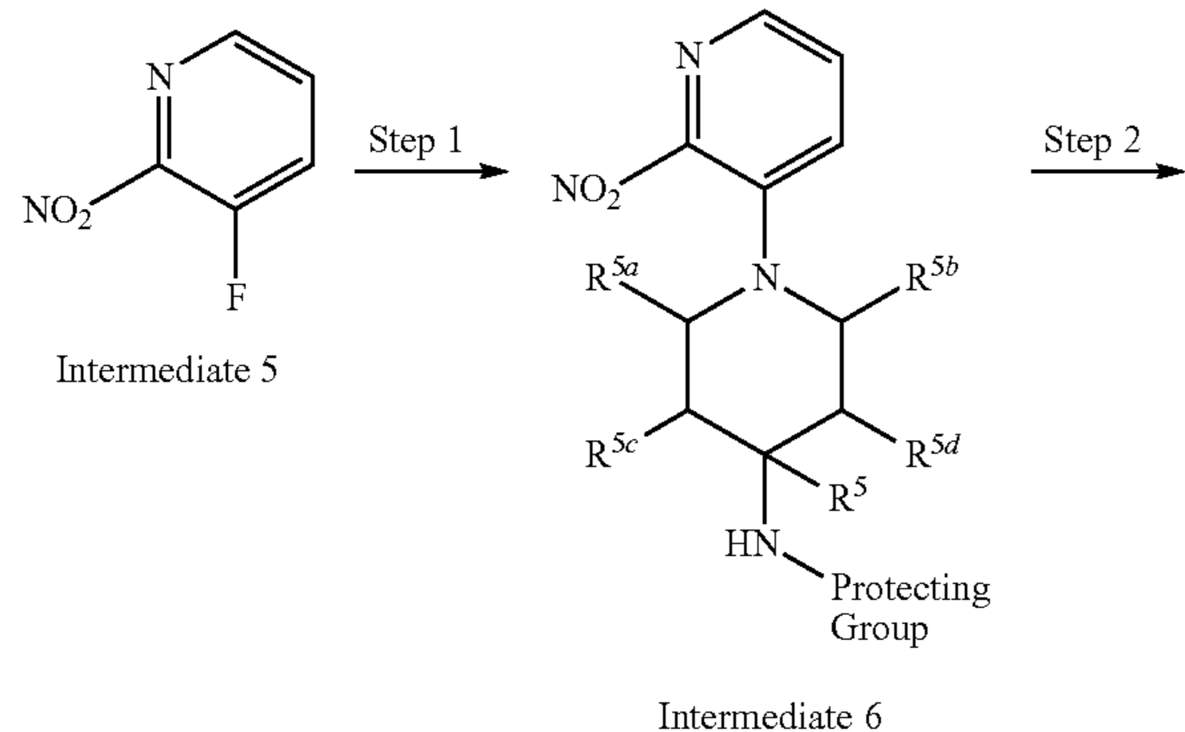
Scheme 3
