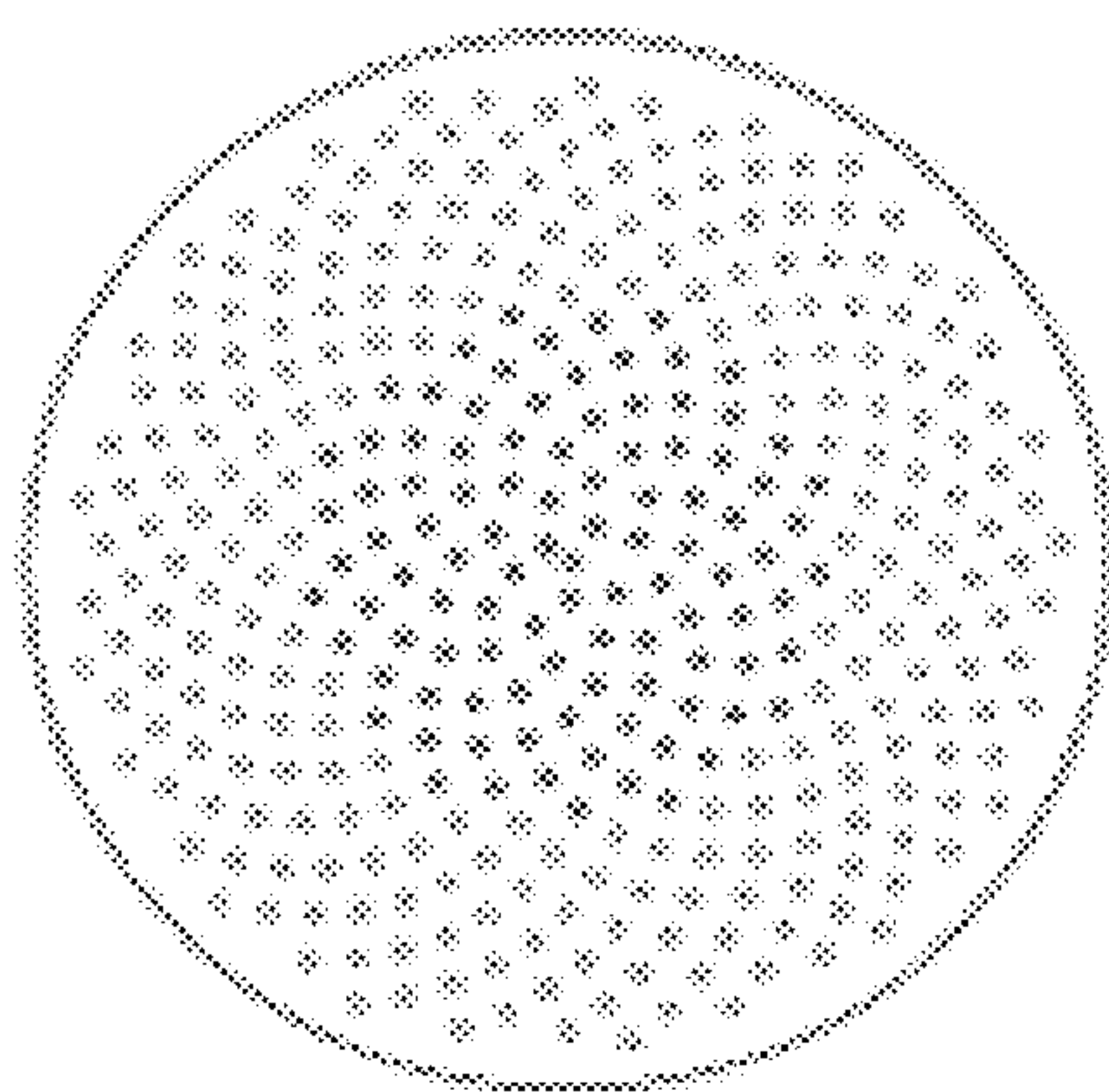
2.225 mm dia 350 holes 5" disc 10.7% removed area
