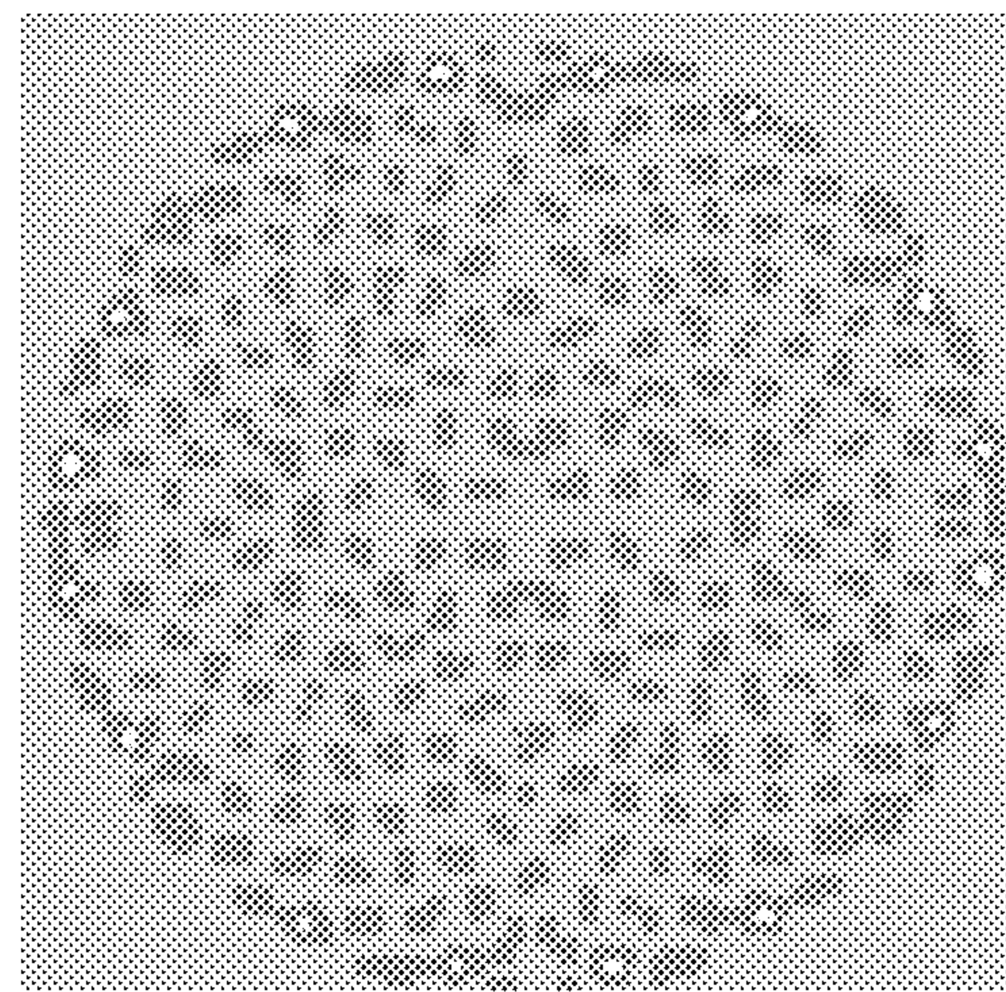
2.65 mm dia 250 holes 5" disc 10.8% removed area
