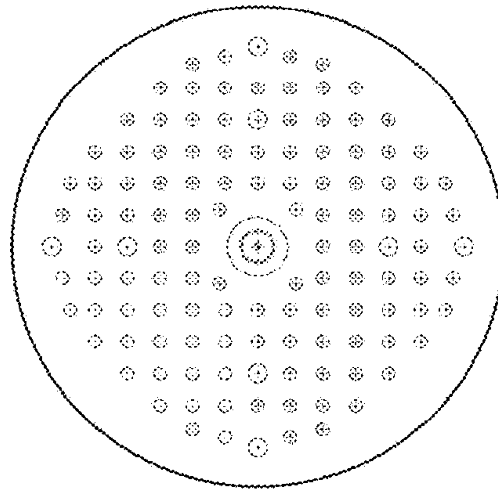
MultiAir 5" 125 holes 10.5% removed area
