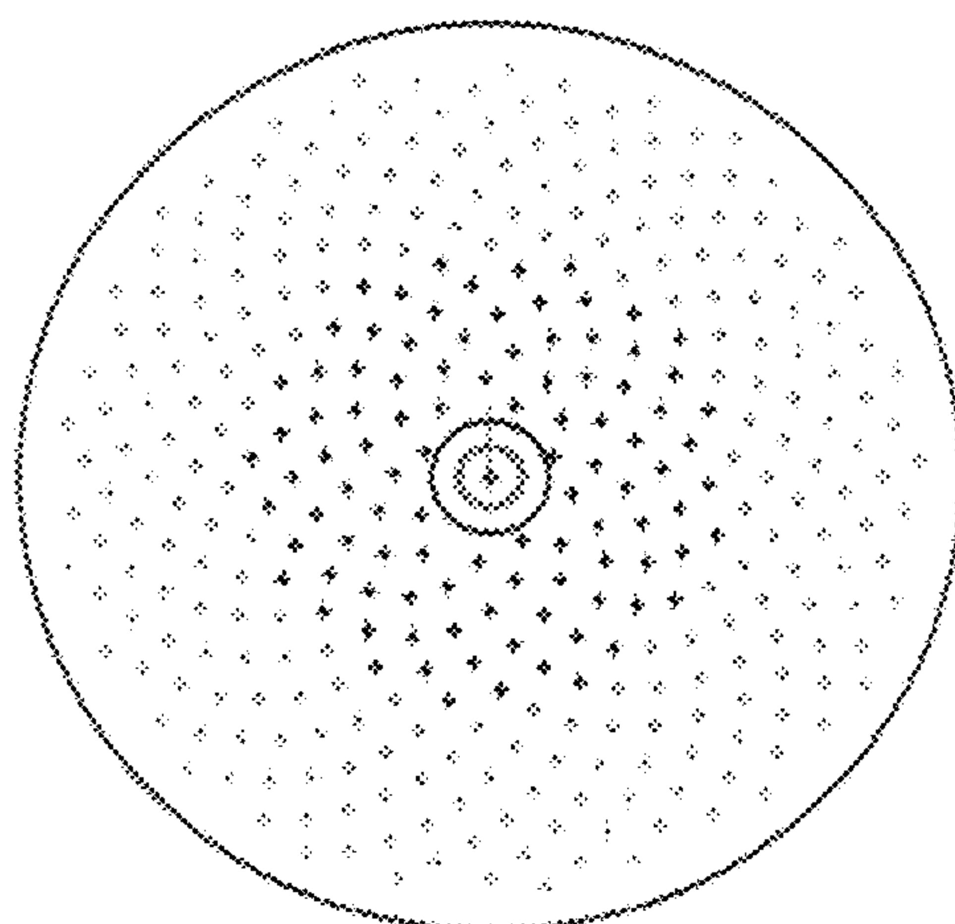
1.0 mm dia 344 holes 5" disc 3.7% removed area
