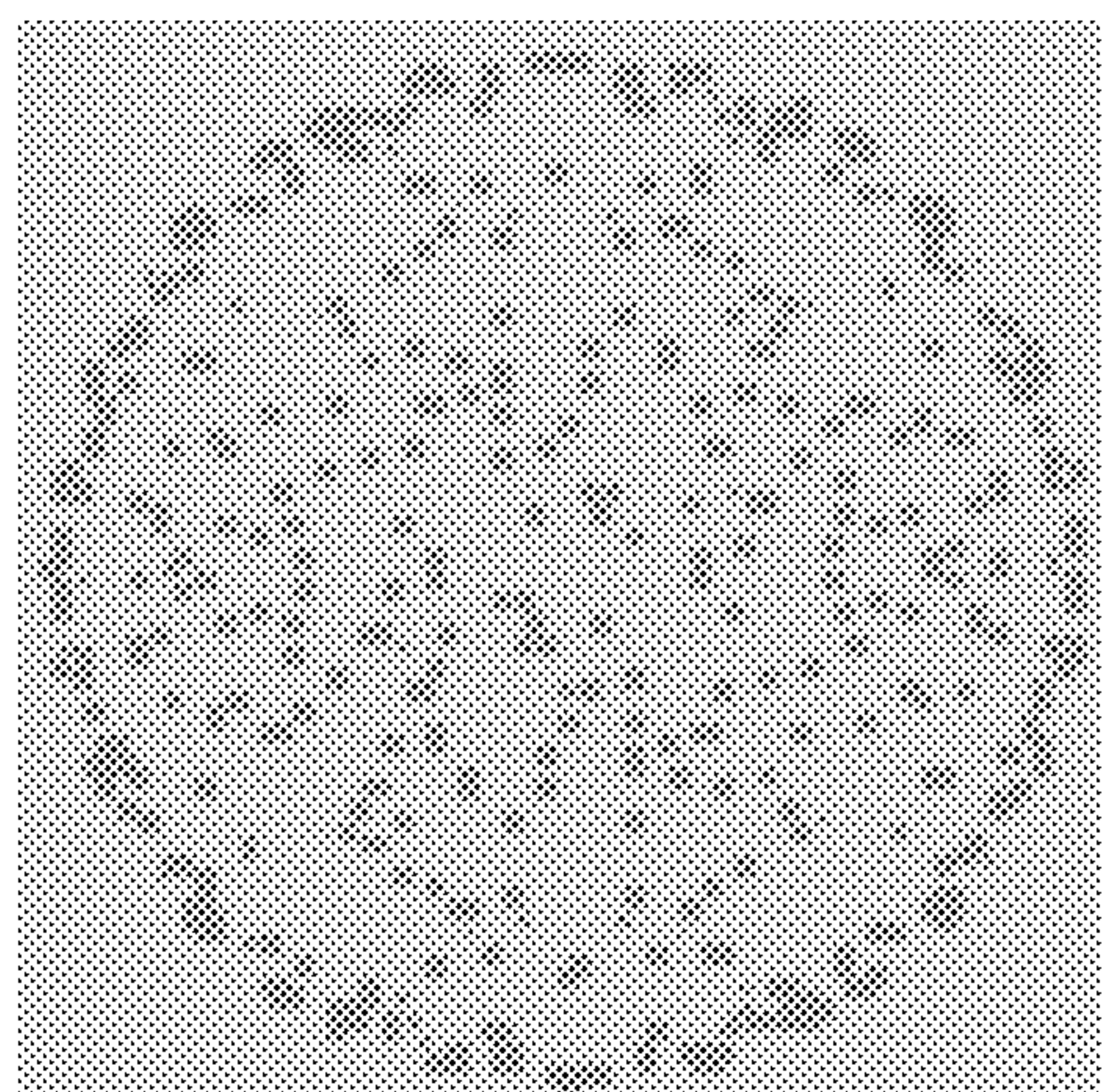
2.225 mm dia 350 holes 5" disc 10.7% removed area
