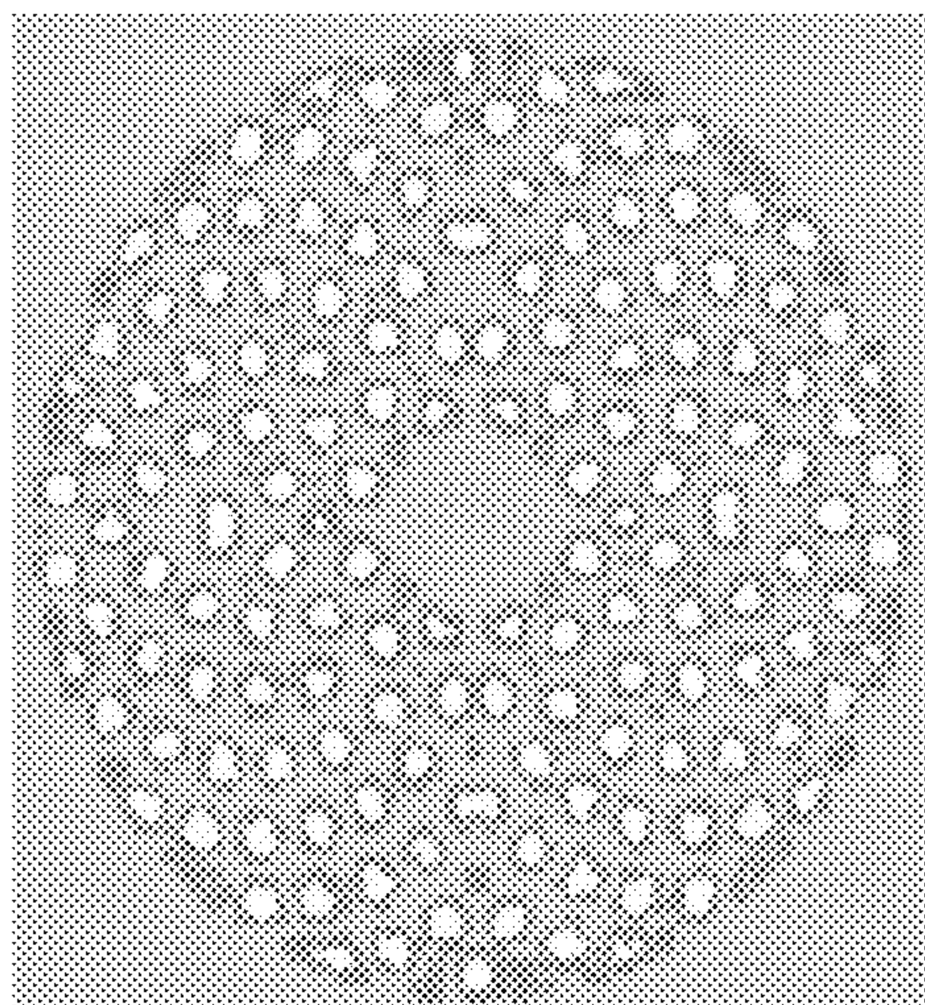
2.6 mm dia 148 holes 5" disc 7.8% removed area
