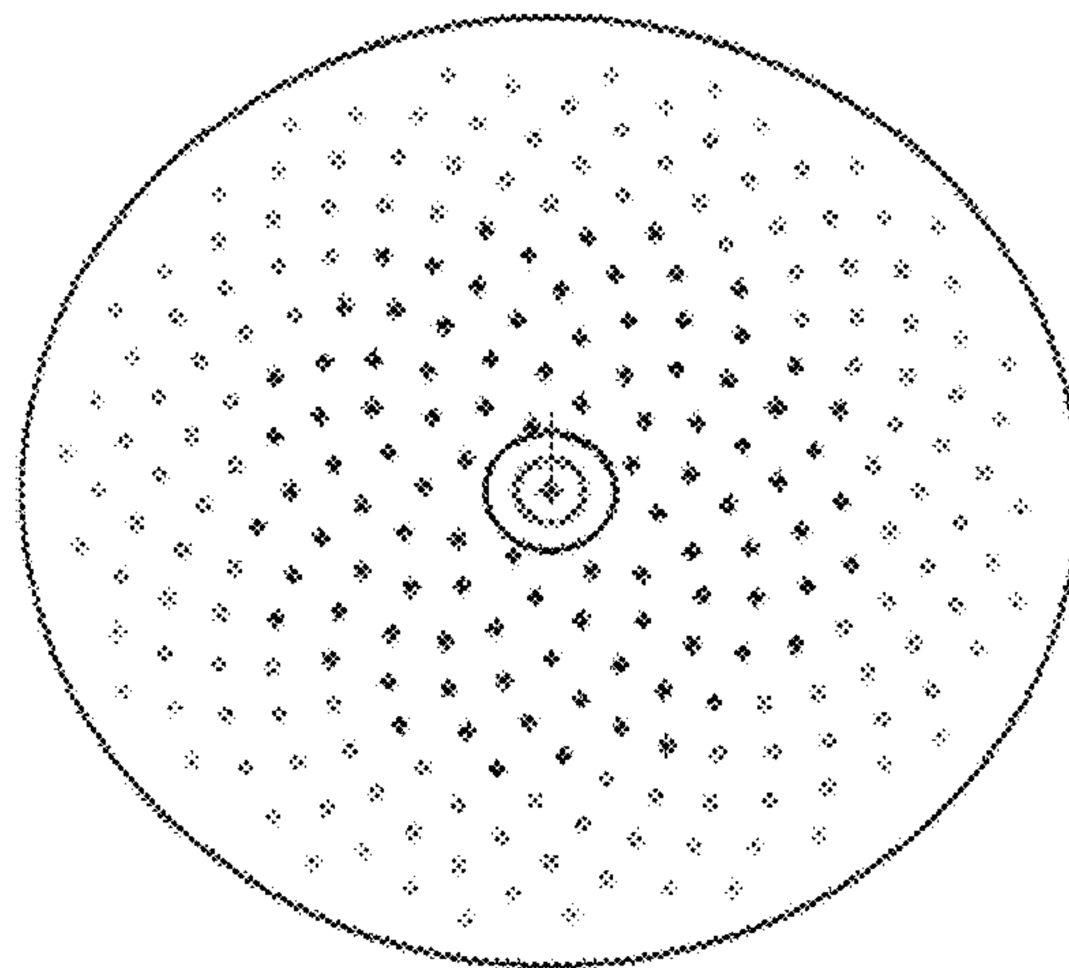
1.5 mm dia 248 holes 5" disc 5.0% removed area
