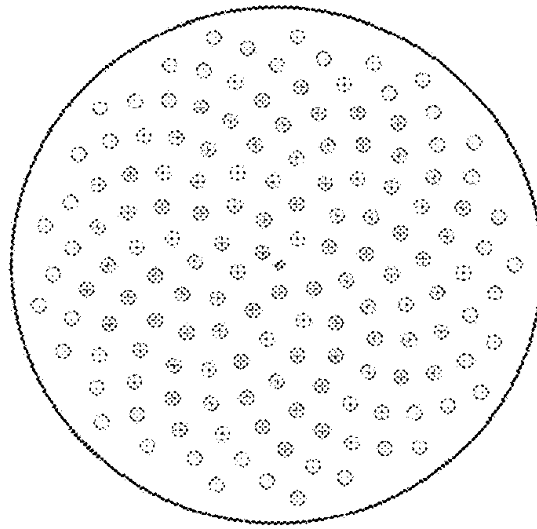
3.4 mm dia 160 holes 5" disc 10.7% removed area
