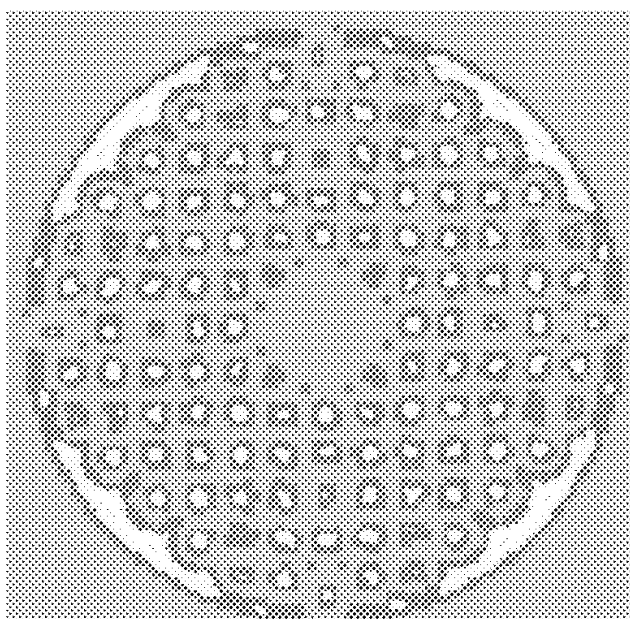
MultiAir 5" 125 holes 10.5% removed area
