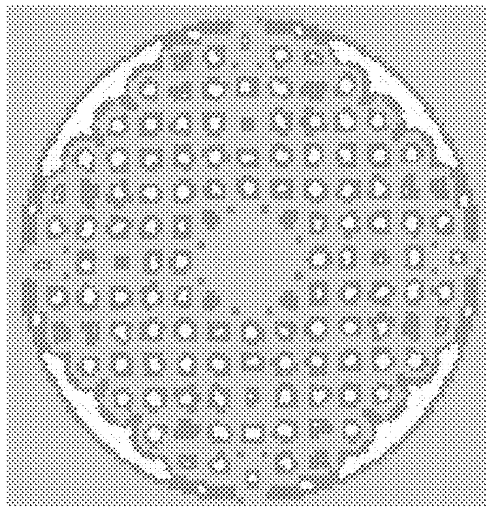
MultiAir 5" 125 holes 10.5% removed area
