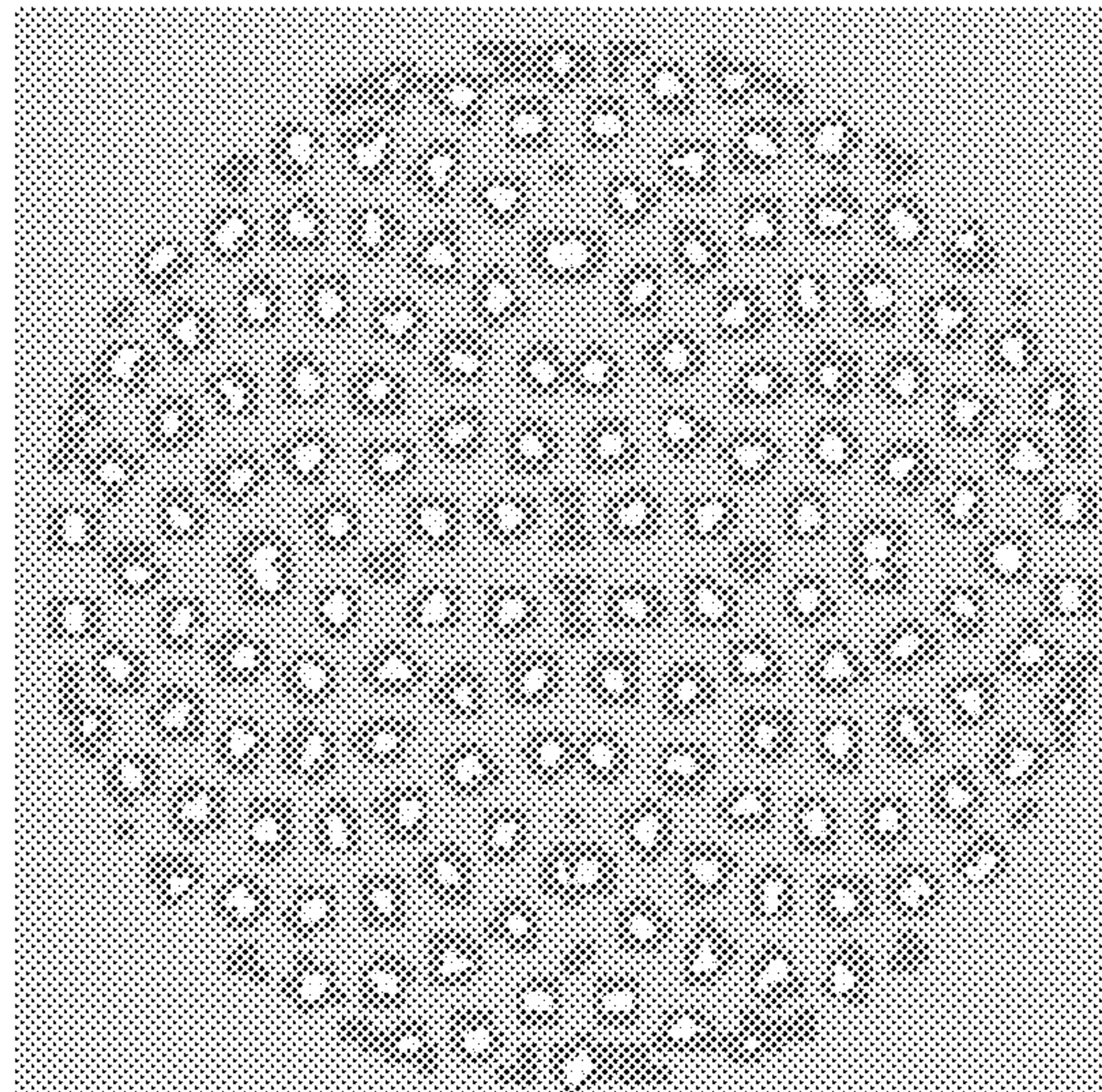
3.4 mm dia 160 holes 5" disc 10.7% removed area
