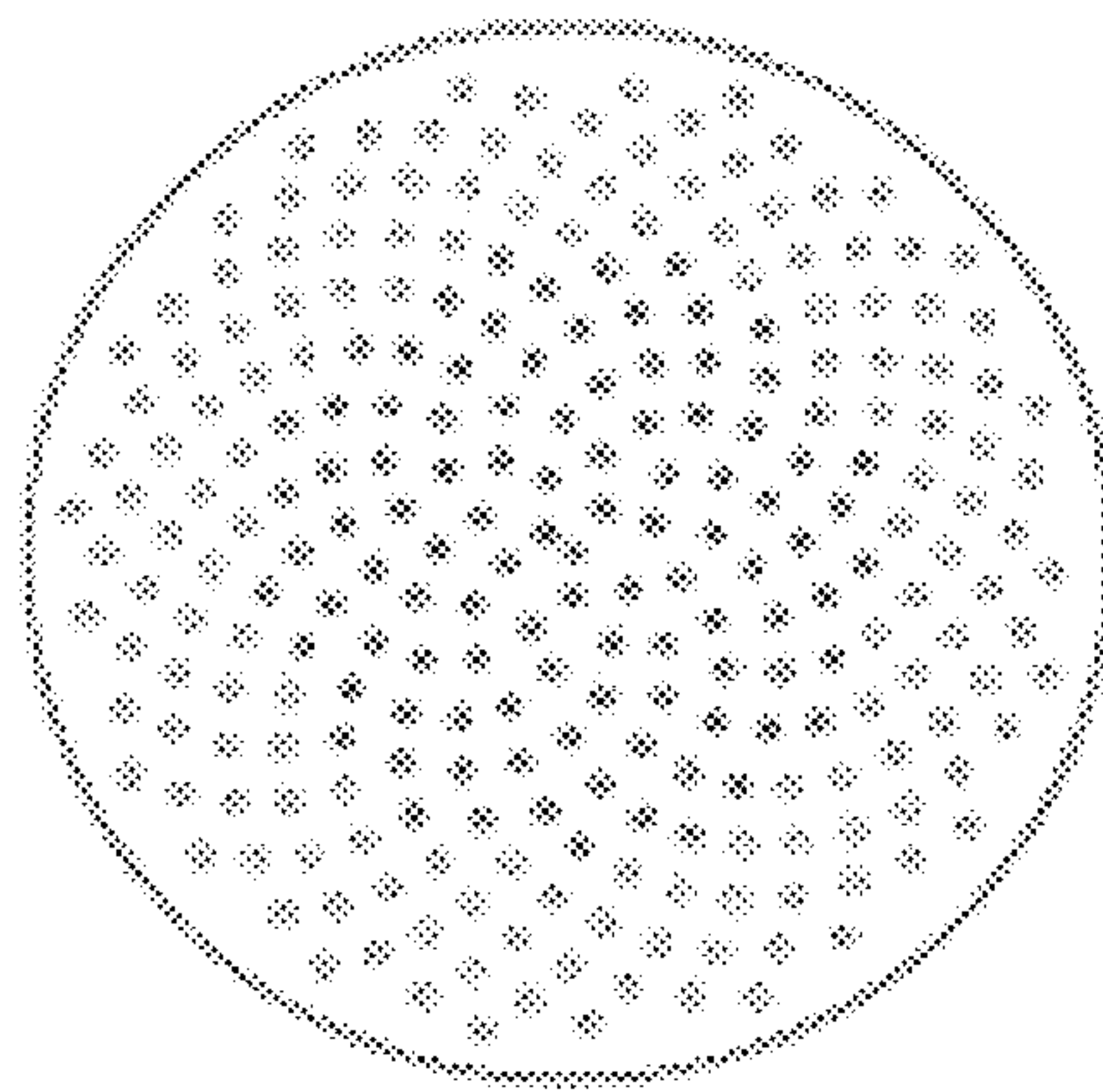
2.65 mm dia 250 holes 5" disc 10.8% removed area
