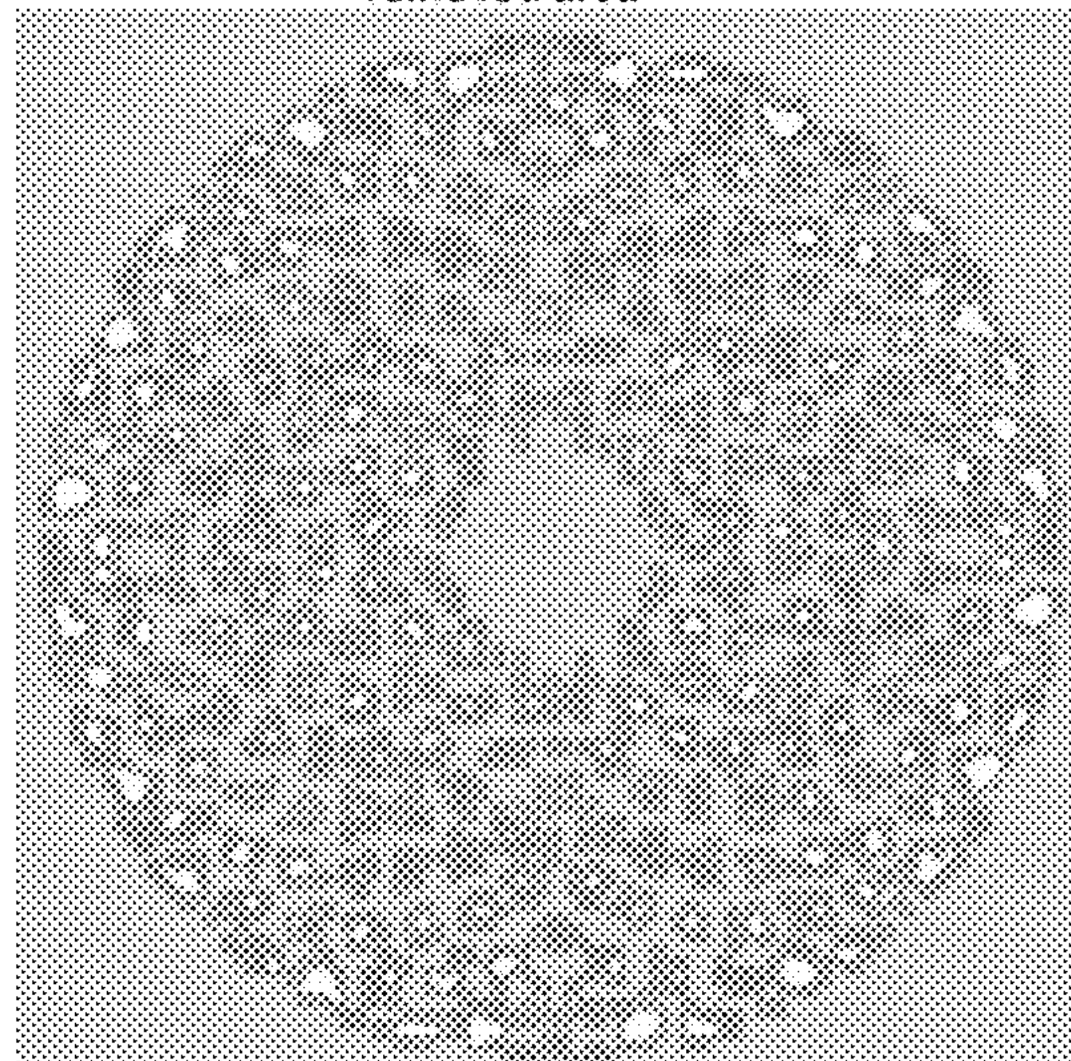
1.5 mm dia 248 holes 5" disc 5.0% removed area
