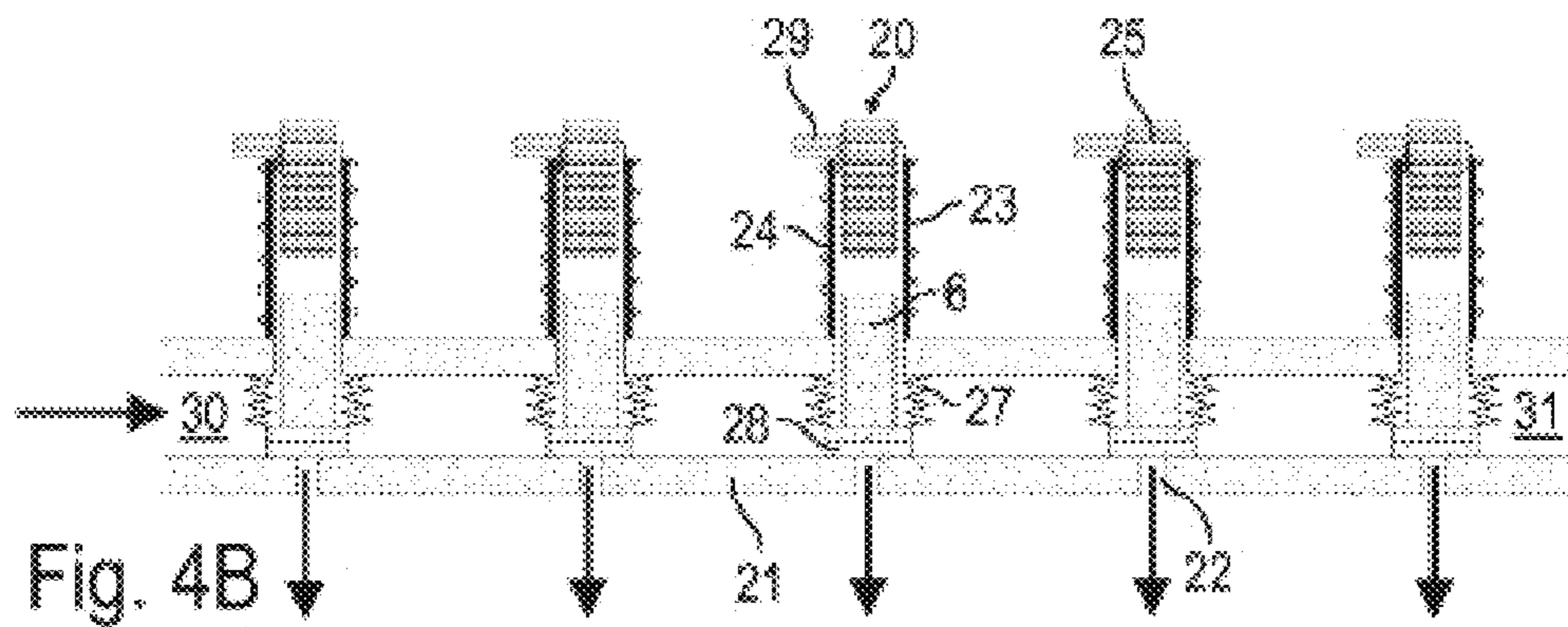
Rinsing through nozzles
