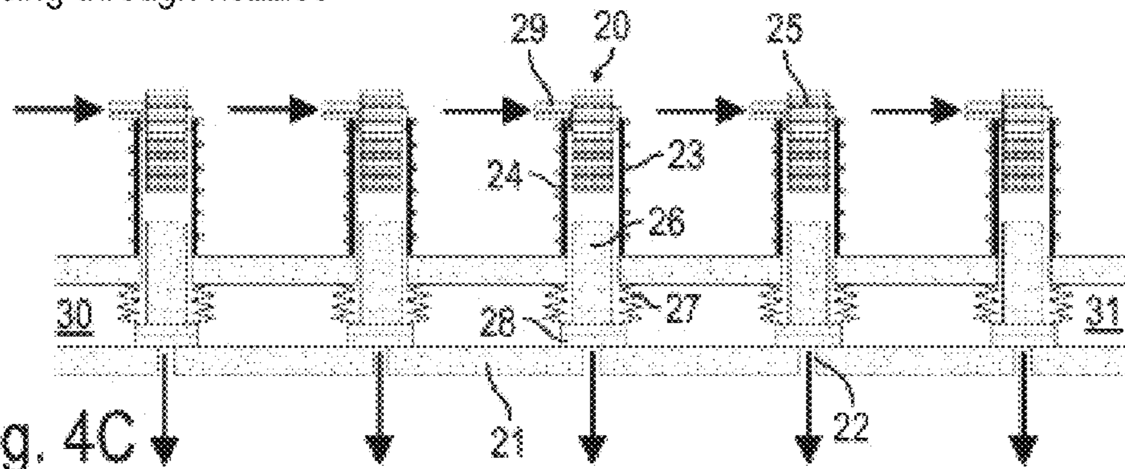
Rinsing through coil tube
