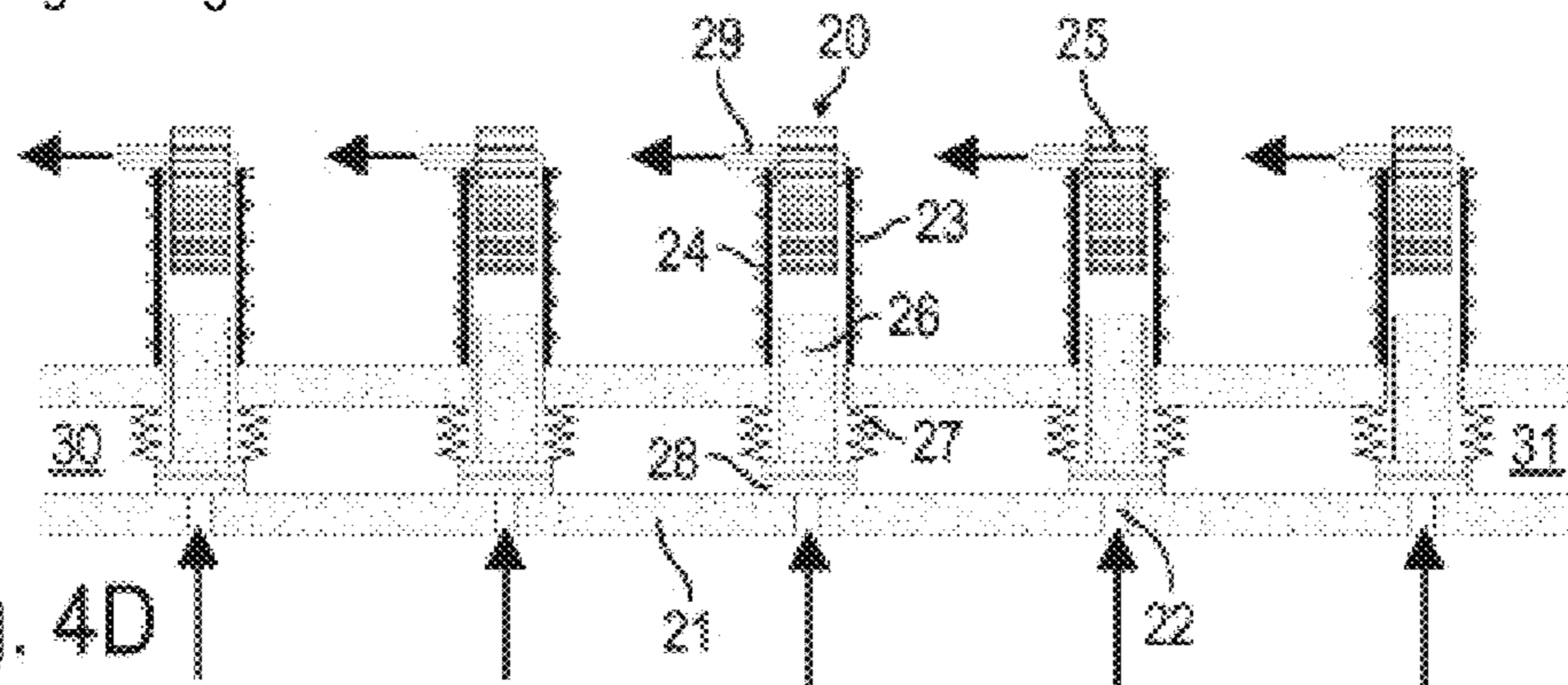
Rinsing back through nozzles
