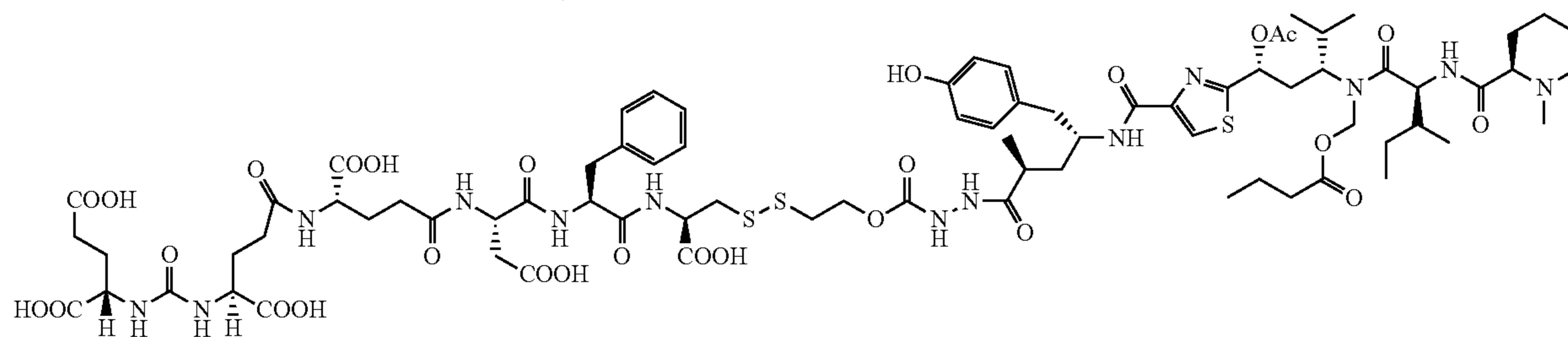
PC01SK71 C_{77}H_{109}N_{13}O_{26}S_3 Mol. Wt.: 1760.95
