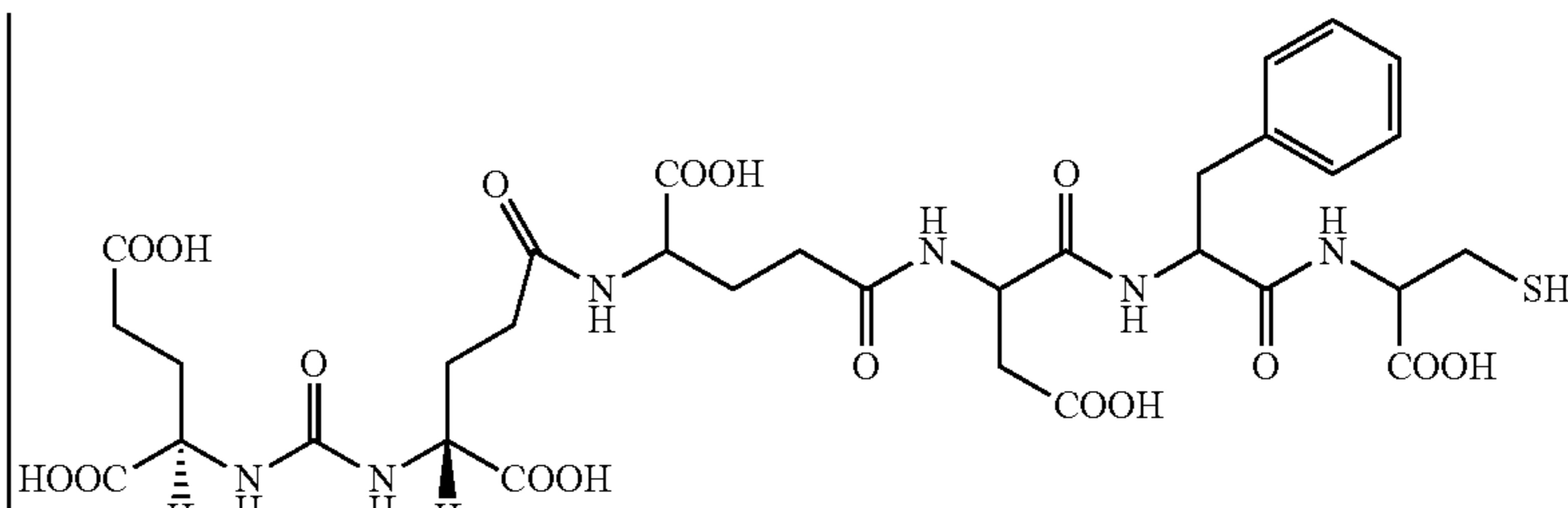
PC01SK68 C_{32}H_{42}N_6O_{17}S Mol. Wt.: 814.77
