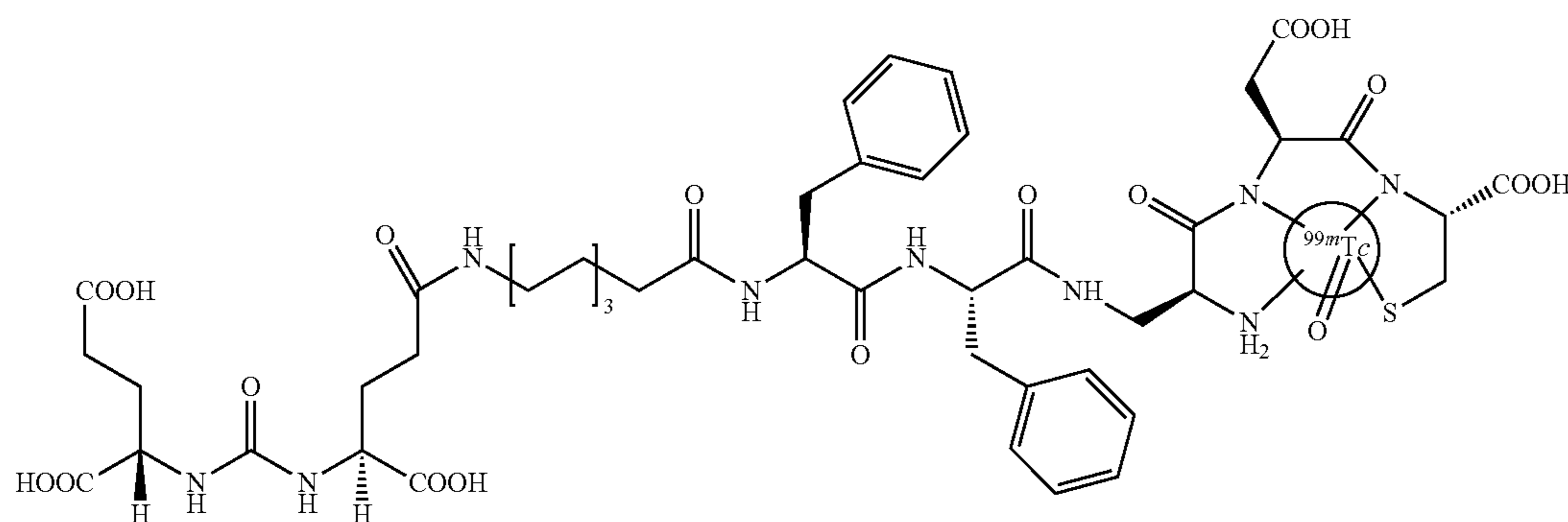
anti-PC01SK33
