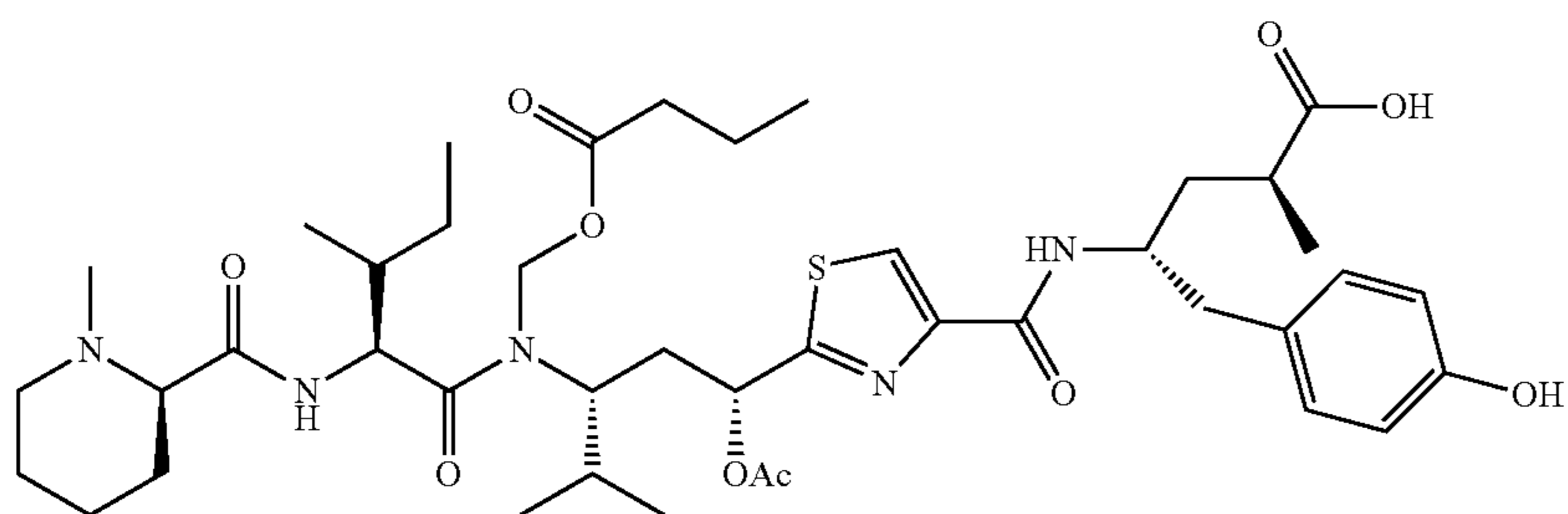
Tubulysin B C_{42}H_{63}N_5O_{10}S Mol. Wt.: 830.04
