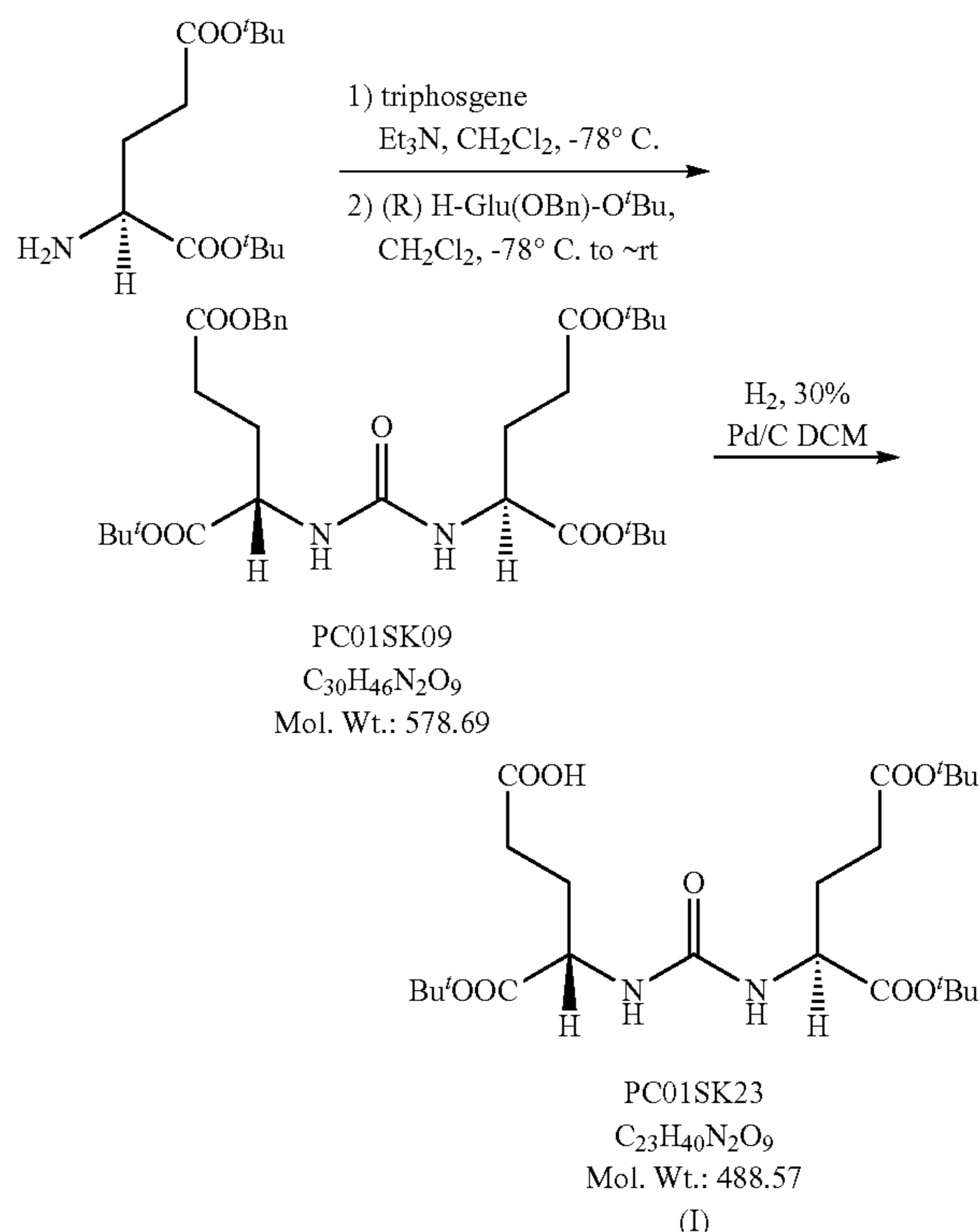
Scheme 2.1
