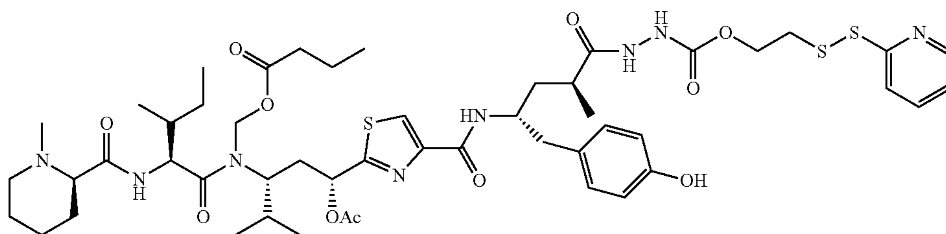
EC0312 C_{50}H_{72}N_8O_{11}S_3 Mol. Wt.: 1057.35
