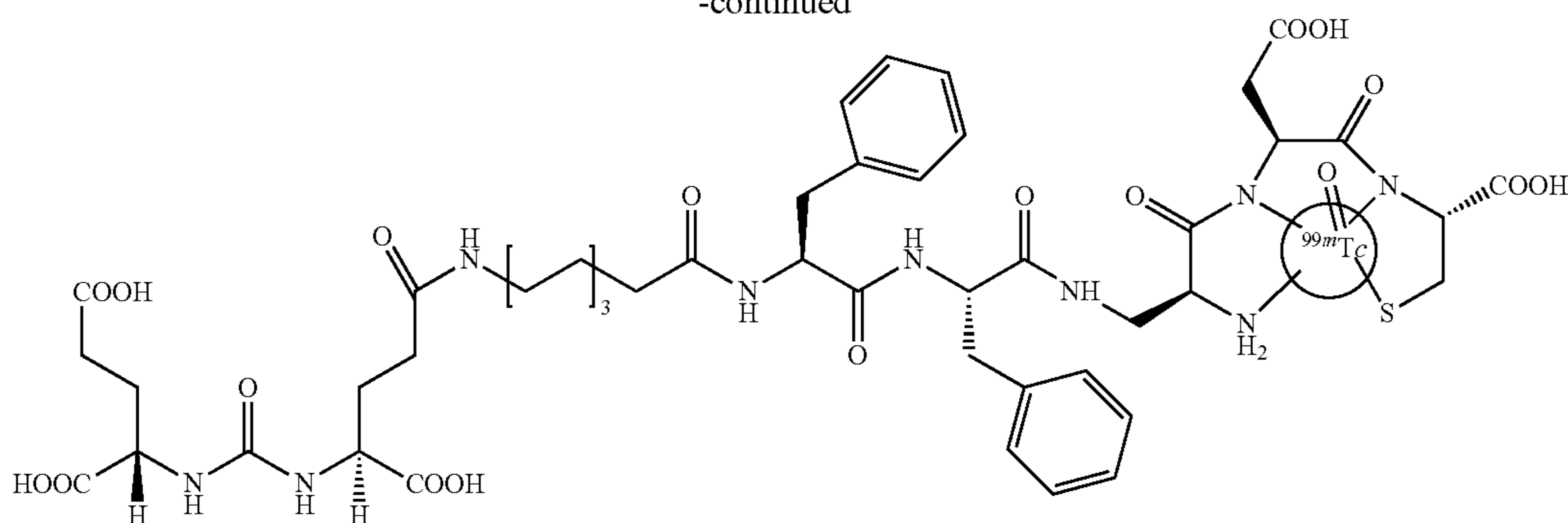
syn-PC01SK33
