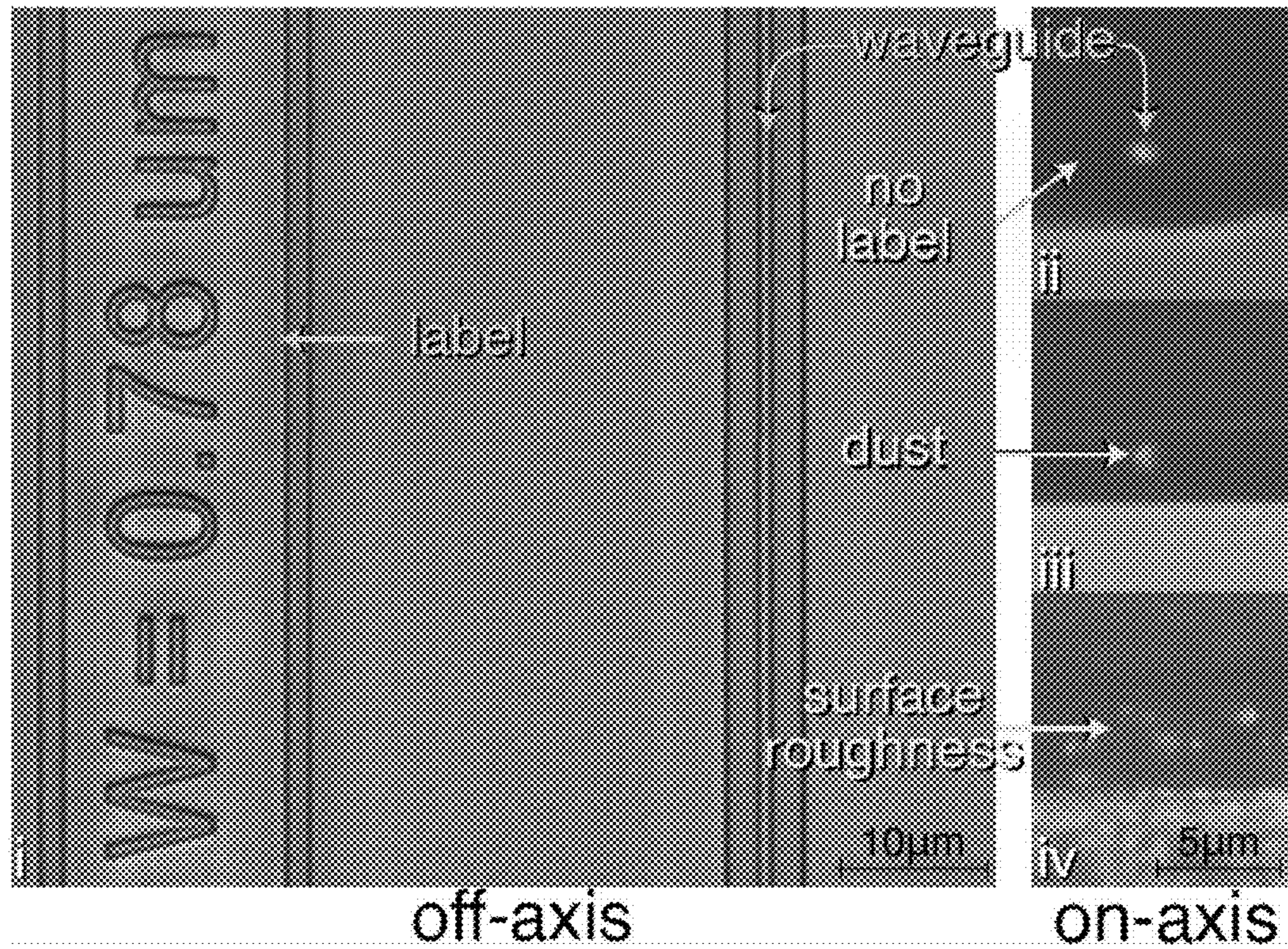
(a) Conventional photonic chip without barcode
