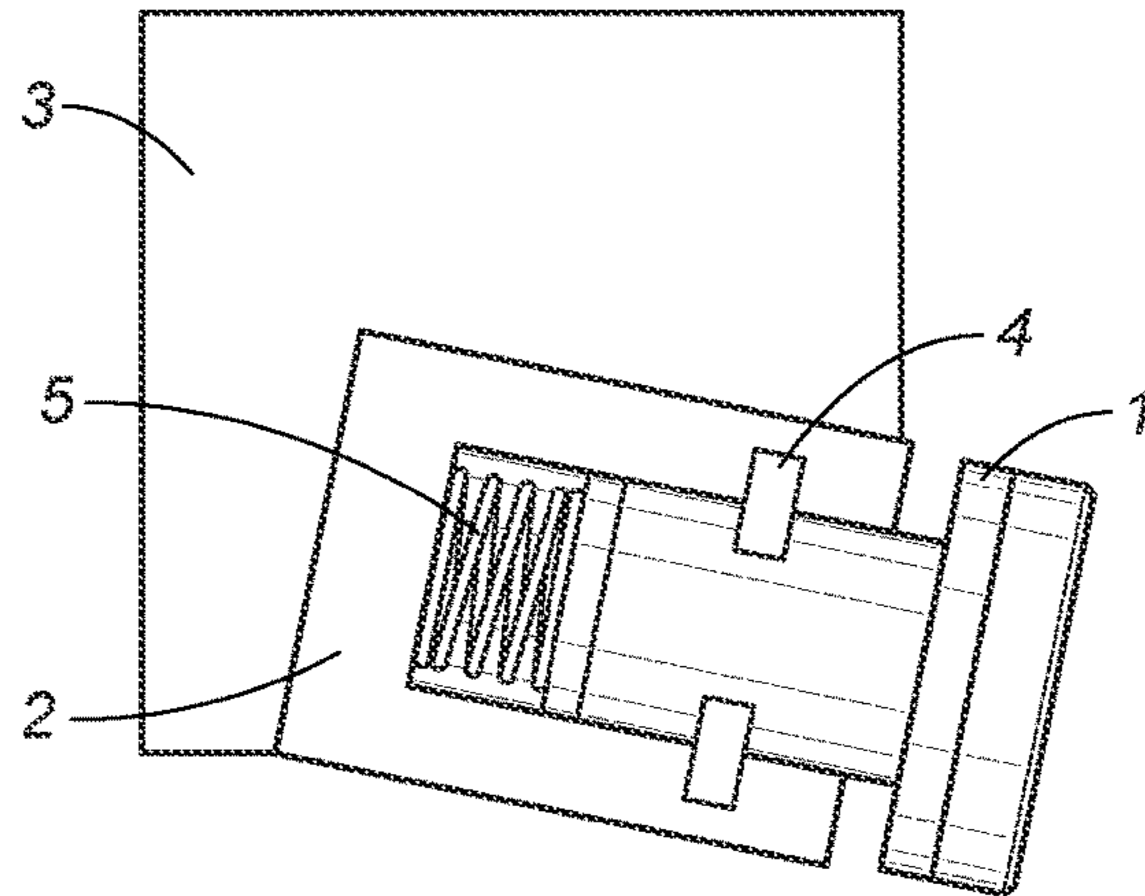
FIG. 1 Prior Art
