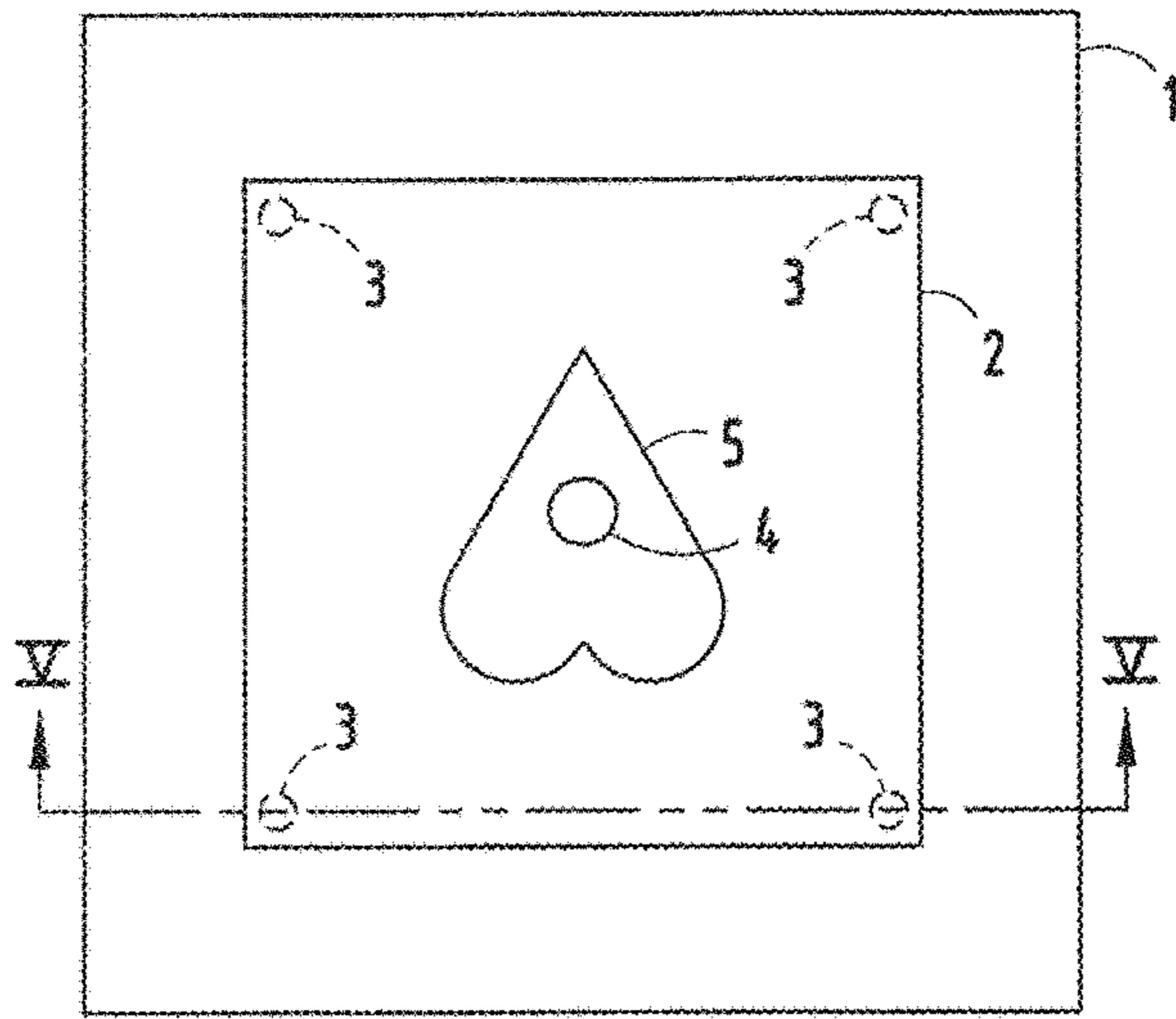
FIG. 4 PRIOR ART
