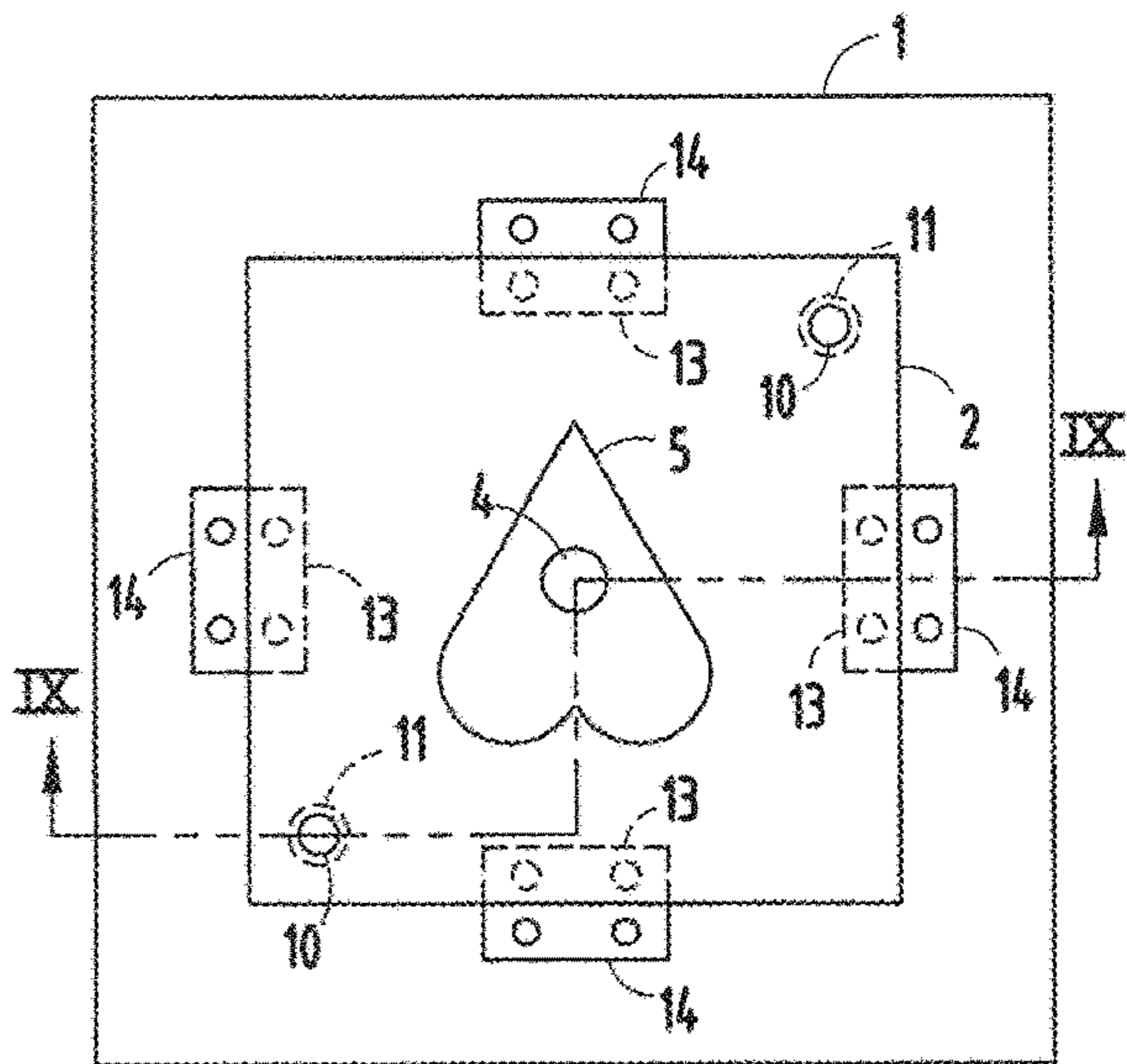
FIG. 8 PRIOR ART
