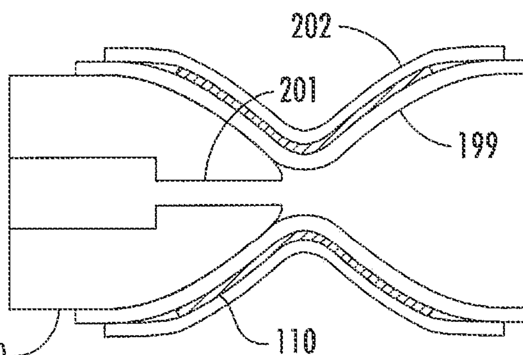
FIG. 13D
