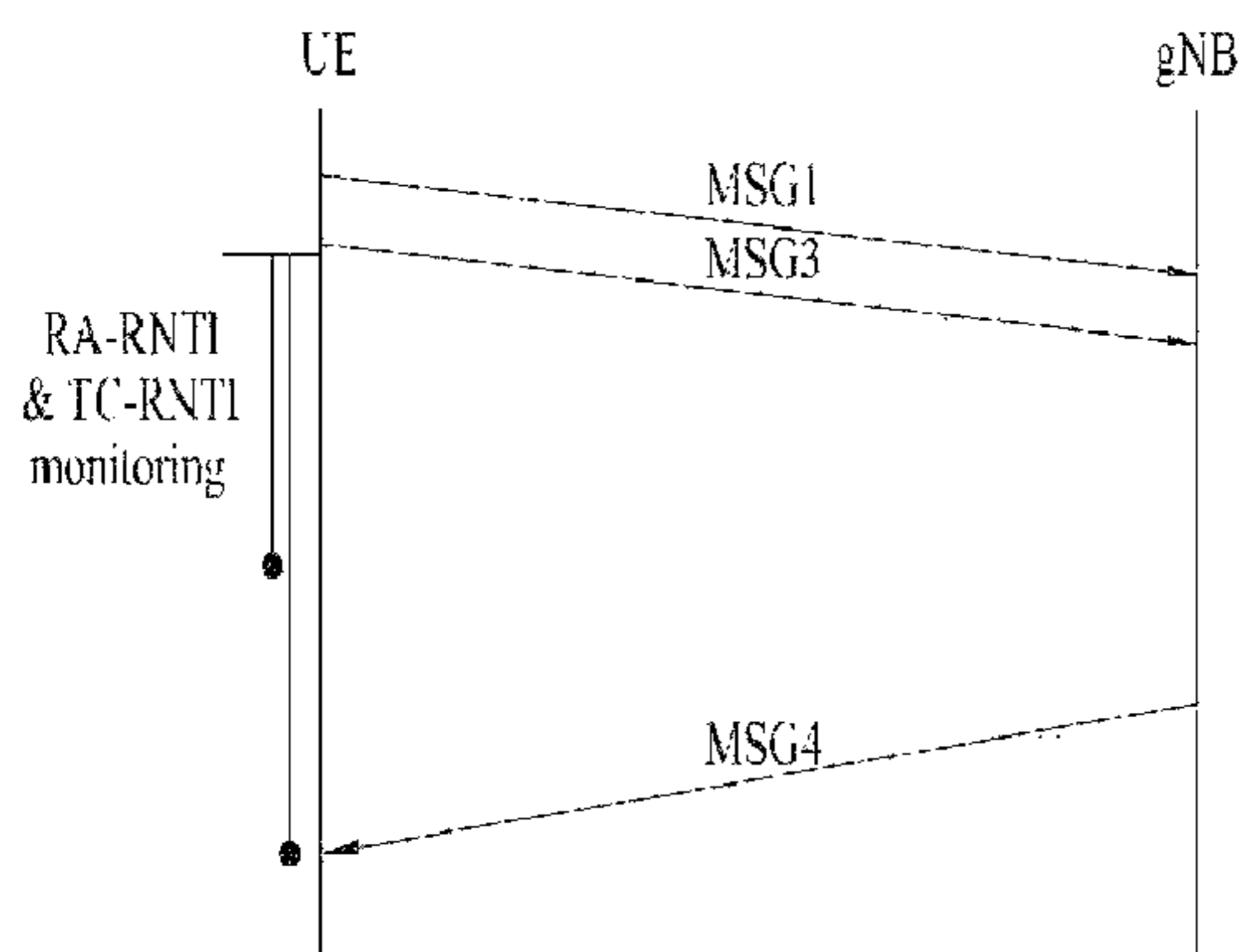
(a) successful reception of MSG3
