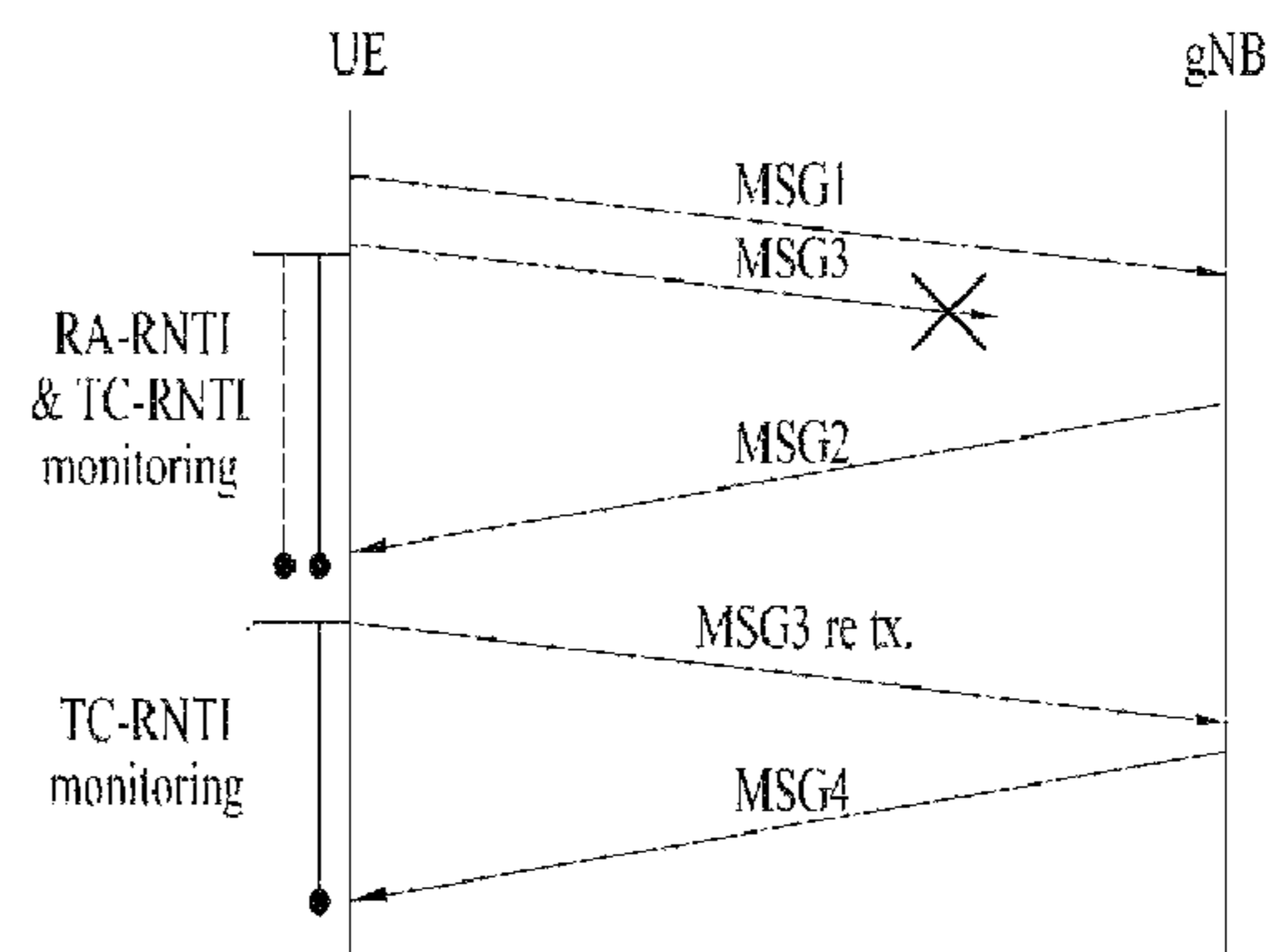
(b) unsuccessful reception of MSG3
