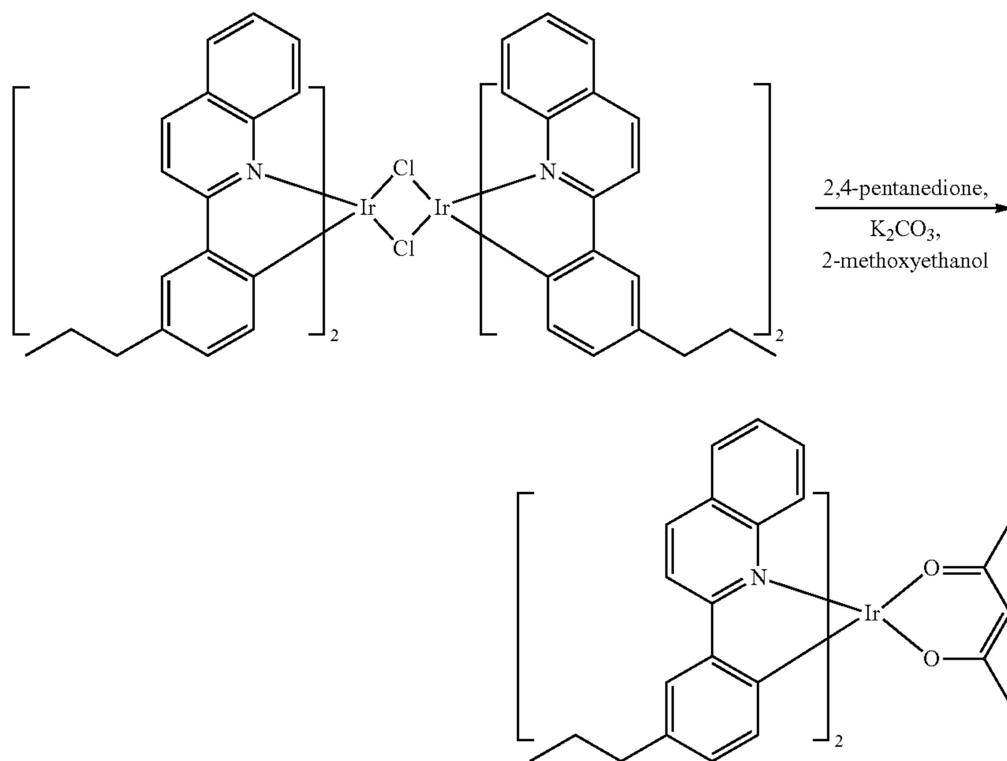
Compound 21
