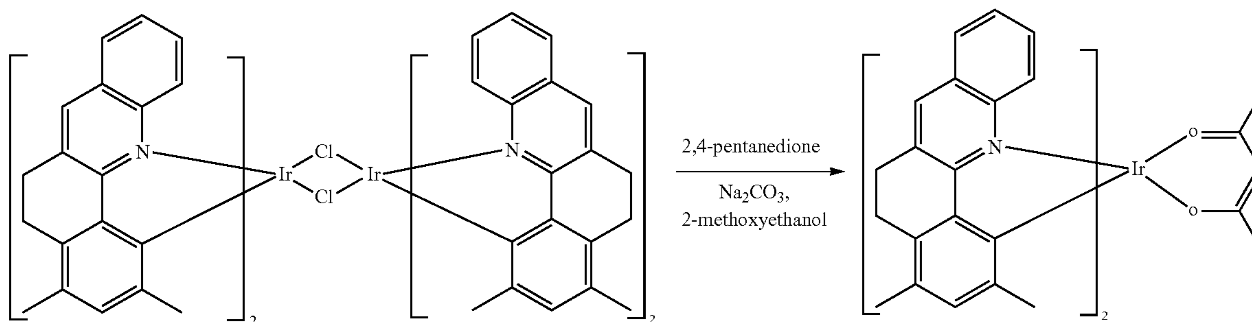
Compound 19
