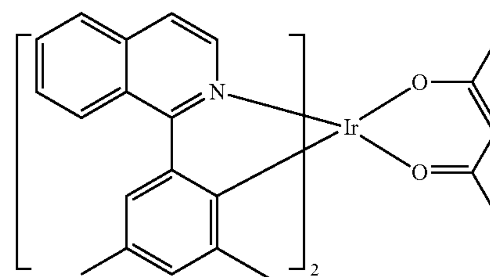
Compound 22
