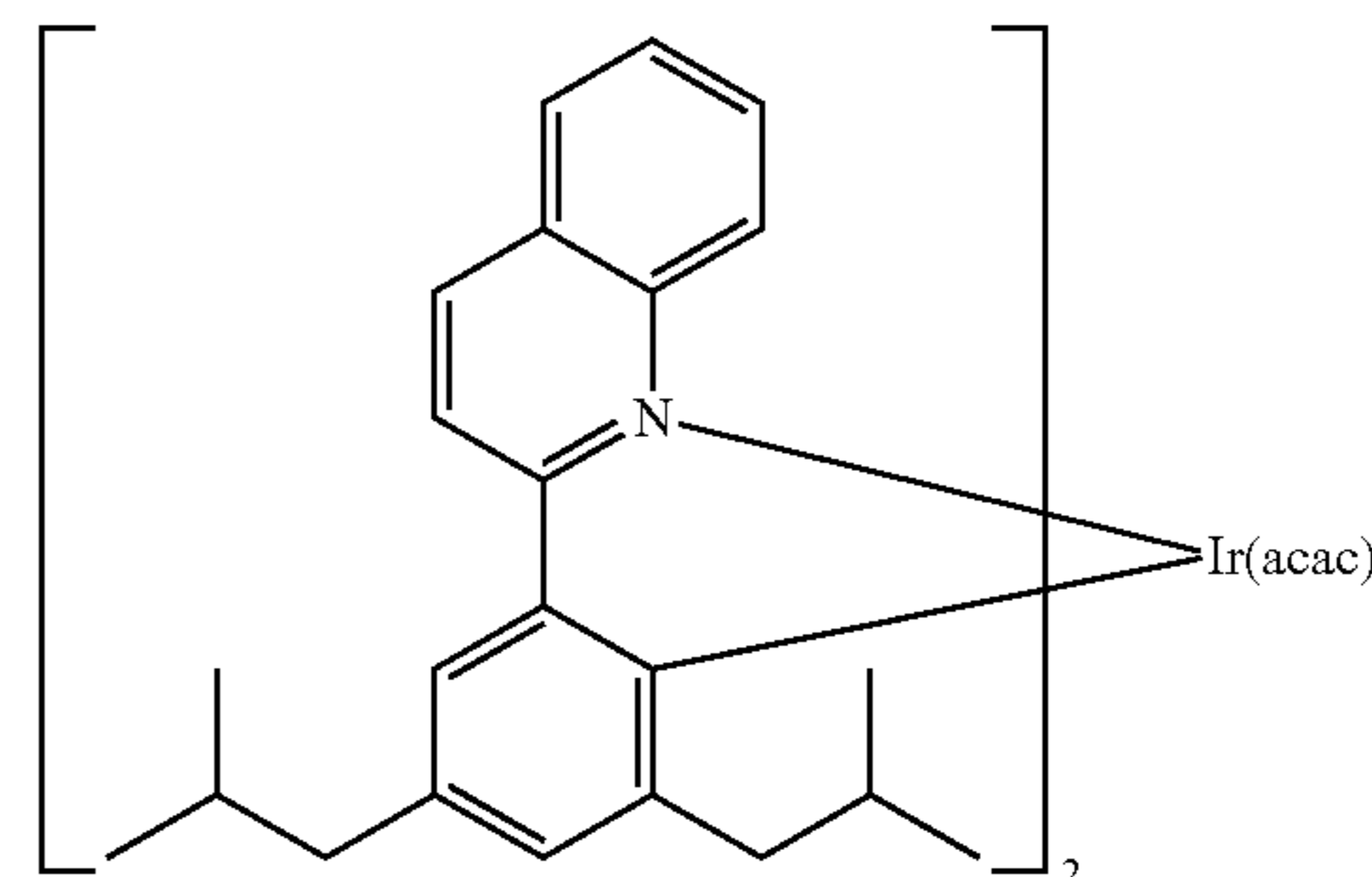
, and Compound 23
