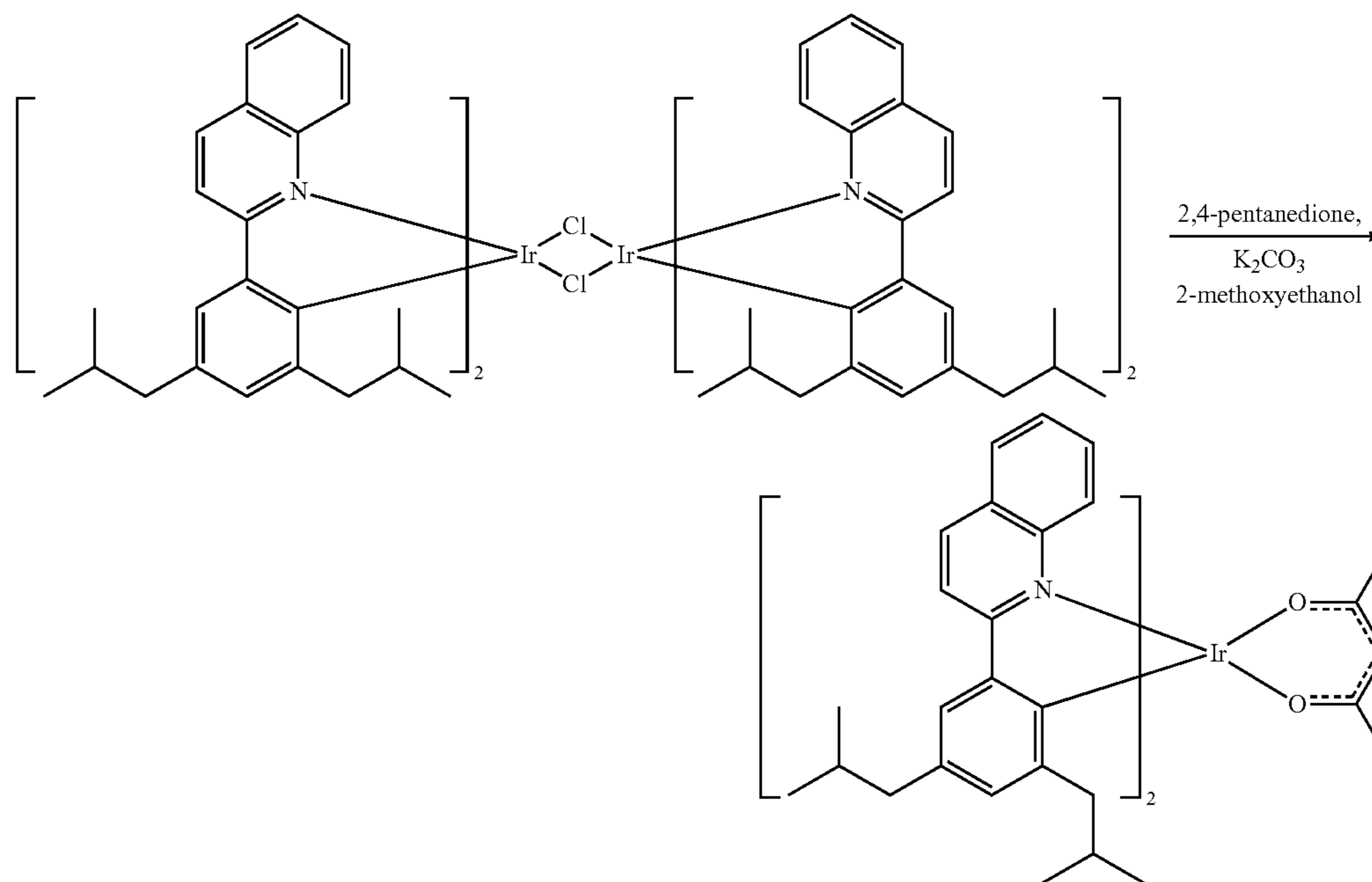
Compound 23
