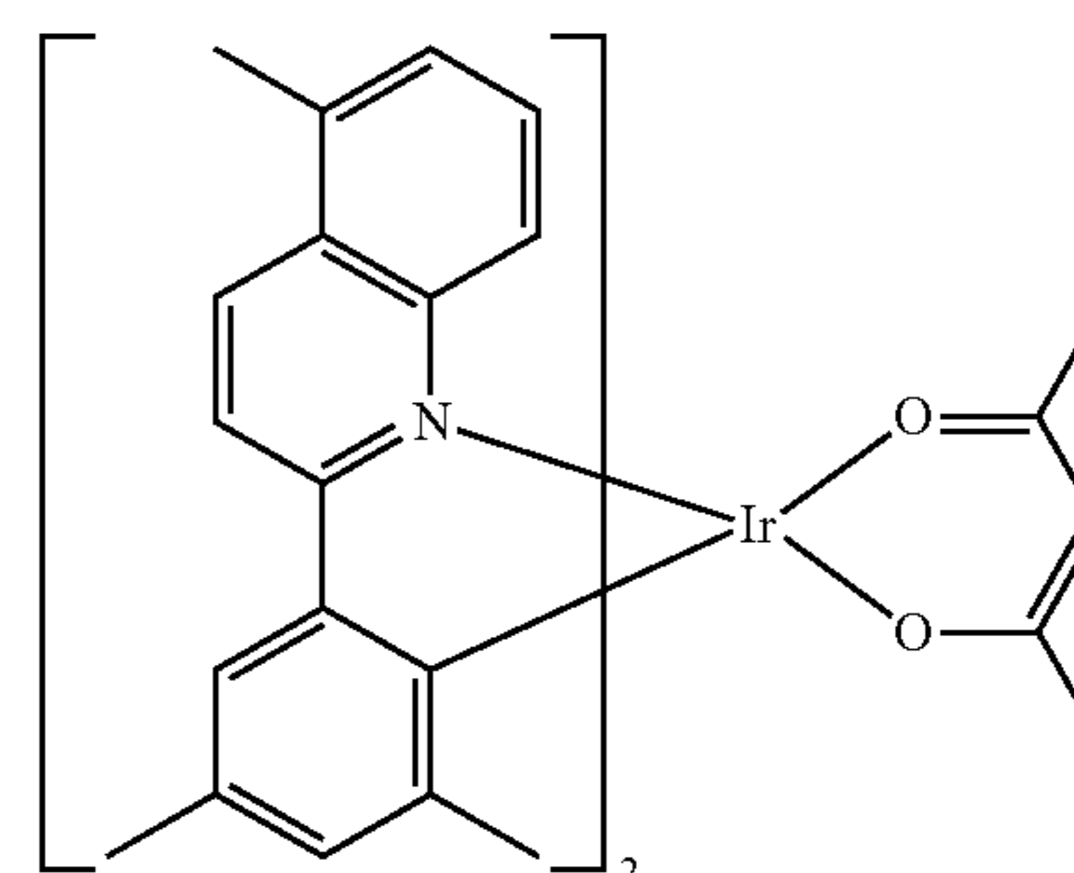
Compound 15
