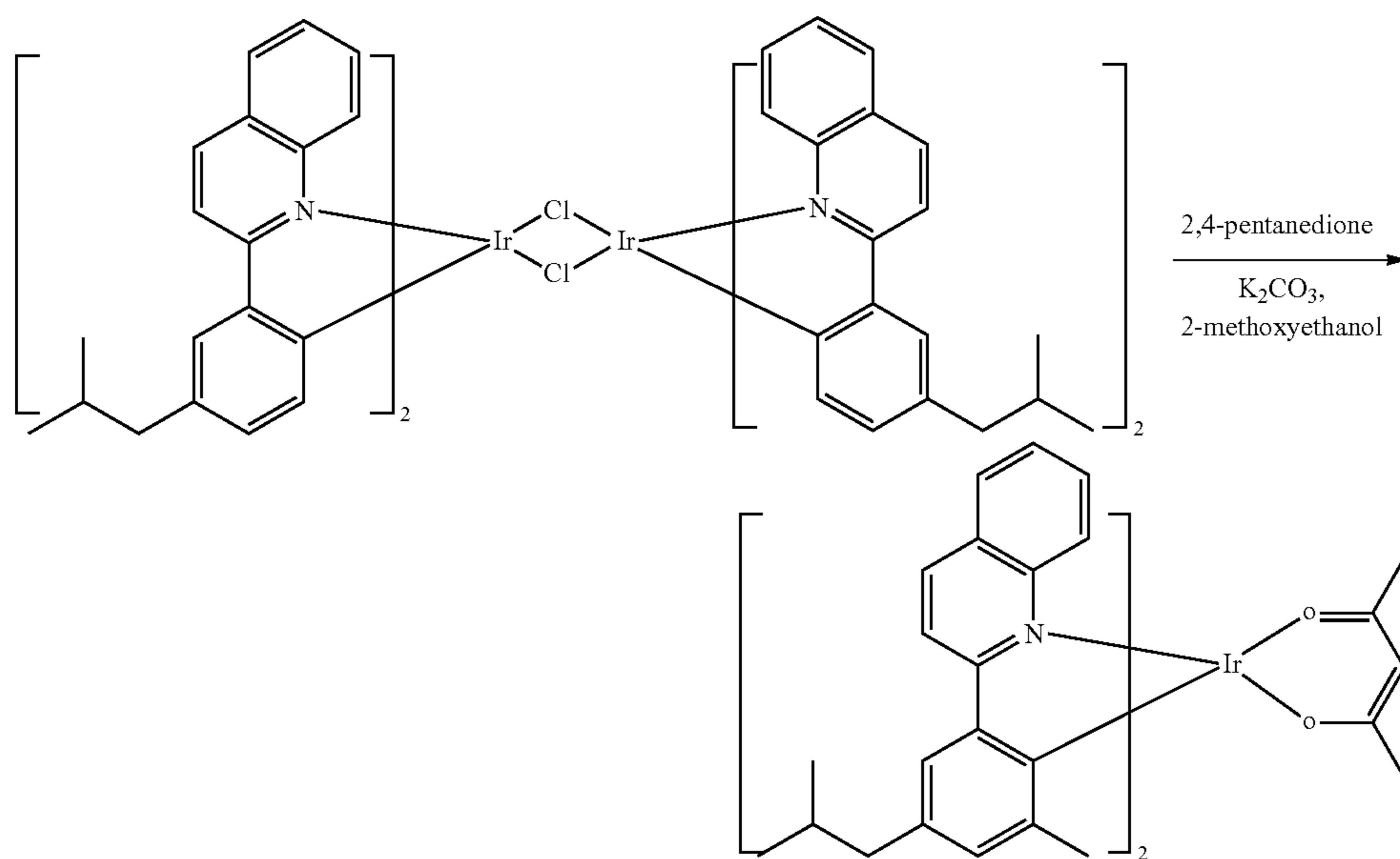
Compound 20
