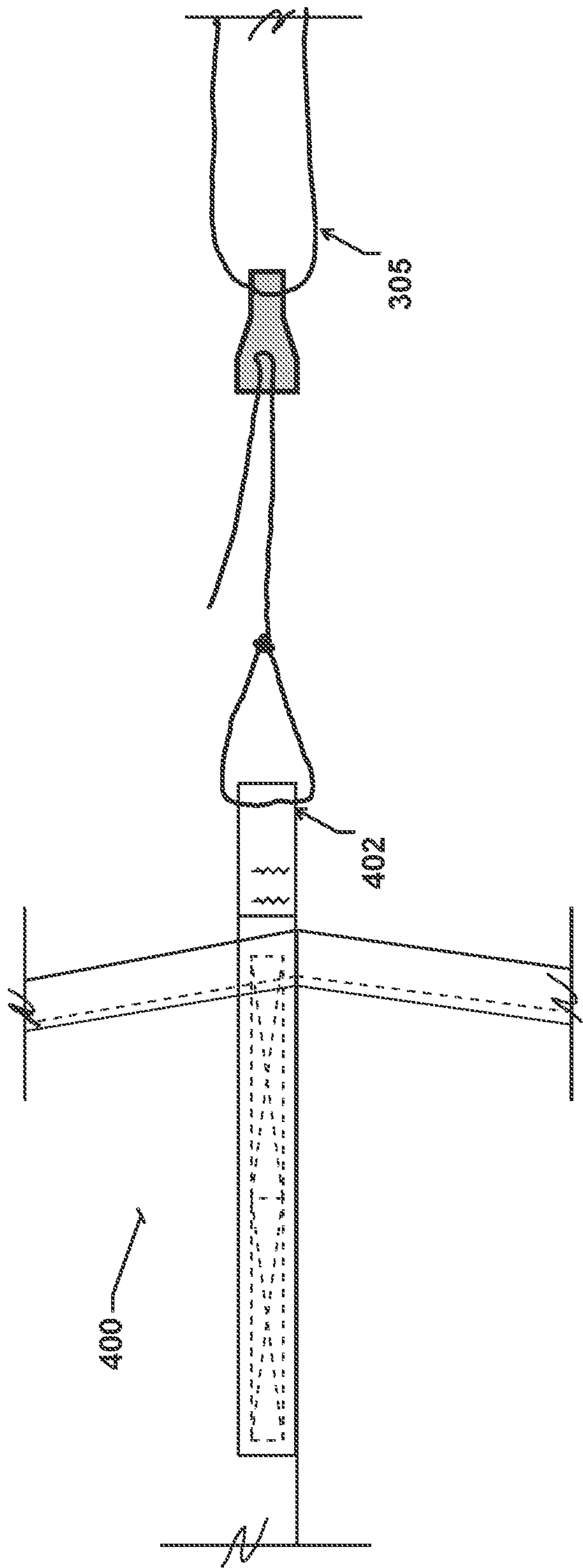
RAINFLY CONNECTION - TOP VIEW FIG 18A
