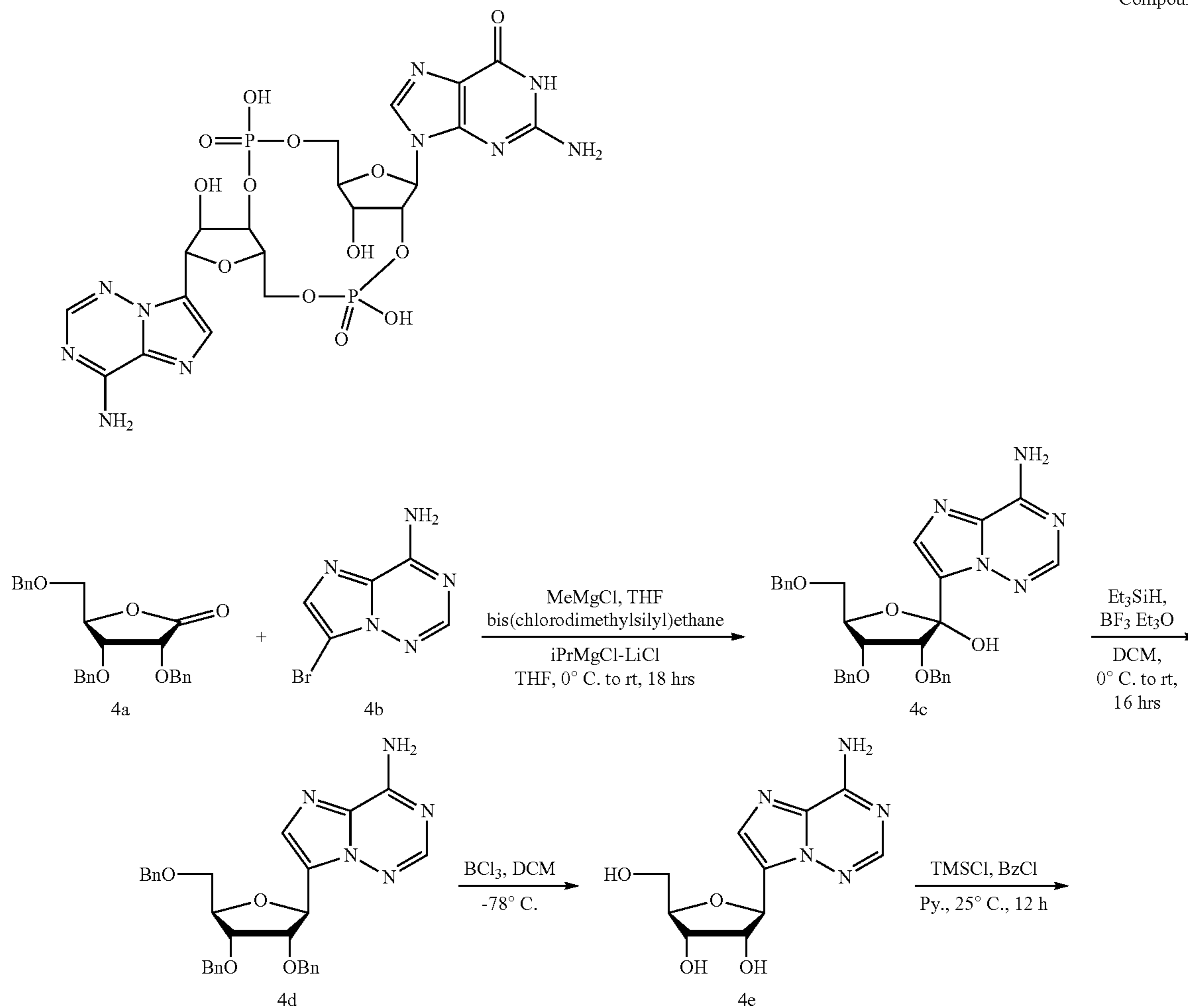
Compound 4
