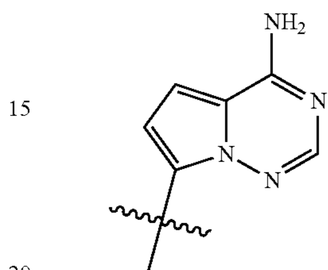
Formula (I)
