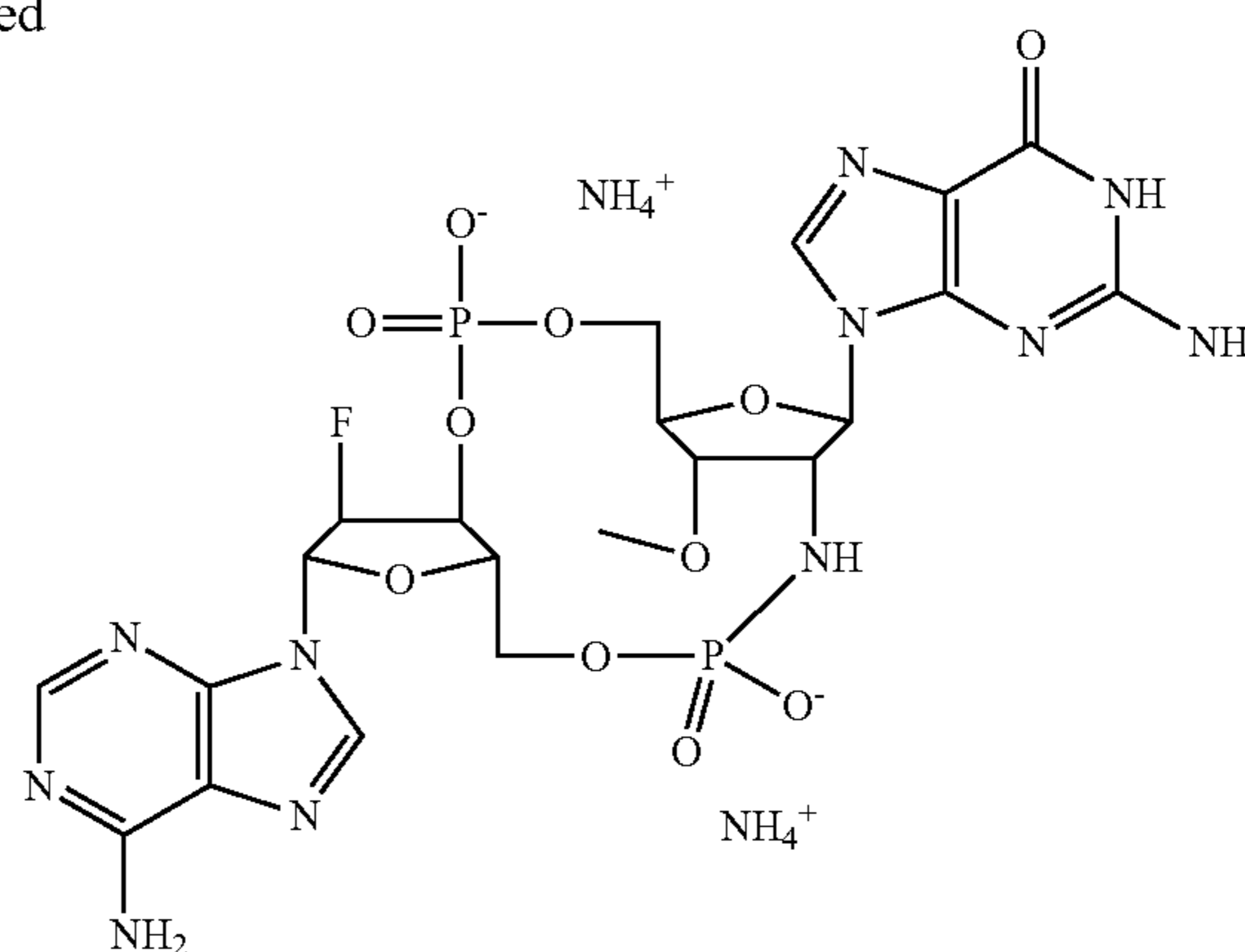
Compound 33
