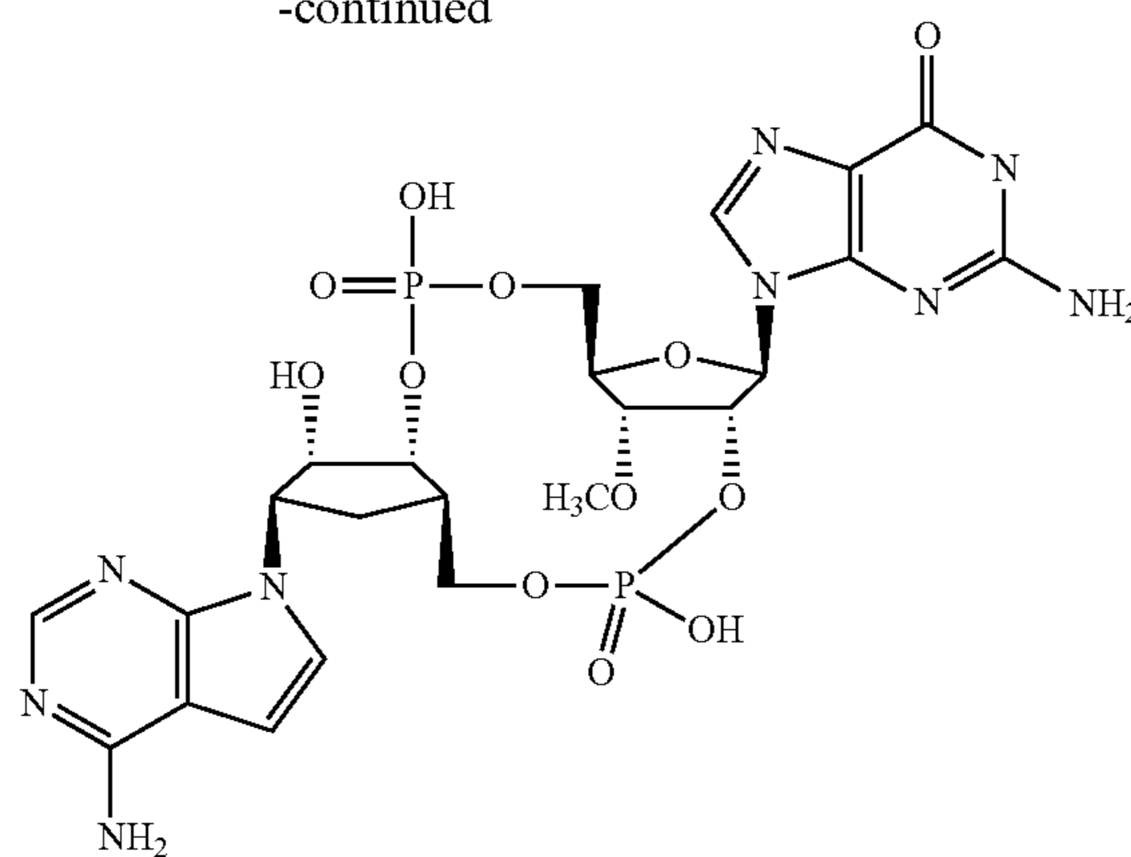
Compound 9
