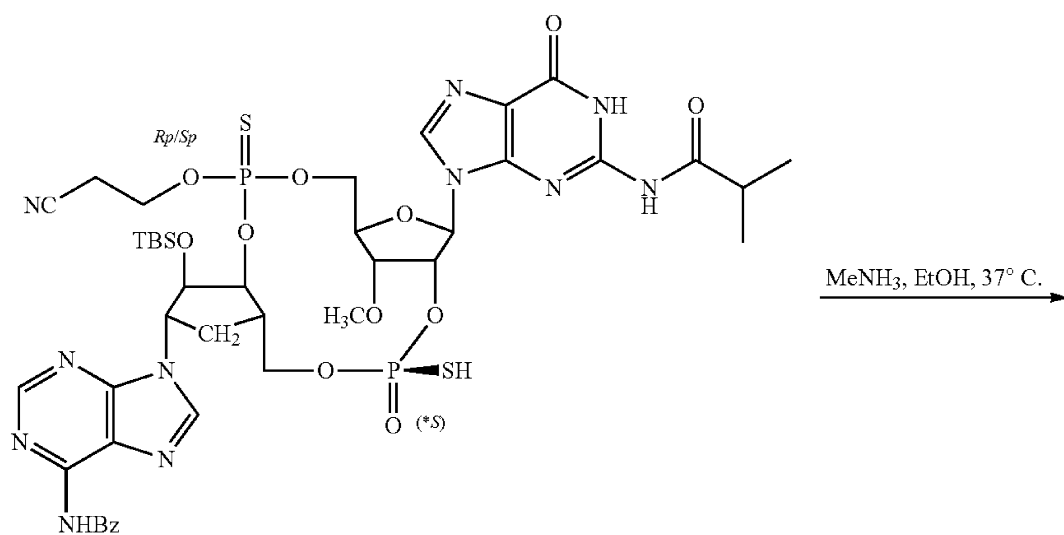
5l
