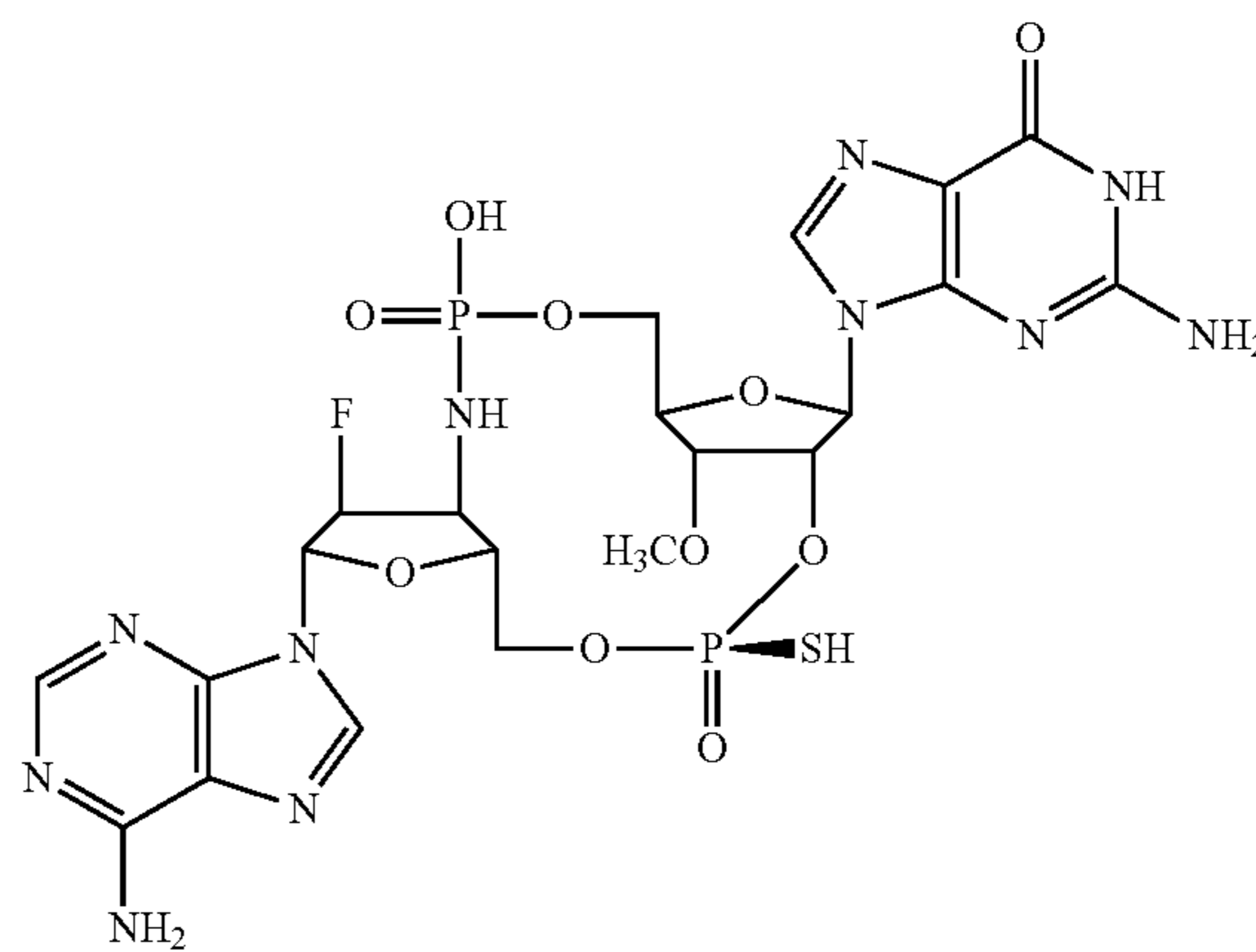
27
