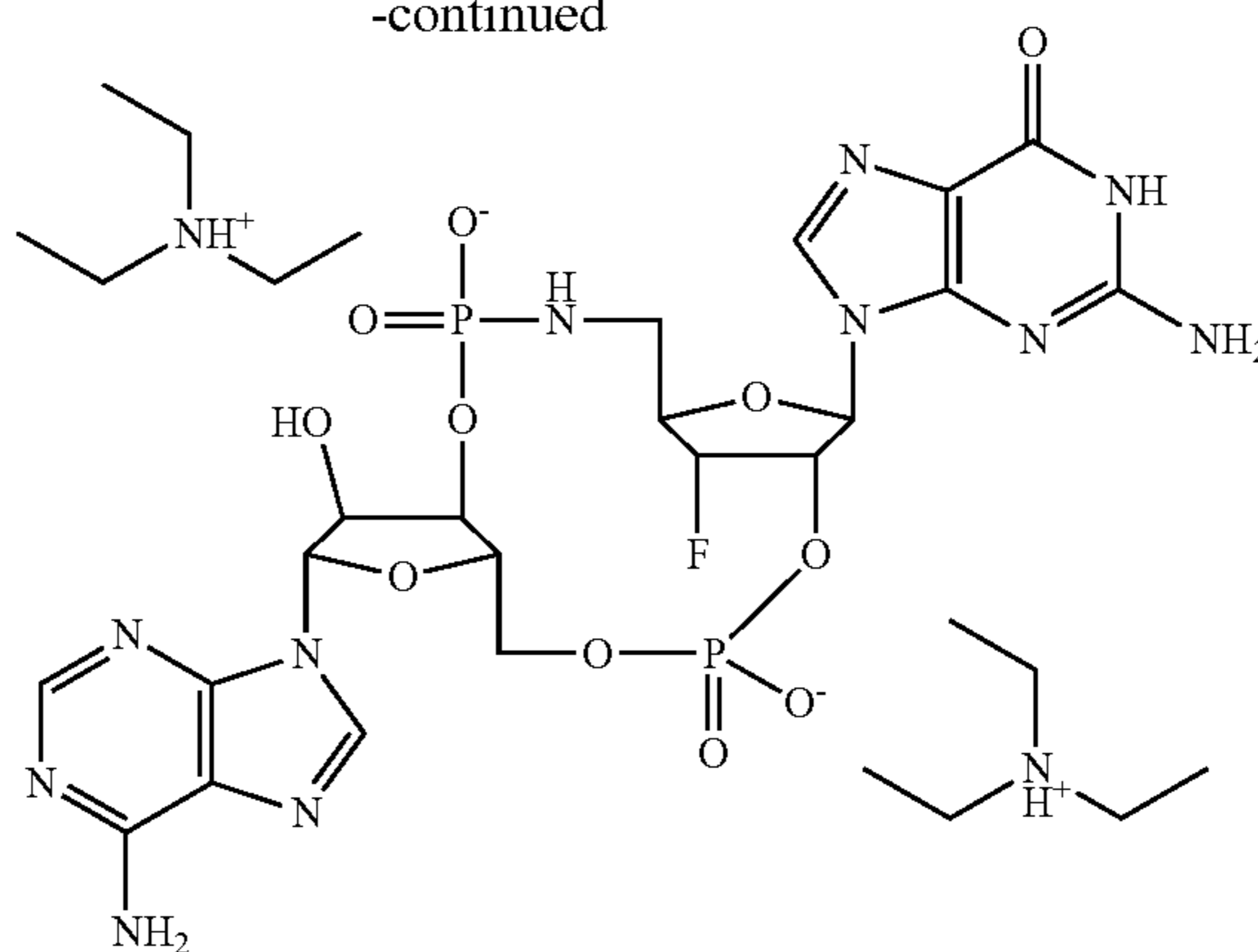
Compound 24
