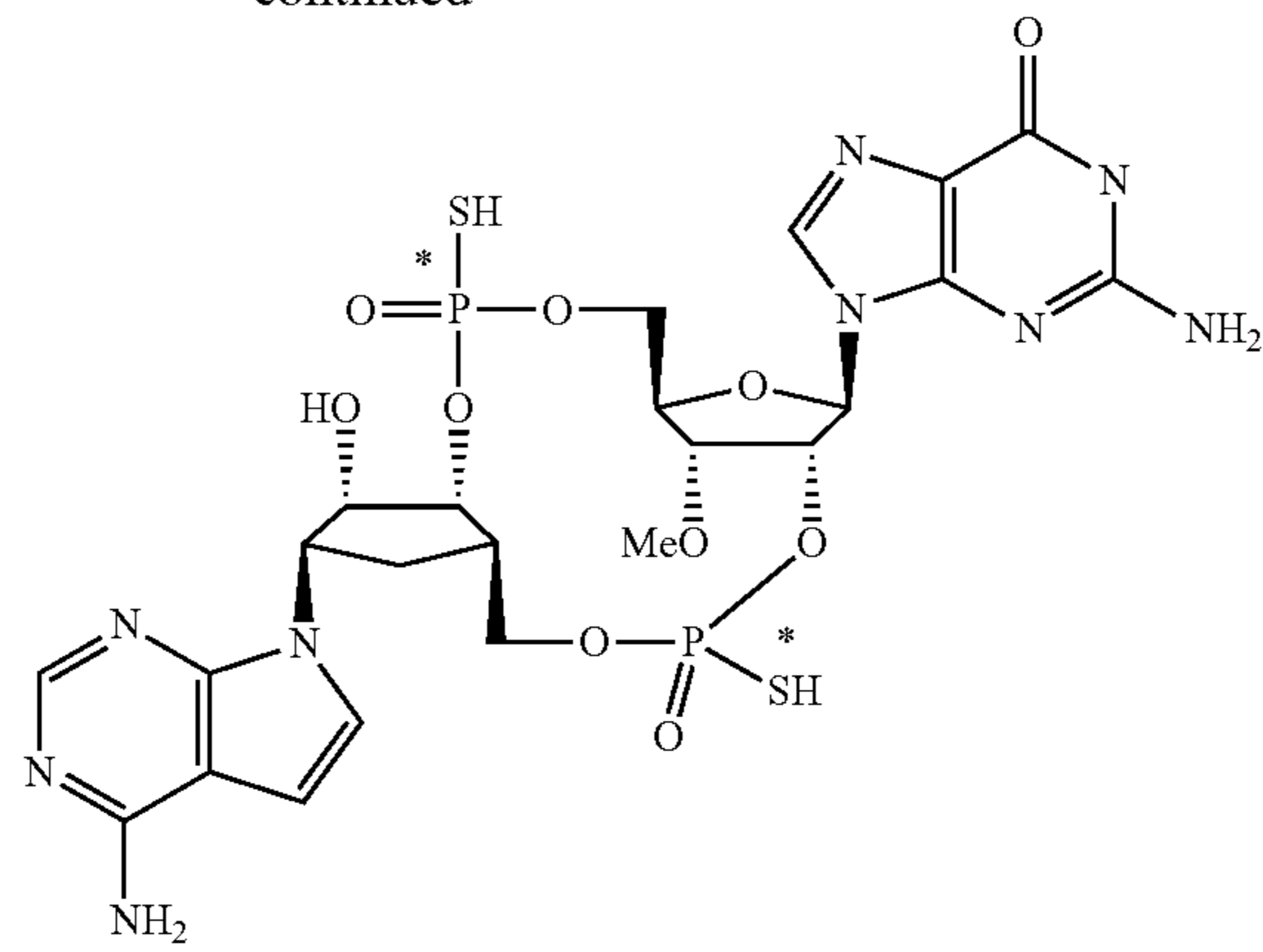
Diastereoisomers 10 to 13
