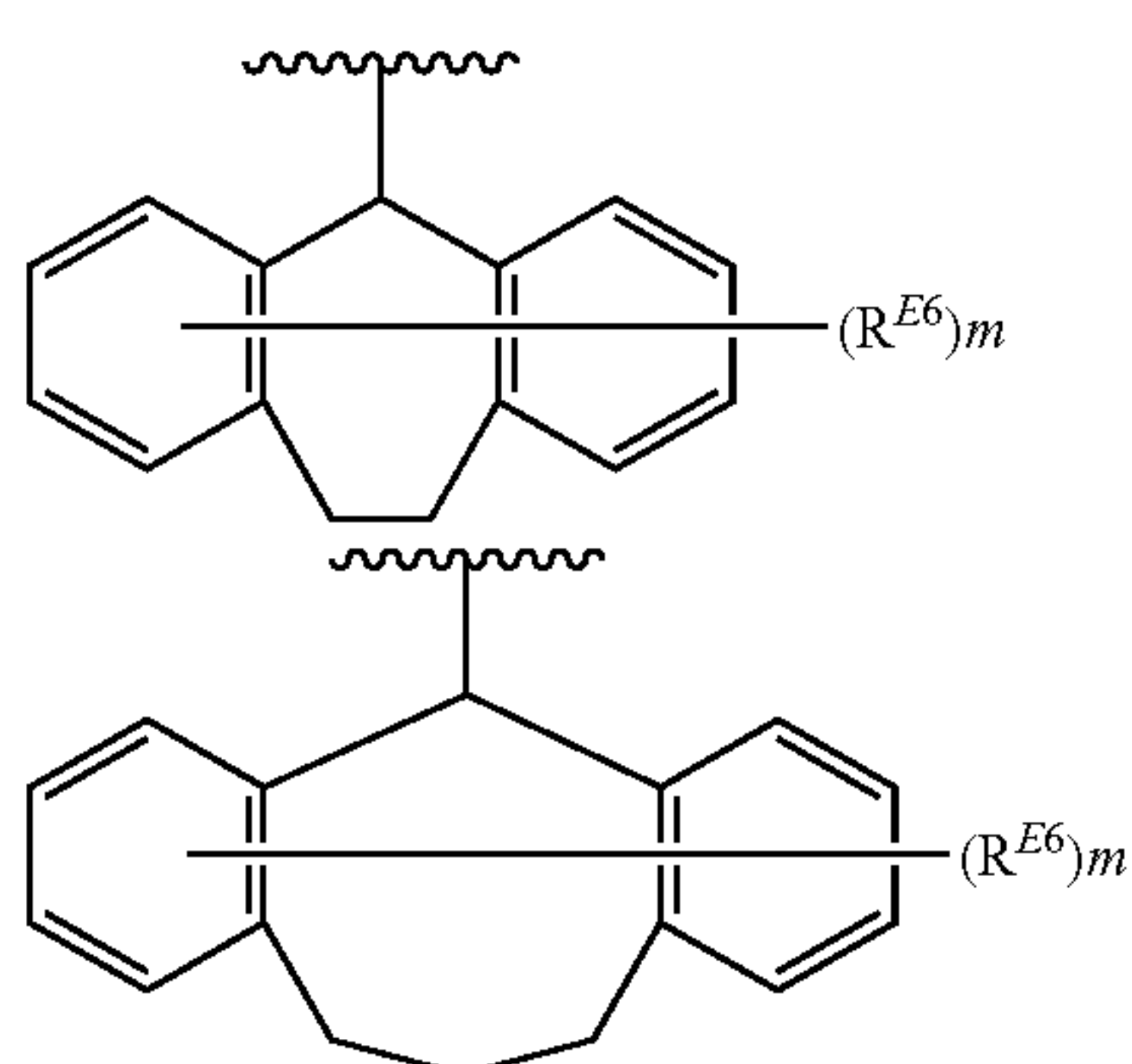
[Chemical Formula 66]
