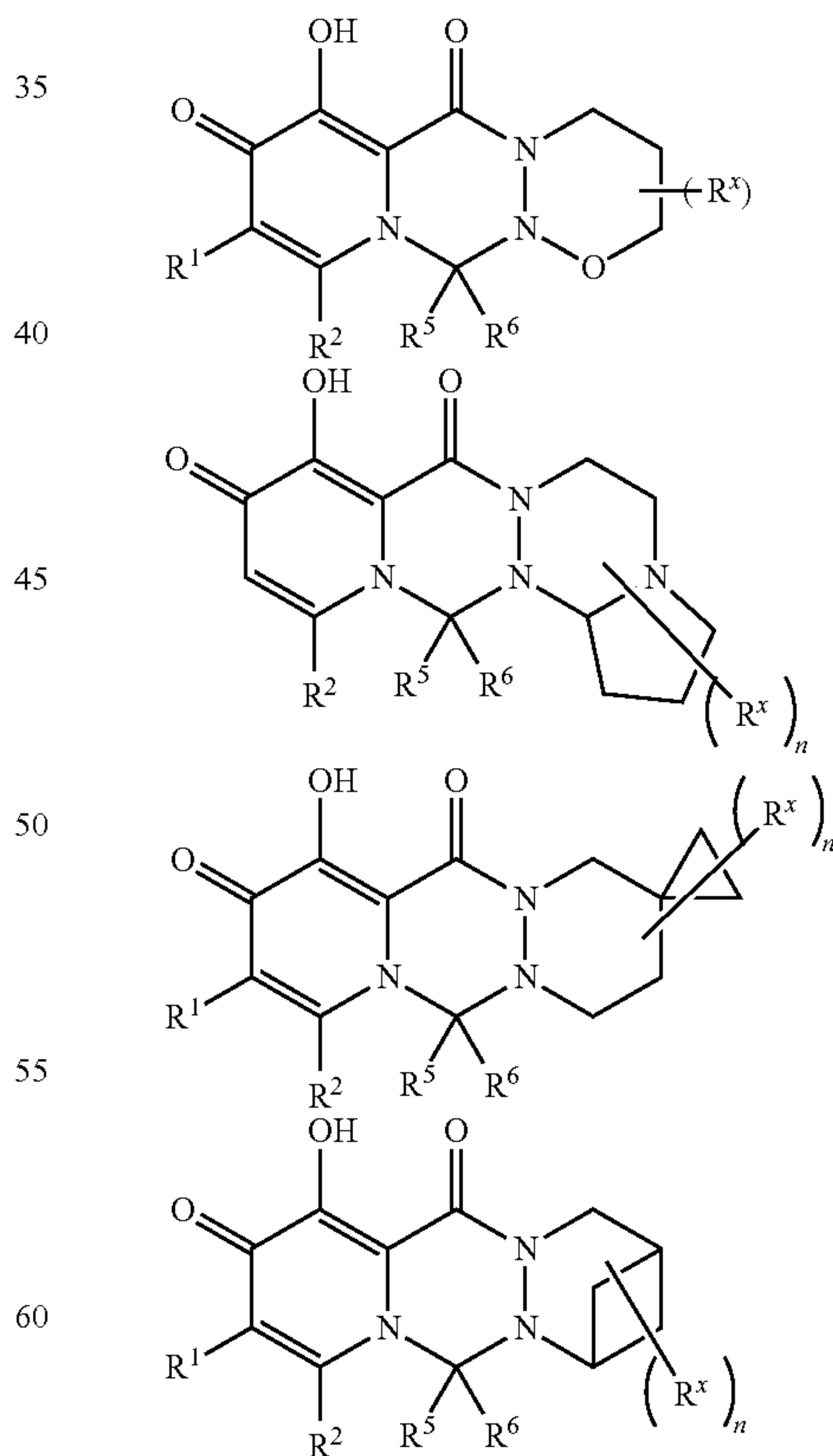
[Chemical Formula 36]
