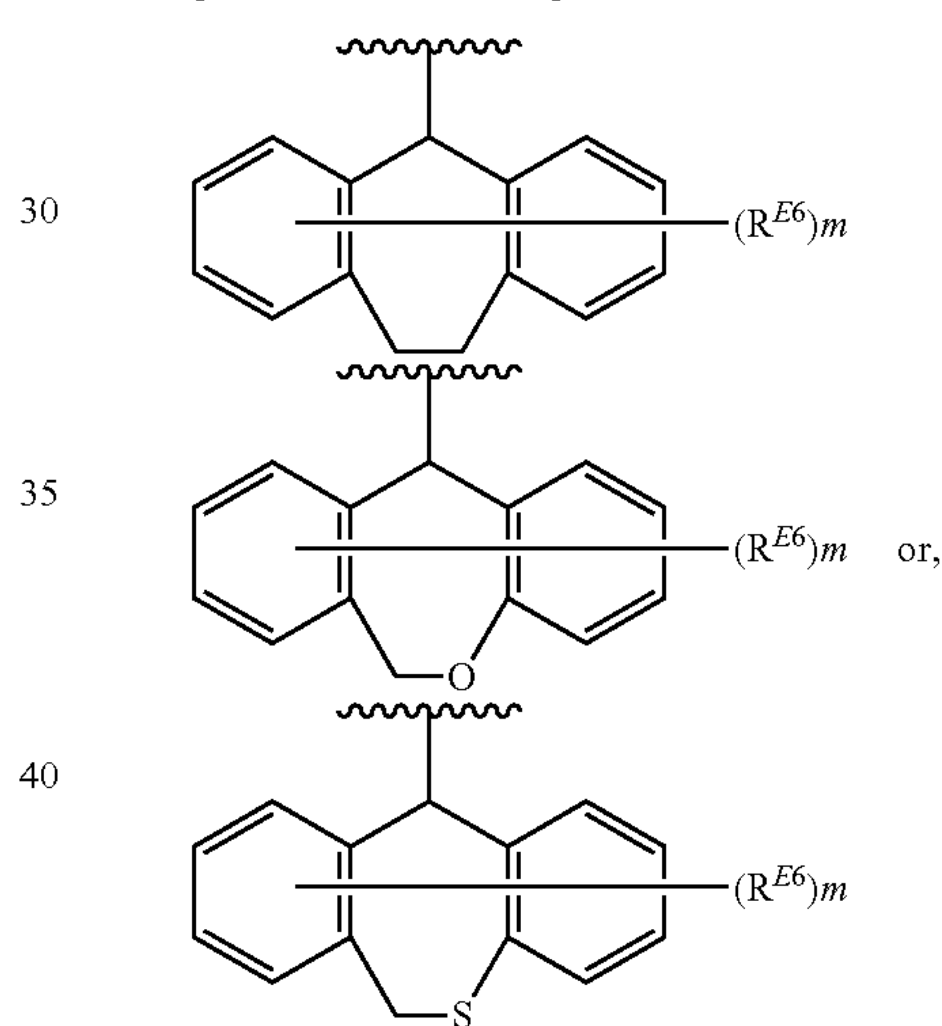
[Chemical Formula 64]
