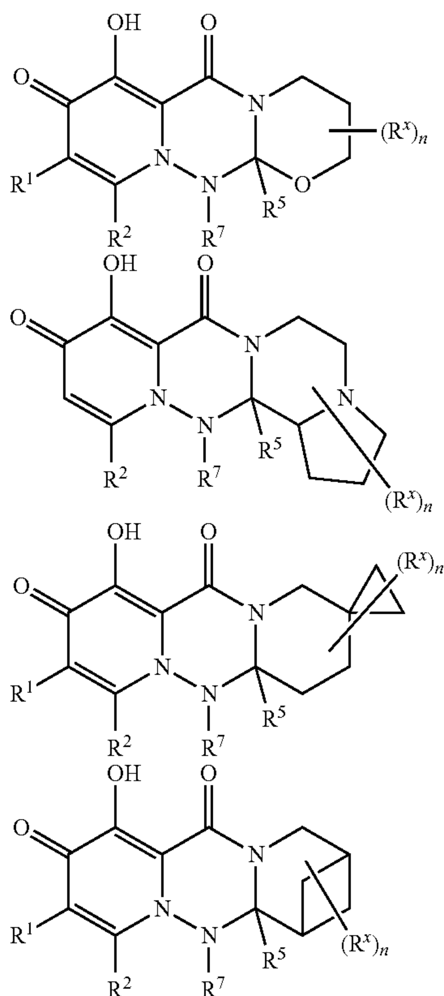
[Chemical Formula 41]
