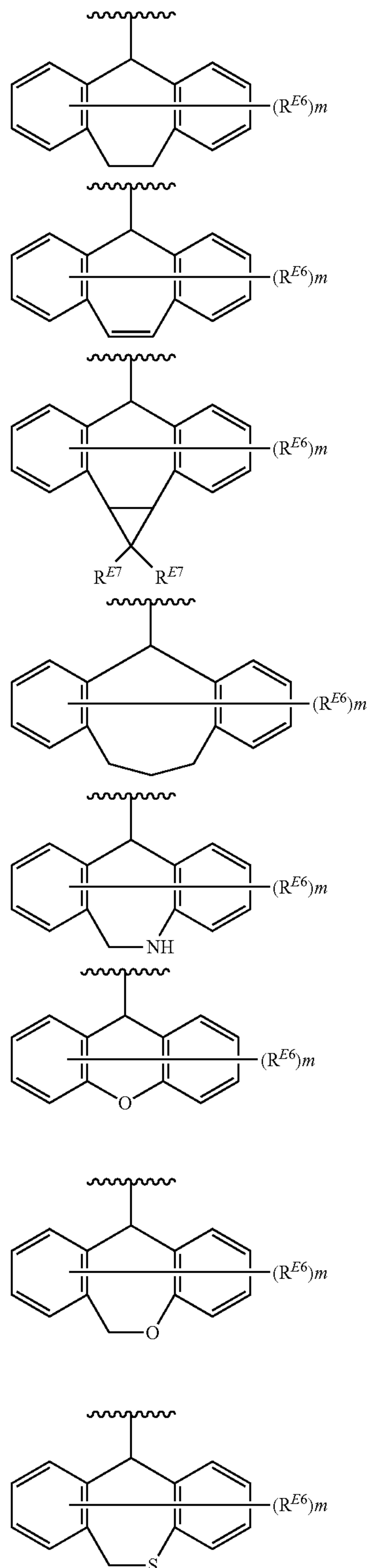
[Chemical Formula 81]
