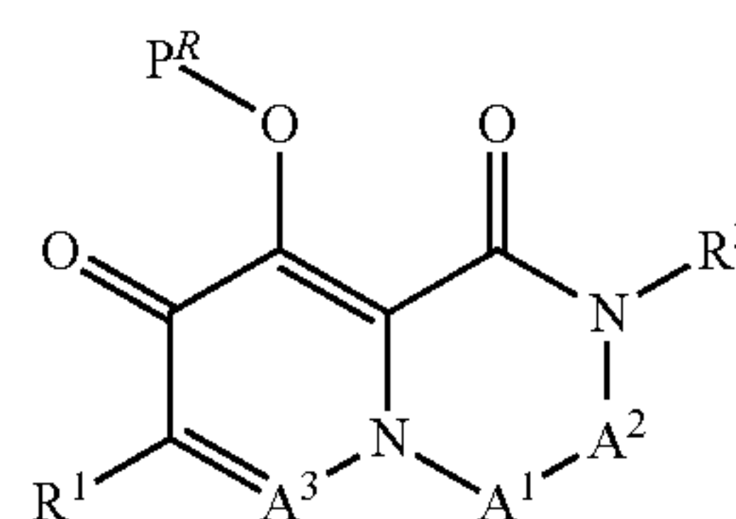
[Chemical Formula 82]
