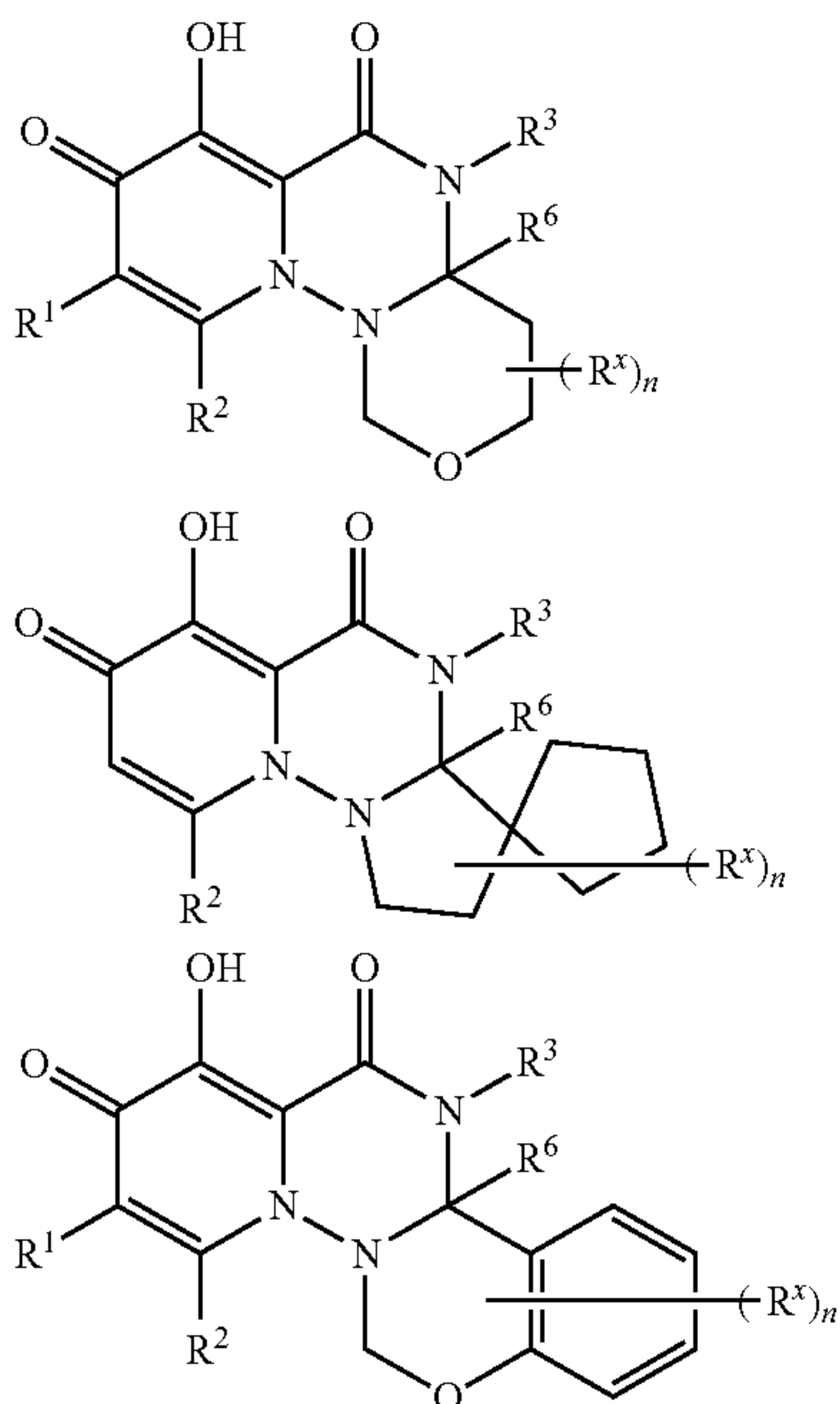
[Chemical Formula 38]
