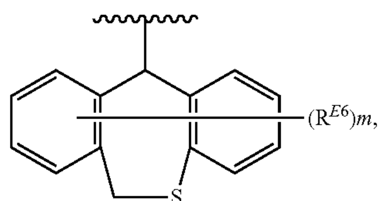
[Chemical Formula 24]
