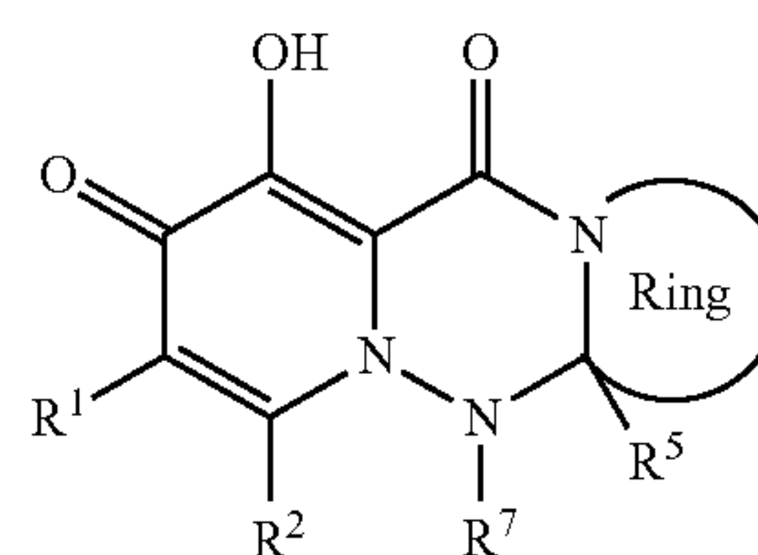
[Chemical Formula 40]
