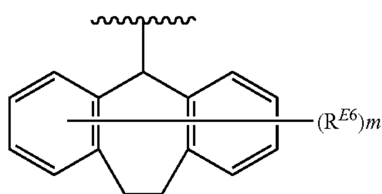
[Chemical Formula 80]
