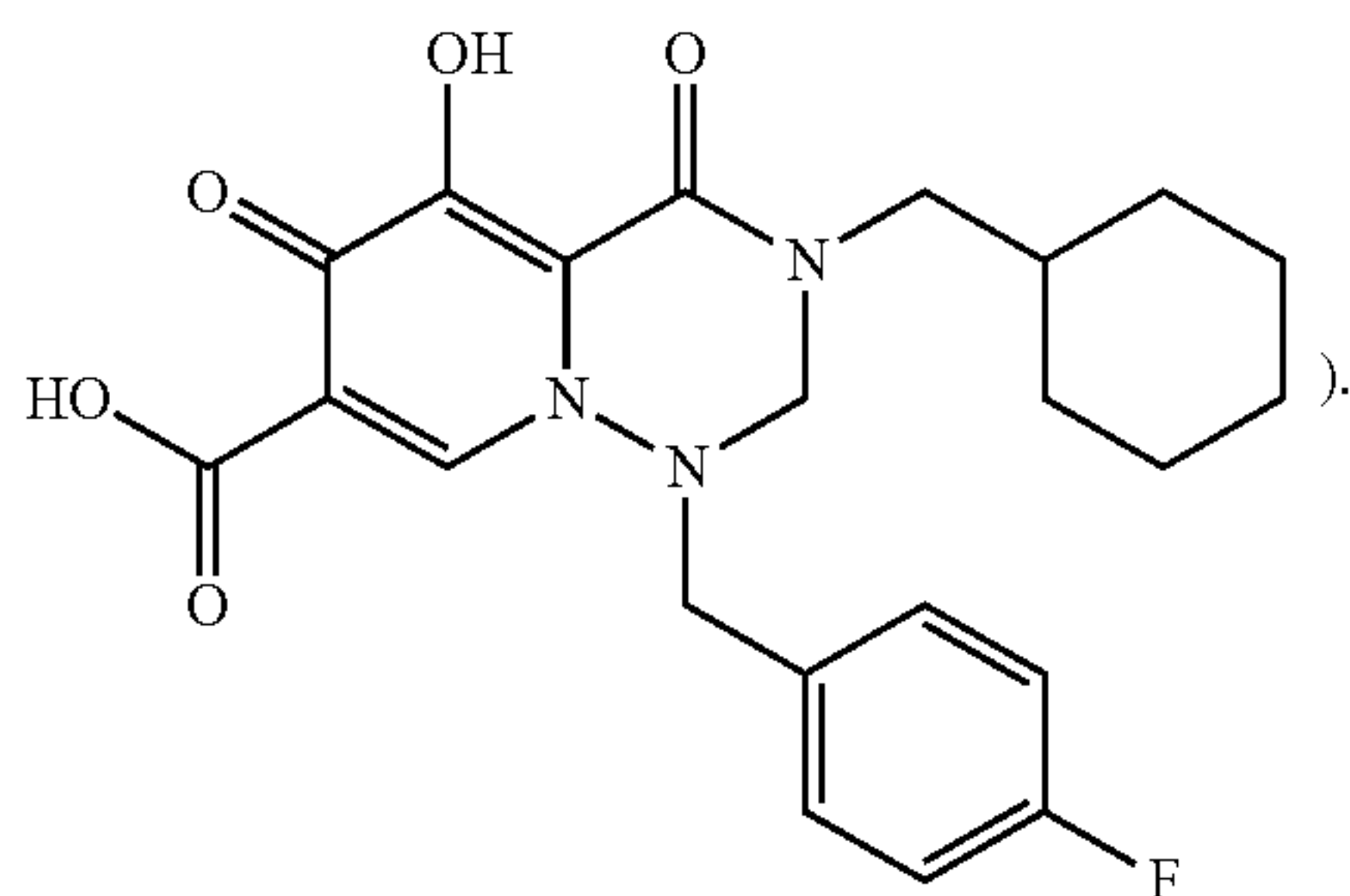
[Chemical Formula 9]
