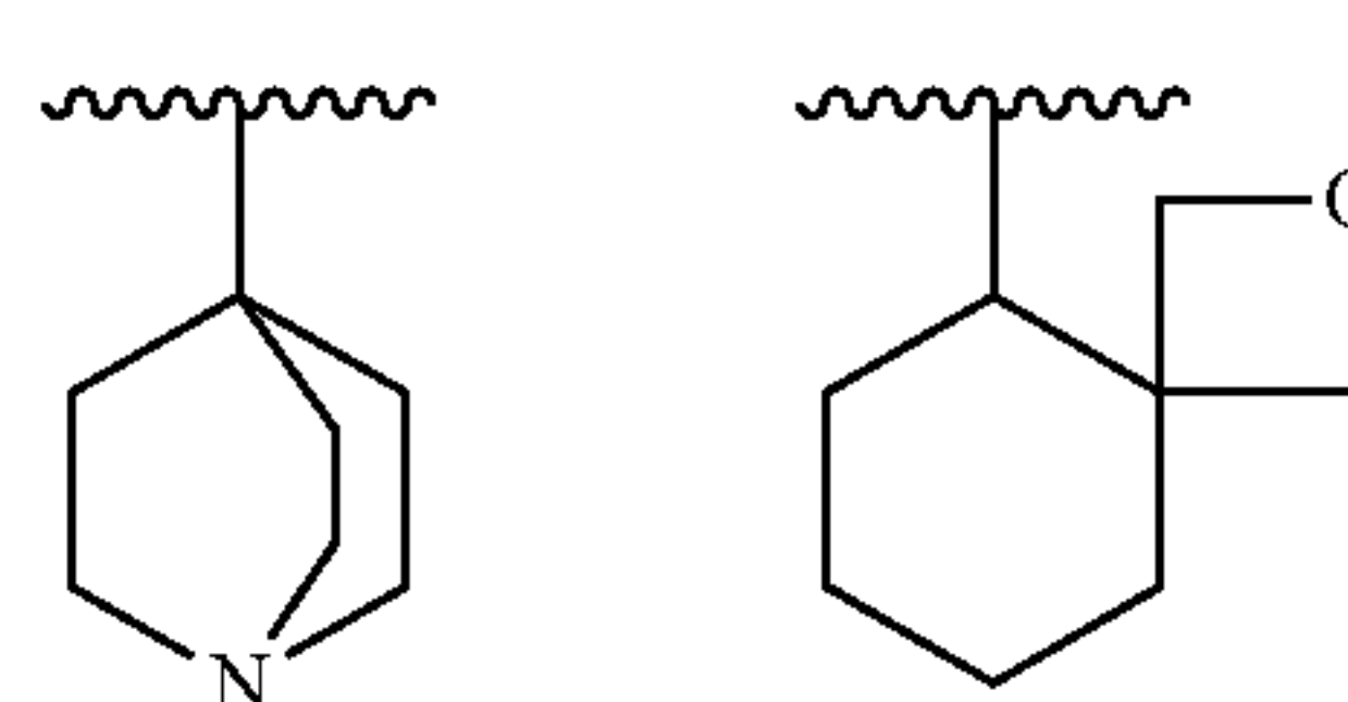
[Chemical Formula 15]
