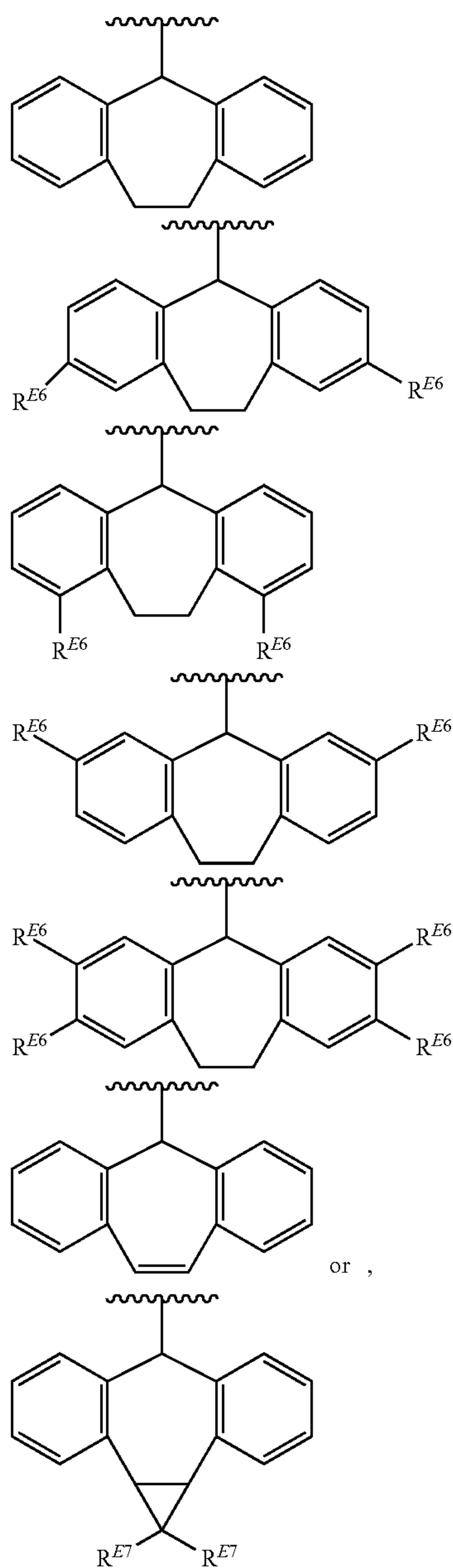
[Chemical Formula 49]
