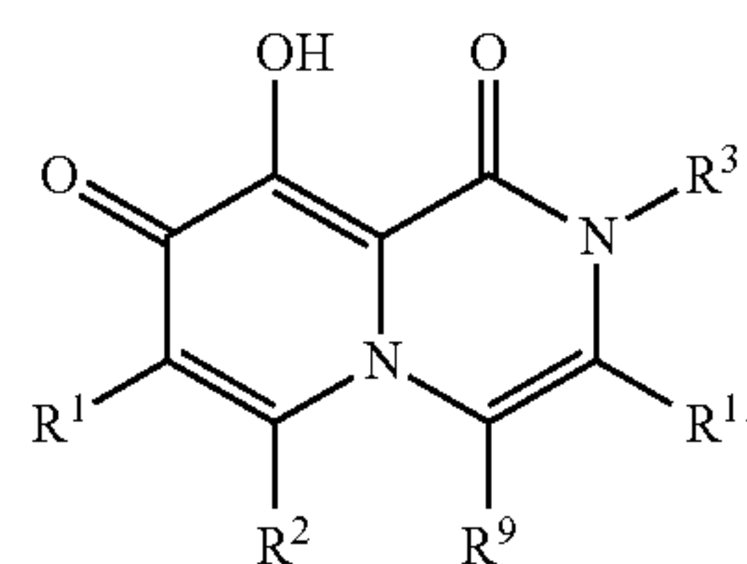
[Chemical Formula 44]
