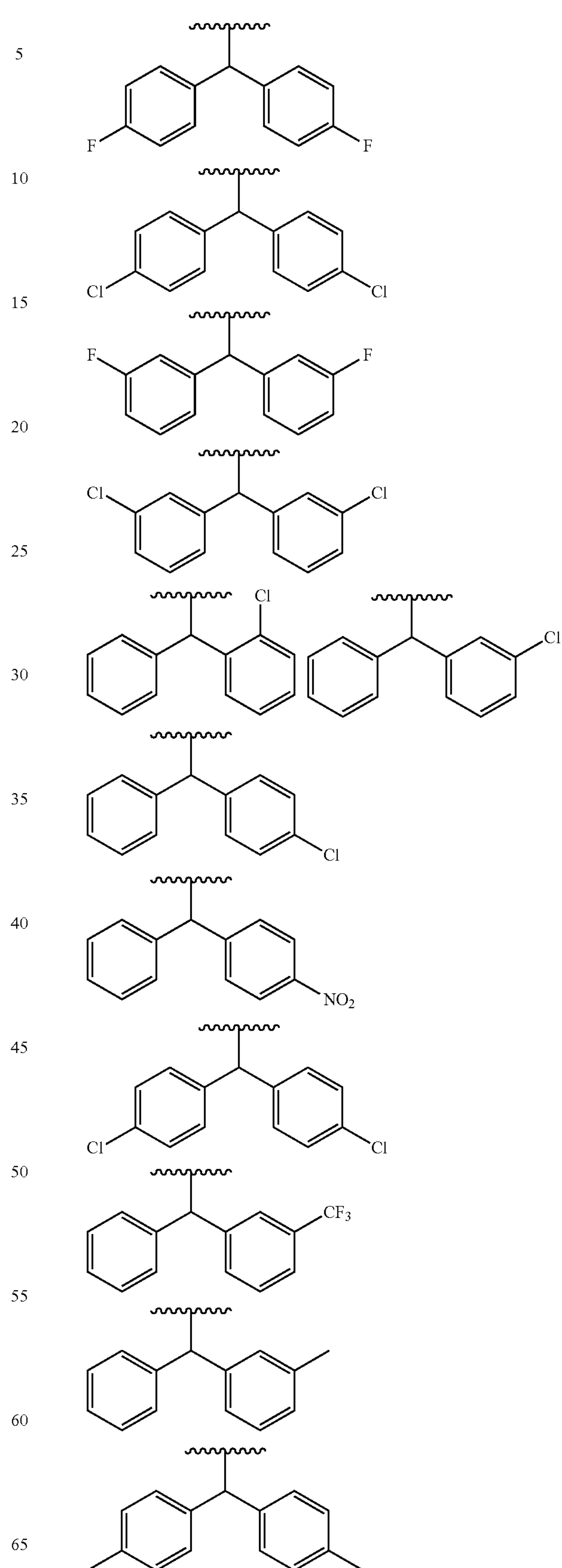
[Chemical Formula 50]
