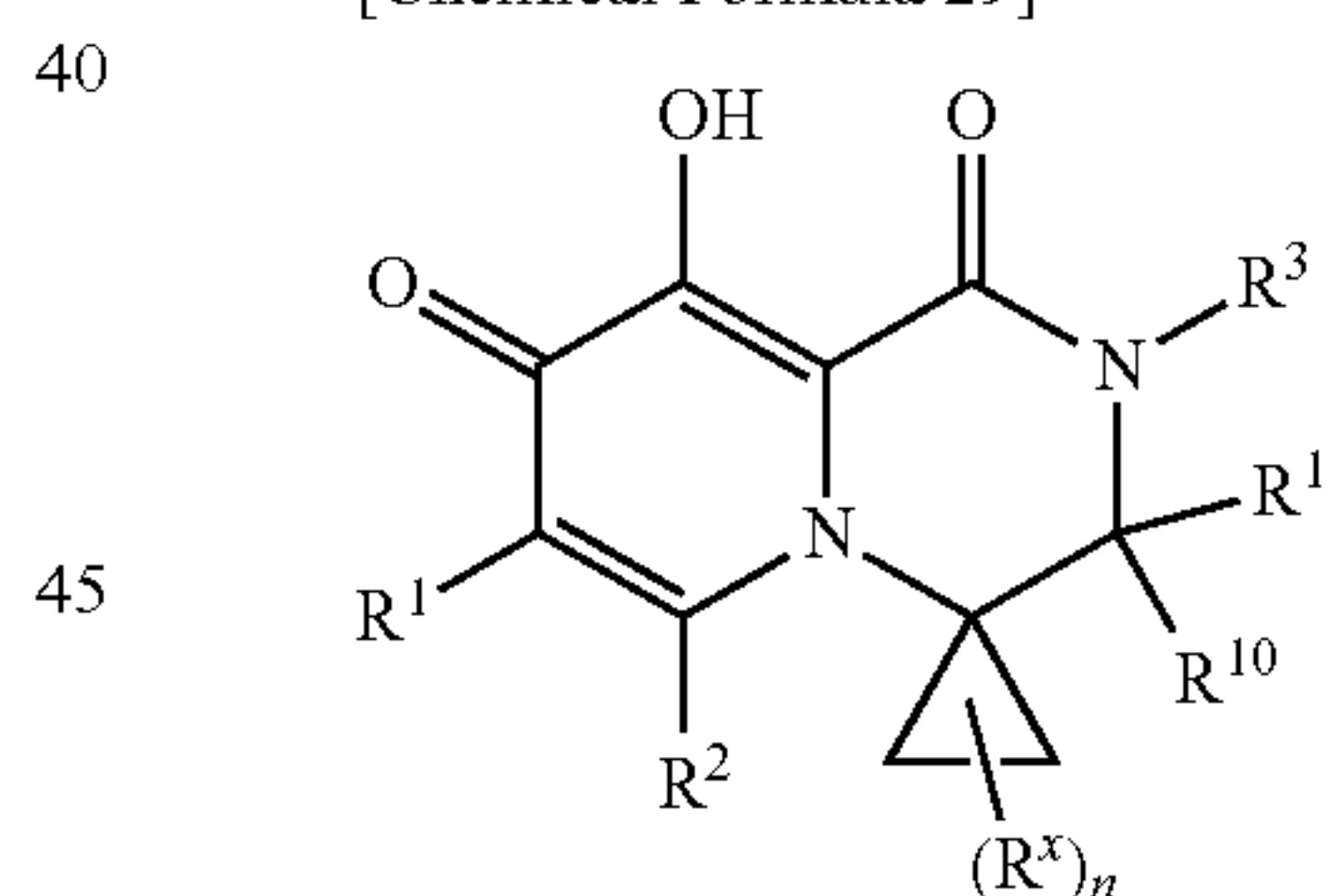
[Chemical Formula 29]
