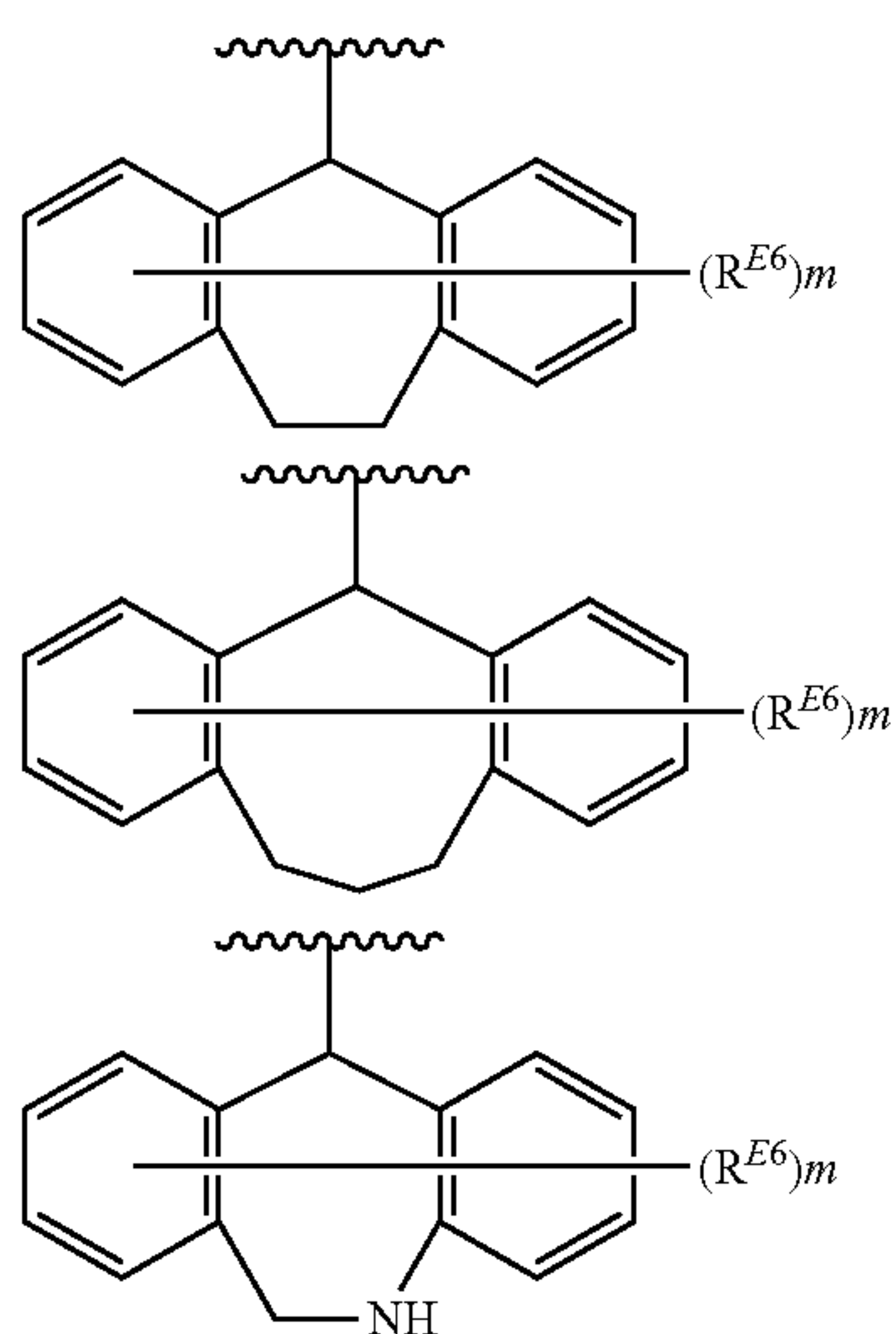
[Chemical Formula 61]
