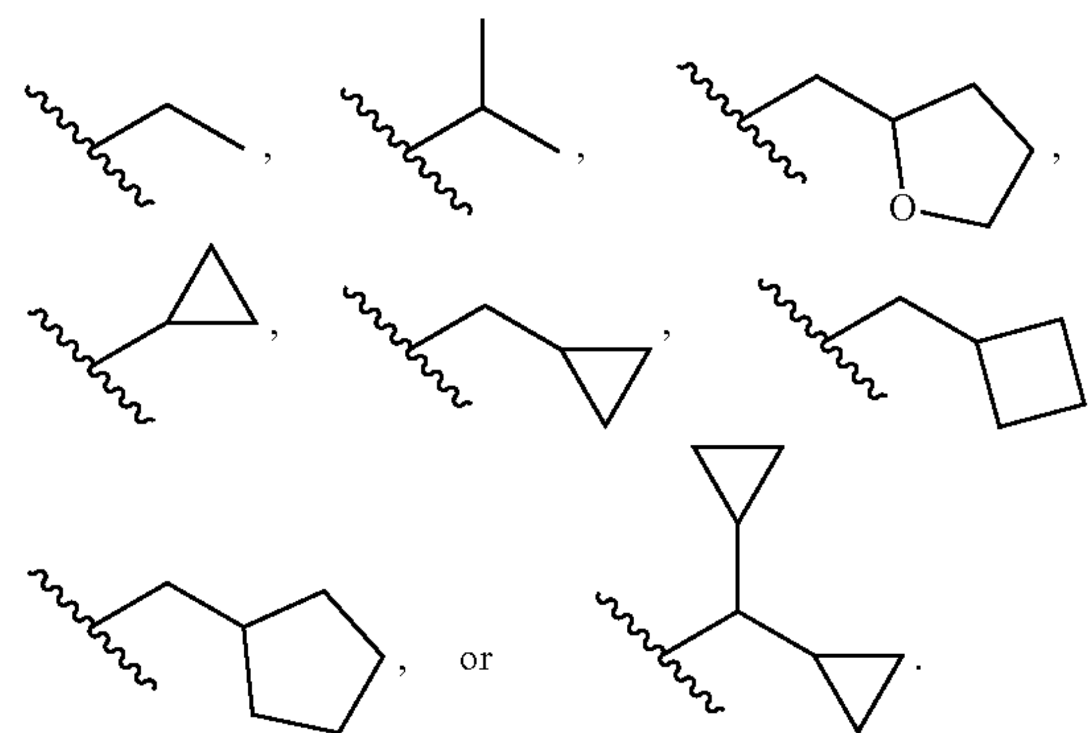
[Chemical Formula 57]
