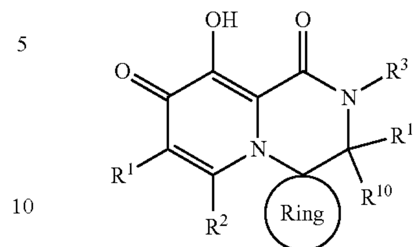
[Chemical Formula 28]
