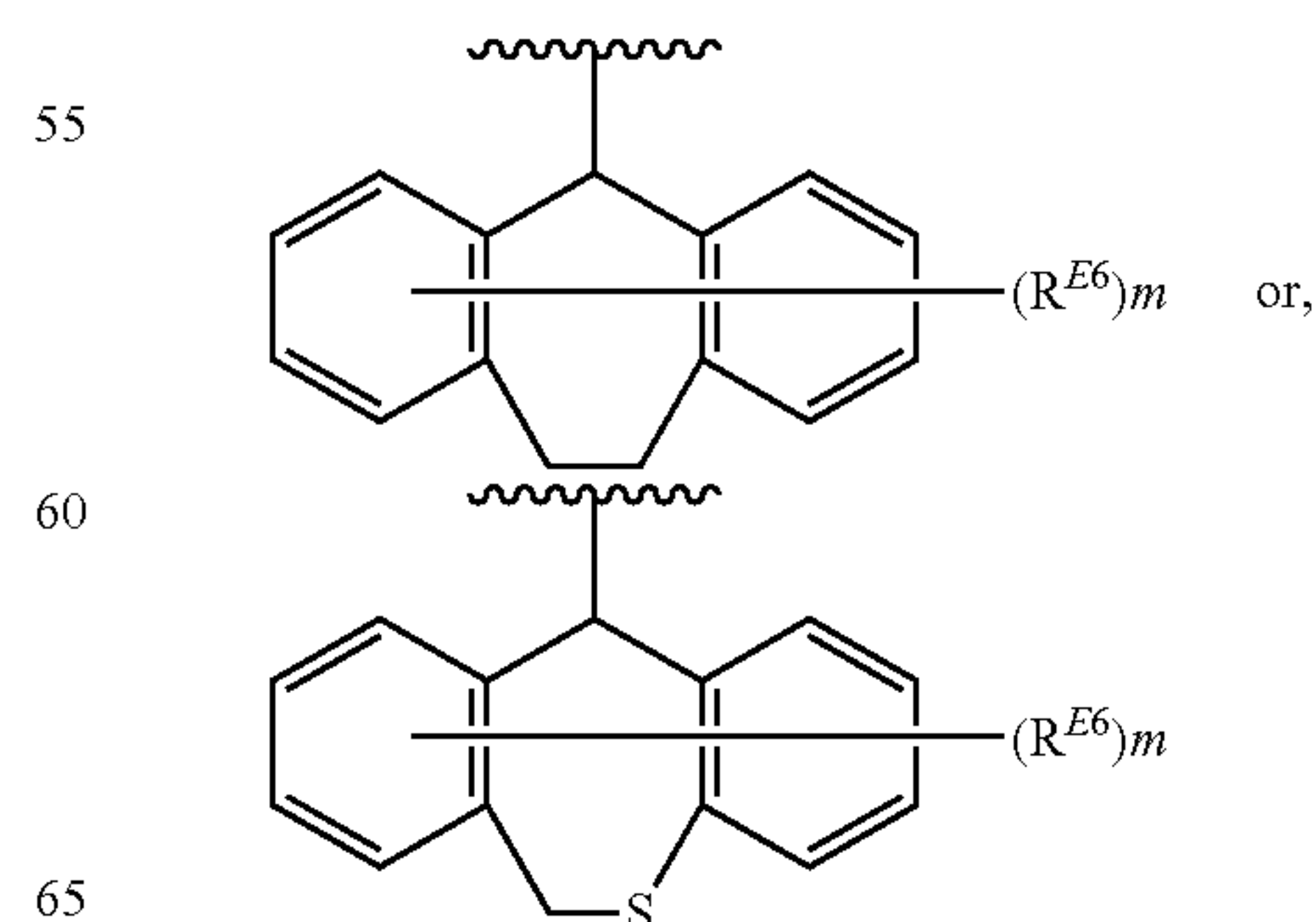
[Chemical Formula 78]
