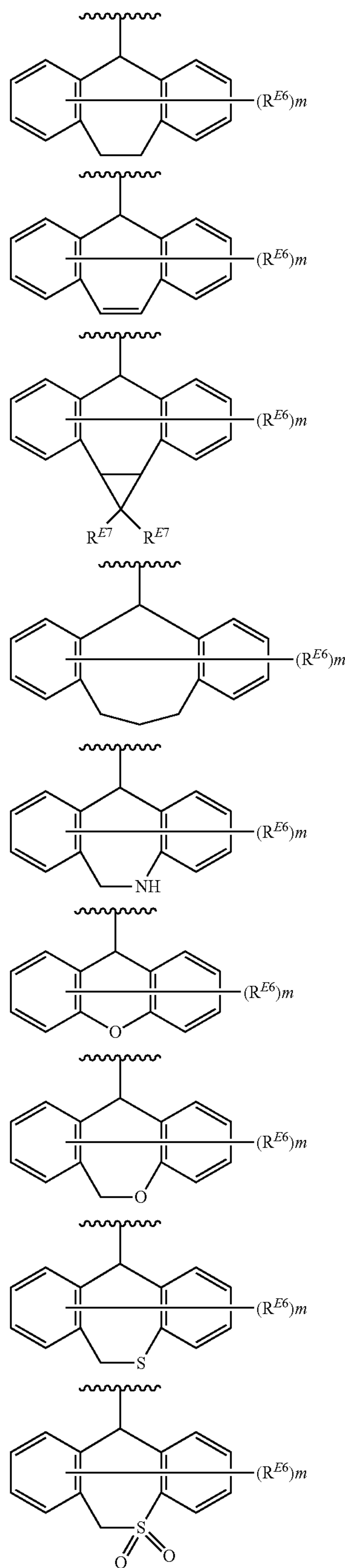
[Chemical Formula 10]
