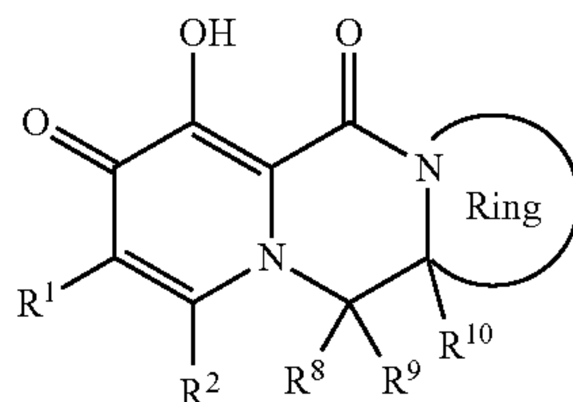
[Chemical Formula 45]
