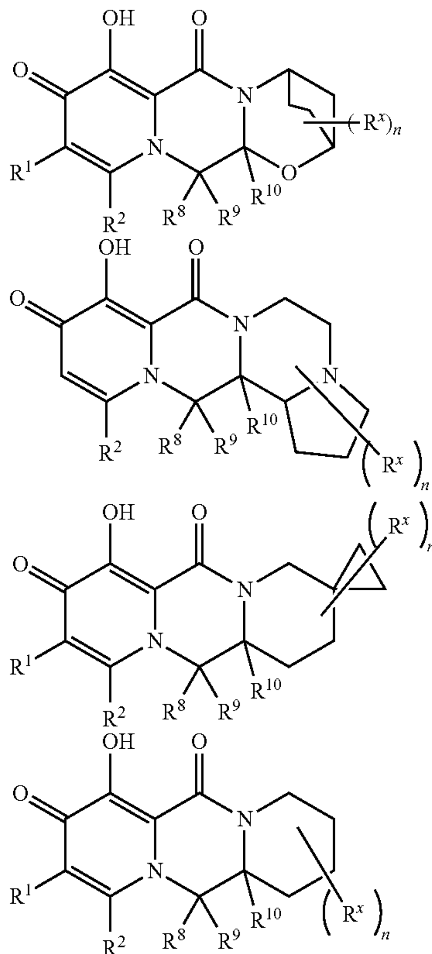
[Chemical Formula 46]
