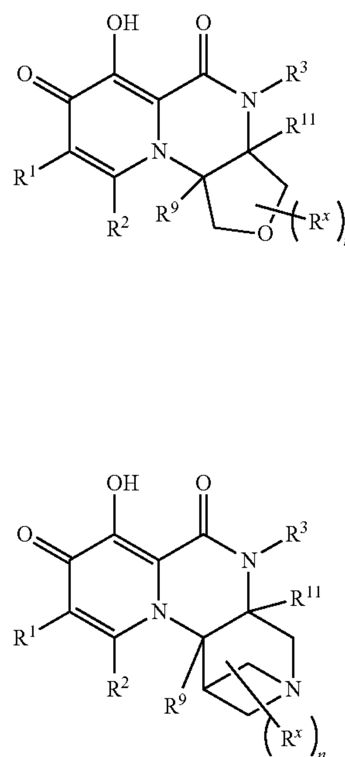
[Chemical Formula 43]
