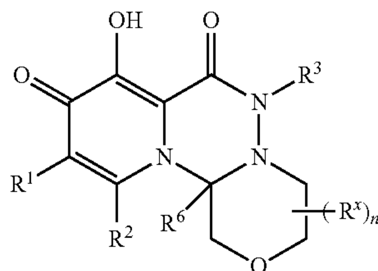
[Chemical Formula 33]
