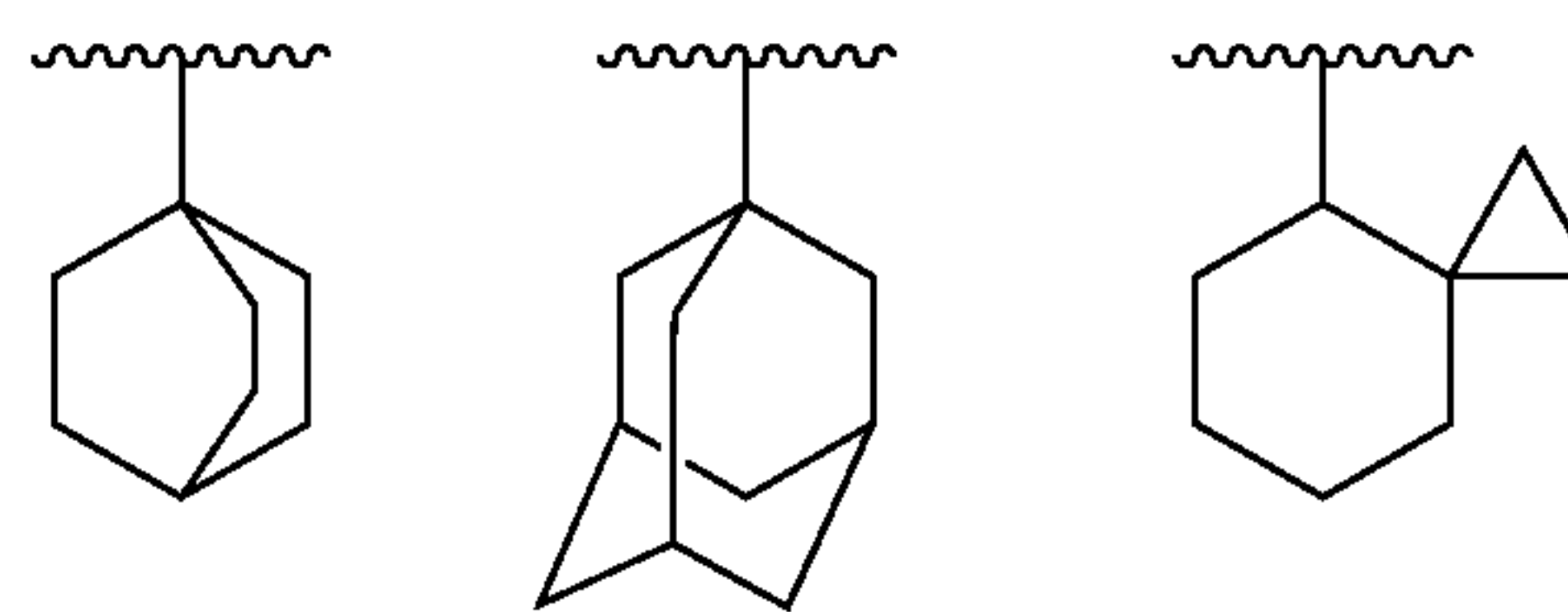
[Chemical Formula 14]
