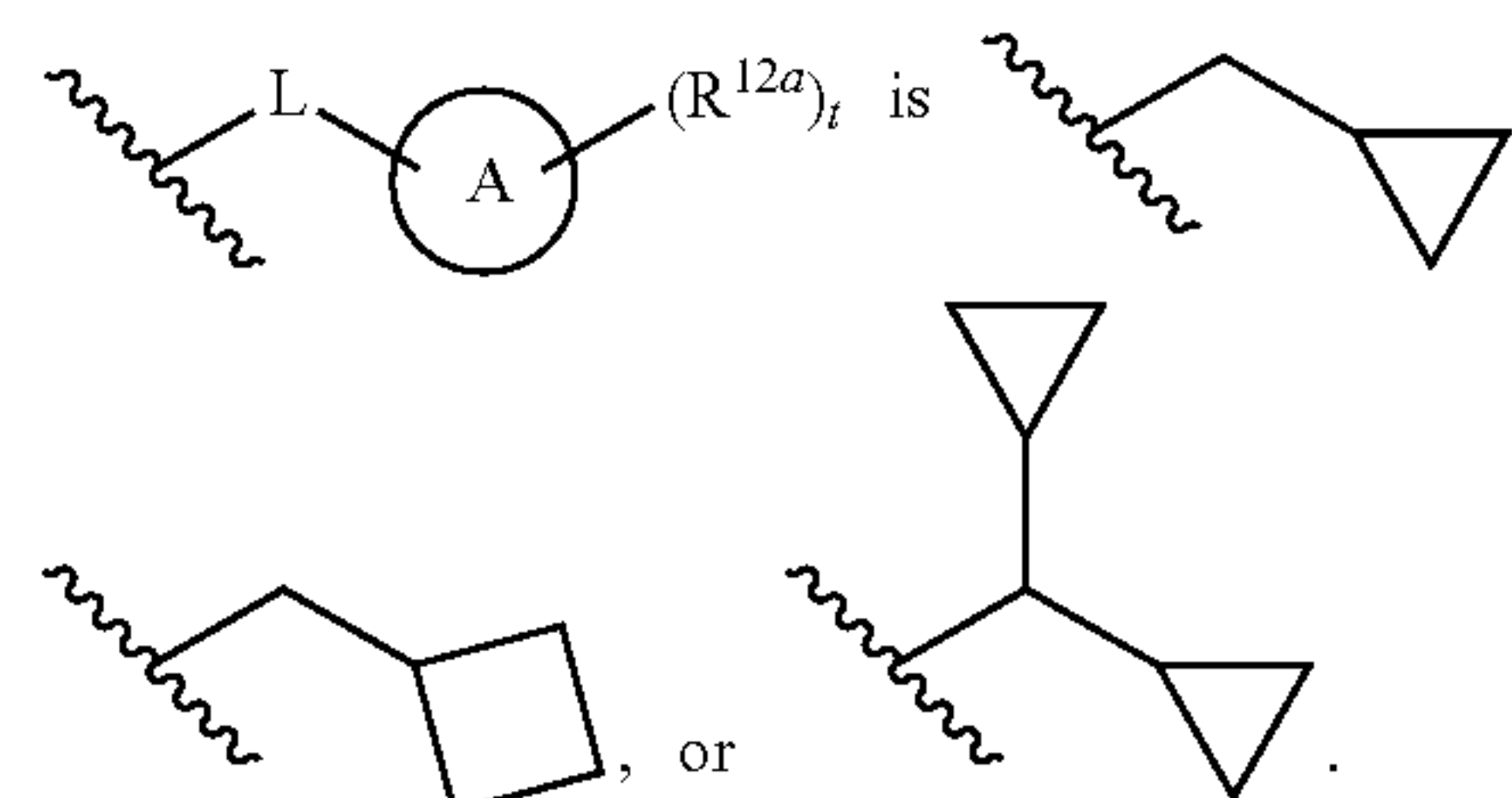
[Chemical Formula 75]
