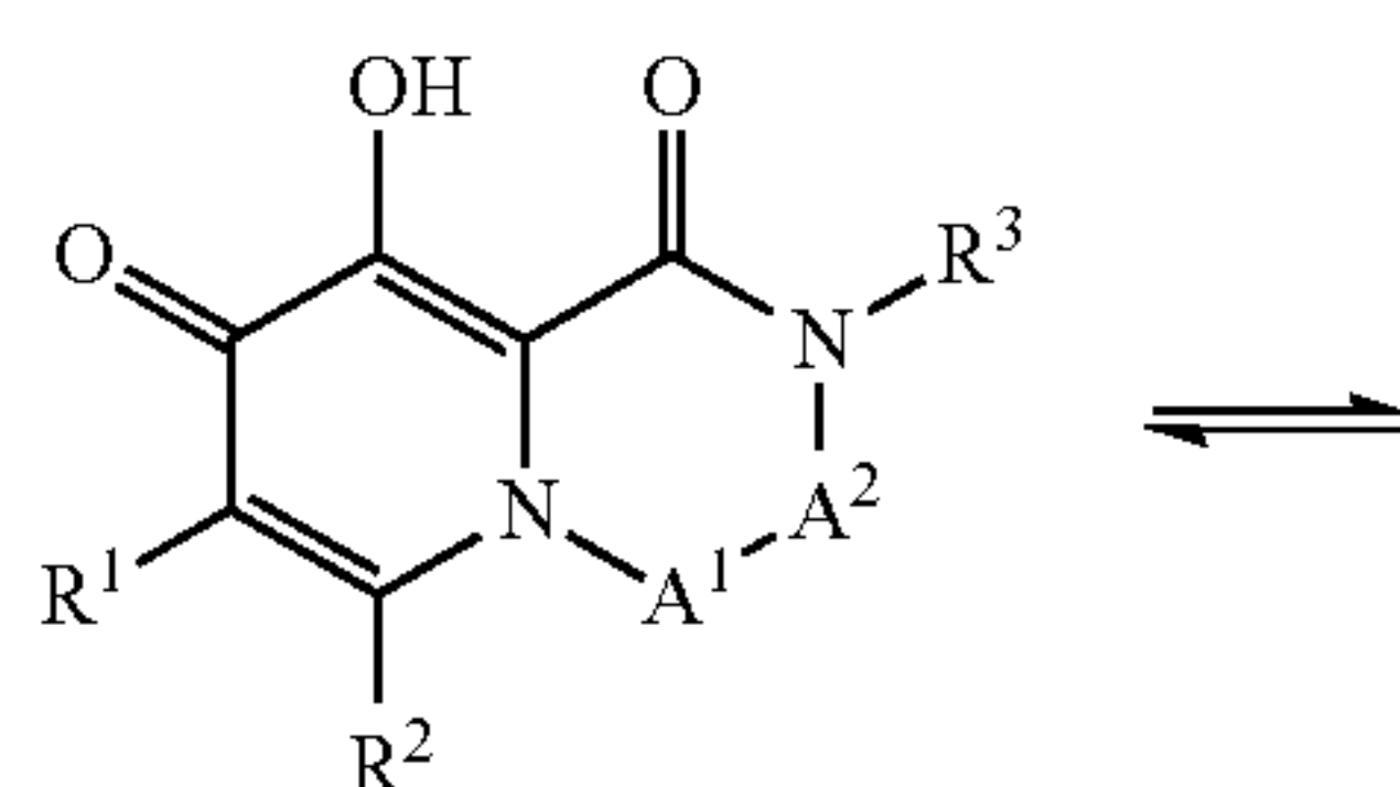
[Chemical Formula 86]
