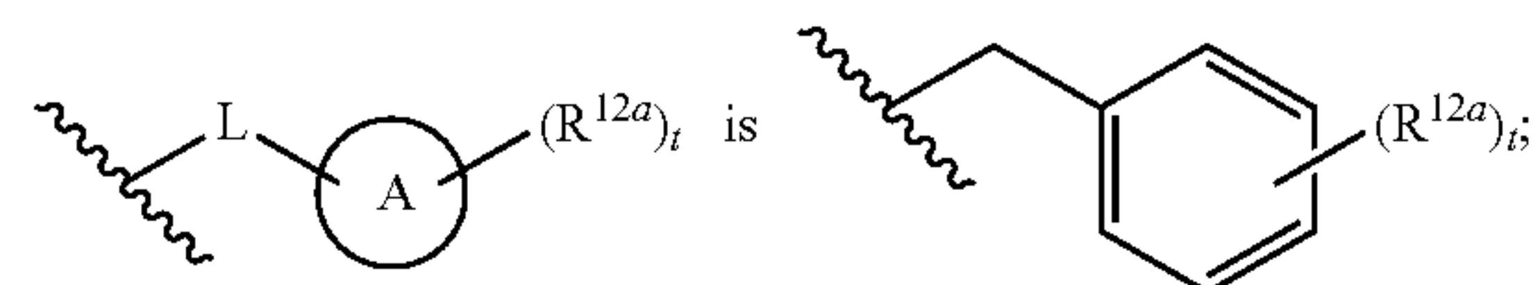
[Chemical Formula 76]
