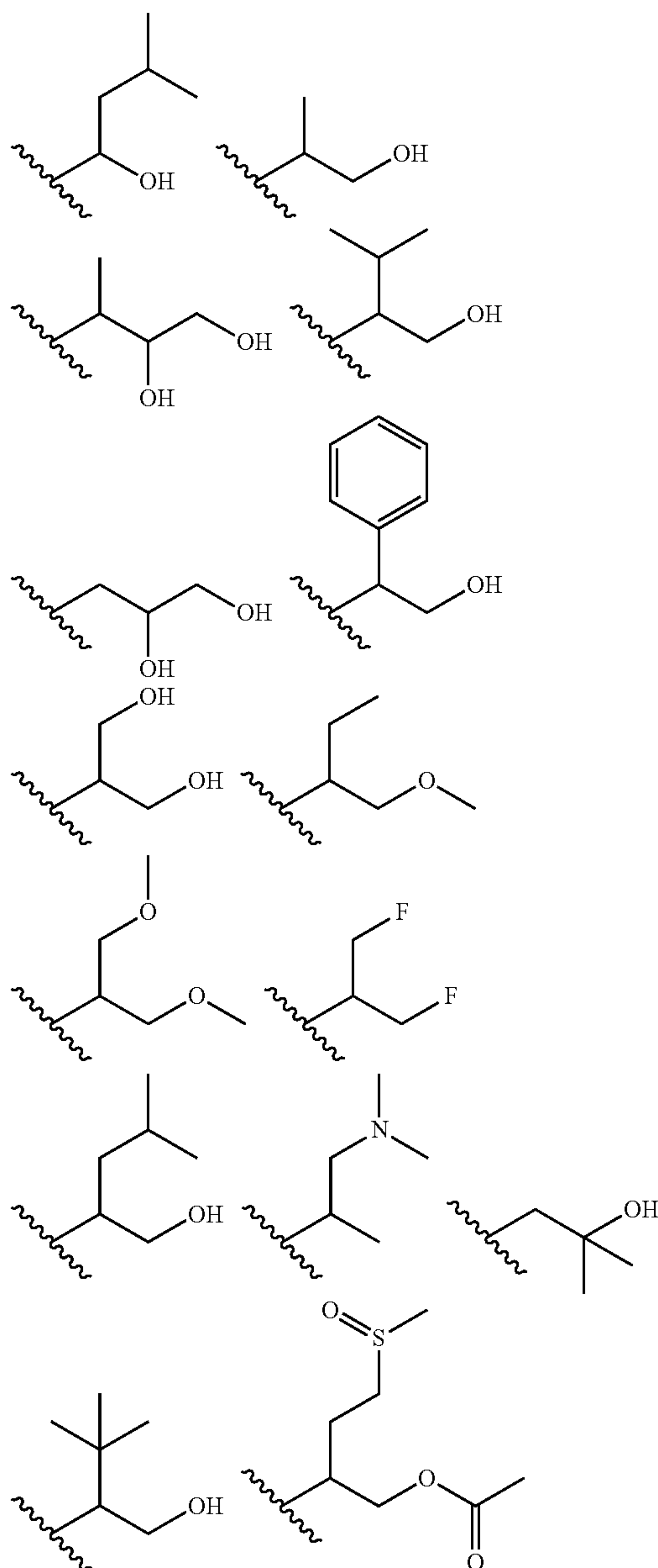
[Chemical Formula 47]
