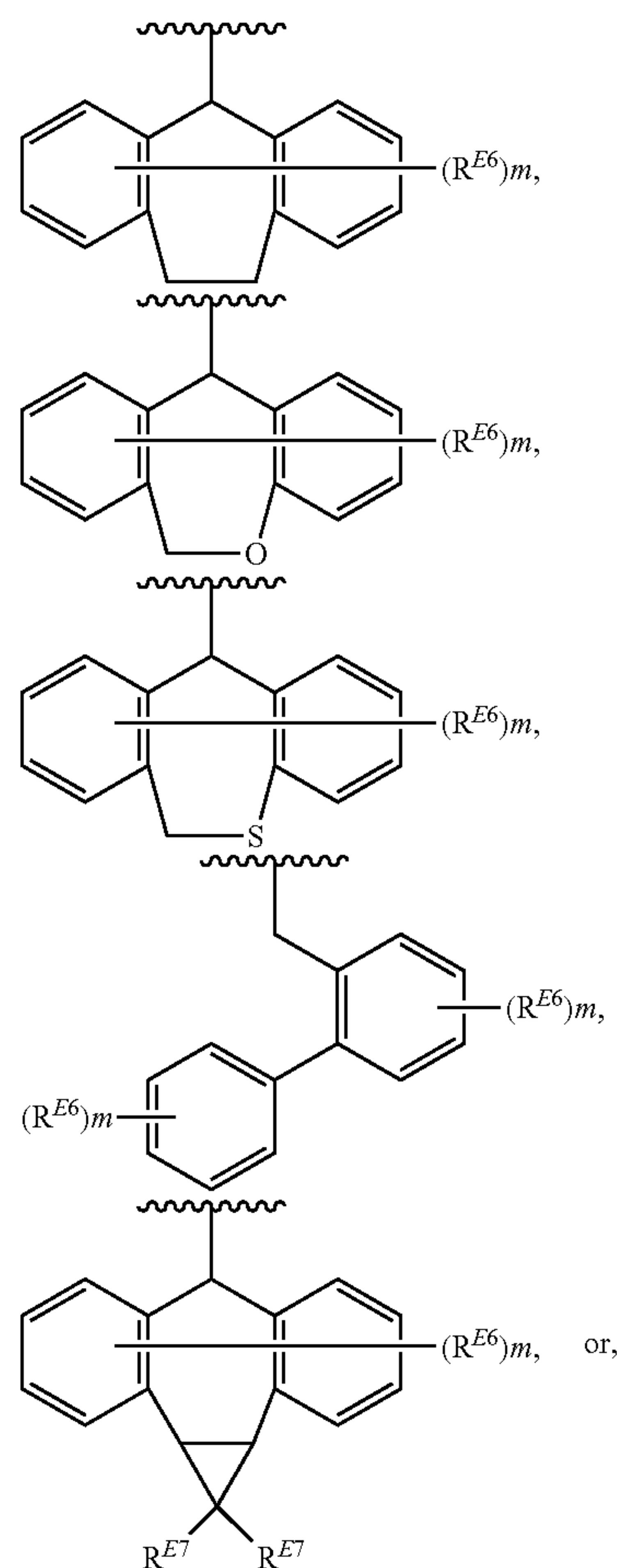
[Chemical Formula 5]
