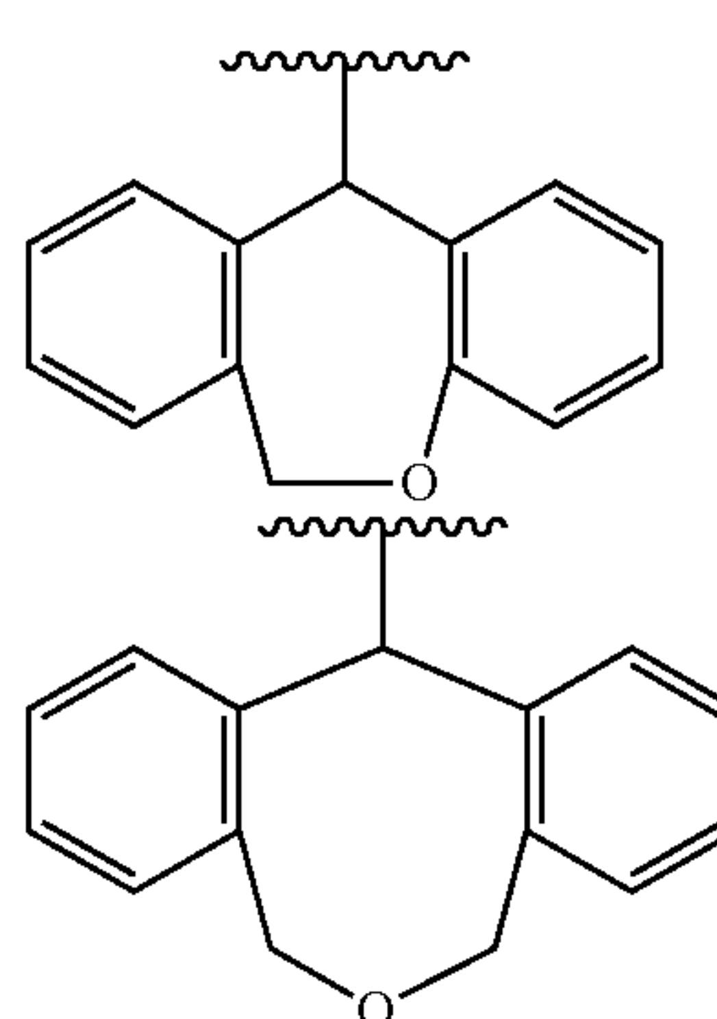
[Chemical Formula 16]
