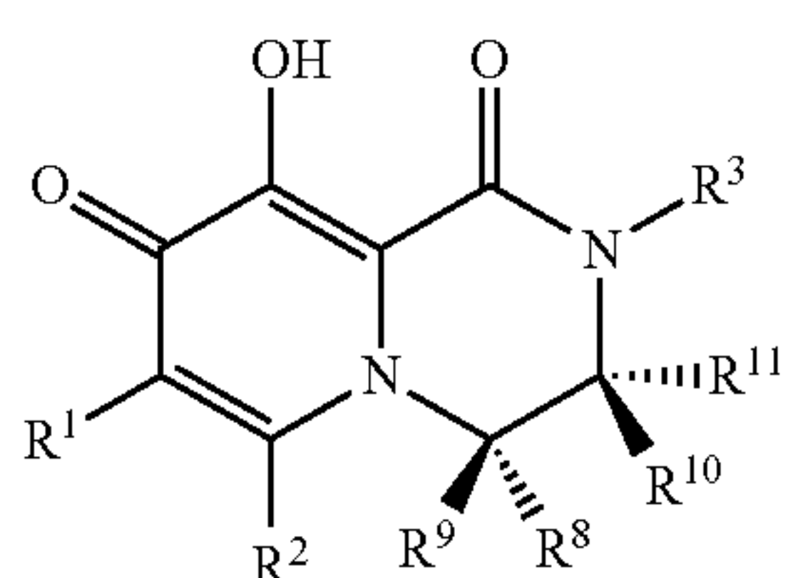
[Chemical Formula 86]
