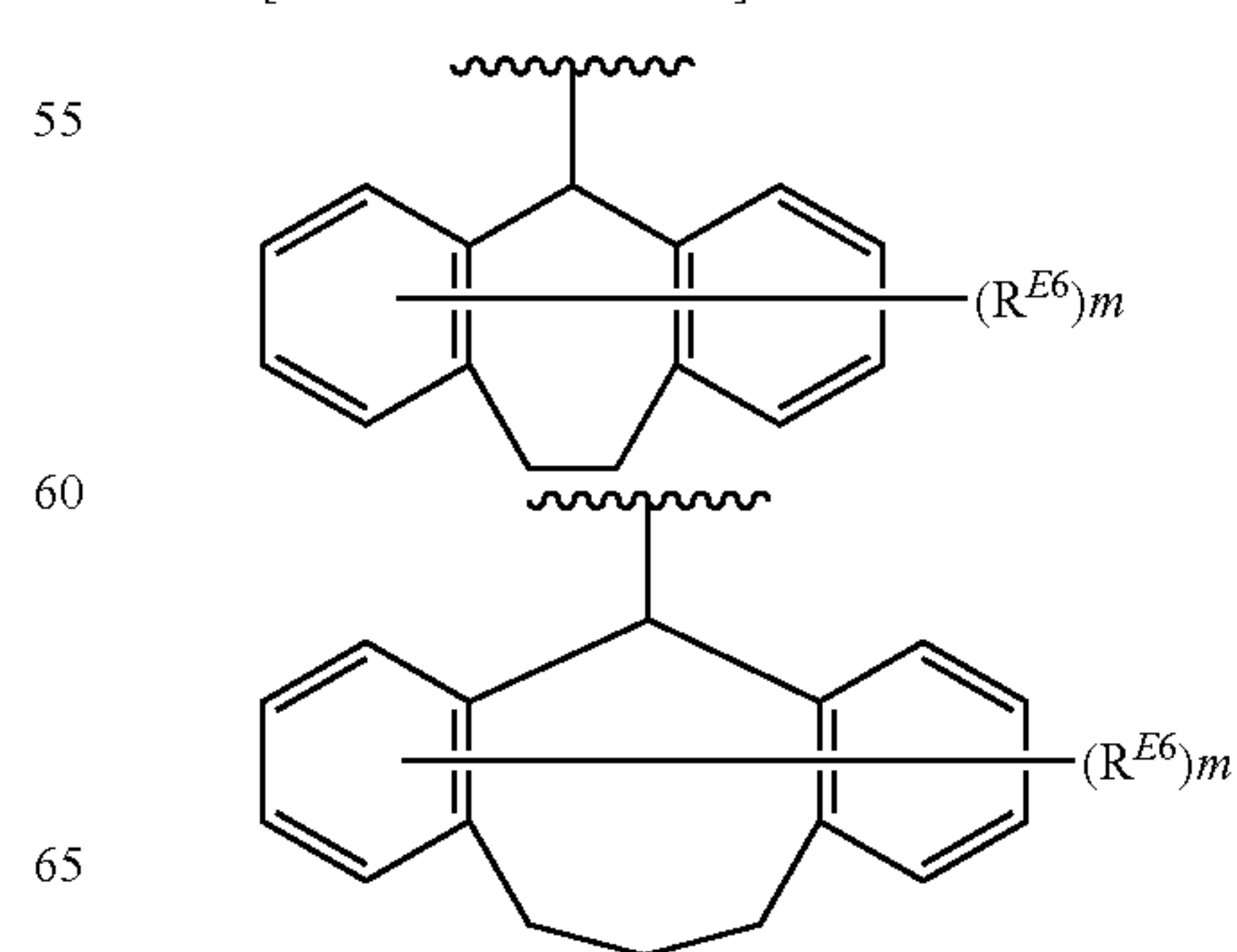
[Chemical Formula 62]
