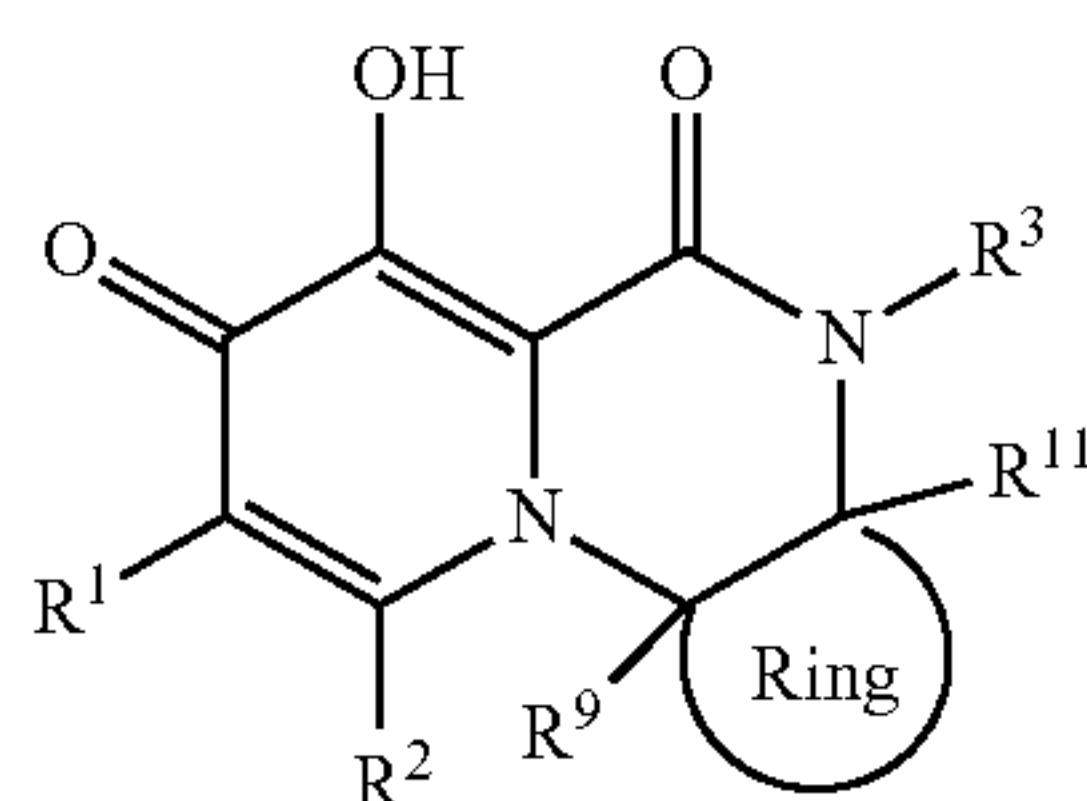
[Chemical Formula 42]
