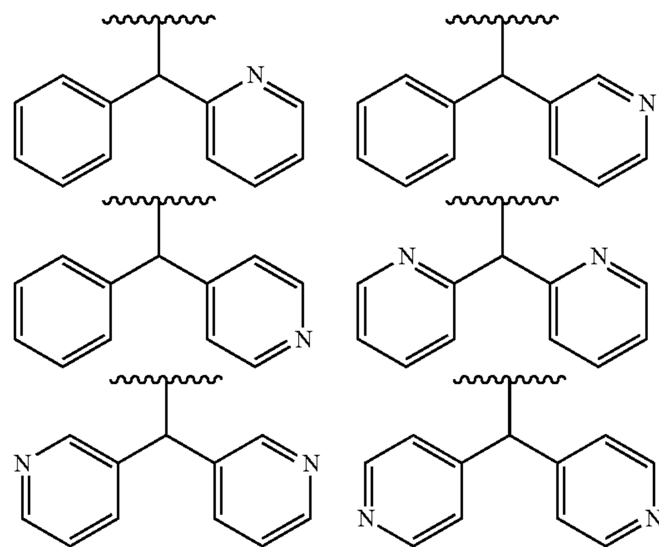
[Chemical Formula 19]
