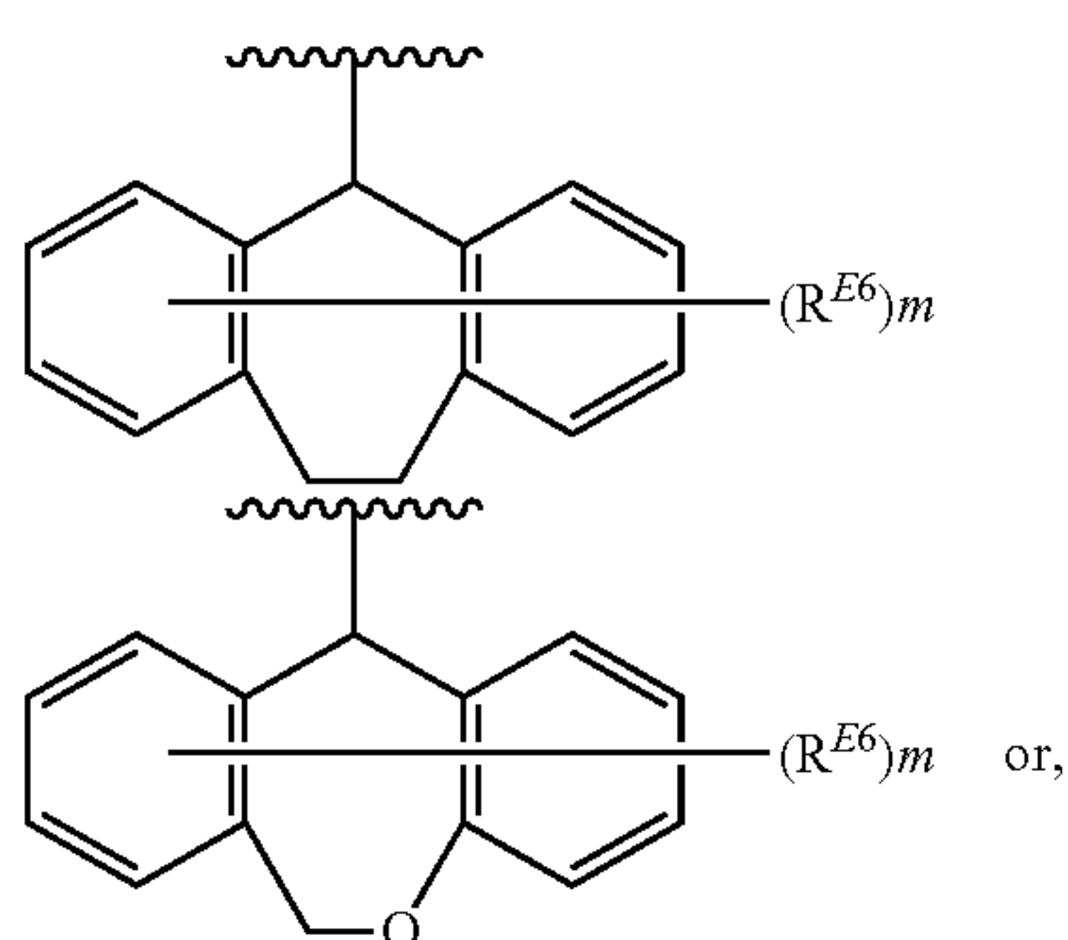
[Chemical Formula 68]
