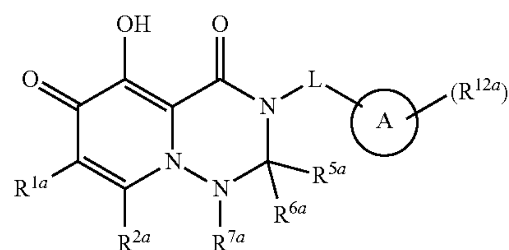
[Chemical Formula 7]
