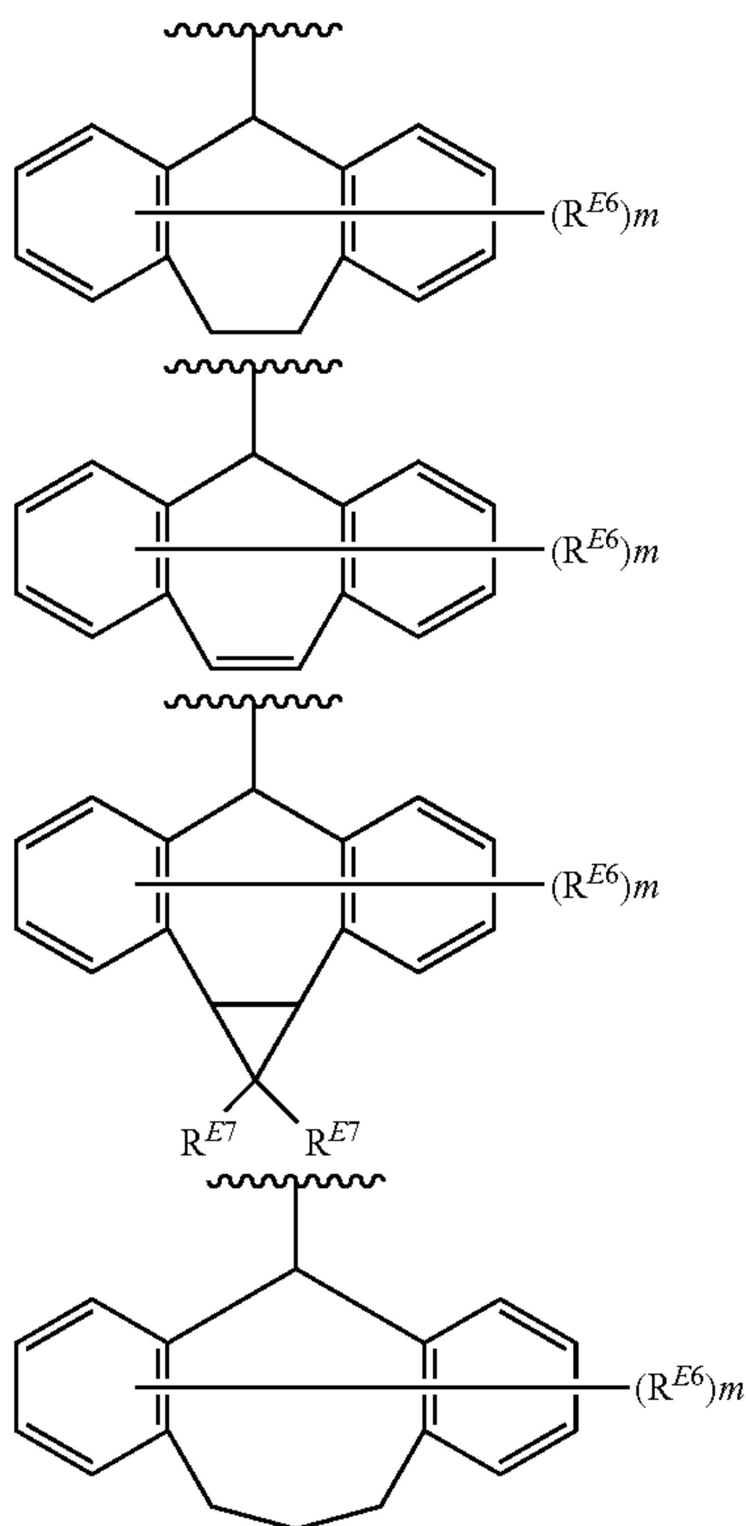
[Chemical Formula 71]
