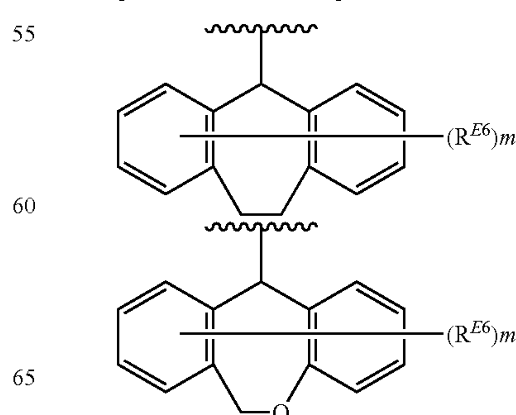
[Chemical Formula 65]
