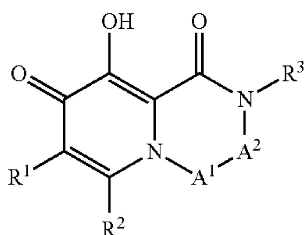
[Chemical Formula 11]
