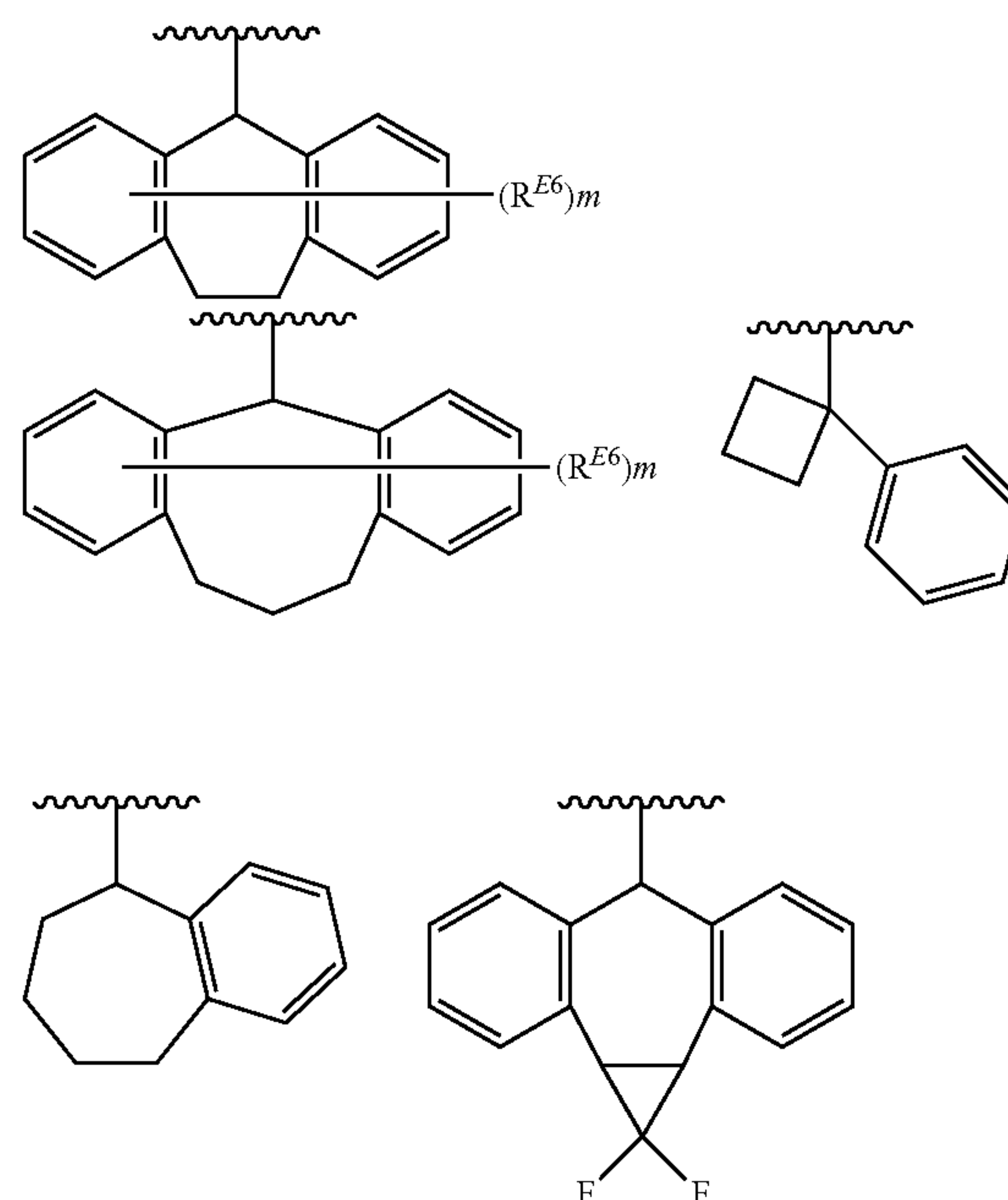
[Chemical Formula 48]
