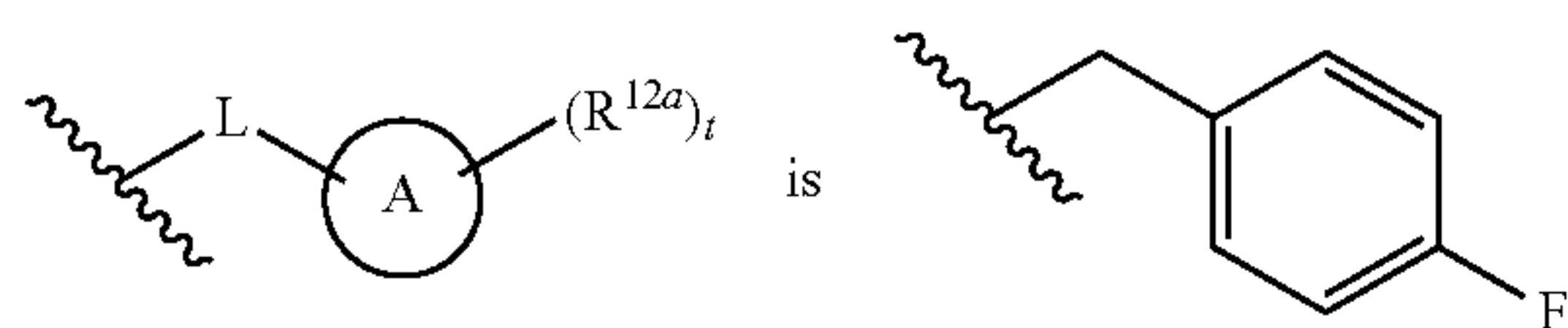
[Chemical Formula 8]
