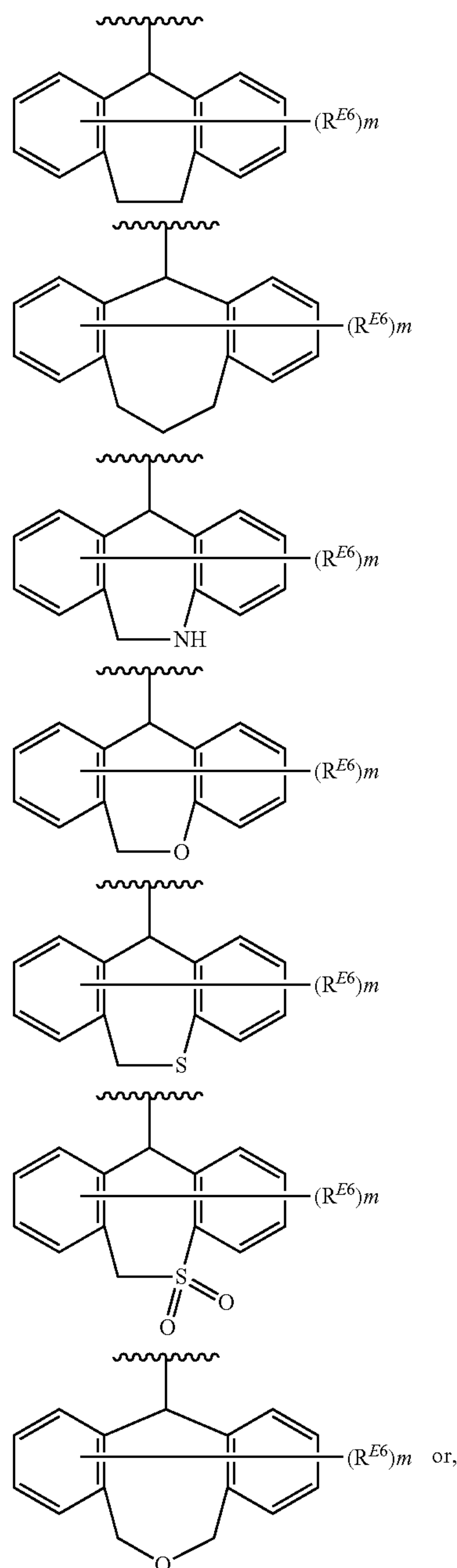
[Chemical Formula 21]
