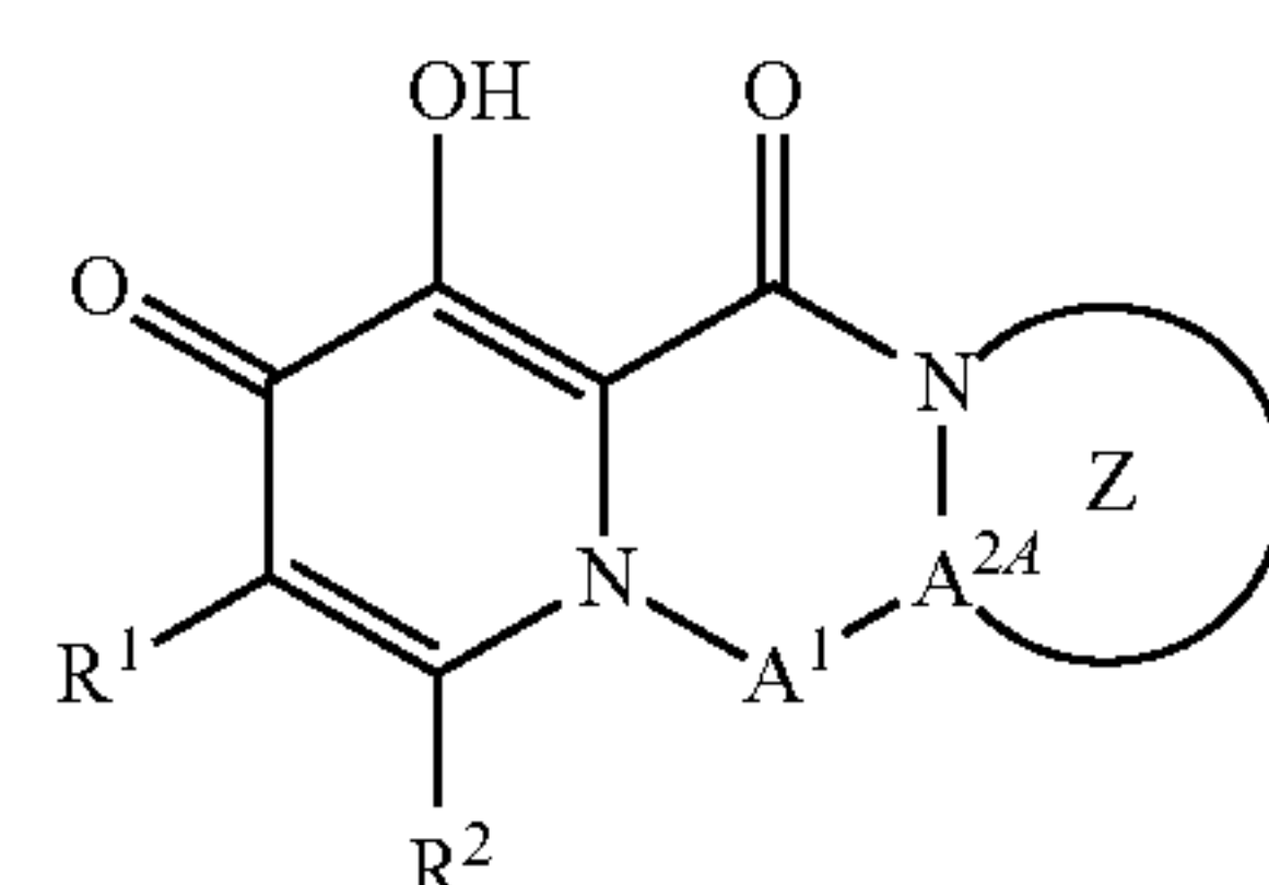
[Chemical Formula 58]
