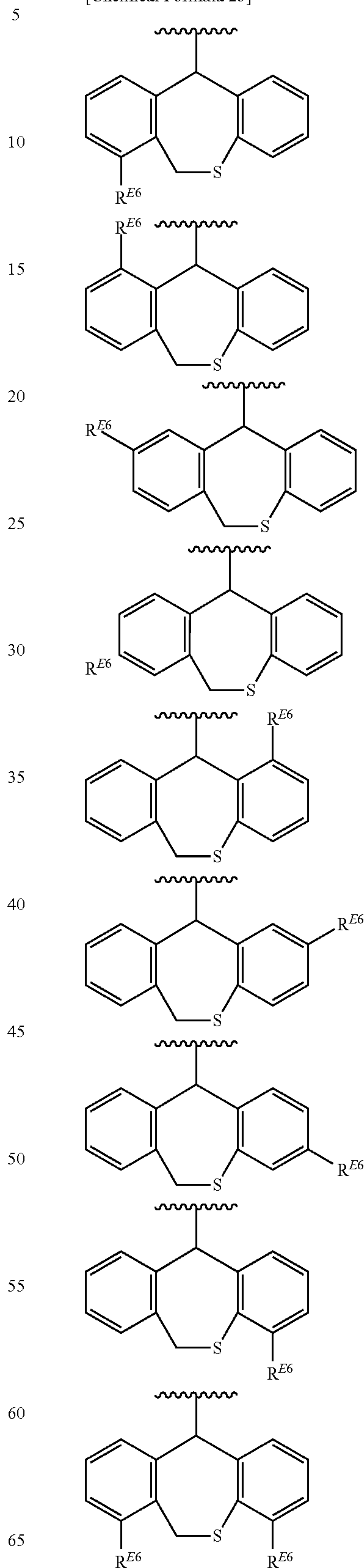
[Chemical Formula 25]
