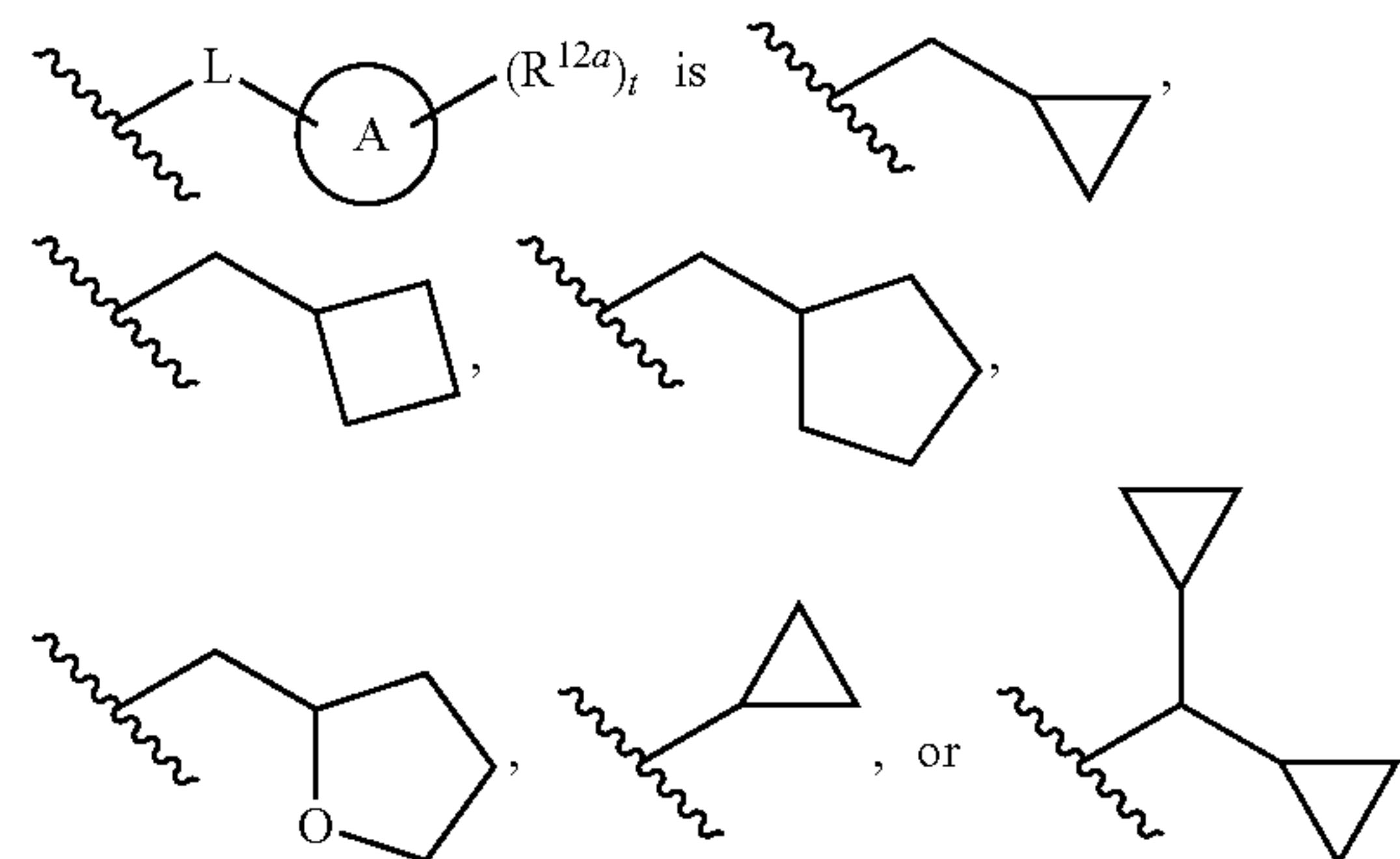
[Chemical Formula 74]
