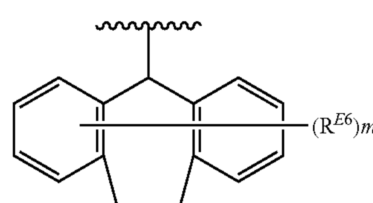
[Chemical Formula 13]
