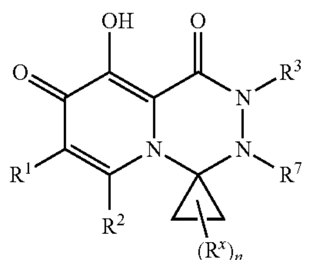
[Chemical Formula 27]
