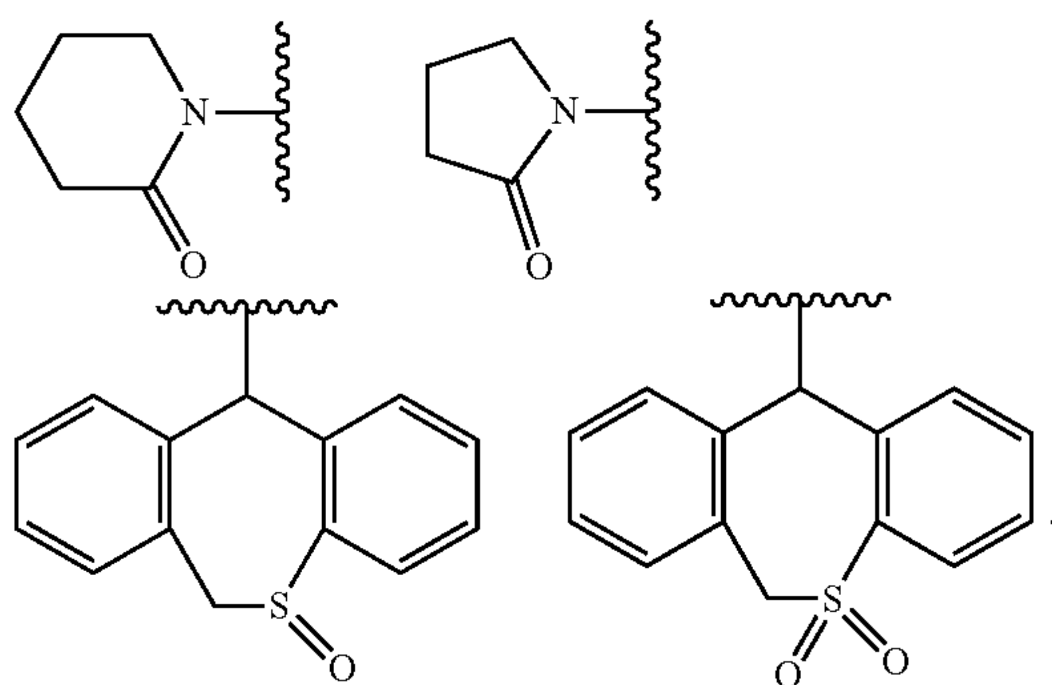
[Chemical Formula 17]
