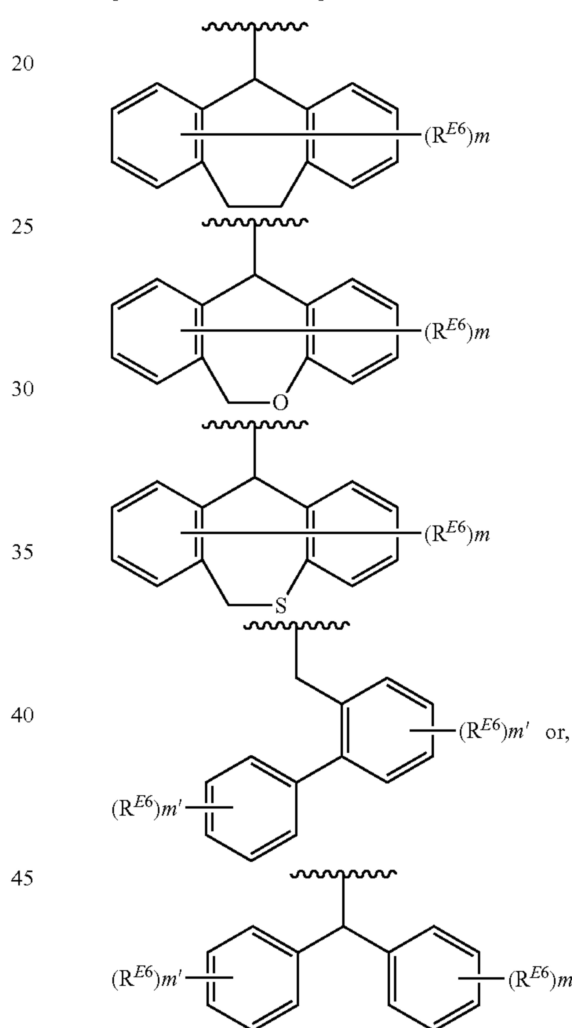
[Chemical Formula 69]
