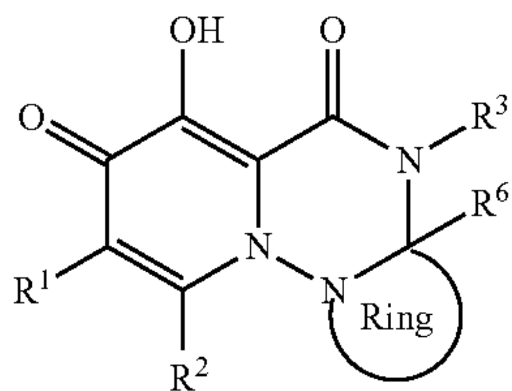
[Chemical Formula 37]
