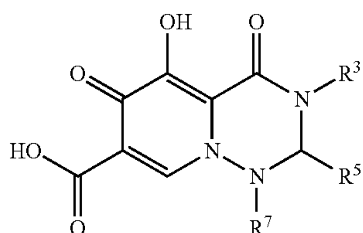
[Chemical Formula 70]
