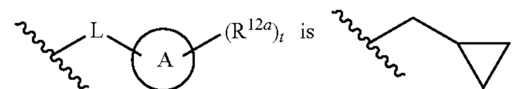
[Chemical Formula 76]
