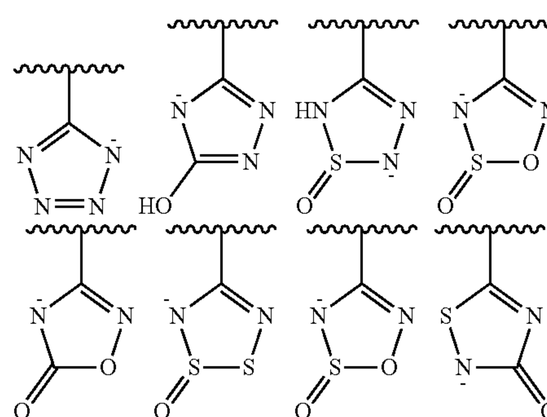
[Chemical Formula 53]
