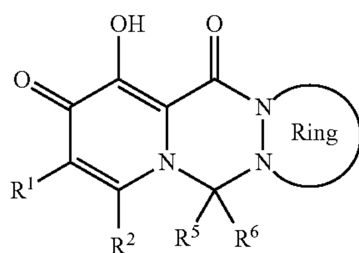
[Chemical Formula 59]
