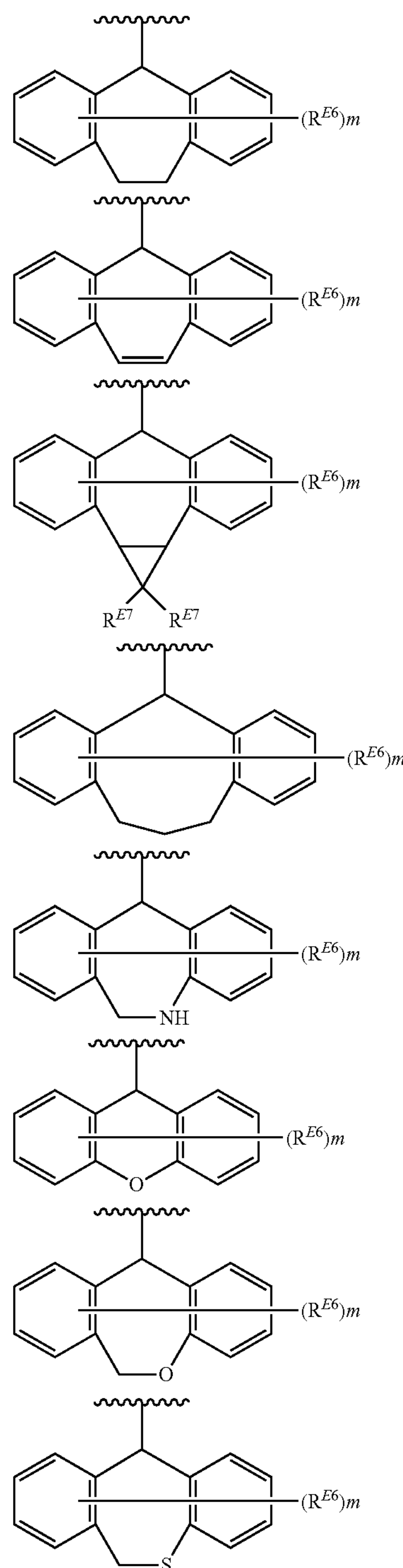
[Chemical Formula 60]
