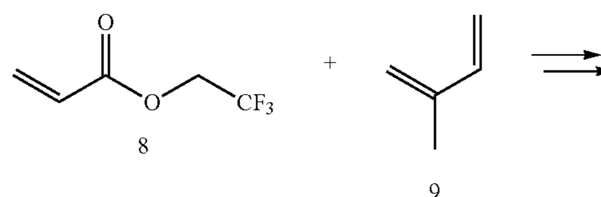
Scheme 9
