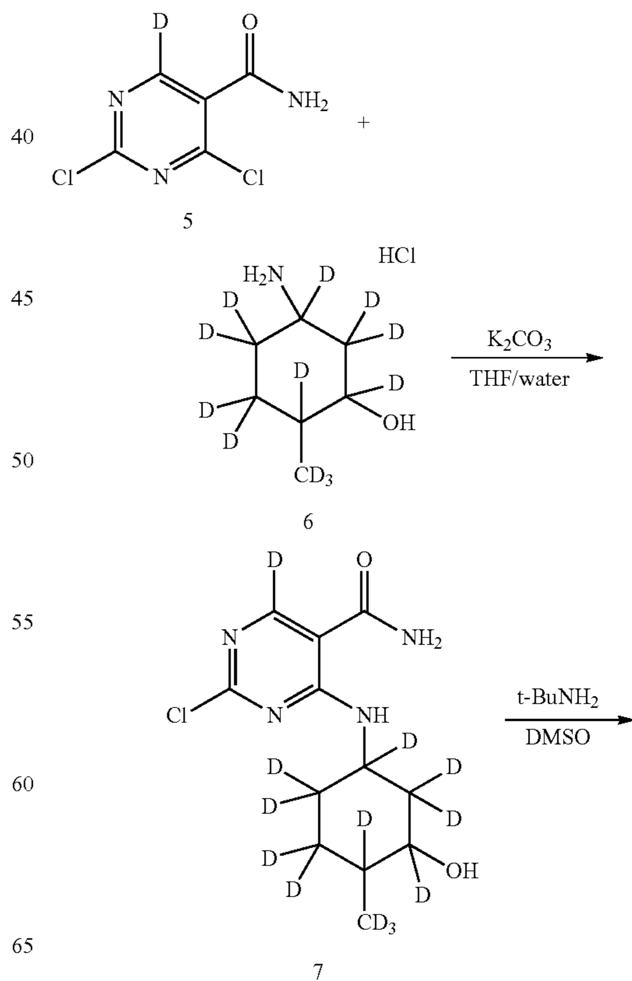
Scheme 19
