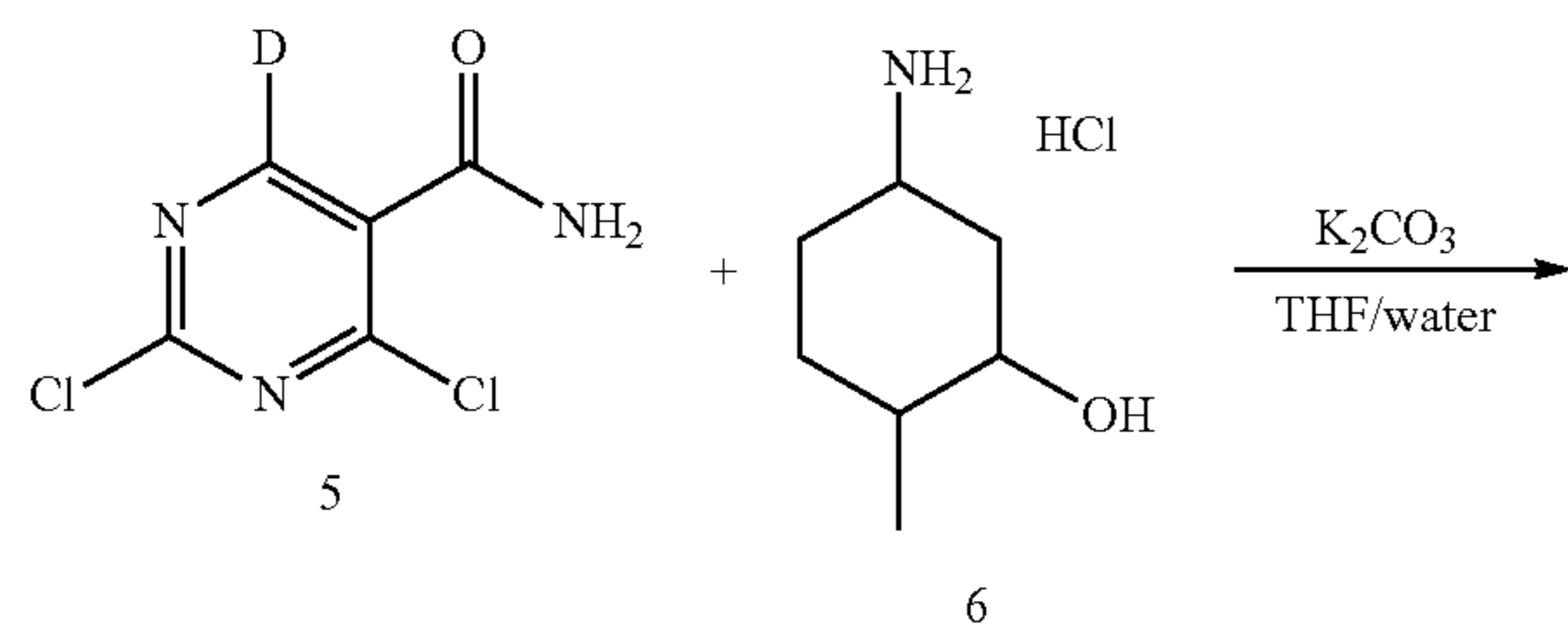
Scheme 17
