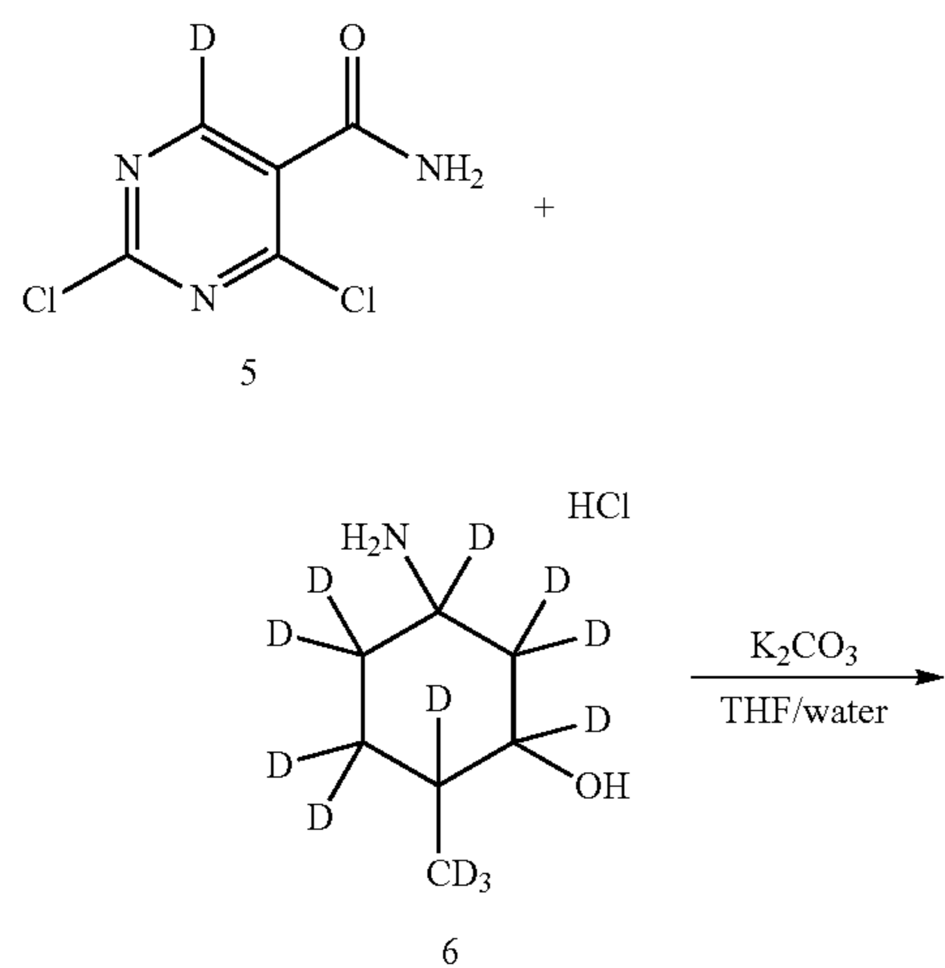
Scheme 18
