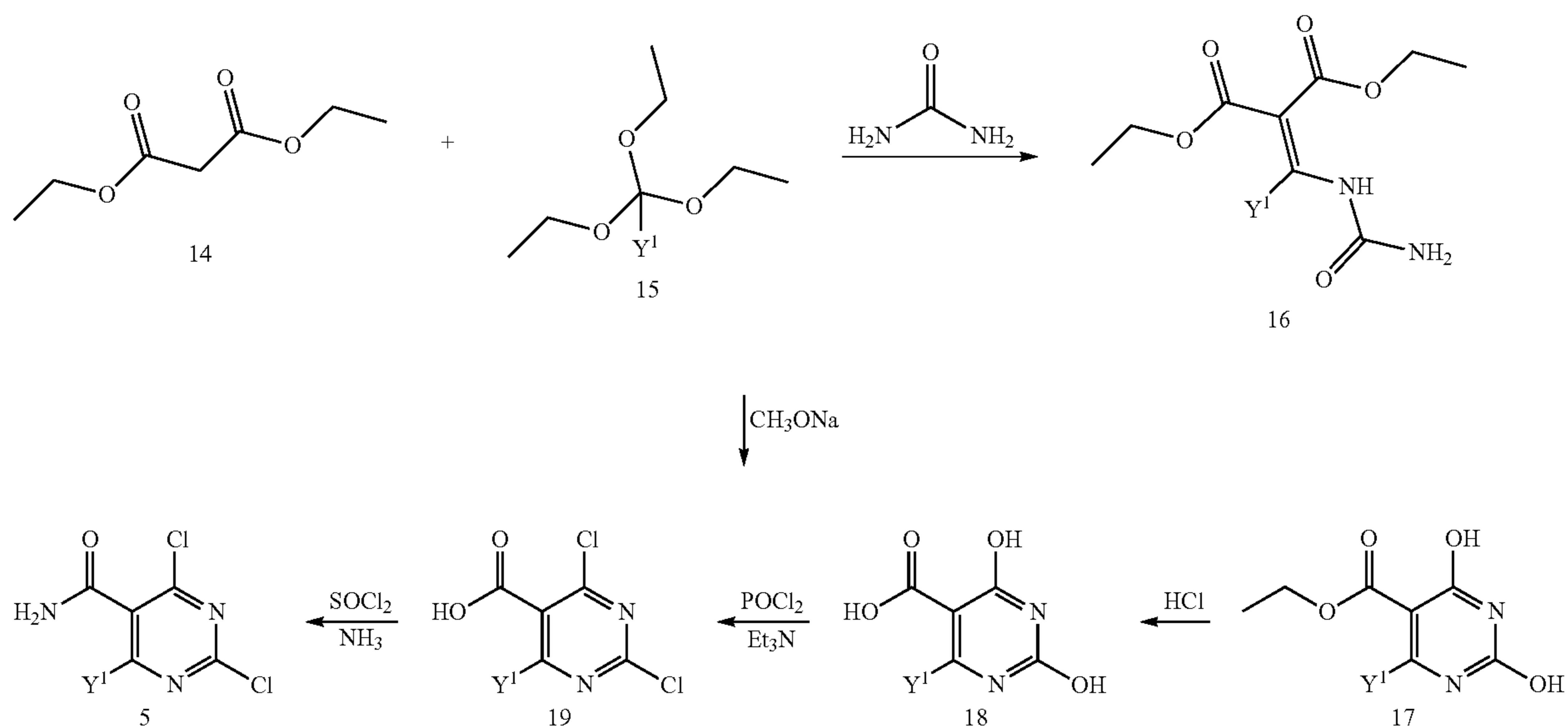
Scheme 6
