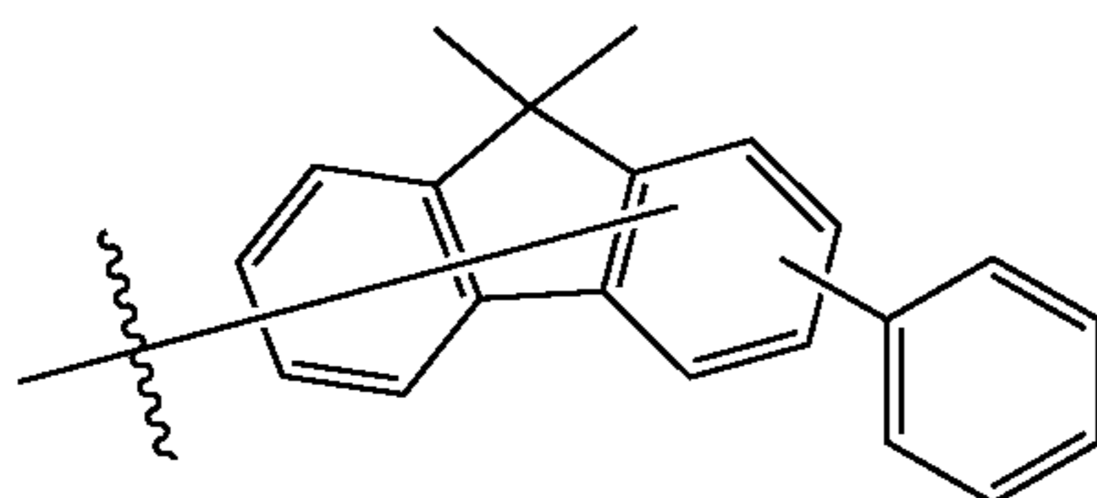
Substituent B31
