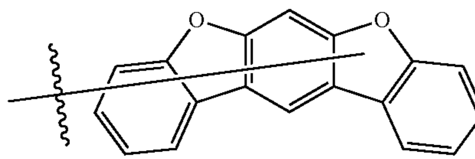
Substituent 36
