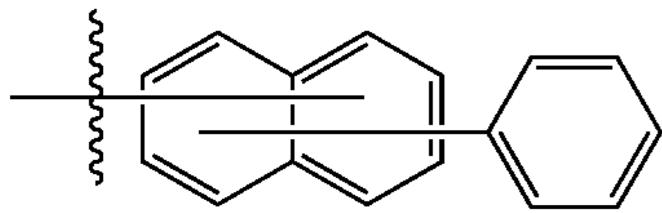
Substituent B3
