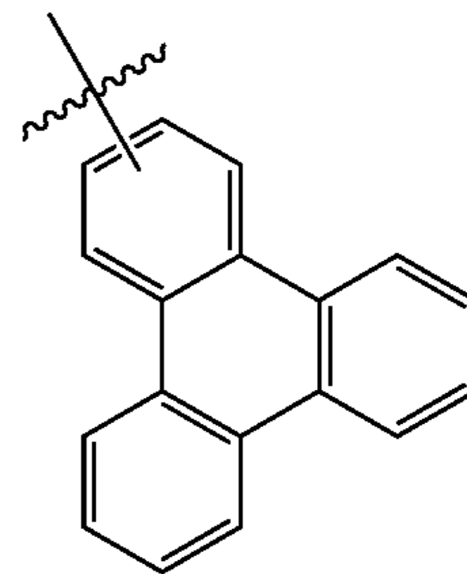
Substituent B6
