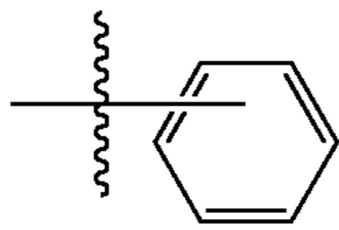
Substituent B1
