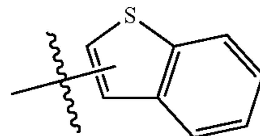
Substituent B20
