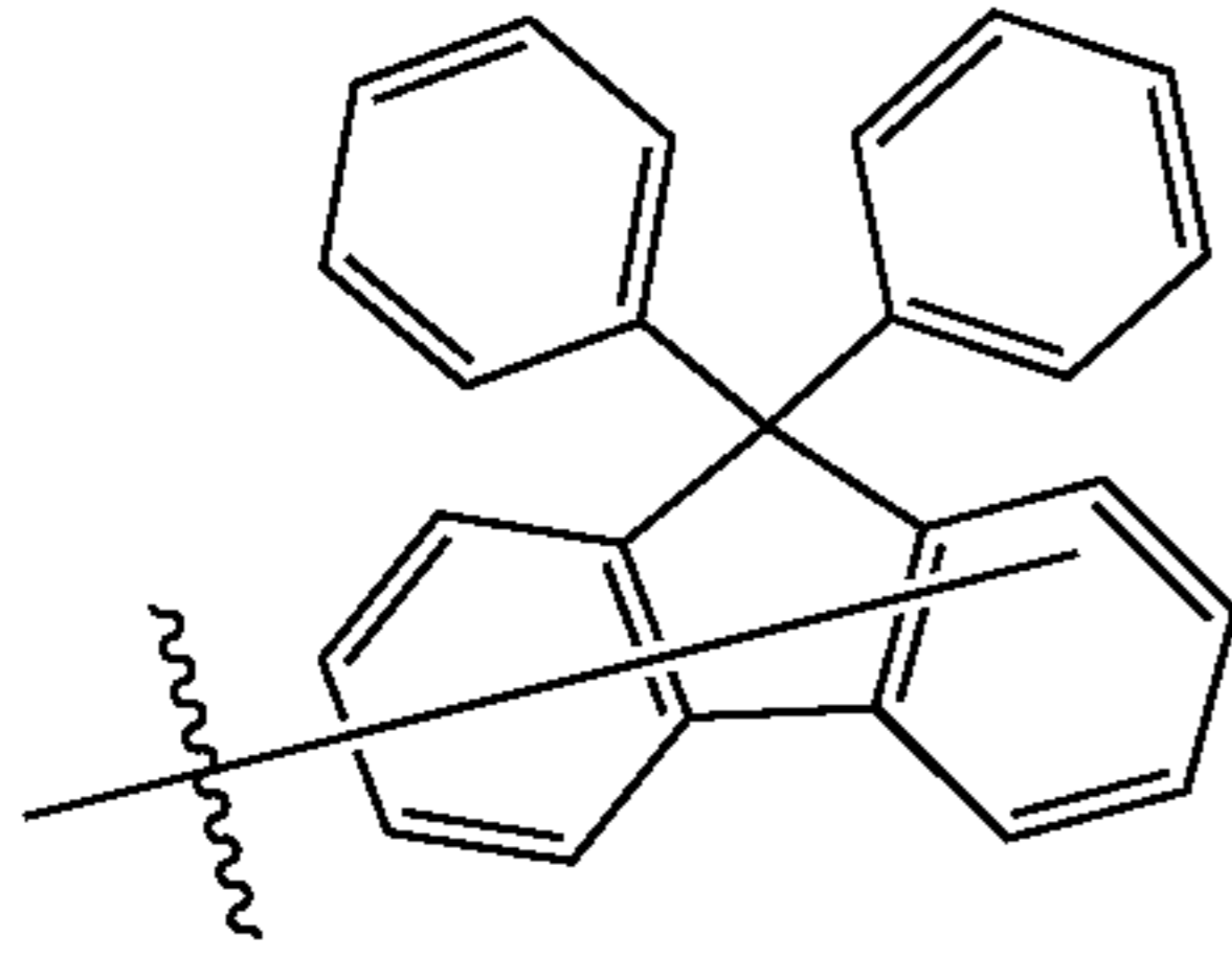
Substituent 17
