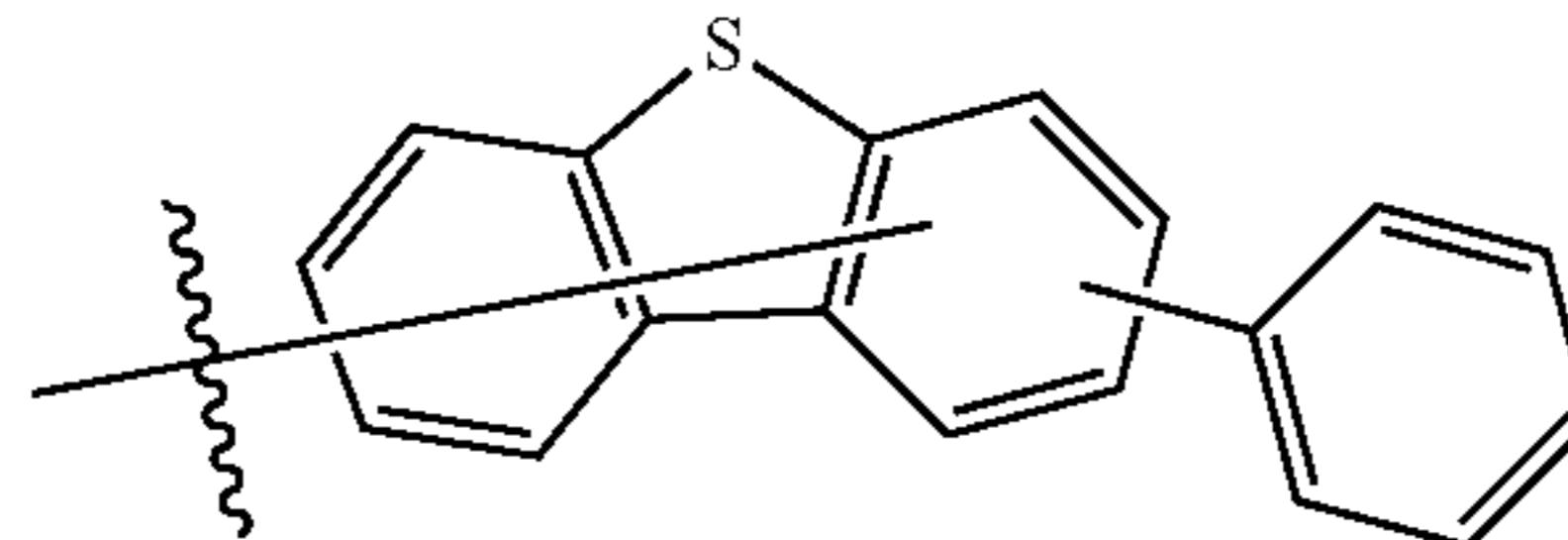
Substituent 26
