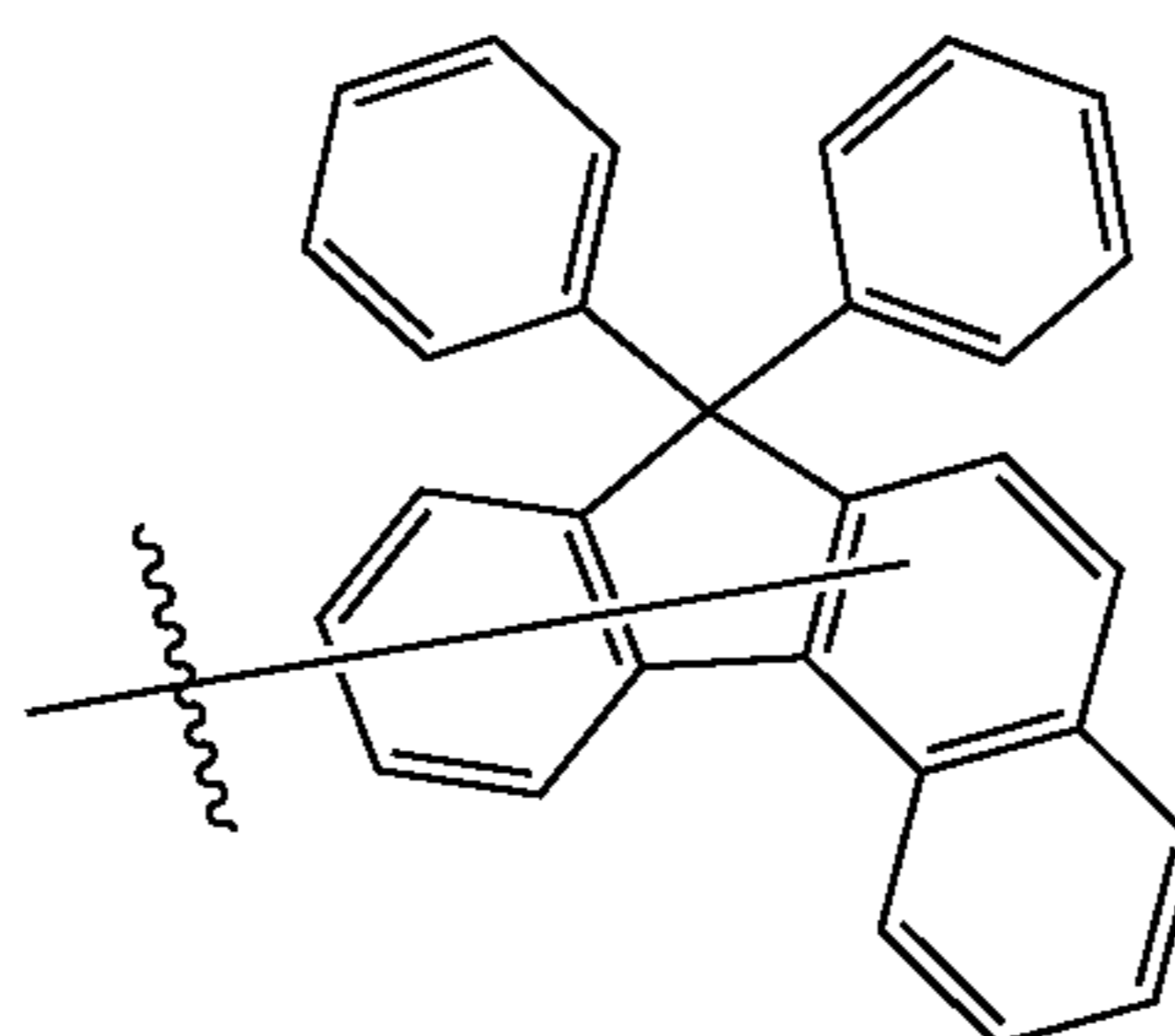
Substituent B34
