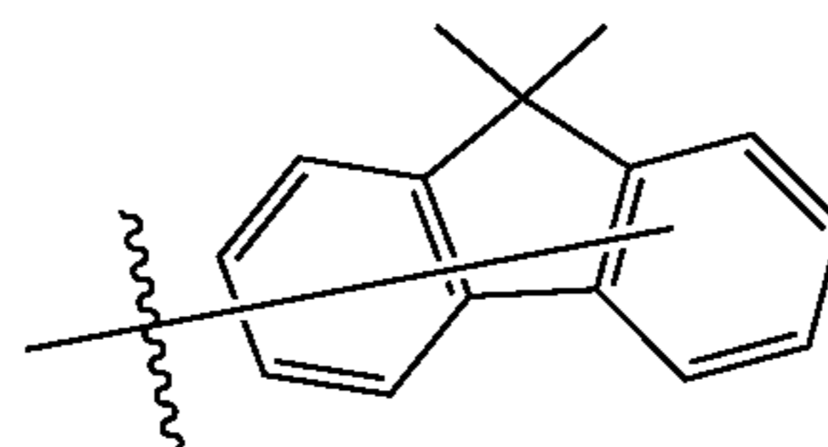
Substituent 14
