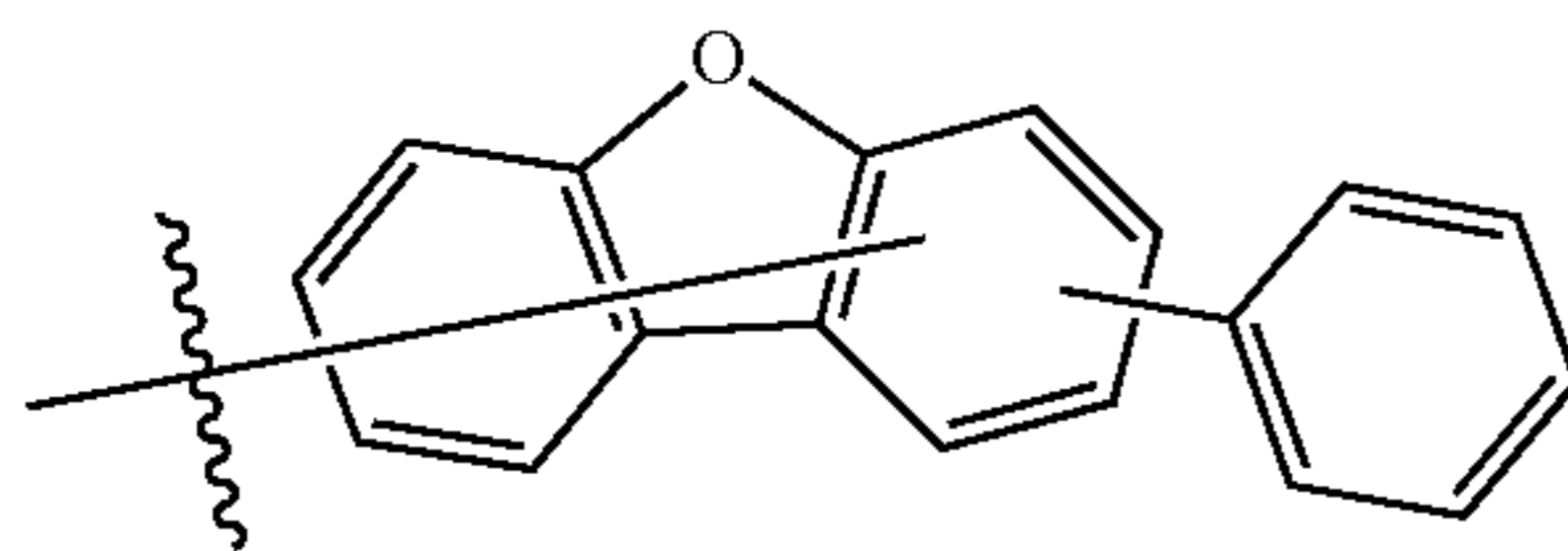
Substituent 27
