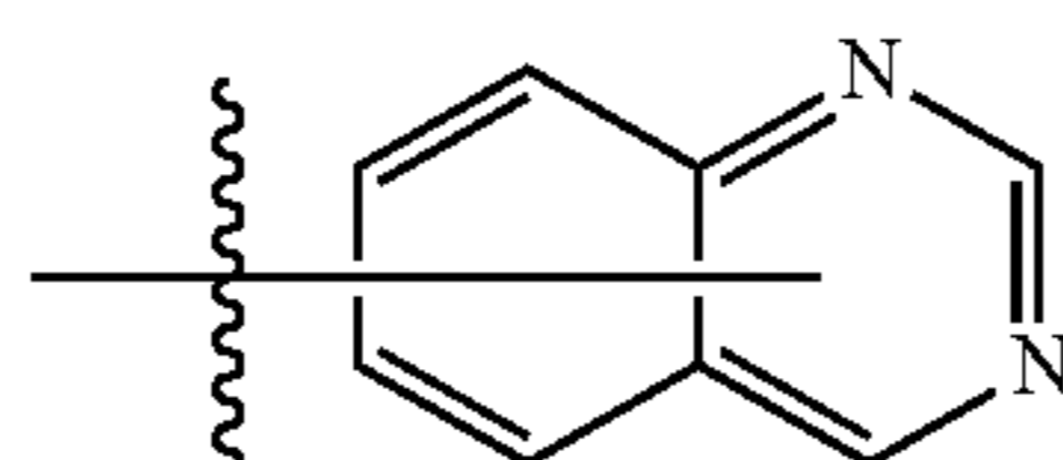
Substituent 44
