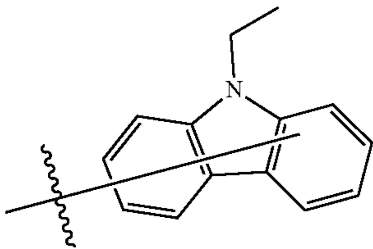
Substituent B13
