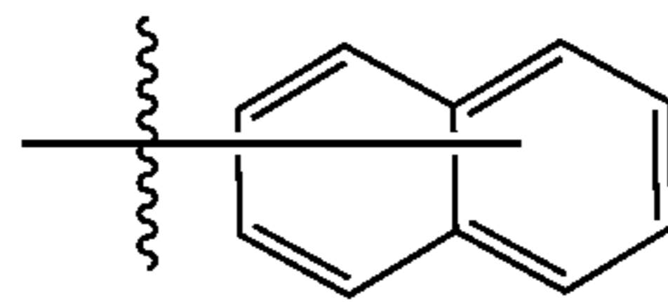
Substituent B2
