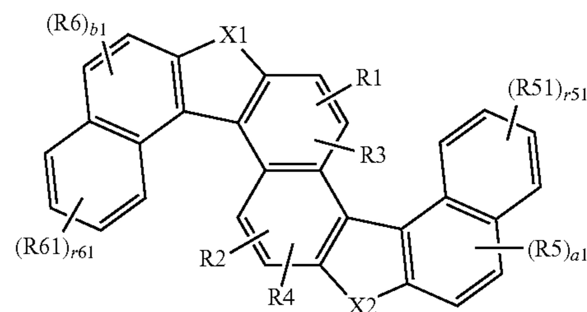
[Formula 1-2]
