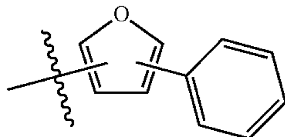
Substituent B19
