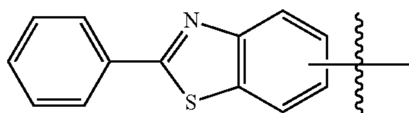
Substituent 51
