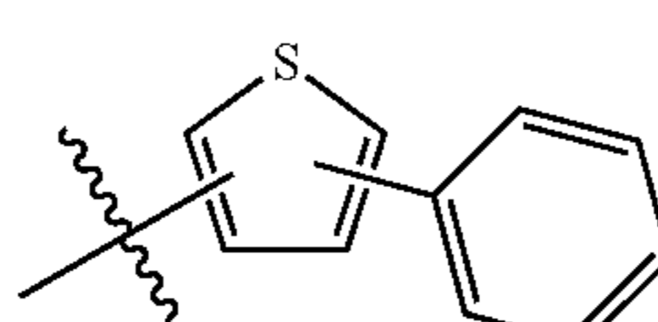
Substituent B18
