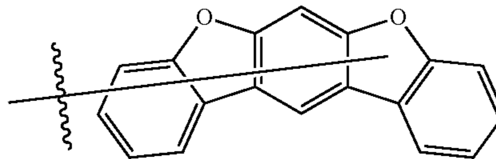
Substituent 36
