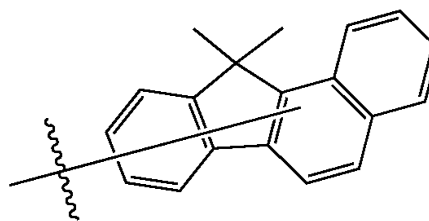
Substituent B28
