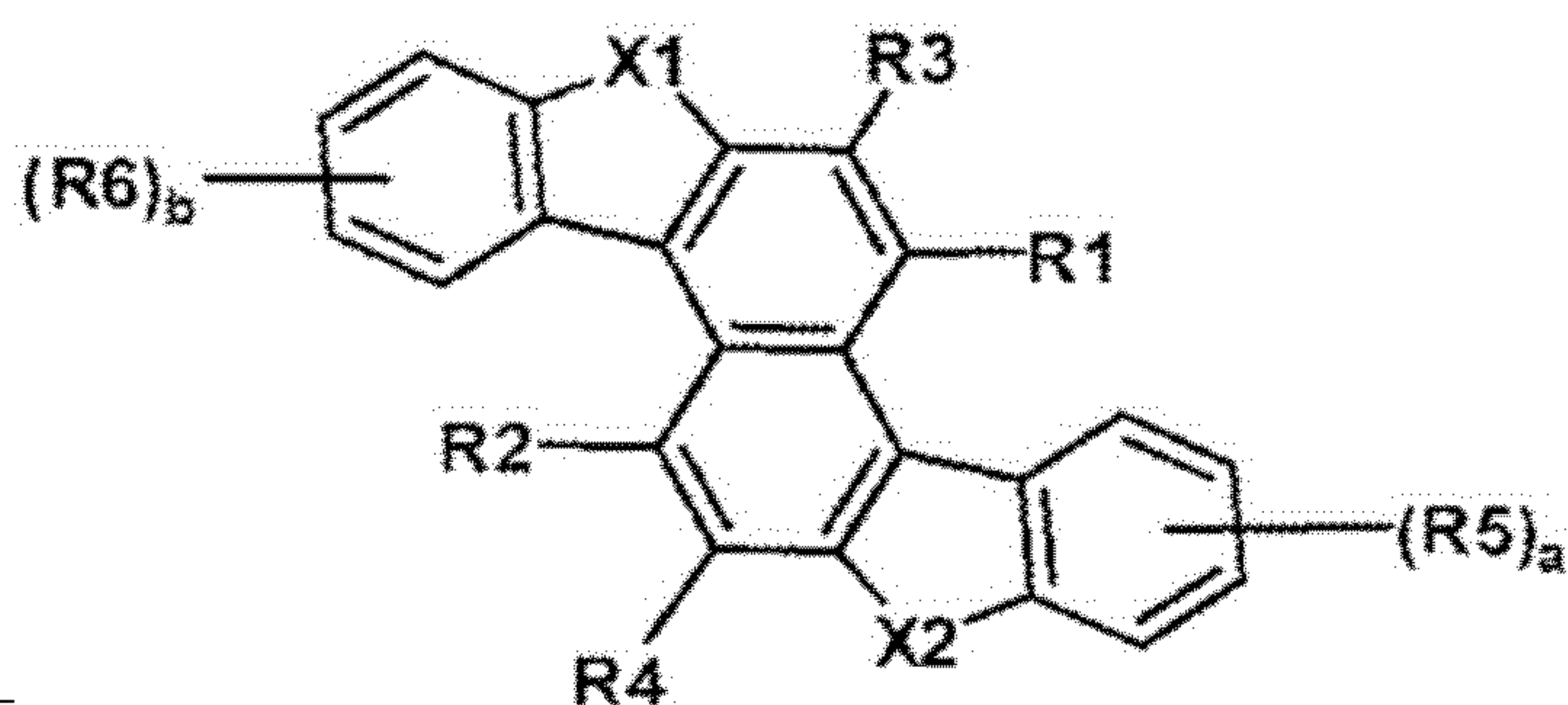
Chemical Formula 1-7
