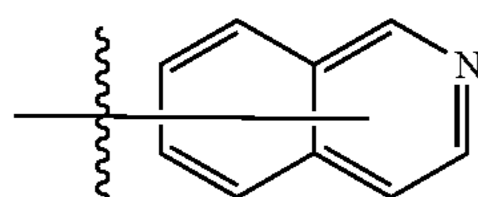
Substituent 42
