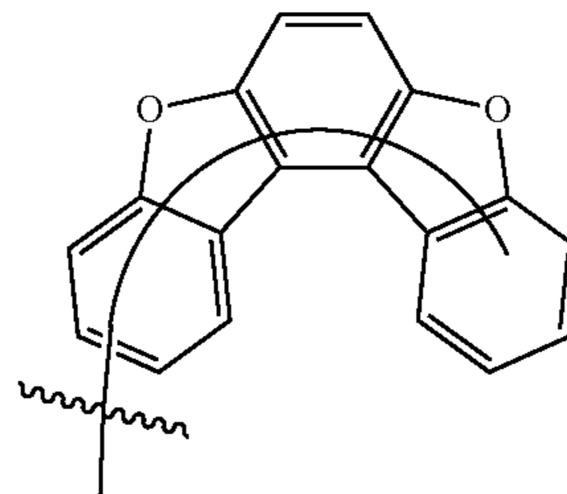
Substituent 40
