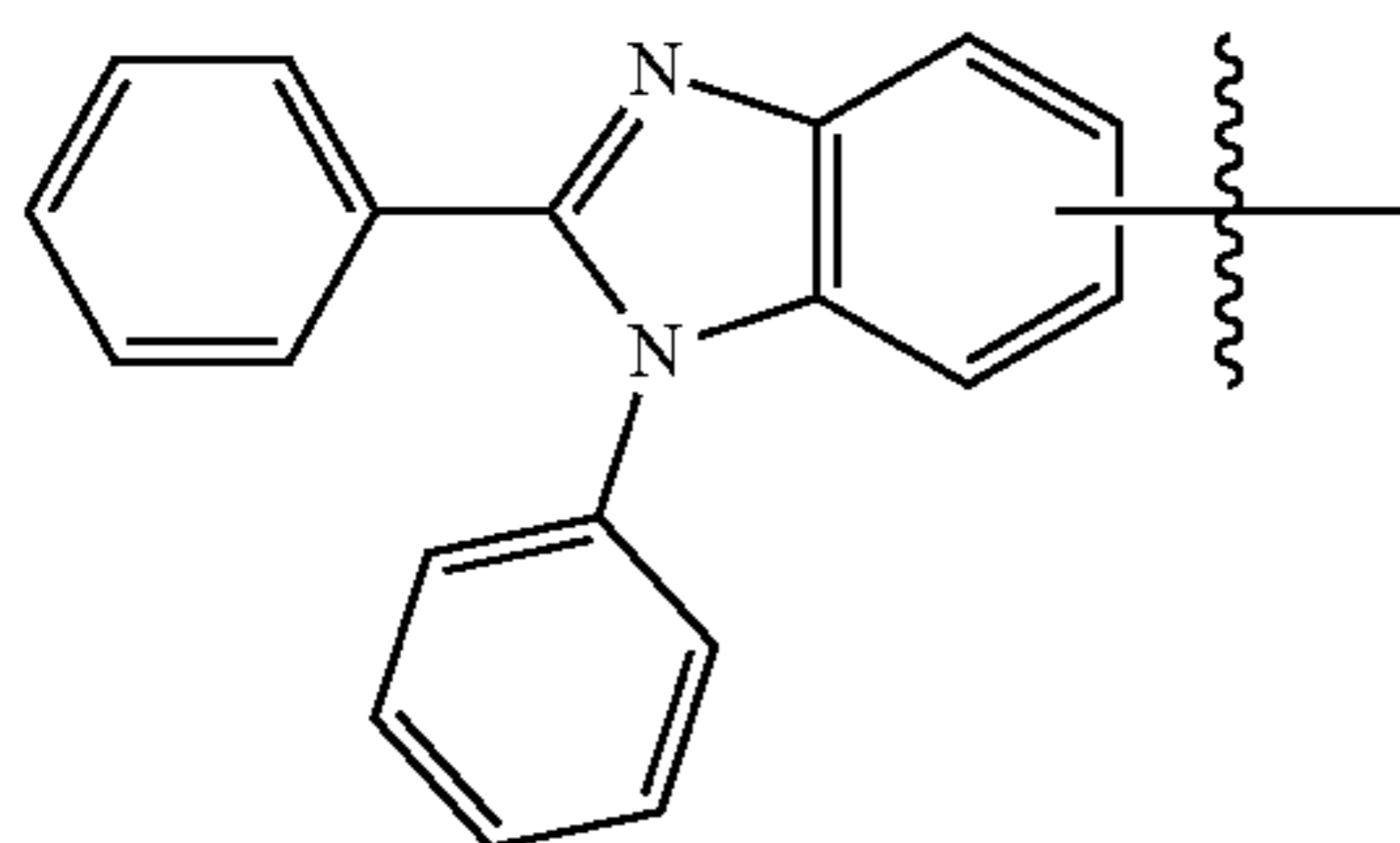
Substituent 47
