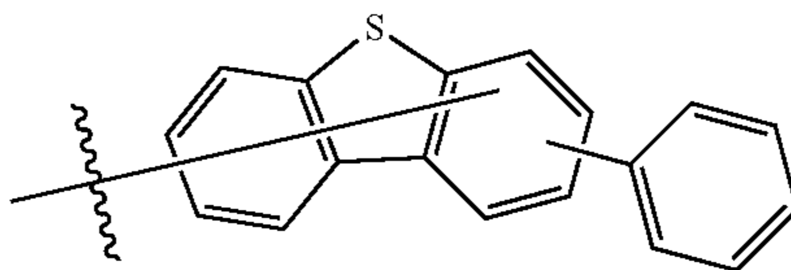
Substituent B26
