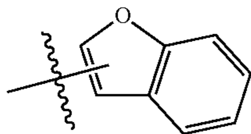
Substituent B21
