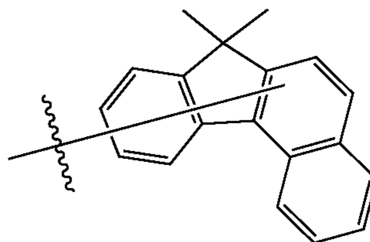
Substituent B30
