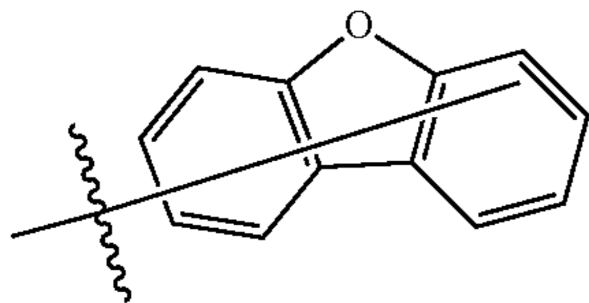
Substituent B7
