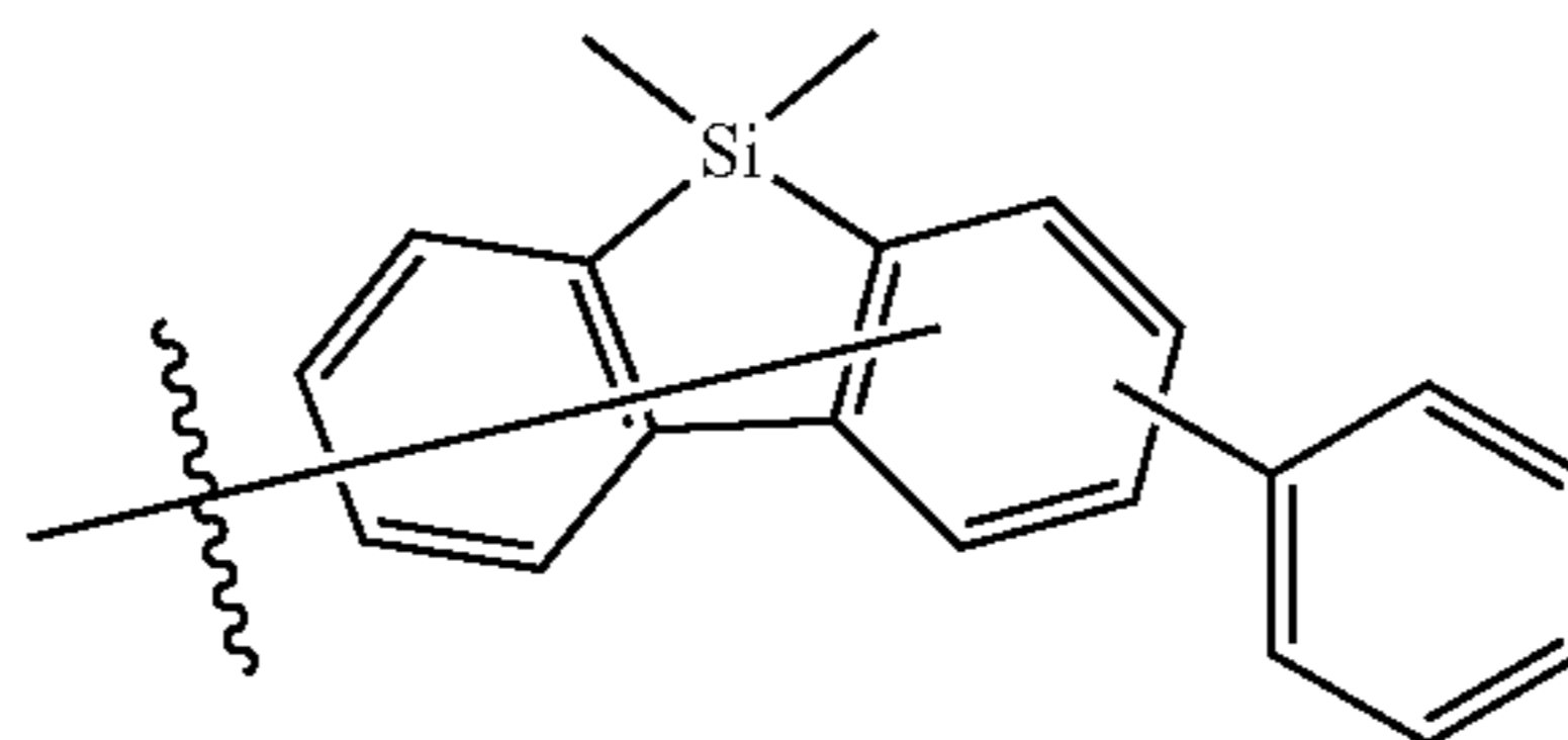
Substituent 54
