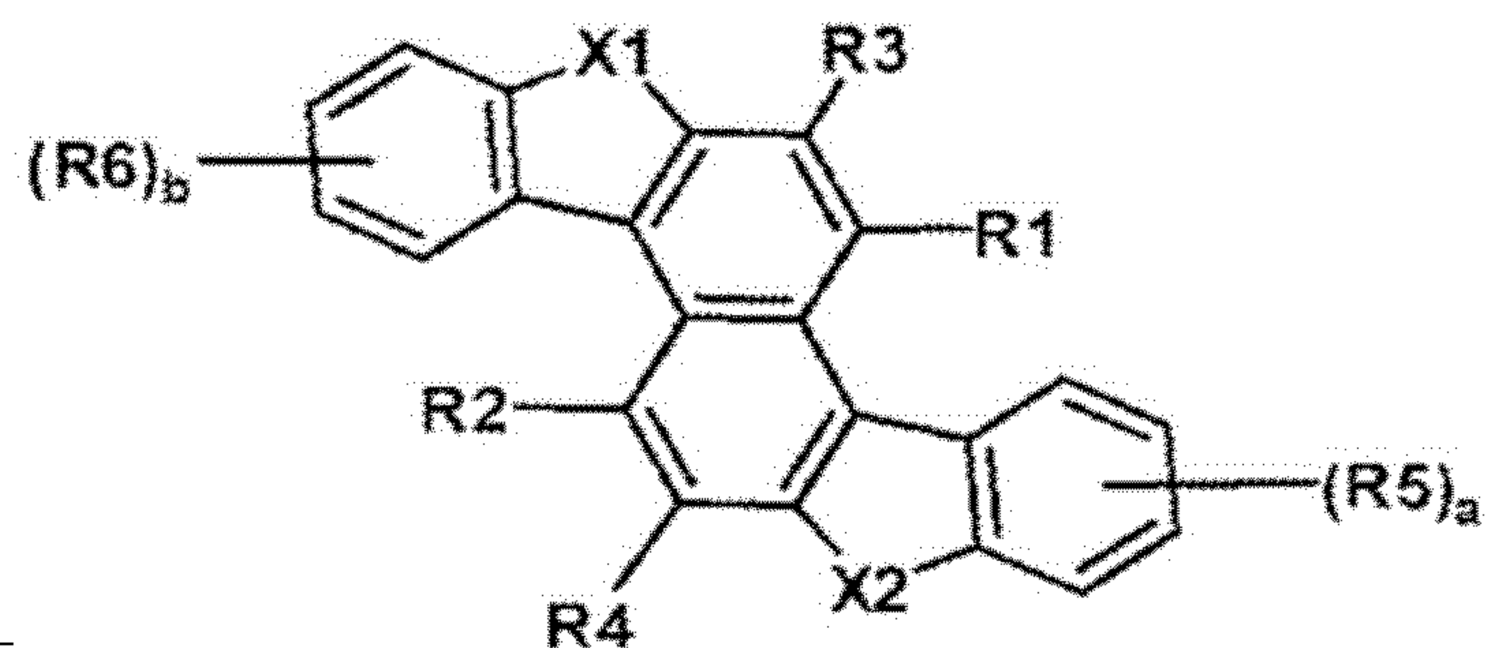
Chemical Formula 1-7
