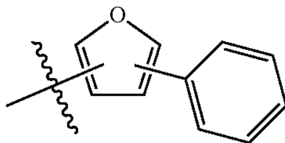
Substituent 21
