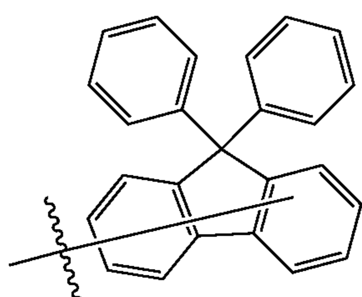
Substituent B15
