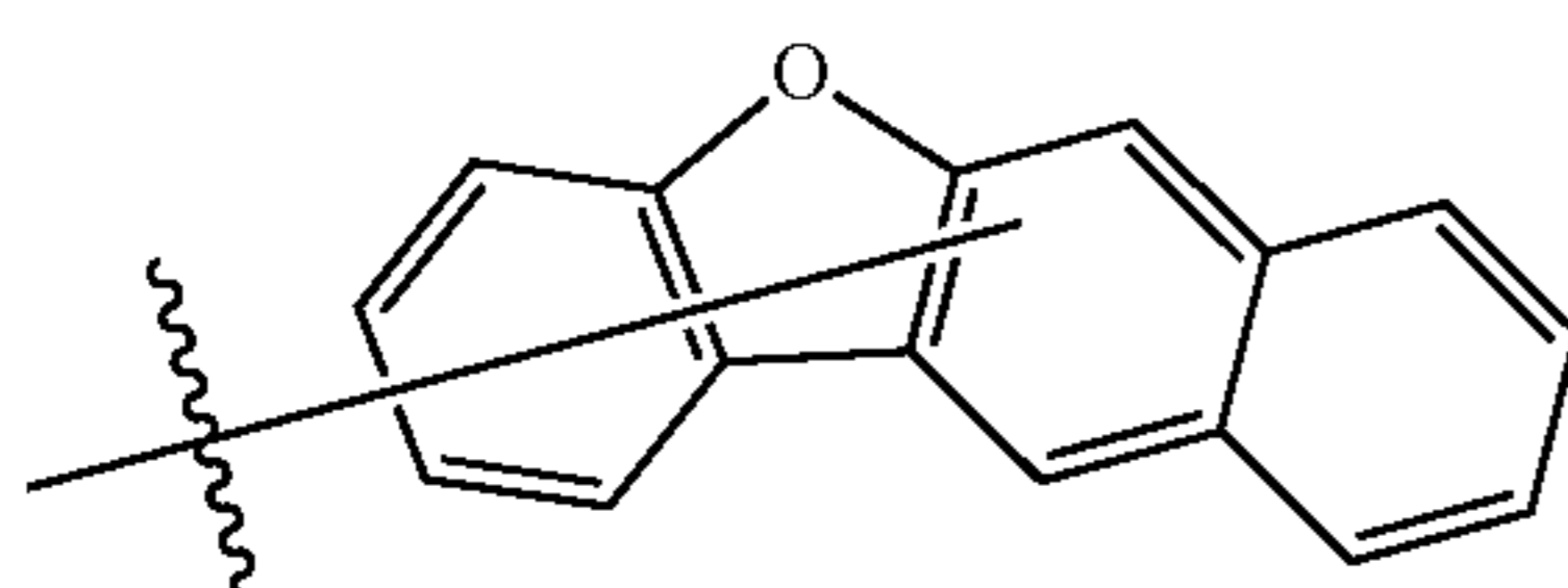
Substituent B9
