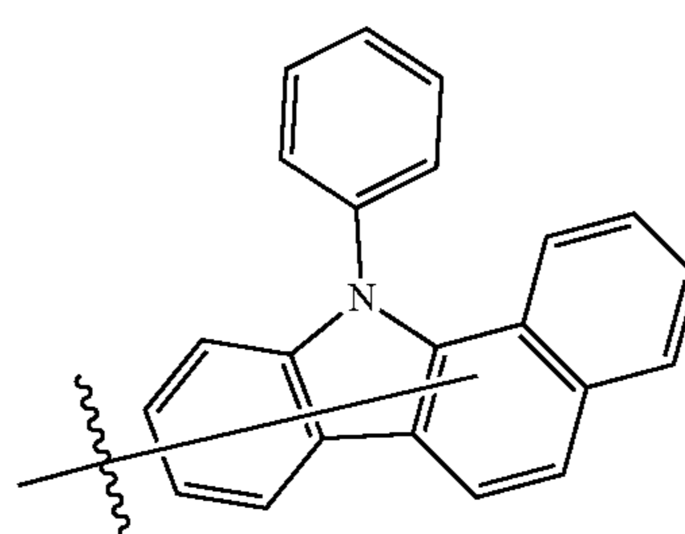
Substituent B22
