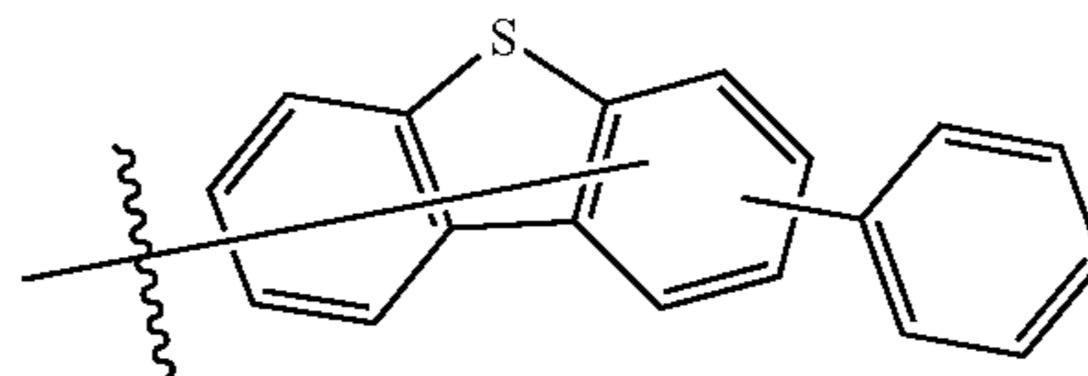
Substituent 26
