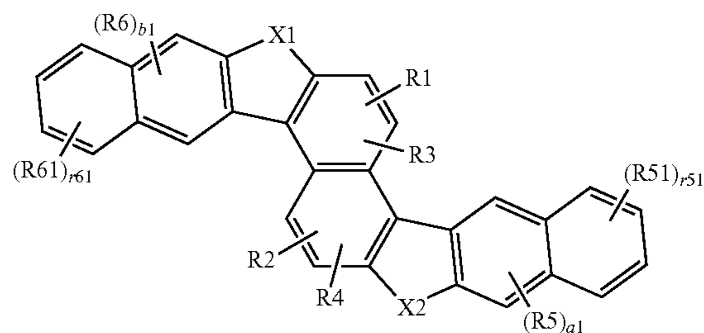
[Formula 1-3]
