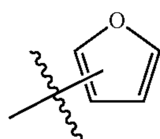
Substituent 17
