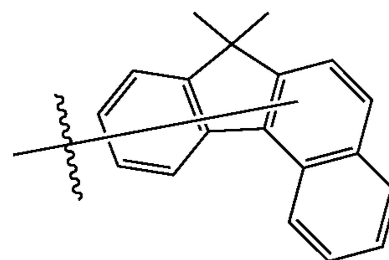
Substituent 30
