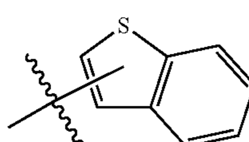
Substituent B20
