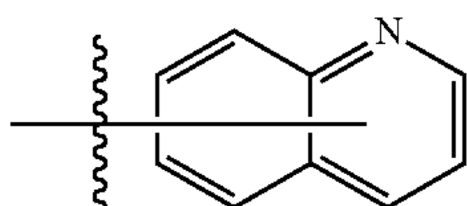
Substituent 43
