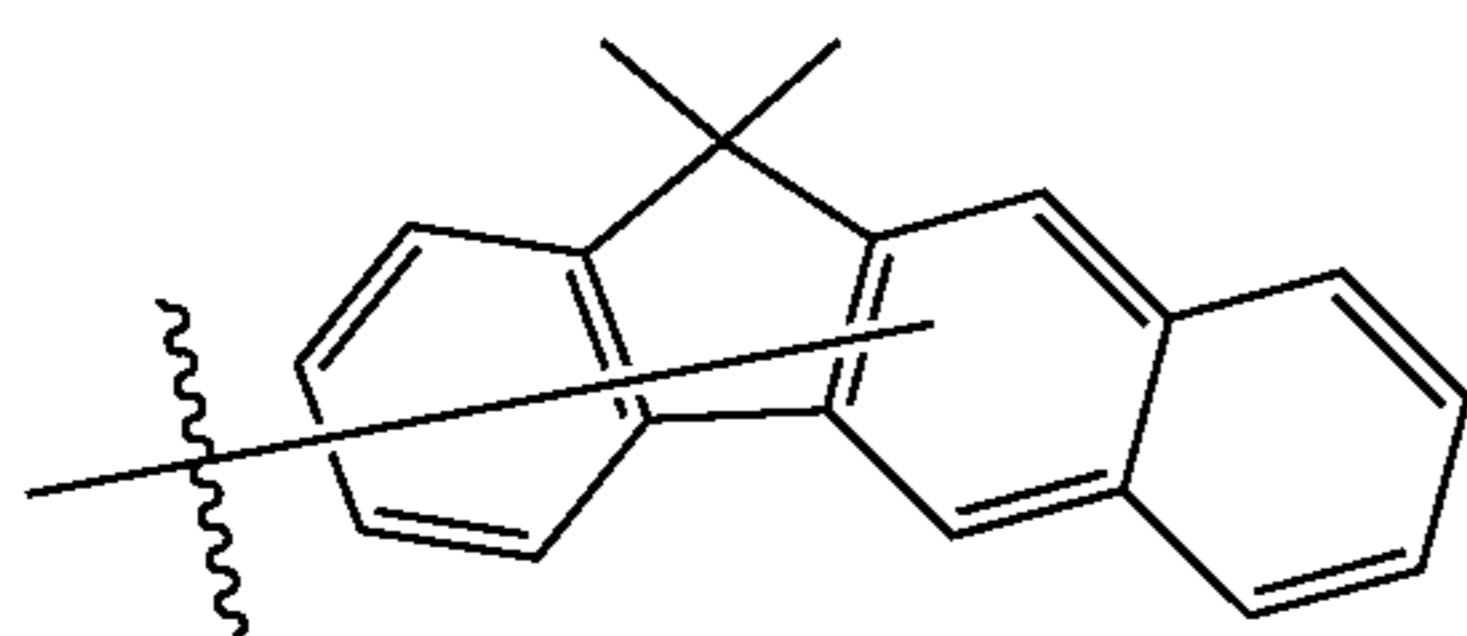
Substituent 29
