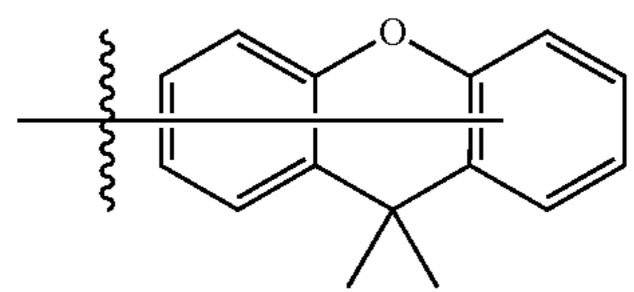
Substituent 53
