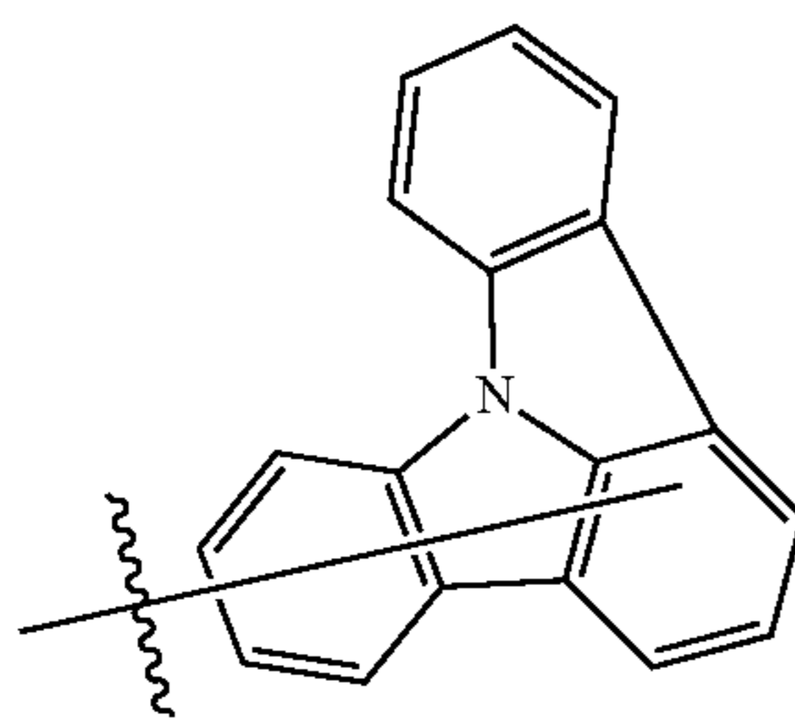
Substituent 39
