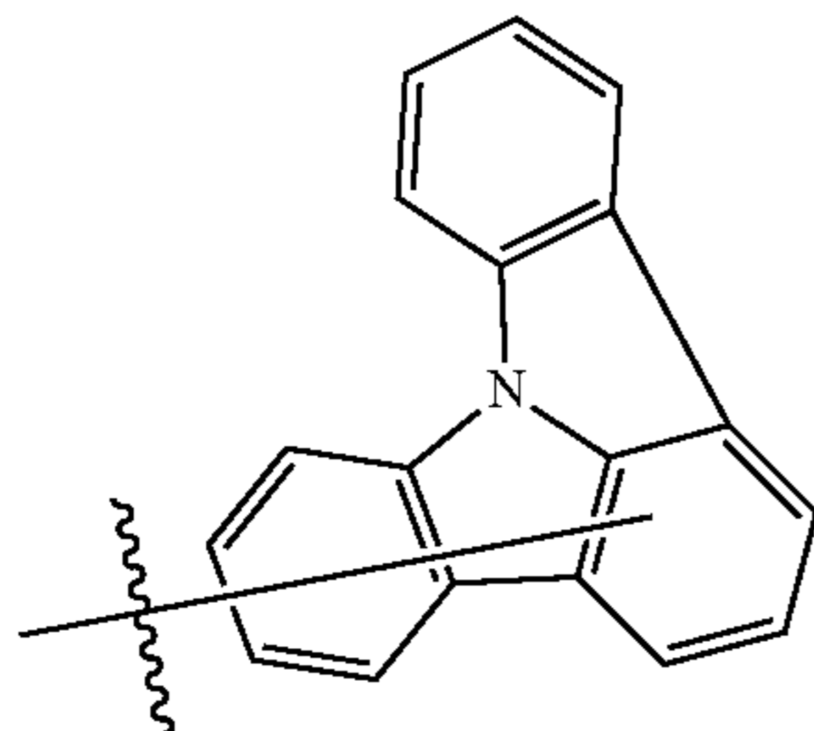
Substituent 39
