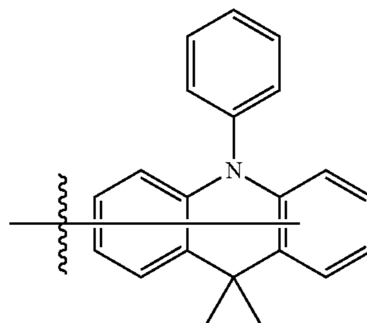
Substituent 52
