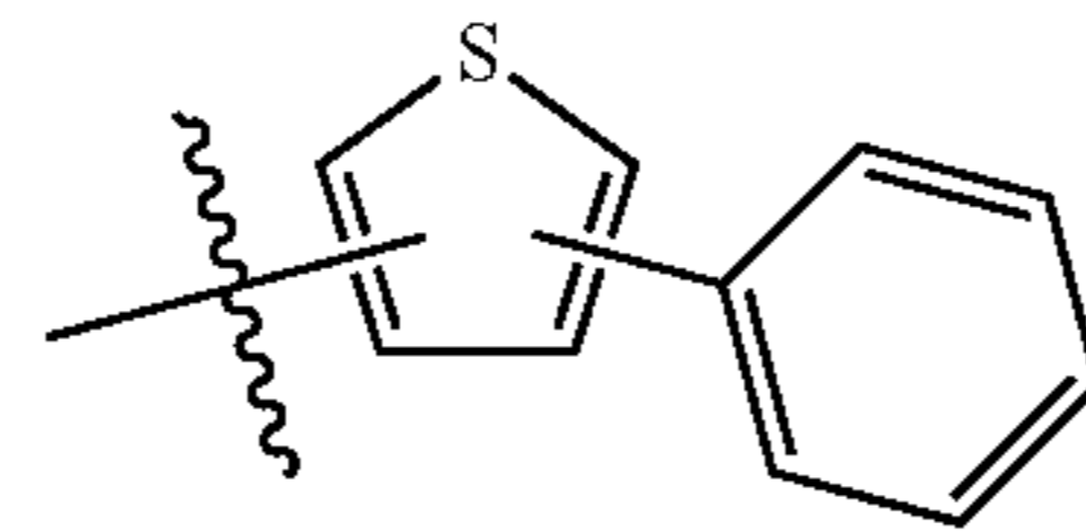
Substituent B18
