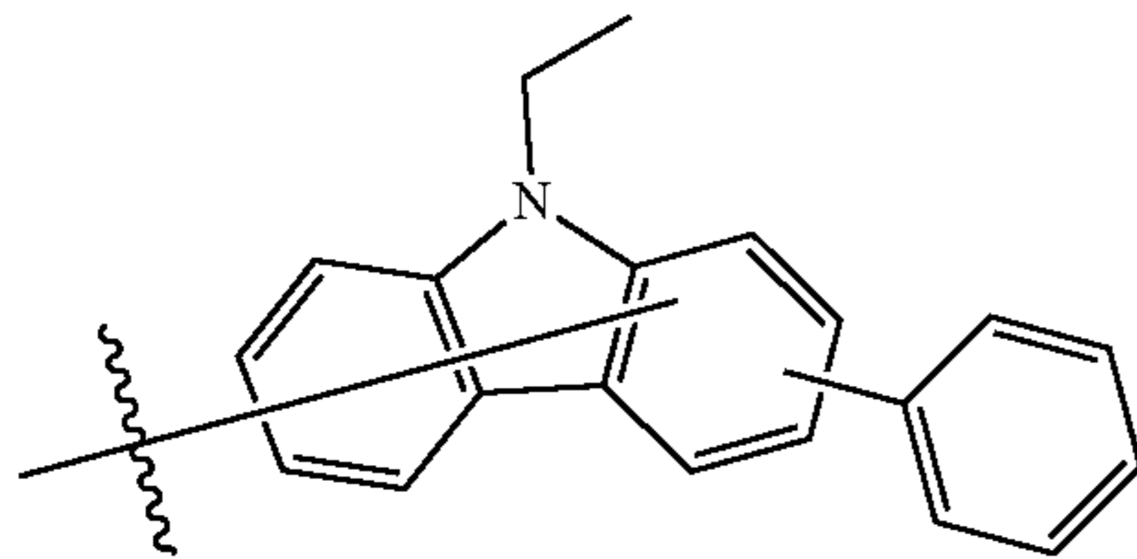
Substituent B25
