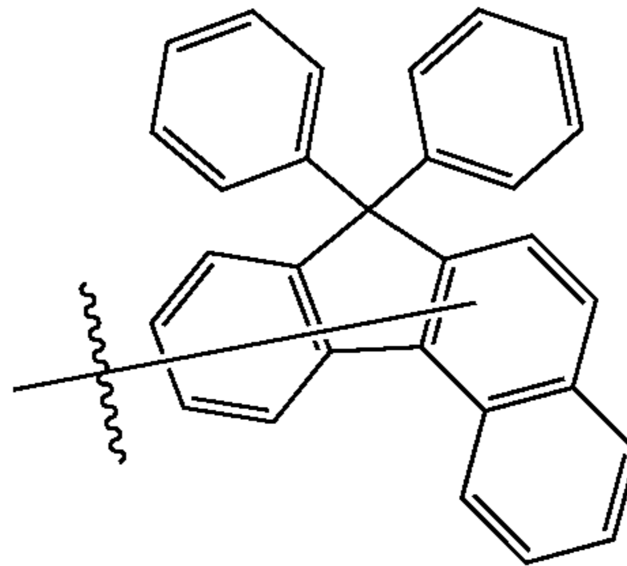
Substituent 36
