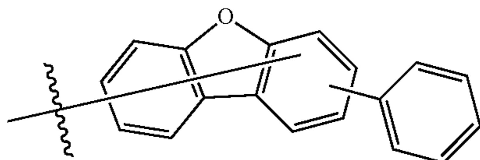
Substituent B27
