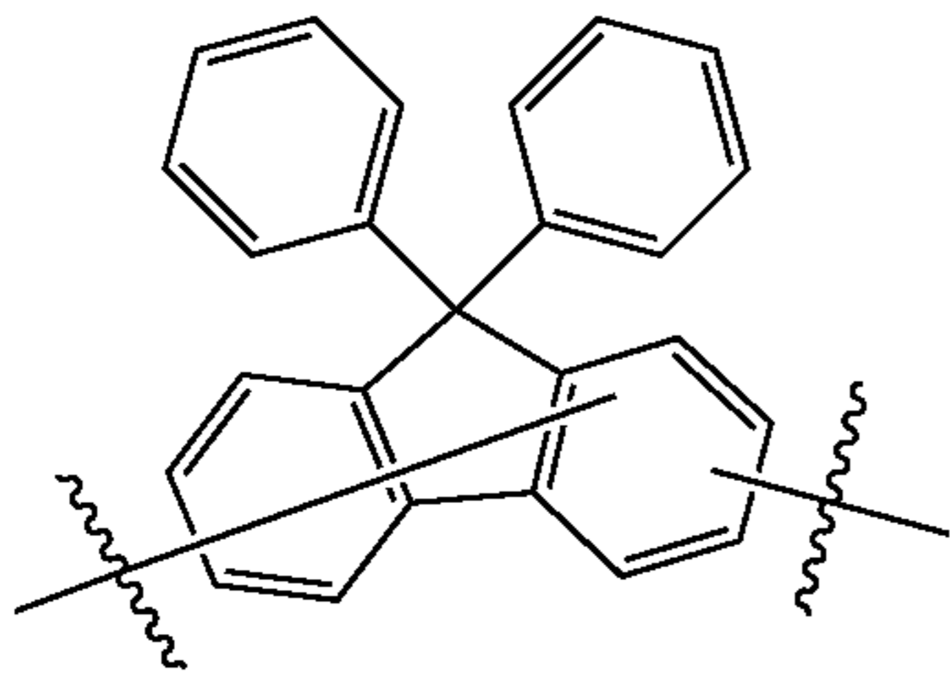
Substituent A15
