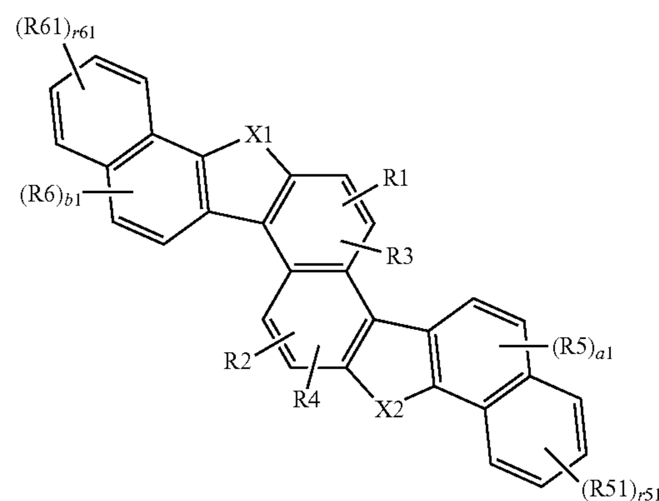
[Formula 1-3]
