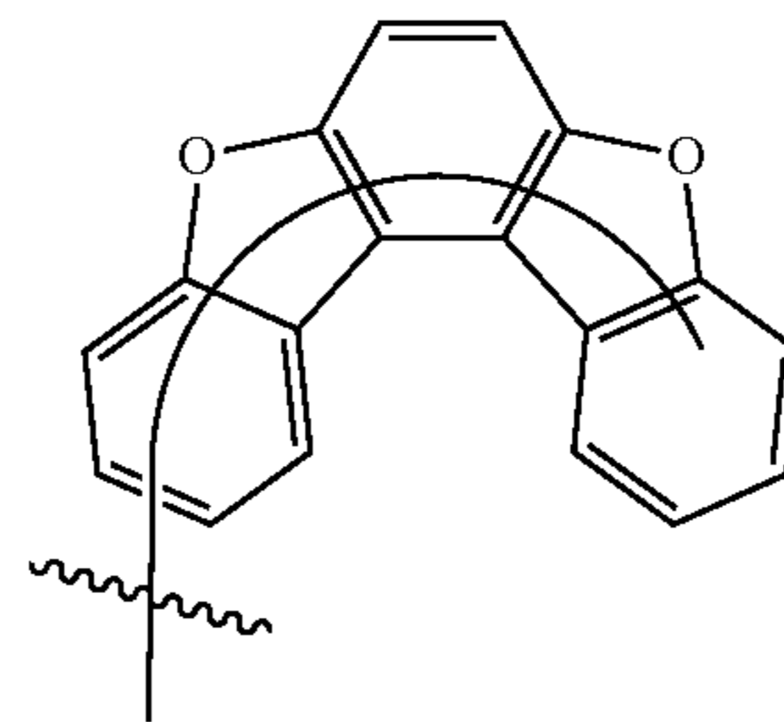
Substituent 40
