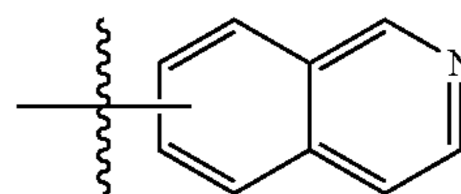
Substituent 42
