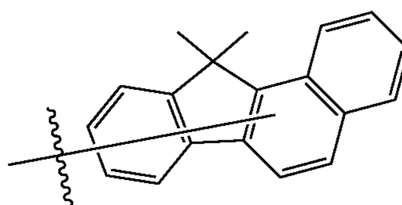
Substituent 28
