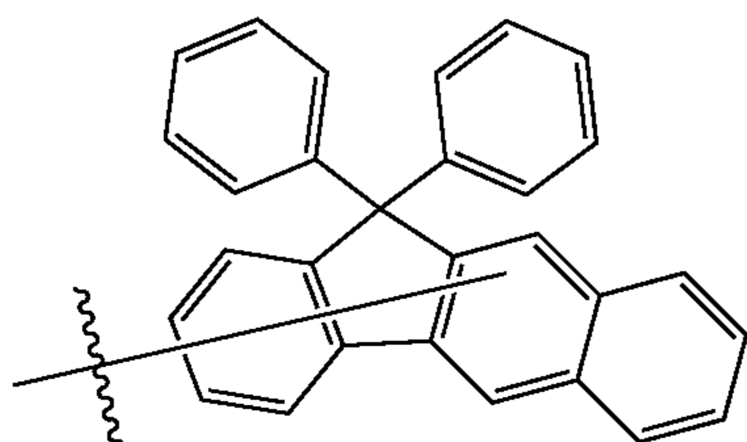
Substituent B33
