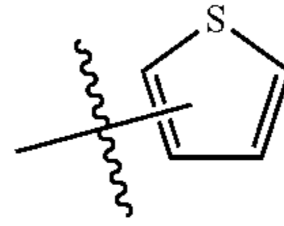
Substituent 16
