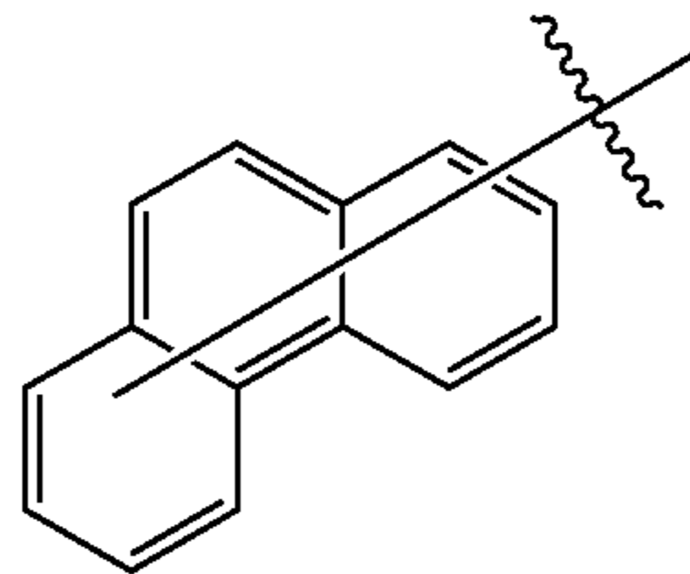
Substituent B4
