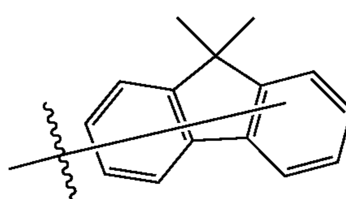
Substituent B14
