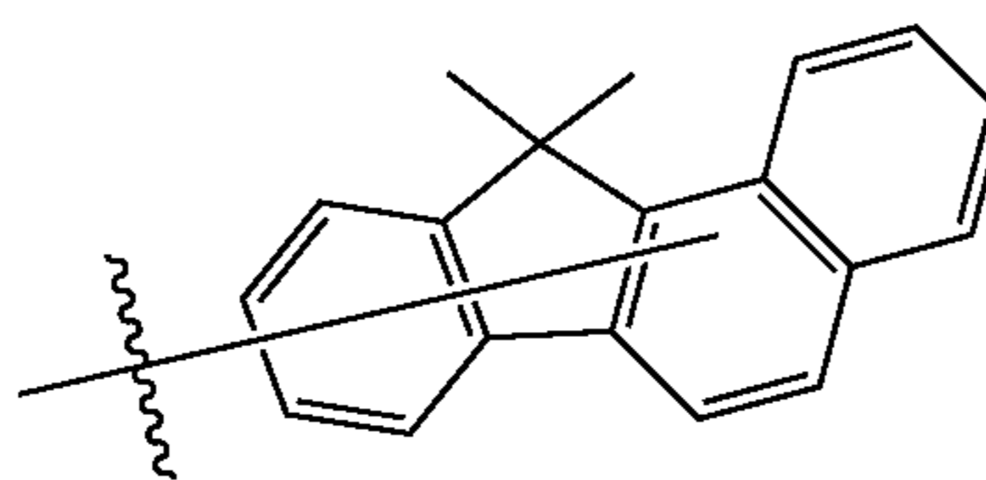
Substituent B28
