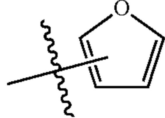
Substituent 17
