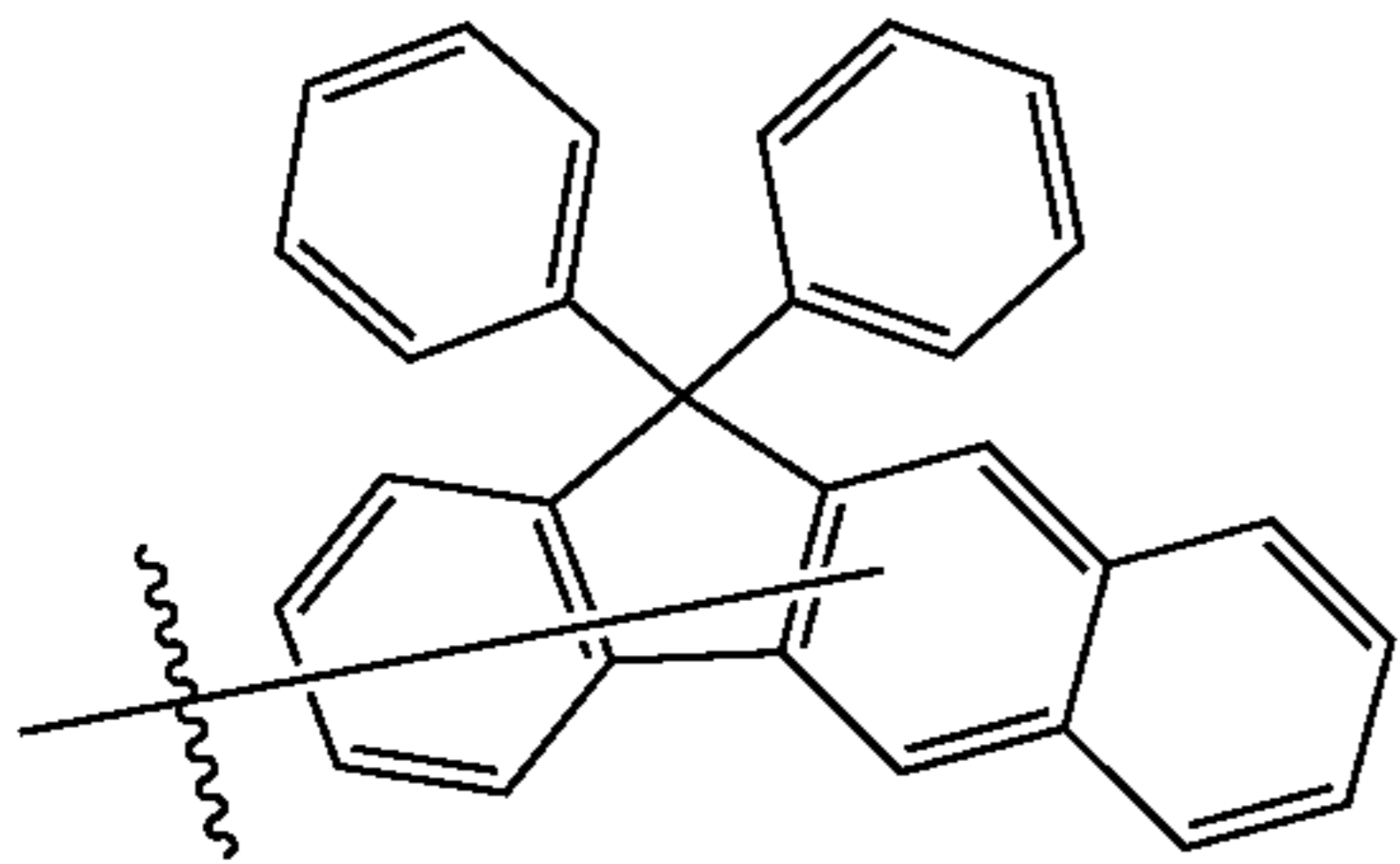
Substituent 33
