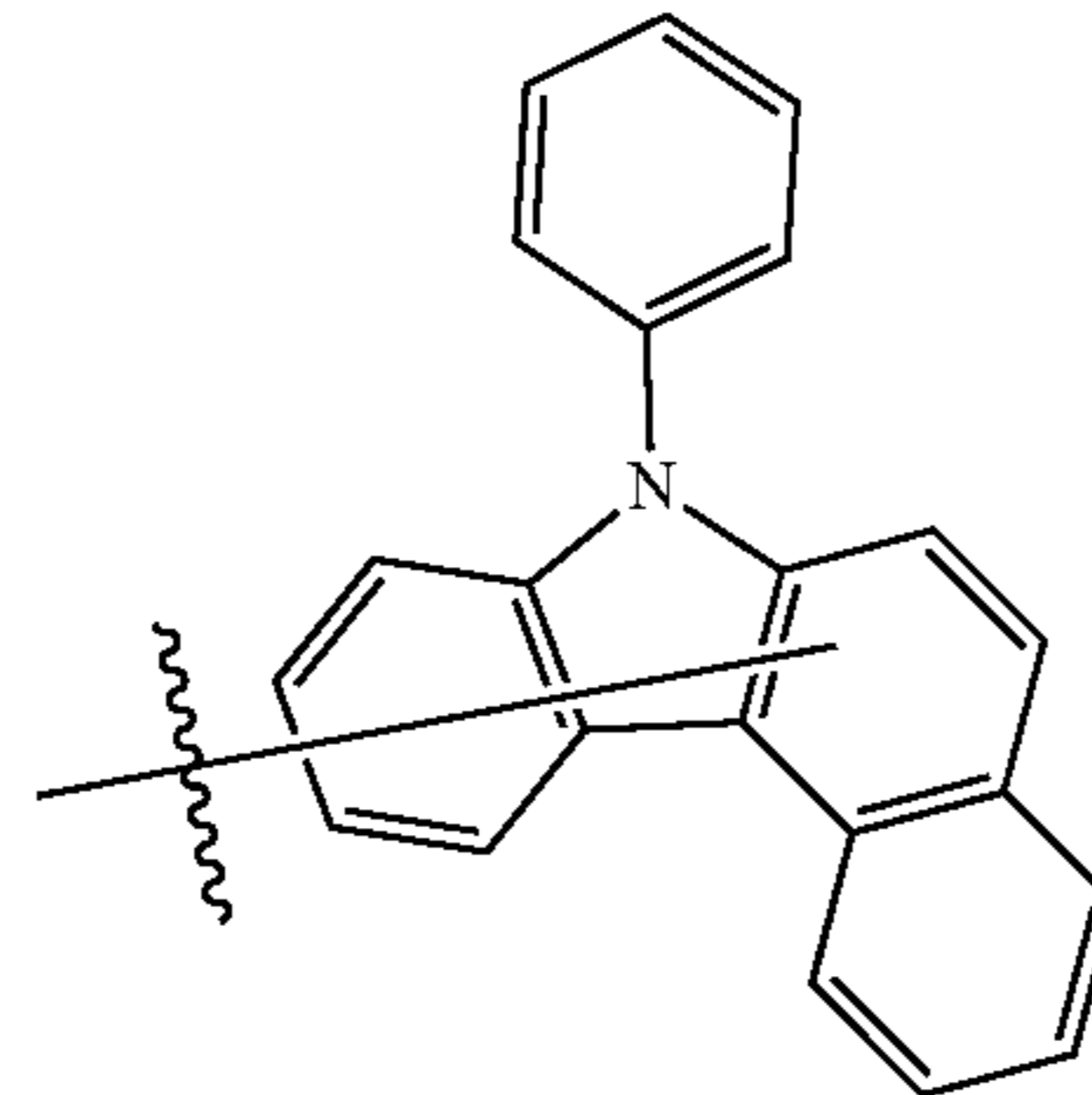
Substituent 24
