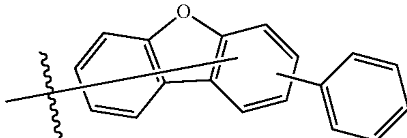
Substituent 27
