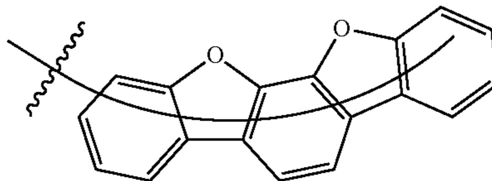
Substituent 38
