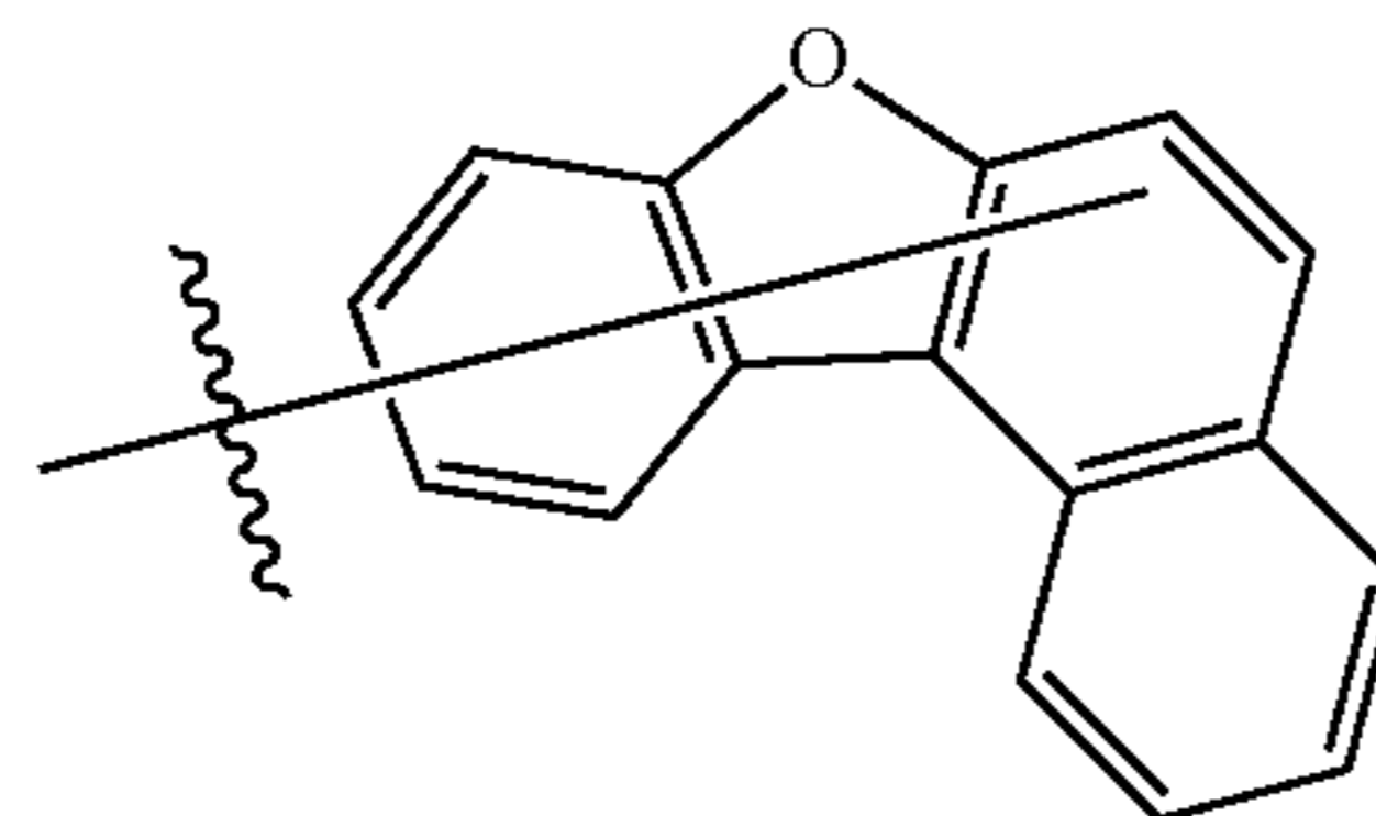
Substituent 10
