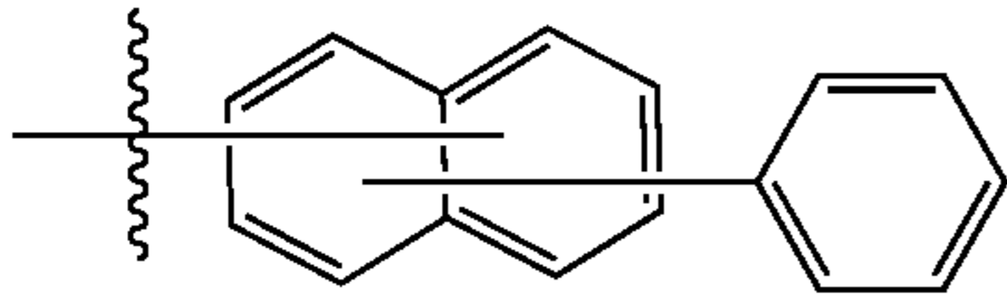
Substituent B3
