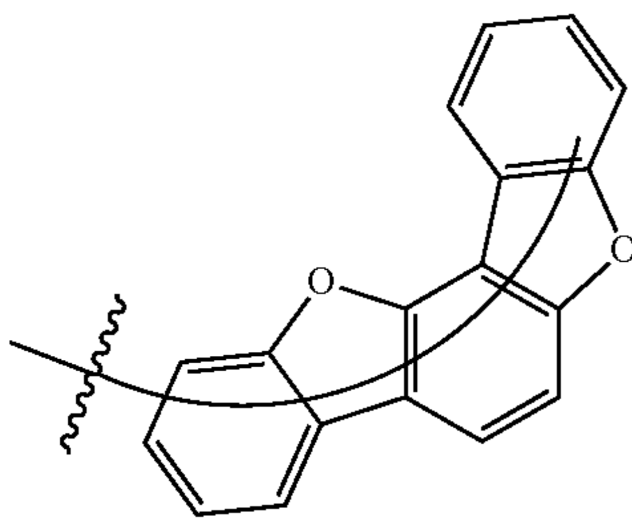
Substituent 37
