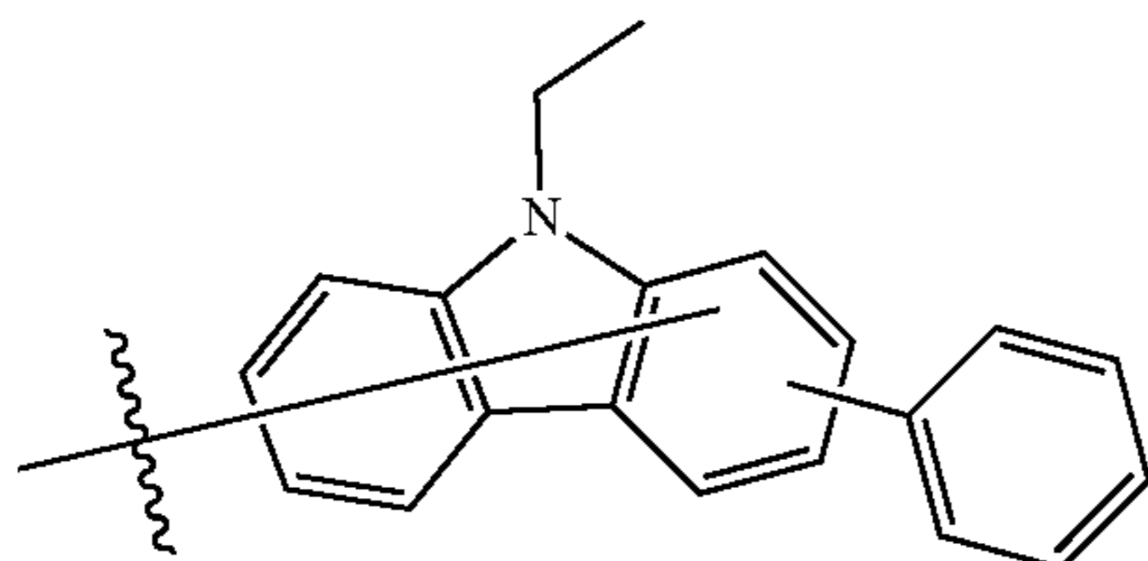
Substituent B25
