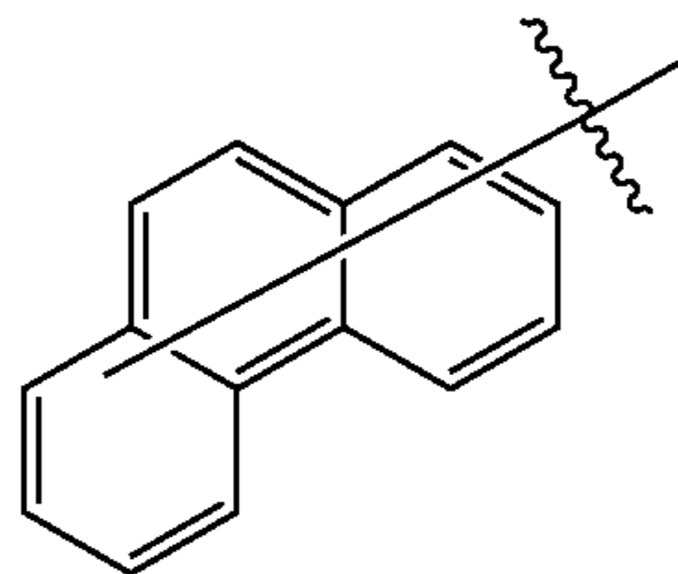
Substituent B4
