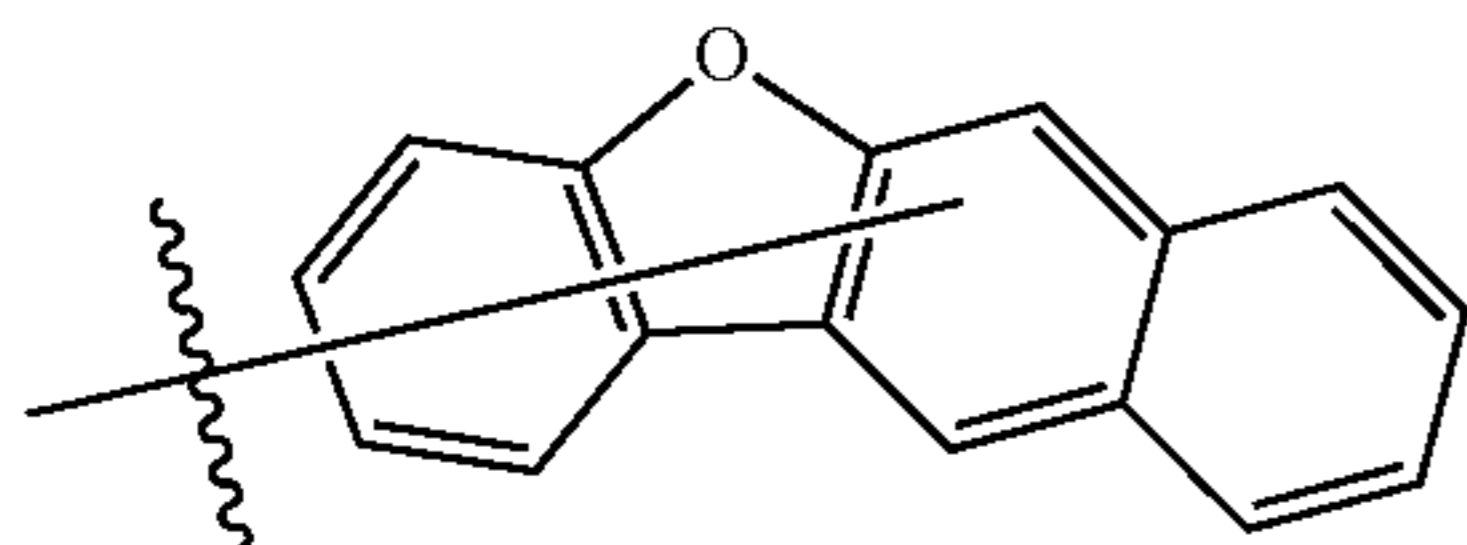
Substituent B9
