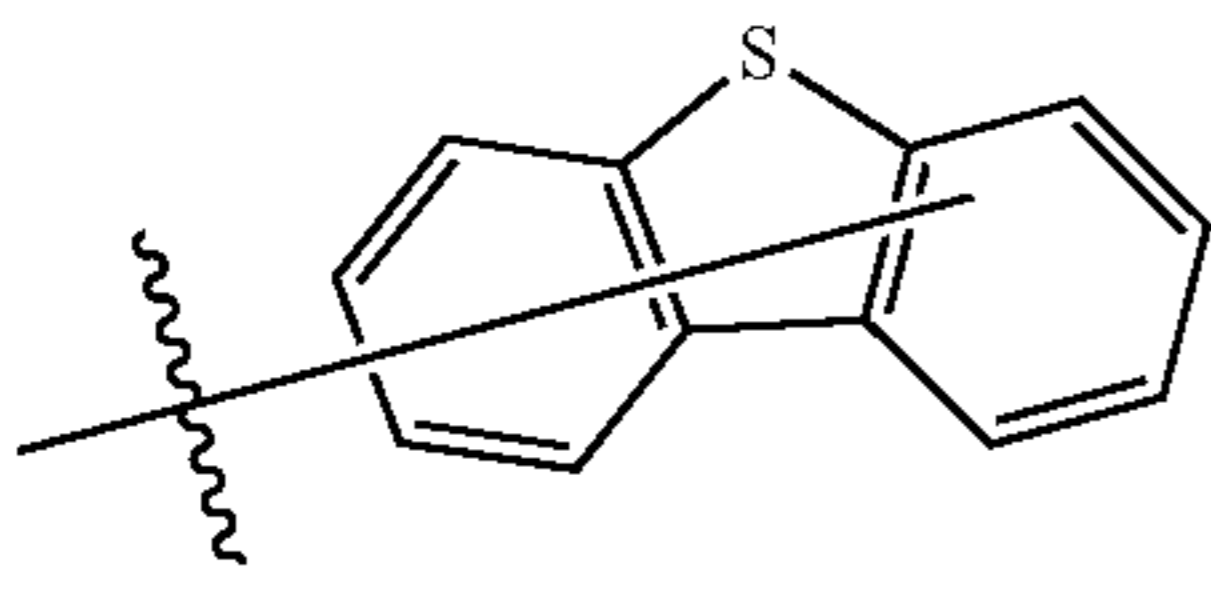
Substituent B11
