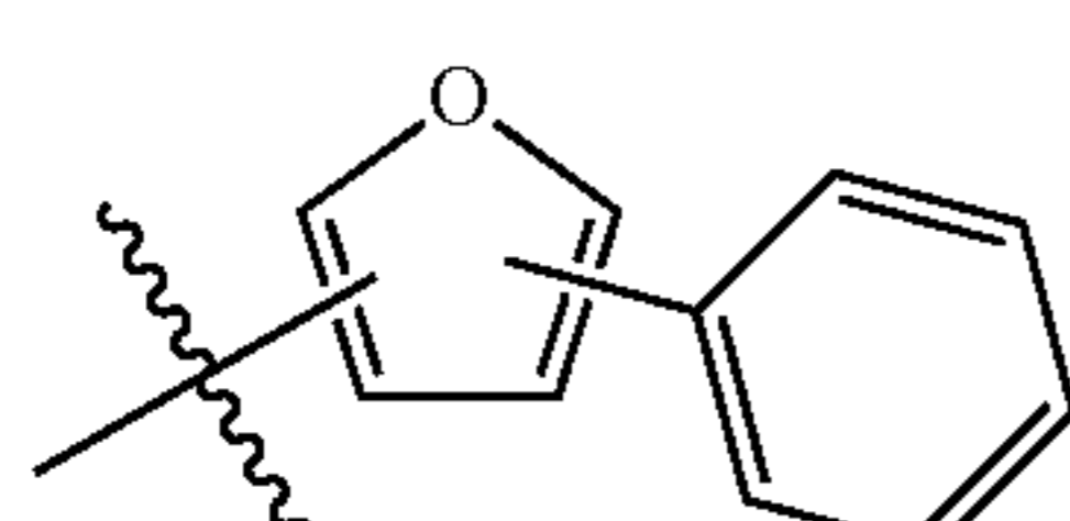
Substituent B19
