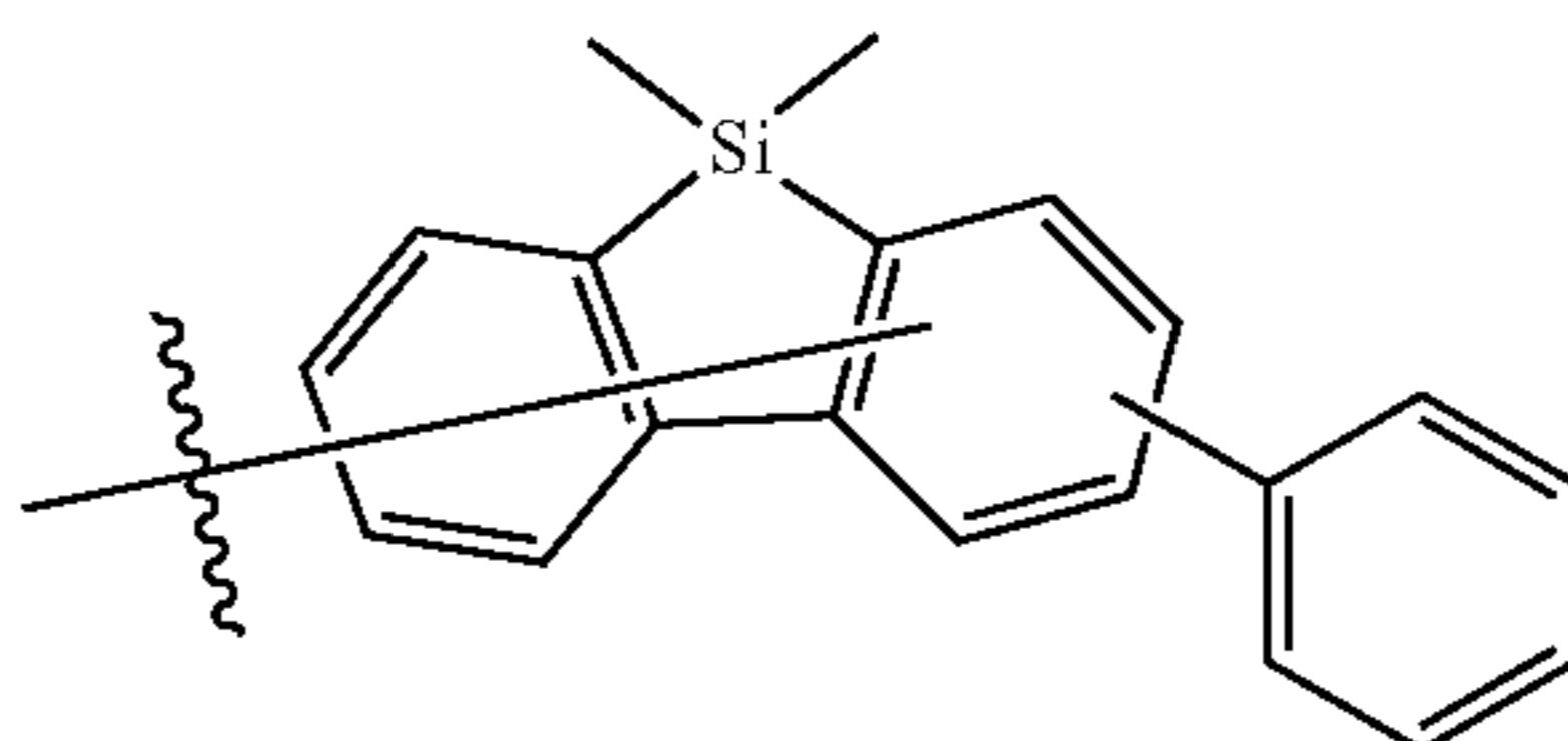
Substituent 54
