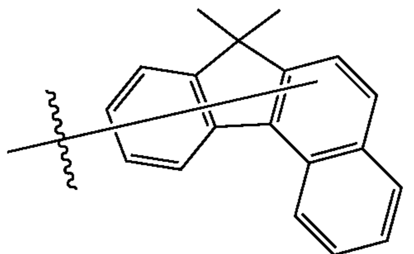
Substituent B30
