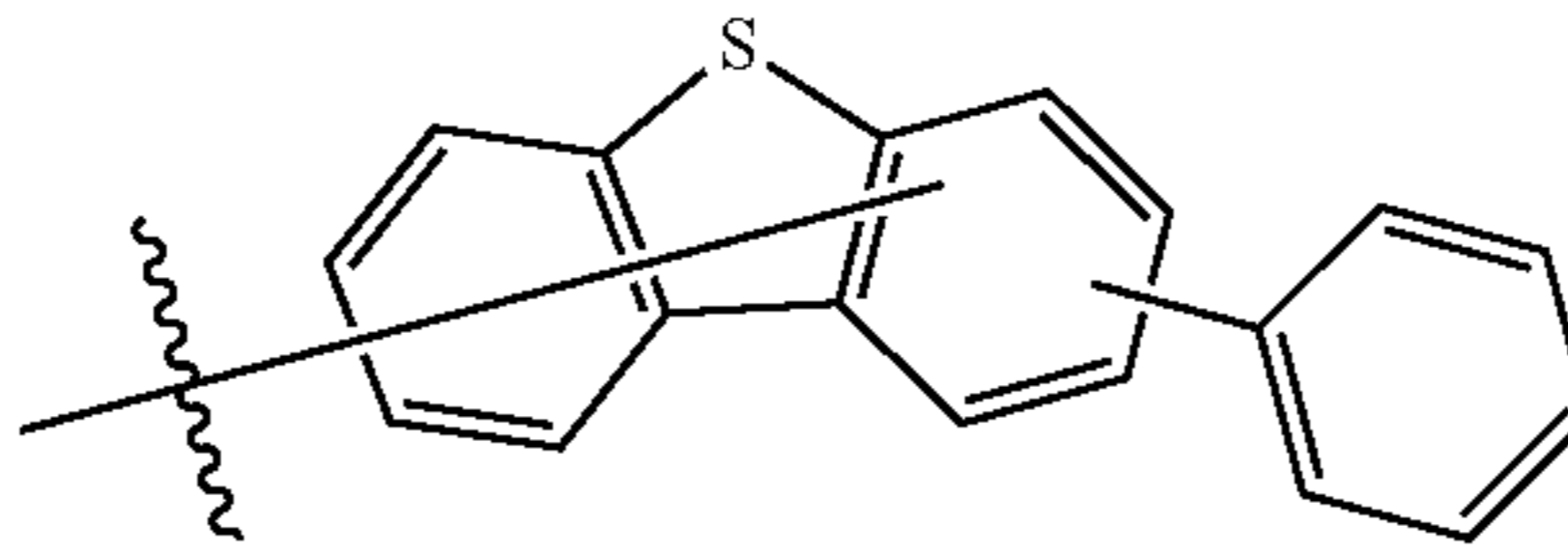
Substituent B26
