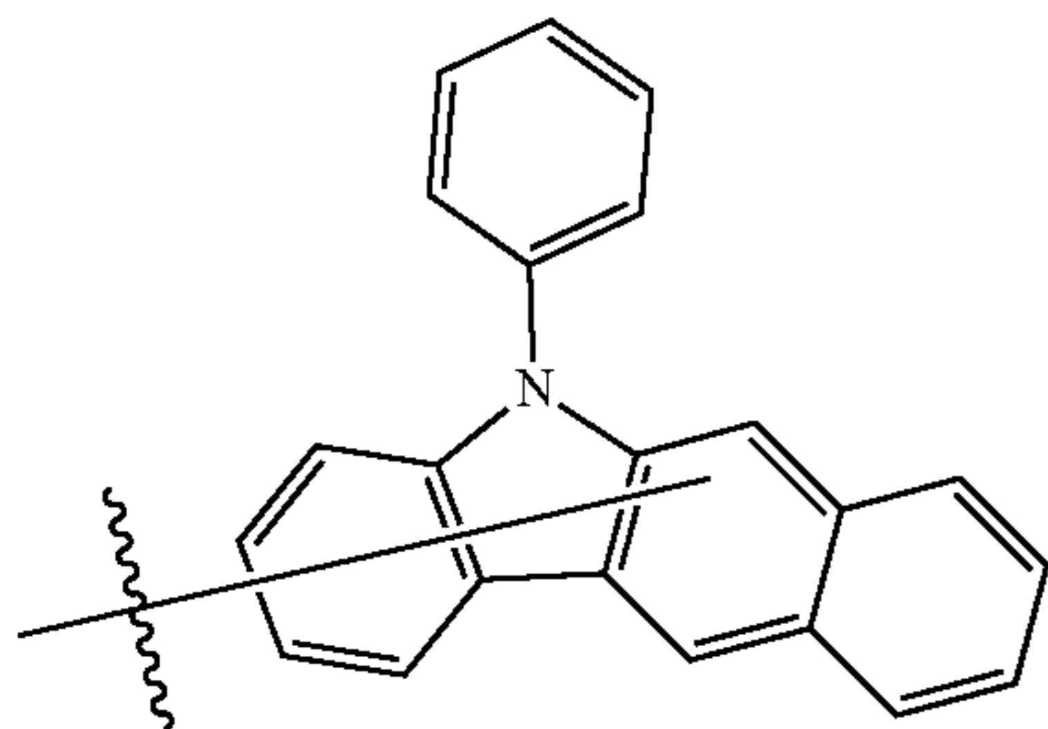
Substituent B23
