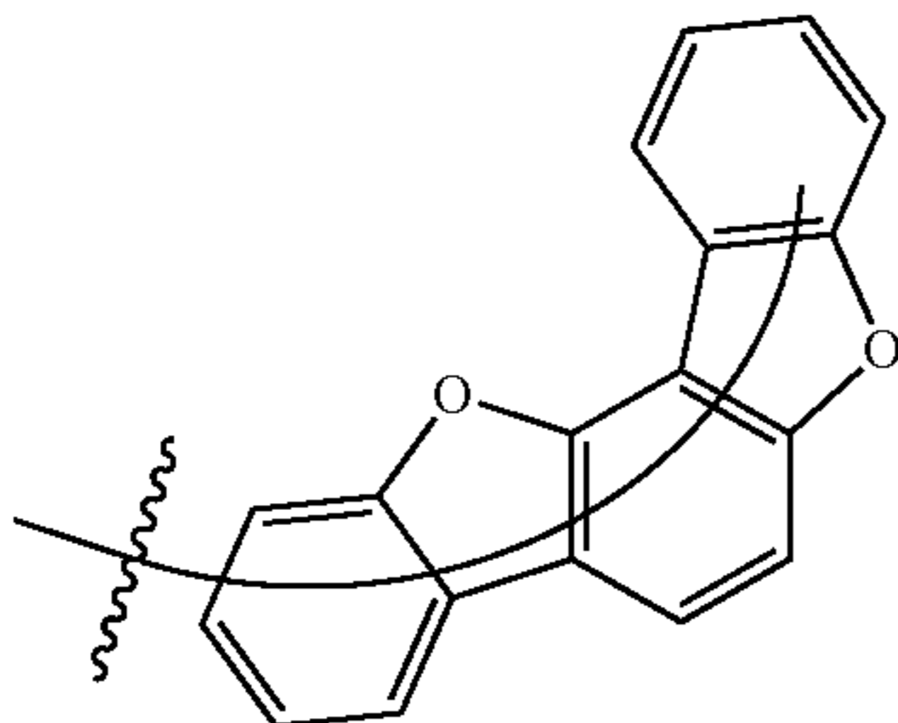
Substituent 39
