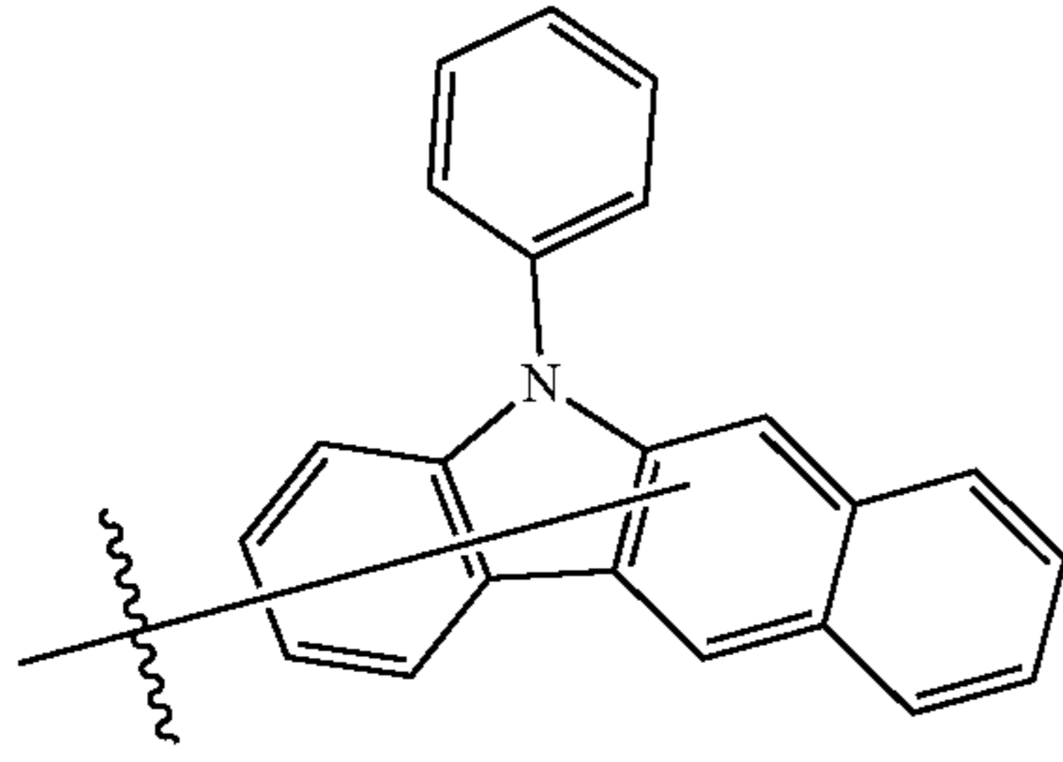
Substituent B23
