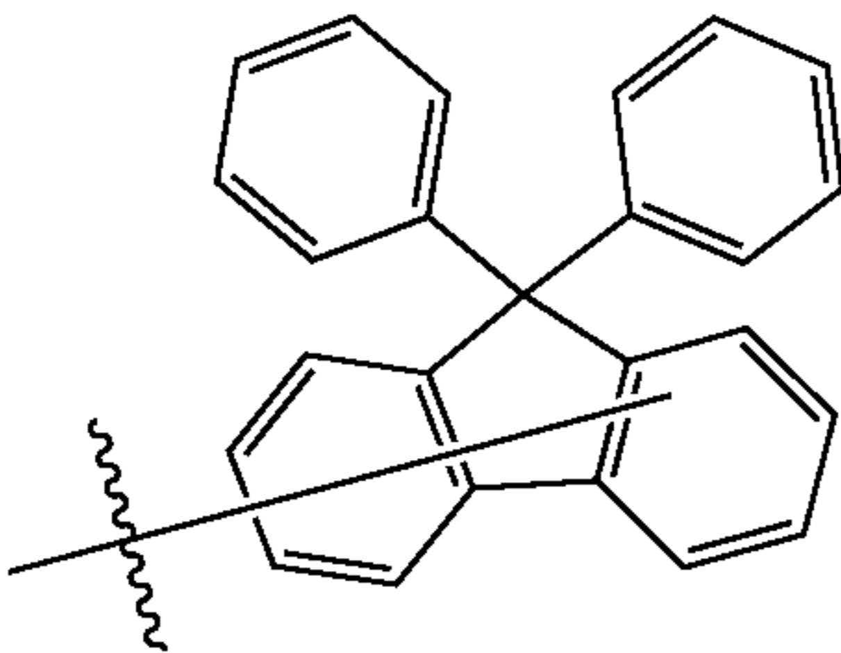
Substituent B15
