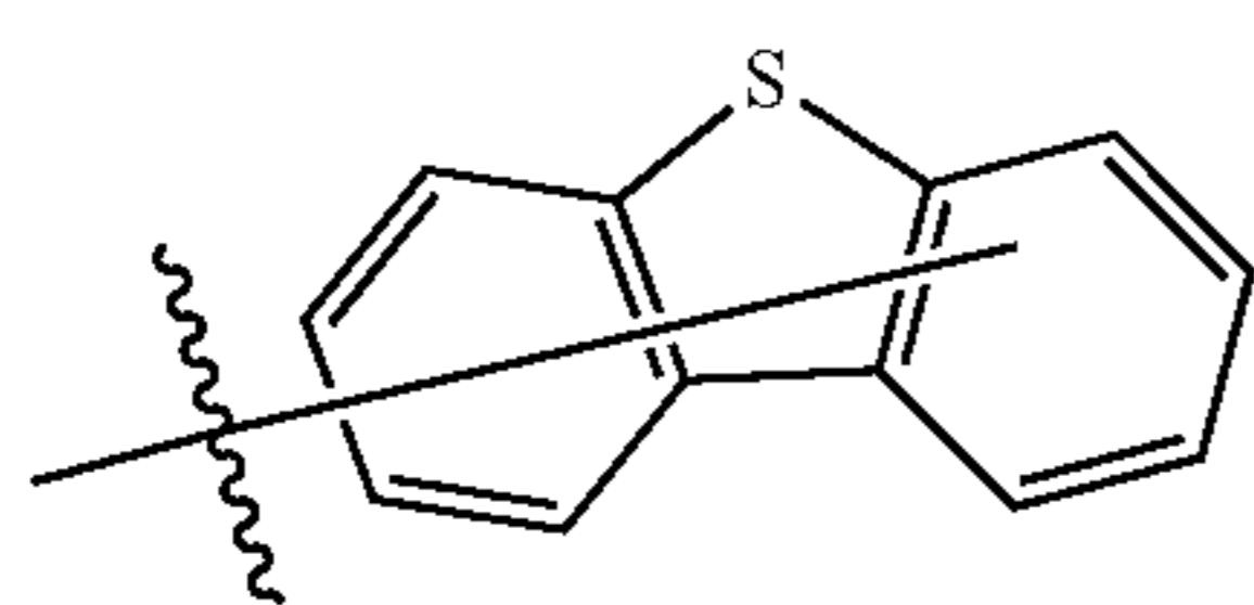
Substituent B11
