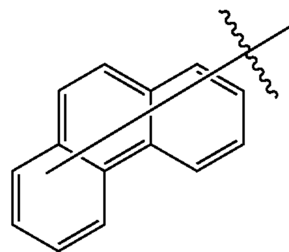
Substituent B4
