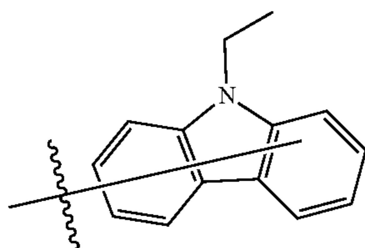
Substituent 13
