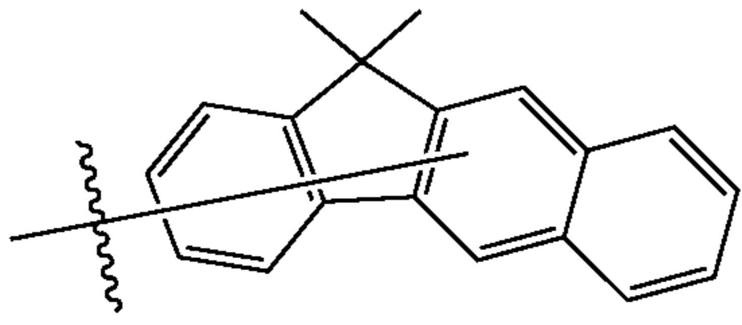
Substituent 29
