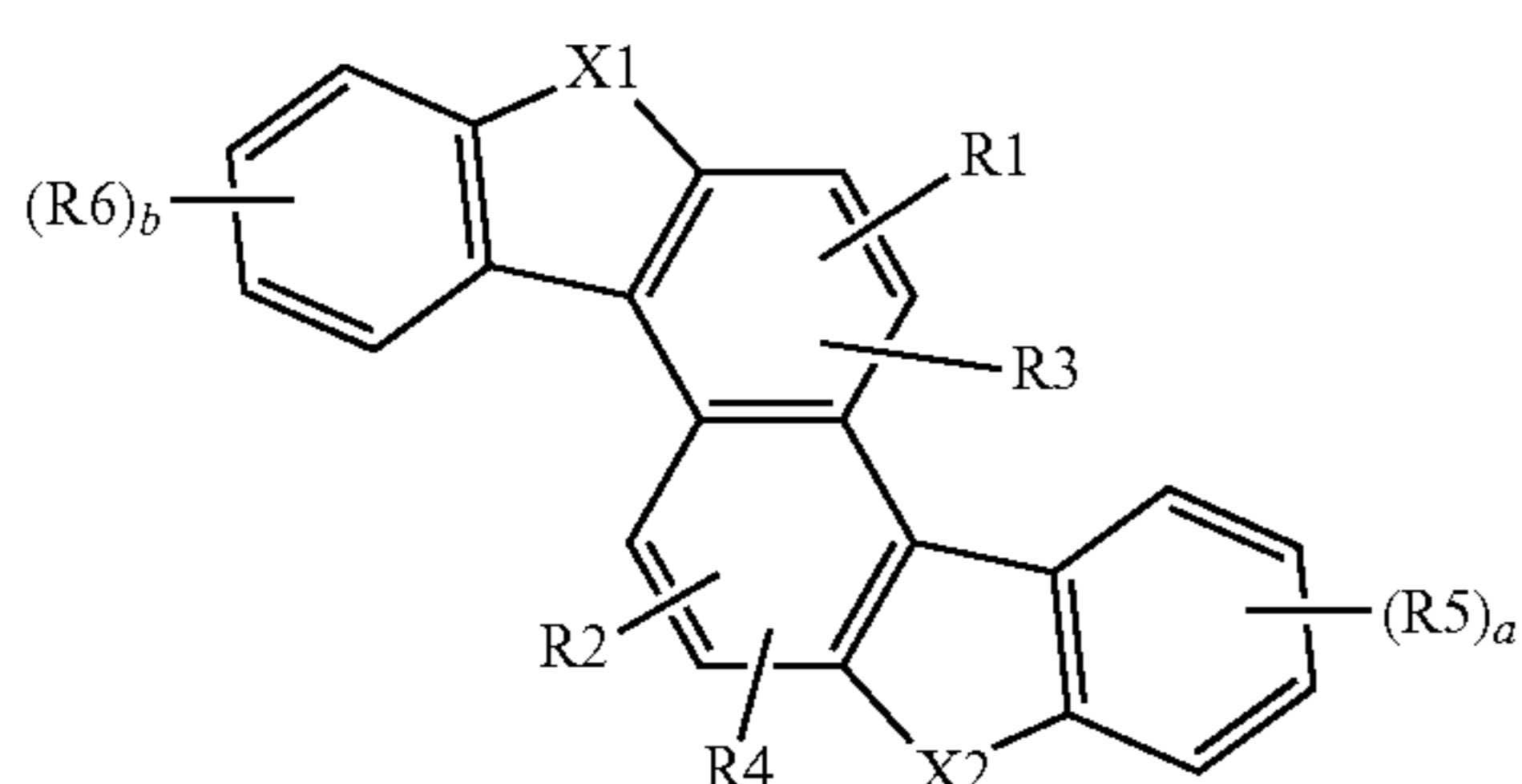
[Formula 1]
