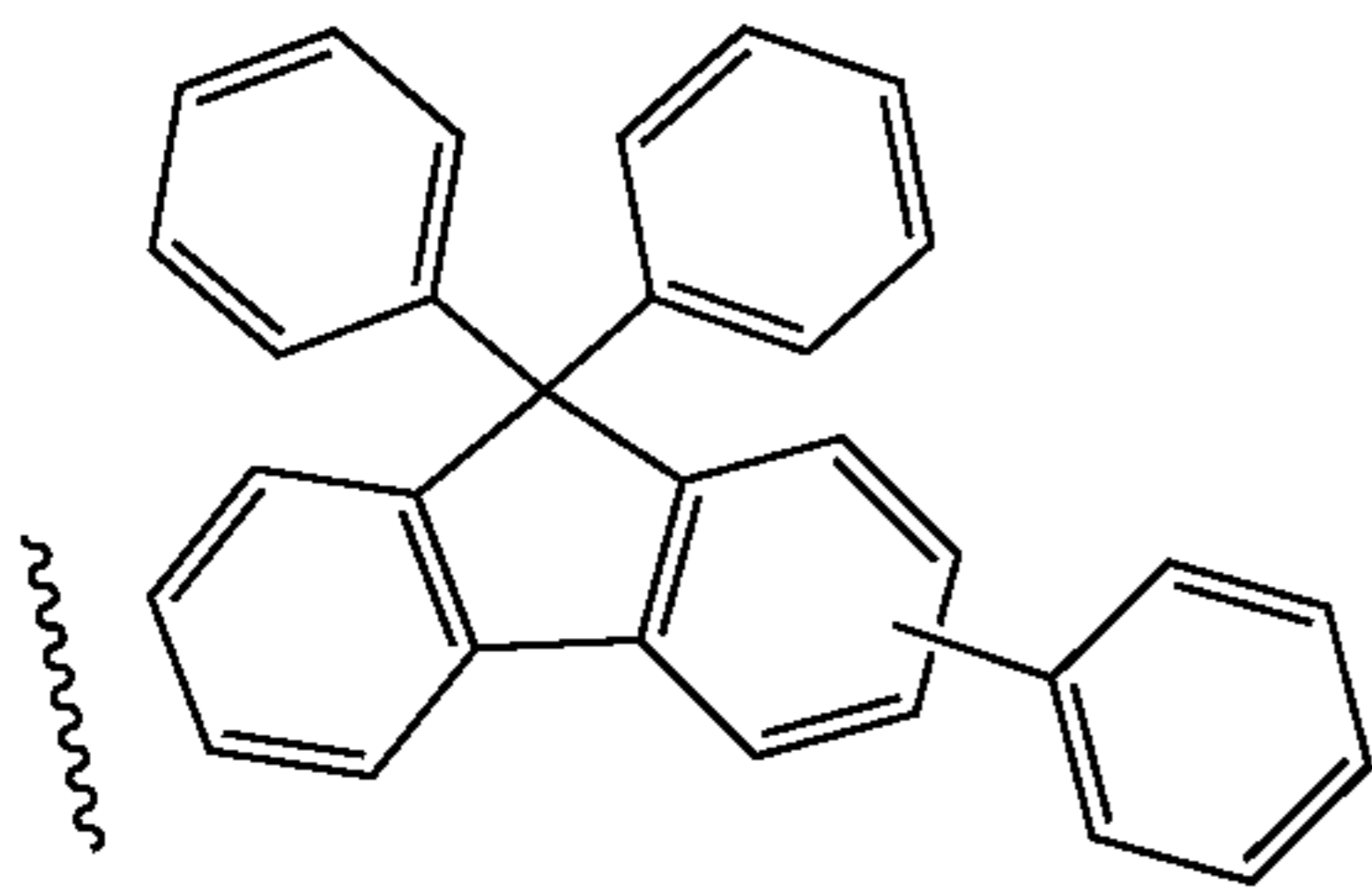
Substituent 35
