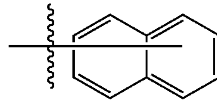
Substituent B2
