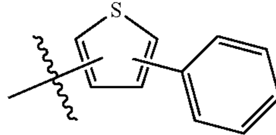
Substituent 20
