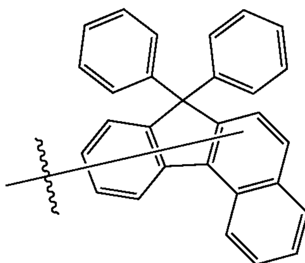
Substituent B34
