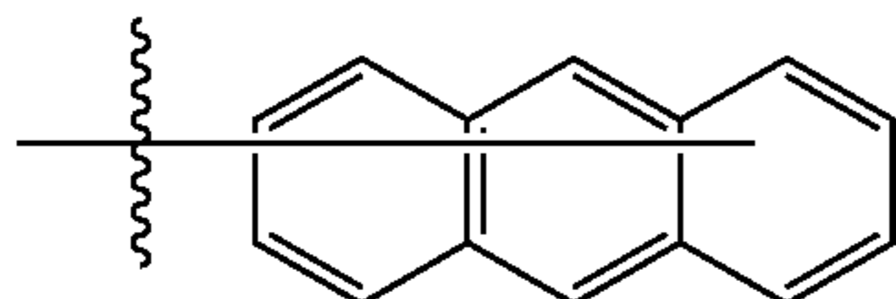
Substituent B5
