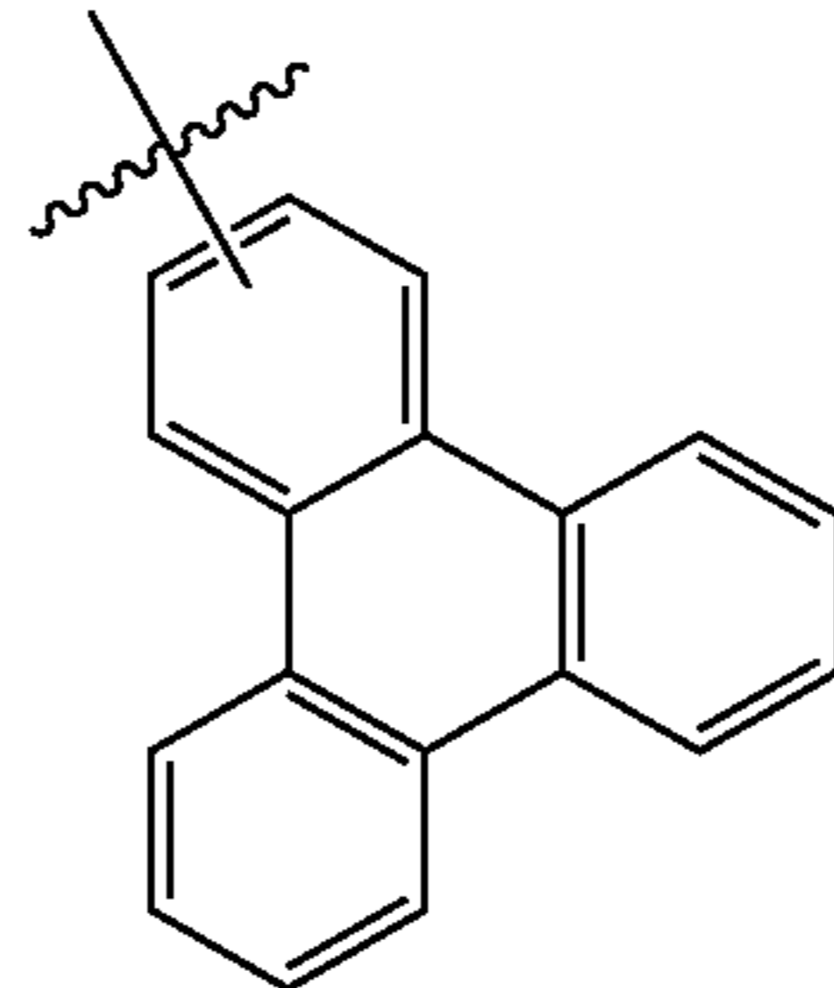
Substituent B6
