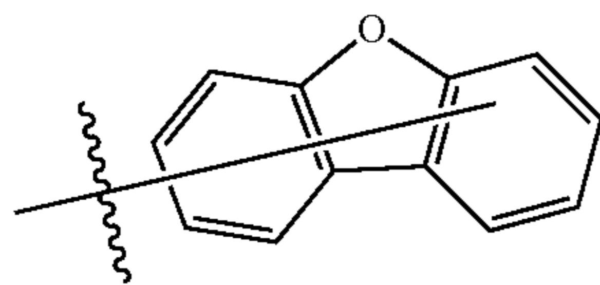
Substituent B7
