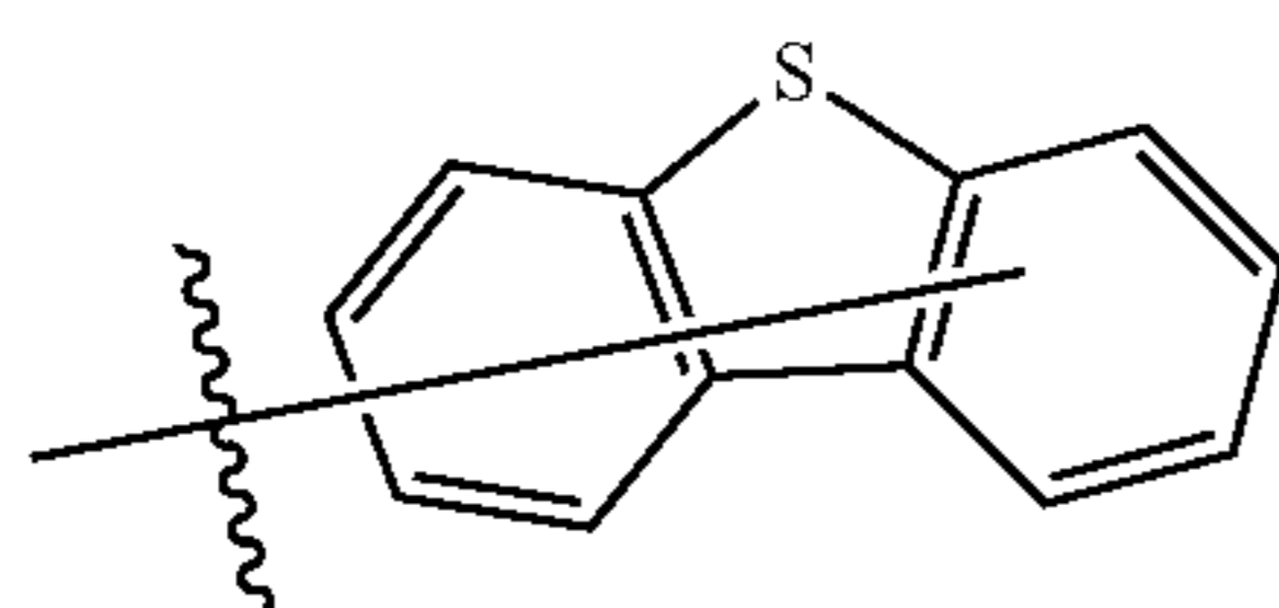
Substituent 11
