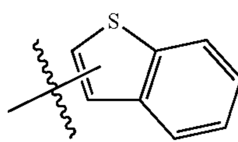
Substituent 20
