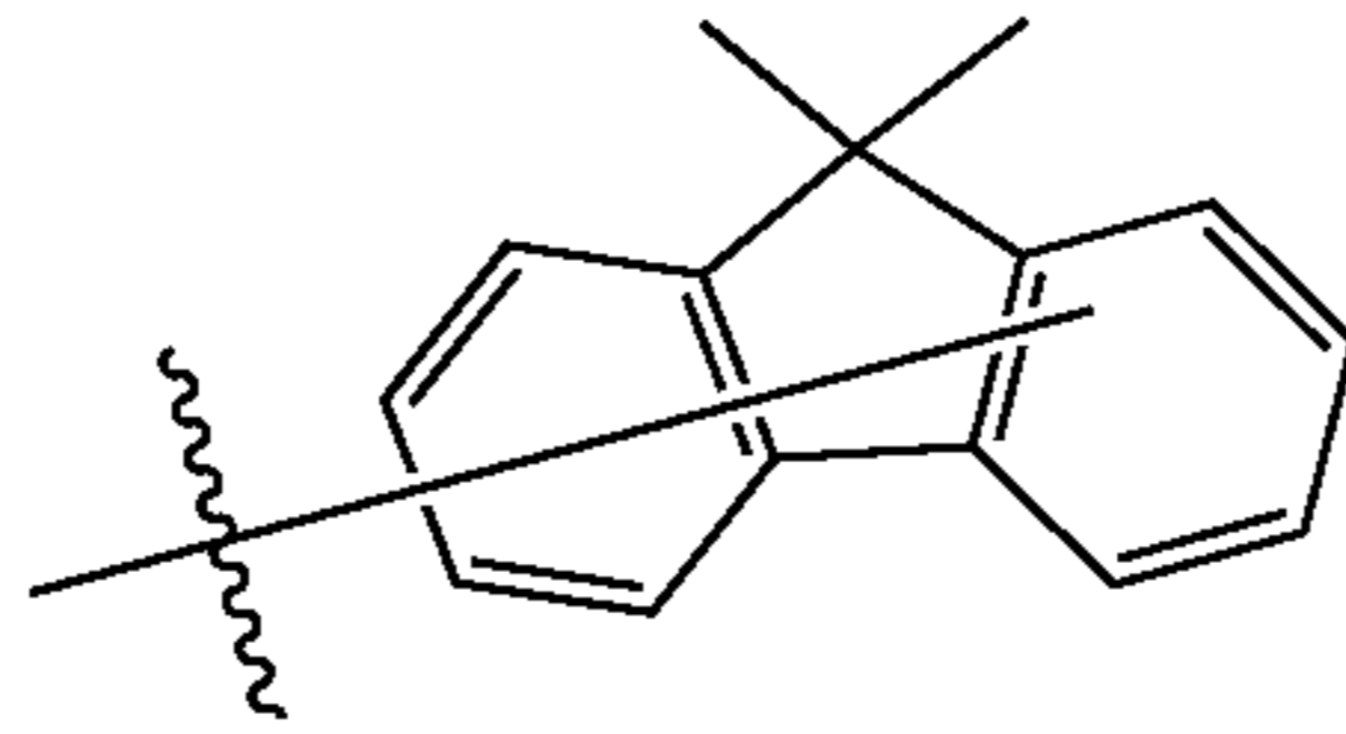
Substituent B14
