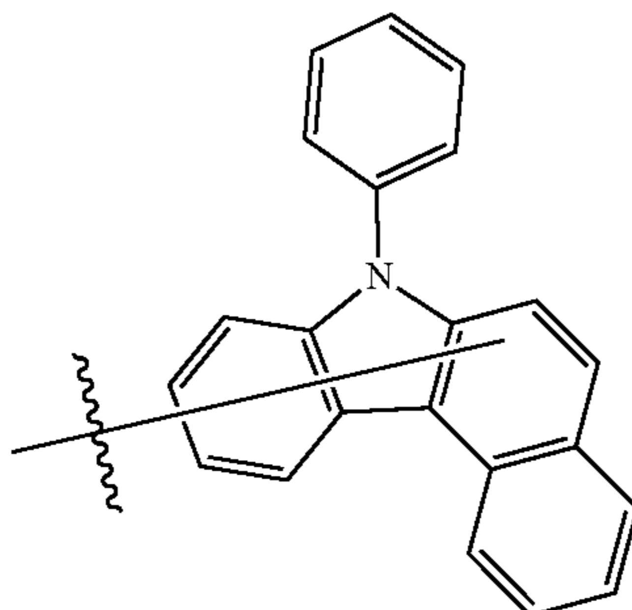
Substituent B24
