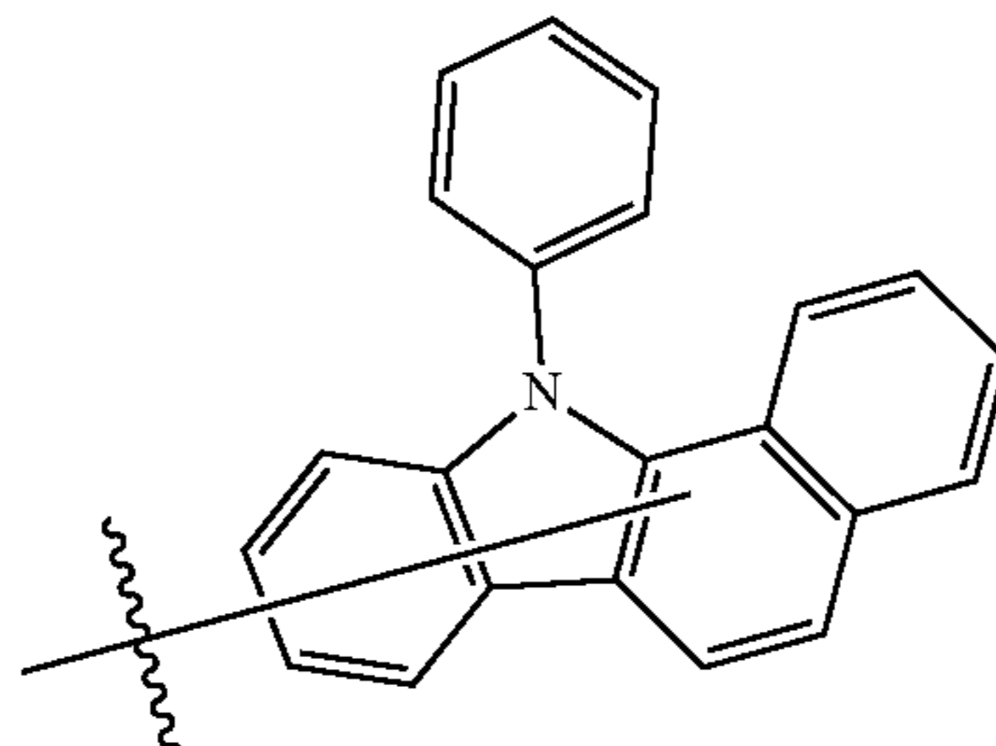
Substituent B22
