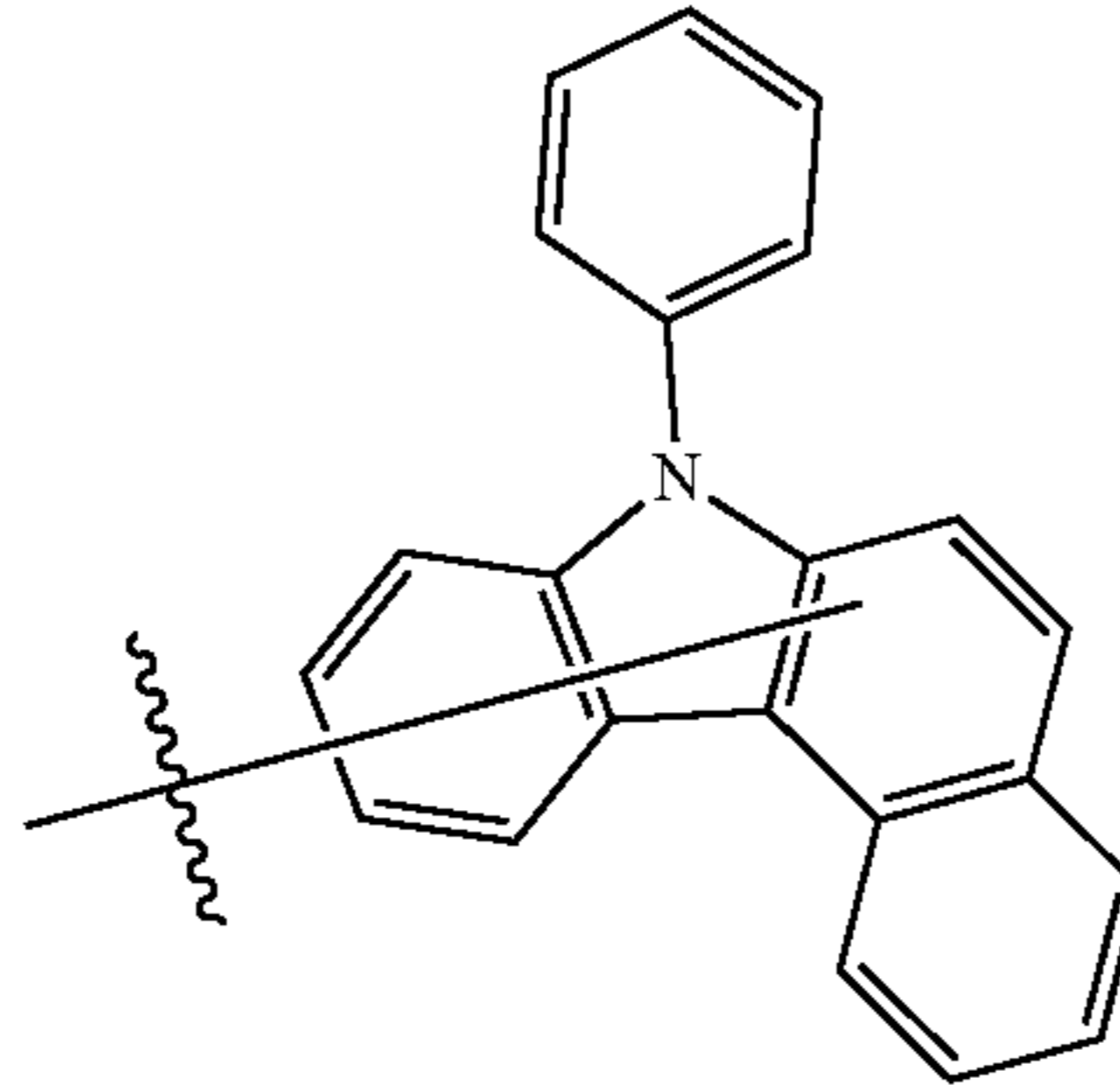
Substituent B24
