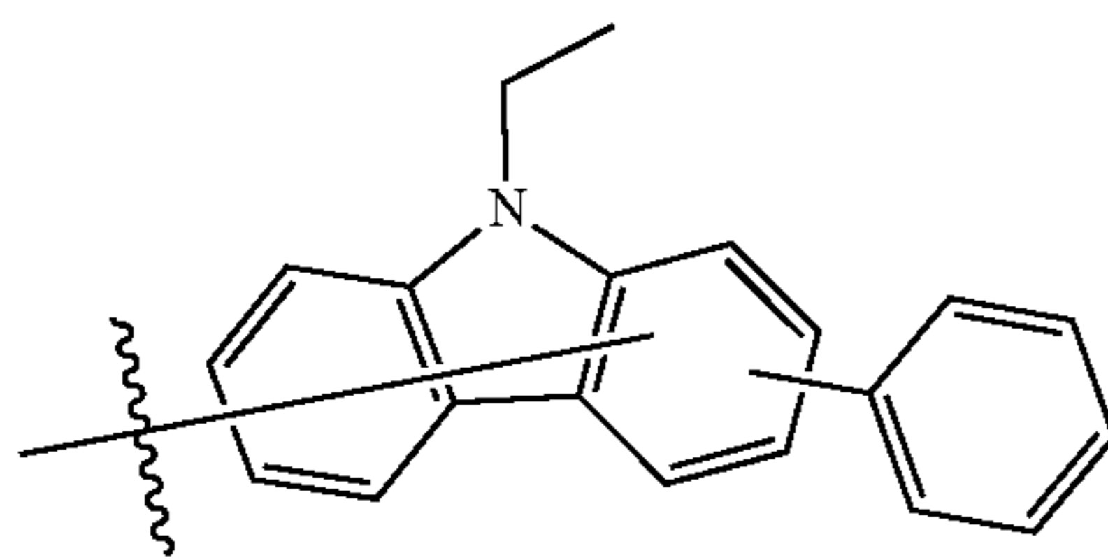
Substituent 25
