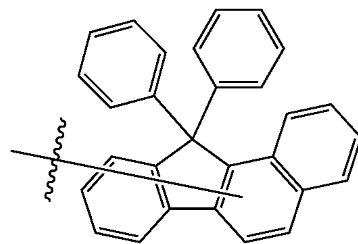
Substituent B32
