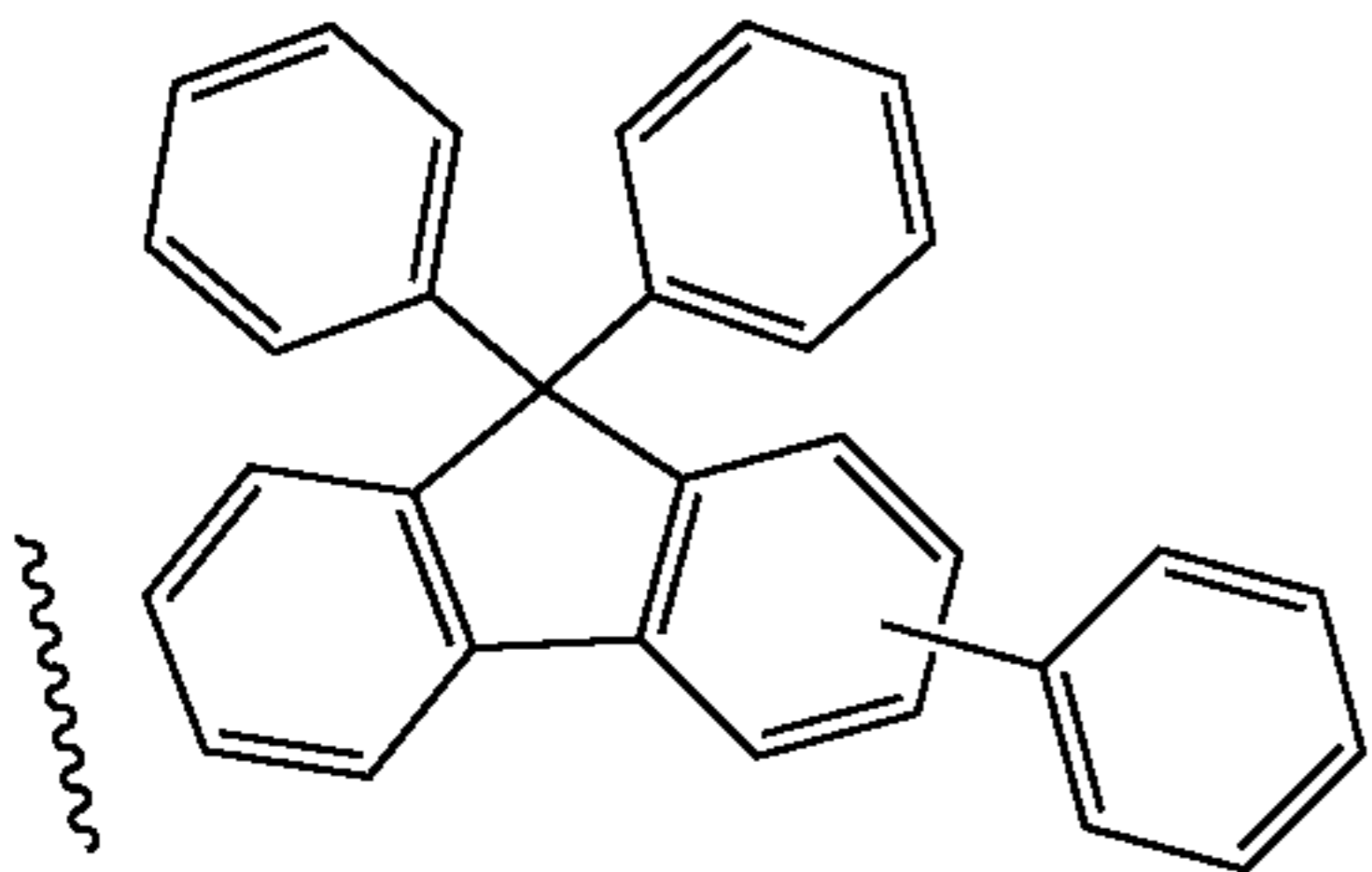
Substituent 37
