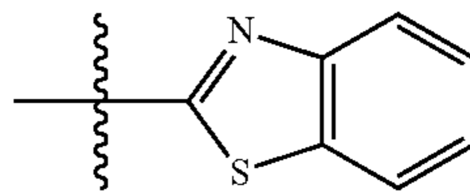
Substituent 50
