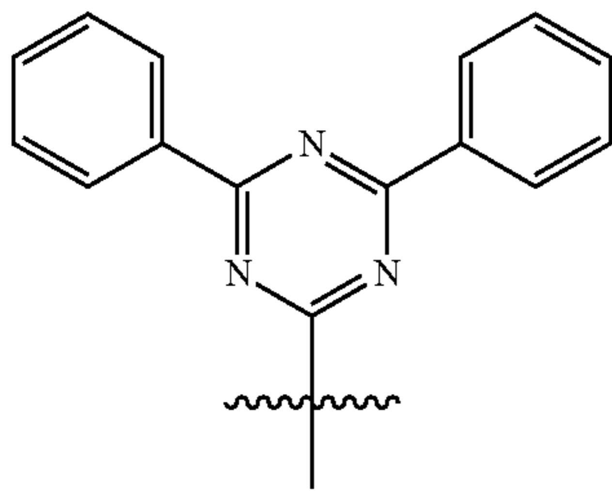
Substituent 45
