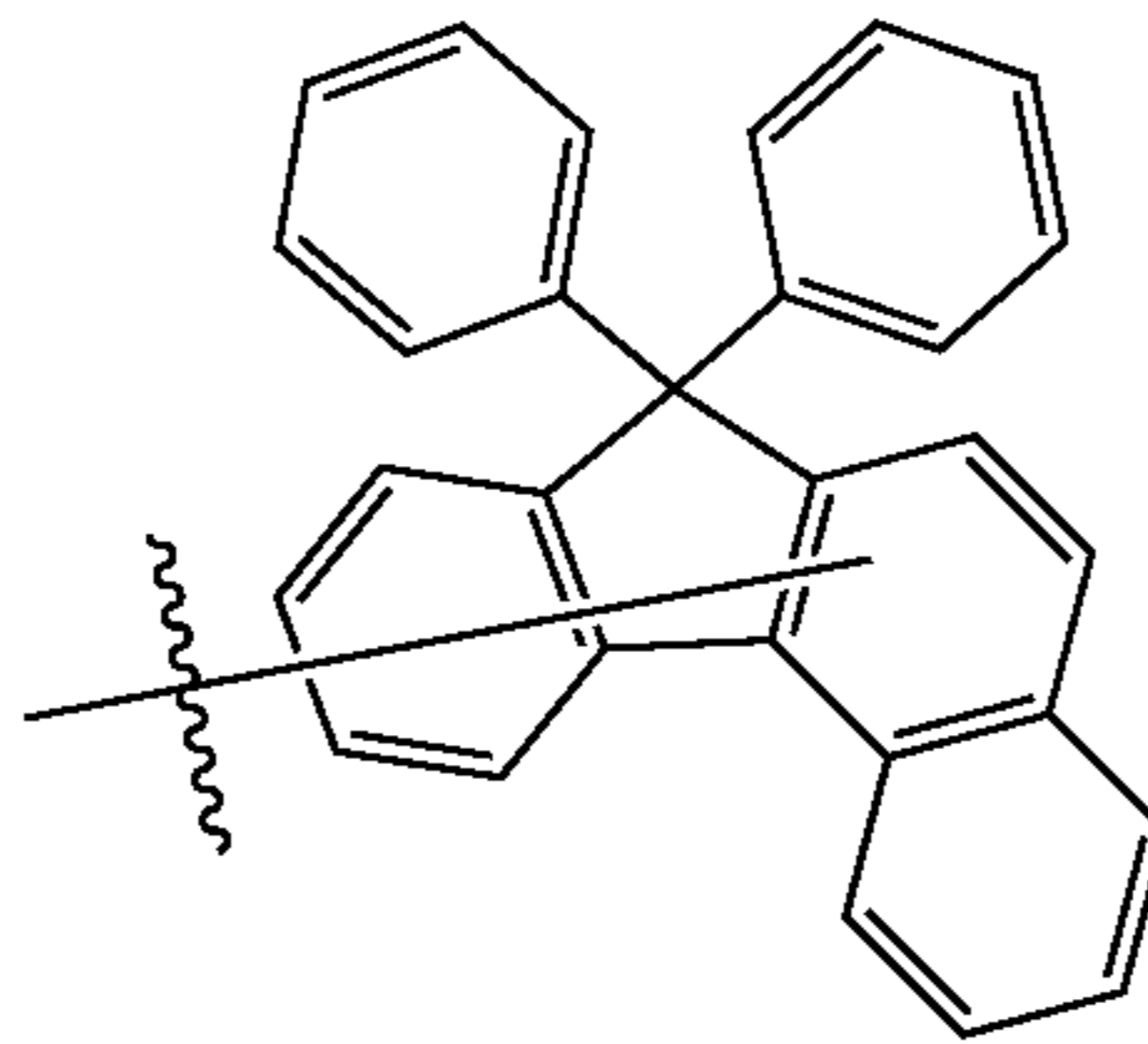
Substituent 34
