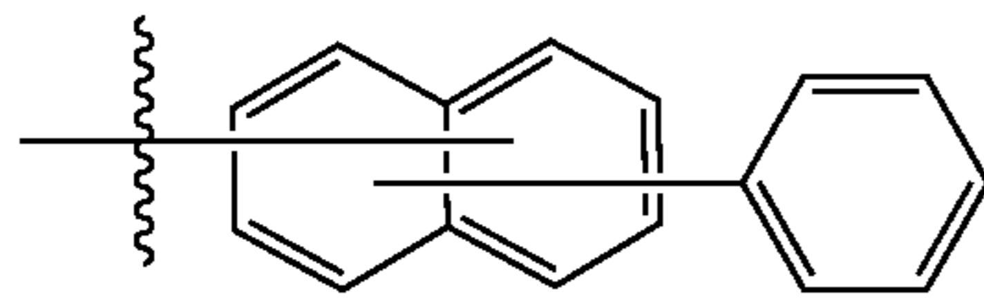
Substituent B3
