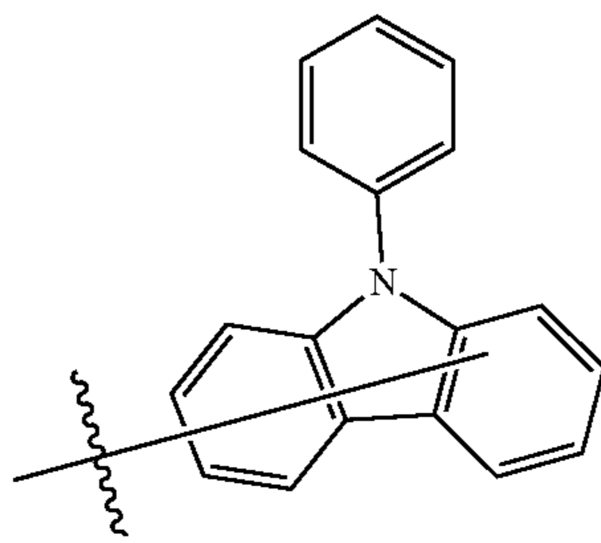
Substituent B12
