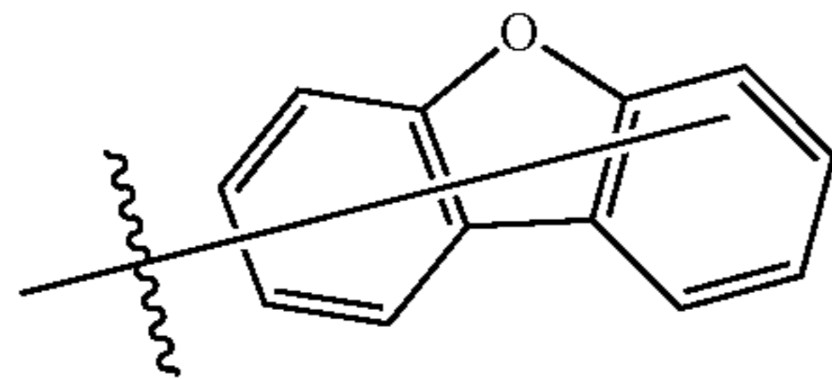
Substituent B7
