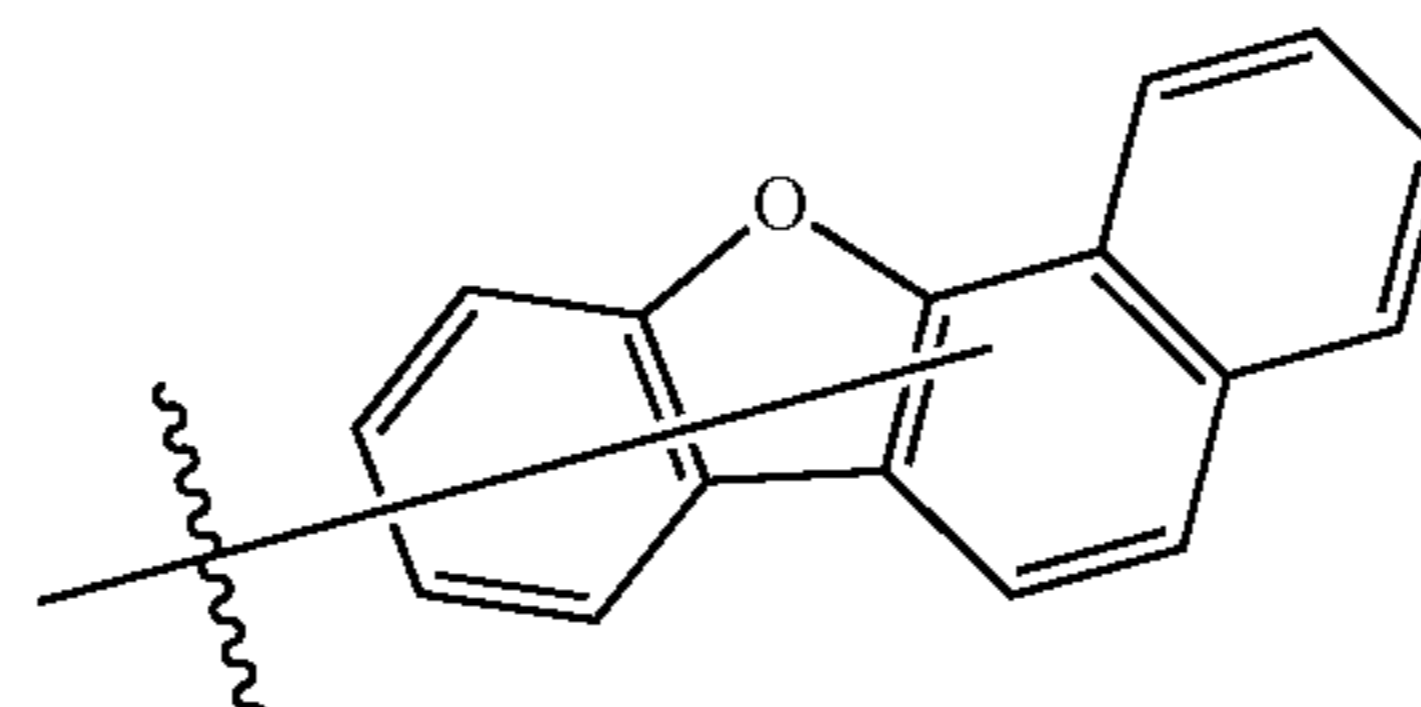
Substituent B8
