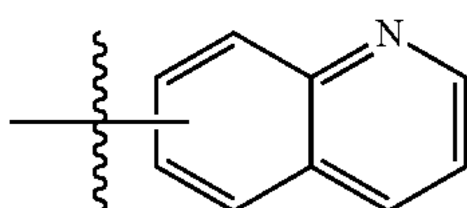
Substituent 43
