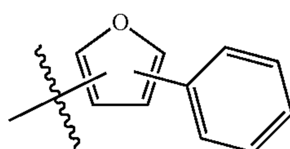
Substituent 19
