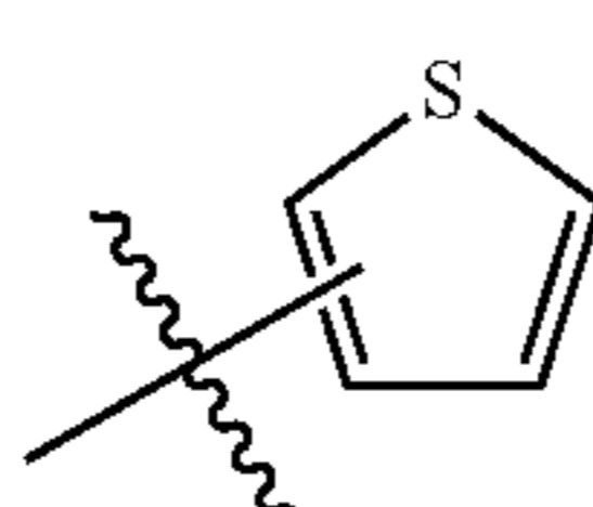
Substituent B16
