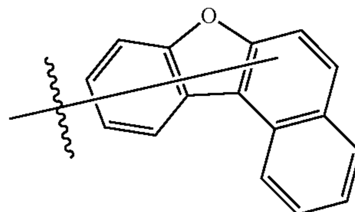
Substituent 10
