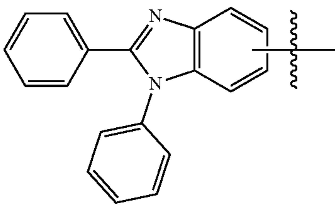
Substituent 47
