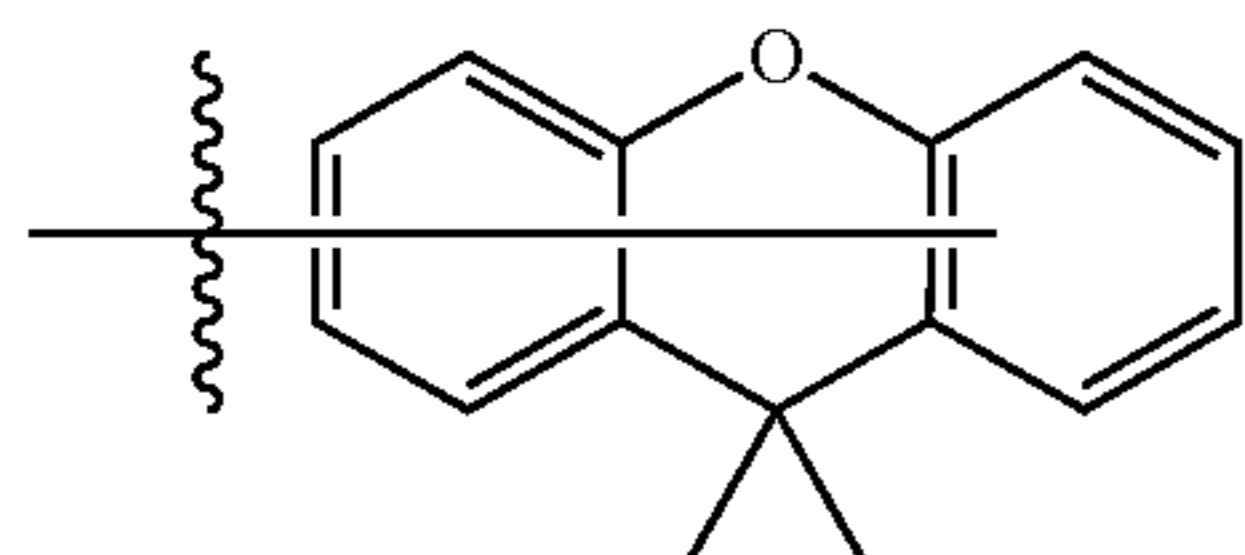
Substituent 53
