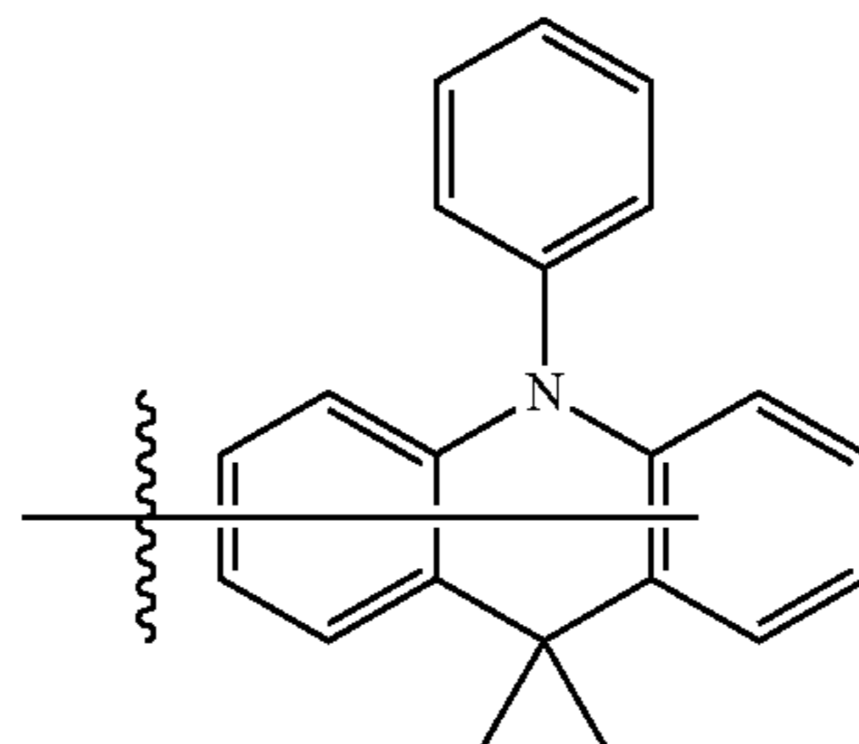
Substituent 52
