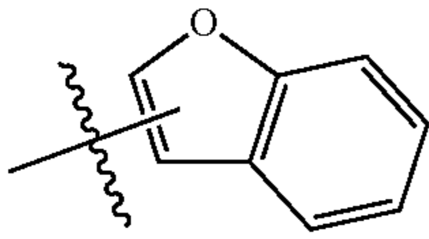
Substituent 21
