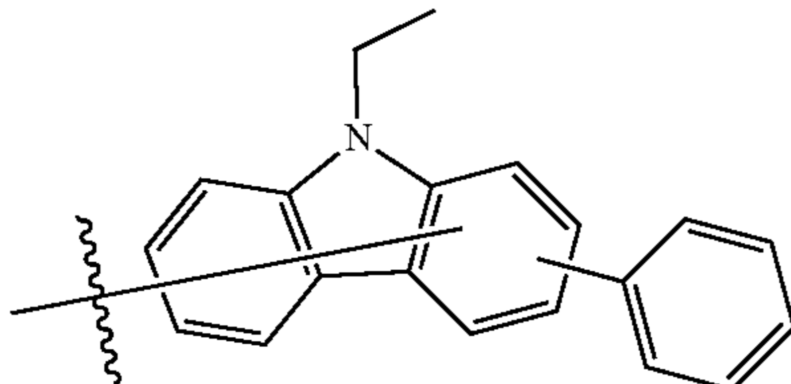
Substituent 25
