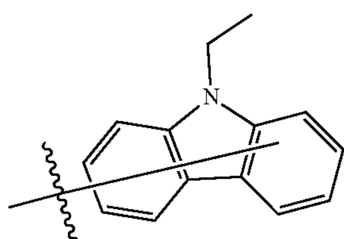
Substituent B13
