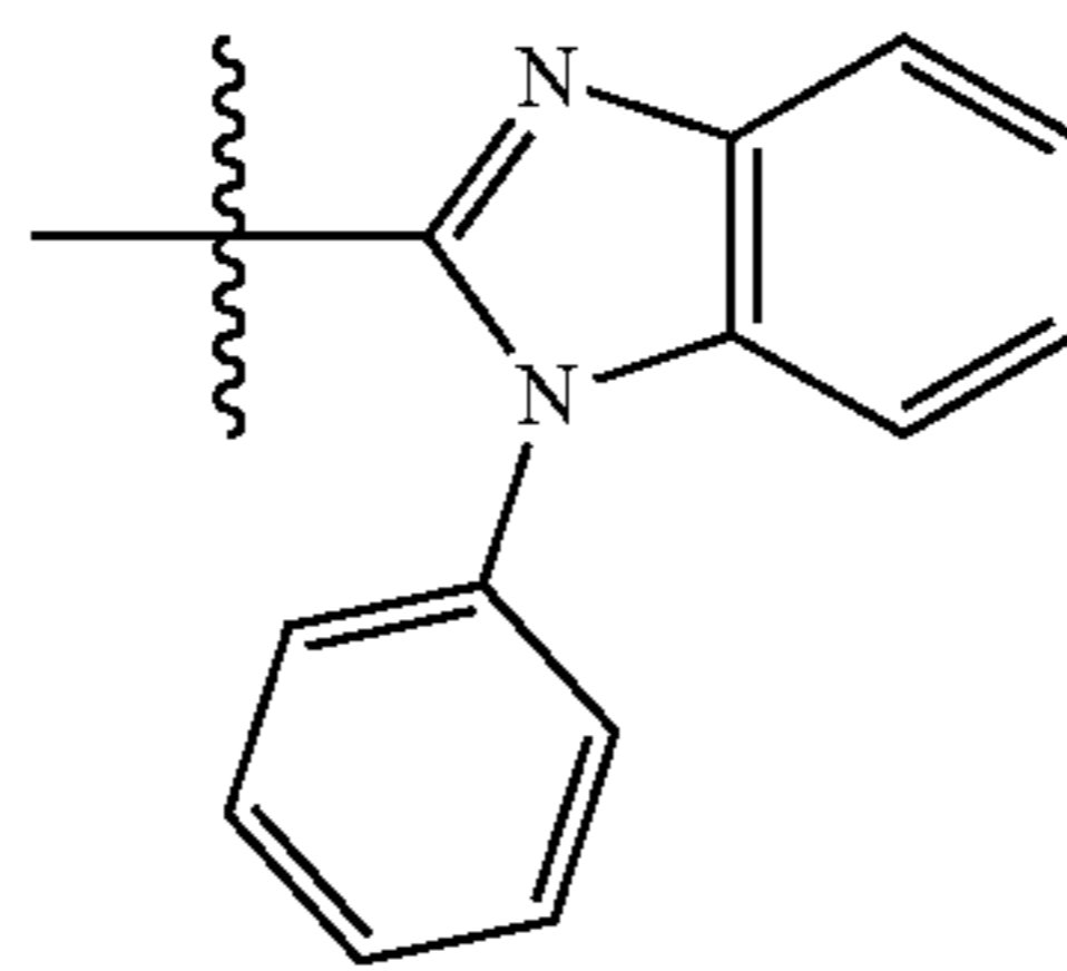
Substituent 46
