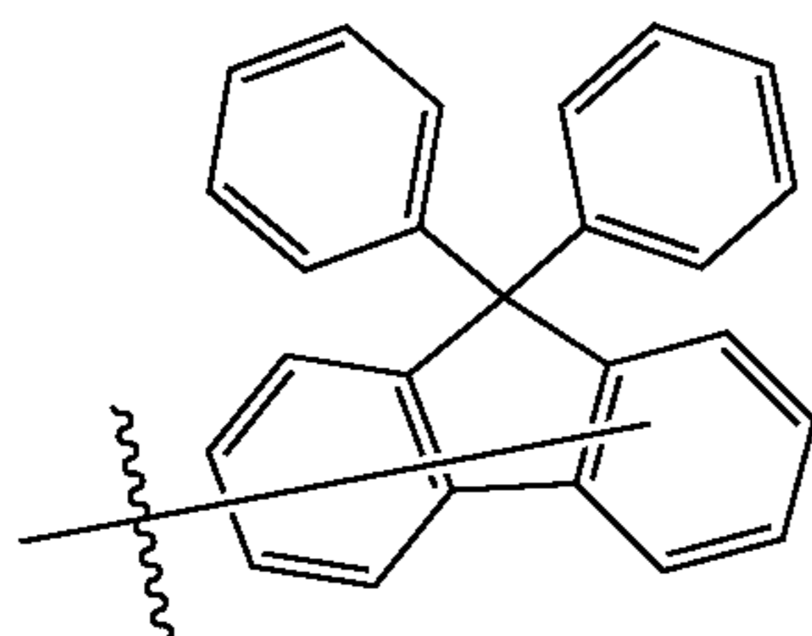
Substituent 15
