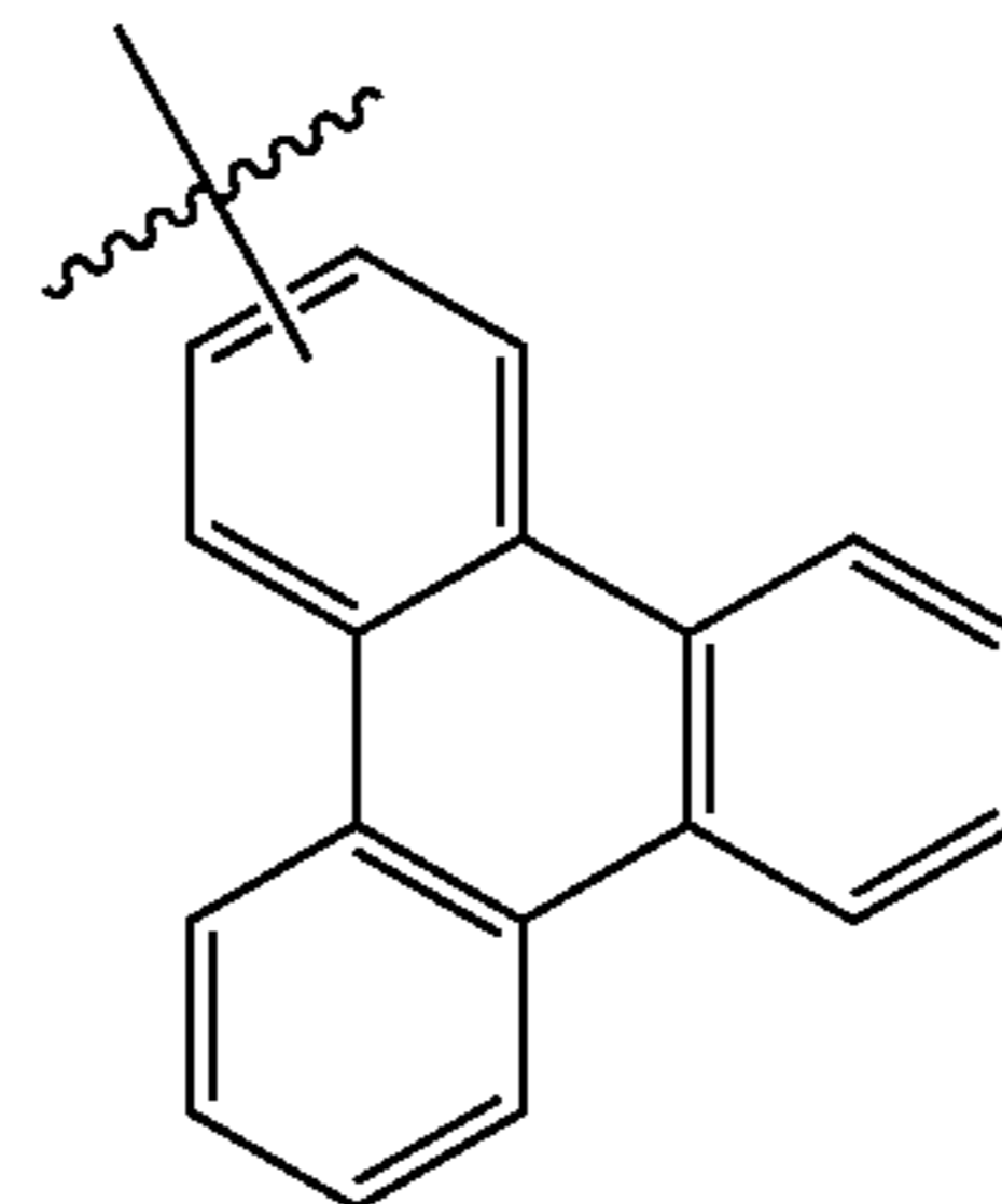
Substituent B6
