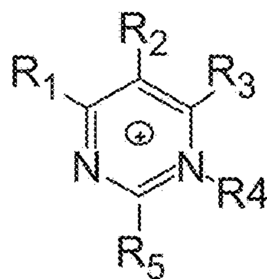
Pyrimidinium
