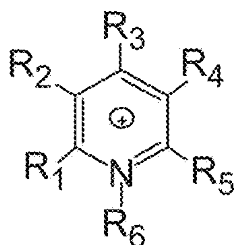
Pyridinium
