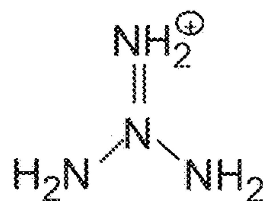
Guanidium
