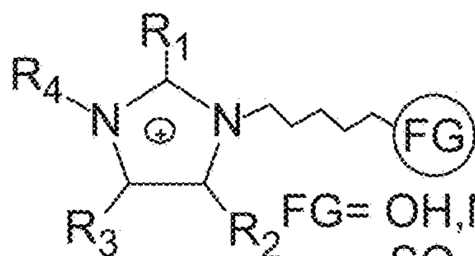
Functionalized Imidazolium Cations
