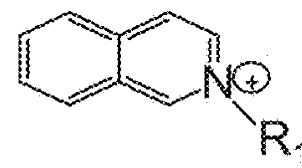
Isoquinolinium
