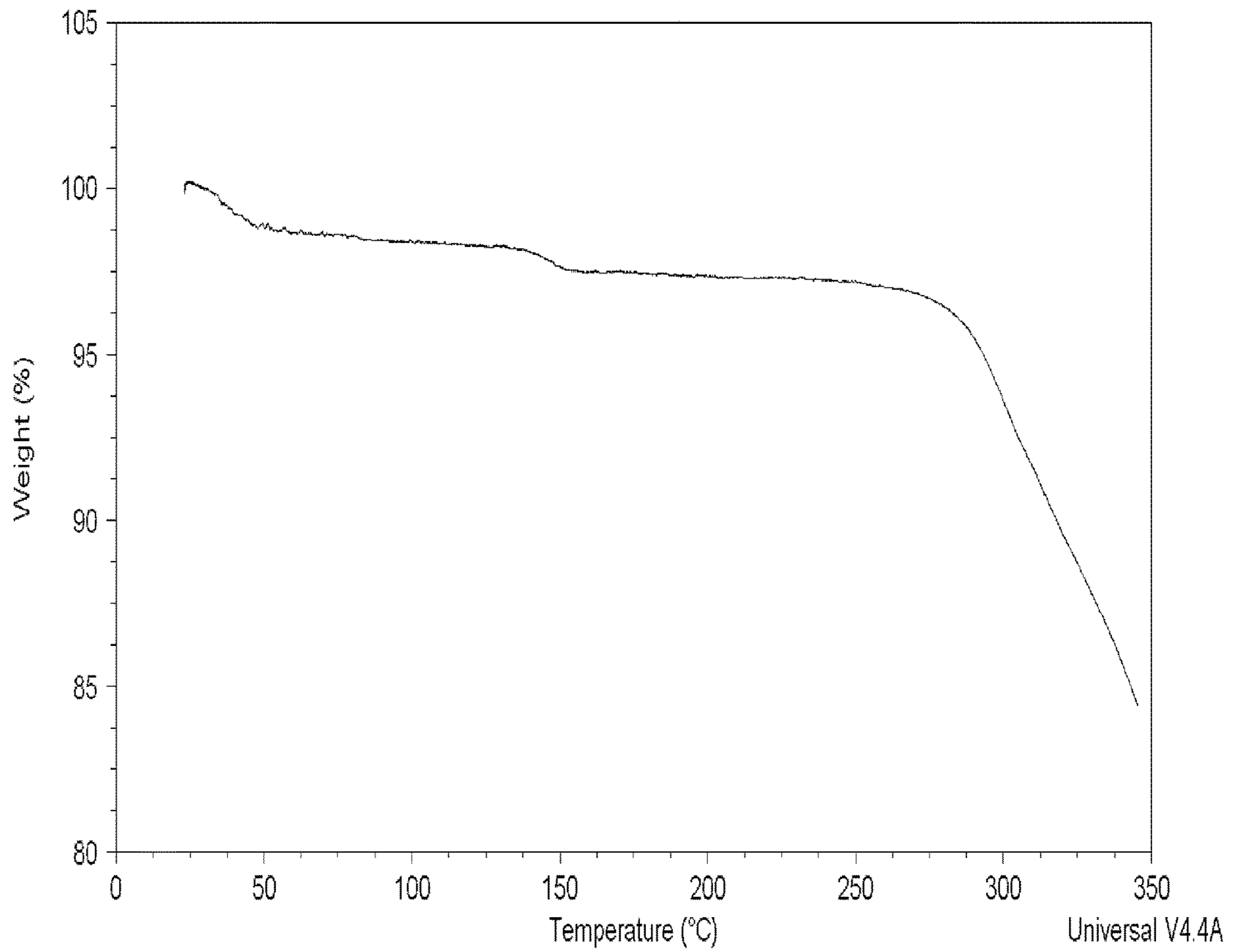
FIGURE 2d: TGA Compound I-1 (anhydrous form B)
