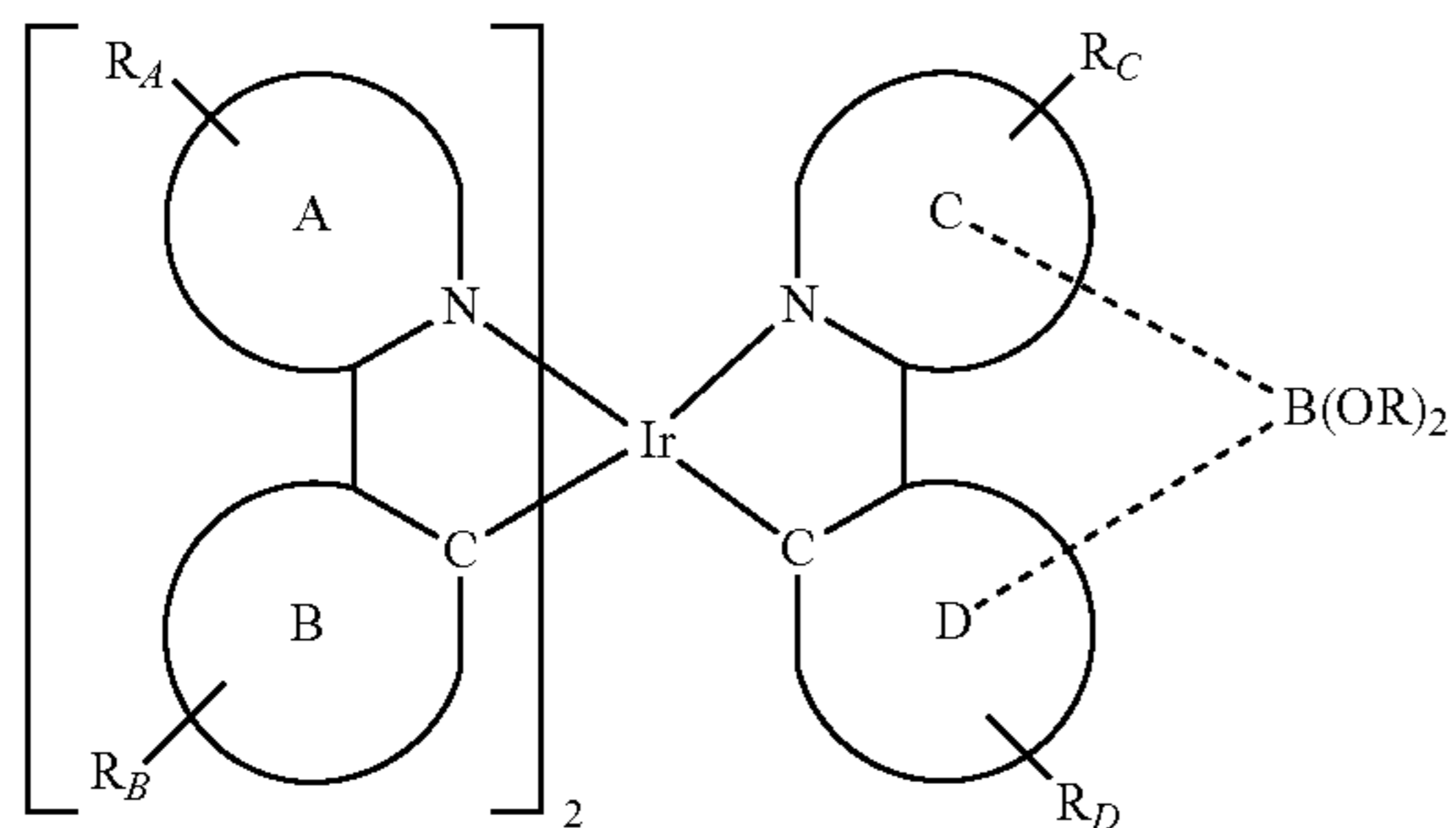
Compound 5
