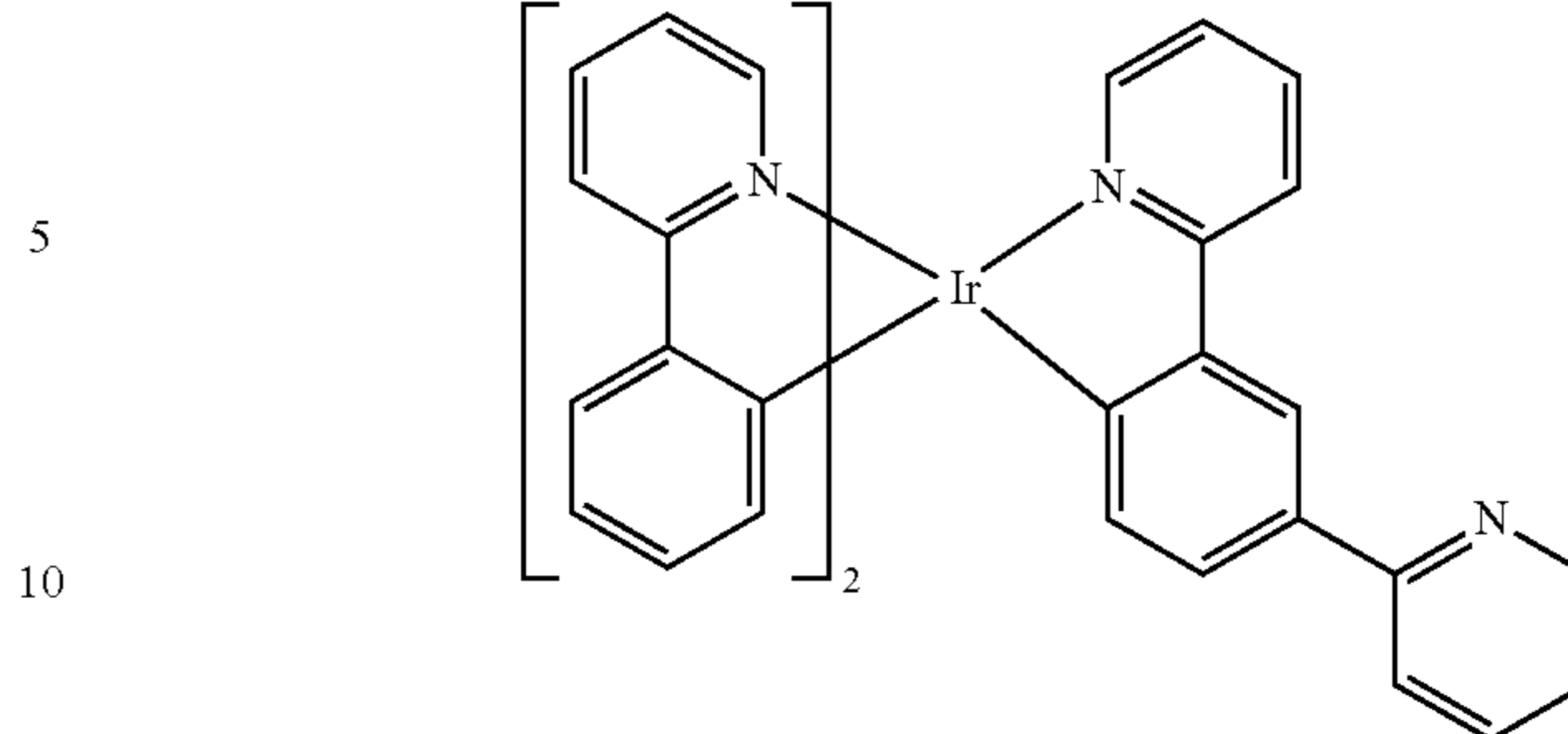
Compound 4
