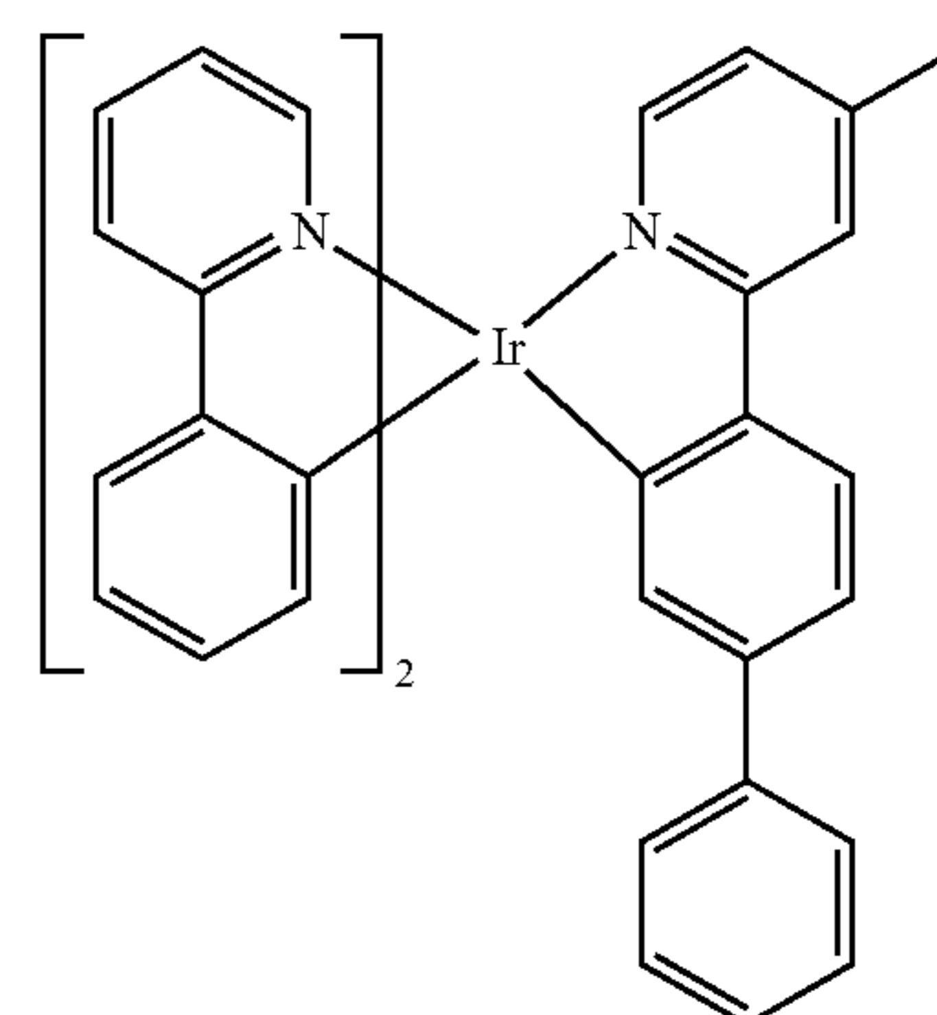
Compound 9
