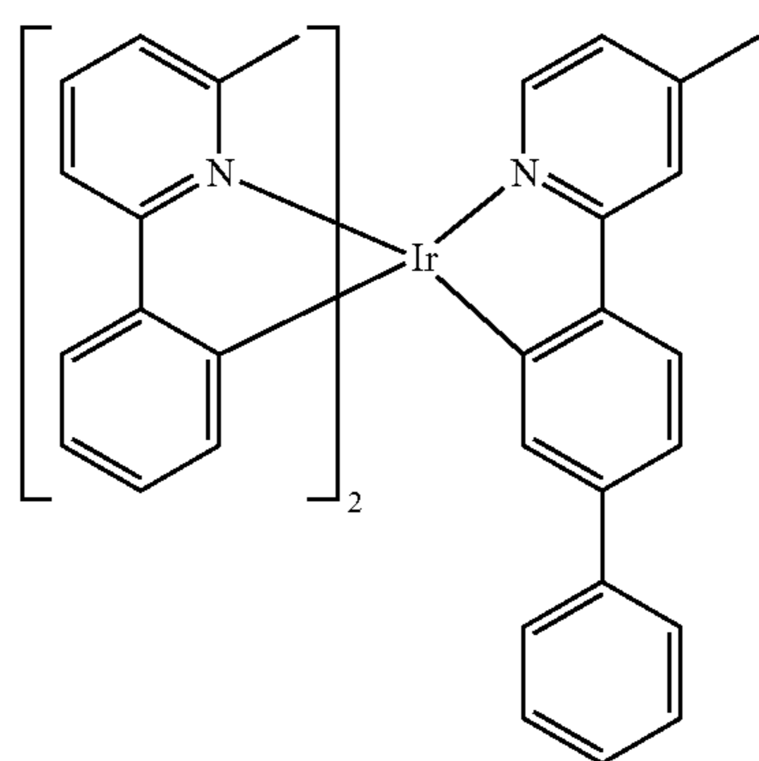
Compound 10
