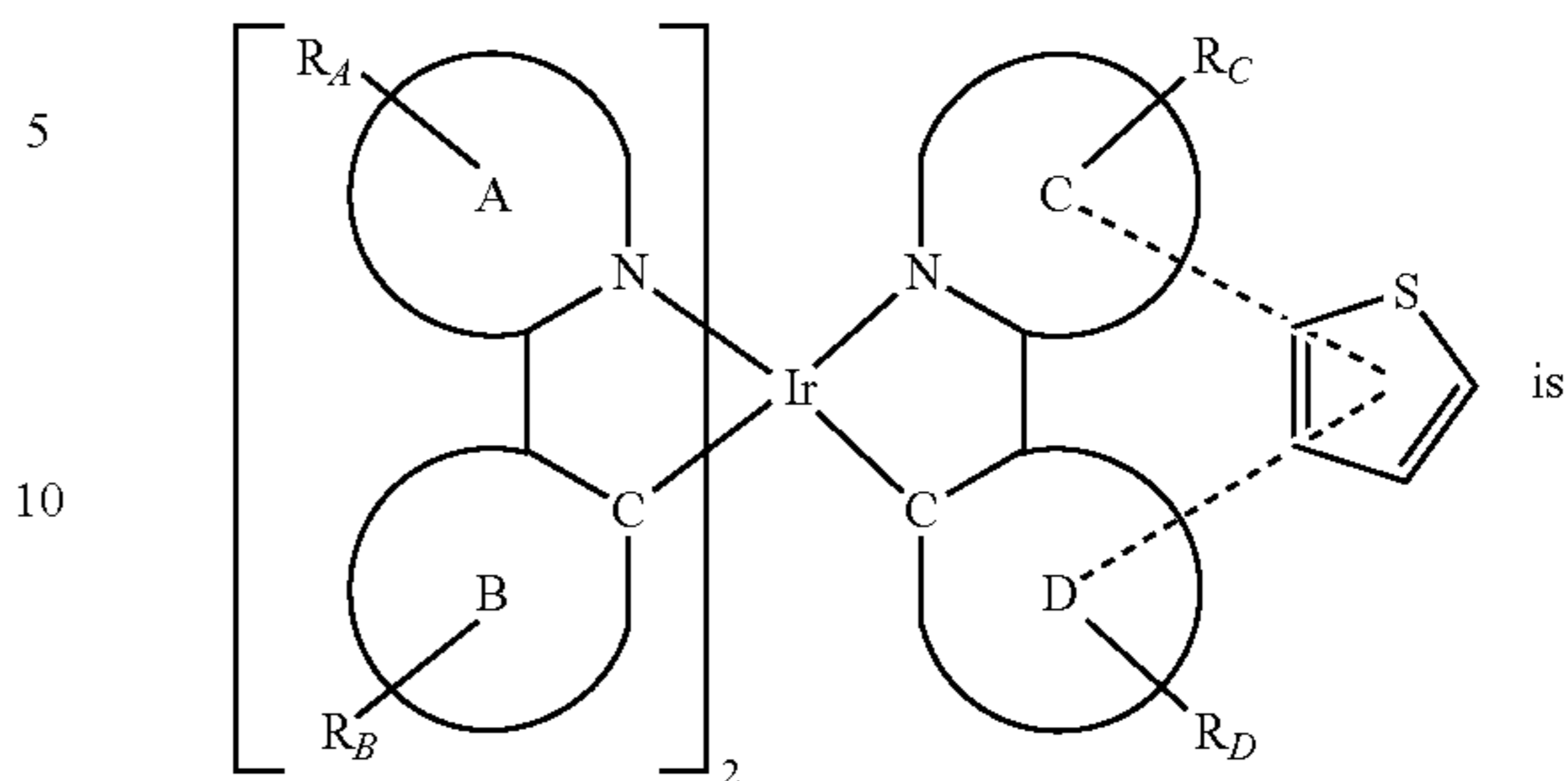
Compound 5
