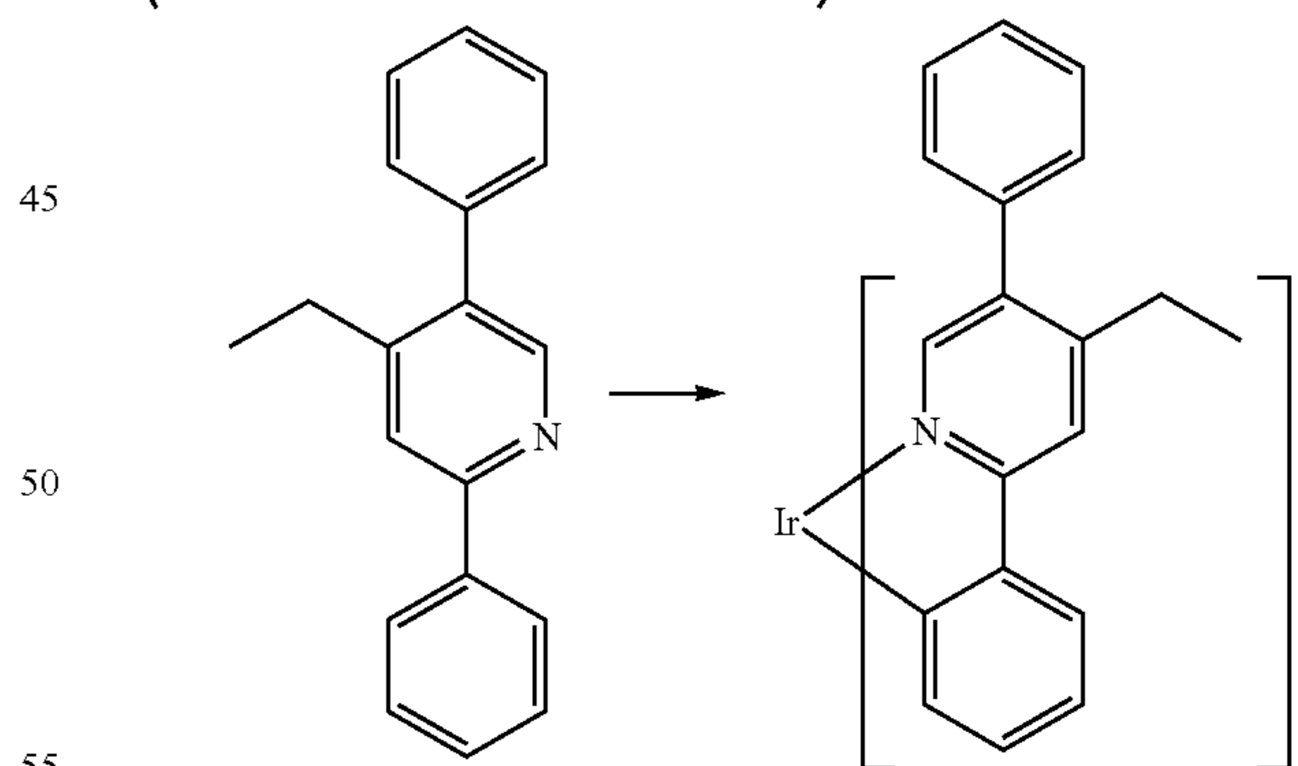
Compound 22
