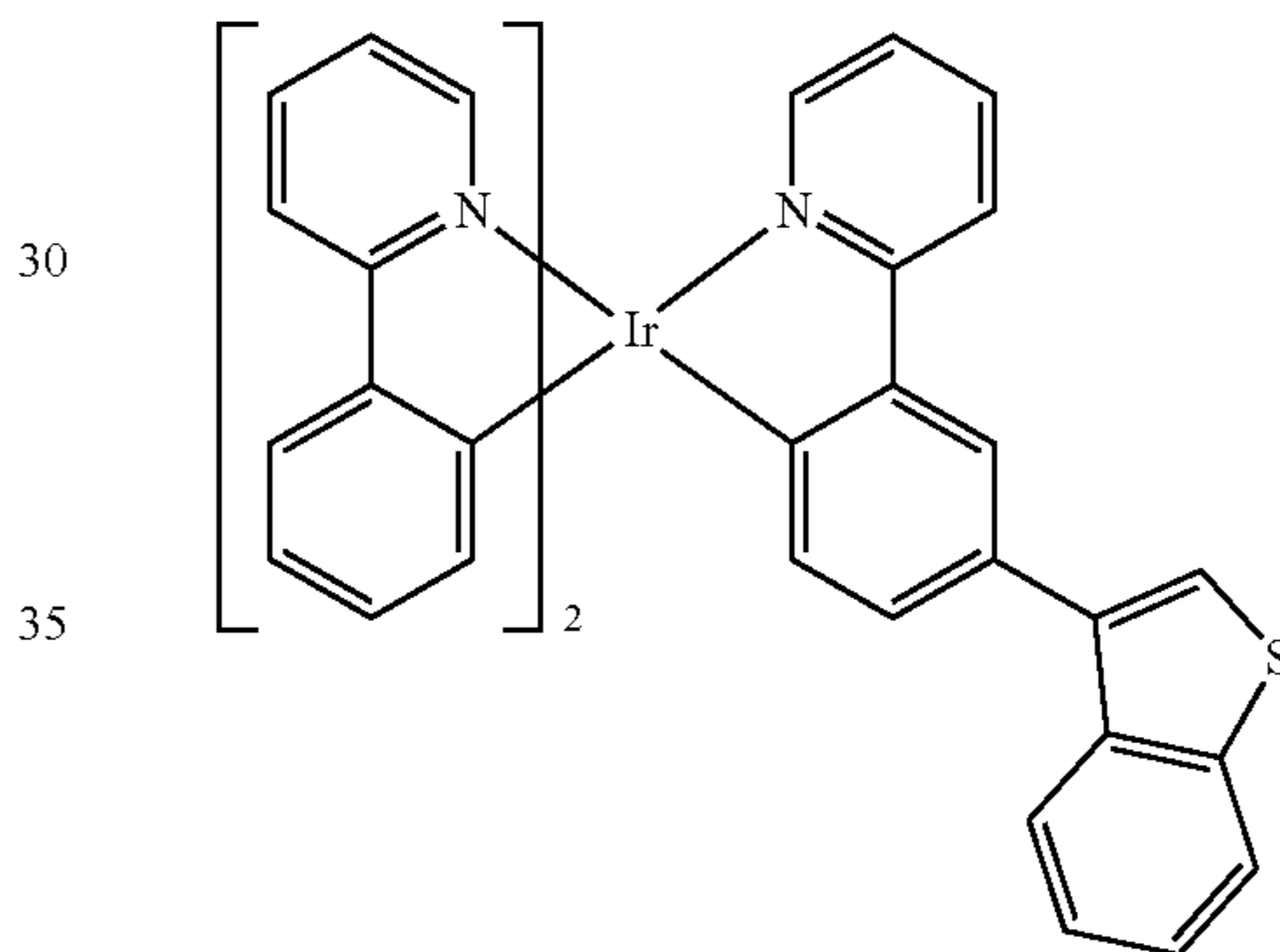
Compound 6
