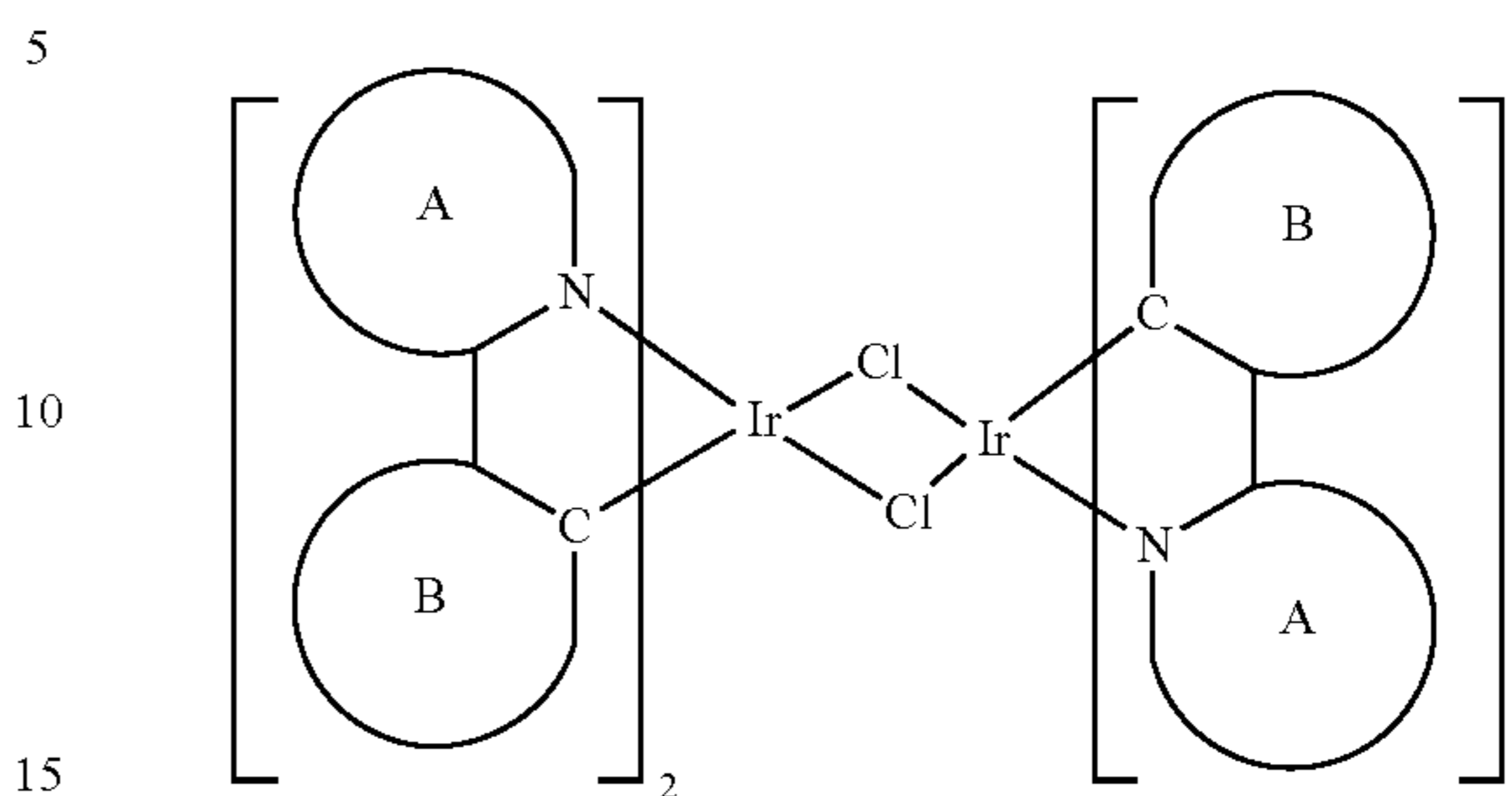
Compound 6
