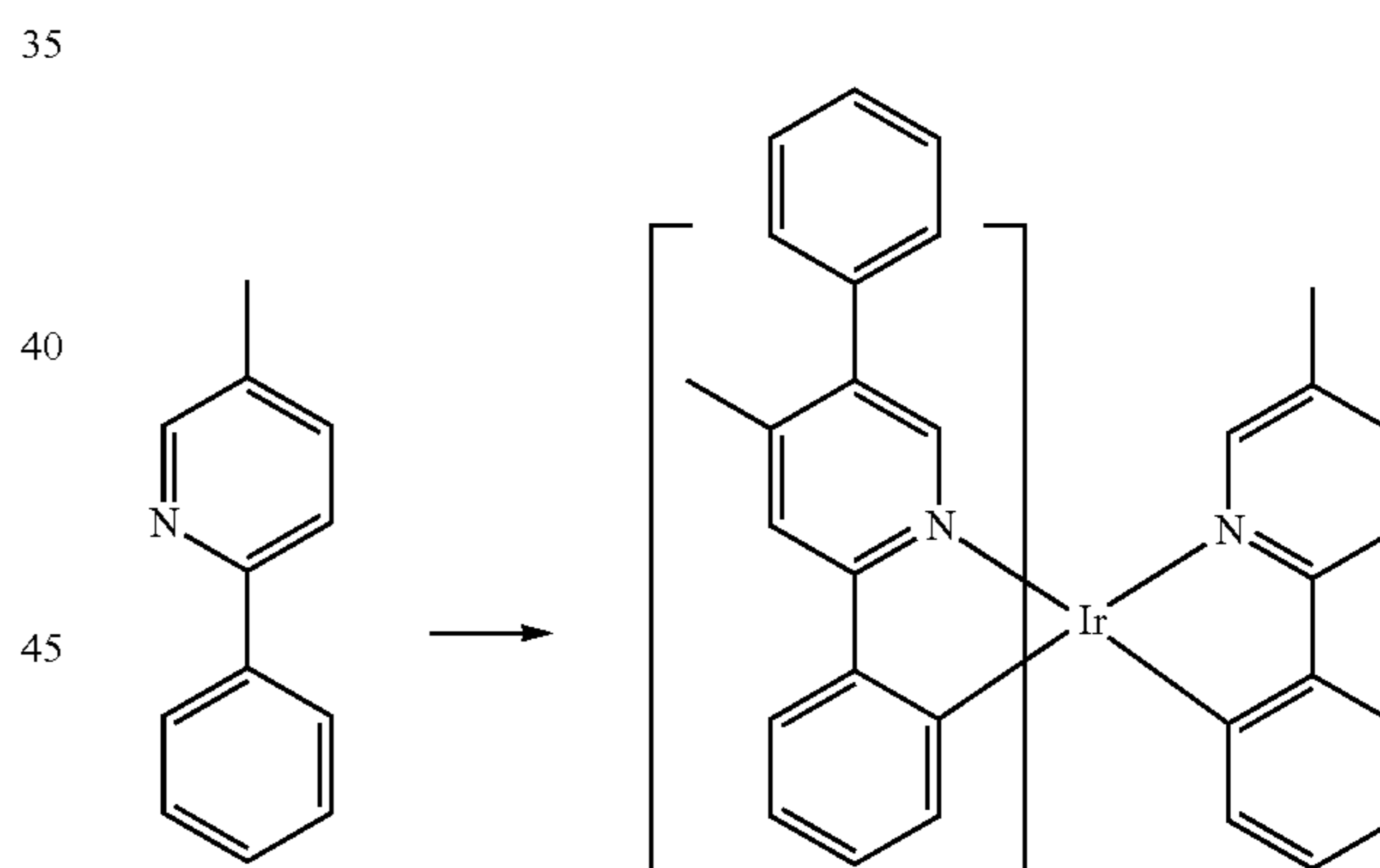
Compound 34
