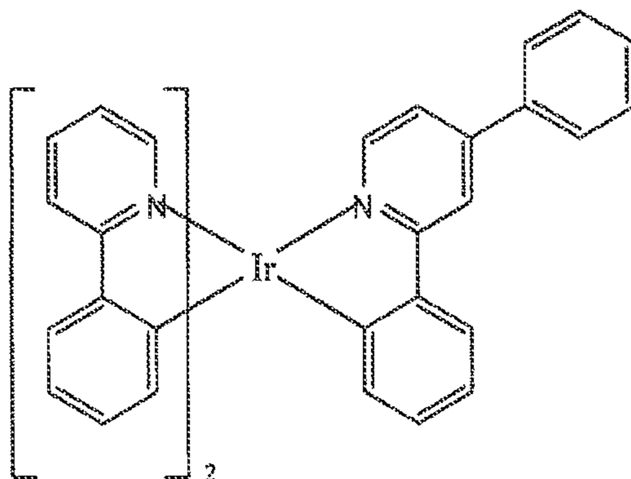
Compound 1
