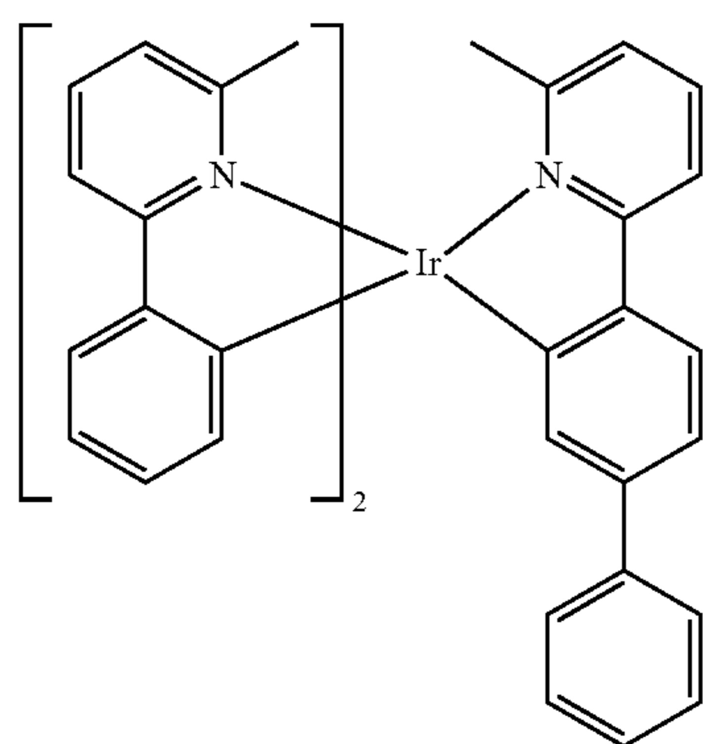
Compound 13
