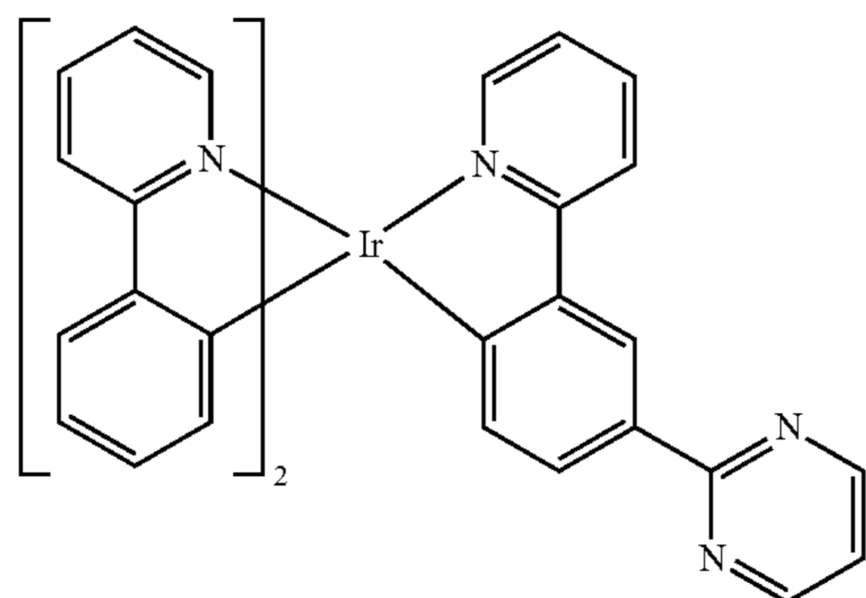
Compound 3
