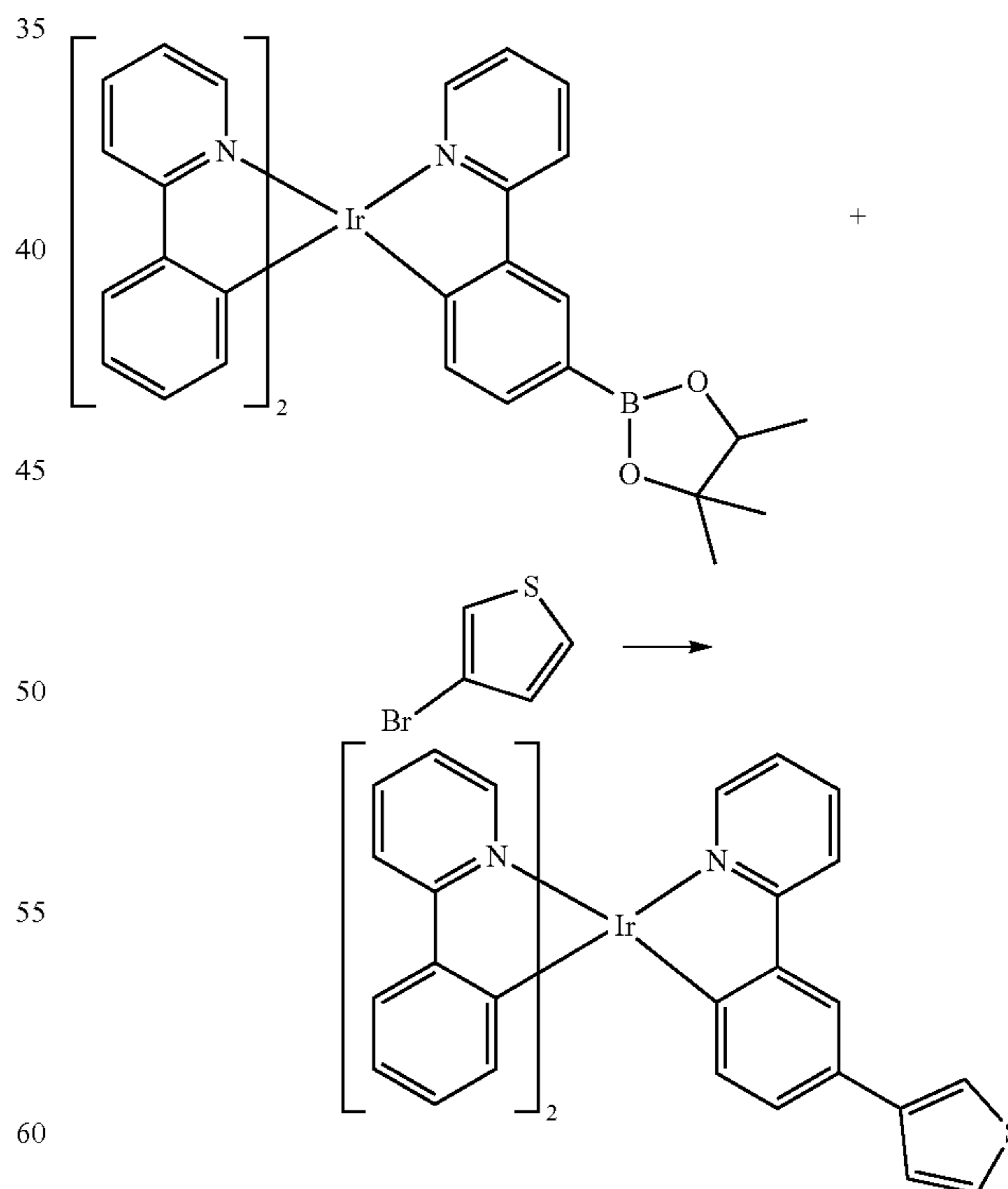
Compound 5
