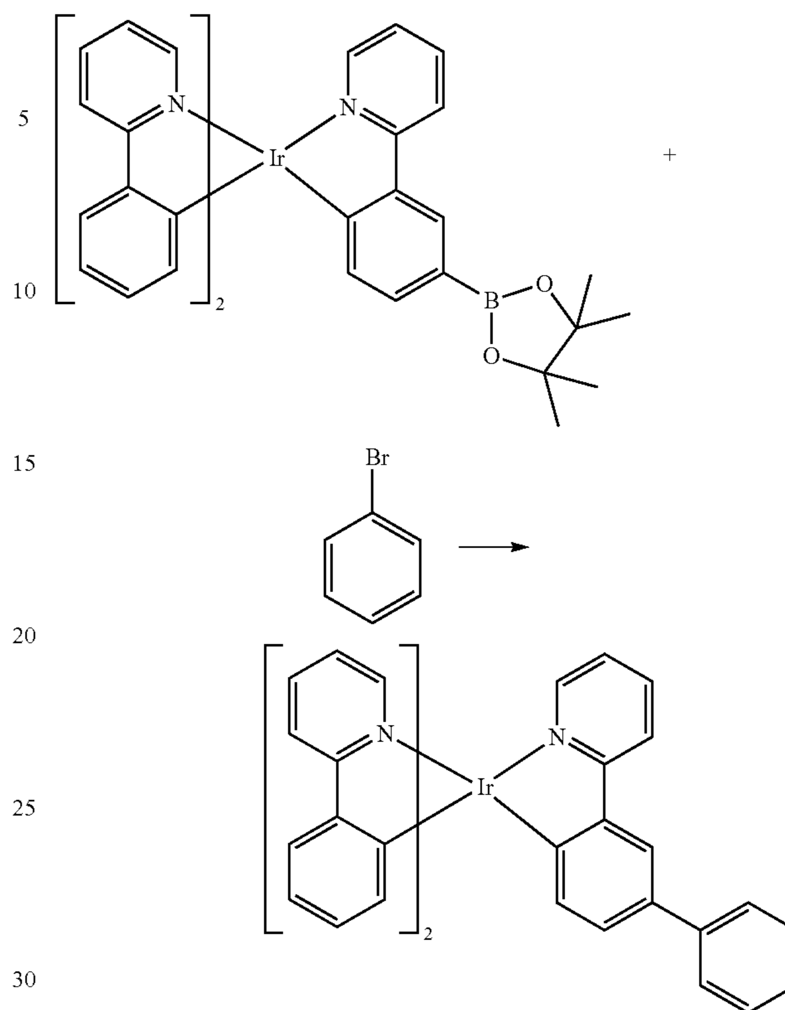
Compound 7
