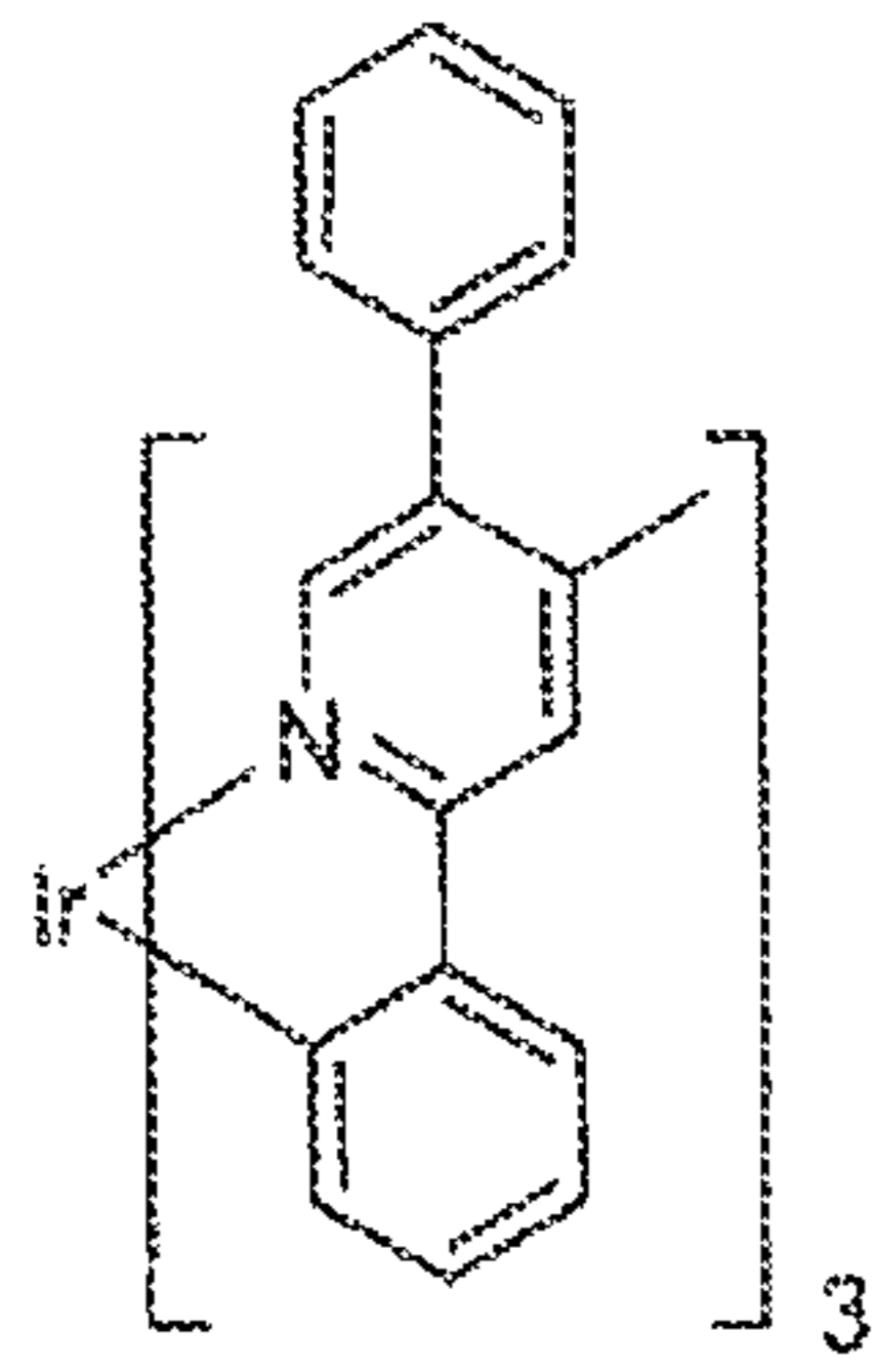
Compound 21
