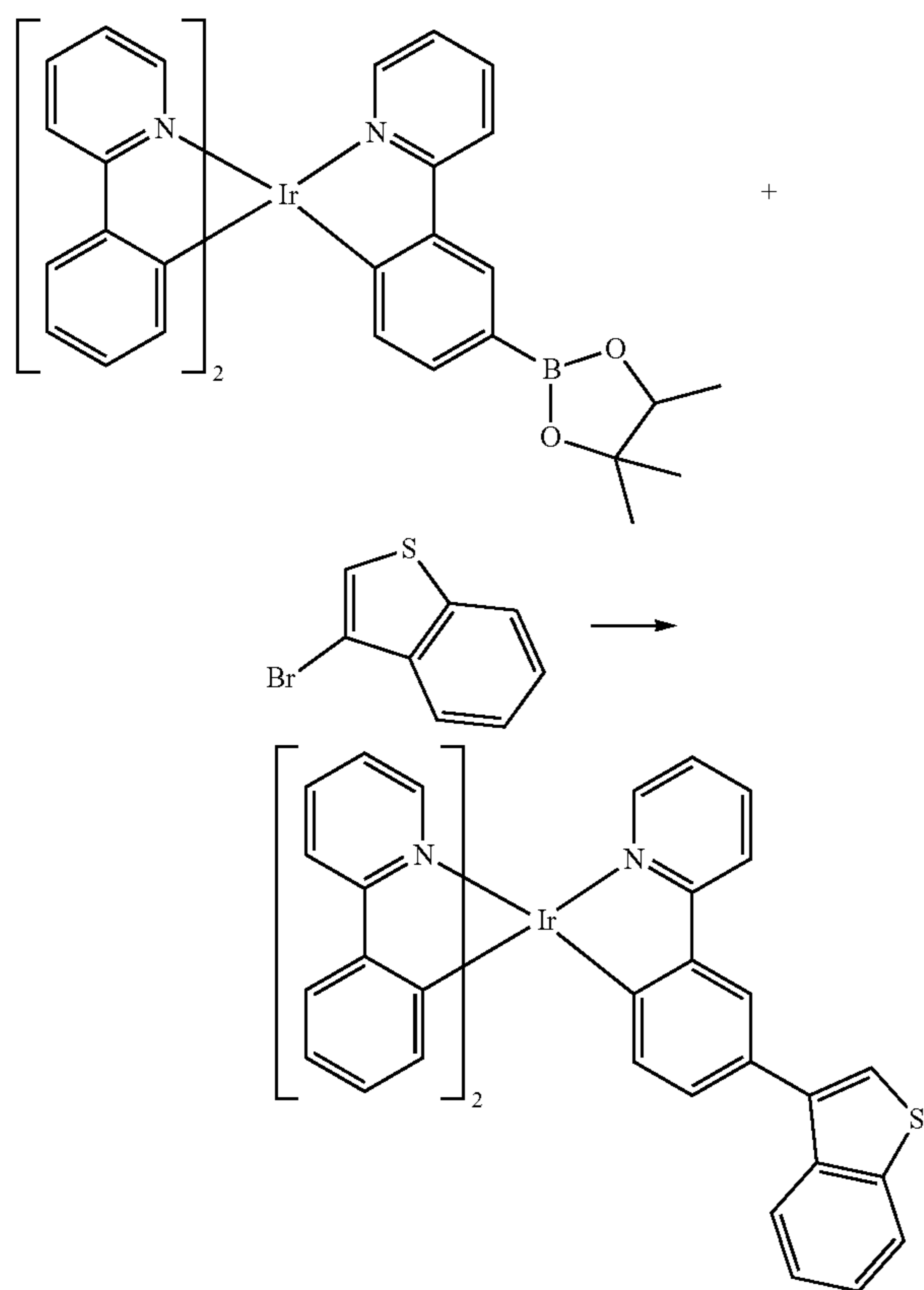
Compound 6
