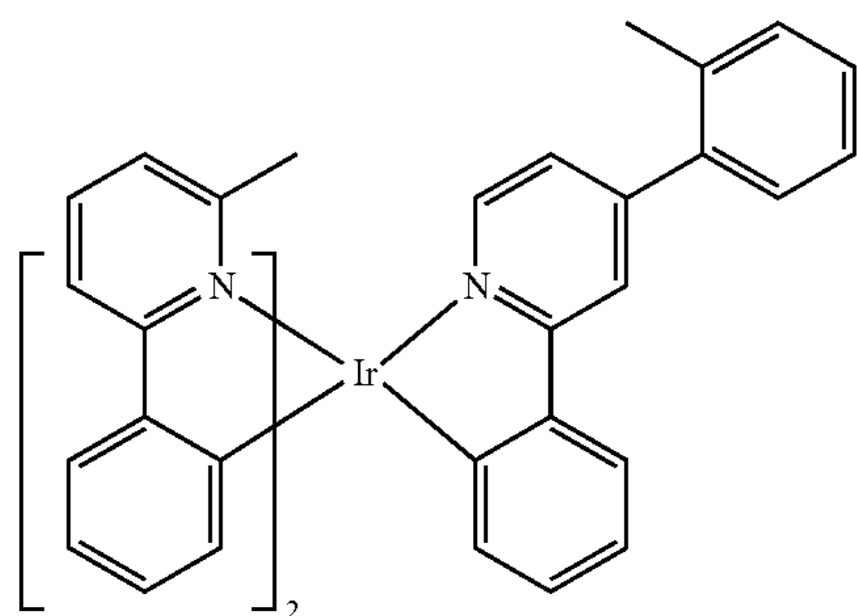
Compound 28
