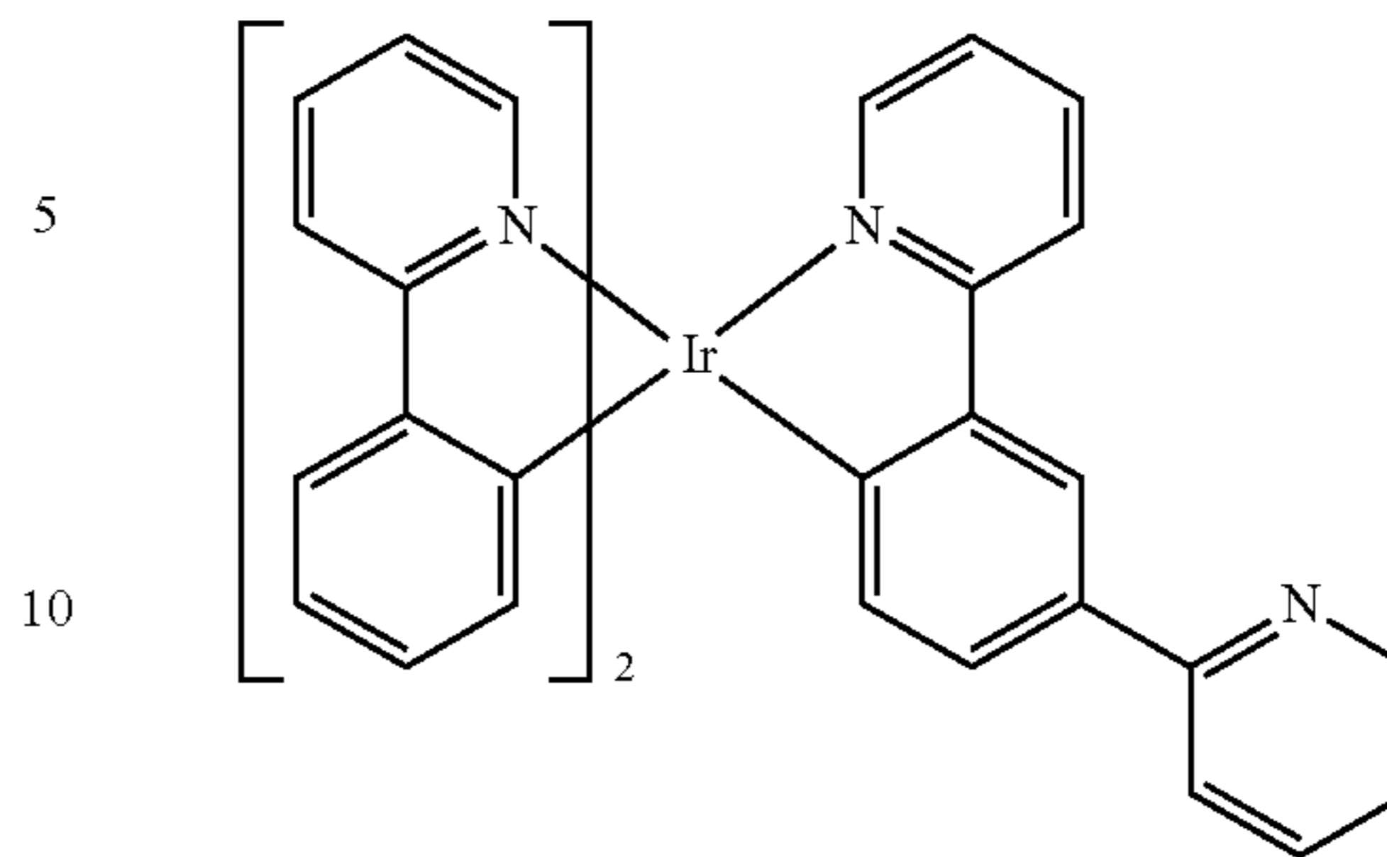
Compound 5
