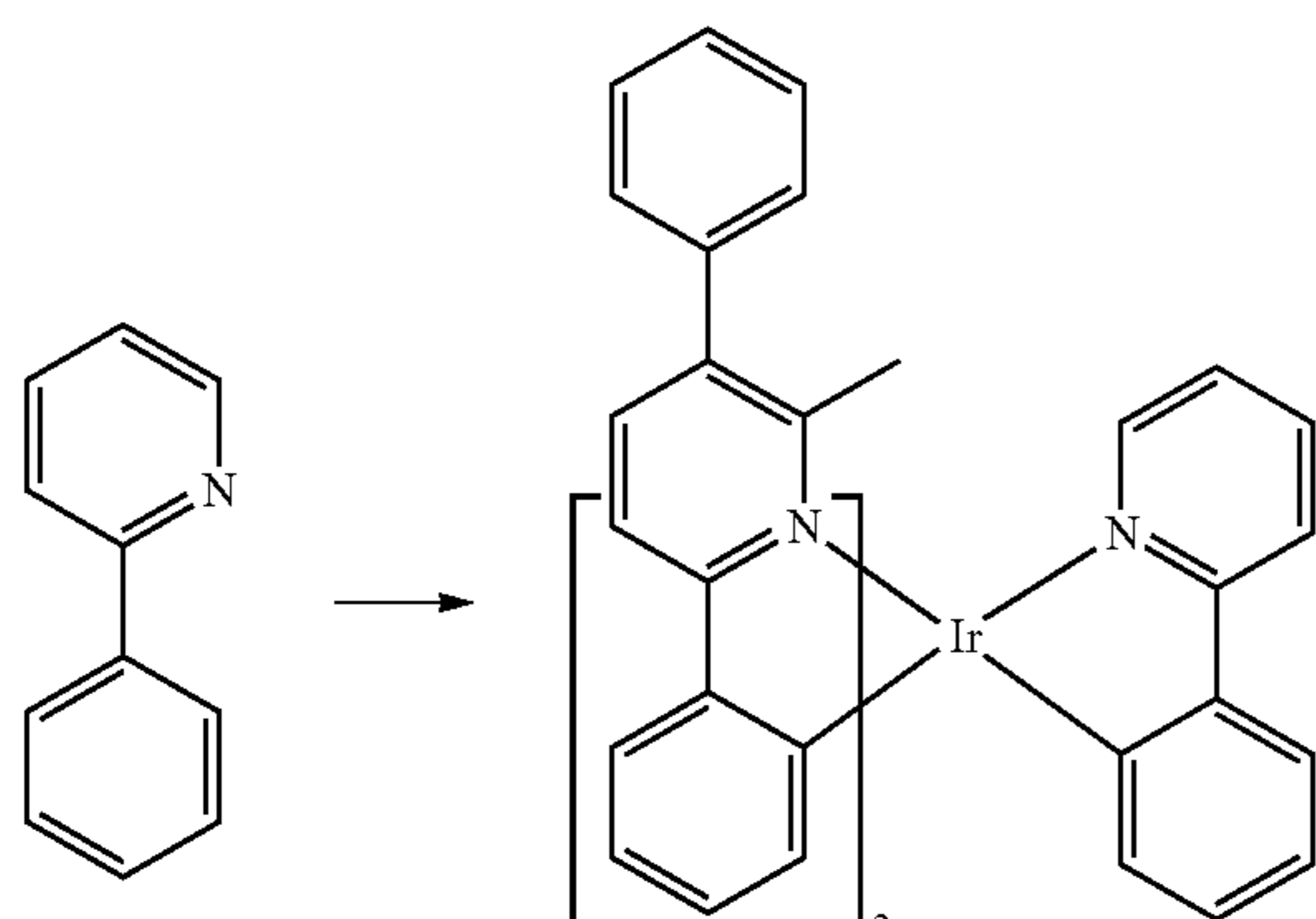
Compound 33
