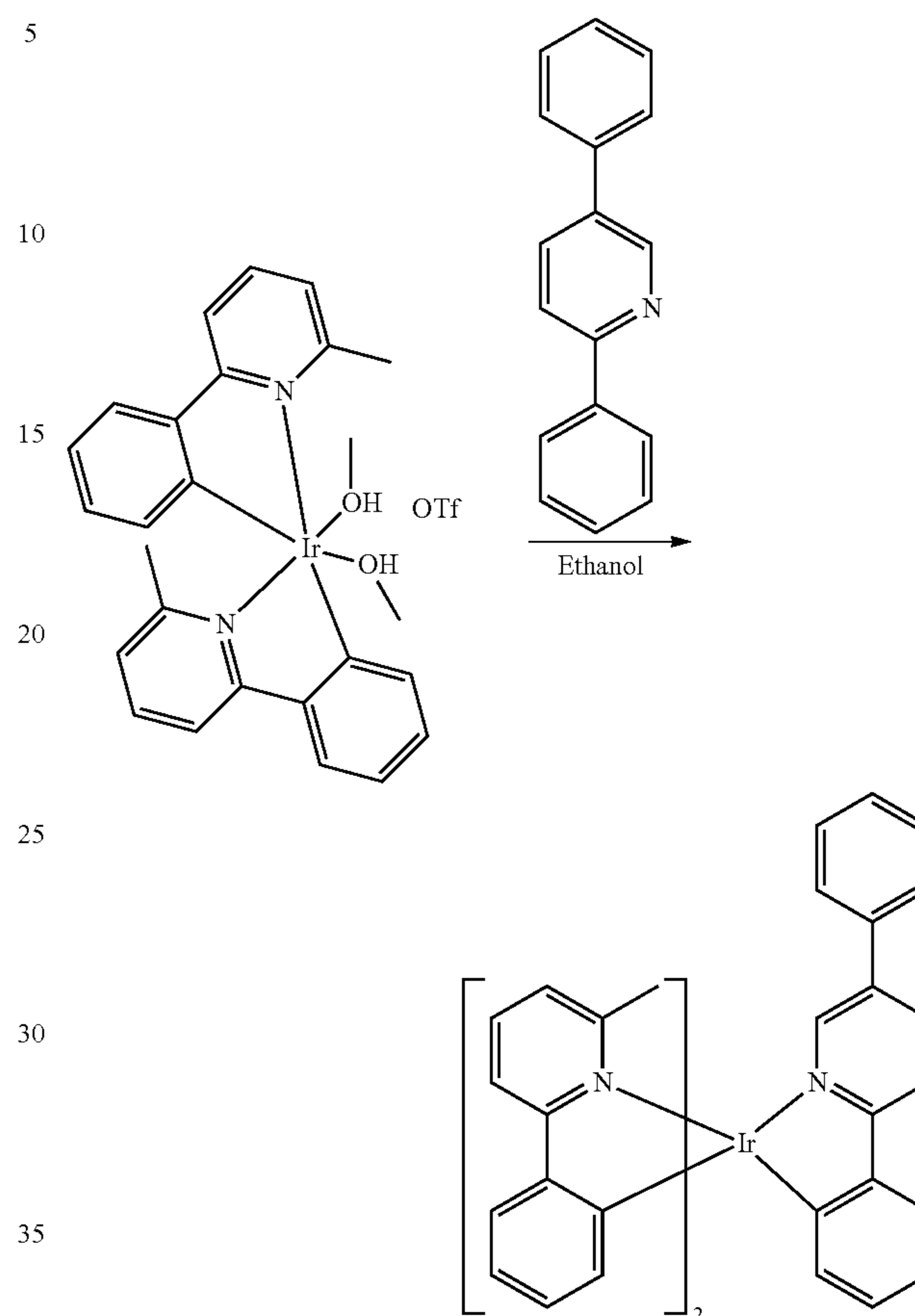
Compound 11
