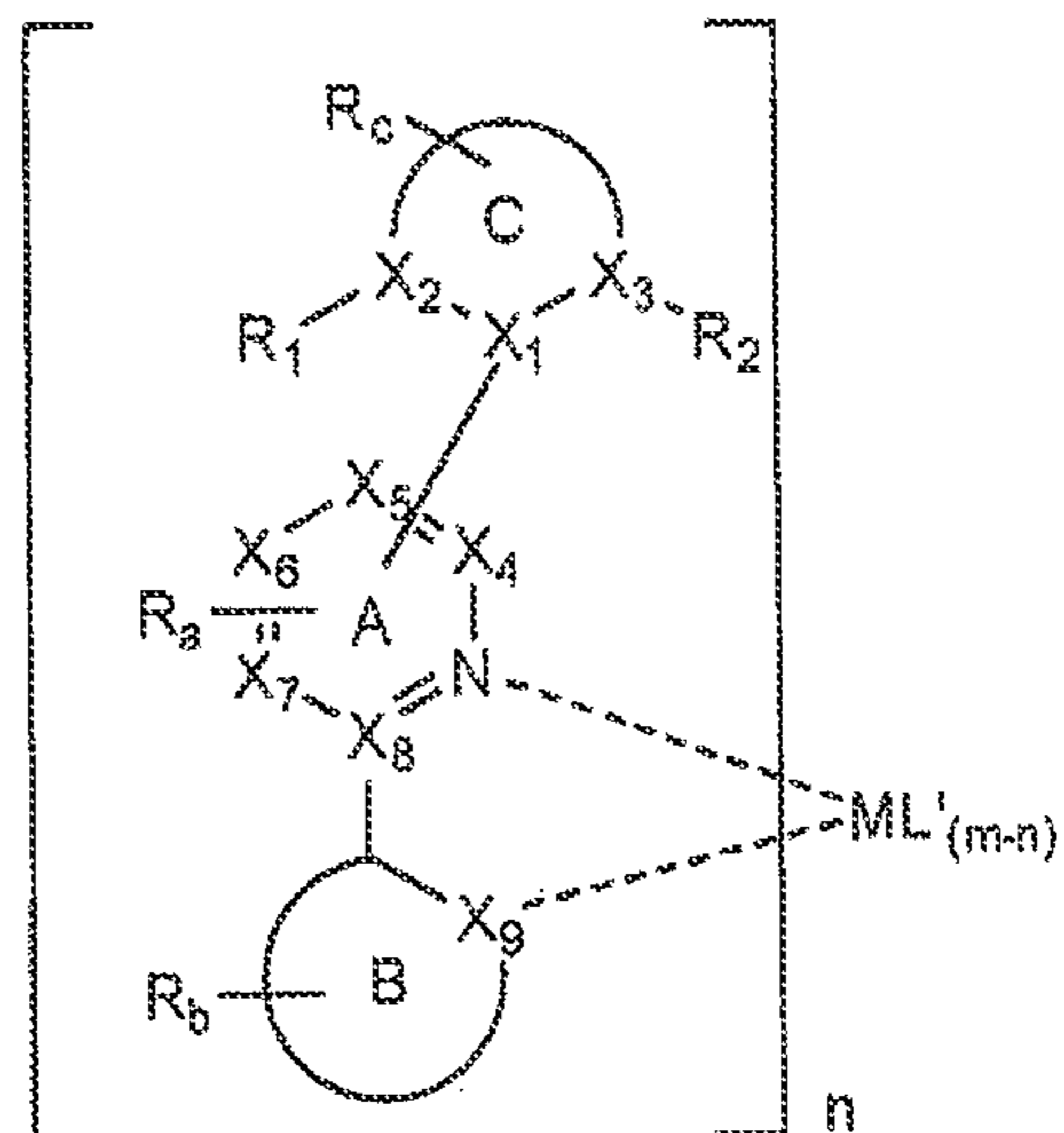
Formula II
