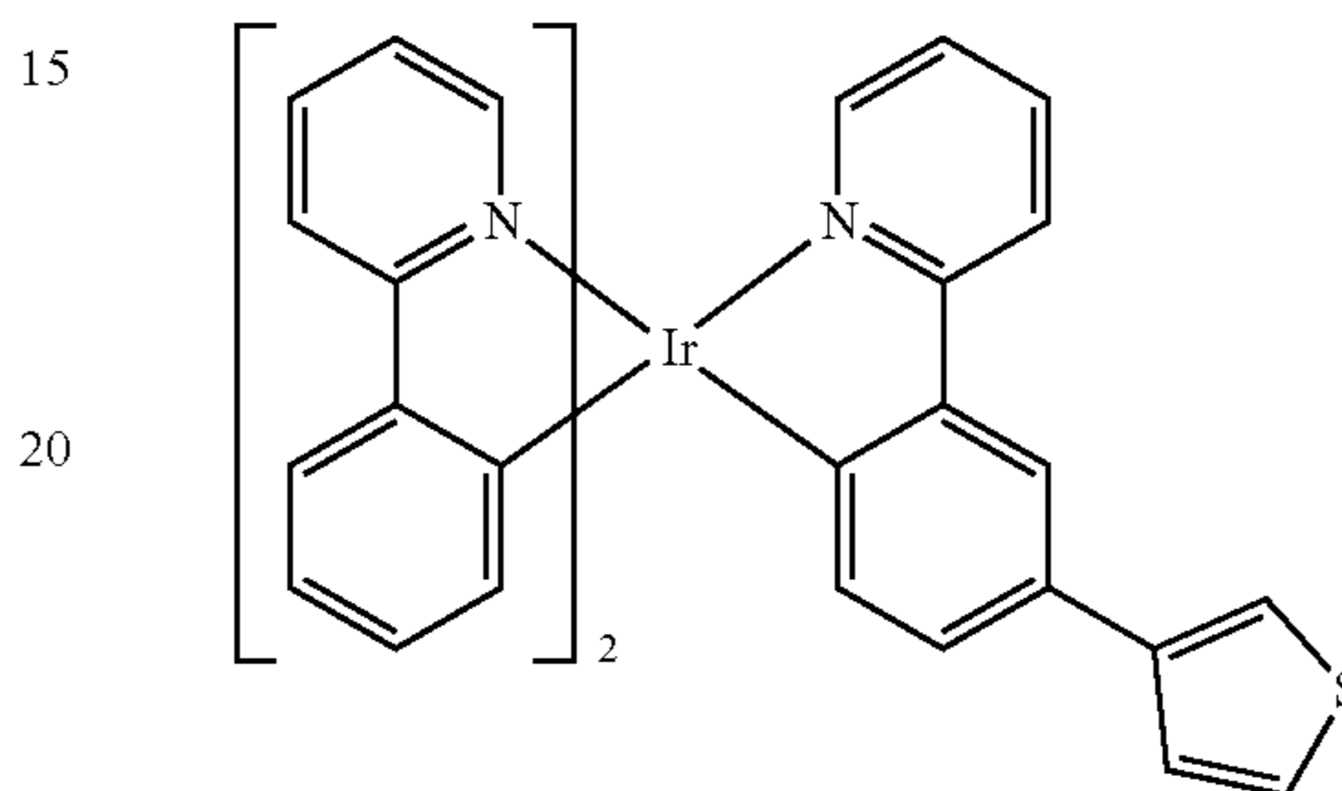
Compound 6
