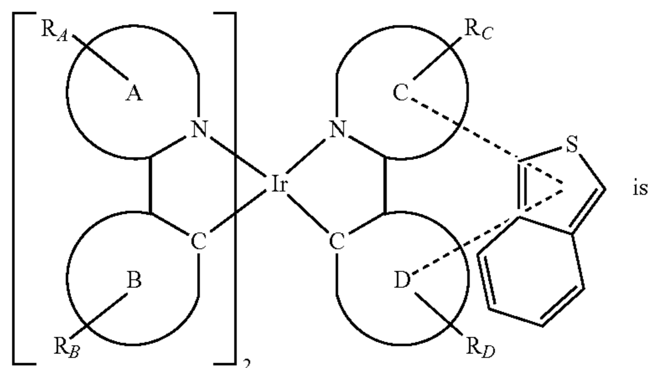
Compound 6
