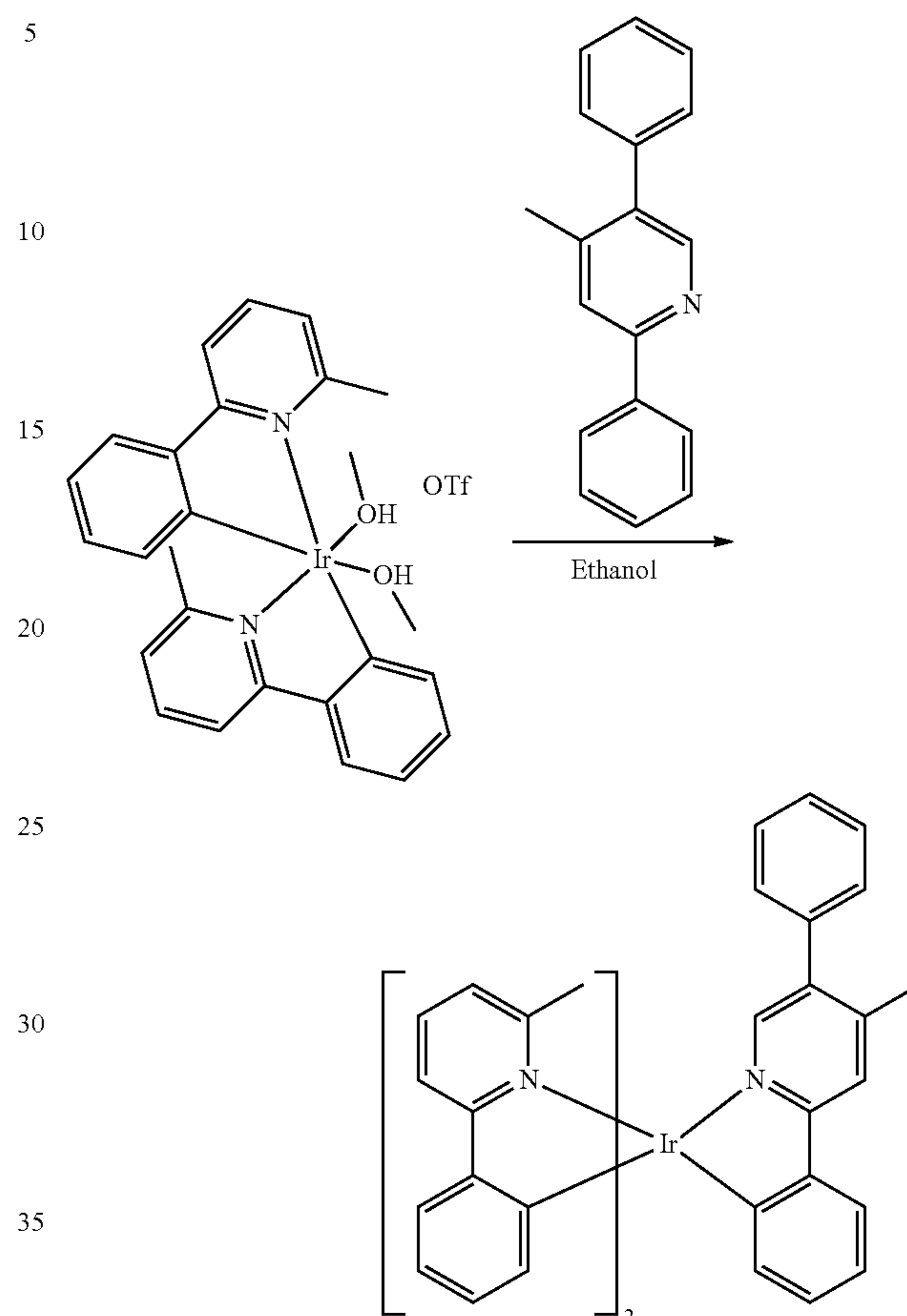
Compound 14
