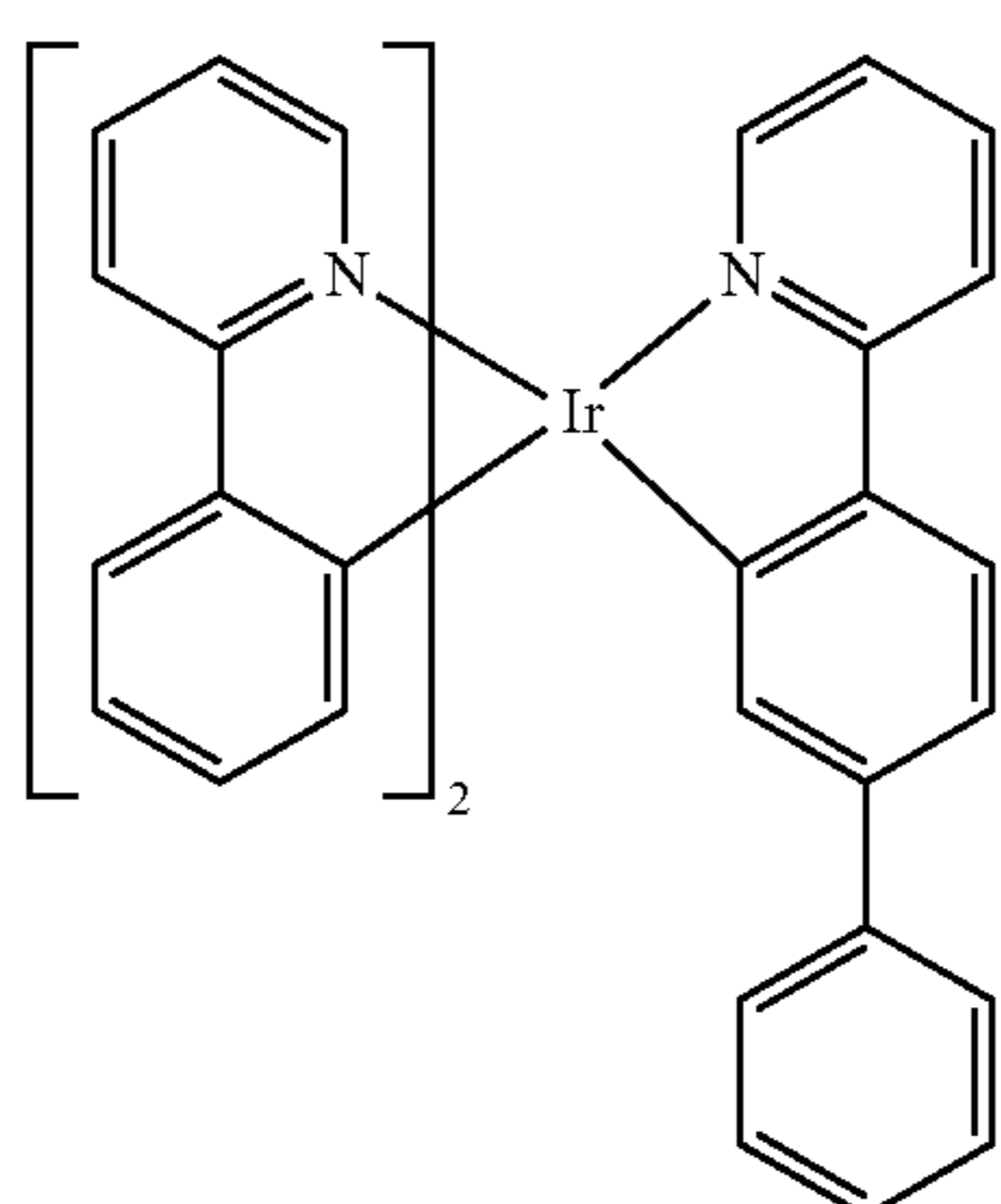
Compound 8
