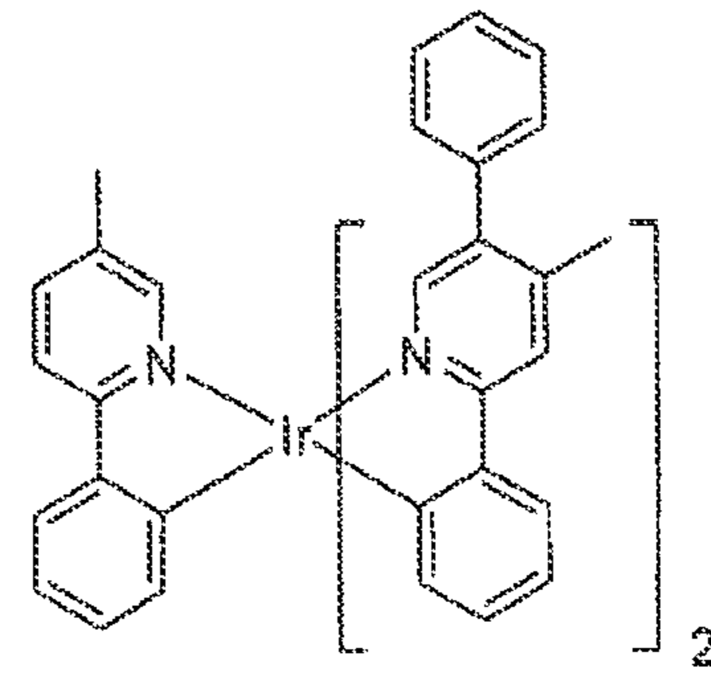
Compound 34
