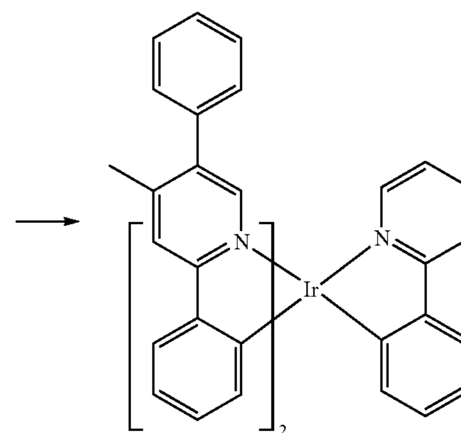
Compound 29
