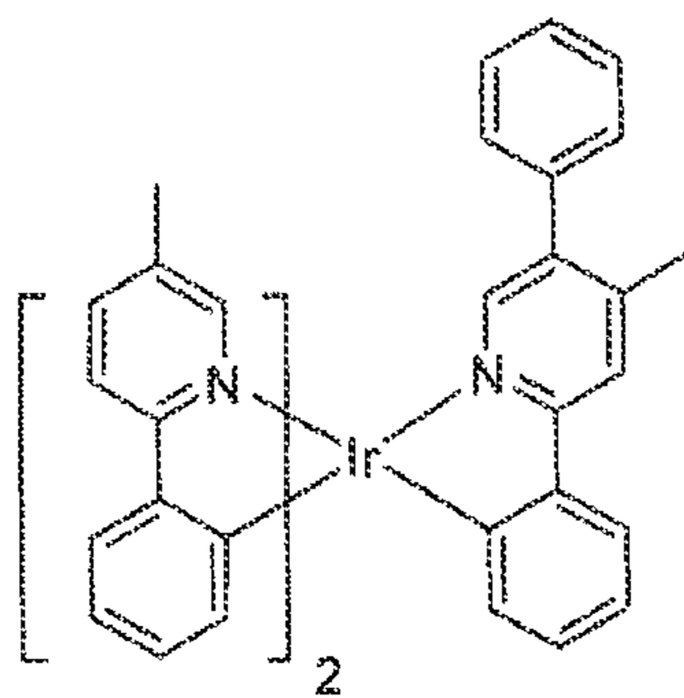
Compound 31
