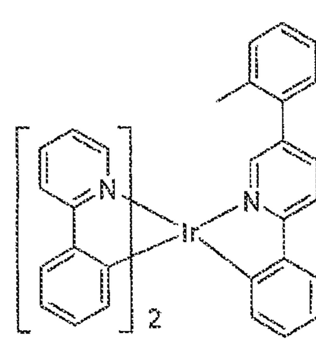
Compound 25
