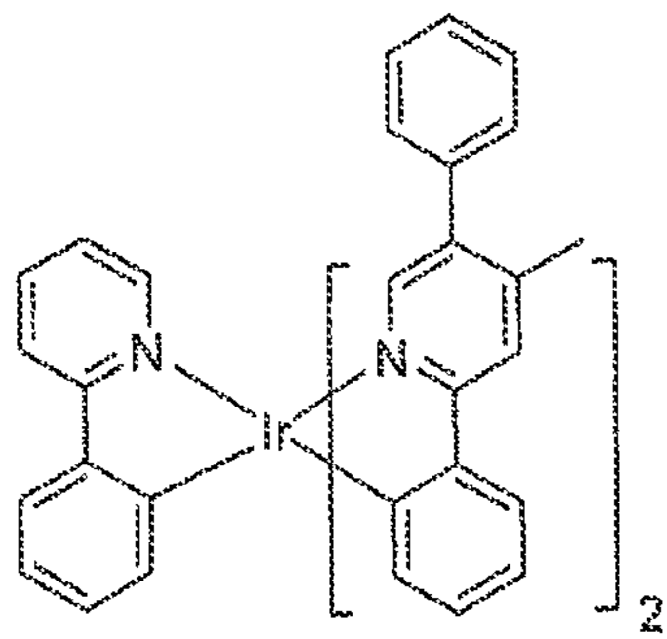
Compound 29
