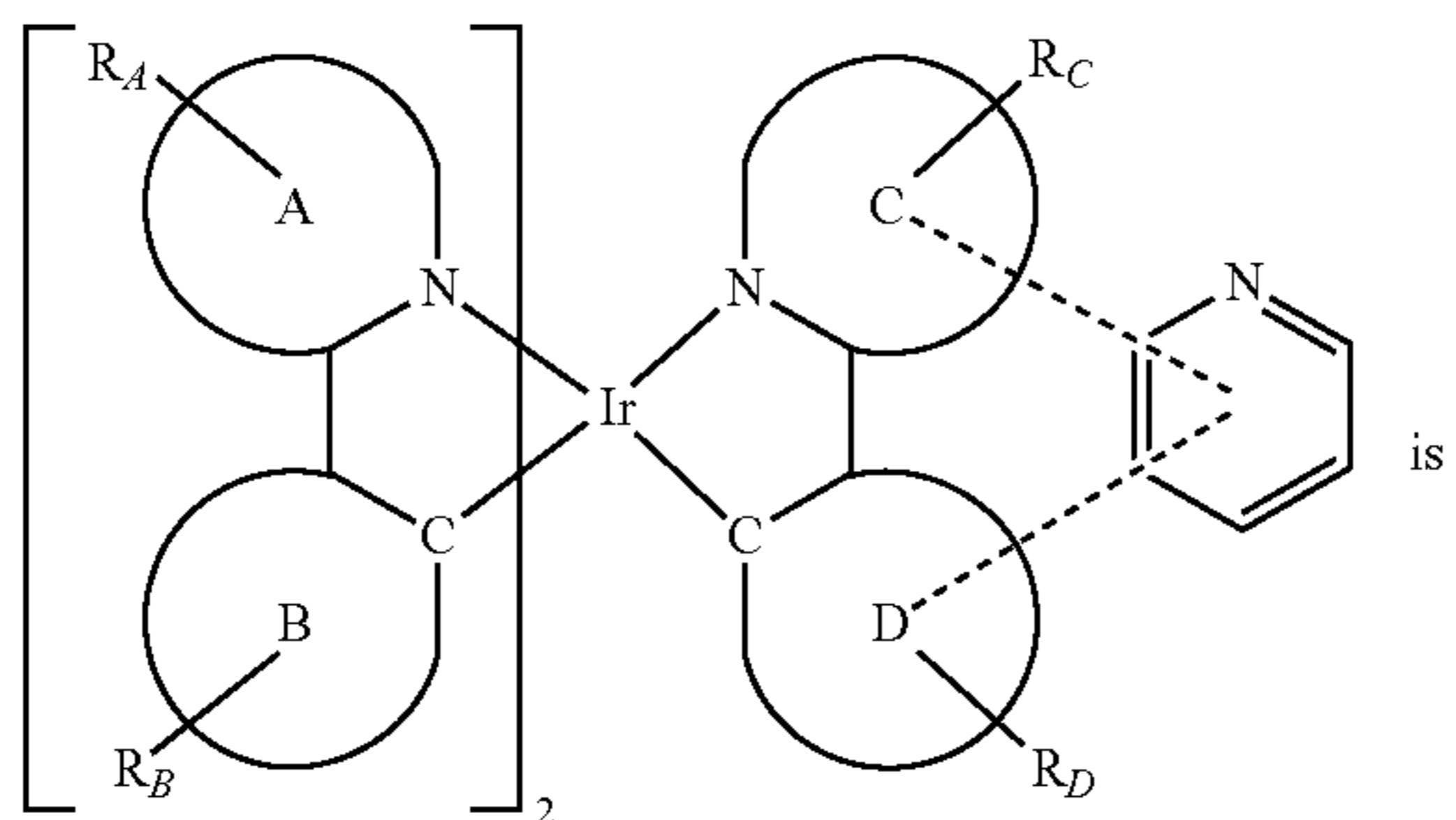
Compound 4
