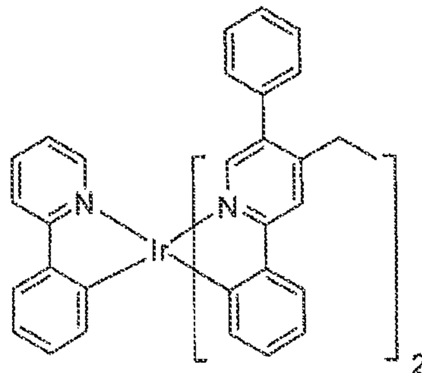
Compound 30
