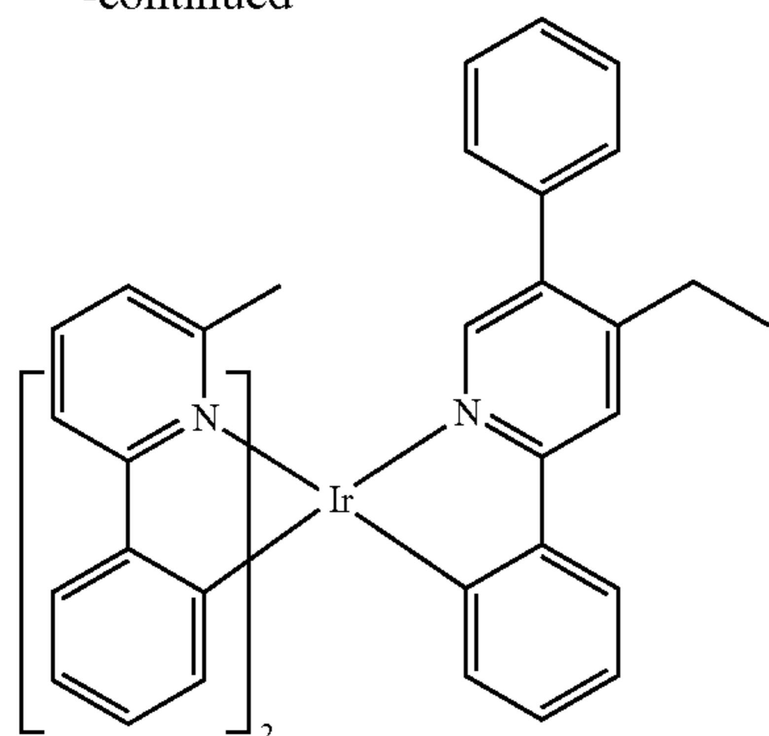
Compound 37
