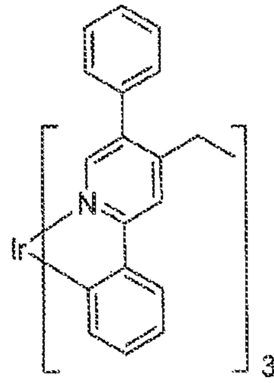
Compound 22
