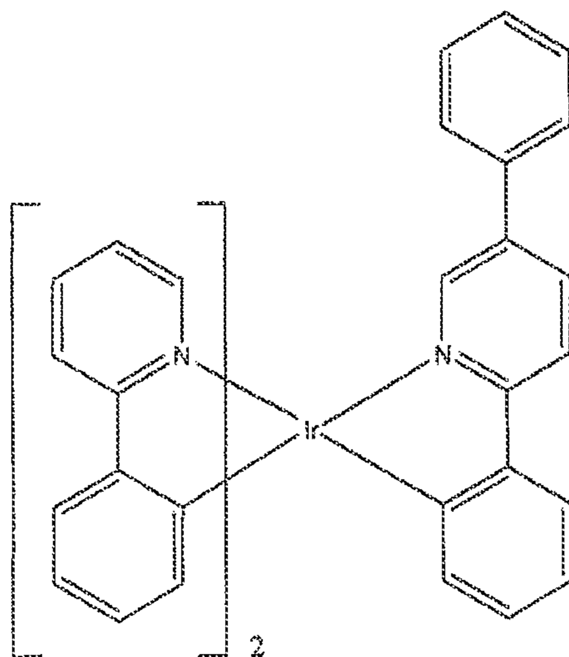
Compound 2
