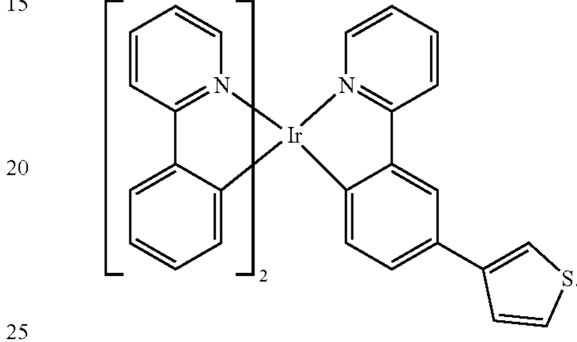
Compound 5
