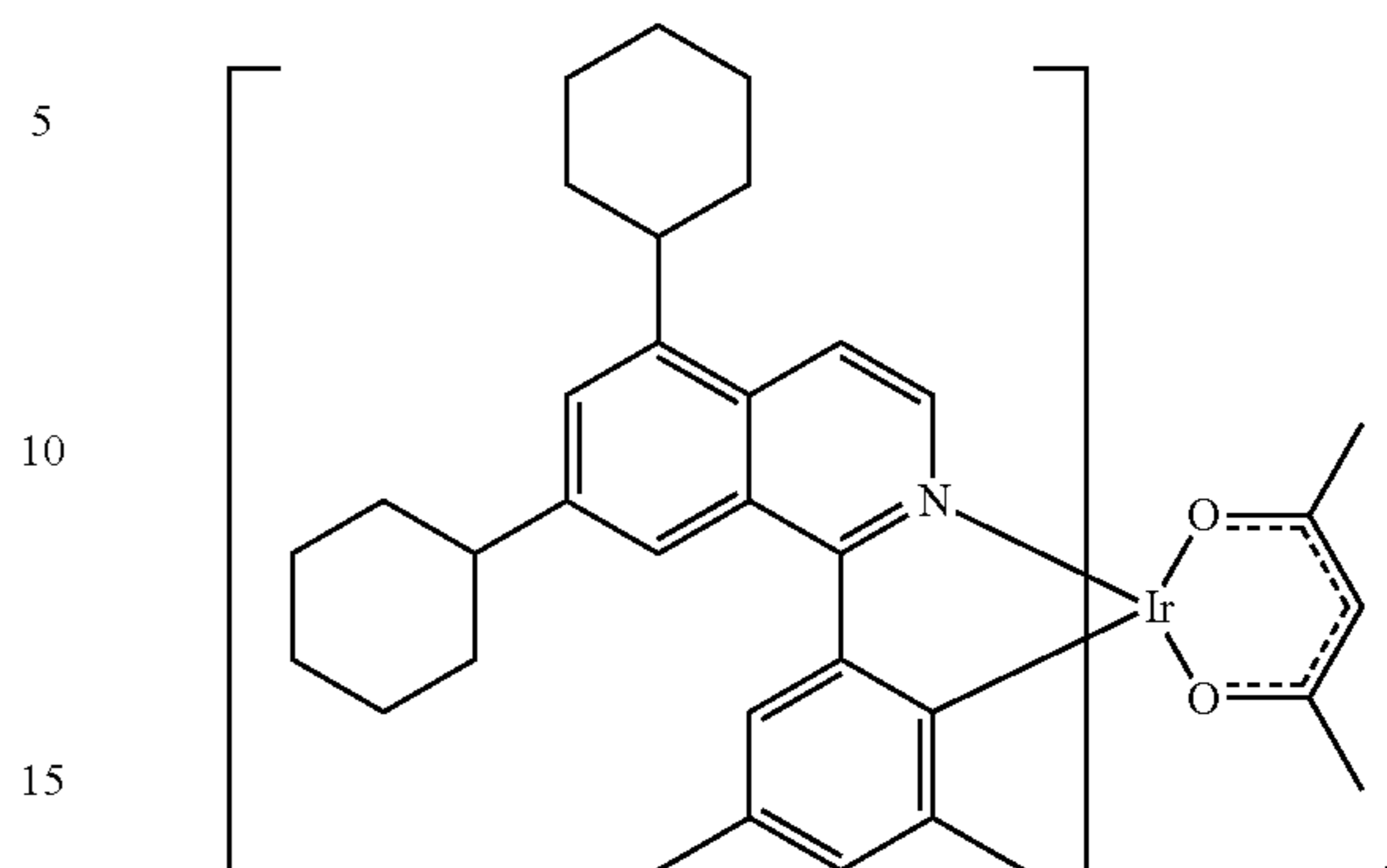
Compound 44
