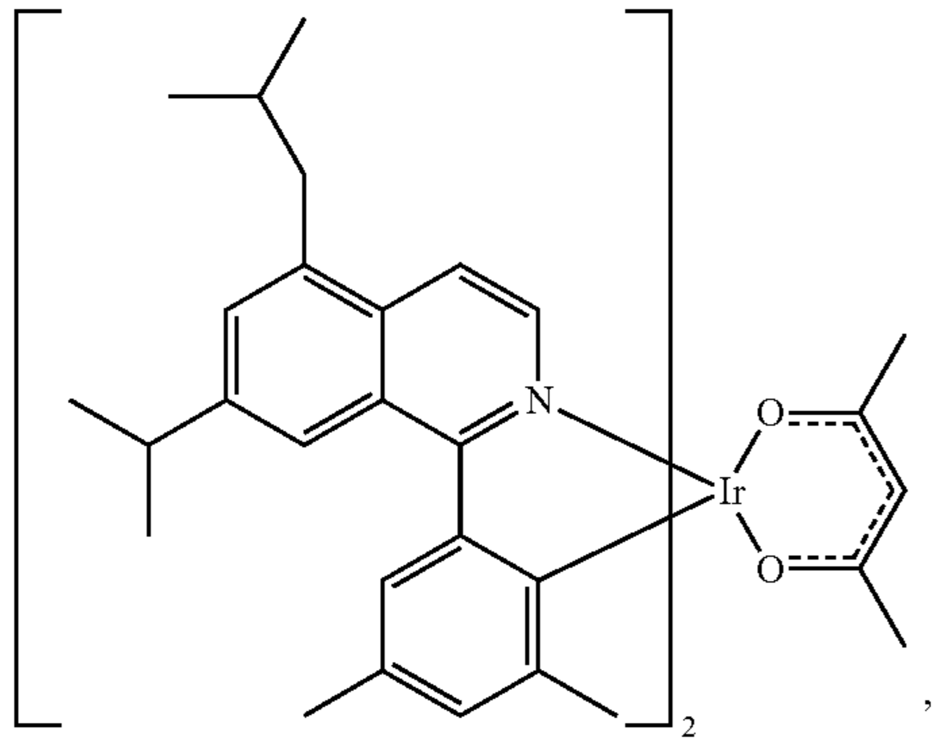
Compound 40
