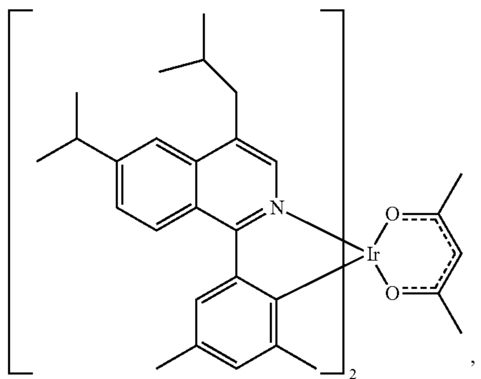
Compound 40
