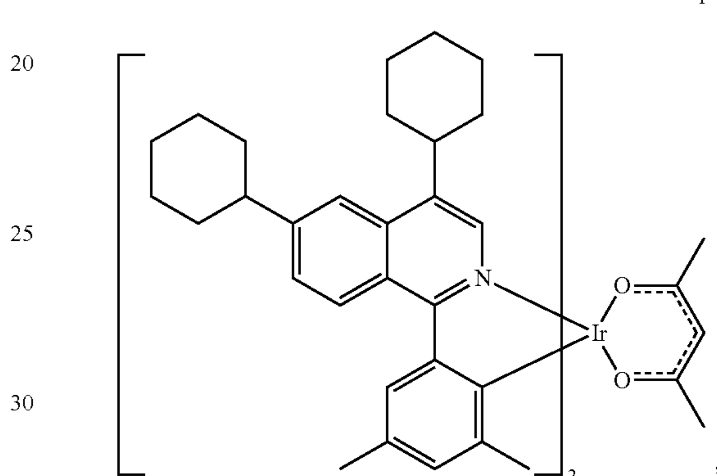
Compound 45
