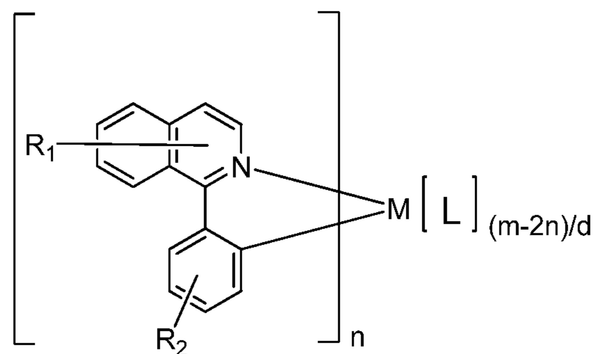
Formula I
