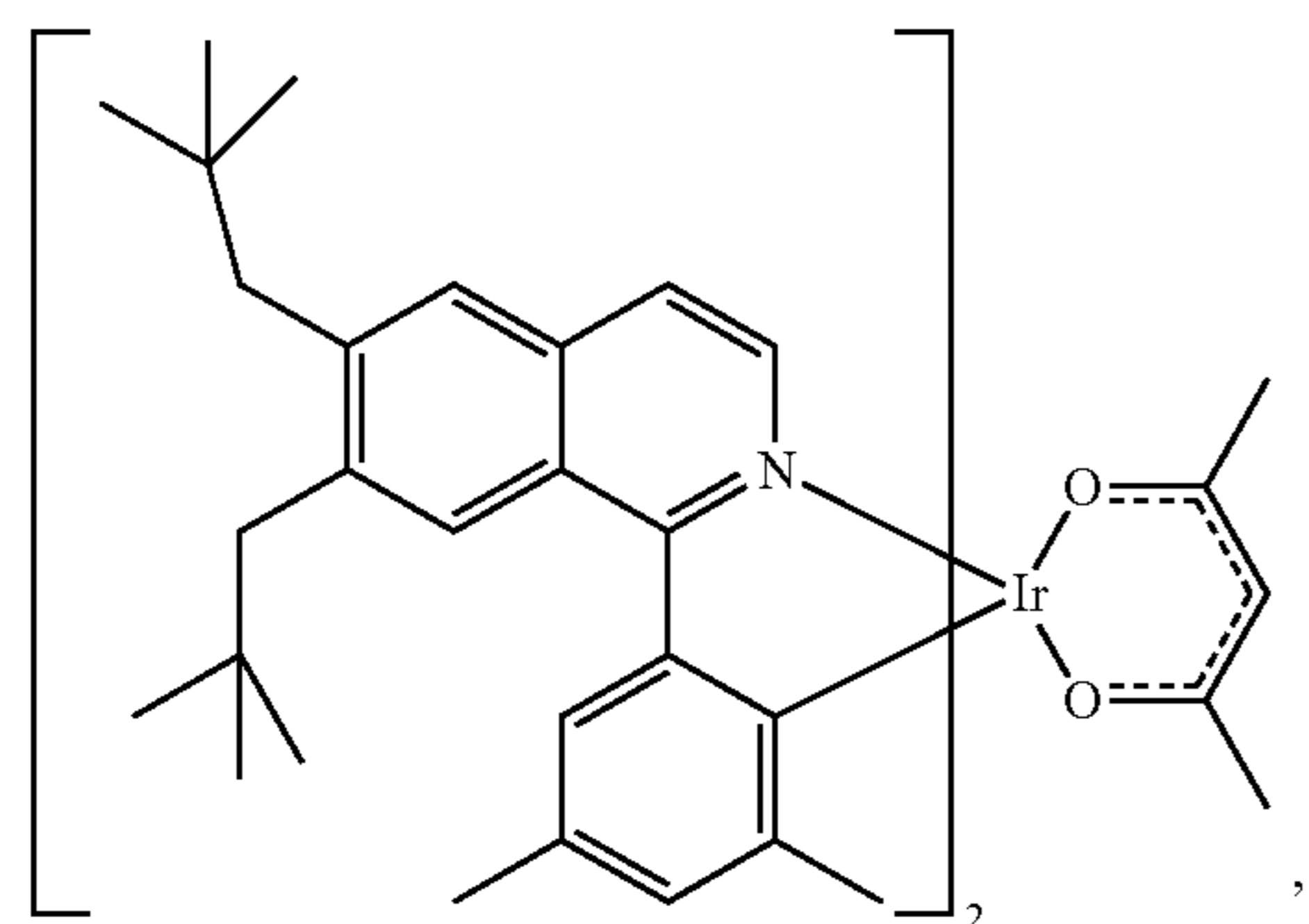
Compound 34
