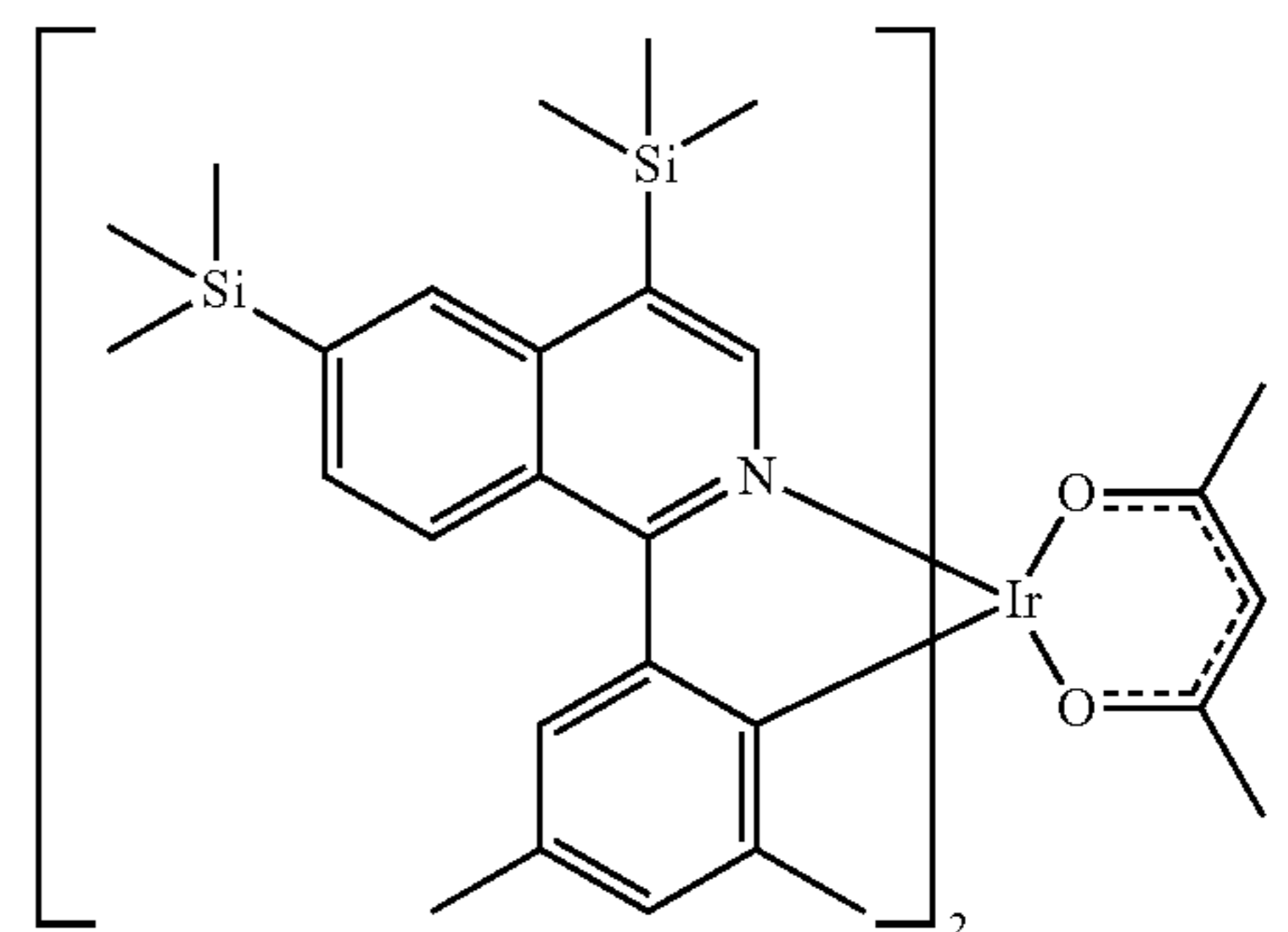
Compound 37
