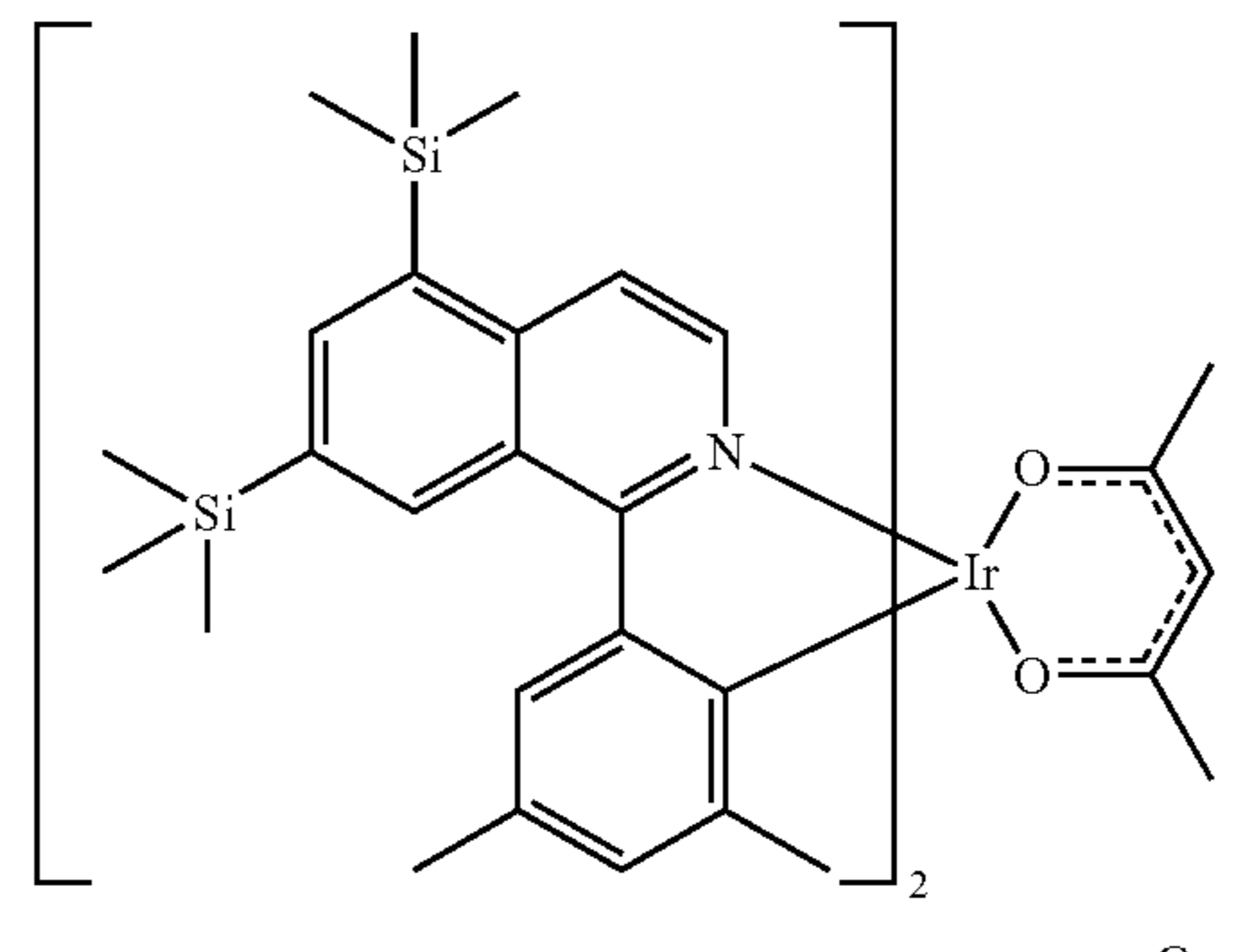
Compound 36
