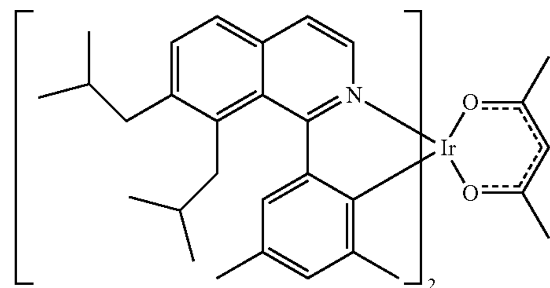
Compound 12
