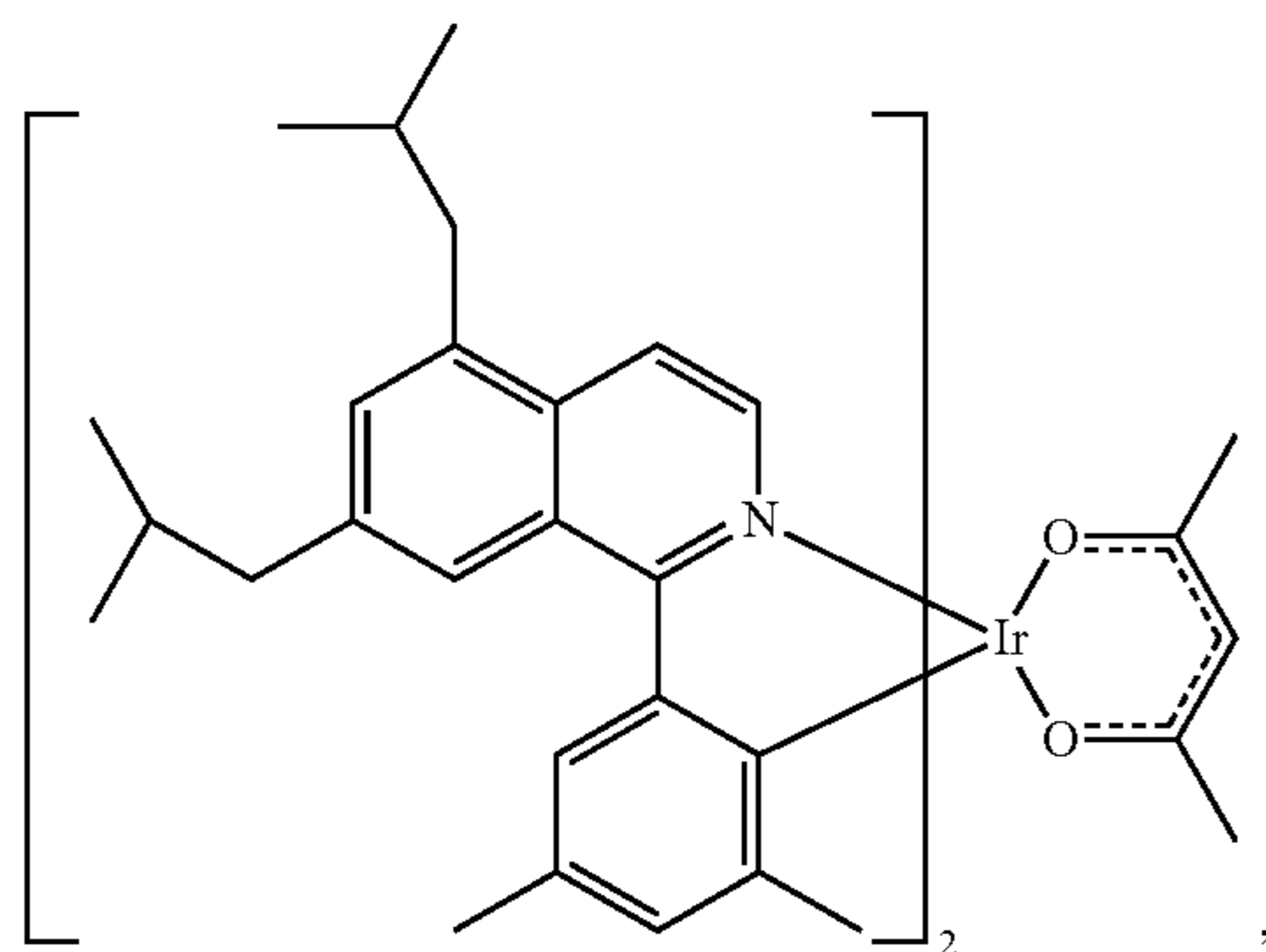
Compound 1
