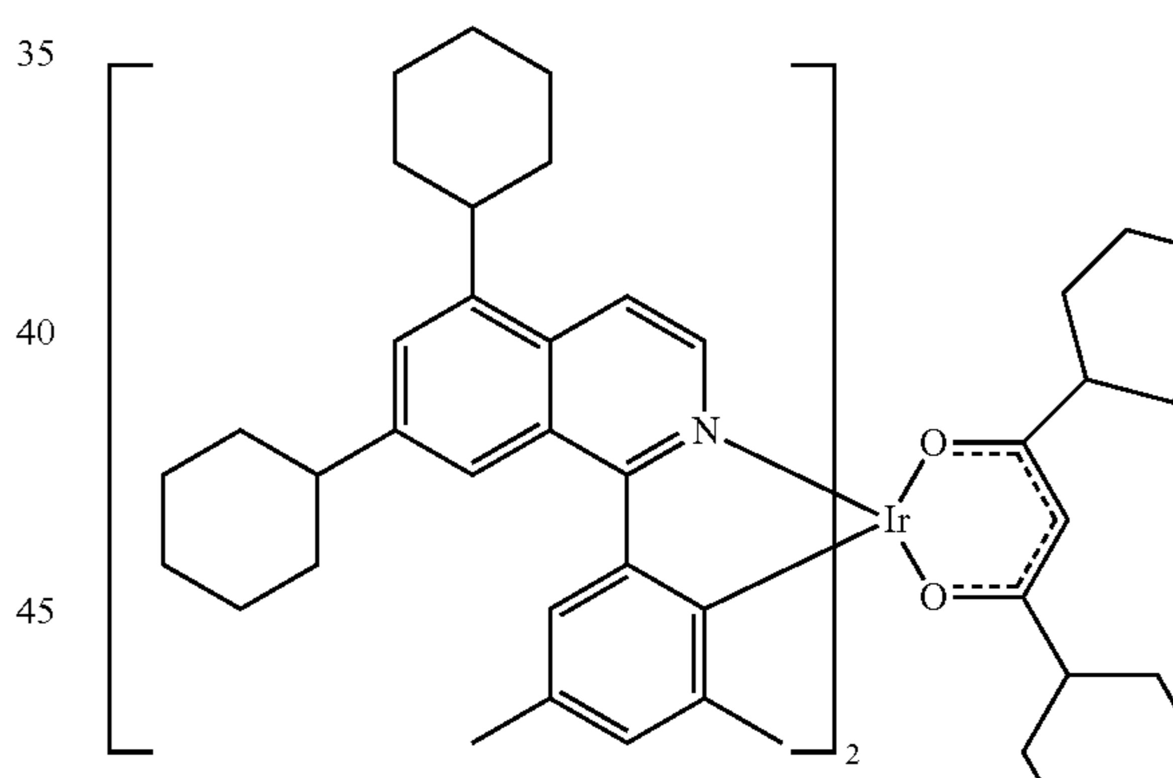
Compound 45
