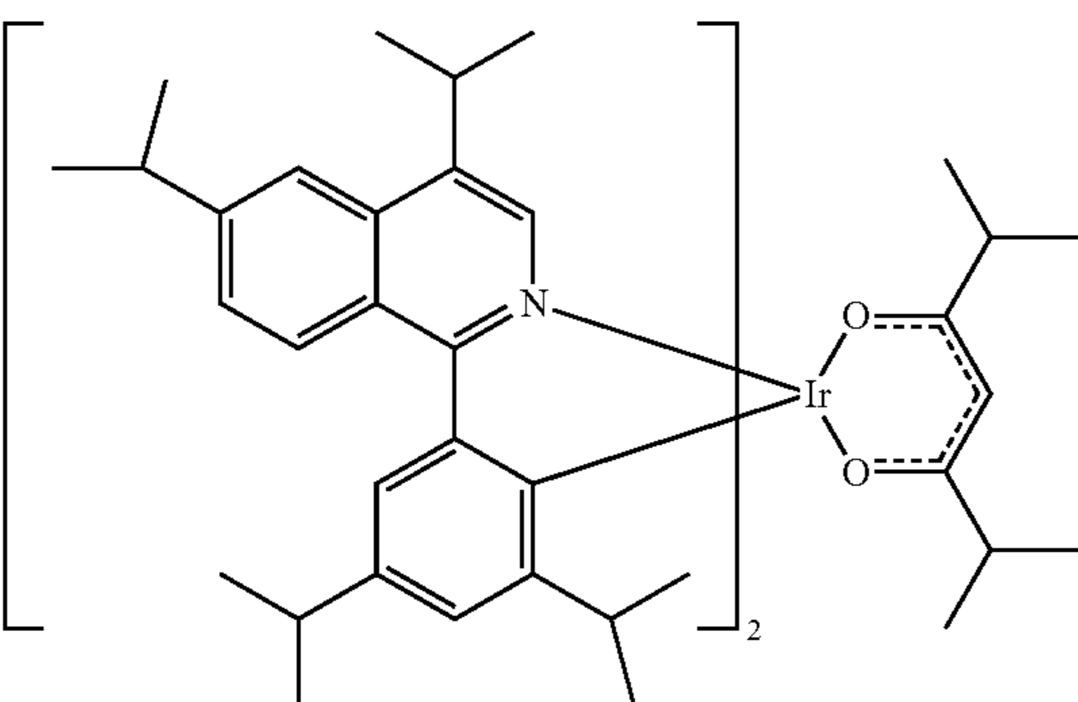
Compound 50
