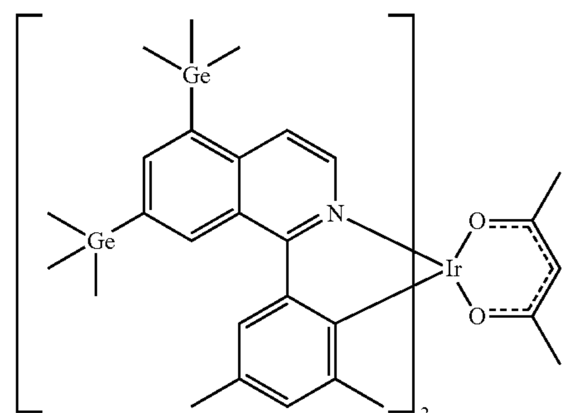
Compound 36
