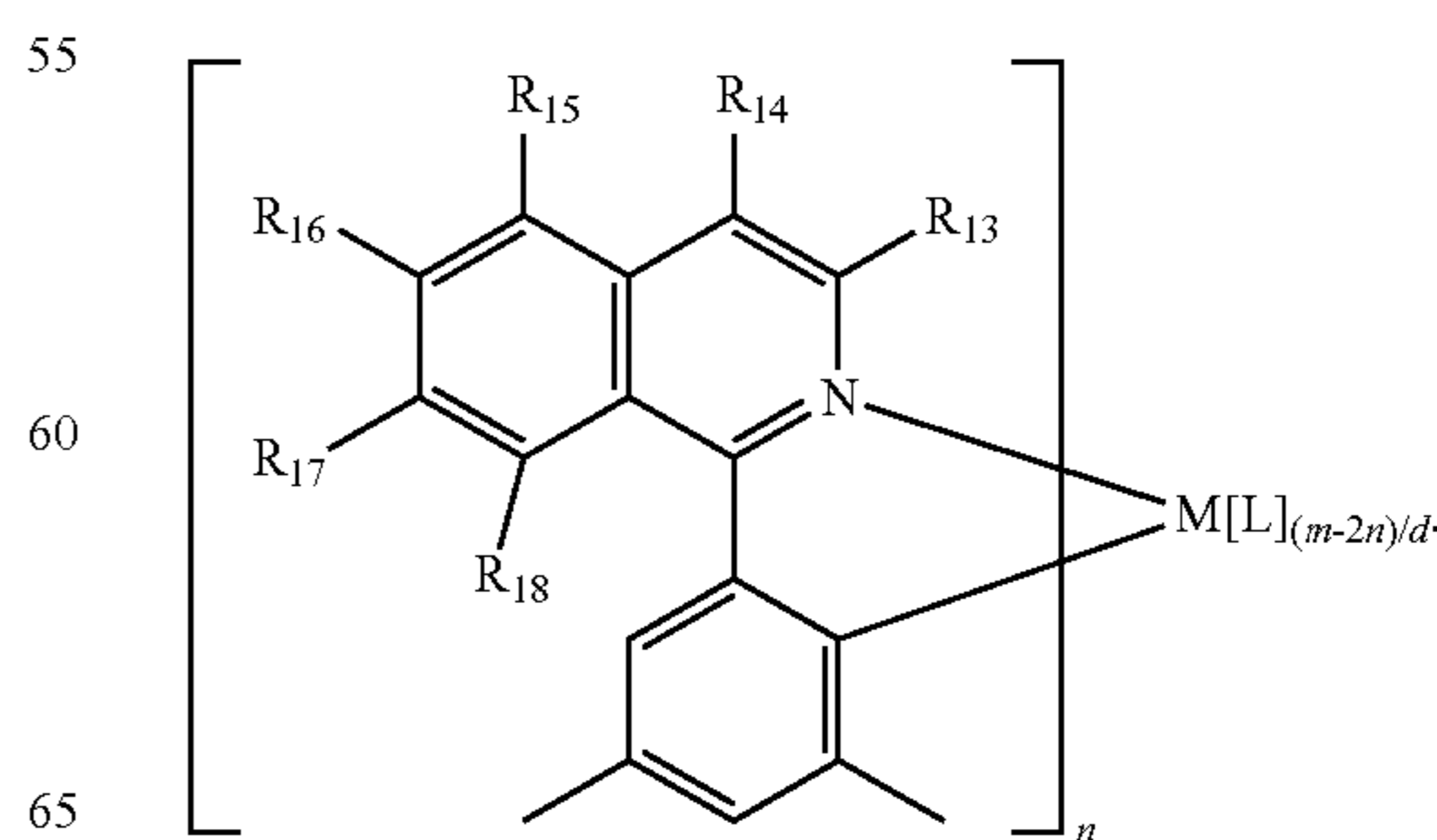
Formula III
