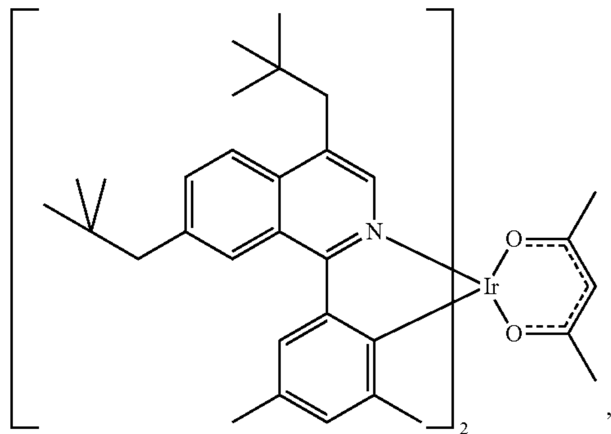
Compound 32
