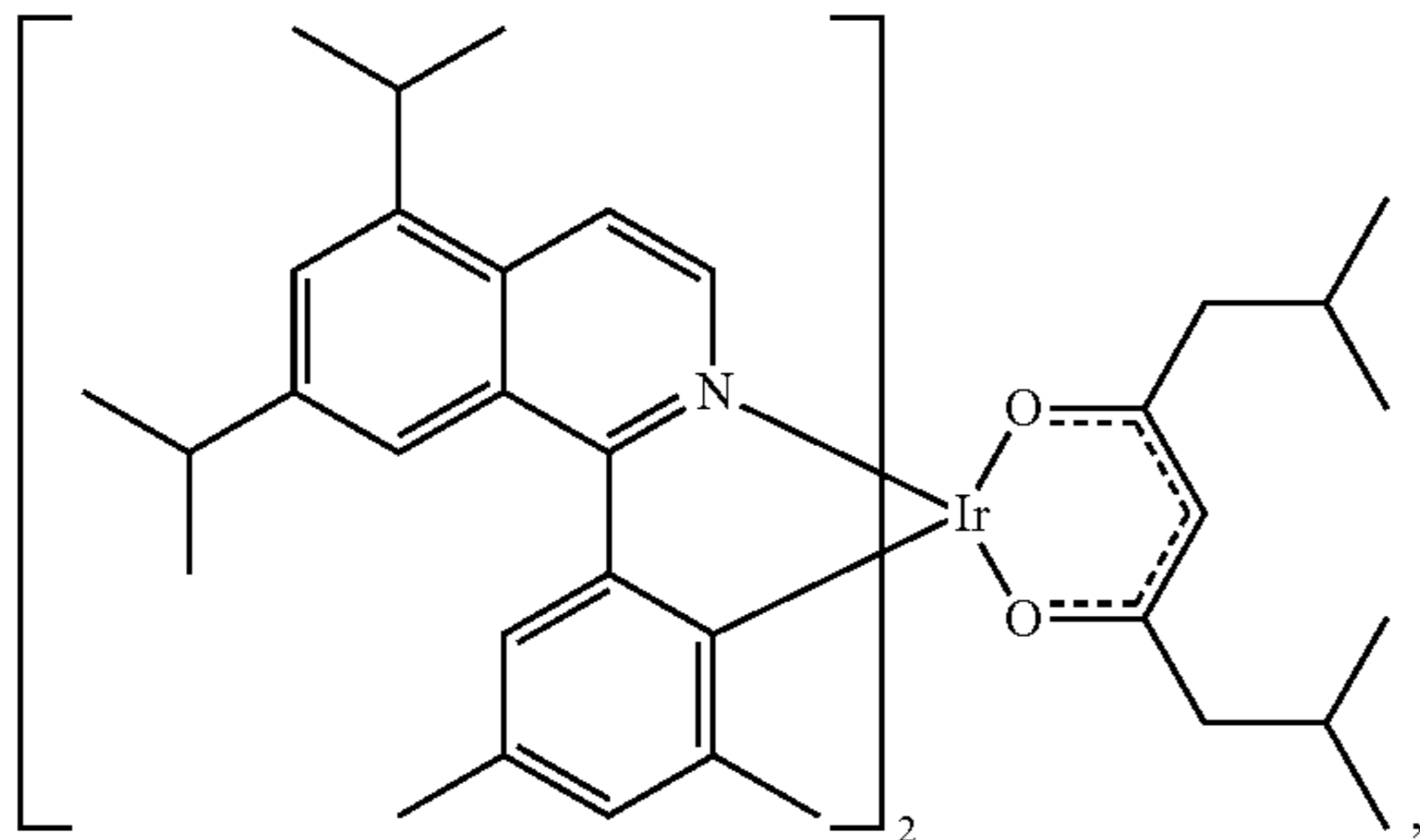
Compound 21
