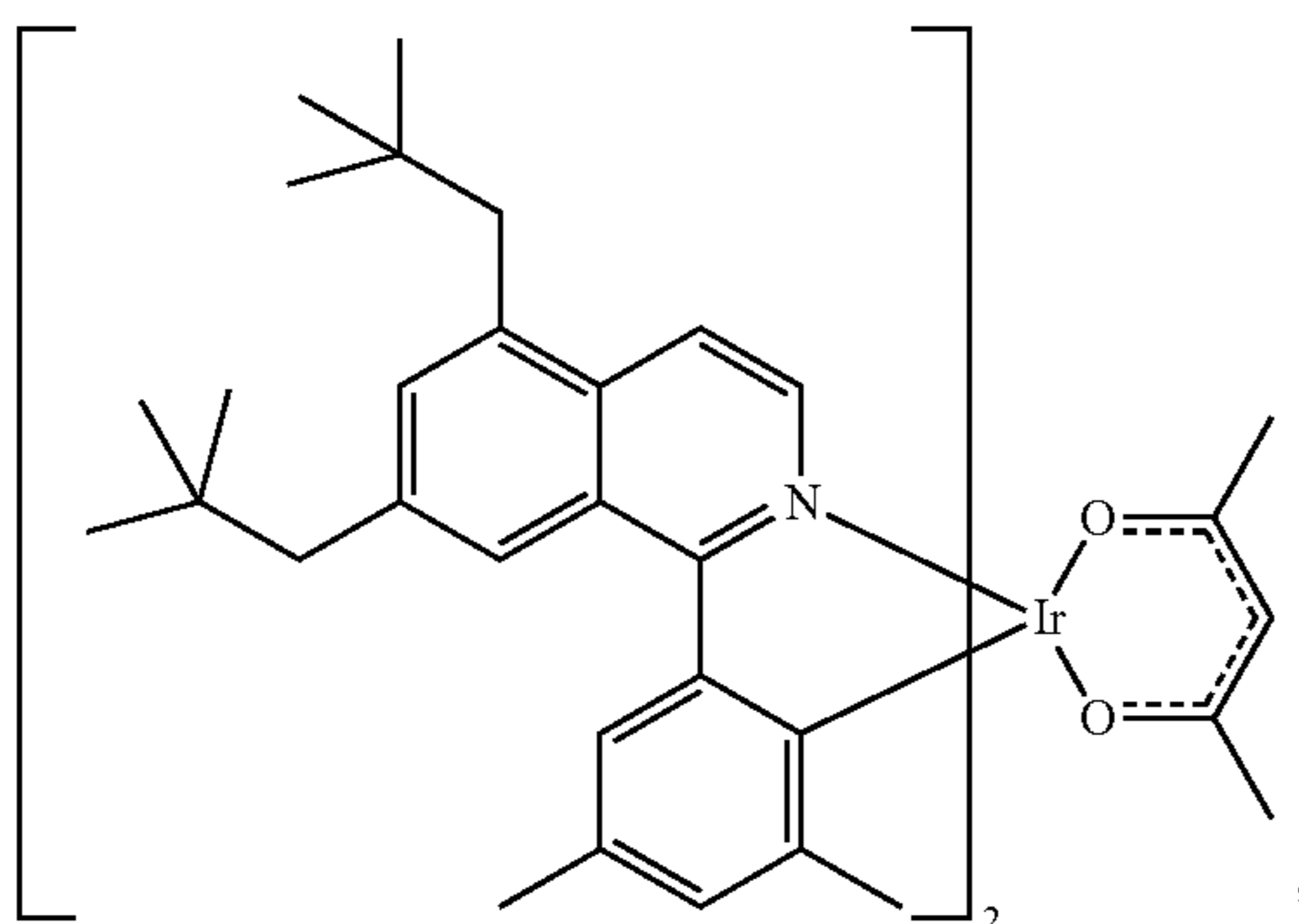
Compound 32
