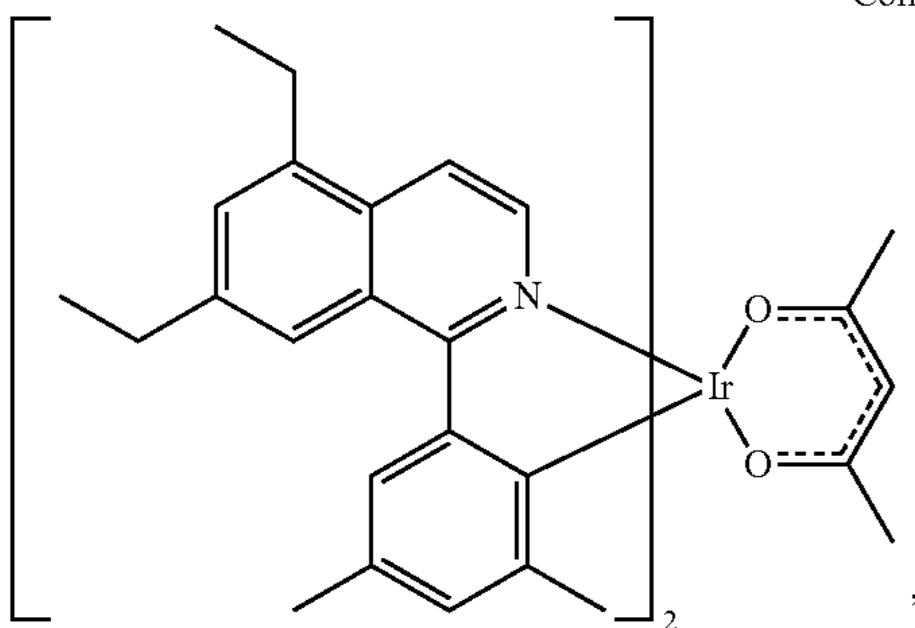
Compound 28
