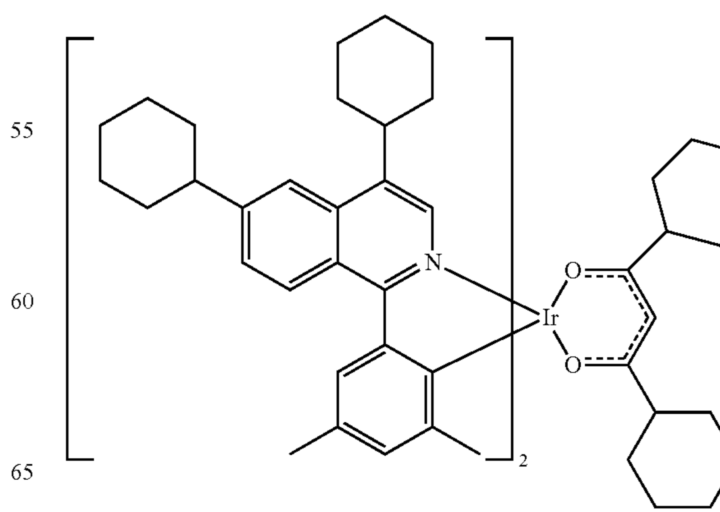
Compound 46
