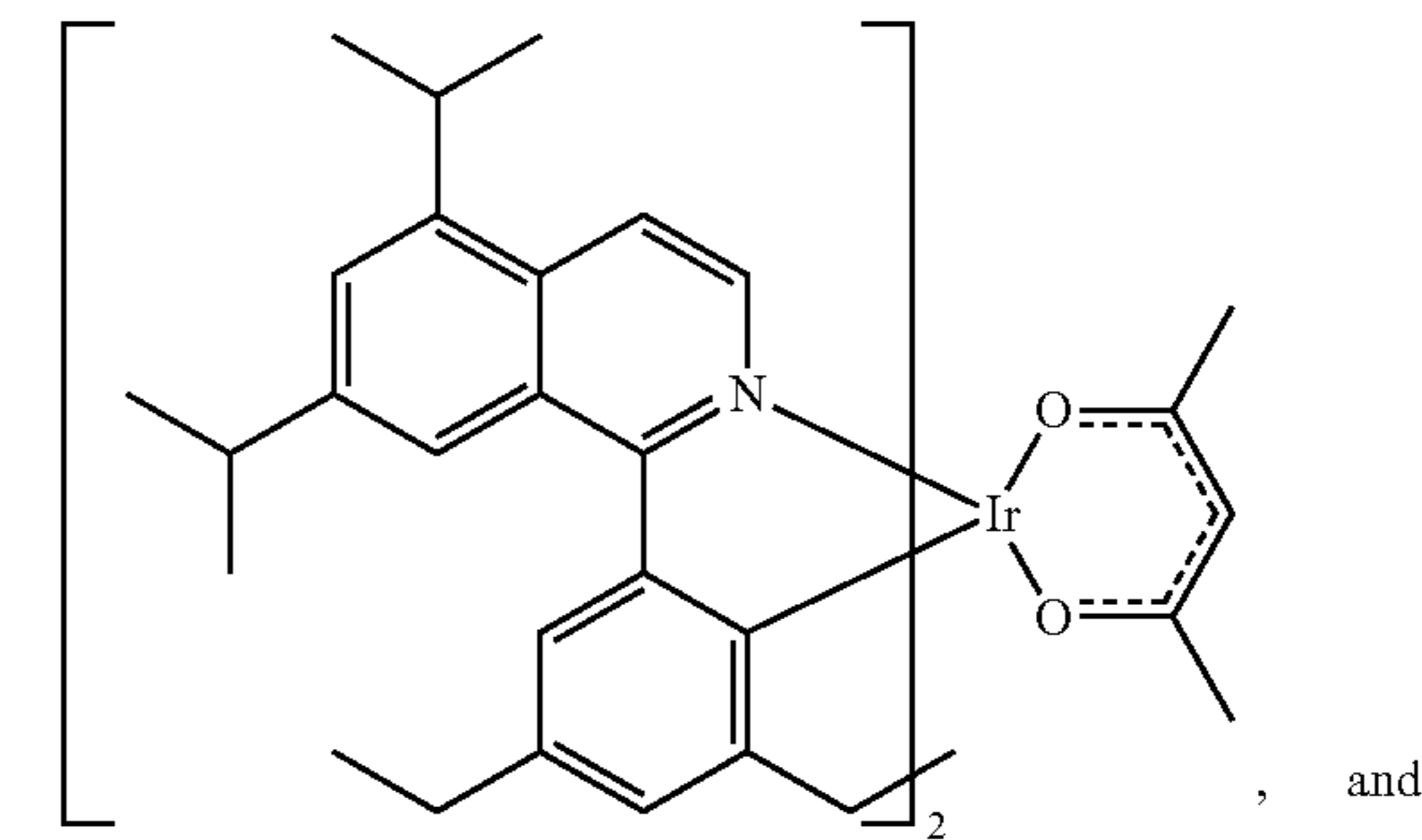
Compound 48
