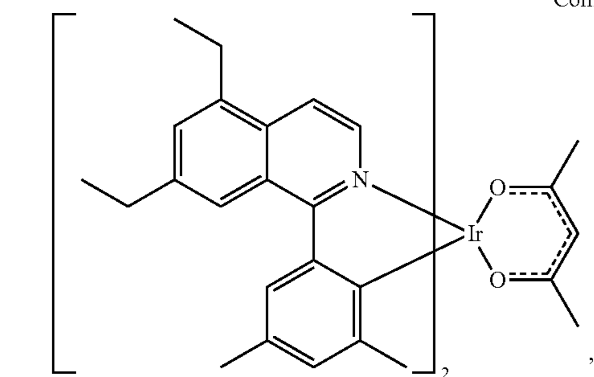
Compound 28
