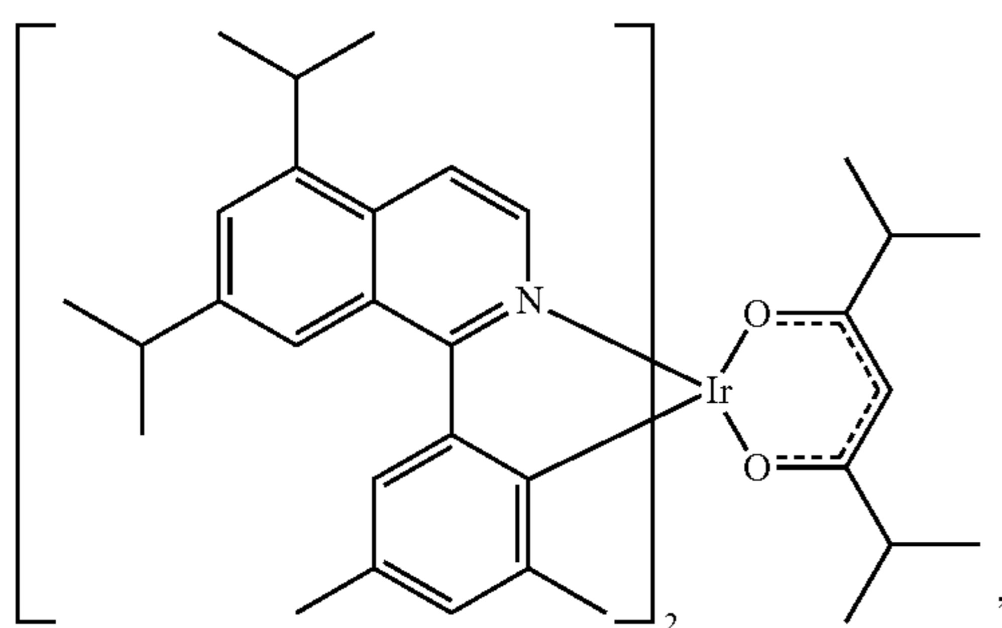
Compound 28
