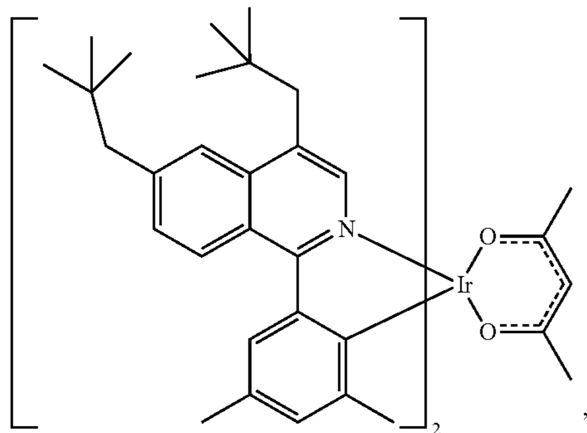
Compound 33
