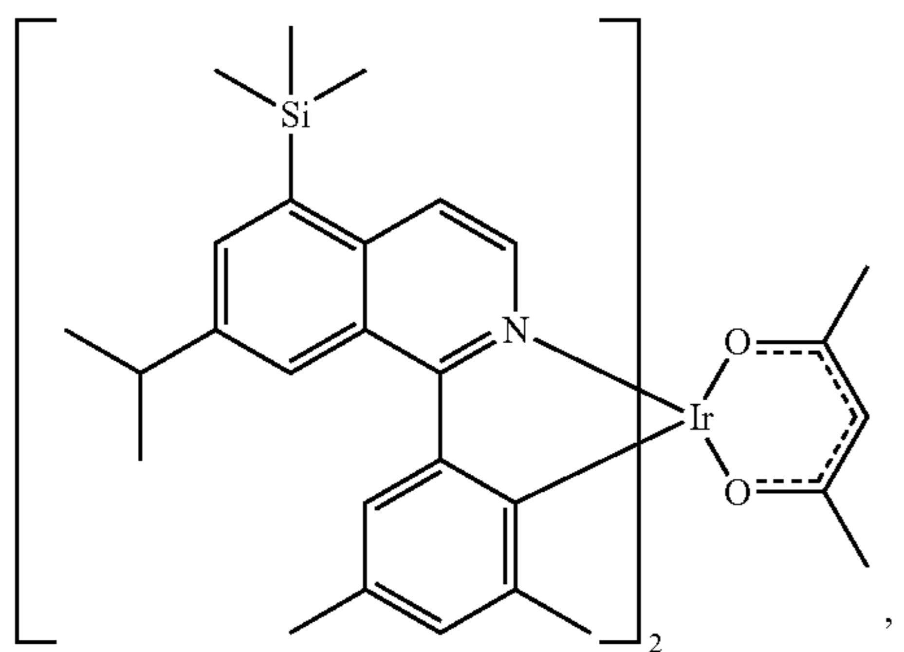
Compound 41
