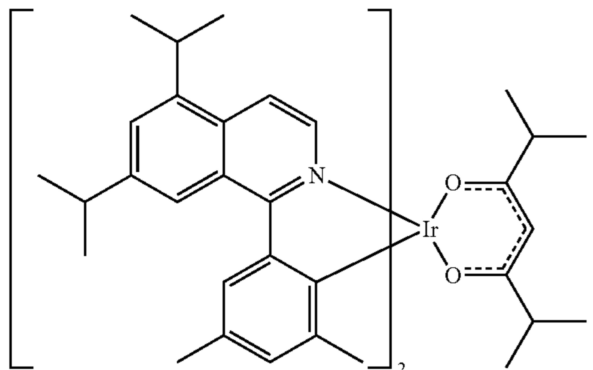
Compound 28
