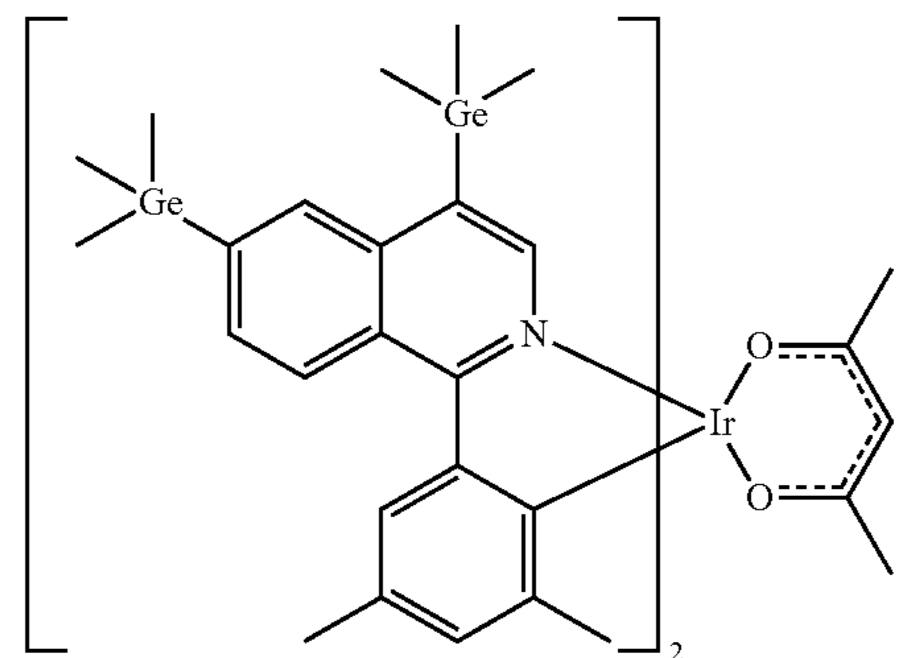
Compound 38
