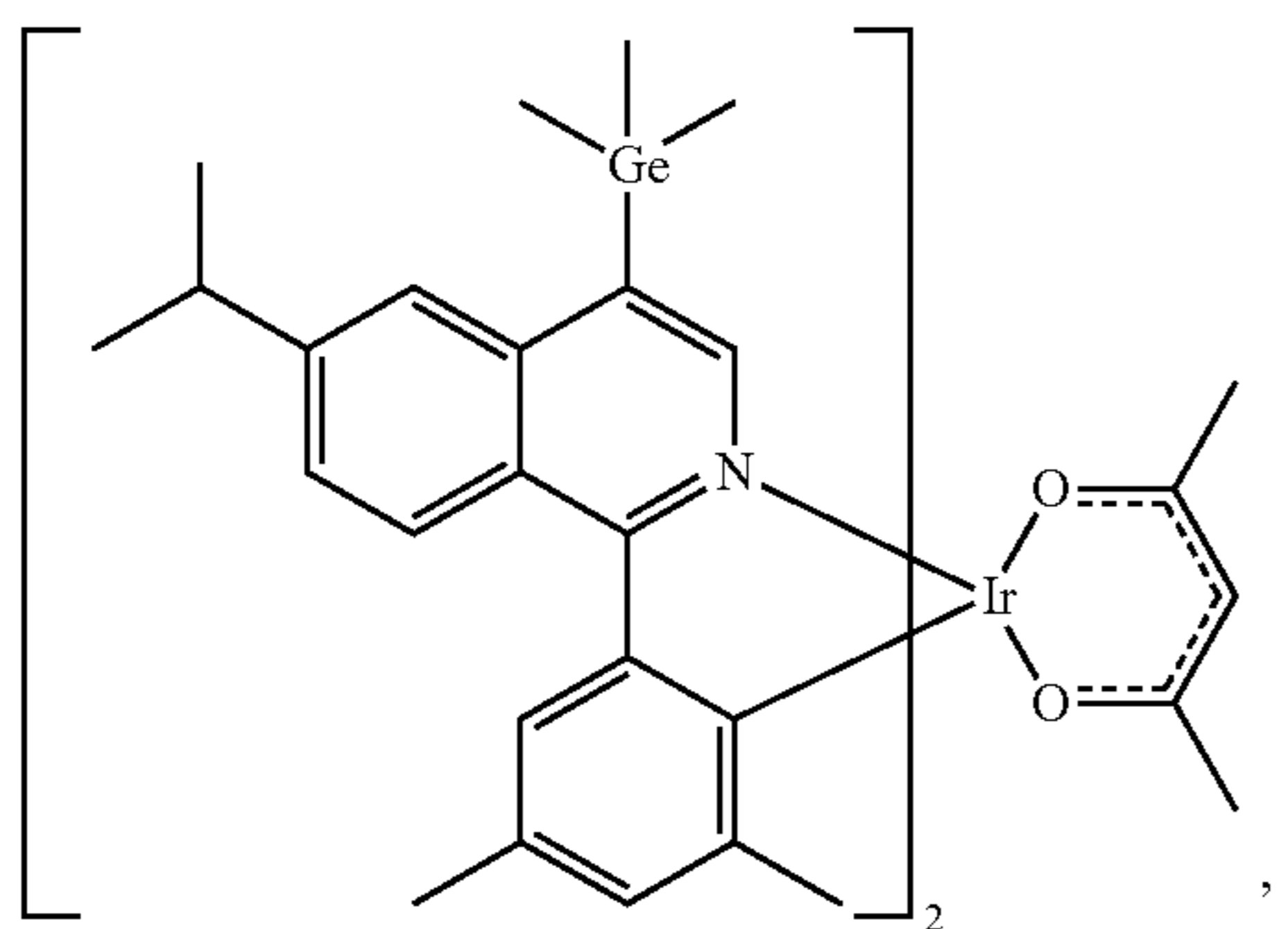
Compound 42
