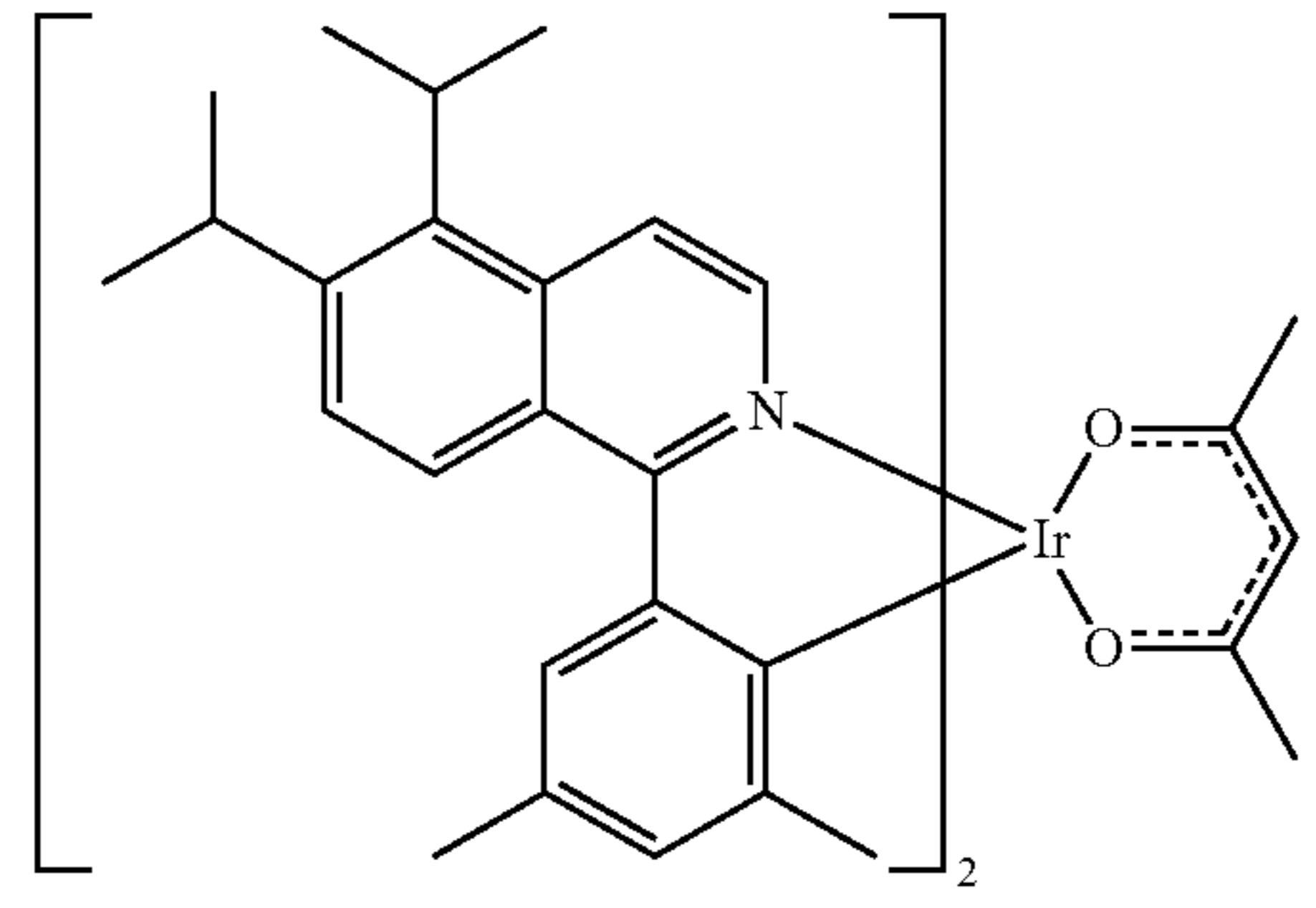
Compound 10
