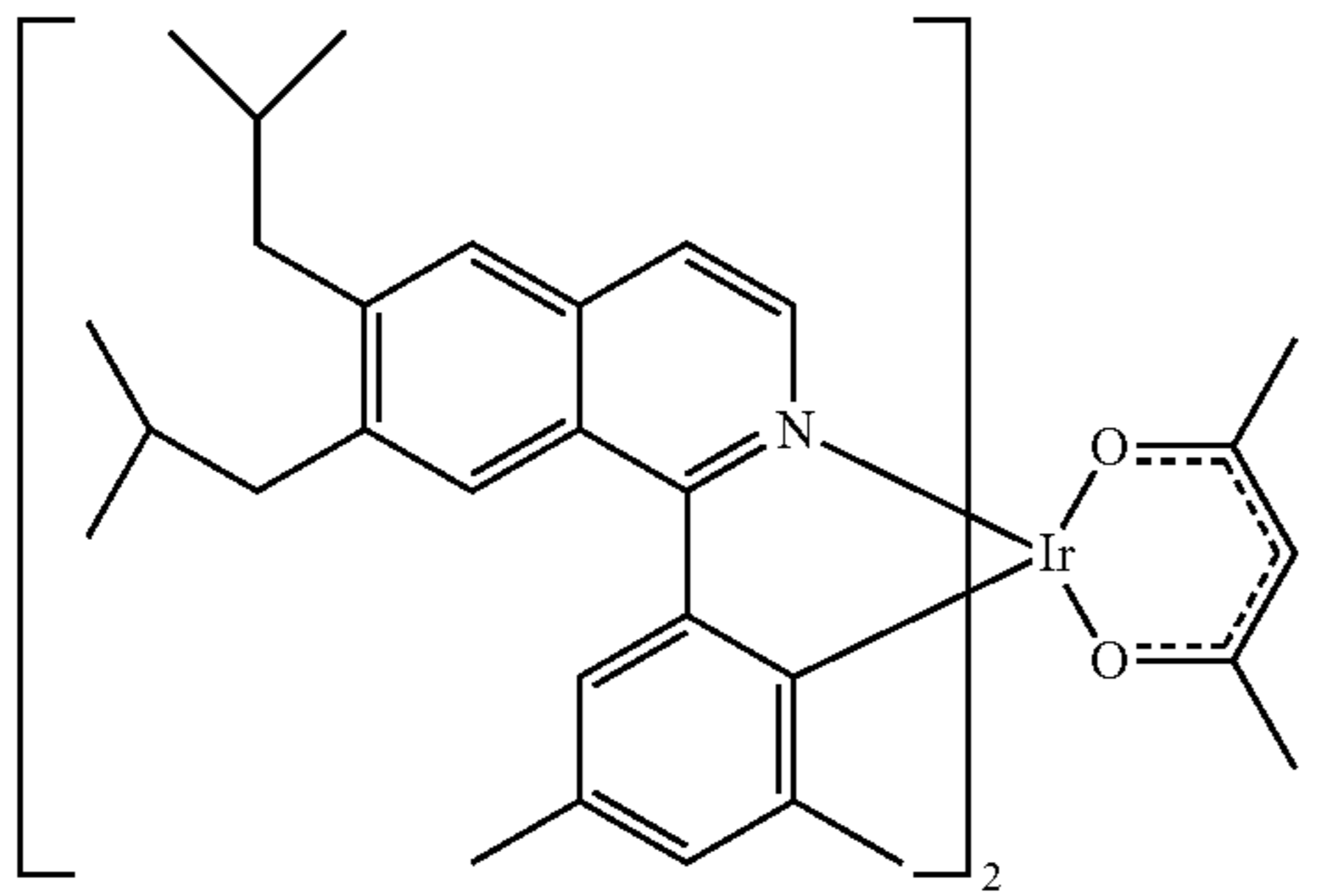
Compound 7
