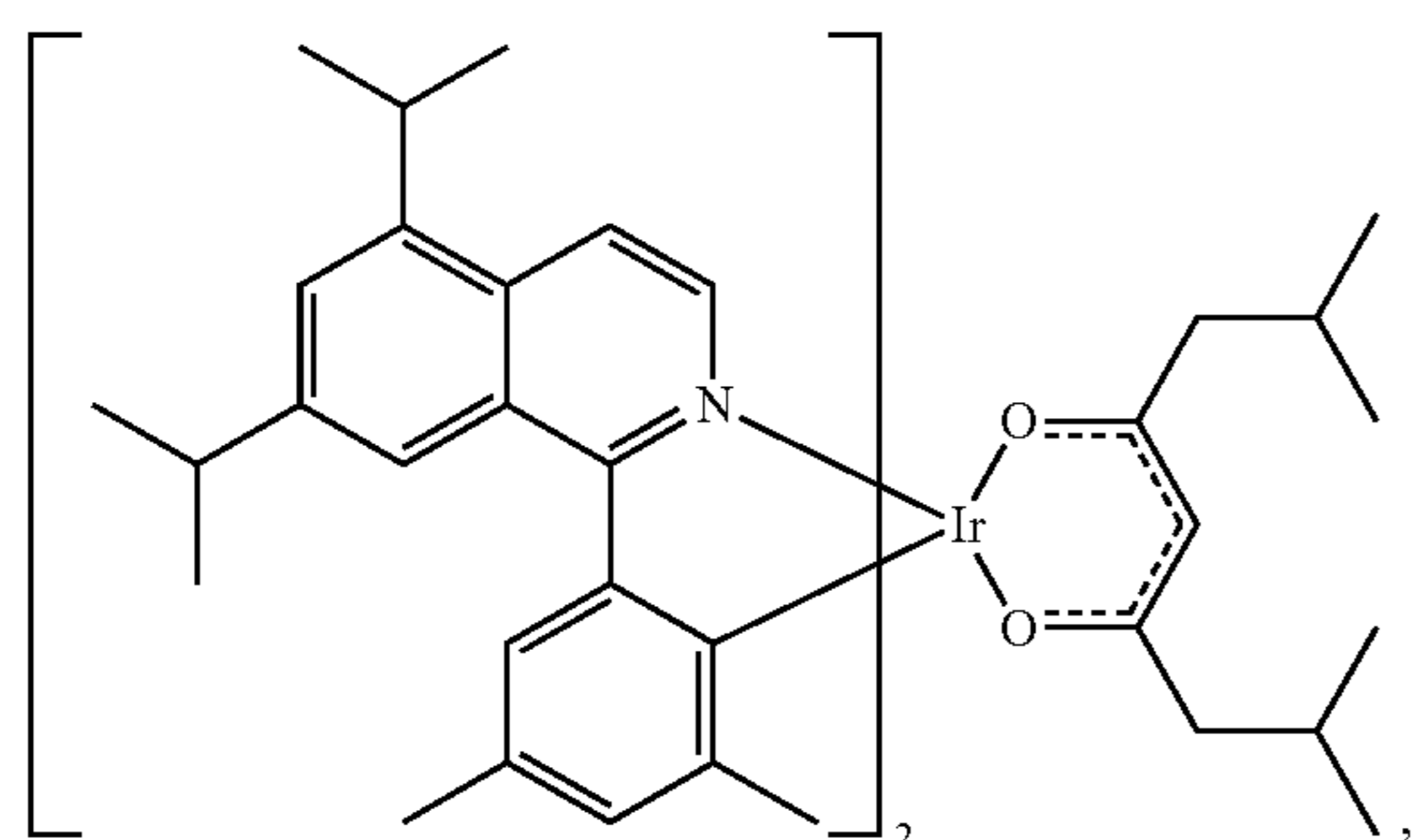
Compound 21
