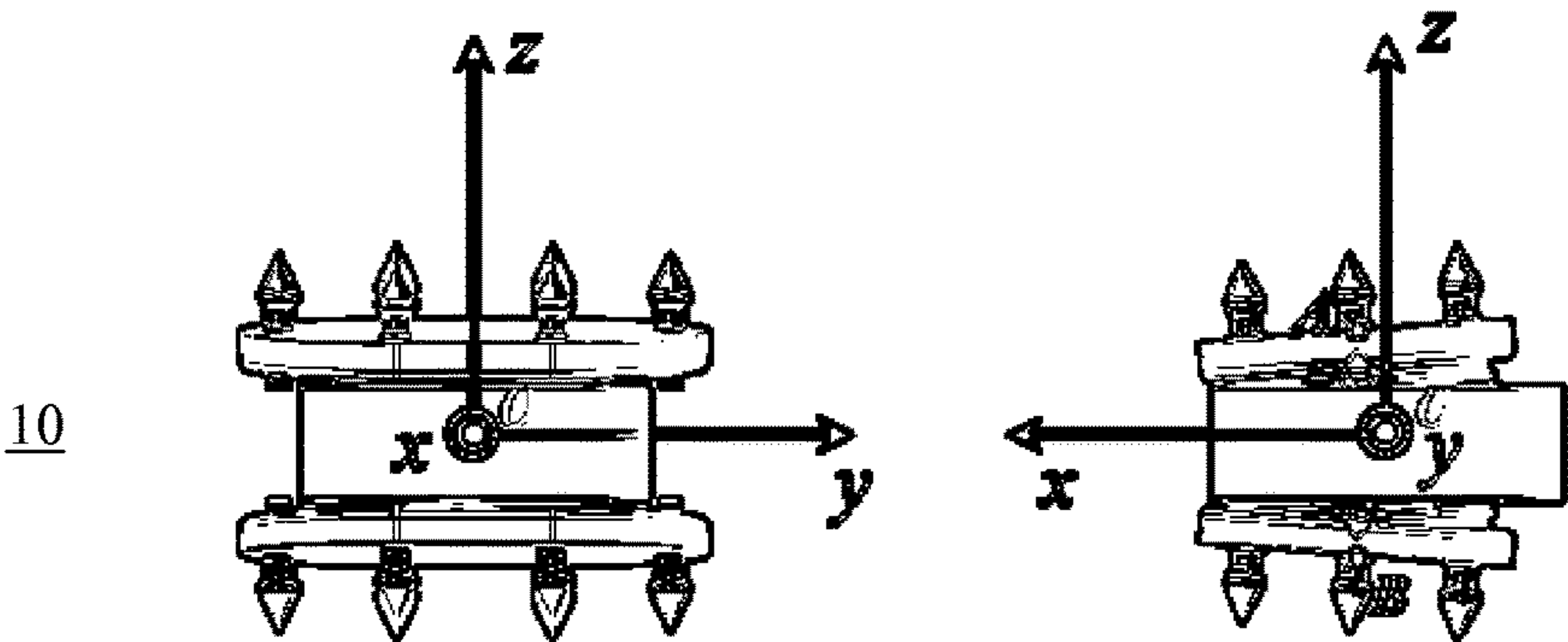
Figure 4Ci: Front View
