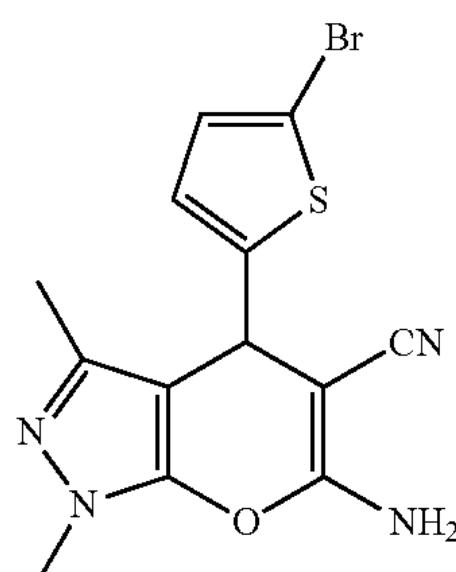
Chemical Formula: C 13 H 11 BrN 4 OS Molecular Weight: 351.22
