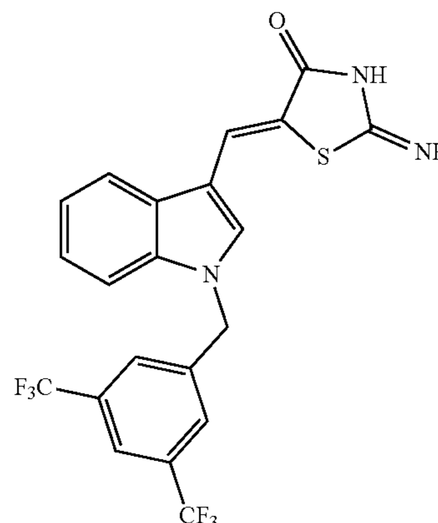
(Z)-5-((1-(3,5-Bis(trifluoromethyl)benzyl)-1H-indol-3-yl)methylene)-2-iminothiazolidin-4-one (JXL067)
