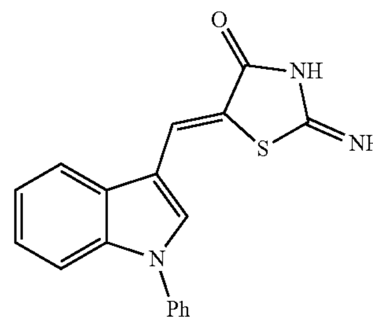
(Z)-2-Imino-5-((1-phenyl-1H-indol-3-yl)methylene)thiazolidin-4-one (JXL023)
