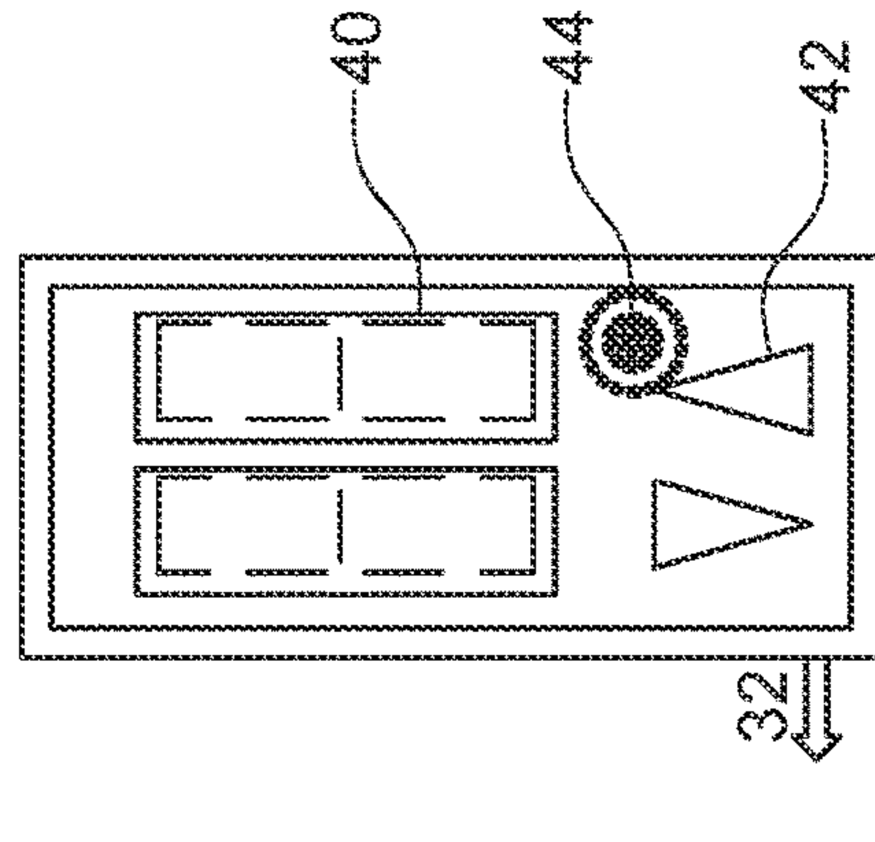
Intermediate Floor FIG. 4.b2
