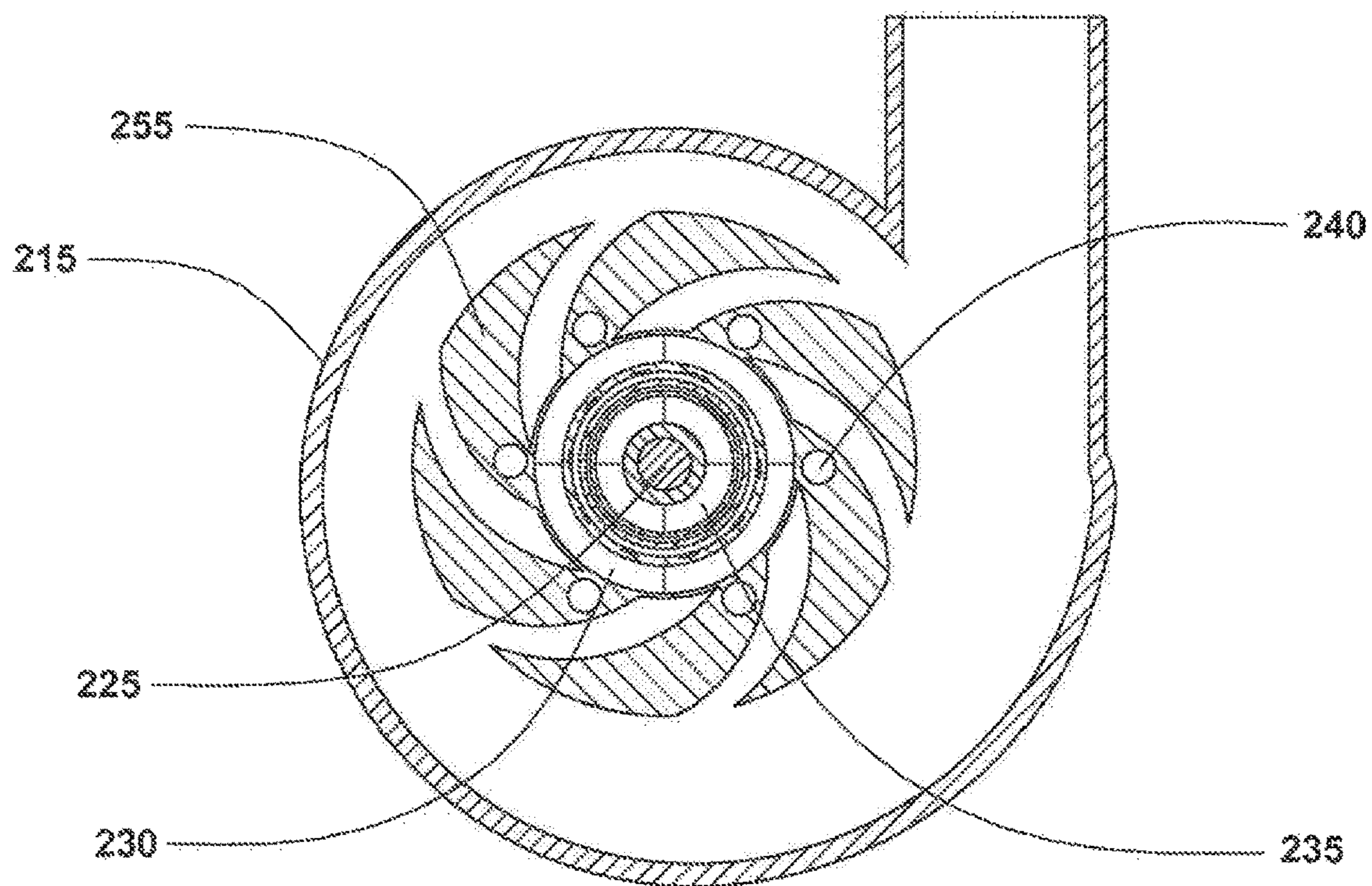
FIG. 19 (Section G-G)
