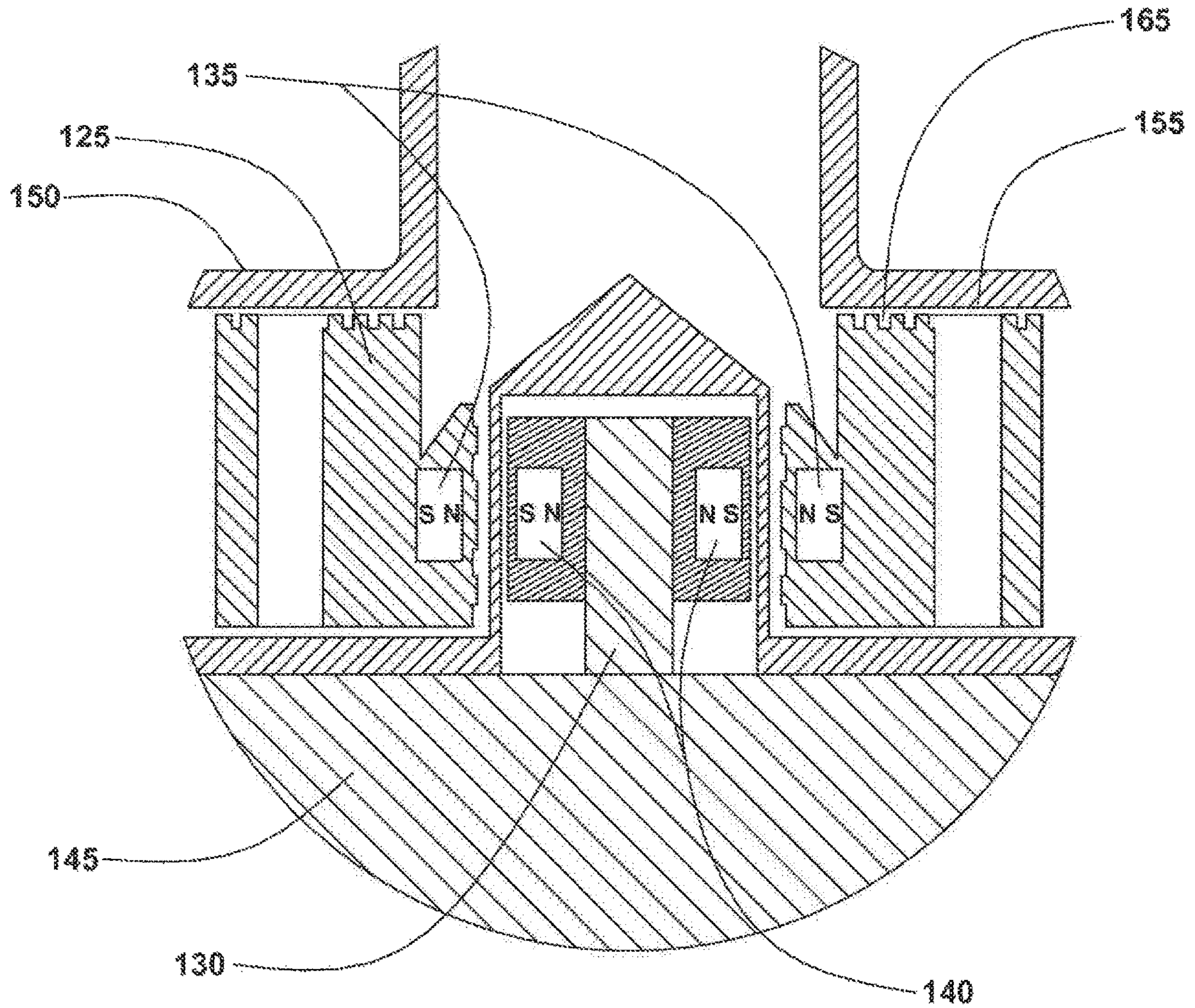
FIG. 13 (DETAIL D)
