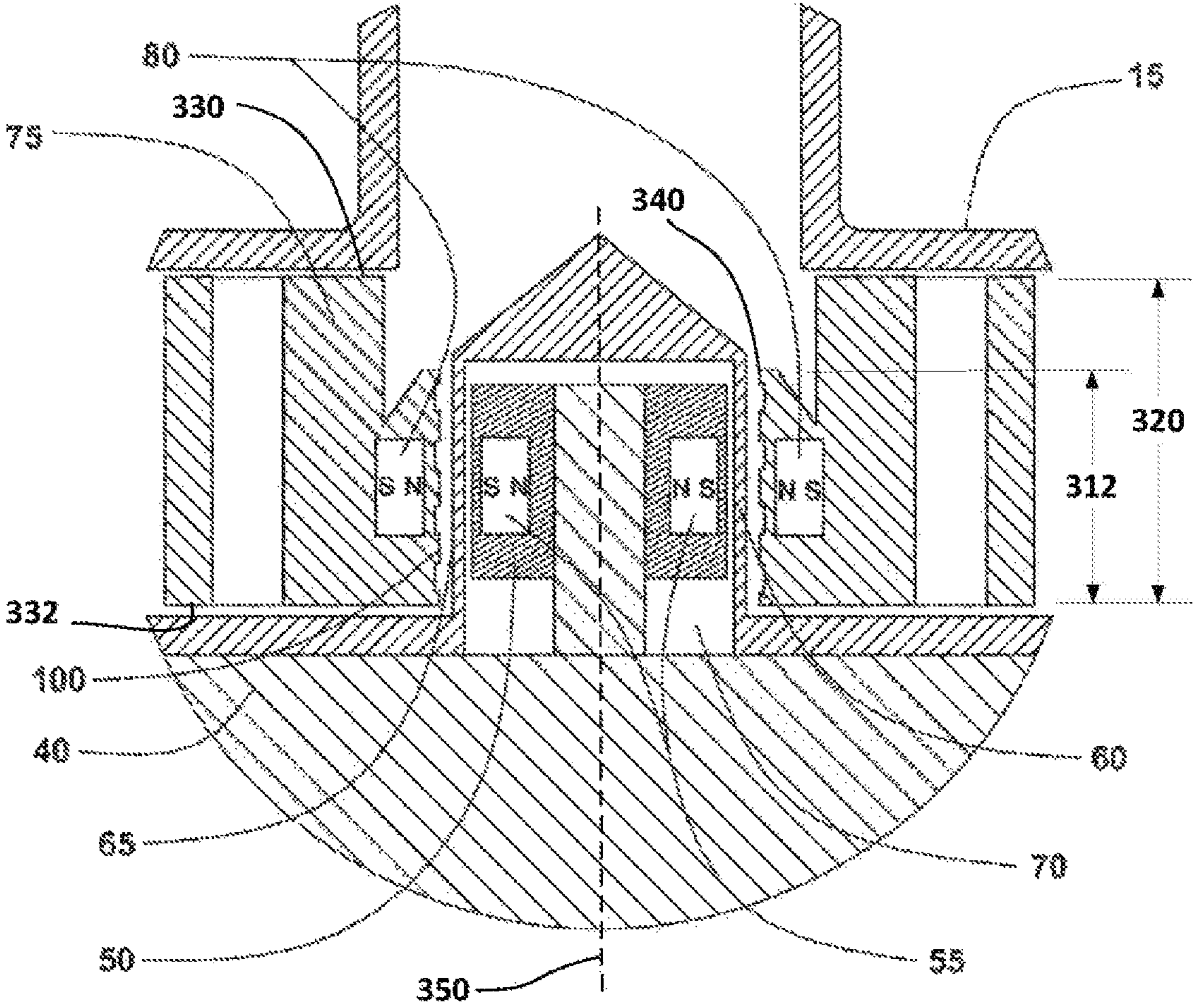
FIG 4 (DETAIL C)
