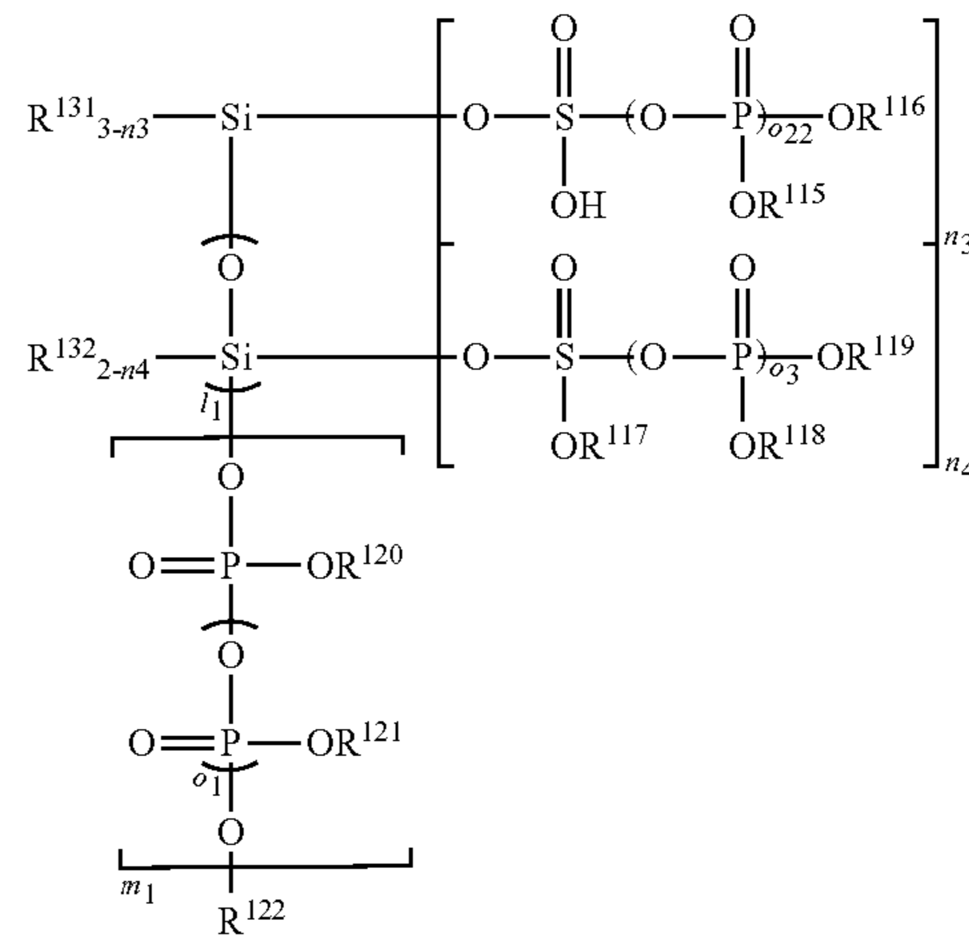
[Chemical Formula C2-1]
