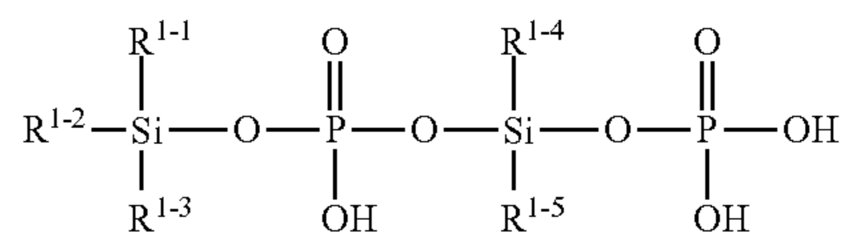
[Chemical Formula A3-6]
