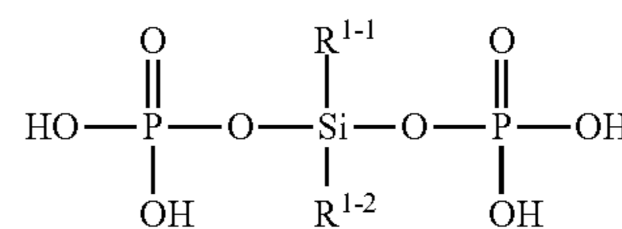
[Chemical Formula A3-3]
