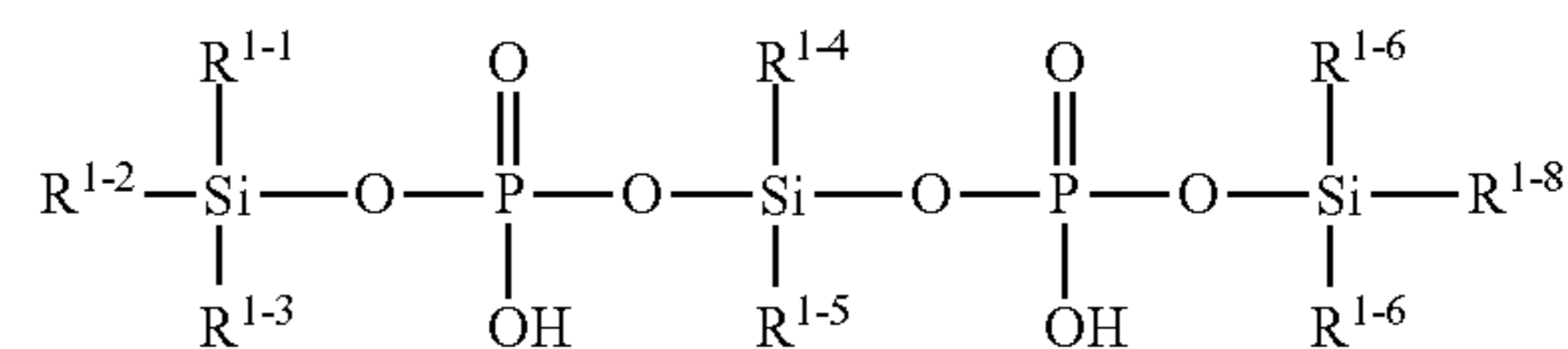
[Chemical Formula A3-6]
