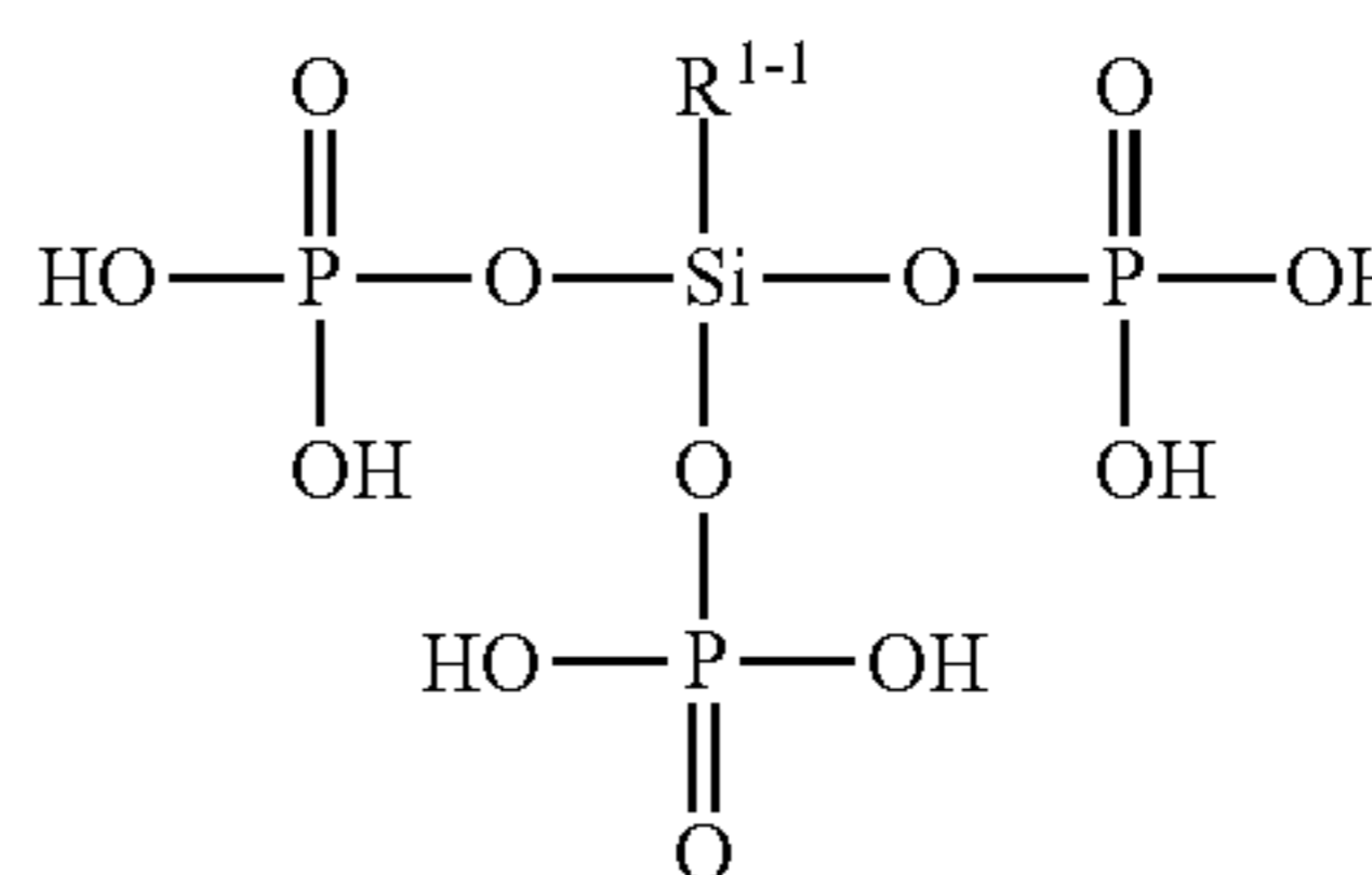
[Chemical Formula A3-5]
