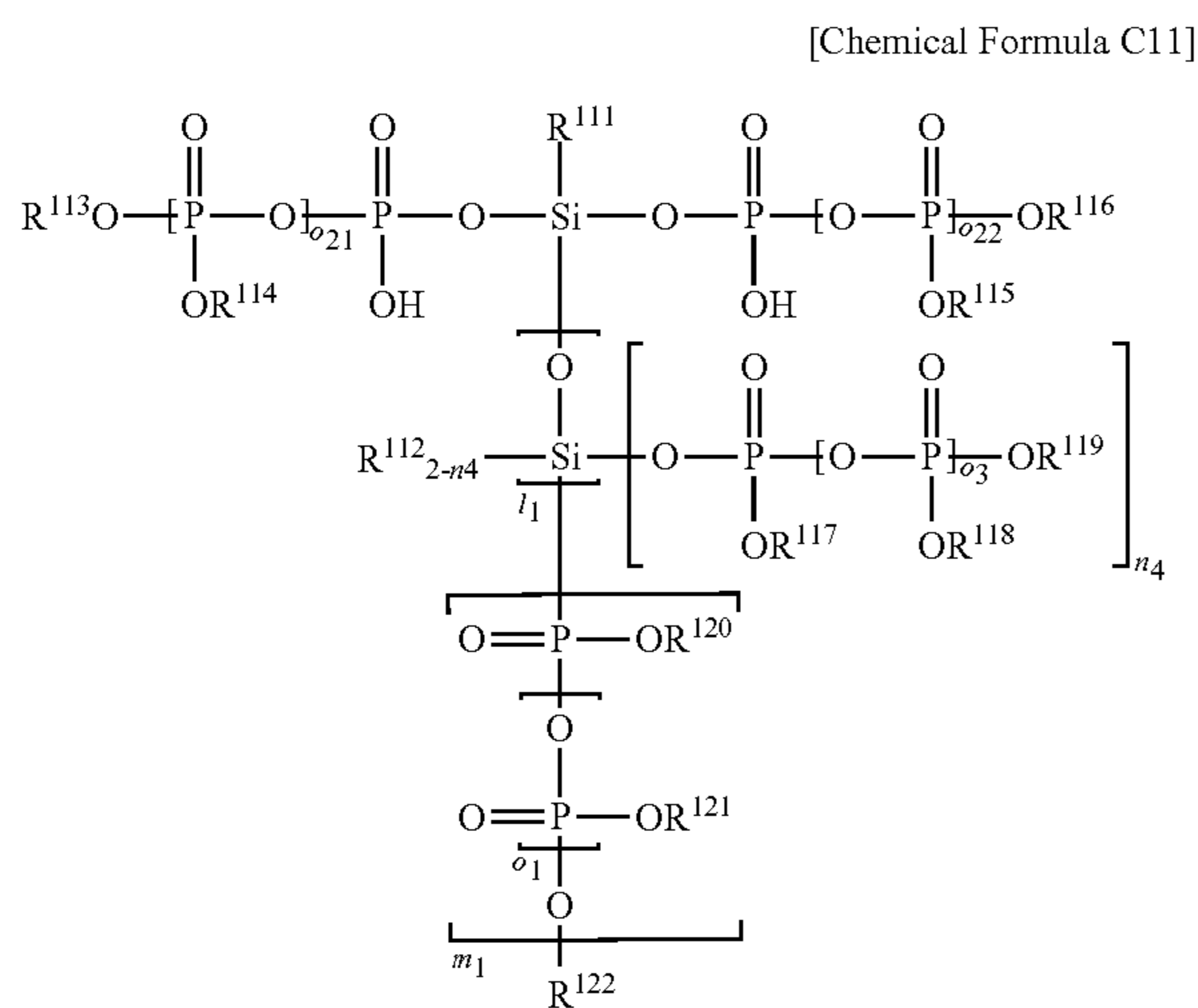
[Chemical Formula A3-2]
