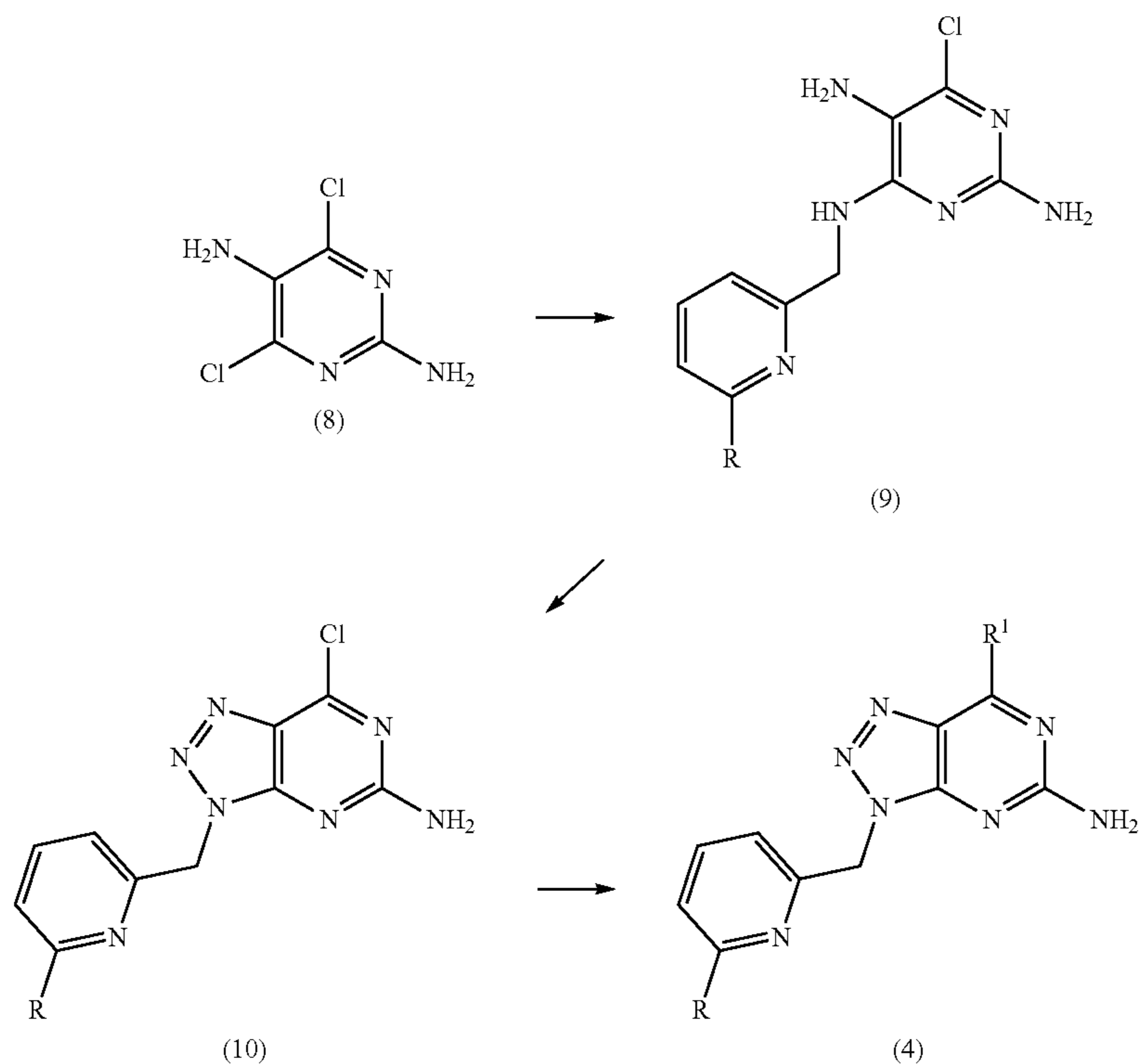
Reaction Scheme 2
