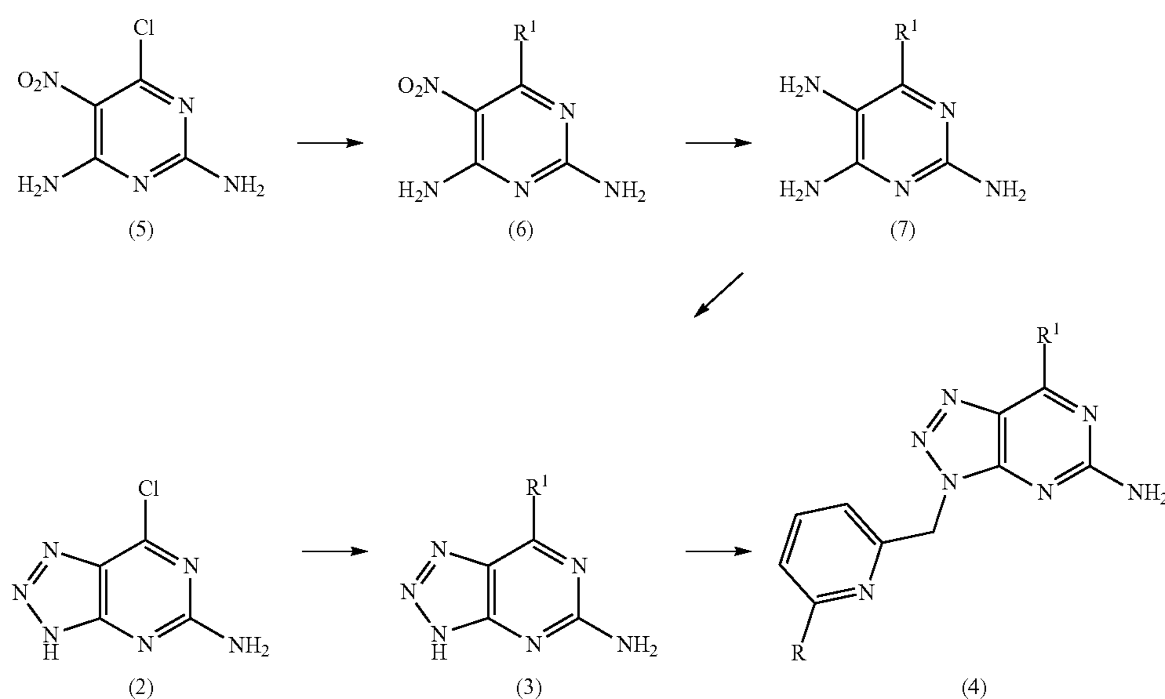
Reaction Scheme 1
