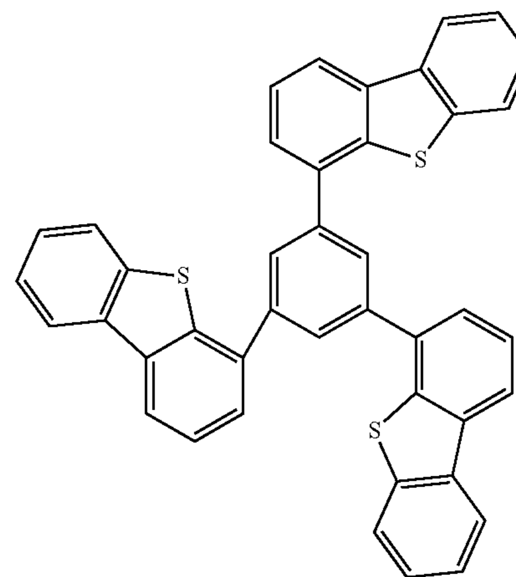
DBT3P-II
