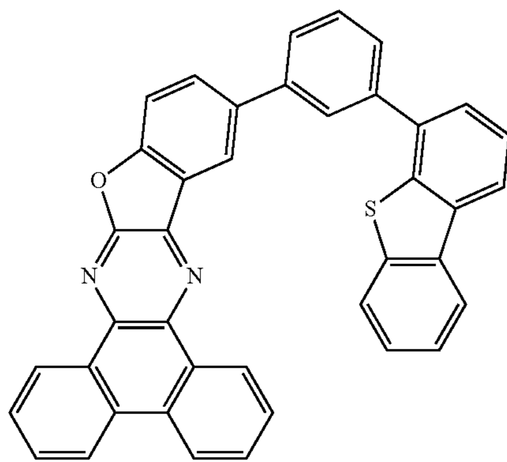
13mDBtPBfdbq
