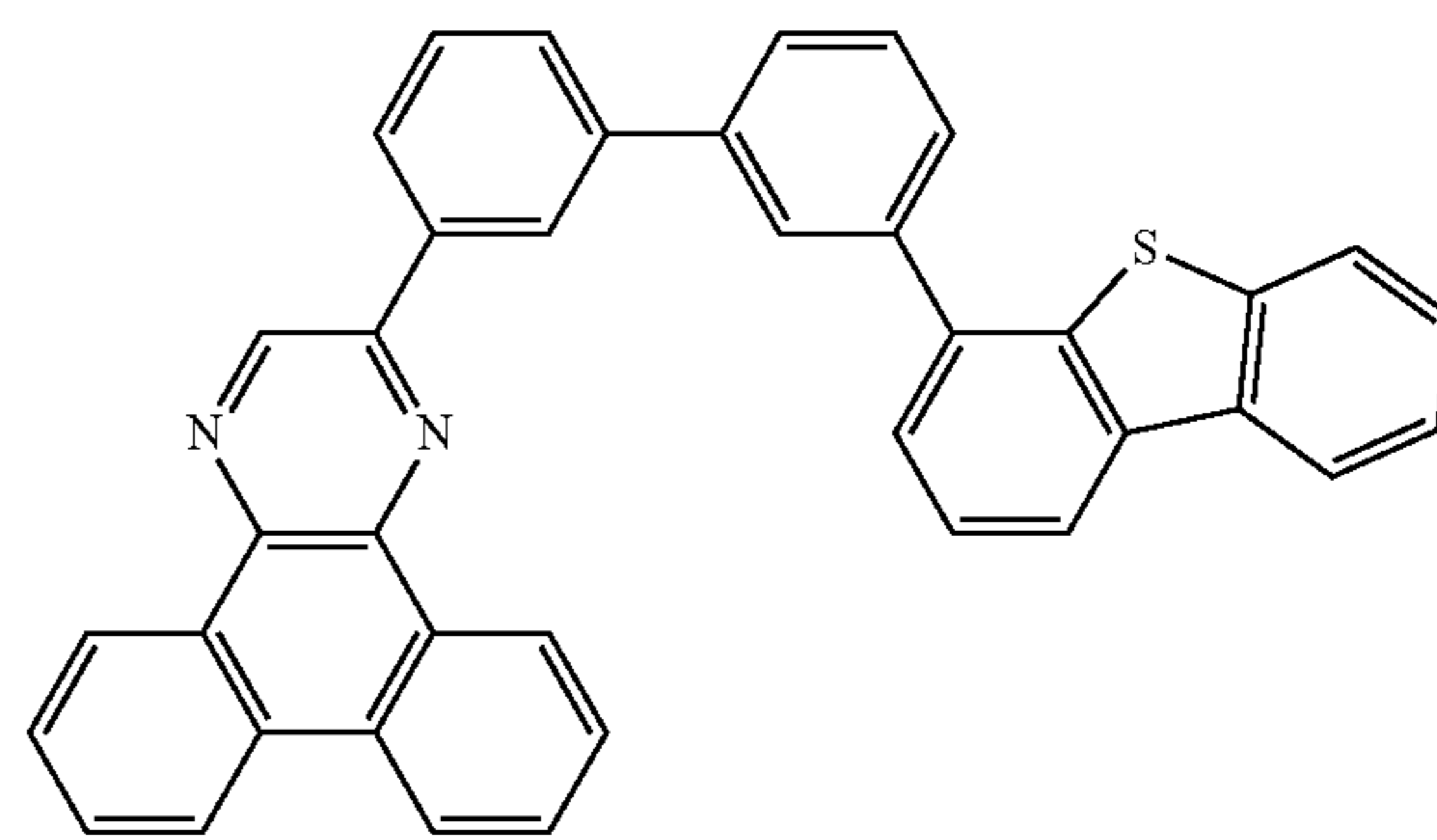
2mDBtBPDBq-II
