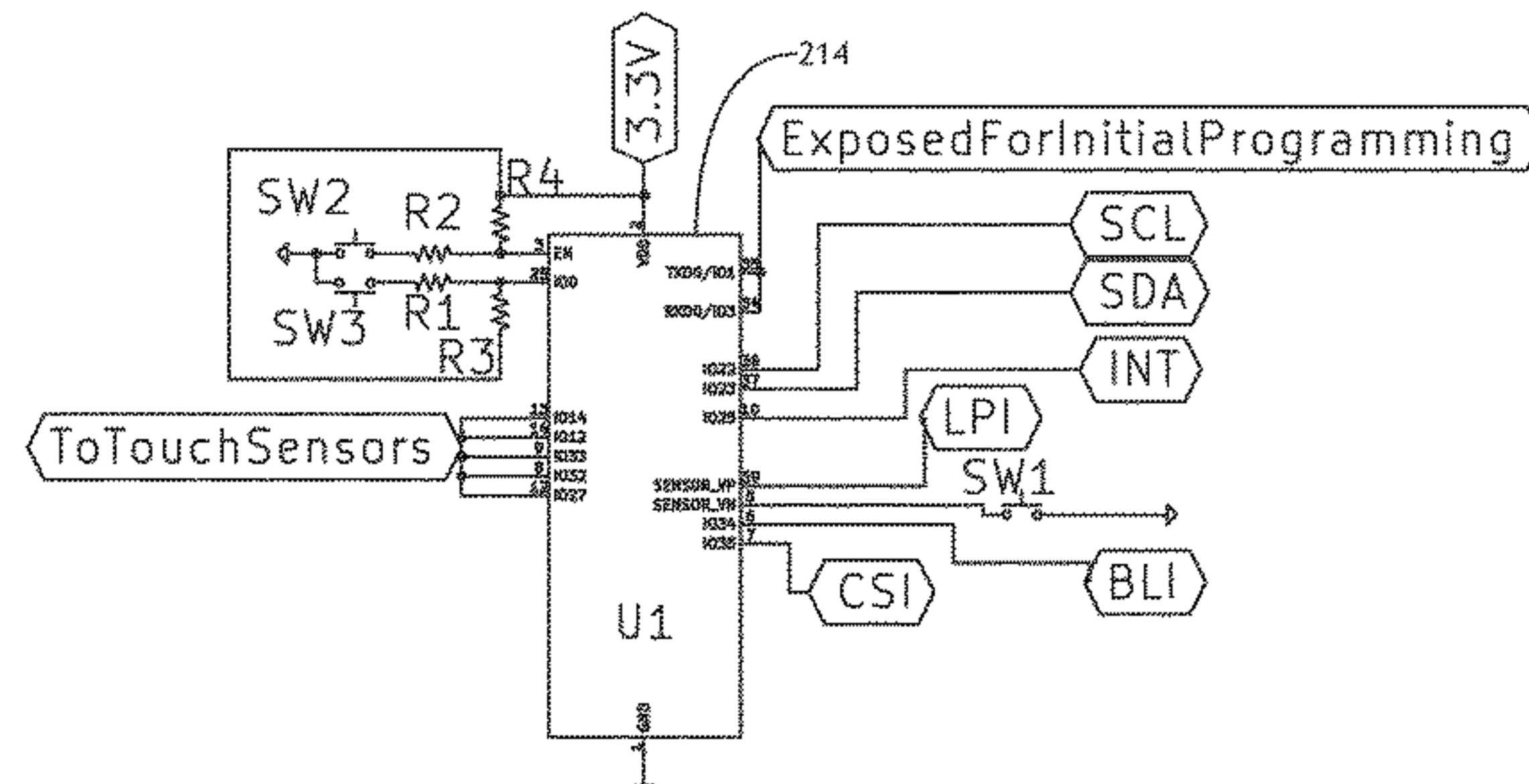
Microcontroller Circuitry
