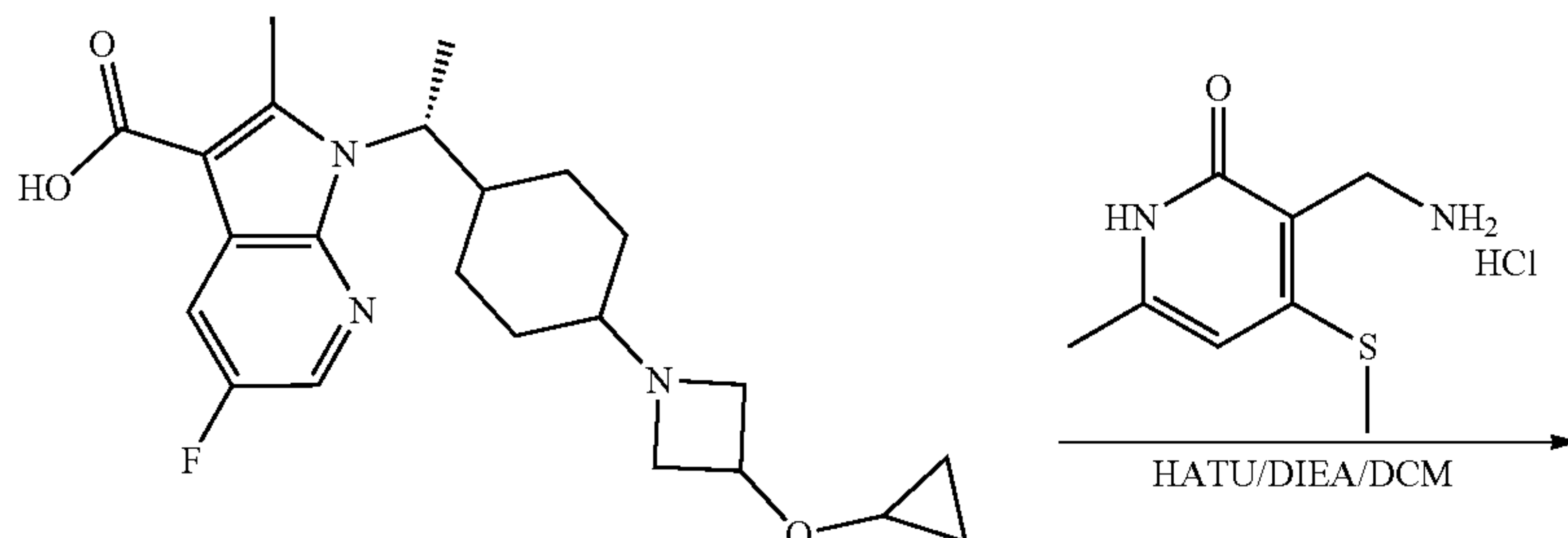
J9 isomer 1
