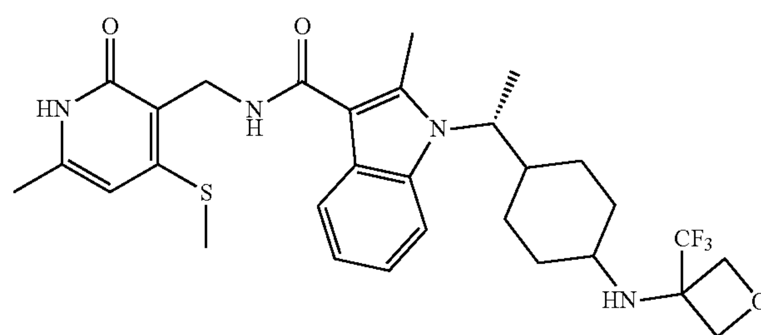
single isomer
