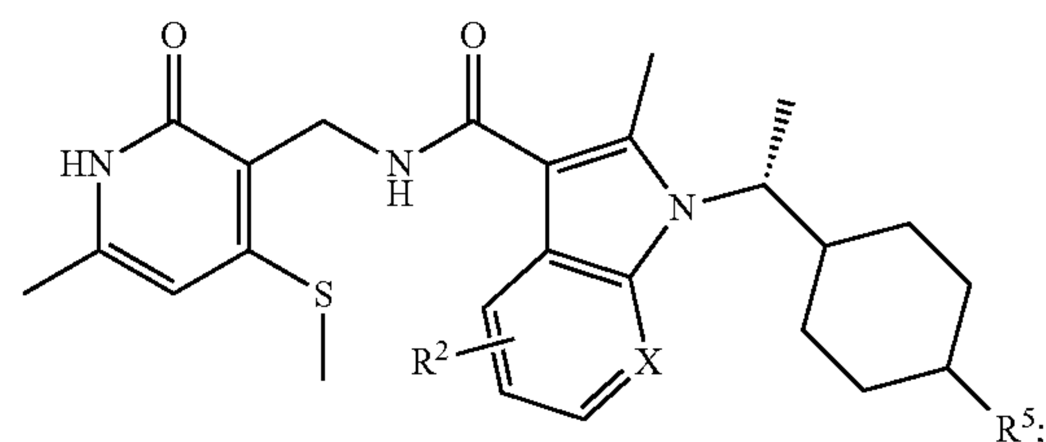
(XXXVI)
