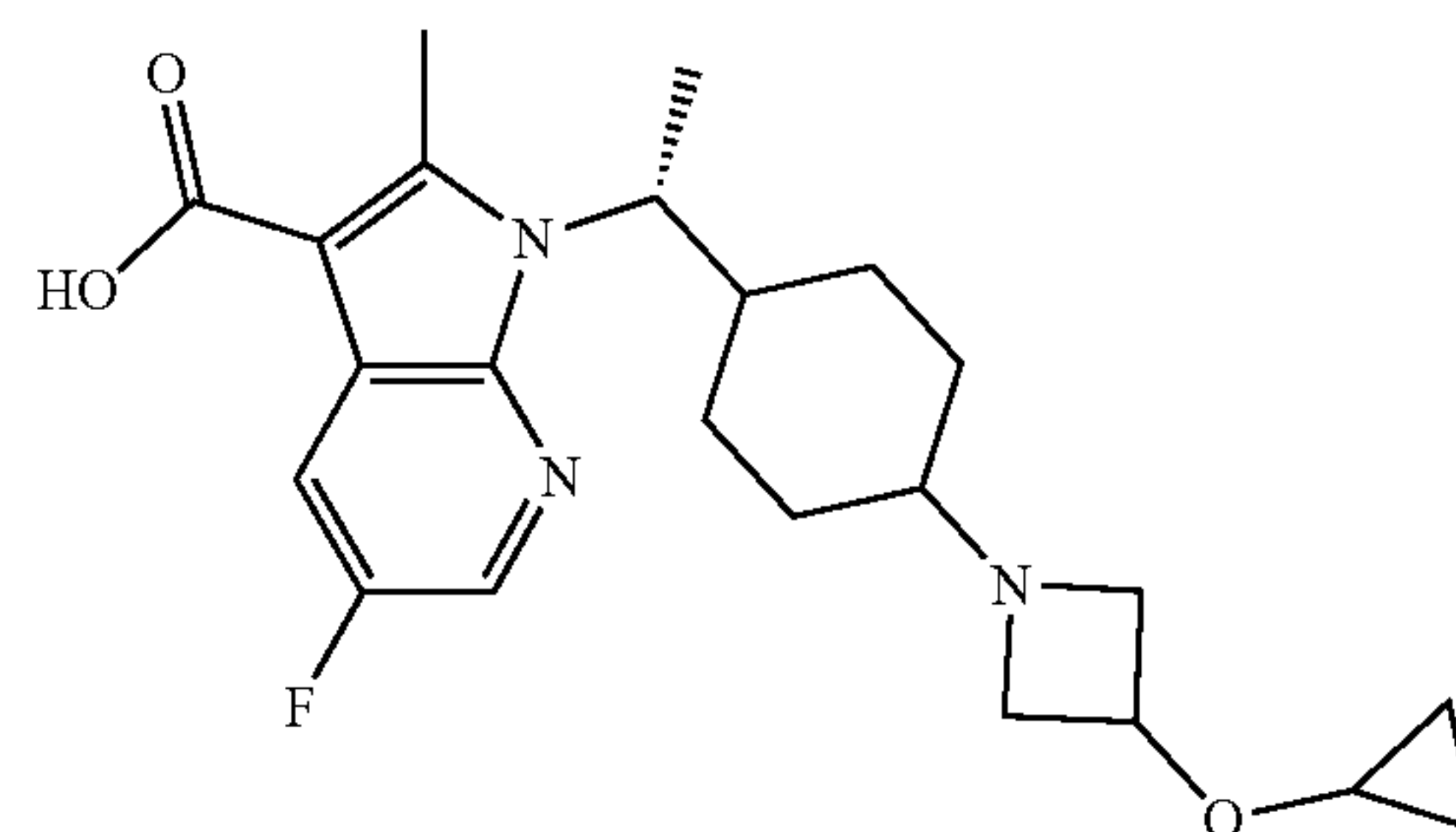
J9 isomer 2
