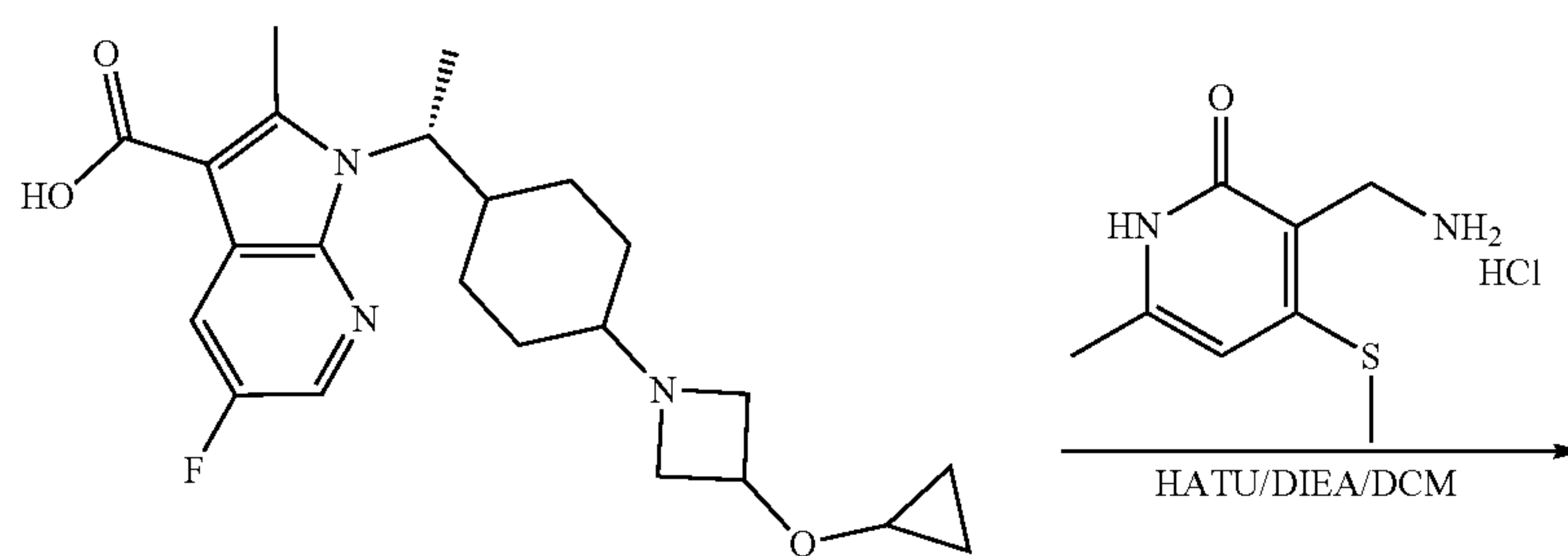
J9 isomer 2
