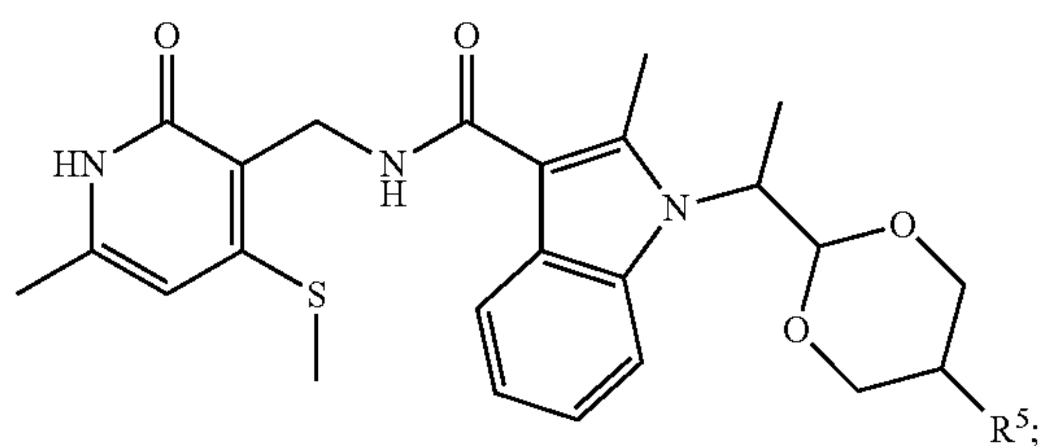
(XXI)
