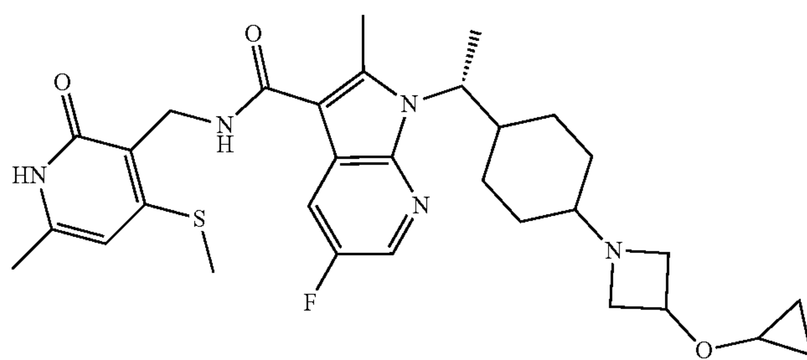
isomer 1
