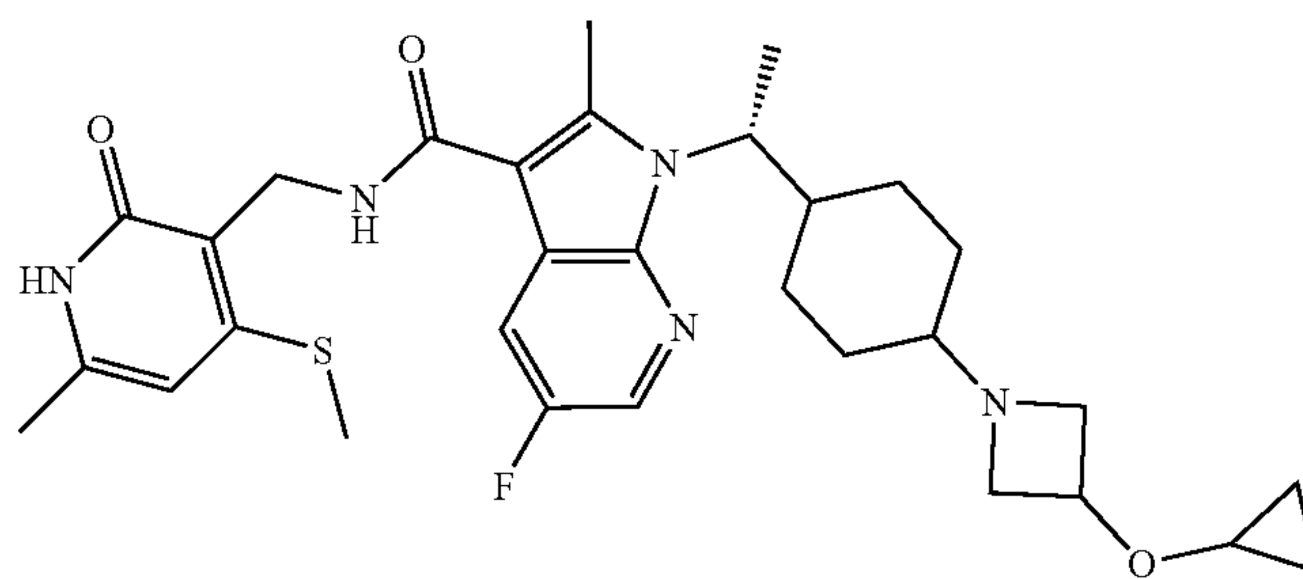
isomer 2
