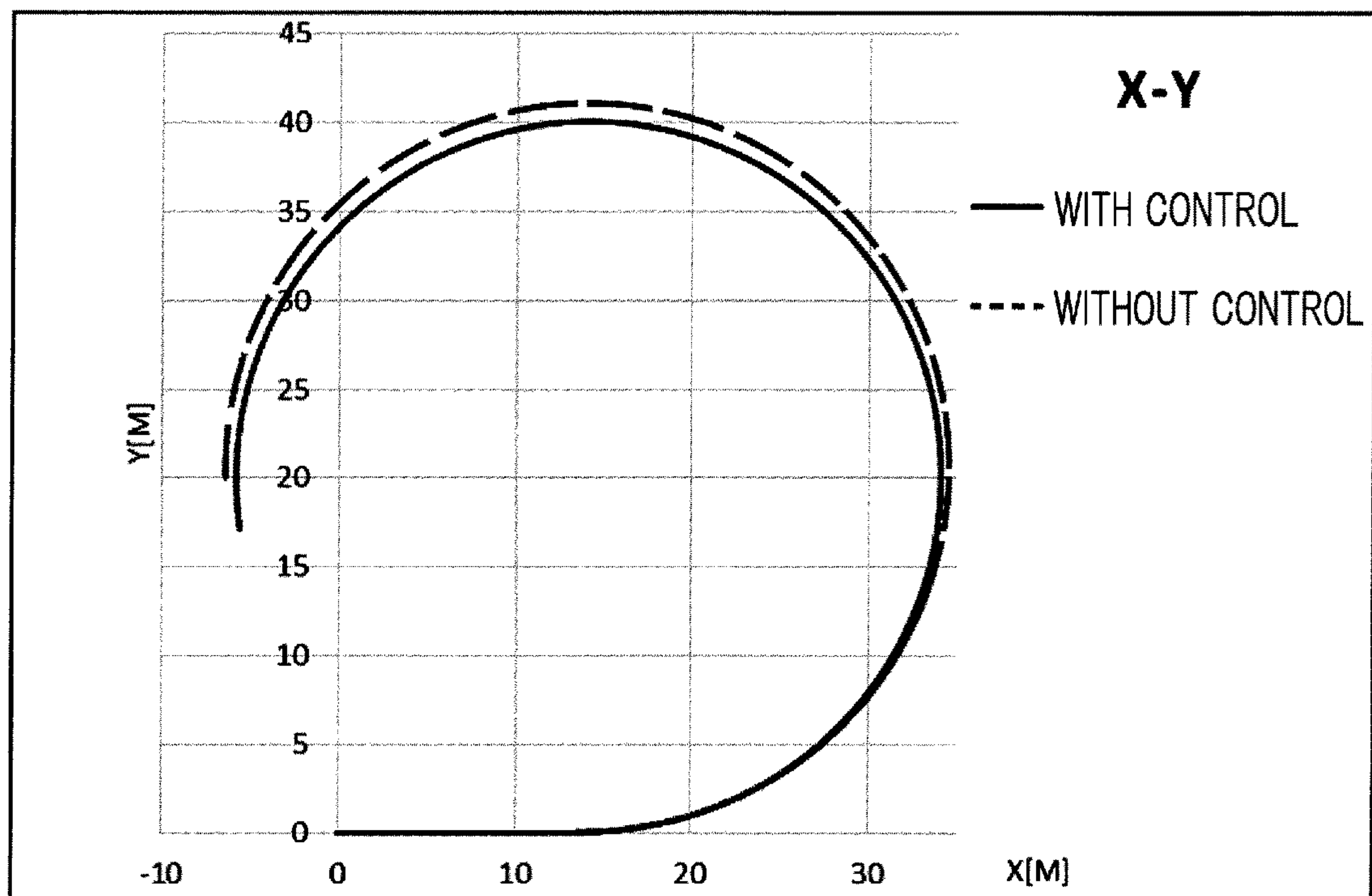
(a) VEHICLE TURNING PATH
