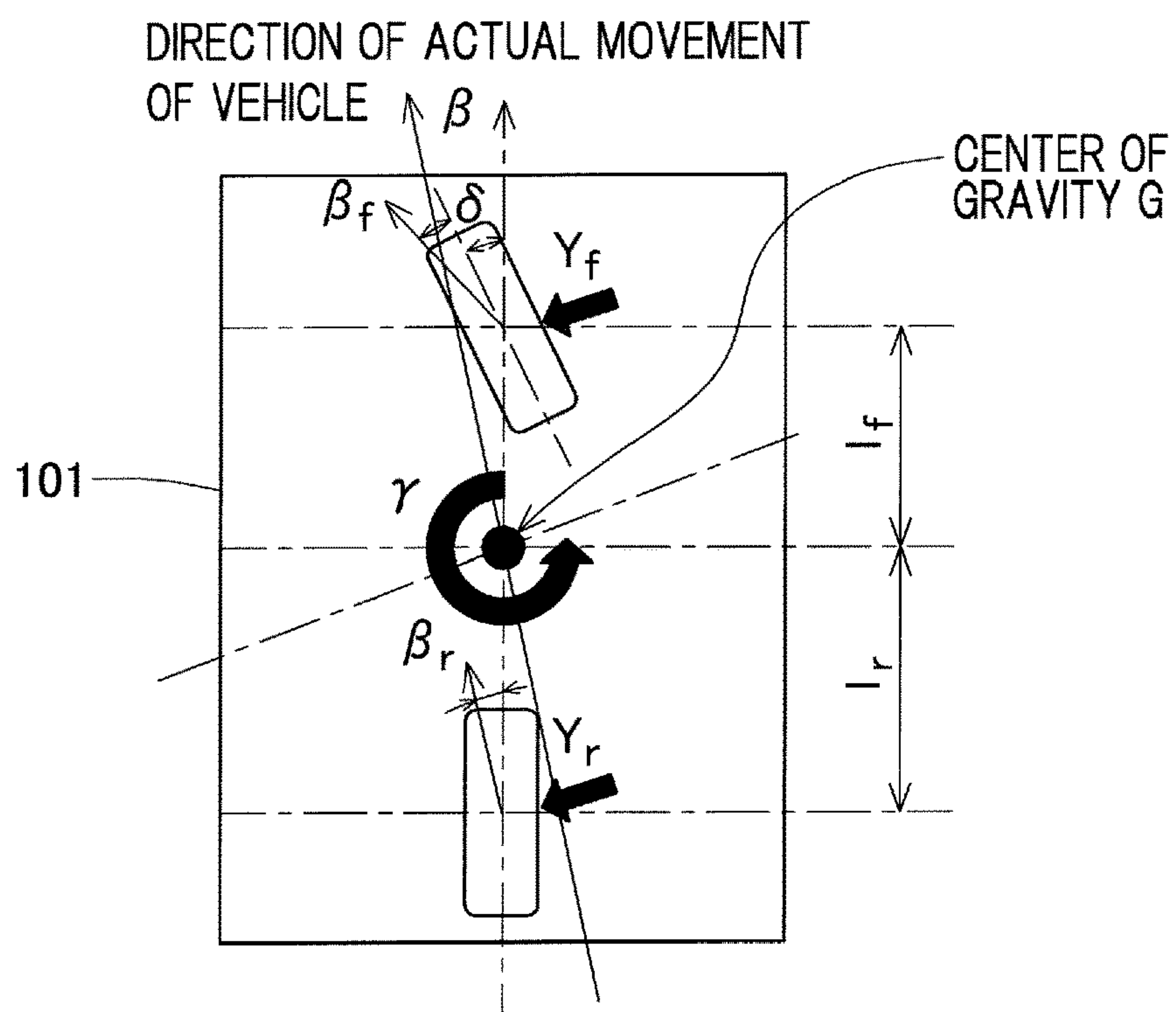
Fig. 5 TWO-WHEEL MODEL
