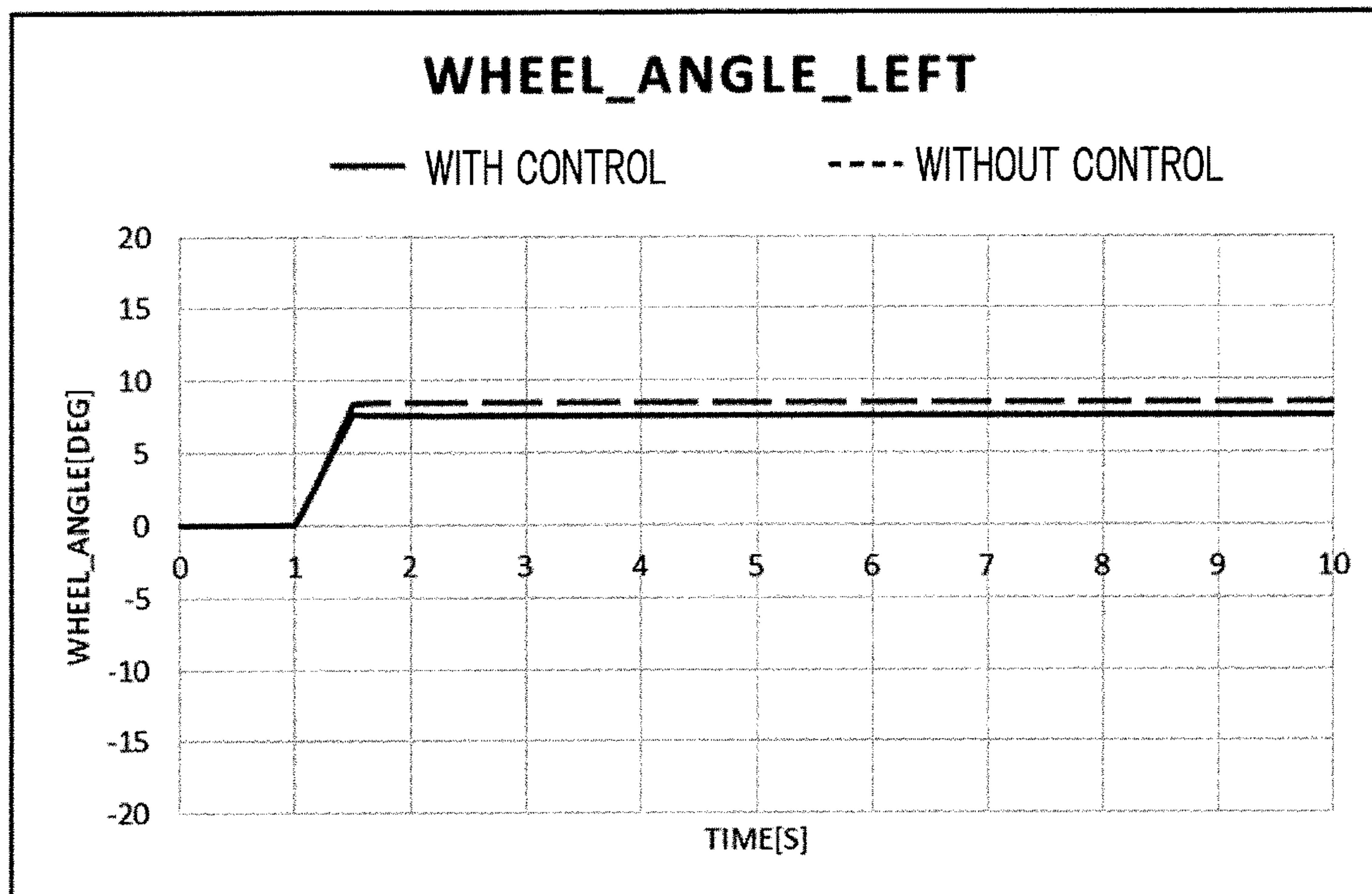
(c) LEFT WHEEL ANGLE
