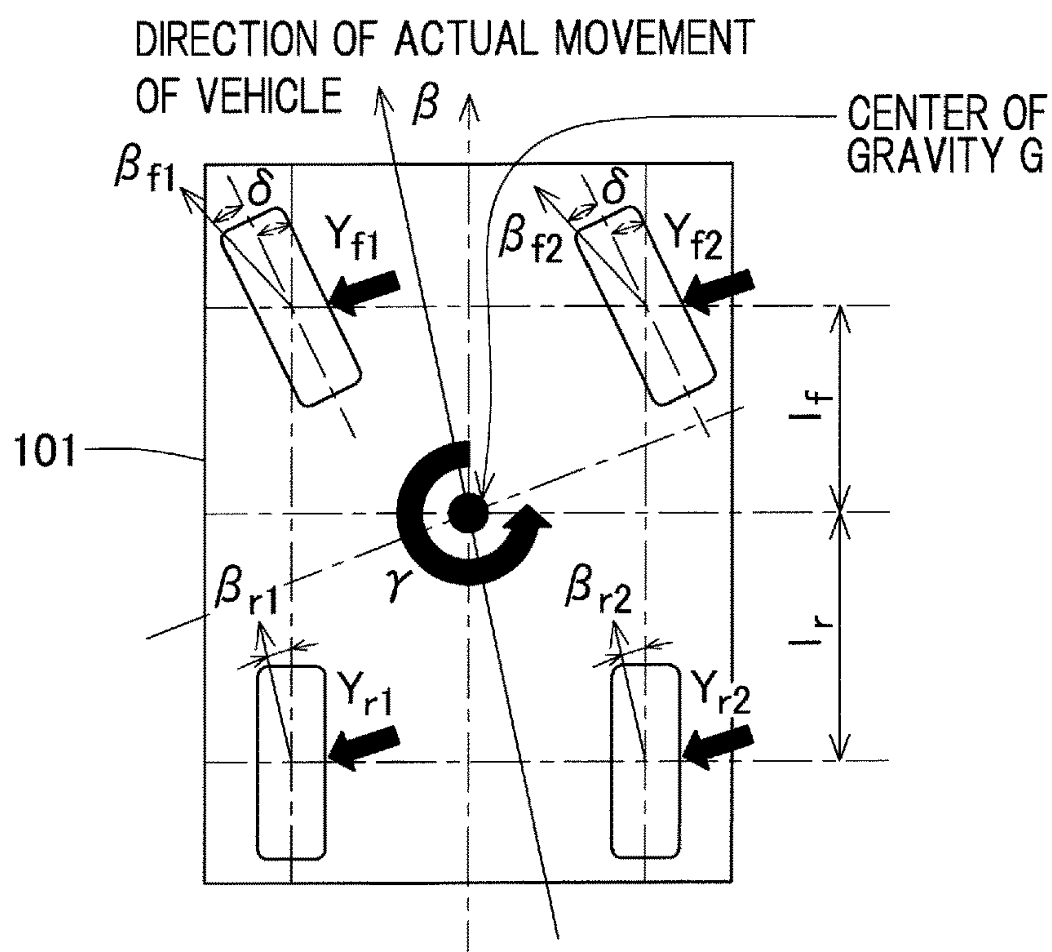
Fig. 4 FOUR-WHEEL MODEL
