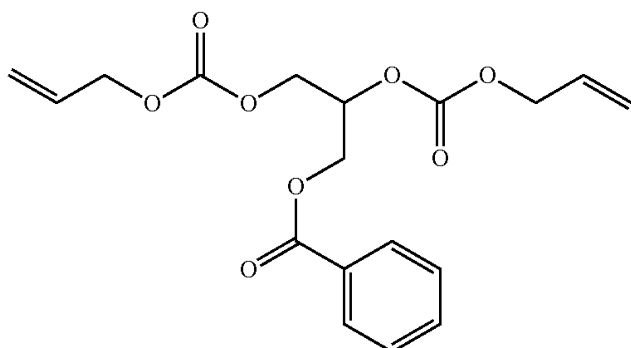
2,3-Bis(((allyloxy)carbonyl)oxy)propyl benzoate
