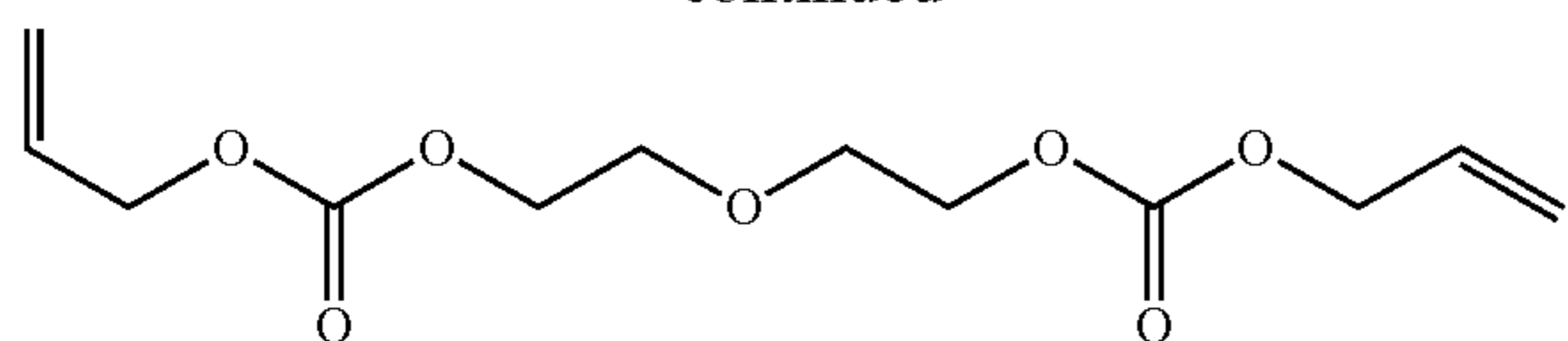
Di(allyl carbonate) bis(ethylene glycol) (CAS No: 142-22-3)
