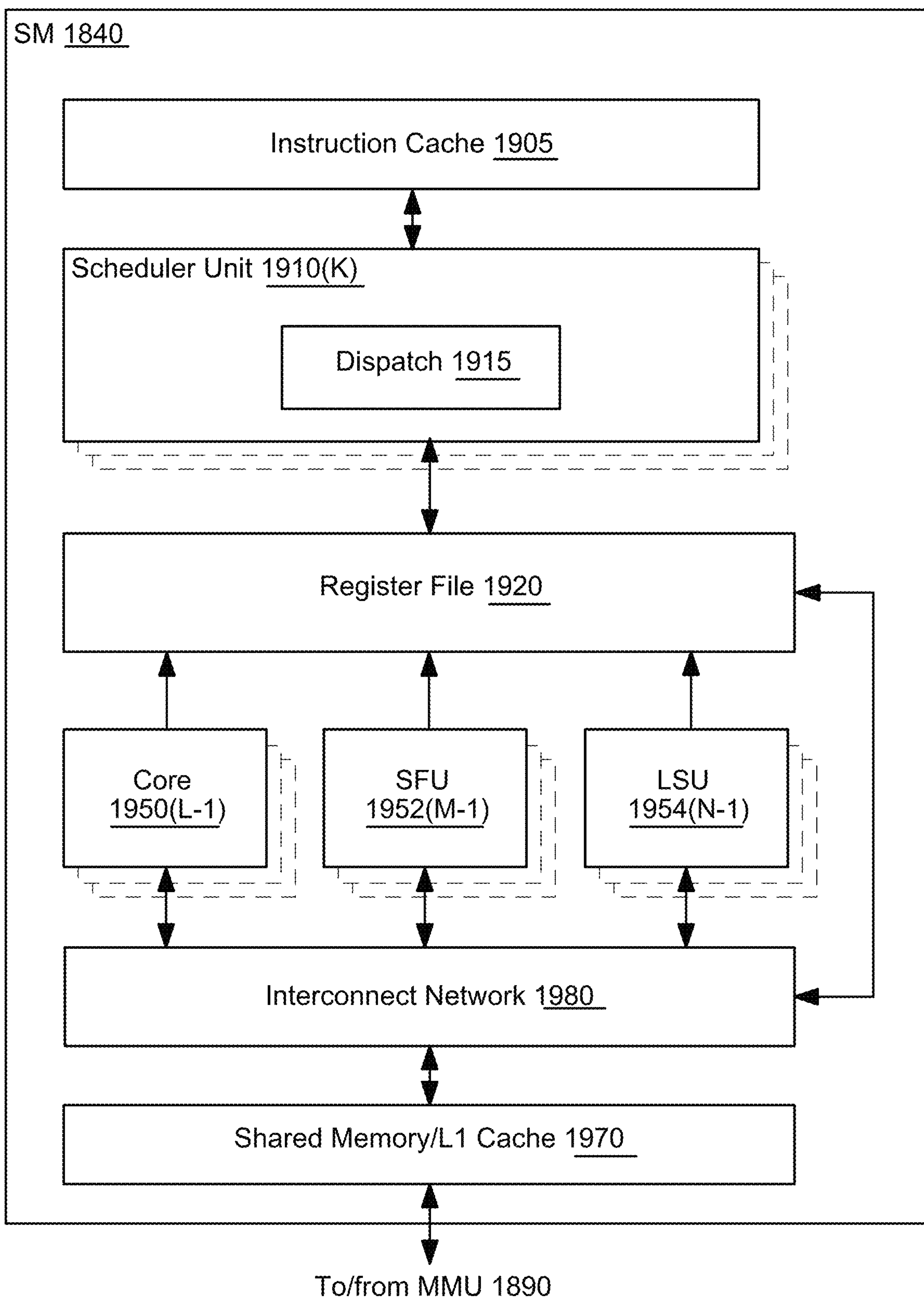
FIG. 19 Example Streaming Multiprocessor
