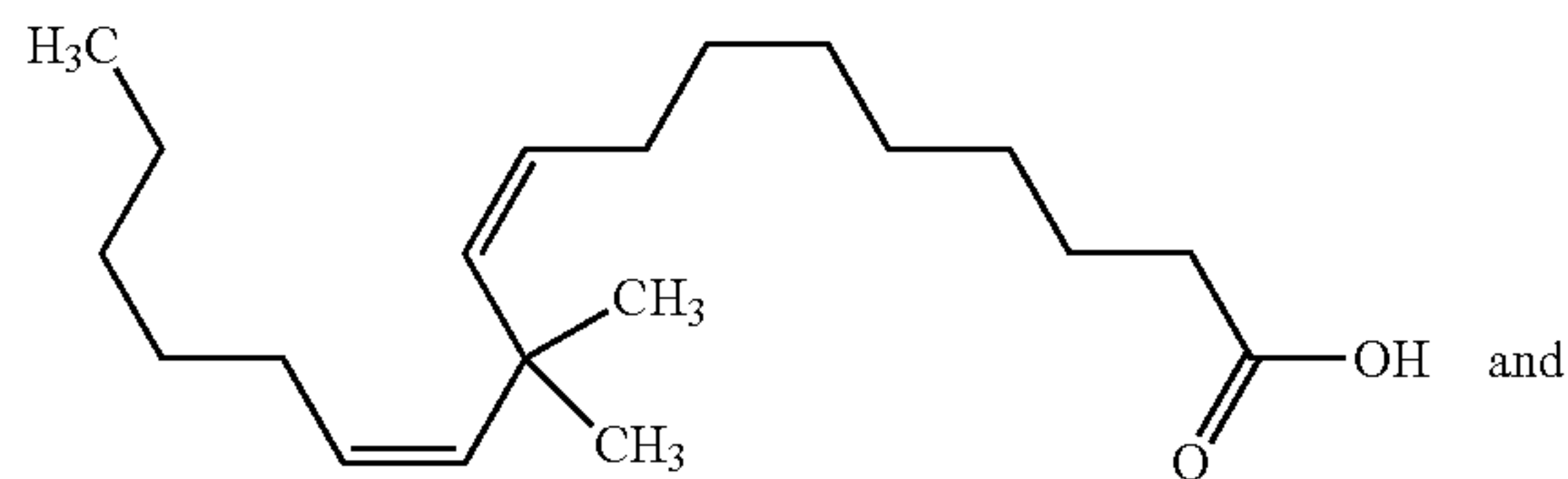
11,11-Dimethyl-octadeca-9,12-dienoic acid
