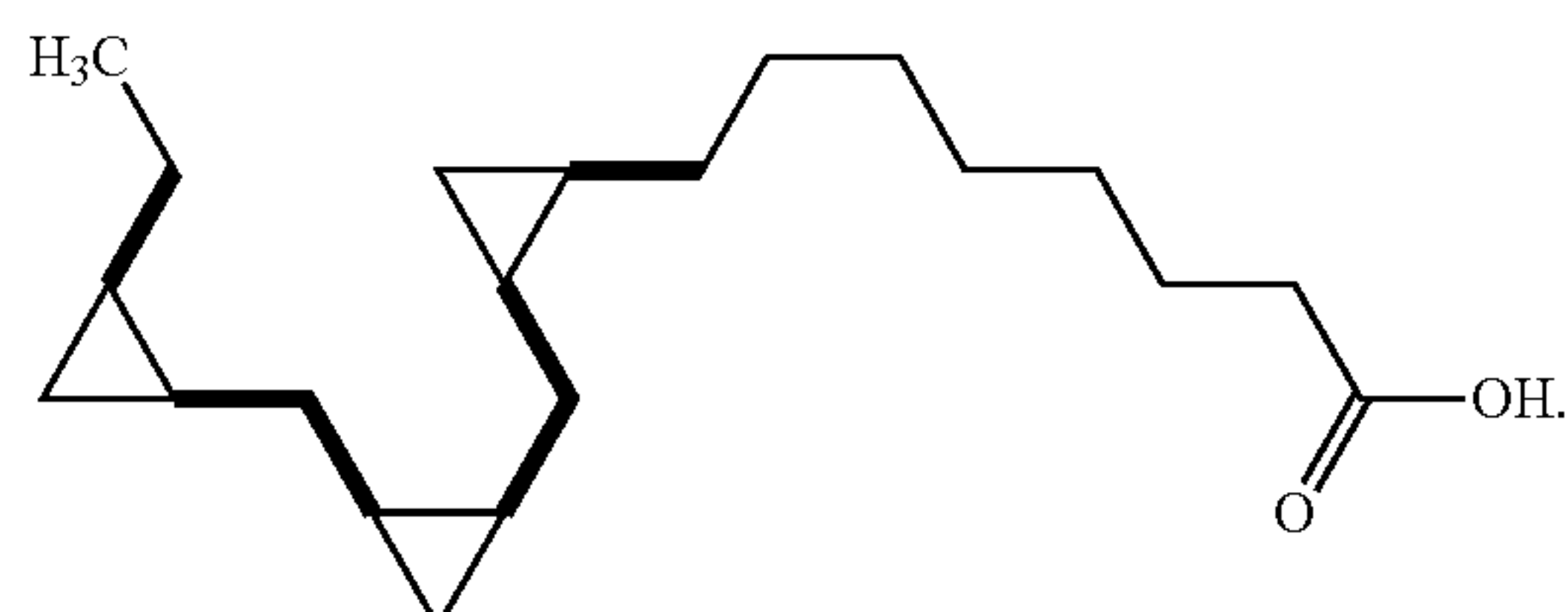
8-{2-[2-(2-Ethyl-cyclopropylmethyl)-cyclopropylmethyl]-cyclopropyl}-octanoic acid
