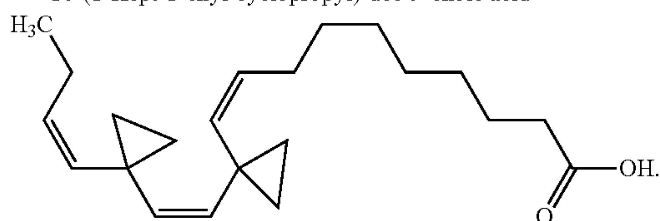
10-{1-[2-(1-But-1-enyl-cyclopropyl)-vinyl]-cyclopropyl}-dec-9-enoic acid
