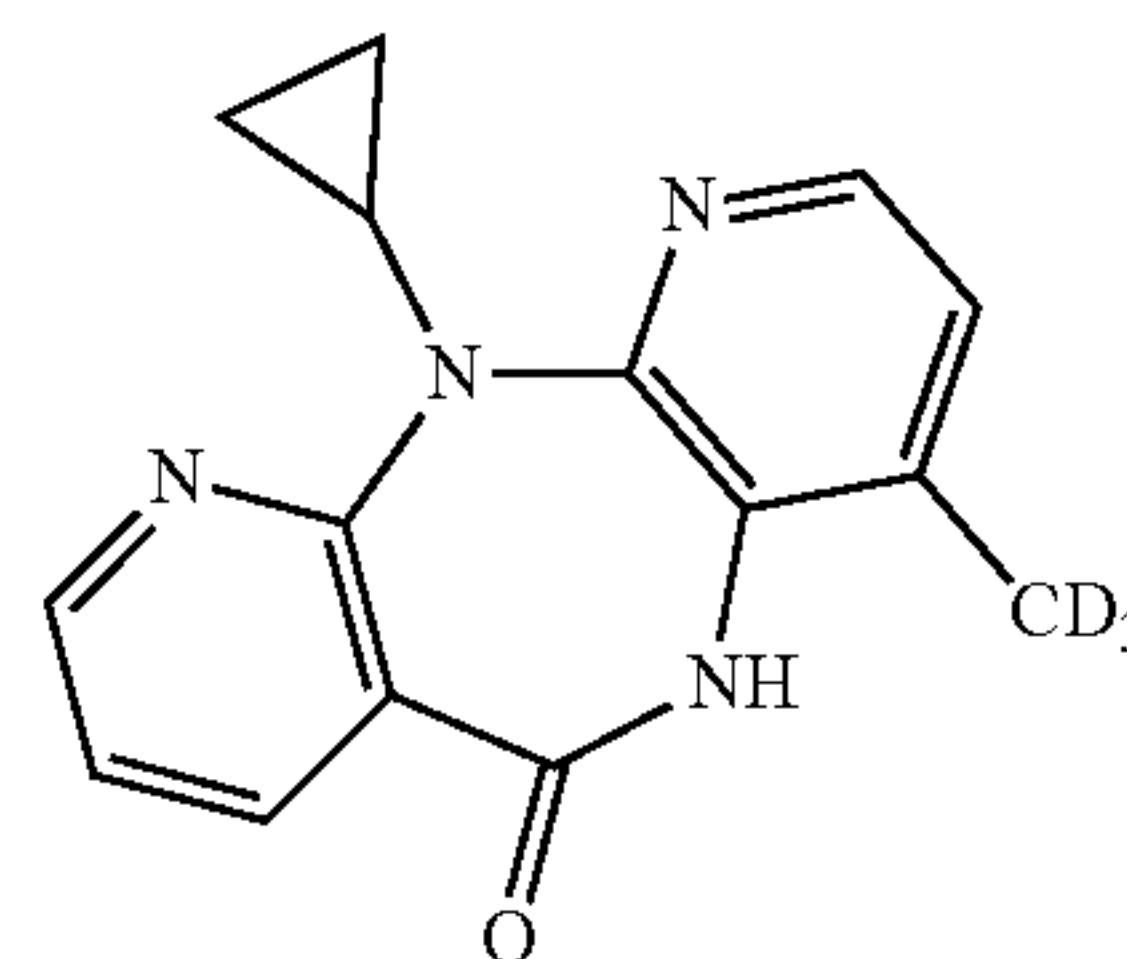
Deuterated Nevirapine
