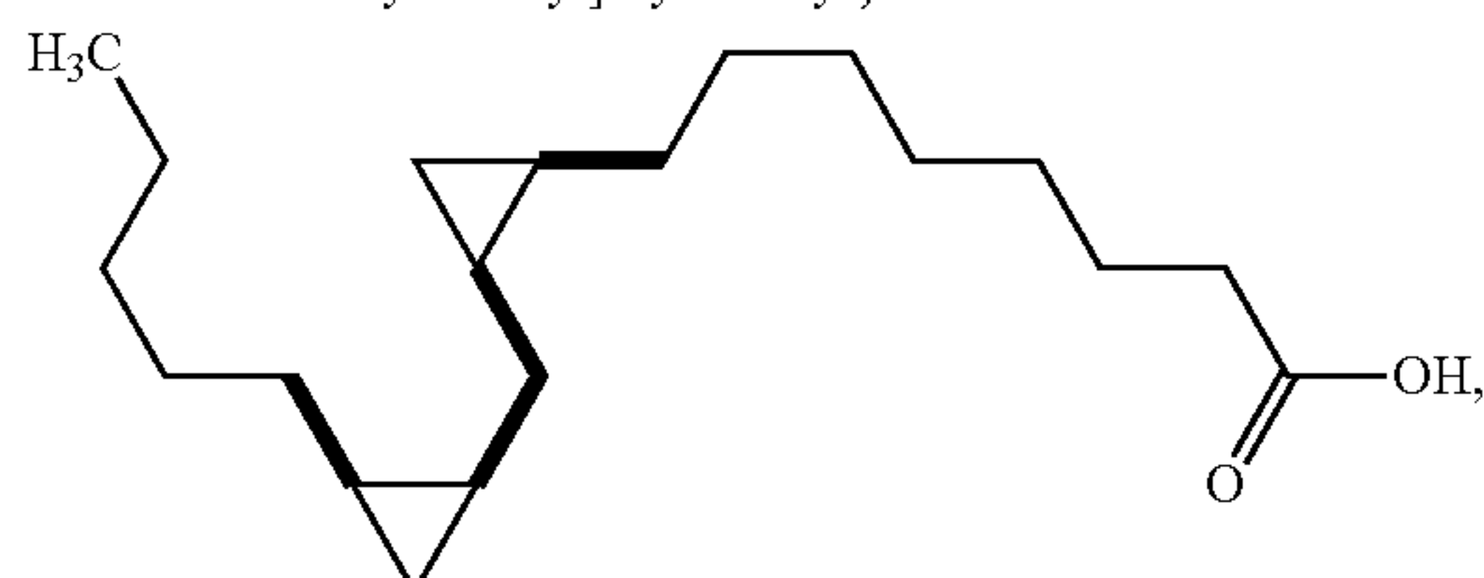
8-[2-(2-Pentyl-cyclopropylmethyl)-cyclopropyl]-octanoic acid
