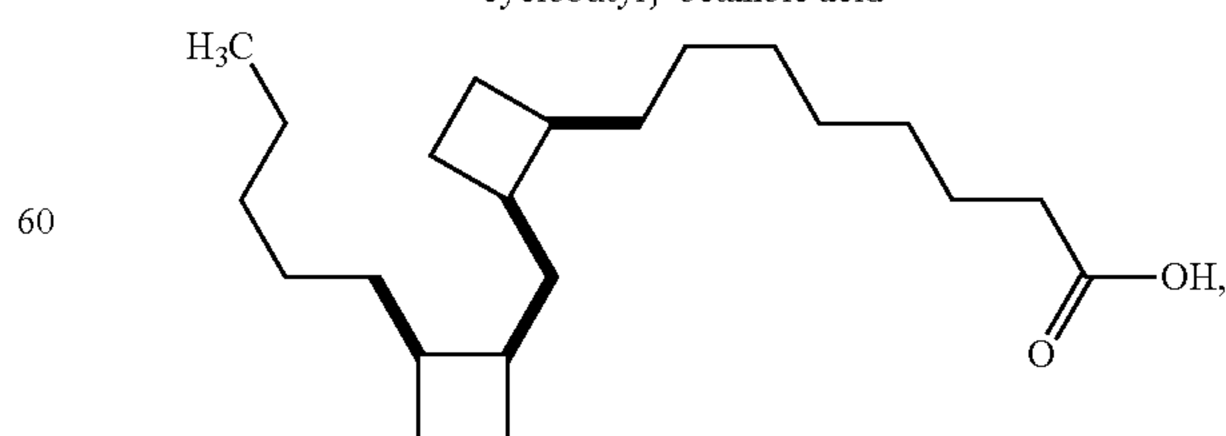
8-[2-(2-Pentyl-cyclobutylmethyl)-cyclobutyl]-octanoic acid
