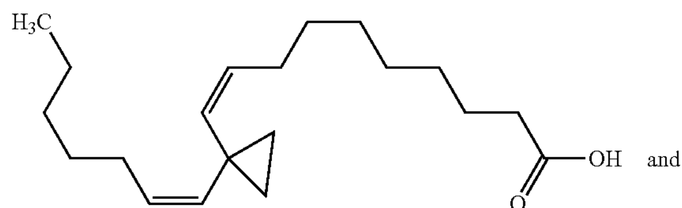
10-(1-Hept-1-enyl-cyclopropyl)-dec-9-enoic acid
