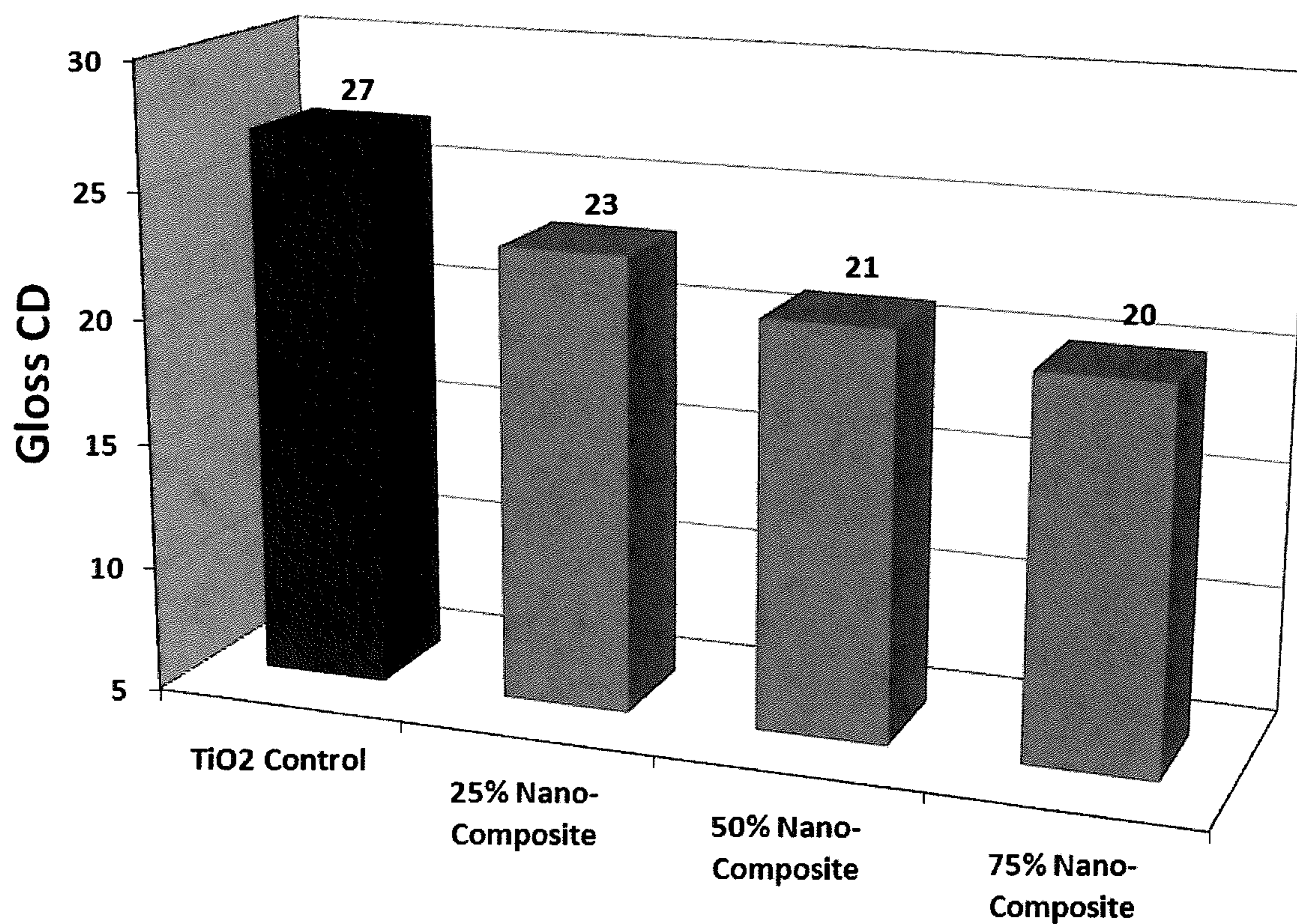
Effect of Replacement of TiO 2 by Nano-Composite
