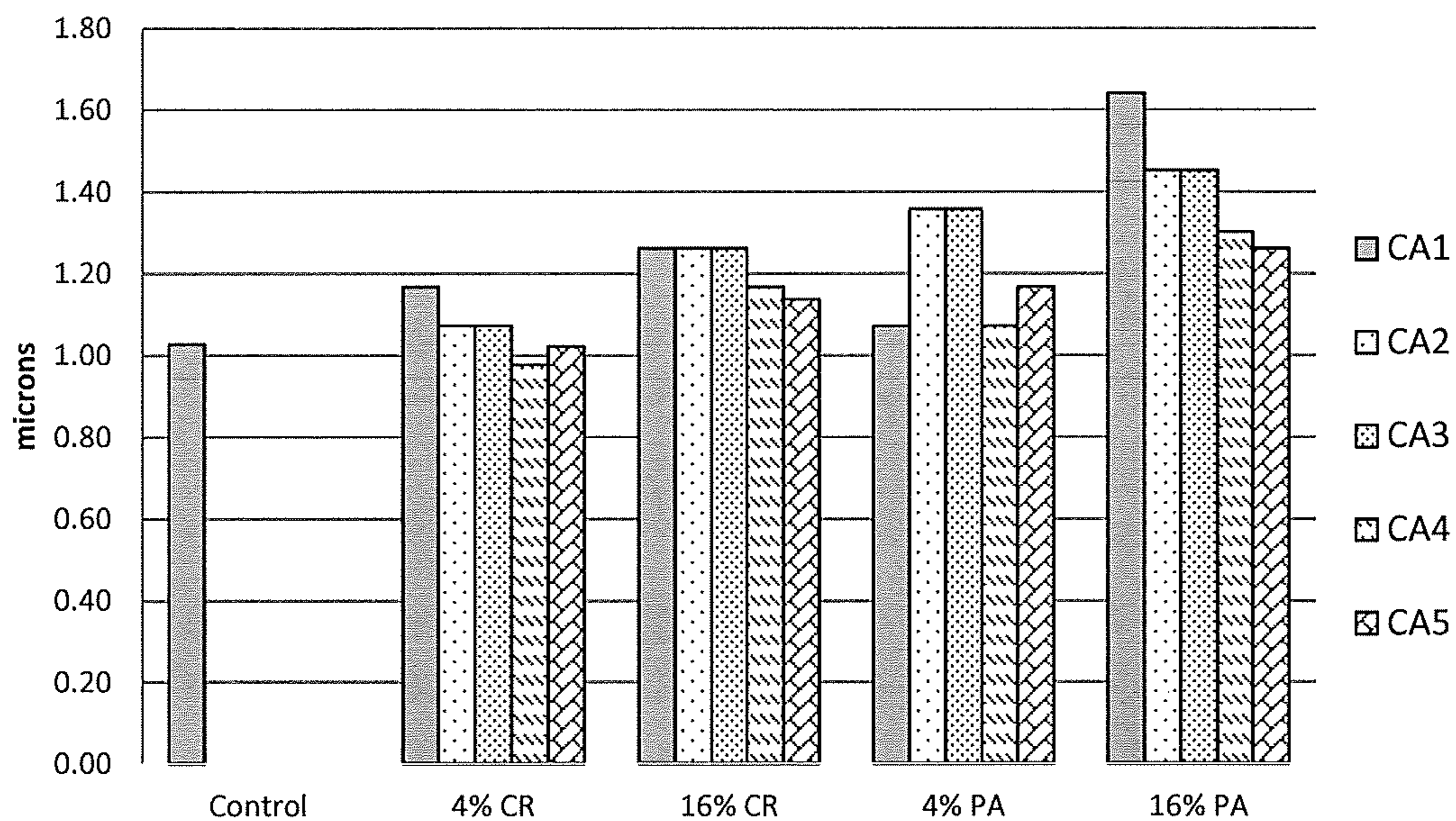
Mean Flow Pore Size: Method 2, Lab 2
