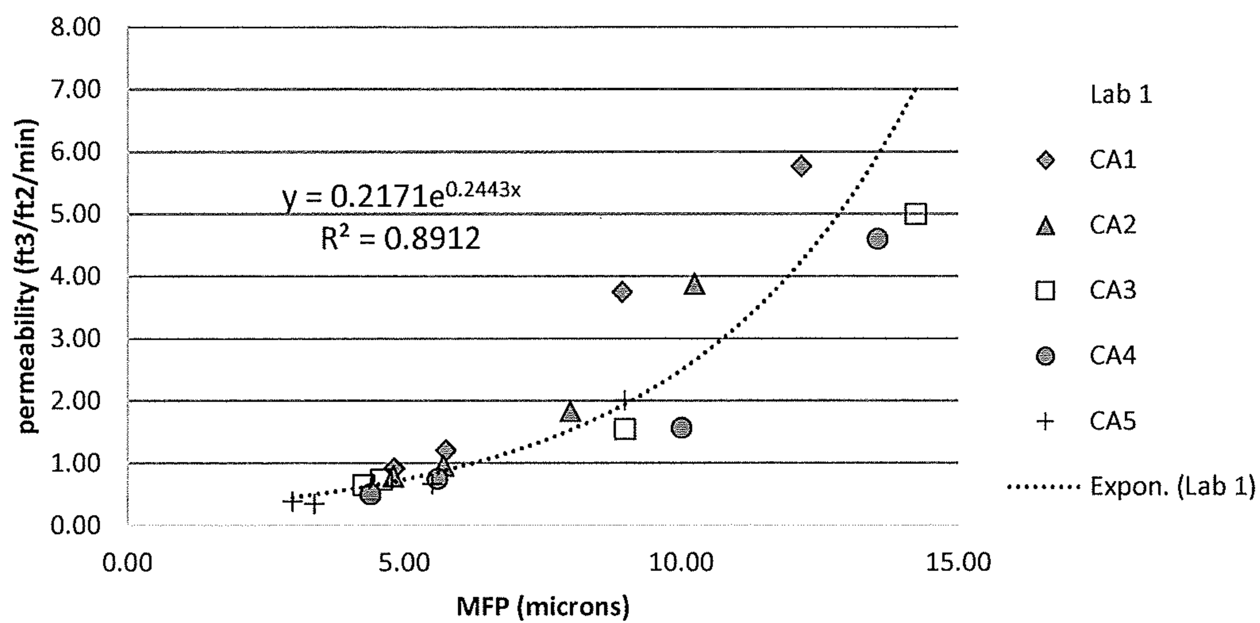
Permeability vs MFP: Method 1, Lab 1
