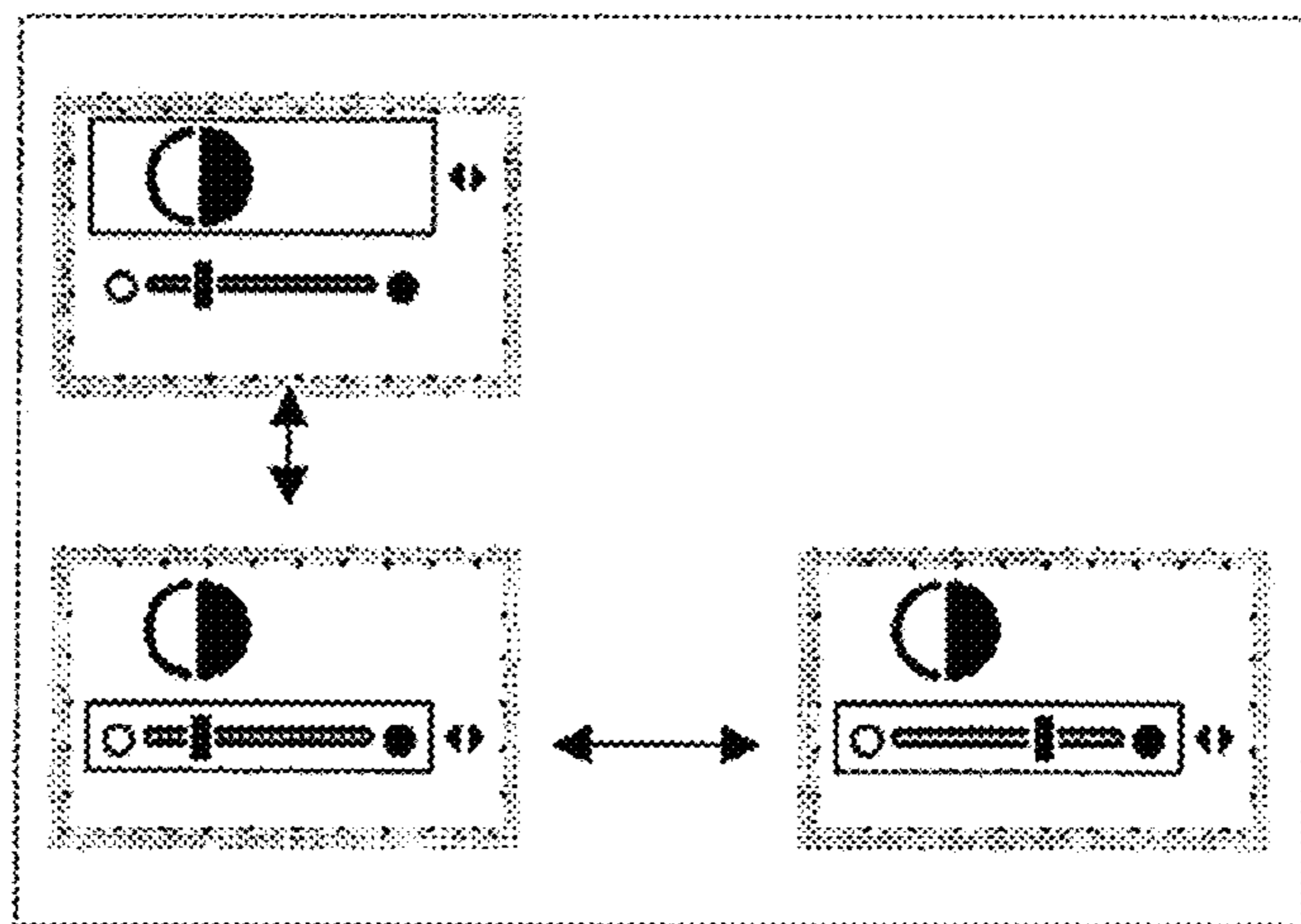
Figure 12 Contrast
