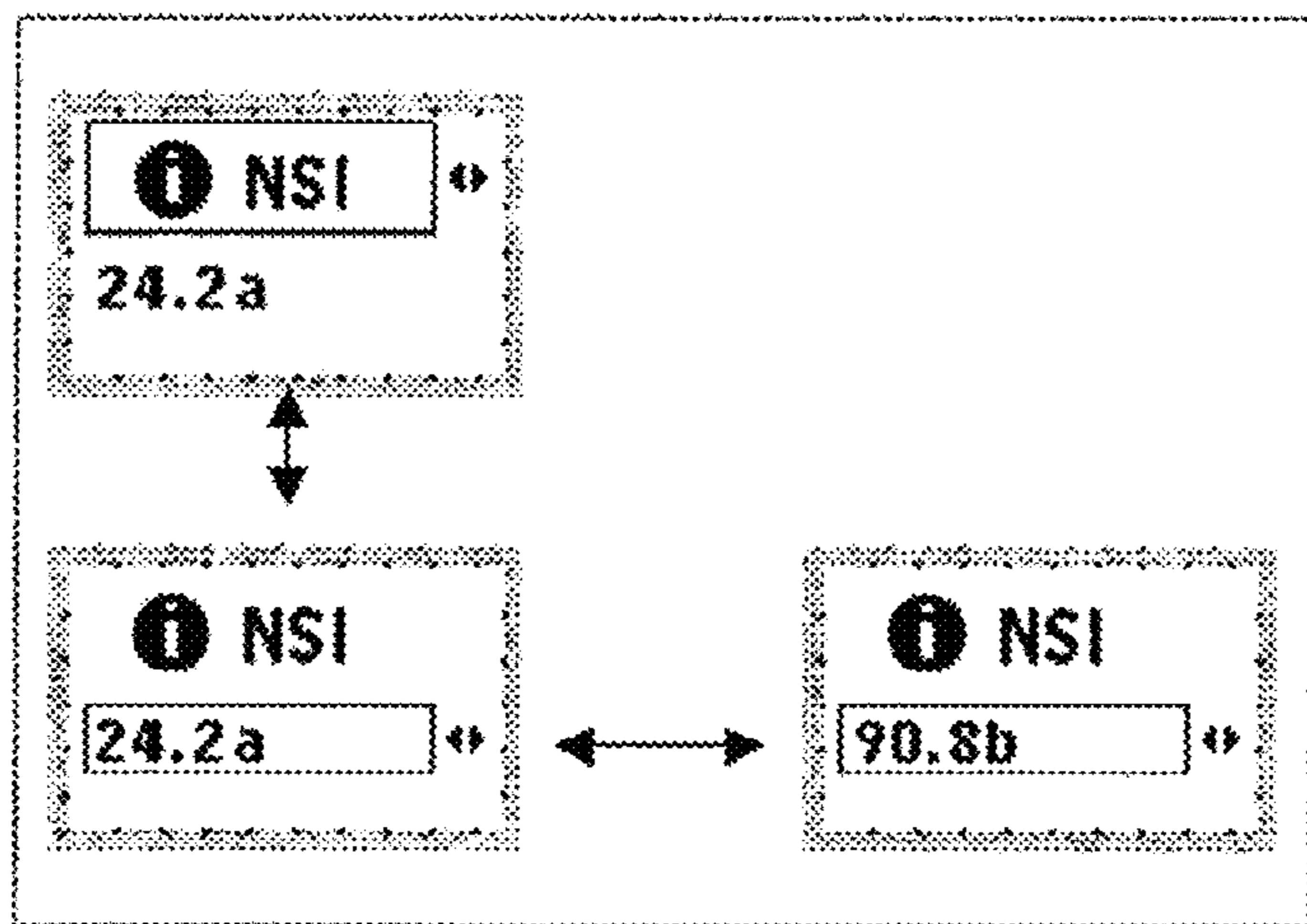
Figure 16 INS/ENS Information
