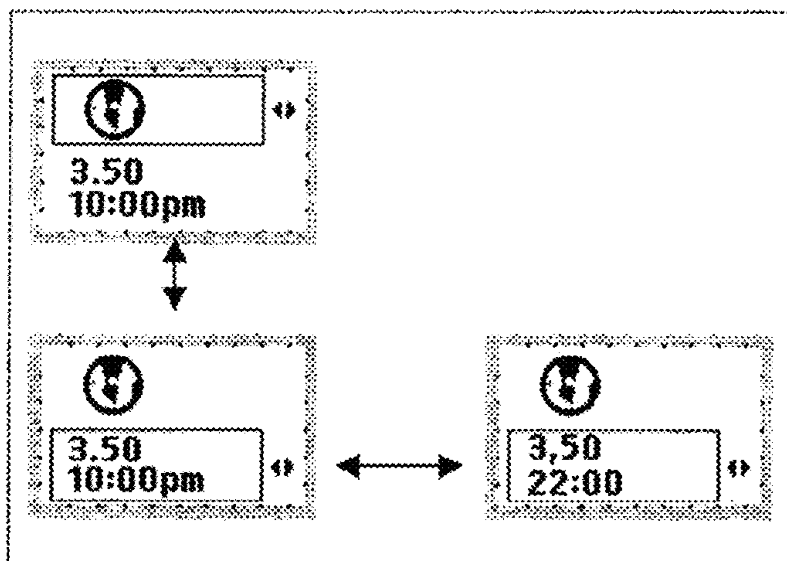
Figure 14 Time/Number Formats
