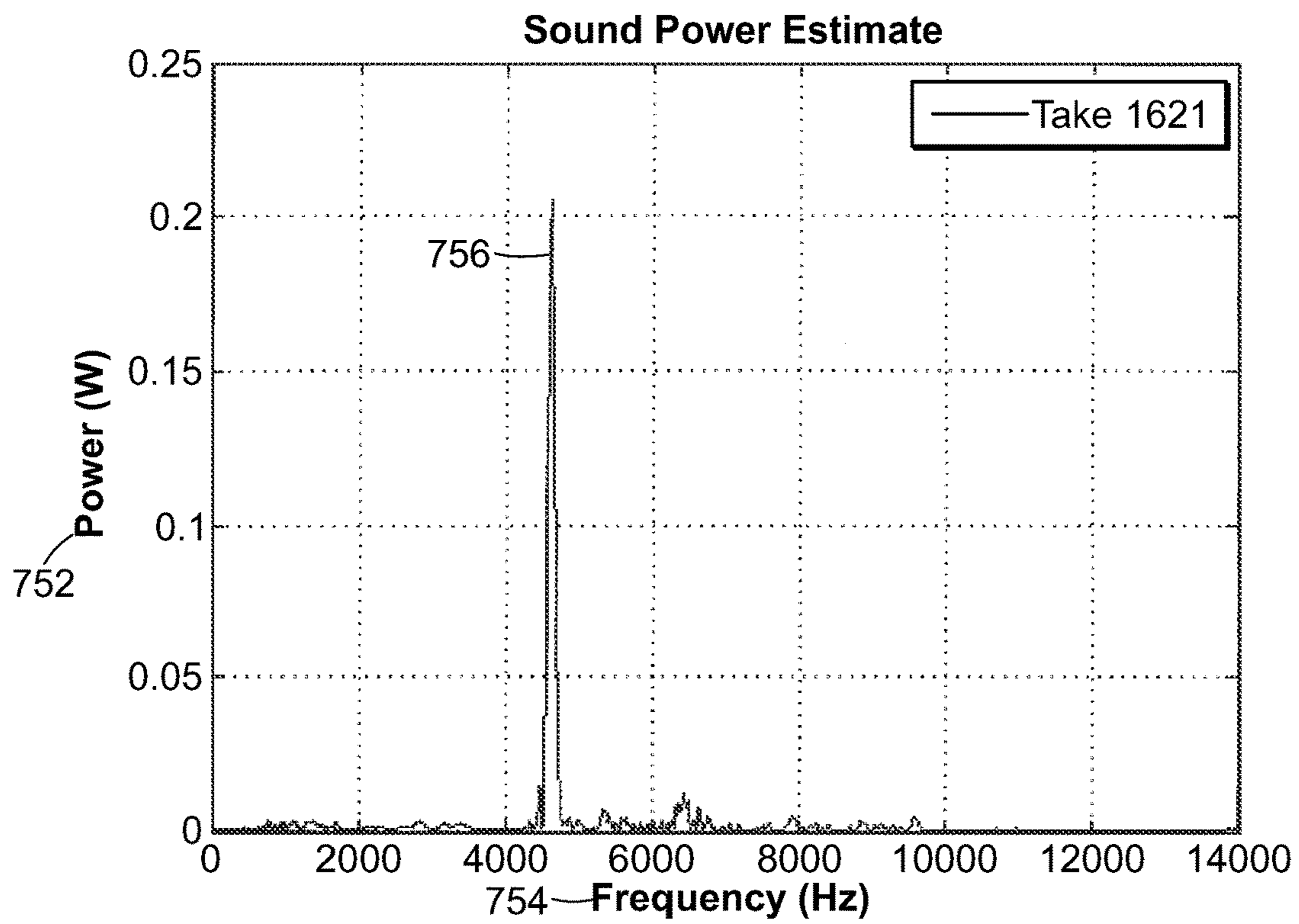
FIG. 7 (Prior Art)
