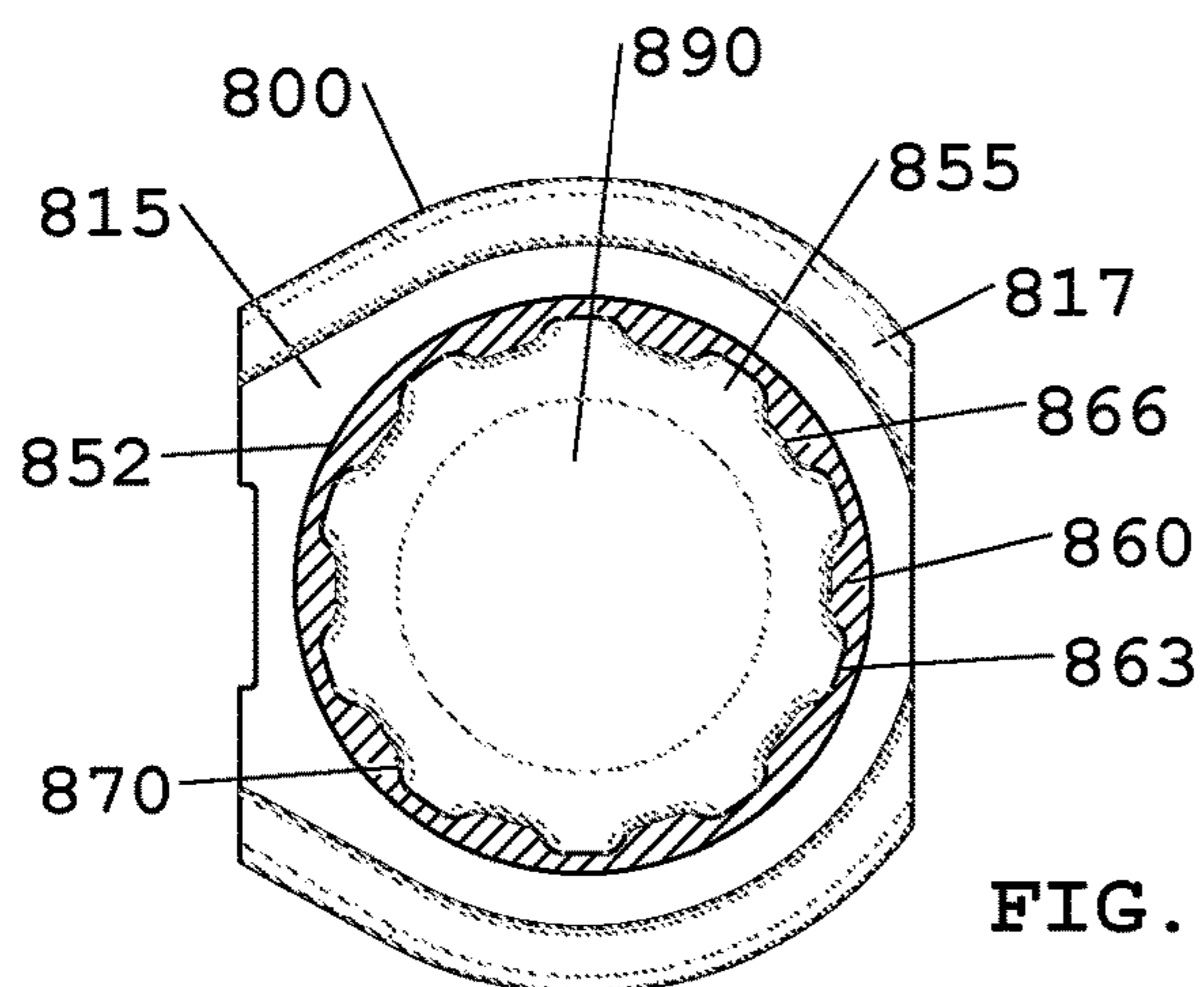
SECTION R-R
