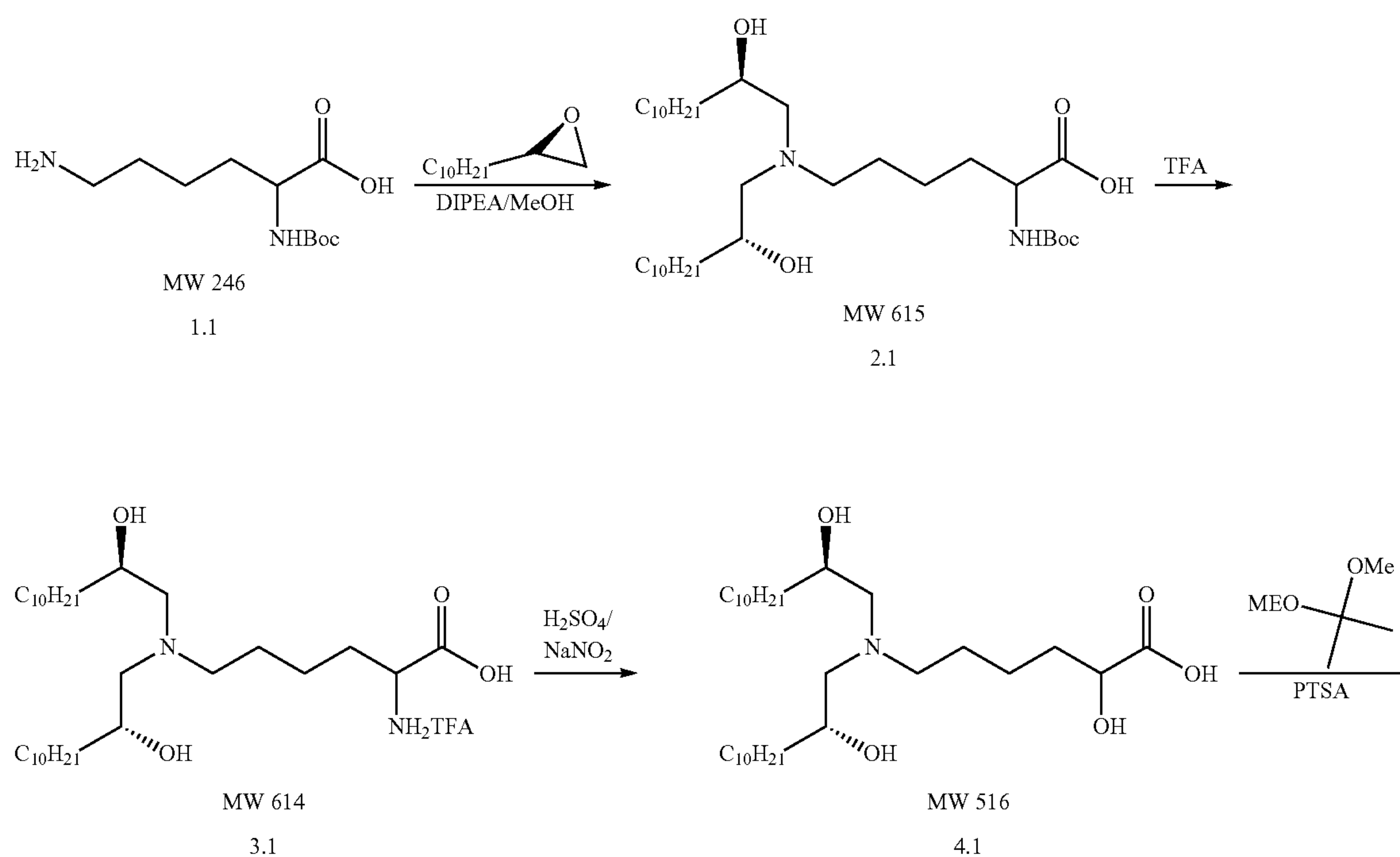
Scheme 3
