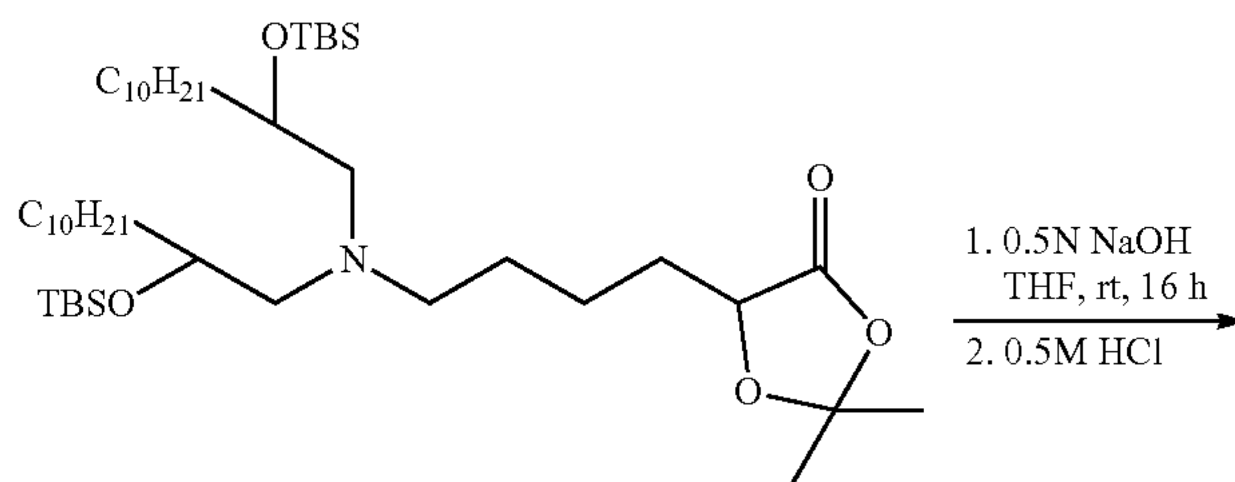
Scheme 2
